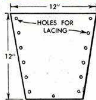
SIDE, 4 REQD.
