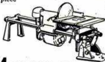
4 SHOPSMITH as a 12" Disc Sander. Adjustable mitre gauge. 14½" x 17" table tilts to 45 degrees. Discs can be removed and replaced in seconds
