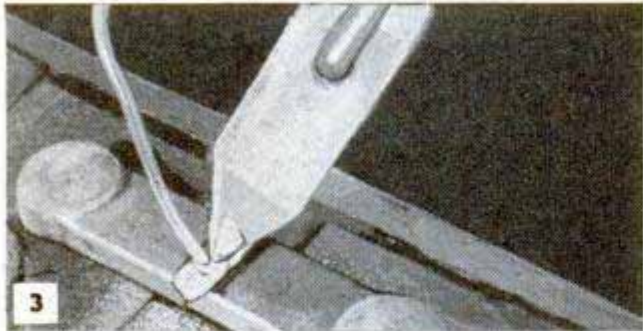
Above, soldering the cell-connector strap after cutting to remove a cell. Below, sealing a repaired cell into the battery case with a hot soldering iron
