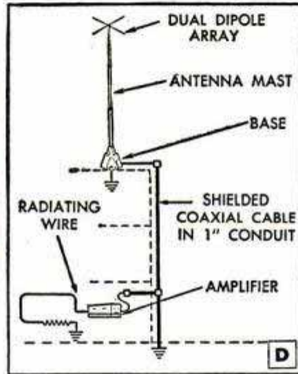
D —Puratone signal-booster system for demonstrating sets in stores located in noisy city areas. Unit covers AM, FM, short-wave bands
