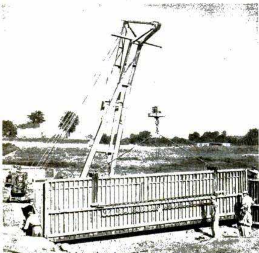
A rear-wall form is lowered into proper position on footing
