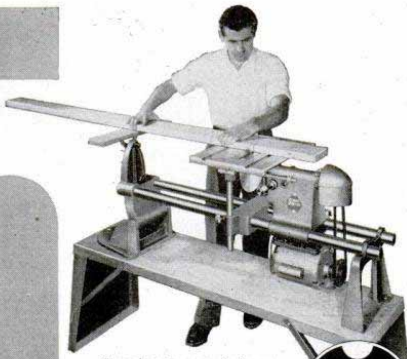
Shown here in use as circular saw, SHOPSMITH quickly converts to vertical drill press, lathe, sander and horizontal drill press
