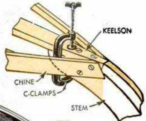
6 HOW KEELSON AND CHINES JOIN STEM
