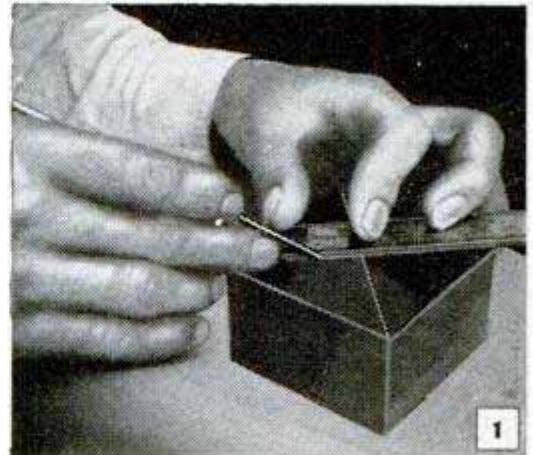
Scribing diagonal lines across corners of the tool-post turret block to locate center
