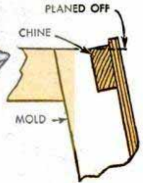
4 CHINE AND SIDE FAIRED FLUSH WITH FRAME BOTTOM
