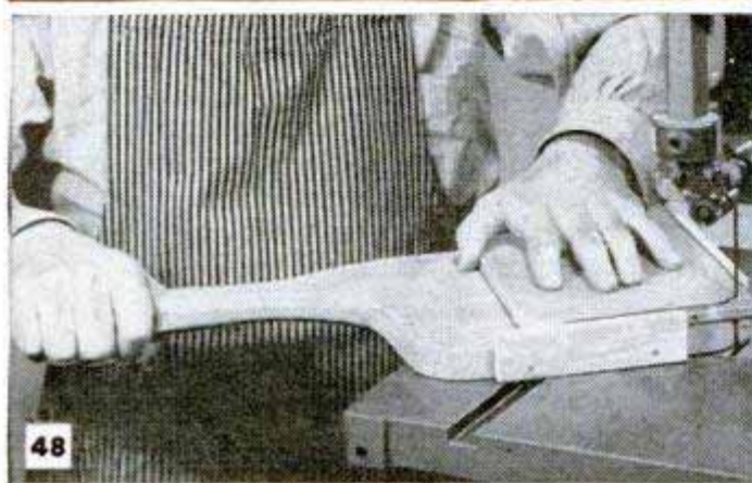
CORNER-ROUNDING JIG IS FAST . . . CUTS ONE SIZE ONLY
