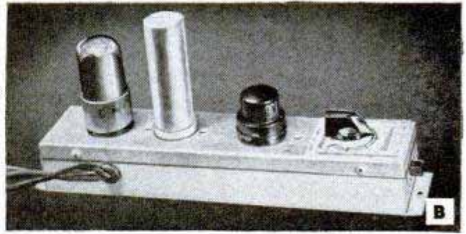
B —Compact Electro-Voice speech clipper operates directly from any high-impedance microphone into the microphone input of a conventional speech amplifier. It is a specially designed peak-limiting preamplifier that clips the tops and bottoms from speech frequencies which rise above a preset amplitude, thus providing higher articulation and intelligibility in radiophone and similar services
