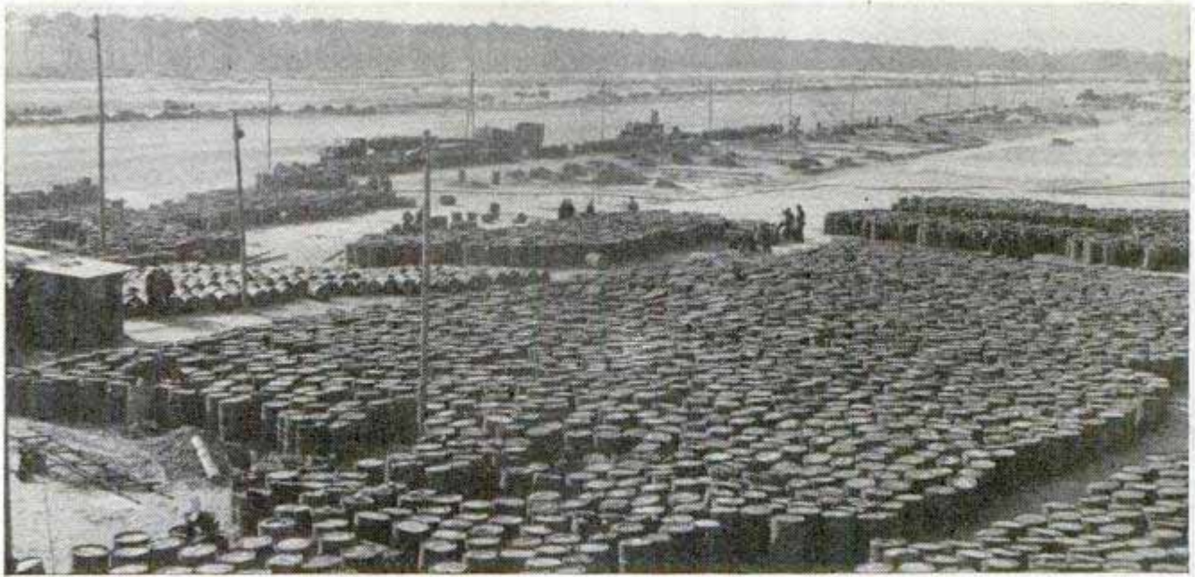
Part of 10,000 barrels of asphalt flown in to complete runway at Tegel, in the French sector. Bulky construction equipment was cut in two by blowtorches, shipped in on C-82s, and welded back together on arrival
