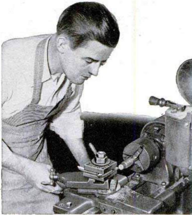
Scribing diagonal lines across corners of the tool-post turret block to locate center
