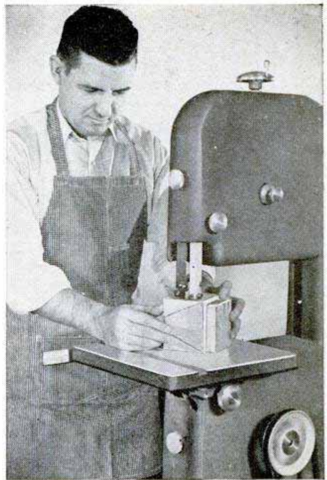
A bandsaw will speed the work of sawing the tapered feet. After two cuts are made, the waste pieces are tacked back on with cardboard between the joint to provide a flat surface for making the other two cuts
