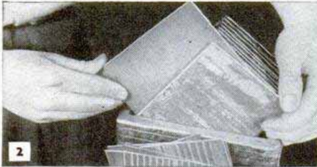
Replacing cracked or warped separators with new ones restores defective battery cell to continued use. Support the cell at an angle in the case as shown
