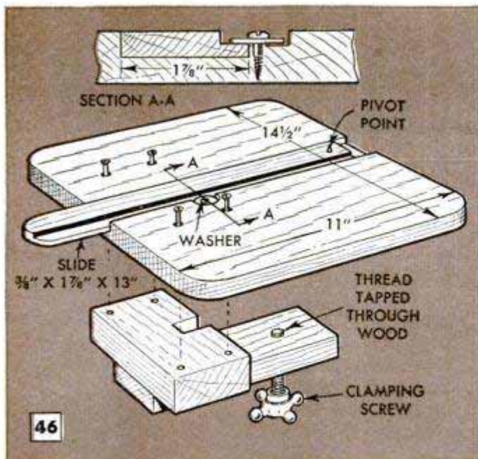
CIRCLE-CUTTING JIG DOES PERFECT WORK, ANY DIAMETER
