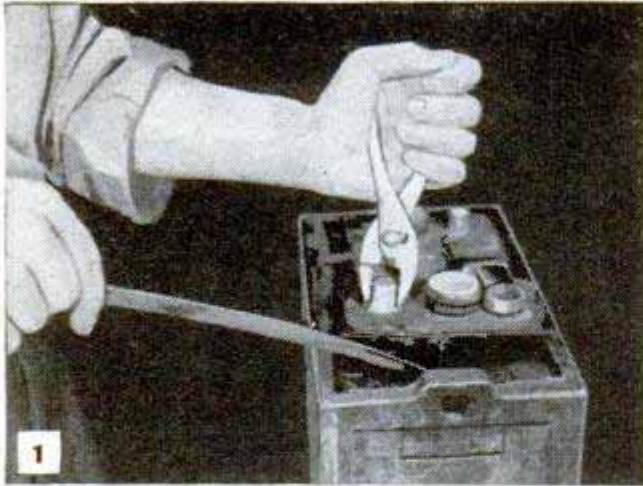
Softening sealing compound with a heated screwdriver will free the cell so that it is easily removed. Be careful not to spill acid solution in the case
