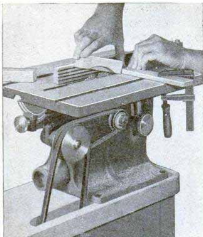
Finger grips in the drawer handles are formed by bringing the work down over the saw blade repeatedly. A block clamped to the table serves as a stop
