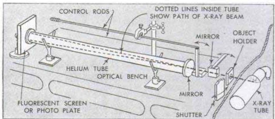
Top, long control rod is used to adjust microscope mirrors while examining X-ray image through eyepiece. Left, X-ray microscope photo of wire gauze with 250 meshes to inch; right, sketch shows how instrument works
