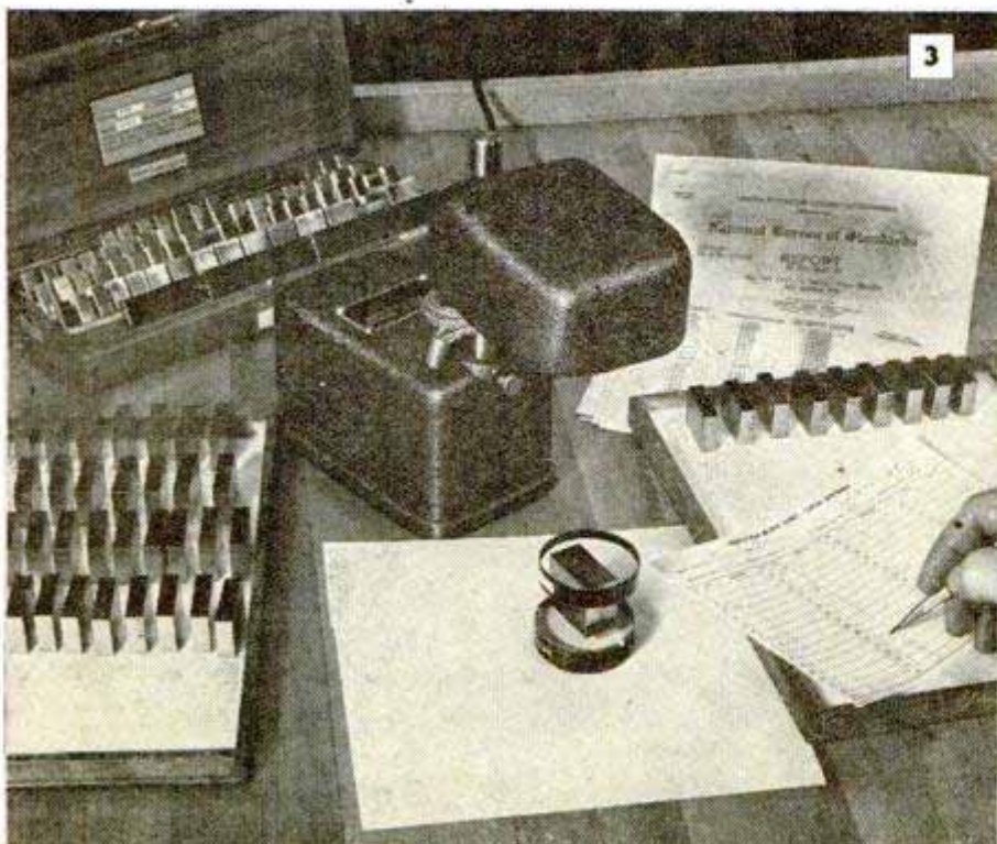
Left, a completed gauge block being tested alongside the master block between optical flats. Above, testing diameter of ball bearing by same system. Lines on block check diameter
