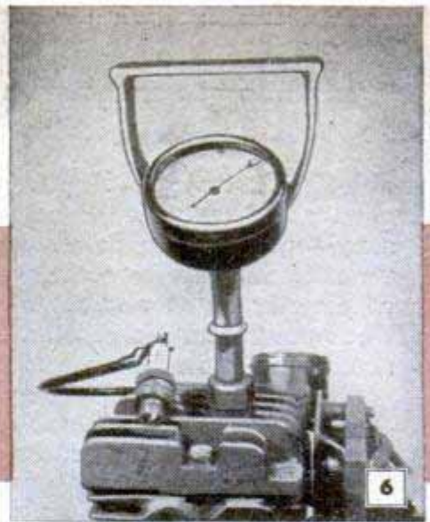
Before disassembling an engine, check compression with a dial gauge such as shown above. It gives a true reading
