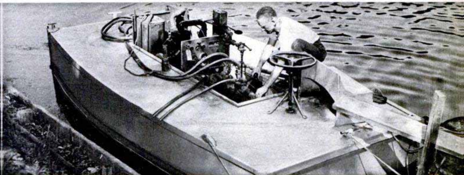
Mounted amidships in the plywood hull is the pumping unit which consists of a 90-hp. gasoline engine and a 500-gallon-per-minute pump. The propulsion nozzle is under the steering wheel at the near end of the boat
