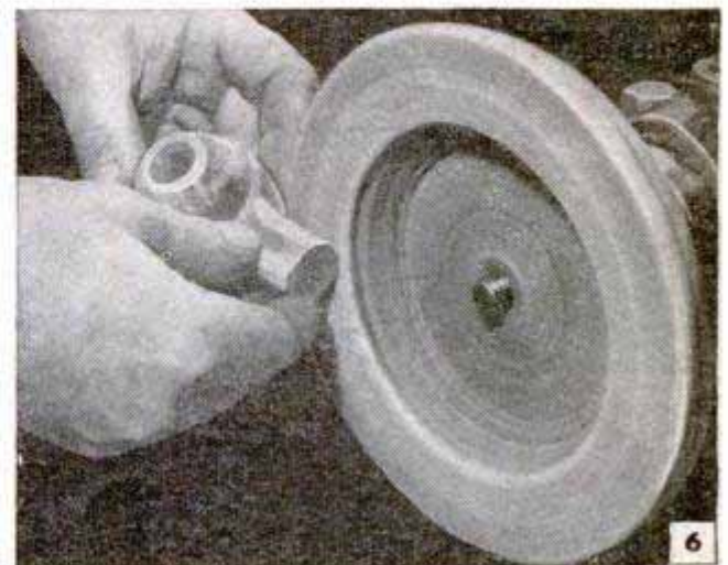
Final shaping of bowl and shank is done on a recessed abrasive disk made especially for the purpose.
