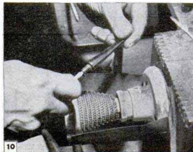
If pusher fits too loosely, expand it by holding the bit over heat and inserting taper pin in the air hole
