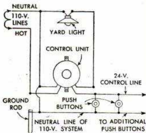
HOOKUP DIAGRAM
