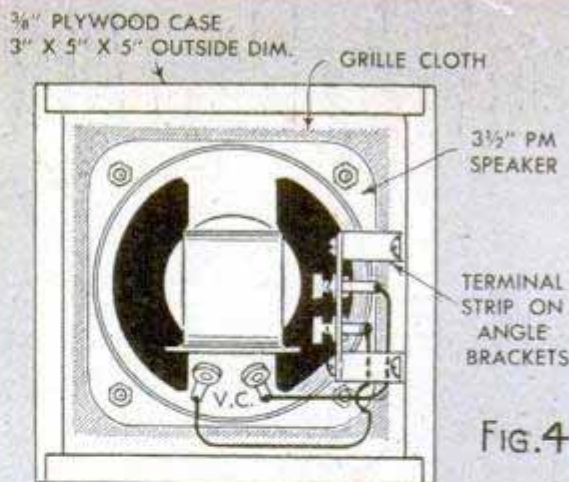
REMOTE SPEAKERS NO. 2 AND NO. 3 (2 REQD.)
