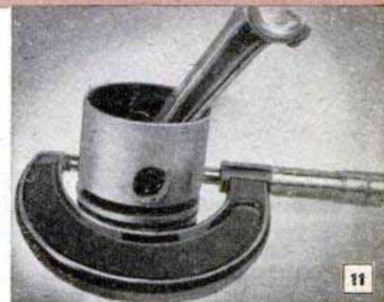
When checking piston diameter, always place the mike at right angles to the wrist pin
