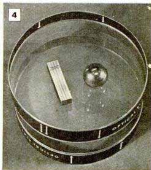
Left, a completed gauge block being tested alongside the master block between optical flats. Above, testing diameter of ball bearing by same system. Lines on block check diameter
