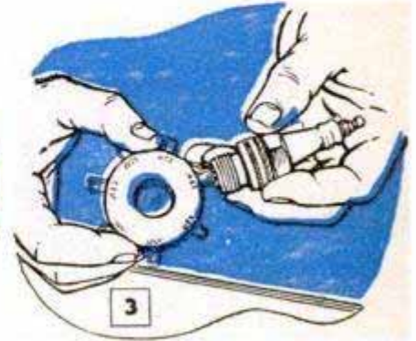
Check the electrode gap with a wire gauge made for the purpose
