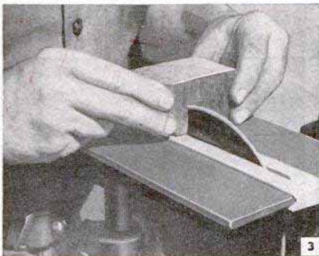
Next, the rough blank is sawed to shape with a circular saw. Be sure to allow stock for finish-sanding.
