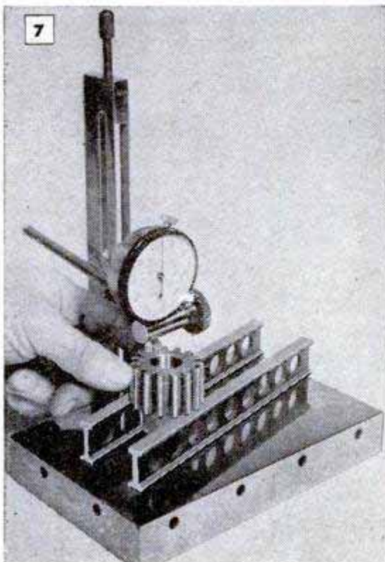
Left, checking spur gear with dial gauge. Right, this gauge gives several bore measurements simultaneously
