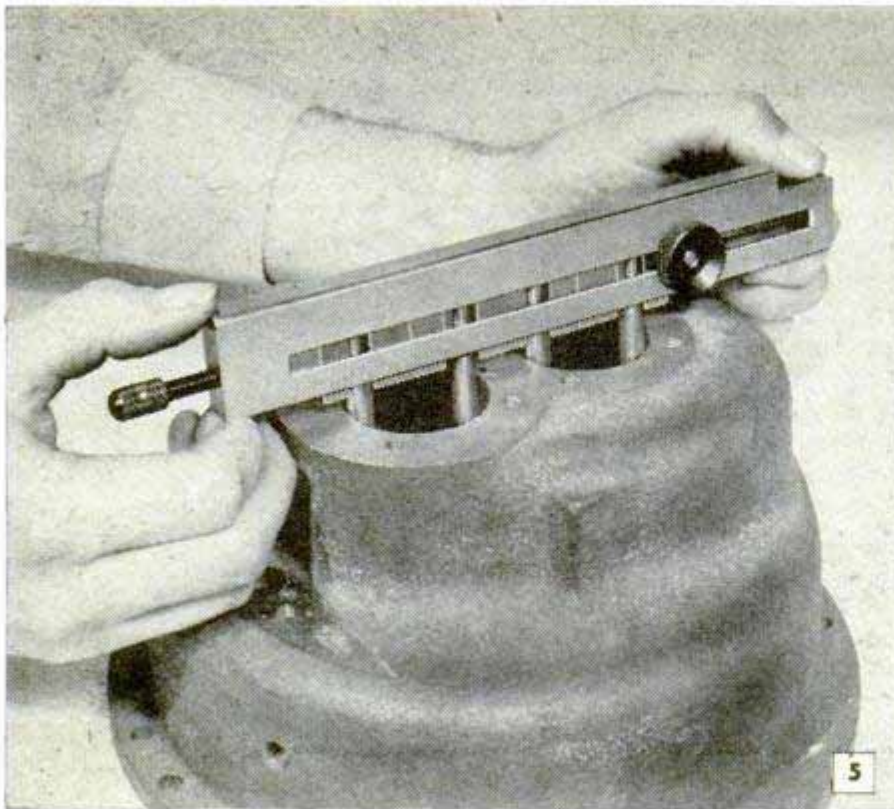
Blocks are inserted in a holder to make a gauge to measure internal diameters in production
