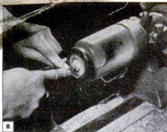
Counterboring the shank to form the air hole and the pusher hole. Pusher hole must be of exact diameter
