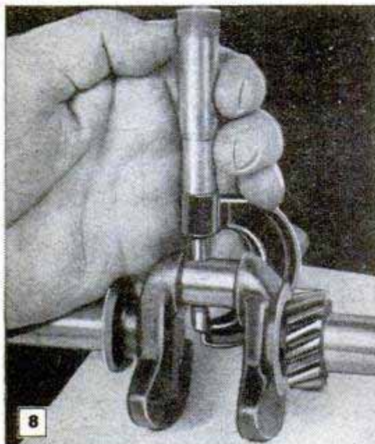
Above, check and double check valve clearances with a feeler gauge. Below, whenever engine is disassembled measure the crankpin
