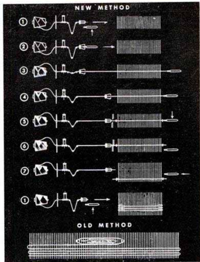
Top, tiny, new shuttle compared with old. Right, the new and old weaving systems. Below, sketch of new shuttle action with enlarged drawing of shuttle and scissors
