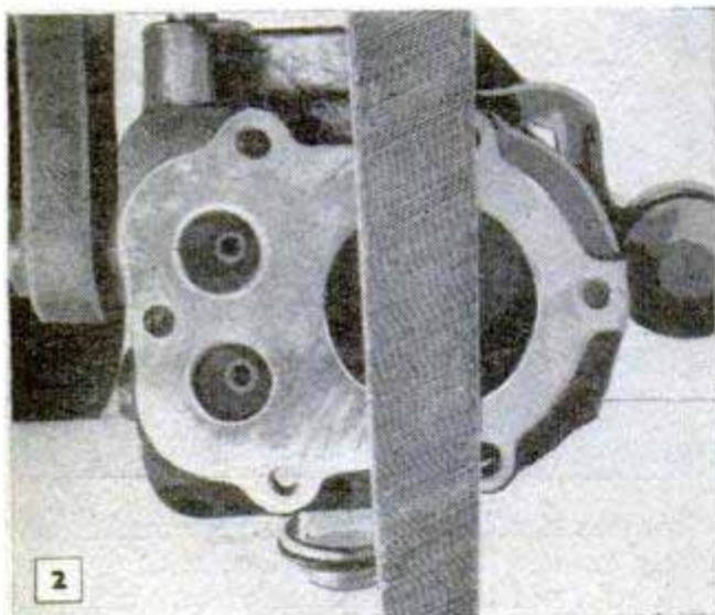
Distorted areas, due to head bolts drawn too tightly, can be located by passing a file lightly over the head flange. Careful filing removes the high places
