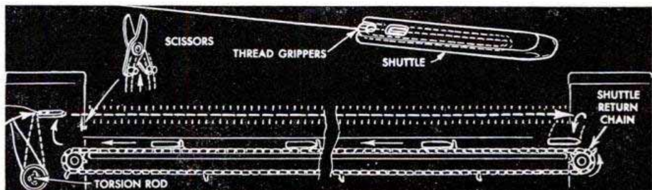
Top, tiny, new shuttle compared with old. Right, the new and old weaving systems. Below, sketch of new shuttle action with enlarged drawing of shuttle and scissors
