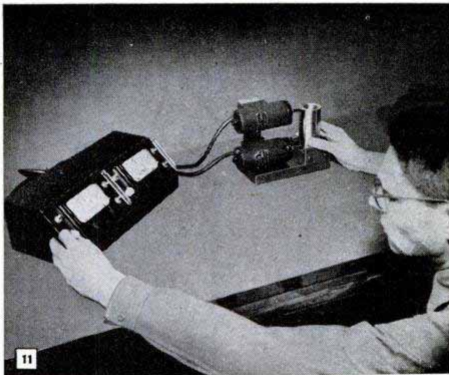
This electromagnetic comparator works the same way as a phonograph pickup arm. Its sensitive needle reacts to infinitesimal amounts of pressure
