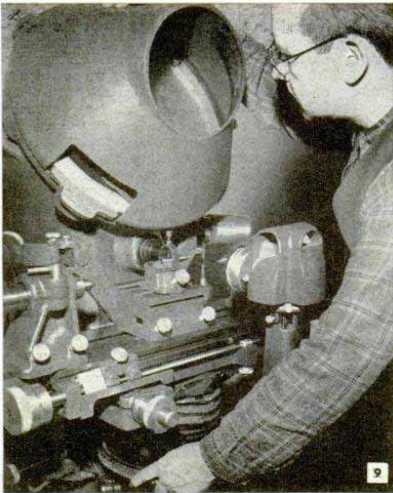
Optical comparator projects magnified image of part on screen
