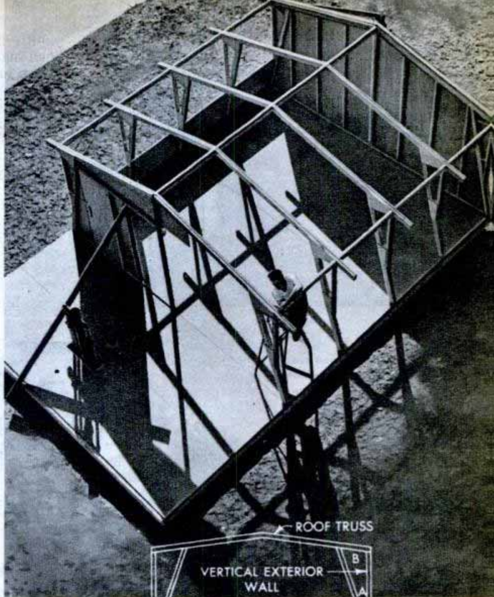
Right, with one of the end walls and part of an interior partition in place, the builder assembles the roof trusses
