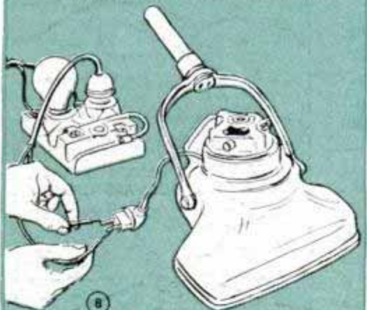
8 A TEST LAMP IS USED TO CHECK FOR "OPEN" CIRCUIT IN FIELD OR ARMATURE COILS
