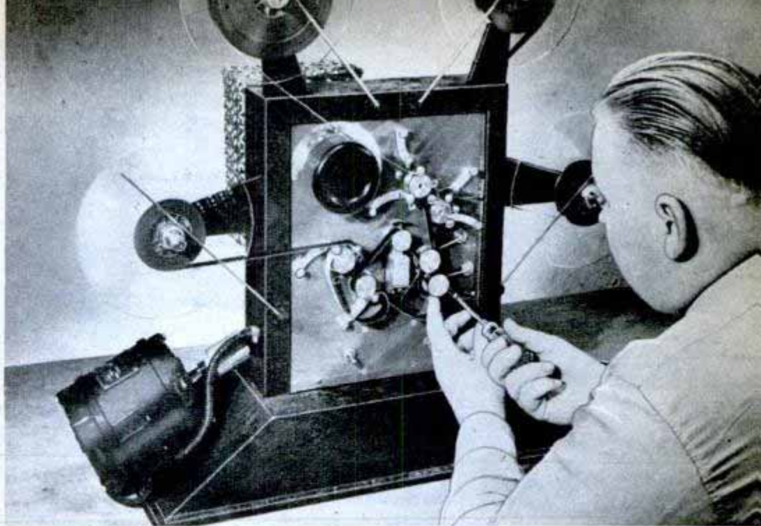
Electrically driven precision sound printer puts the reversed sound track on a 16-mm. color film. Printer's reels are made of transparent plastic
