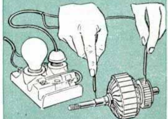
13 LIGHT HERE INDICATES THE ARMATURE COIL IS GROUND TO THE SHAFT
