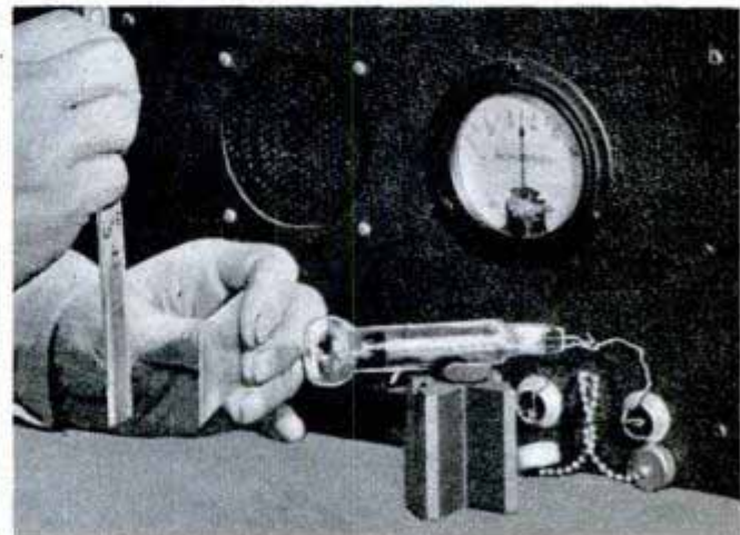
Thin brass sheet halts less penetrating beta radiation
