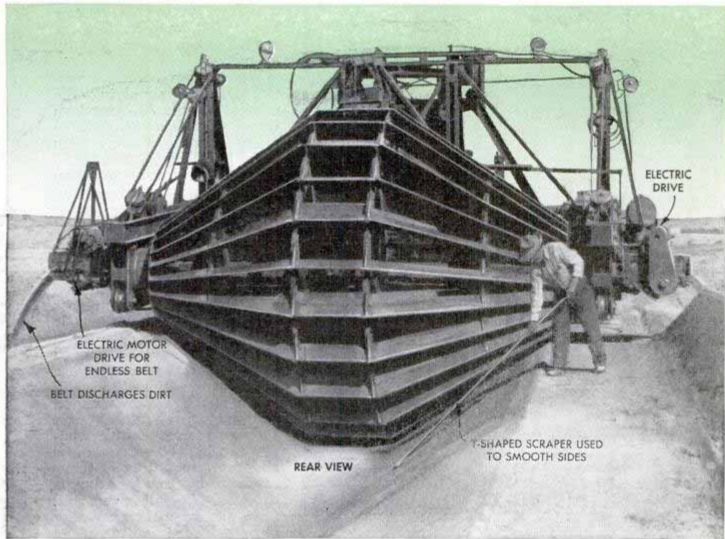
With mathematical precision the "paddle-wheel" digger carves out a canal at the rate of one foot per minute
