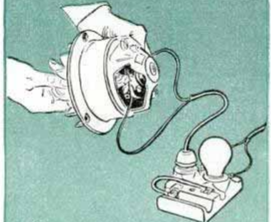
12 TURN FAN SLOWLY TO CHECK ARMATURE COILS FOR "OPEN" CIRCUIT
