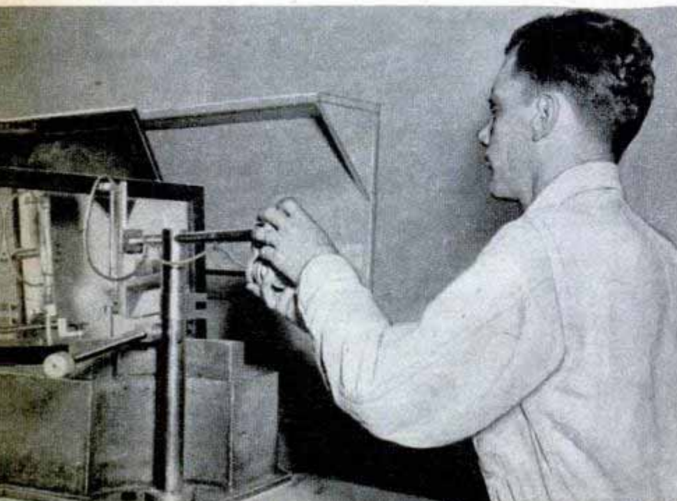
Remote control device measures out tiny portions of radioactive products in solution. Sample, shielded by lead, is viewed in mirror
