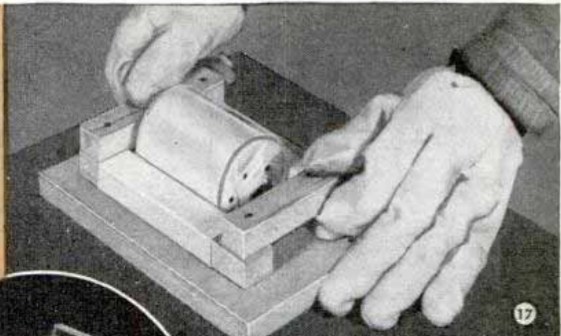
RING METHOD OF FORMING HALF CYLINDER
