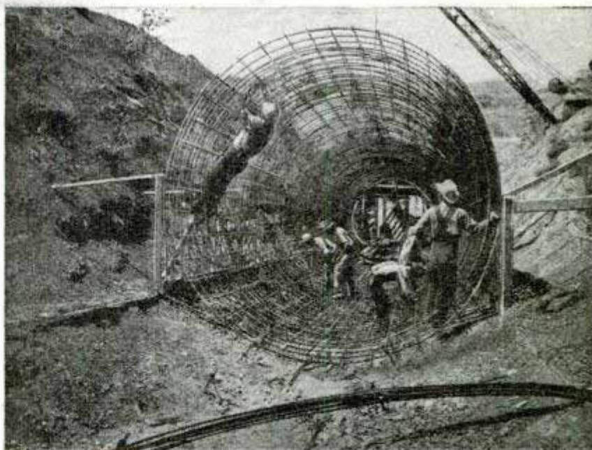
↑ Steel reinforcing bars are installed to hold concrete for siphons to carry the big Conchas irrigation canal across the bed of a stream
