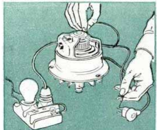
11 LIGHT SHOWS THIS FIELD COIL IS CONTINUOUS ALTHOUGH IT MAY BE SHORTED
