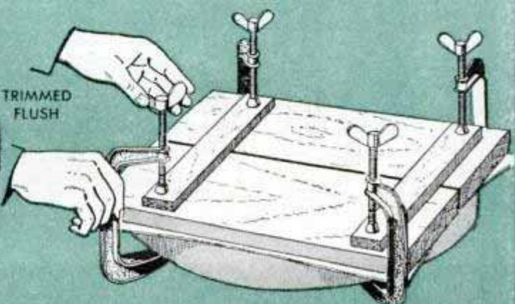
AFTER WHICH TOP IS VENEERED AND TRIMMED
