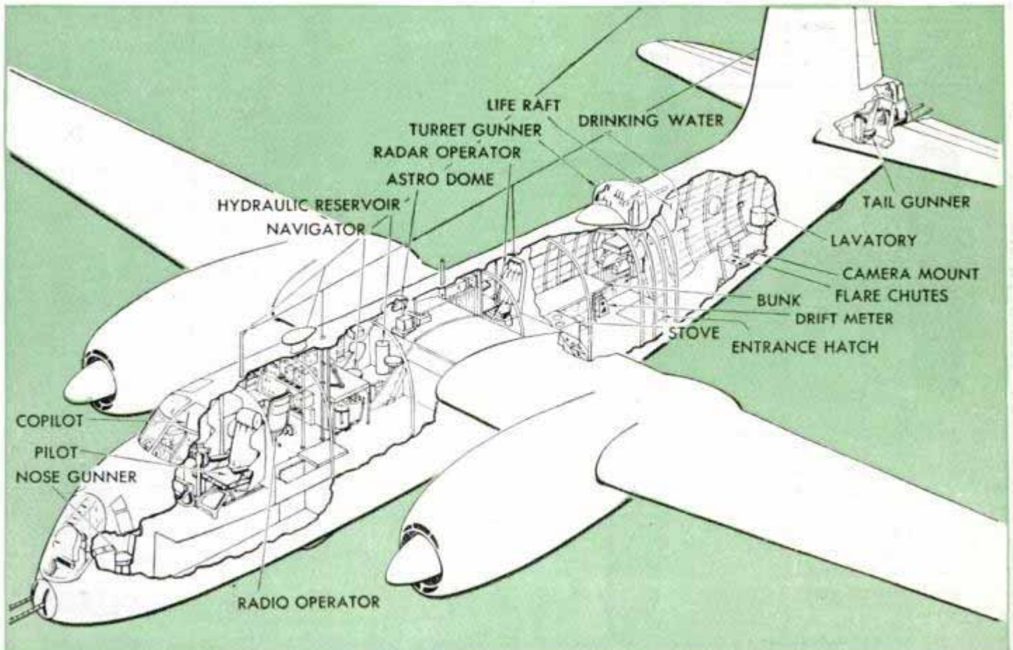
Cutaway diagram of crew stations in combat version of the Lockheed P2V Neptune. Its wing span is 100 feet and length 75 feet 6 inches. Its height of 28 feet 1 inch is equivalent to that of a three-story building
