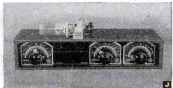
(G) Plastic stand-off insulator for 300-ohm twin-lead transmission line keeps line at fixed distance from any surface. (H) Shockproof plastic radio pliers. (J) Absorption wave meters available in many ranges. These handy frequency meters can be poked into small shield compartments, coil stages and corners to check harmonics and for similar applications, thus enabling the experimenter to find out exactly what is "going on" in the circuit
