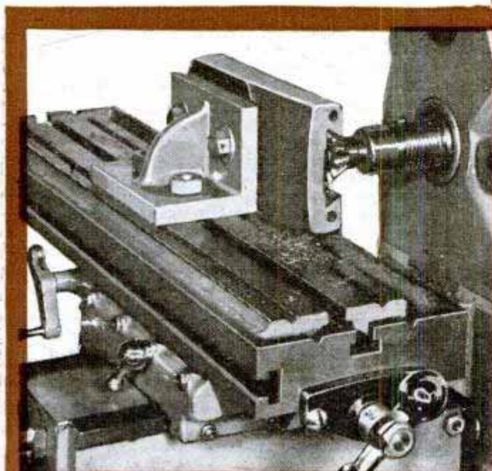
12 ANGULAR MILL CUTTING FEMALE HALF OF DOVETAIL
