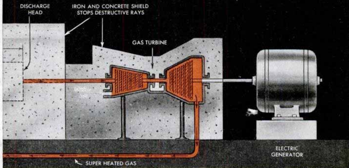
Artist's conception of a 200,000-horsepower atomic power plant for a battleship. It would weigh 500 tons but would require less space than today's engines. Ship could stay at sea for long periods without refueling
