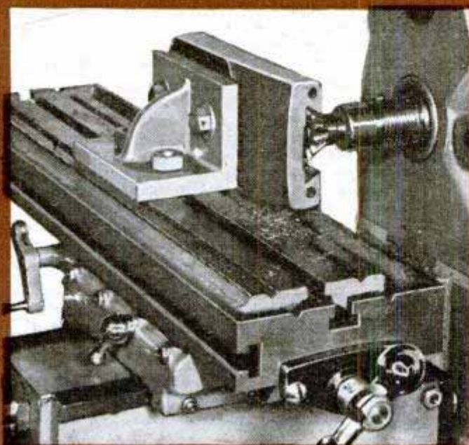
12 ANGULAR MILL CUTTING FEMALE HALF OF DOVETAIL
