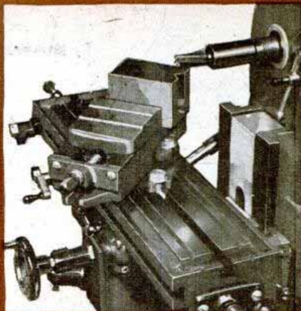
9 END MILL CUTTING VEE IN WORK SET AT 45 DEGREES
