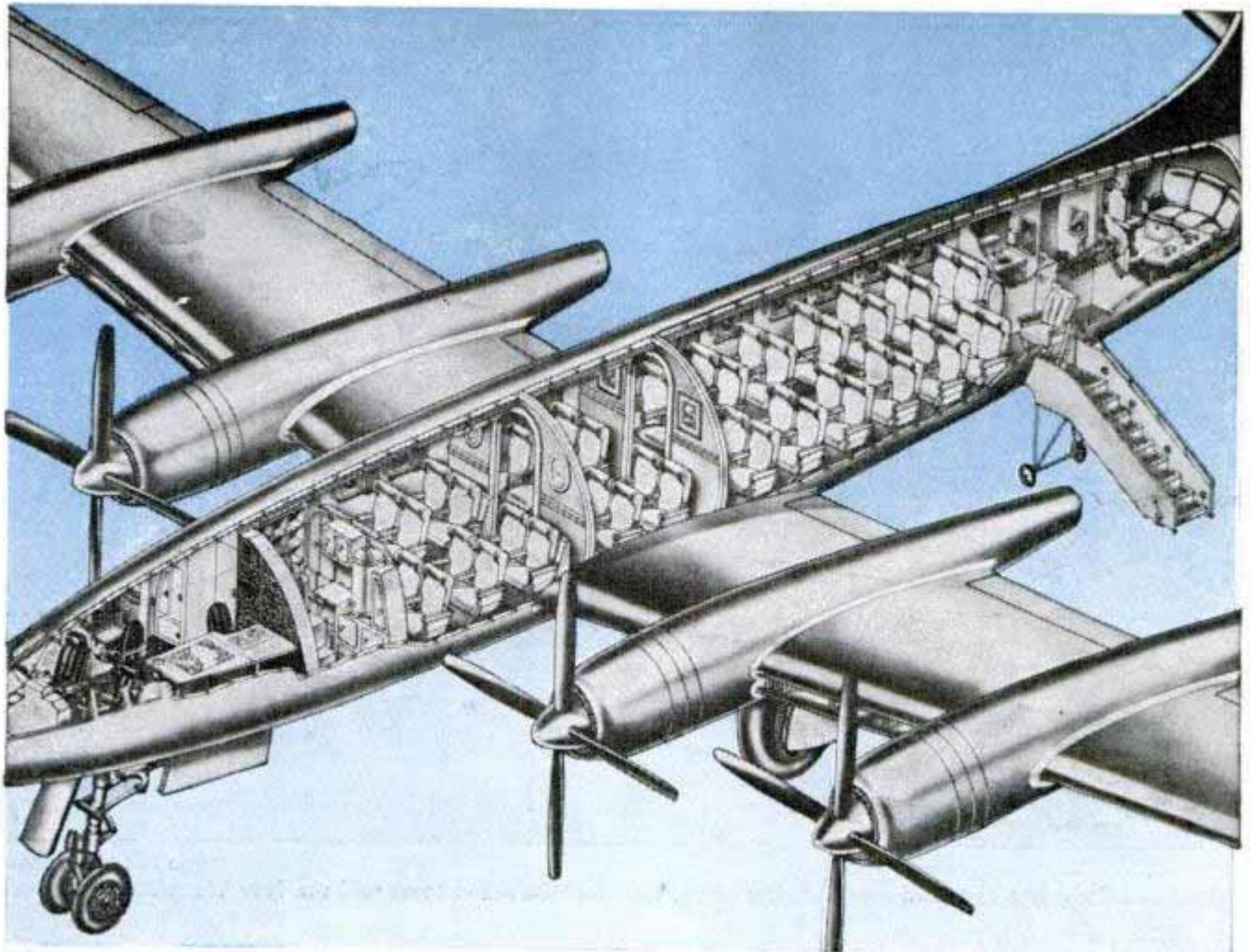
Sectioned view of the Rainbow (above) shows three passenger compartments, galley and a lounge in the tail Republic Aircraft photo
