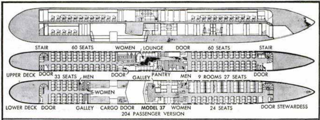
Sectioned view of the Rainbow (above) shows three passenger compartments, galley and a lounge in the tail Republic Aircraft photo
