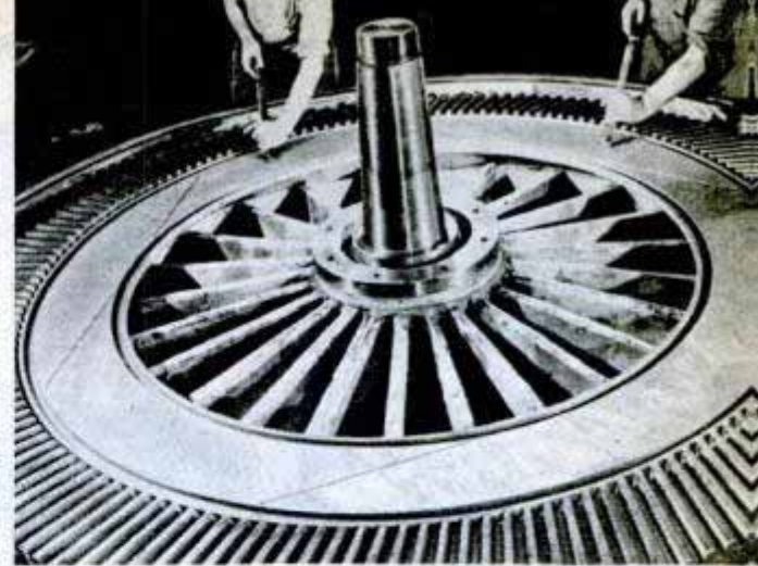
TURNTABLE aids in polishing huge bearings used in giant generators. Westinghouse workers grind the "doughnuts" with abrasives, then rub with hands
