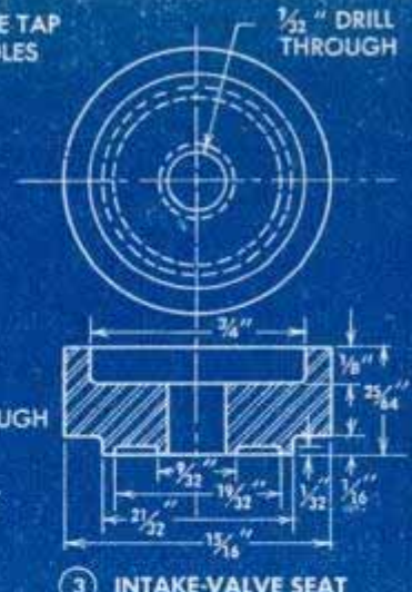
③ INTAKE-VALVE SEAT
