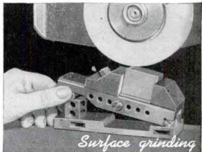
With the aid of precision gauge blocks any angle can be set up within plus or minus 5 minutes of a degree
