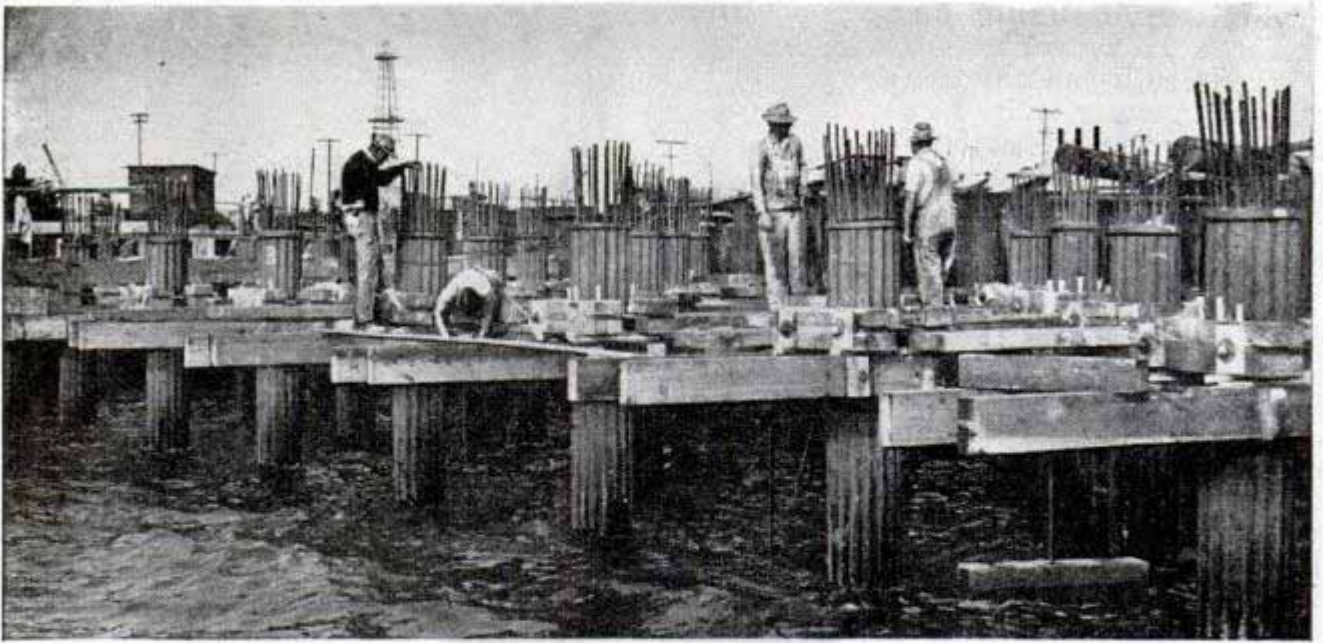
Reinforcing rods for pier are placed in tubular piles that sink deep into the earth 40 feet beneath water surface
