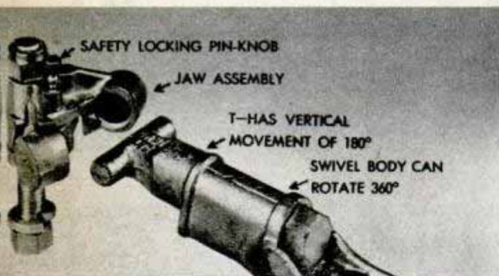
TRAILER HITCH has a universal joint which prevents overturning by providing swivel in all directions
