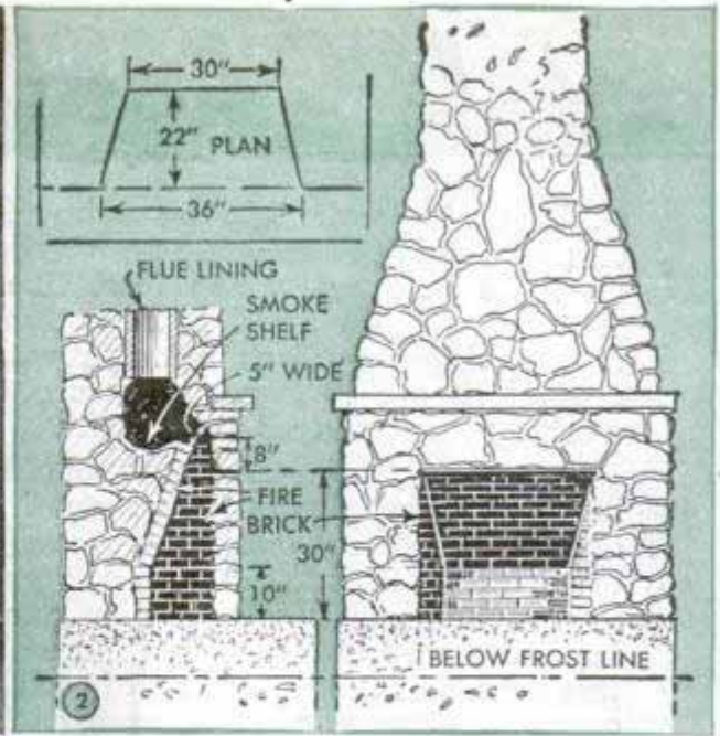
Properly made, a fireplace can give both atmosphere and comfort. Structural details above at the right show the proper throat construction to give maximum efficiency. The dimensions should be followed quite closely
