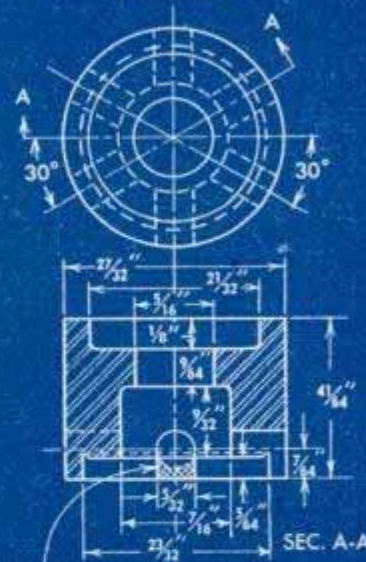
④ INTAKE-VALVE RETAINER
