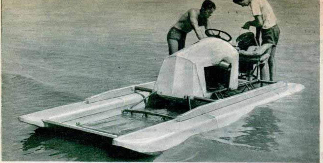
Ideal boat for towing water skiers on quiet lakes is this pontoon rig made of automobile gasoline tanks
