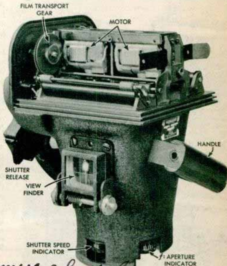
Sharp action shots are assured with the Navy-modified K-20 camera (above) and the K-25 shown below with cover removed
