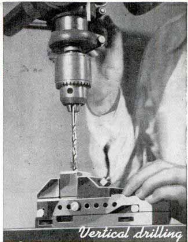
Here the sine bar vise is being used as an ordinary drill vise to hold work for a common drilling operation
