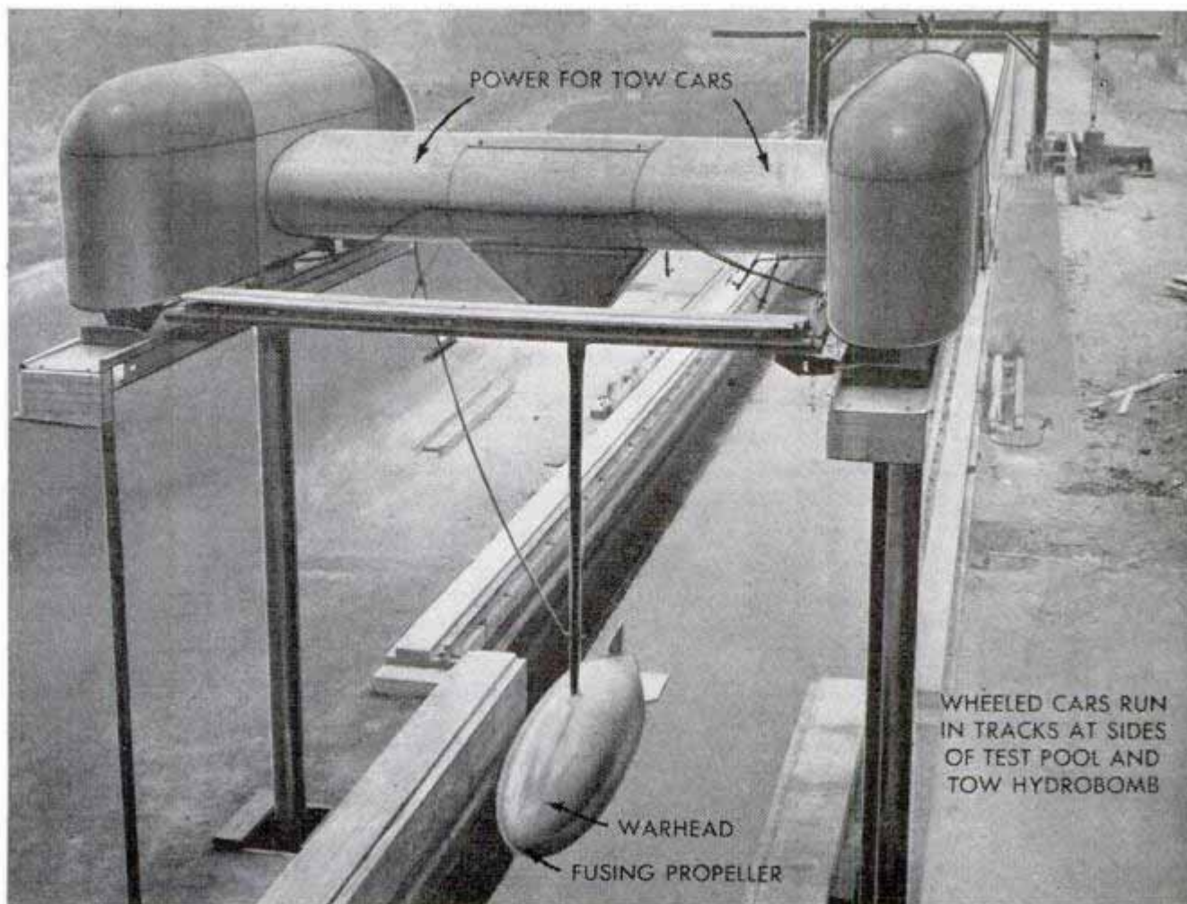
Hydrobomb tests are made in this 500-foot tank with underwater observation windows. The electric-powered tow car is lowered to the tracks at either side of the tank, completely straddling it when in operation. Still experimental, this plane-borne supertorpedo can carry a heavier charge twice as fast as current types
