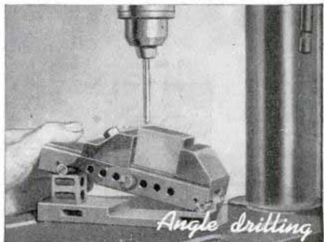
Angle setup for drilling on an ordinary drill press. Drill must be properly ground to prevent drifting
