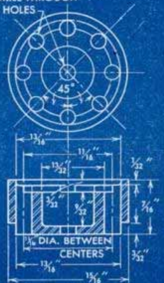
④ INTAKE-VALVE RETAINER
