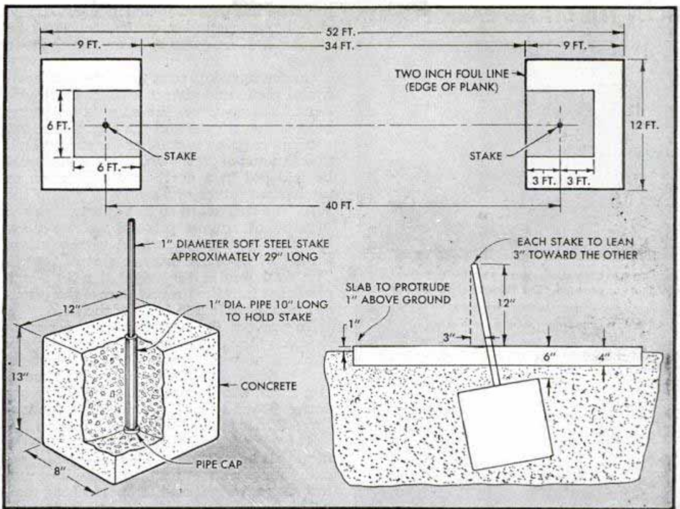
Drawing from National Horseshoe Pitchers Association of America Here are dimensions for building your own horseshoe court. The equipment and materials are inexpensive
