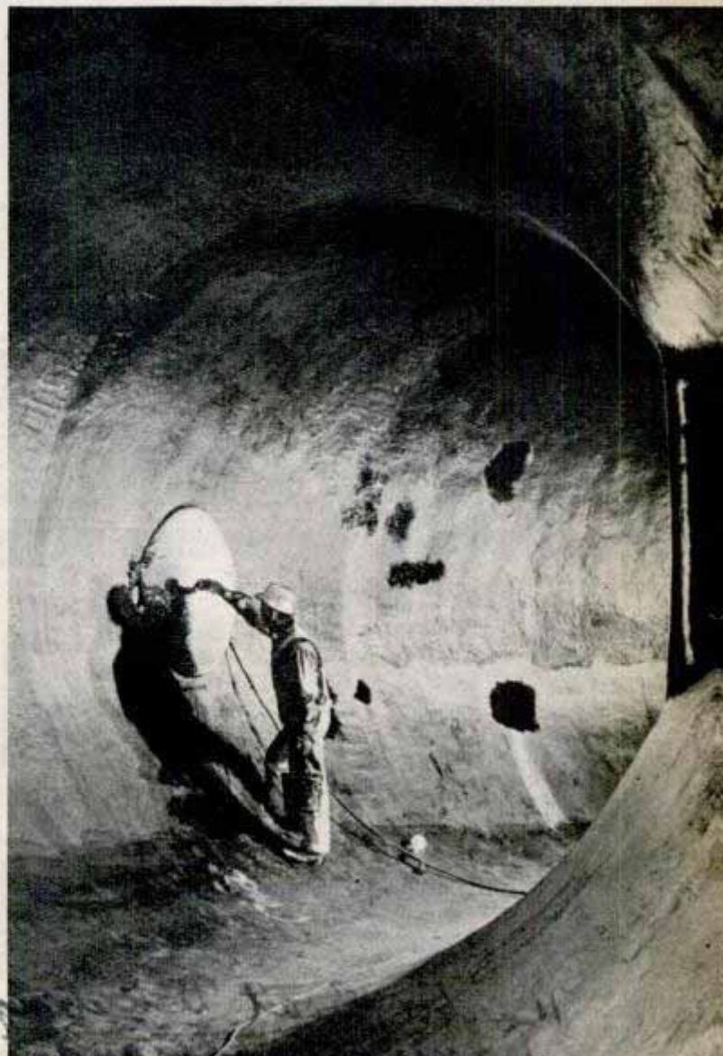
Cliff where power drills, above, opened pumping tunnels is now under water. Right, view inside the steel case surrounding one of the hydroelectric power units
