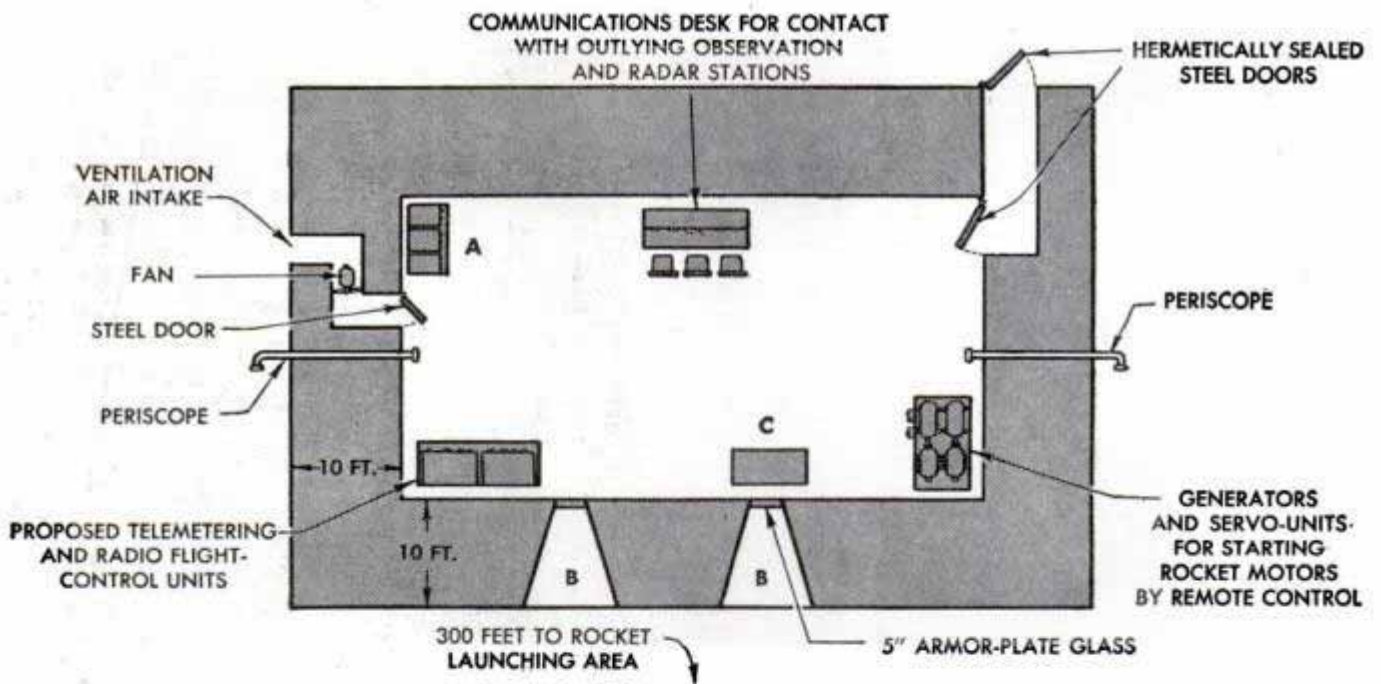
A Apparatus to establish time base for all stations observing rocket's flight in trial
