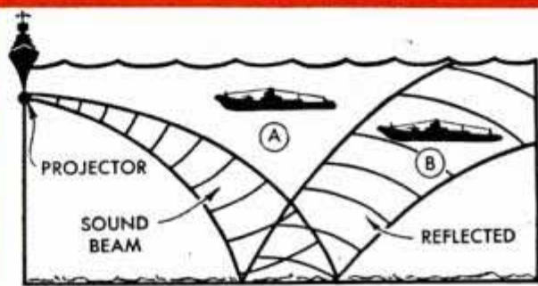
Here sound beam has hit bottom and reflected upward, catching sub B; sub A is in dead spot
