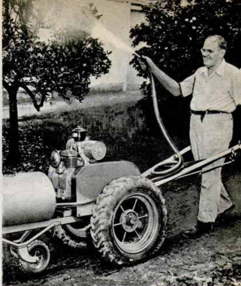
POWER SPRAY attached to garden tractor combats insects on trees and plants, develops 300-lb. pressure
