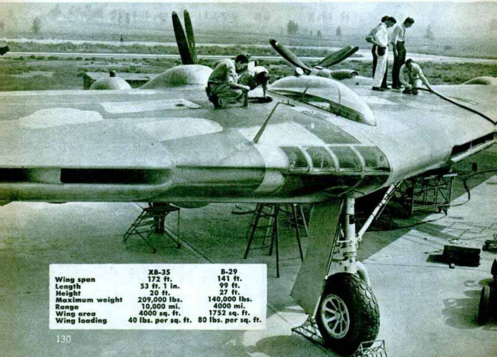
Close-up of the nose shows long blister used by pilot and the broad window area for copilot and bombardier
