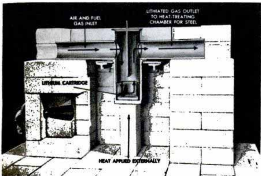
Protective blanket of gas from lithium generator shown in cross-section guards heated steel parts from ravages of oxygen and water vapor. Below, pound of lithium hydride makes 40 cubic feet of gas to lift the aerial Photo below by Lithalloys Corp.
