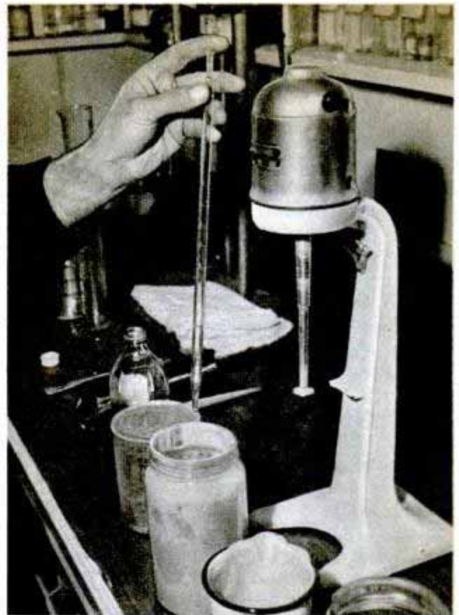
Colloidal material picked up in the underground bore has thickened this mud (left). The mud engineer can reduce its viscosity by adding a few drops of complex or poly phosphates to the sample as shown at right
