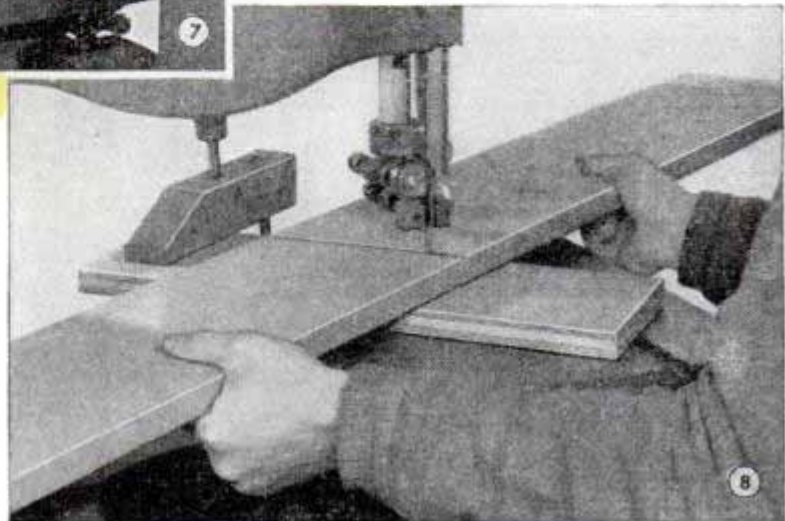
Fig. 8 shows this setup being used to cut a 6-in.-wide board in one pass.
