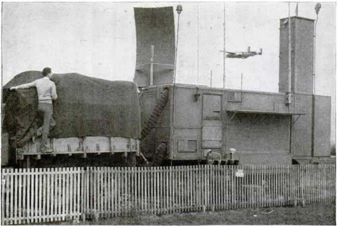
Truck and trailer, with search antenna assembly in upper center and elevation antenna housing at upper right
