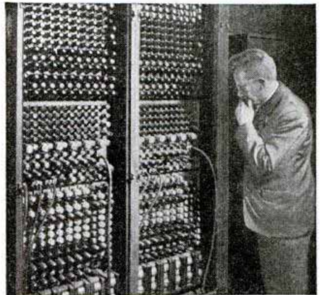
Getting ENIAC ready for operation, top. Above, rear view of section of machine showing tubes, plug-in chassis and transformers. Below, overall view of ENIAC being prepared to solve mathematical problem
