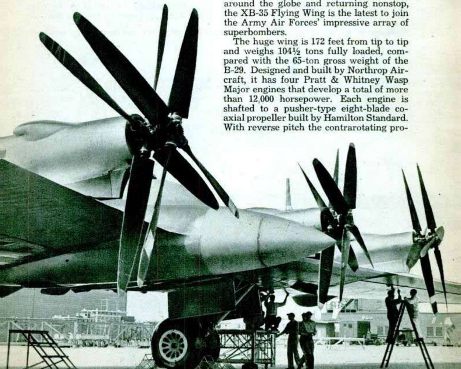
Side and rear views of 104½-ton XB-35. Diameter of the contrarotating propeller is 15 feet four inches
