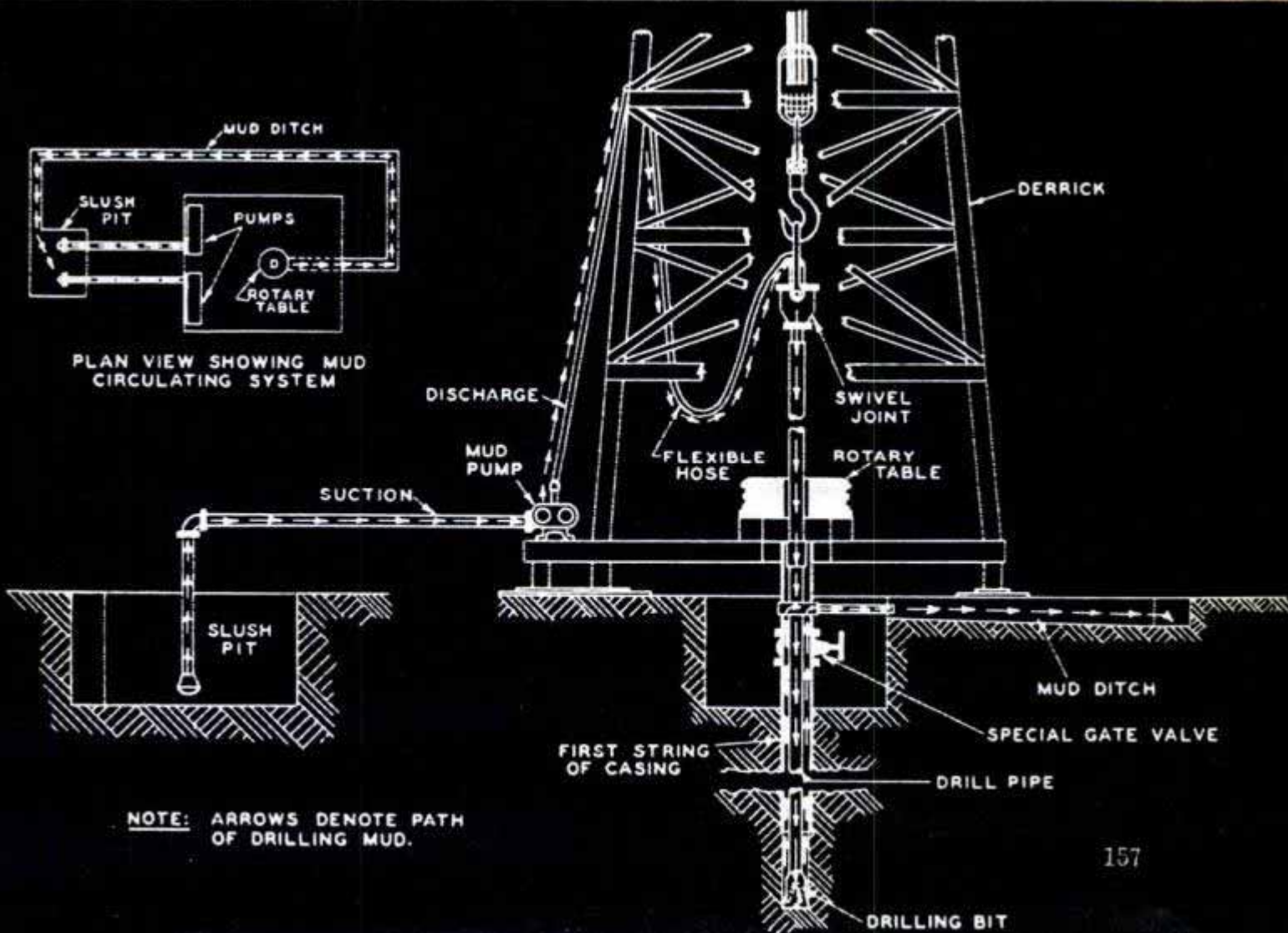
Diagram shows circulation of the mud around a rotary drill. Note the mud channel around the two pumps. Diagram from Pure Oil Co.
