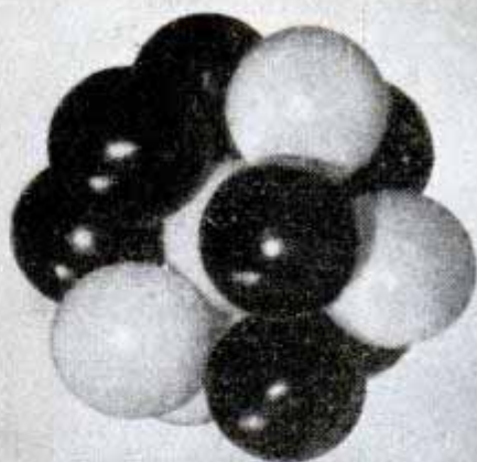
CARBON 13 ATOM NUCLEUS
