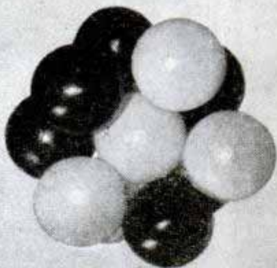
ORDINARY CARBON ATOM (C 12) NUCLEUS
