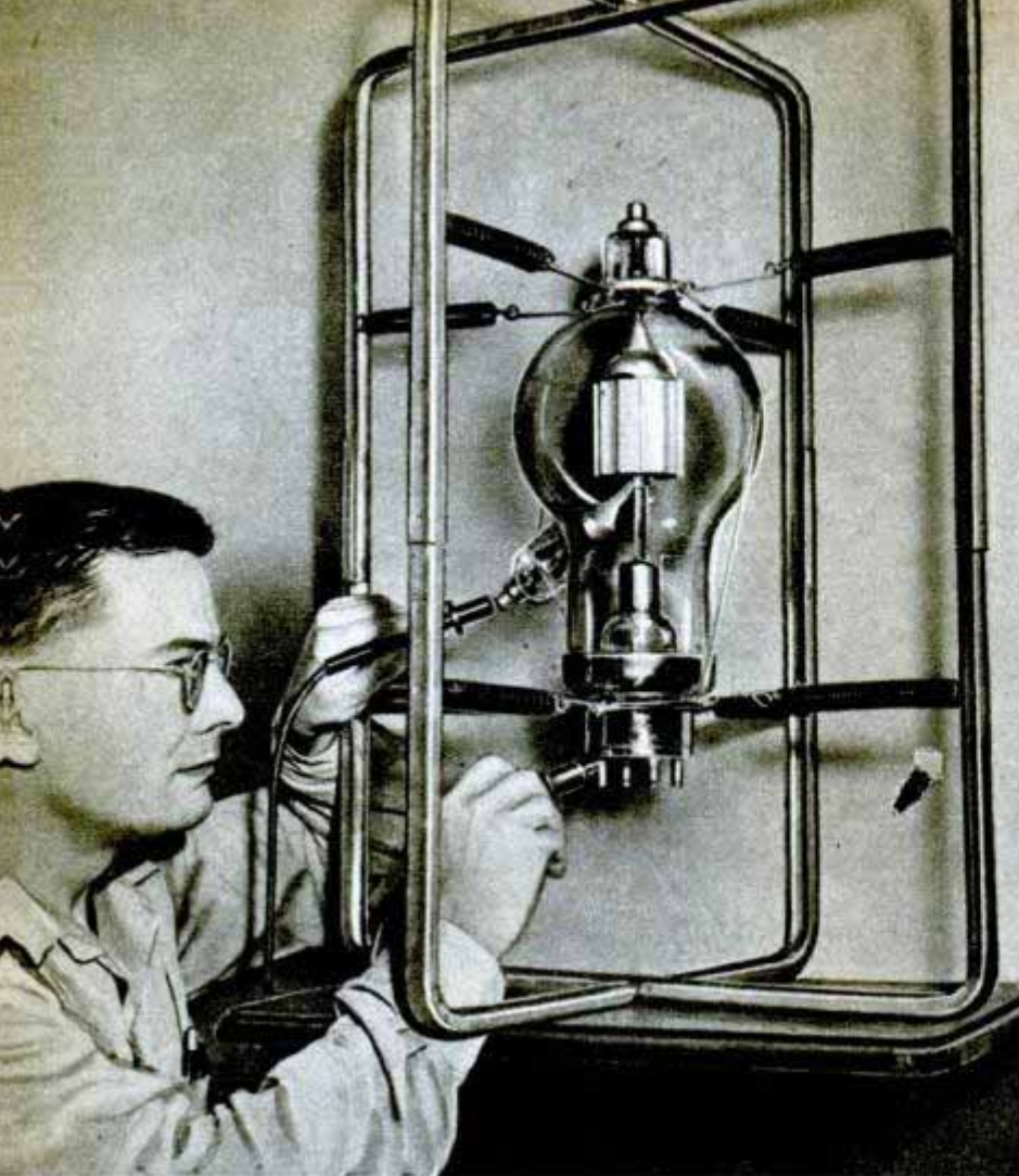
A technician tests the circuits of a large electronic tube that generates high-frequency waves. The waves are approximately the same length as those used by short-wave broadcasting stations
