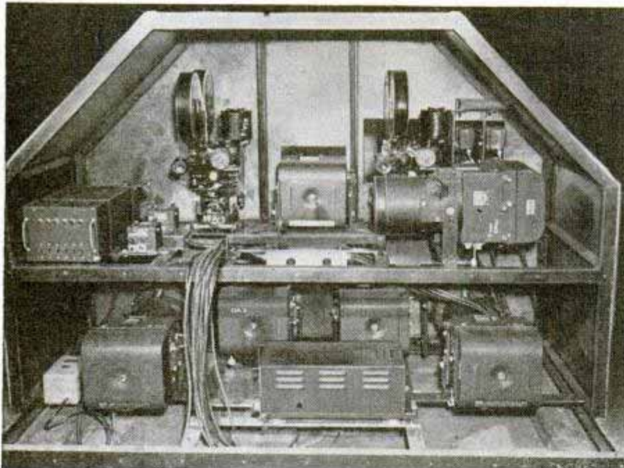
Platform containing batteries of radio-controlled cameras to be stored atop 100-foot steel towers on islands near the blast site. In the event radio control fails the cameras will be operated by a "magic eye" set in motion by the flash of the bomb itself. Below, rear view of the platform
