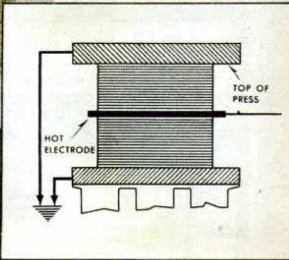
DIELECTRIC HEATING: Plastic preforms are heated by placing them between two electrodes carrying high-frequency current as shown in the sketch Westinghouse photos and drawings
