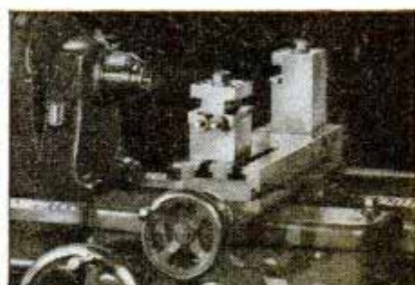
Screw Feed Double Tool Cross Slide for 16" lathes has both manual and power cross feed. Large graduated feed dial.
