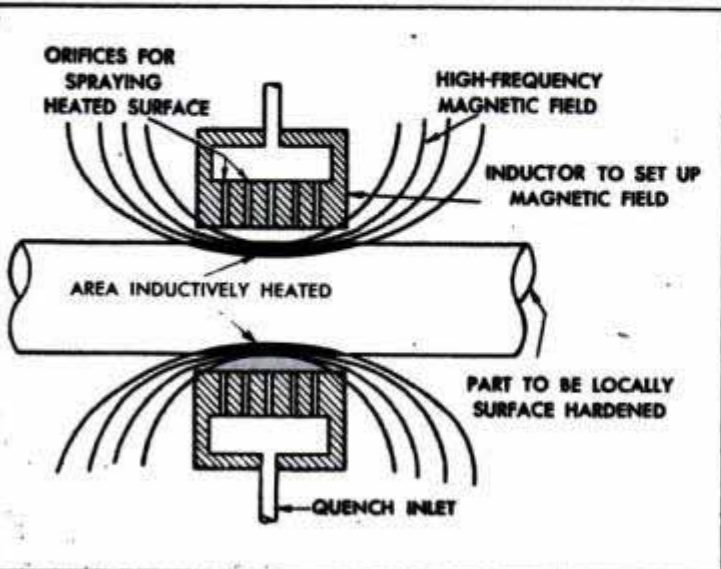
A typical surface hardening block for induction heating is diagrammed below. It includes openings to cool the work quickly by quenching it after heating. At right, hacksaw blades are hardened by a similar block
