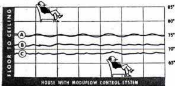
A — Temperature at ceiling B — at five foot level. C — temperature at floor.
