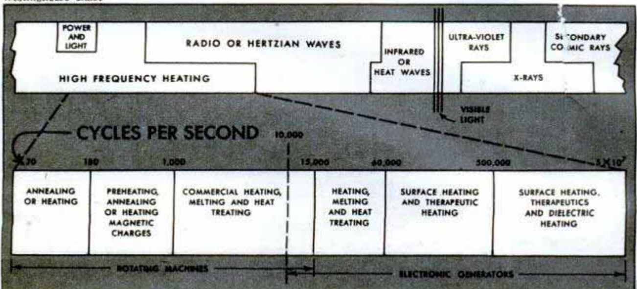
Diagram shows that part of the high-frequency radio wave spectrum that can be used for electronic heating Westinghouse chart
