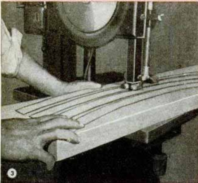
3 The back posts or legs are rough-sawed from a single piece of solid stock. This piece should be uniform in grain otherwise defects may show in the work
