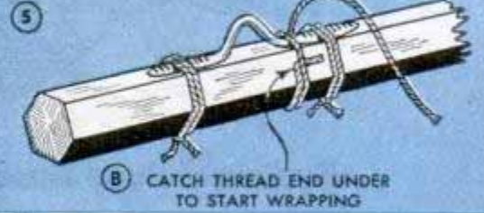
A TEMPORARY THREADS HOLD SNAKE GUIDE
