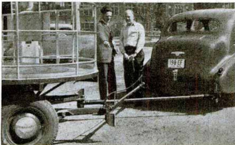
View of the criss-cross coupler which eliminates sidesway and zigzagging
