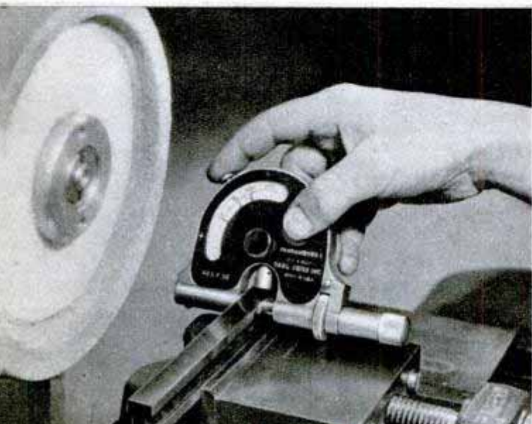
HANDY SNAP GAUGE with dial covers measurements up to three fourths inch and replaces several solid ones that were previously used in covering this range
