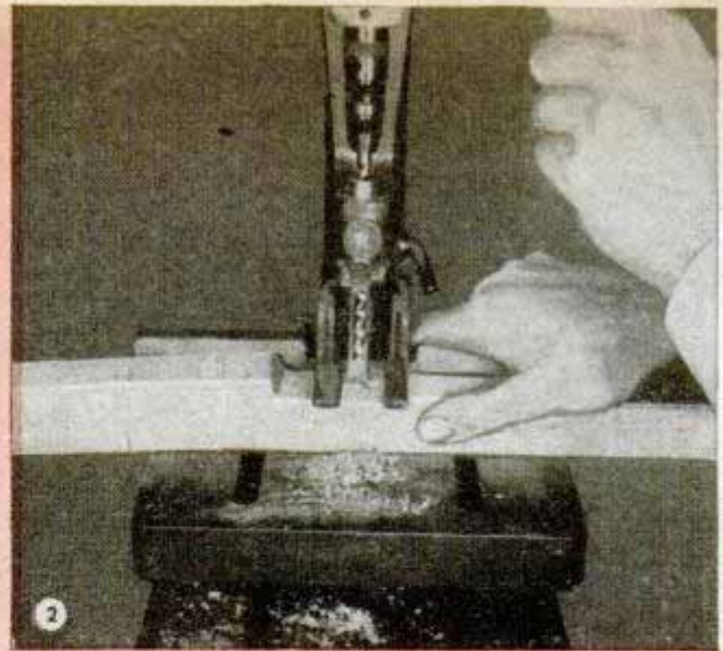
2 In making mortise-and-tenon joints a close fit assures strength equal to that of the wood itself. Be sure that the square chisel is tight in the holder
