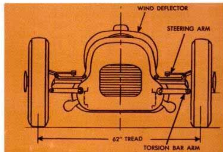
Front view of the Novi Special front-end-drive car
