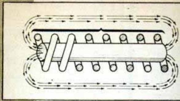
INDUCTION HEATING: Agricultural mower blades are hardened electronically. The sketch shows work in the magnetic field that is created by current in an induction coil
