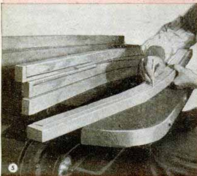
5 Use a sheet-metal or cardboard template to mark the parts for the second bandsaw cuts. Saw cut should be kept outside the line in the waste wood
