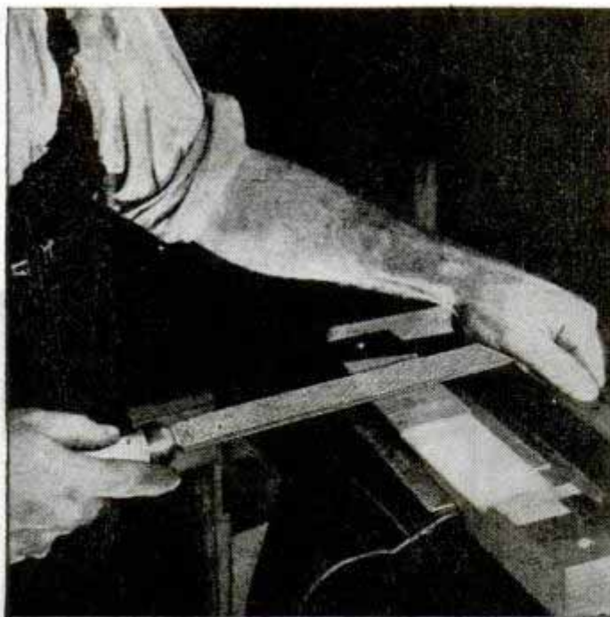
A Nicholson 12-inch Flat Second Cut File is being used here in filing a punch die.
