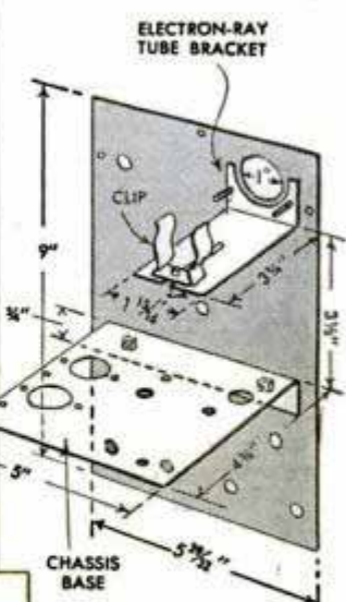
FIG. 3 DETAIL OF 1/16" METAL PANEL AND BASE
