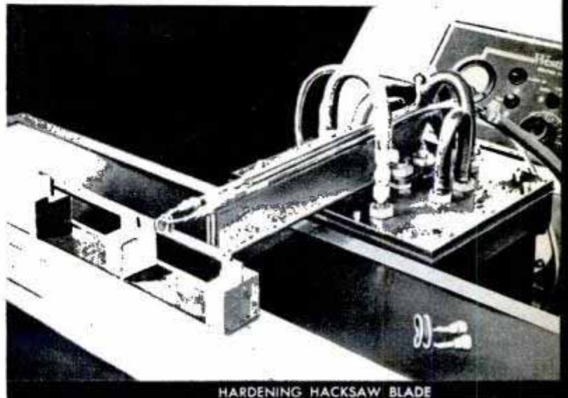
A typical surface hardening block for induction heating is diagrammed below. It includes openings to cool the work quickly by quenching it after heating. At right, hacksaw blades are hardened by a similar block
