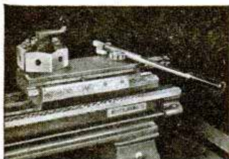
Handlever Bed Turret for 9" or 10" lathes multiplies their versatility through multiple tooling for repetitive operations.
