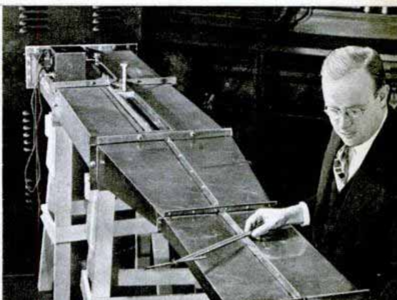
EXPERIMENTAL "BLOWTORCH" resembling a xylophone beams radio waves instead of concentrated flame to heat any object uniformly, regardless of shape
