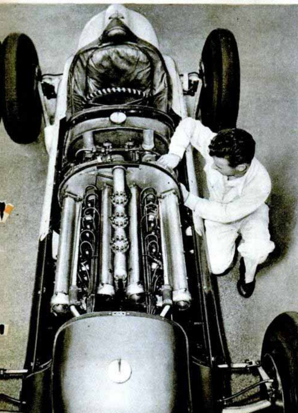
These two views of a "special" show the stable low-slung chassis and the supercharged 16-cylinder engine
