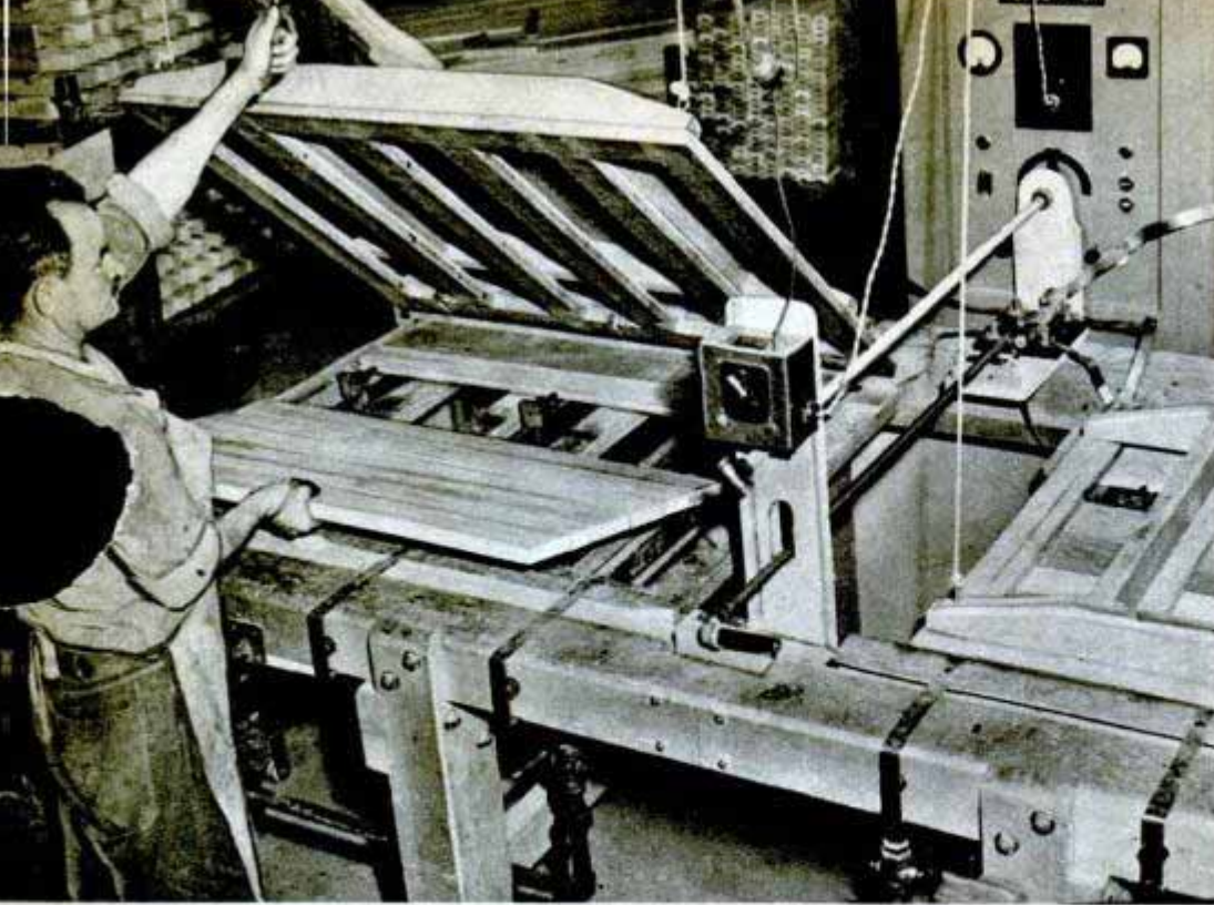
Glue in wood table top is cured in two minutes in a high-frequency heating jig. Below, these curved plywood beams were bonded by radio heat for use in building the giant Hughes flying boat
