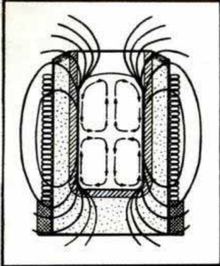
Induction furnace heats metal alloys. Diagram shows magnetic fields set up in furnace Westinghouse photo and drawing
