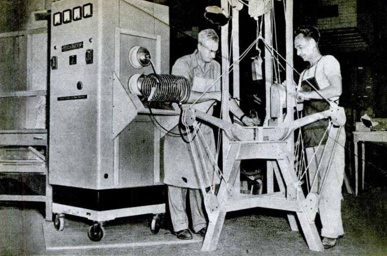
This complicated machine tests the strength of wood reinforcing angles after they are bonded by radio heat. Right, a heat "gun" cures glue inside wooden furniture
