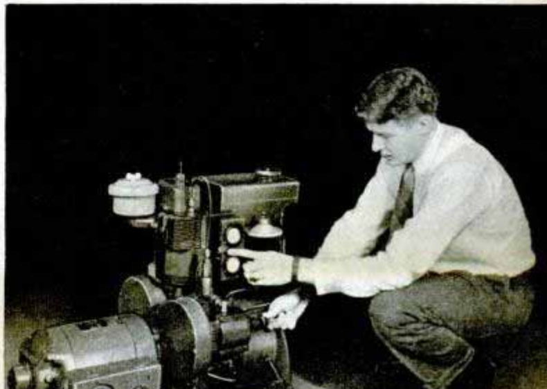
AIR-COOLED DIESEL ENGINE only 28½ inches high develops 3¾ horsepower. It was produced for powering communication systems, pumps and conveyors
