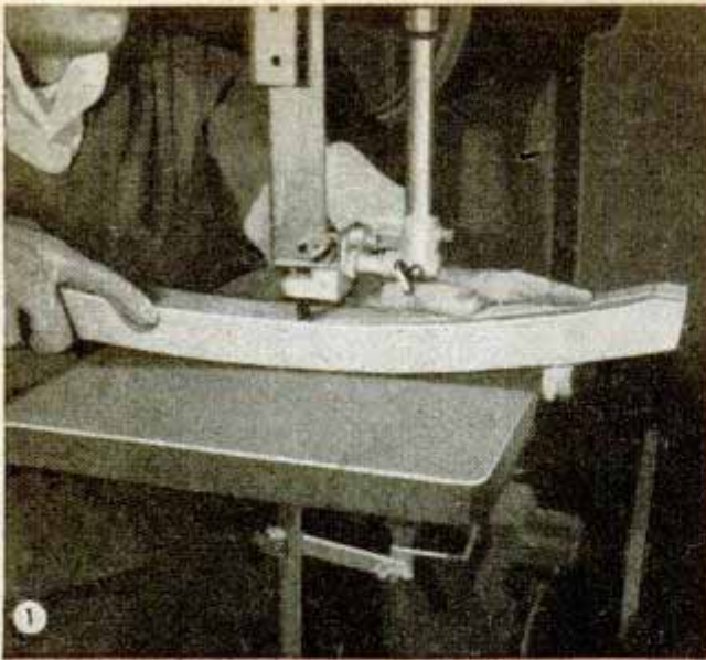
1 In bandsawing the first and second cuts care should be taken to keep the blade just outside the dimension line. This will allow for finishing to exact size
