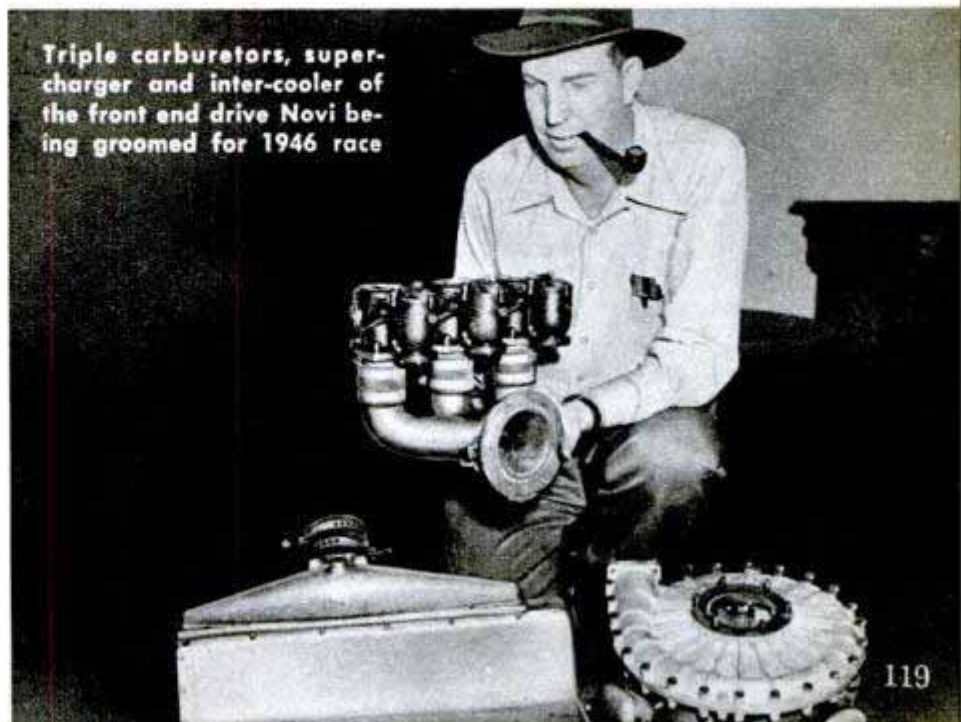
Measuring engine clearances after power plant has been put in chassis. Note the tubular frame construction
