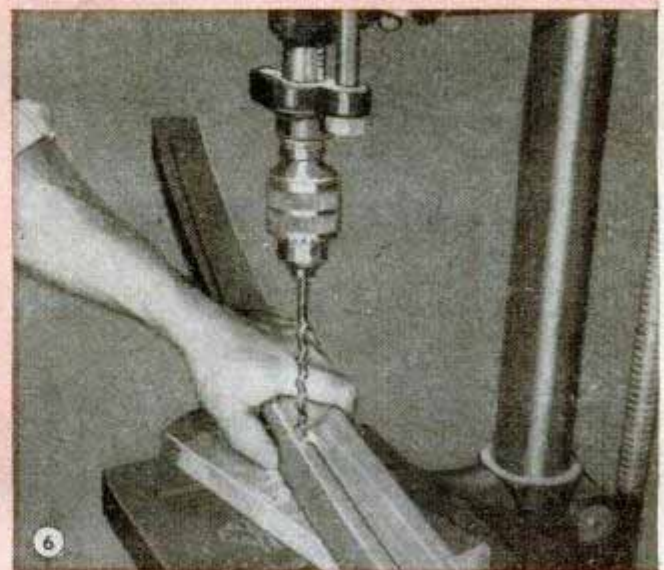
6 The hole forming the curved offset in the back leg is drilled before bandsawing. Select a bit of the same radius as the curve indicated in the details
