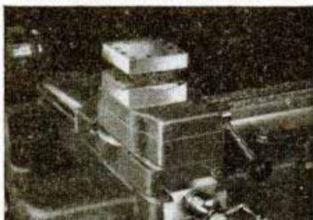
4-Way Turret Tool Block permits use of four cutting tools which simplifies tooling for repetitive operations.
