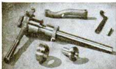
Handlever Draw-in Collet Attachment saves time on bar work. Collet can be operated and stock fed without stopping spindle.
