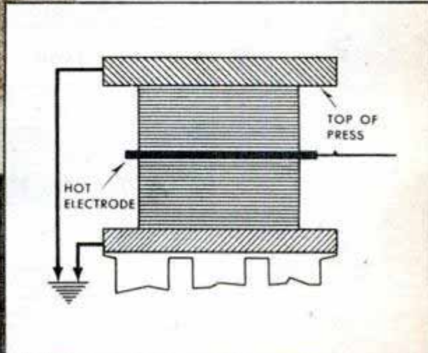
DIELECTRIC HEATING: Plastic preforms are heated by placing them between two electrodes carrying high-frequency current as shown in the sketch Westinghouse photos and drawings
