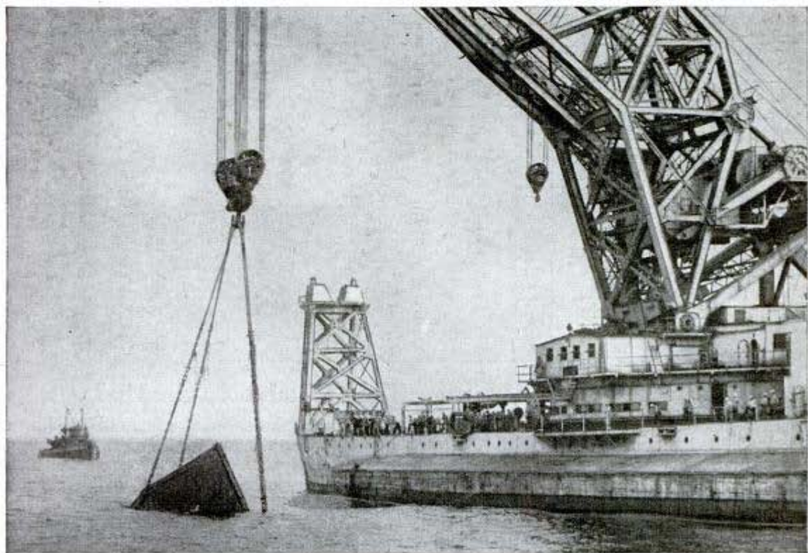
Below, lifting bow of U.S.S. Turner, ripped apart by explosion
