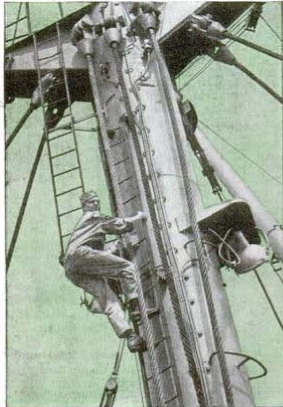
A soldier (above, left) mans a donkey engine while a crewmate lowers a steel pump over the side of a harbor repair ship. Below, a radio operator climbs up the "king post" to repair an aerial on the ship
