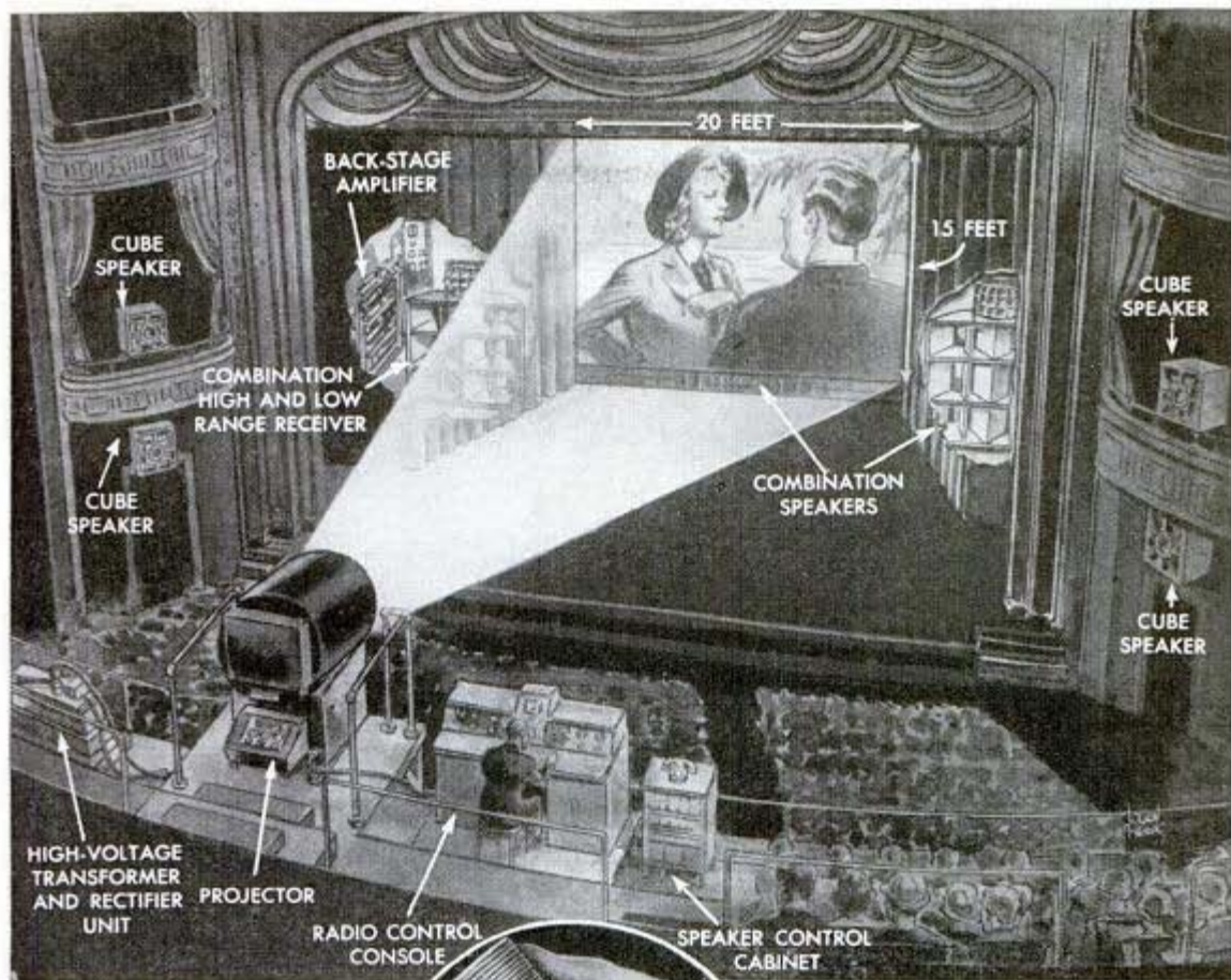
Sketch shows setup for the projection of television in a theater. The tube (left) makes ultra-high frequency relaying possible. Below, using television cameras in studio
