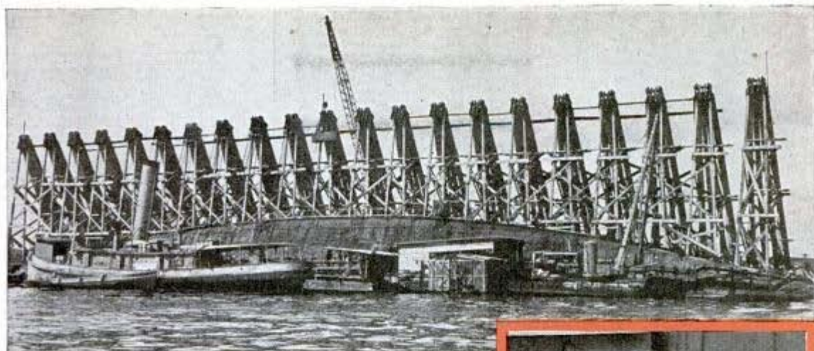
Above, U.S.S. Oklahoma, sunk at Pearl Harbor, is raised with help of timber frames. Right, rescue ship's kedge anchor which is dropped and pulled against in hauling vessels off shore U. S. Navy photo
