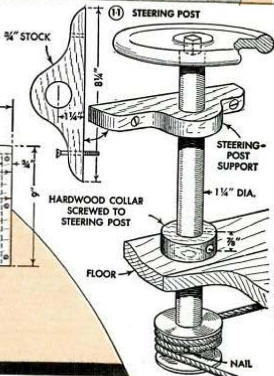
10 UNDERSIDE VIEW OF SIDE STEERING ARRANGEMENT
