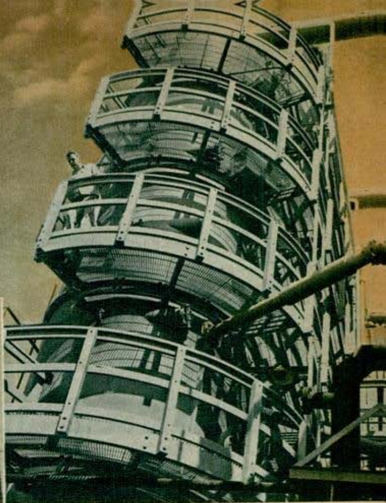
Above, a styrene extraction tower at a synthetic rubber plant. Left, raising a distillation tower. Below, box kites to lift radio antennas on rafts
