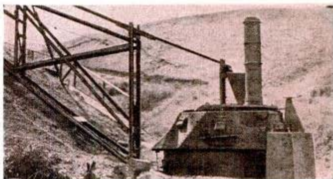
Salvaged M-3 tank with smokestack on top serves as exploding chamber for defective primers and fuses carried on an endless belt. Below, test firing carbine in the underground gallery
