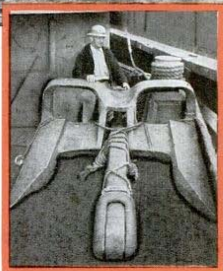
Above, U.S.S. Oklahoma, sunk at Pearl Harbor, is raised with help of timber frames. Right, rescue ship's kedge anchor which is dropped and pulled against in hauling vessels off shore U. S. Navy photo
