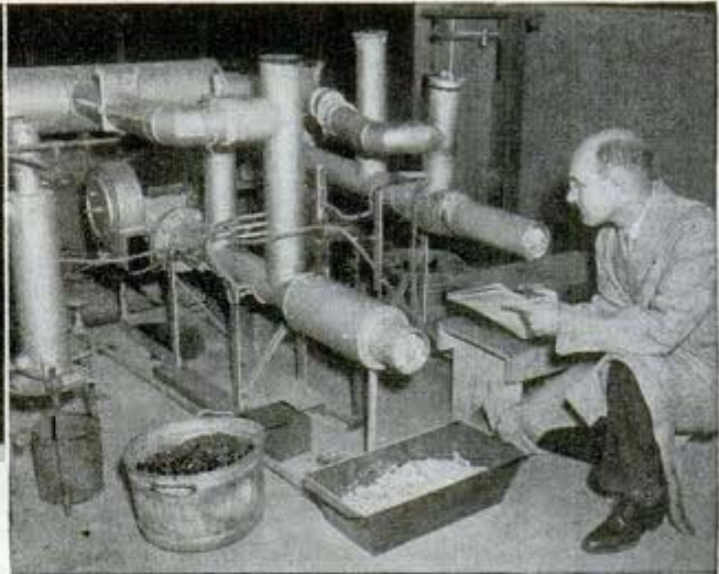
The 75-pound tubular burner is dwarfed by conventional furnace. Right, conducting ash tests on two units. Below, cutaway of tube
