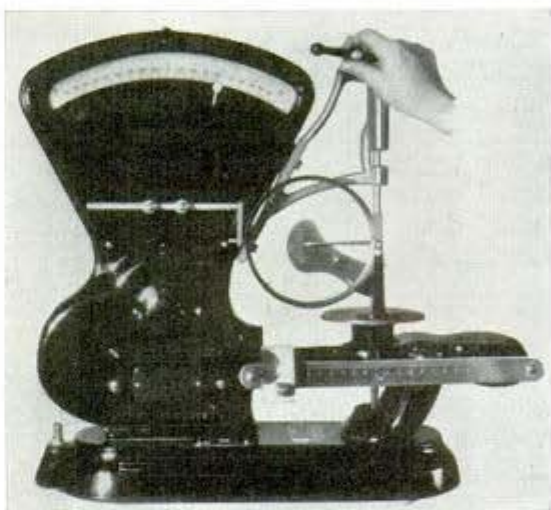
Scale "weighs" pressure exerted by auto piston ring
