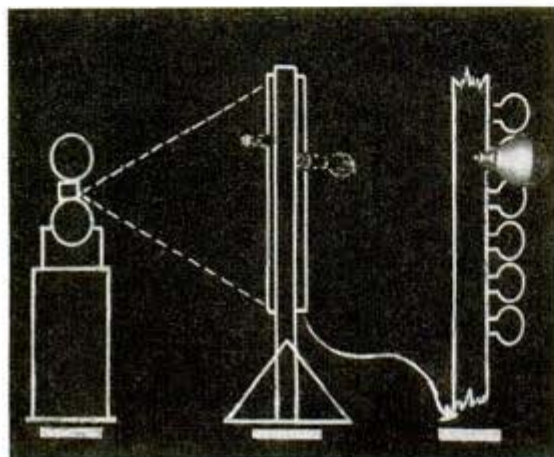
Diagram shows how animated cartoons are projected from machine, left, via photocells to electric screen
