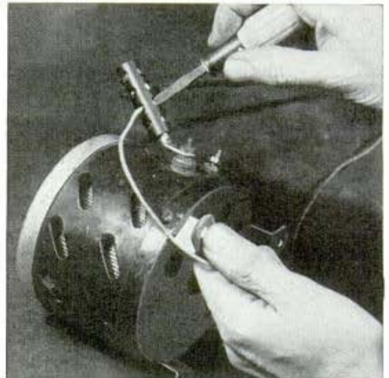
Connector bolted to binding post holds several wires
