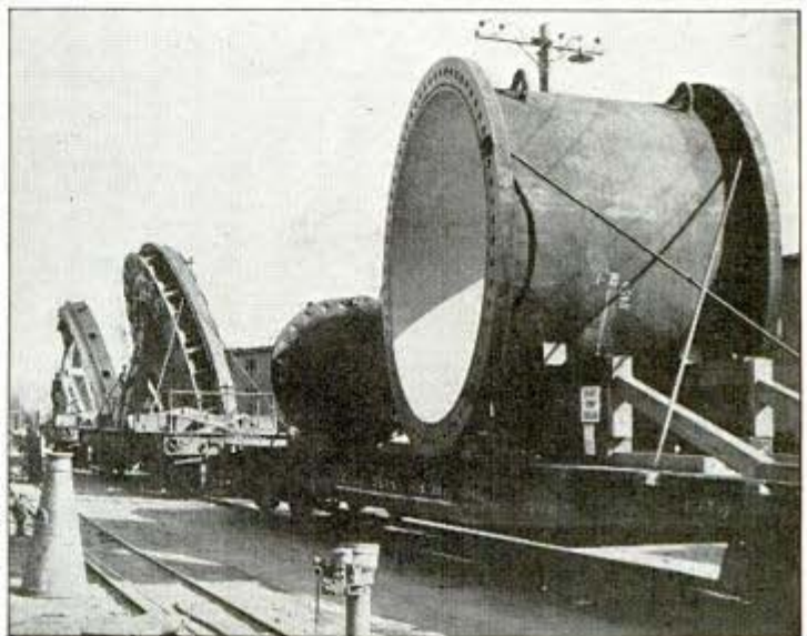
These gigantic turbine parts for a western dam had to be shipped on specially built freight cars
