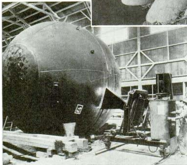
200,000-volt X-ray inspects seams of 18-foot steel welded plug to be used for closing off penstocks and pipe line of Grand Coulee Dam
