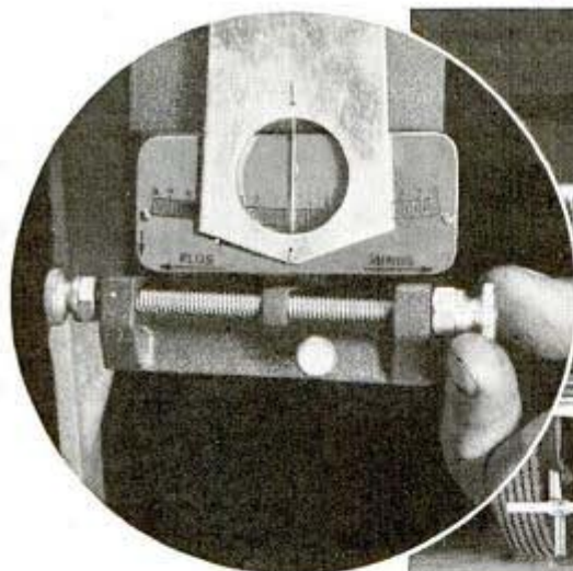
Dial, above, indicates both camber and caster. Right, top, toe-in trammel bar and gauge; bottom, angle gauge shows up bent radius rod. All parts are easy to handle
