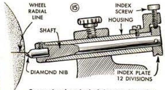
Conventional method of dressing face of a grinding wheel for external cylindrical grinding is shown in Fig. 14. The improved diamond dressing fixture above permits obtaining fresh cutting edges by slight rotation of the shaft on which the diamond is mounted
