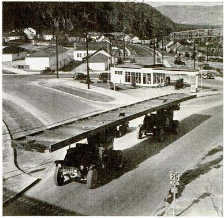
Trucks arranged in tandem are equipped with special crib-work to carry 100-foot girder
