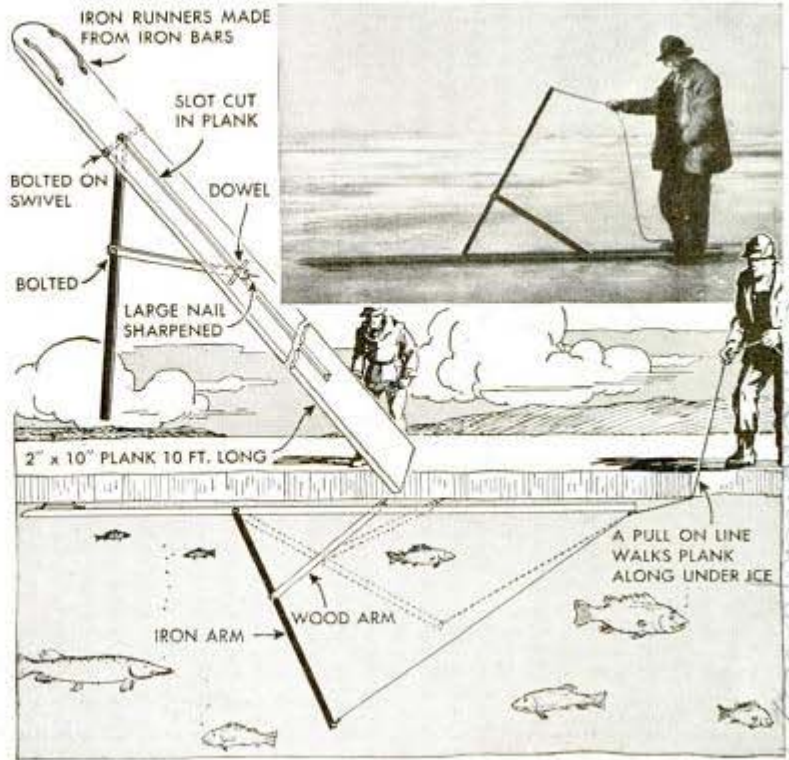
Sketches show how "walking jigger" travels under ice by remote control.
