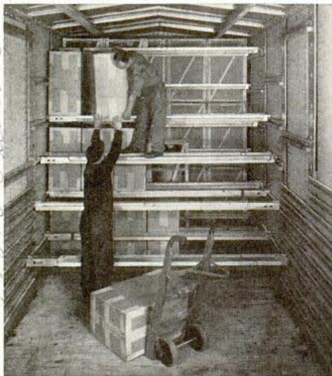
↑ Workmen using cross members of utility loader as platform while stowing cargo on top
