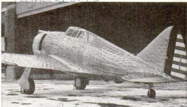
Little tufts of string "planted" on plane indicate flow of air currents
