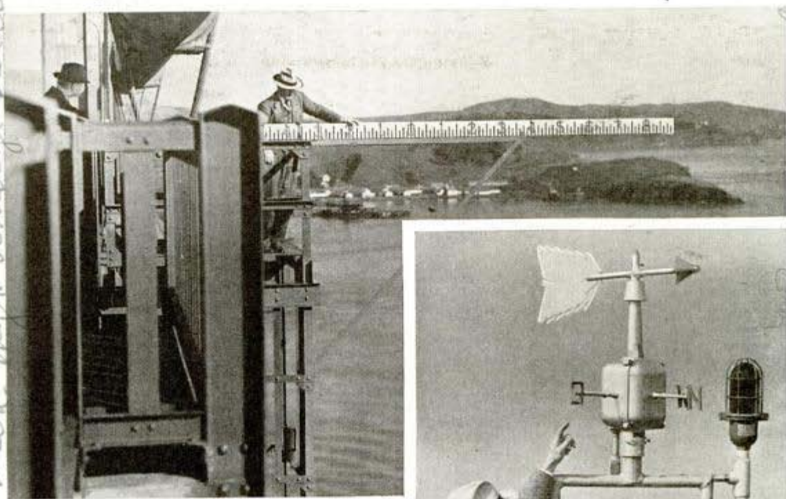
Photos, courtesy Redwood Empire Association Horizontal measuring rod, above, is 17 feet long; right, instruments chart wind speed and direction
