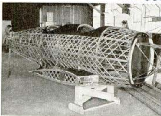
Skeleton of a "Plexweve" plane of geodesic construction, formed by wrapping spruce spirally over laminated bulkhead
