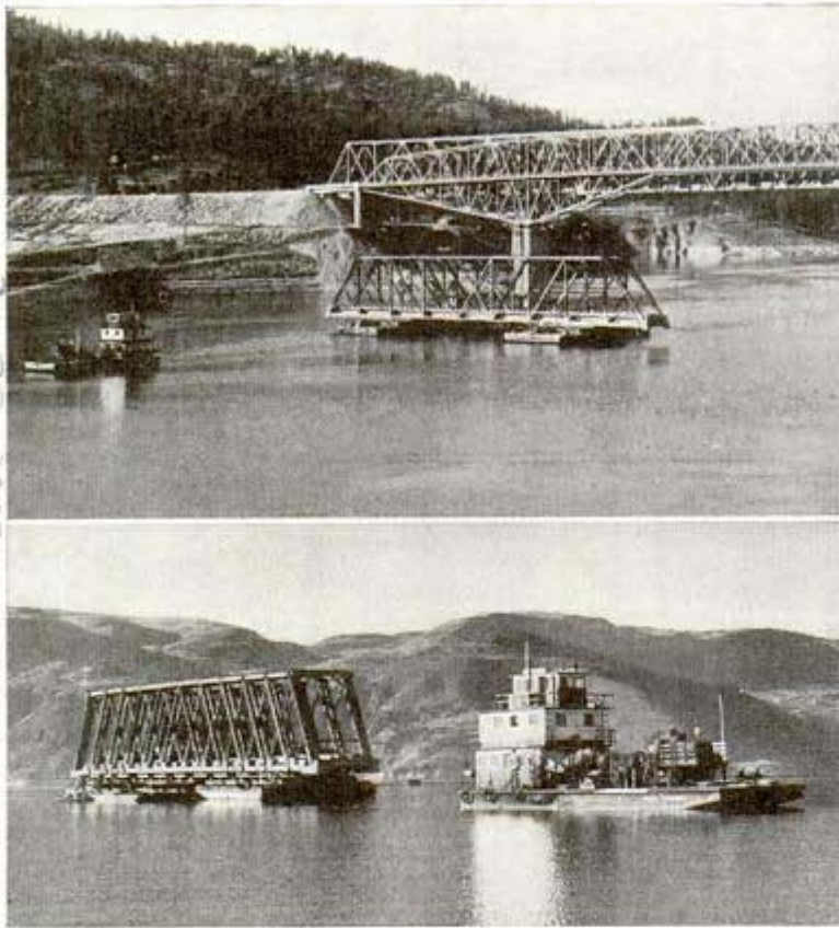
Old span, top, passing under new railroad and highway bridges five miles downstream. Bottom, one of the wooden spans towed by a motor barge
