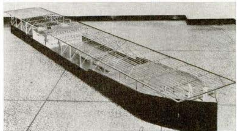
Models show (top) special wheels to grip deck; (bottom) "lattice deck" on ship
