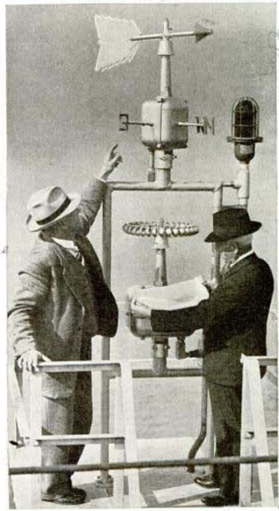
Photos, courtesy Redwood Empire Association Horizontal measuring rod, above, is 17 feet long; right, instruments chart wind speed and direction
