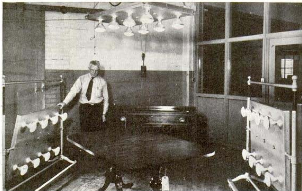
Portable banks of 250-watt lamps dry the finish on a table. Furniture finishes can be dried in 20 minutes
