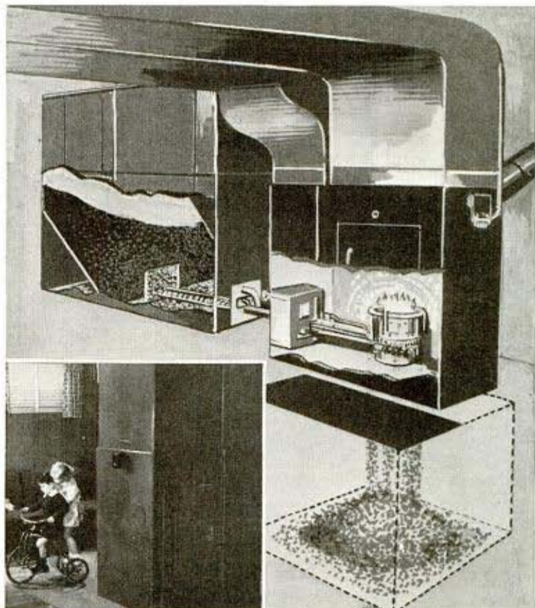
Cutaway sketch shows stoker, and ash pit under fire chamber. Inset, exterior view of cabinet
