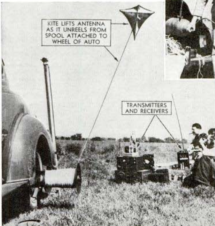
Two methods used by amateur radio operators for erecting emergency antennas. Above, inflating balloon with hydrogen, and, left, sending up kite attached to spool mounted on auto wheel
