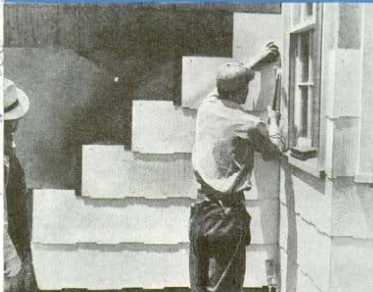
Nailing asbestos siding over plywood on home in "smokeless community" Meadow Hills Automatic electric heating unit being installed in a Fonde-built home ↓
