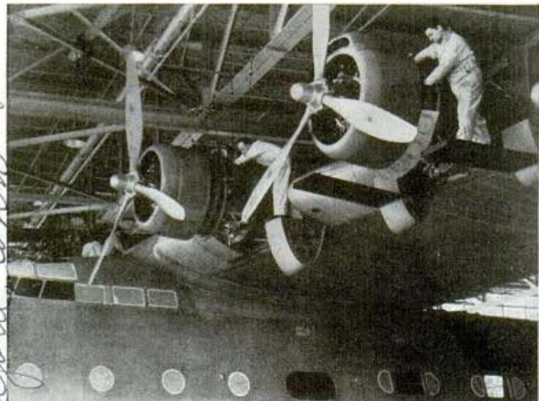
Mechanics installing two of the power units that will contribute their share in non-stop crossings of the Atlantic. Propellers have three full-feathering type blades
