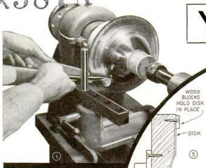
STARTING CHUCK IS RECESSED TO HOLD DISK
