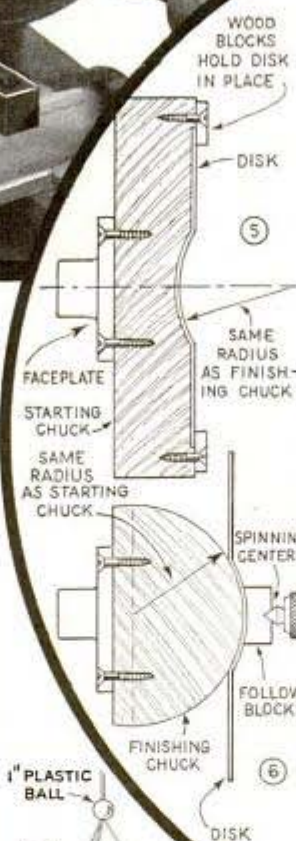
STARTING CHUCK IS RECESSED TO HOLD DISK
