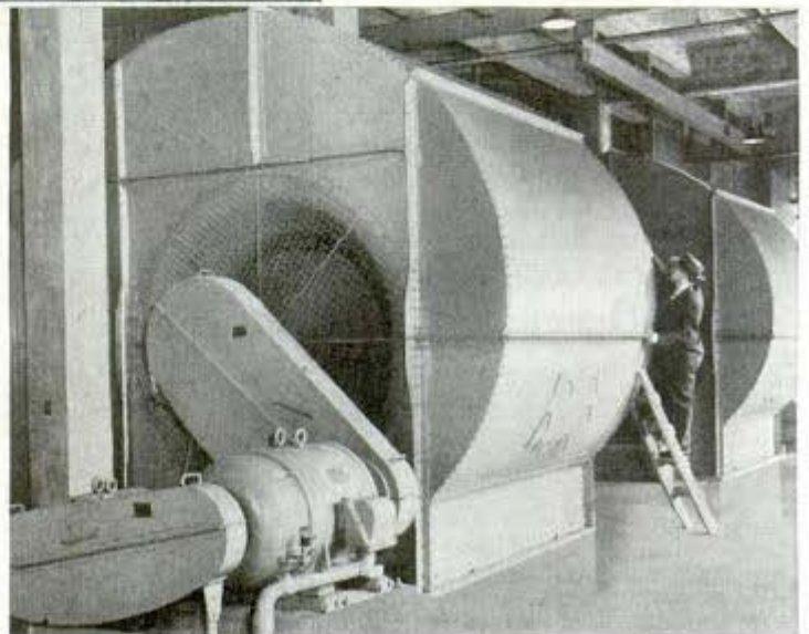
Tunnel Authority inspector examines one of 23 huge blowers that change air 42 times an hour in Queens Midtown Tunnel
