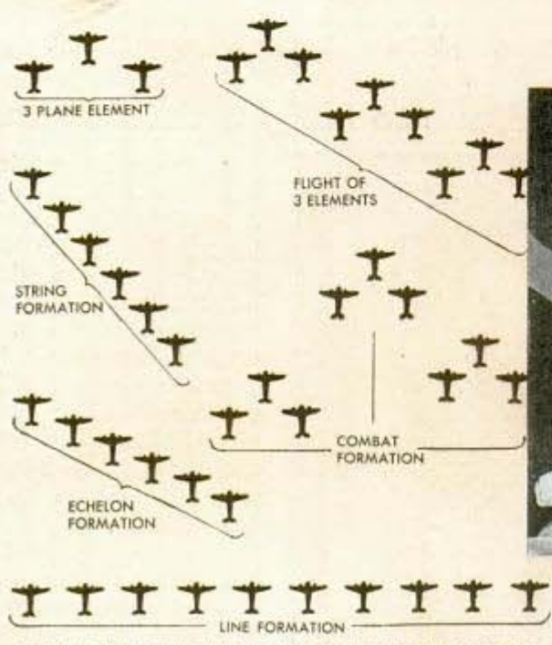
Pilot sighting through electric gunsight. Below, formations used by pursuit plane groups. Note the formations employed in combat
