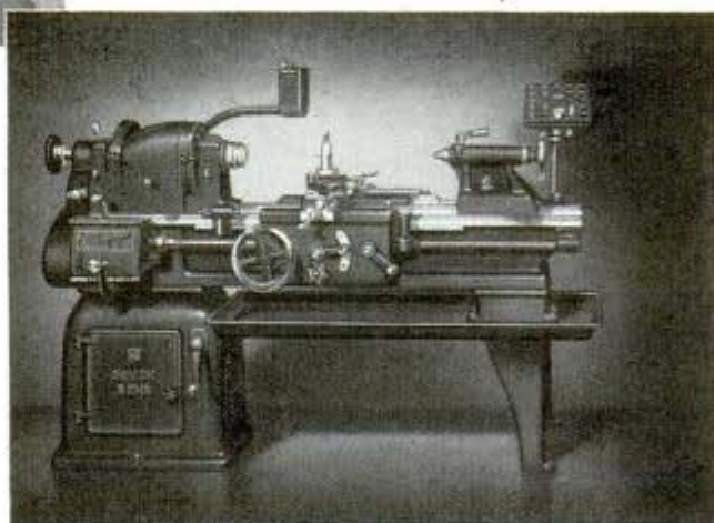
South Bend 16" Toolroom Precision Lathe
