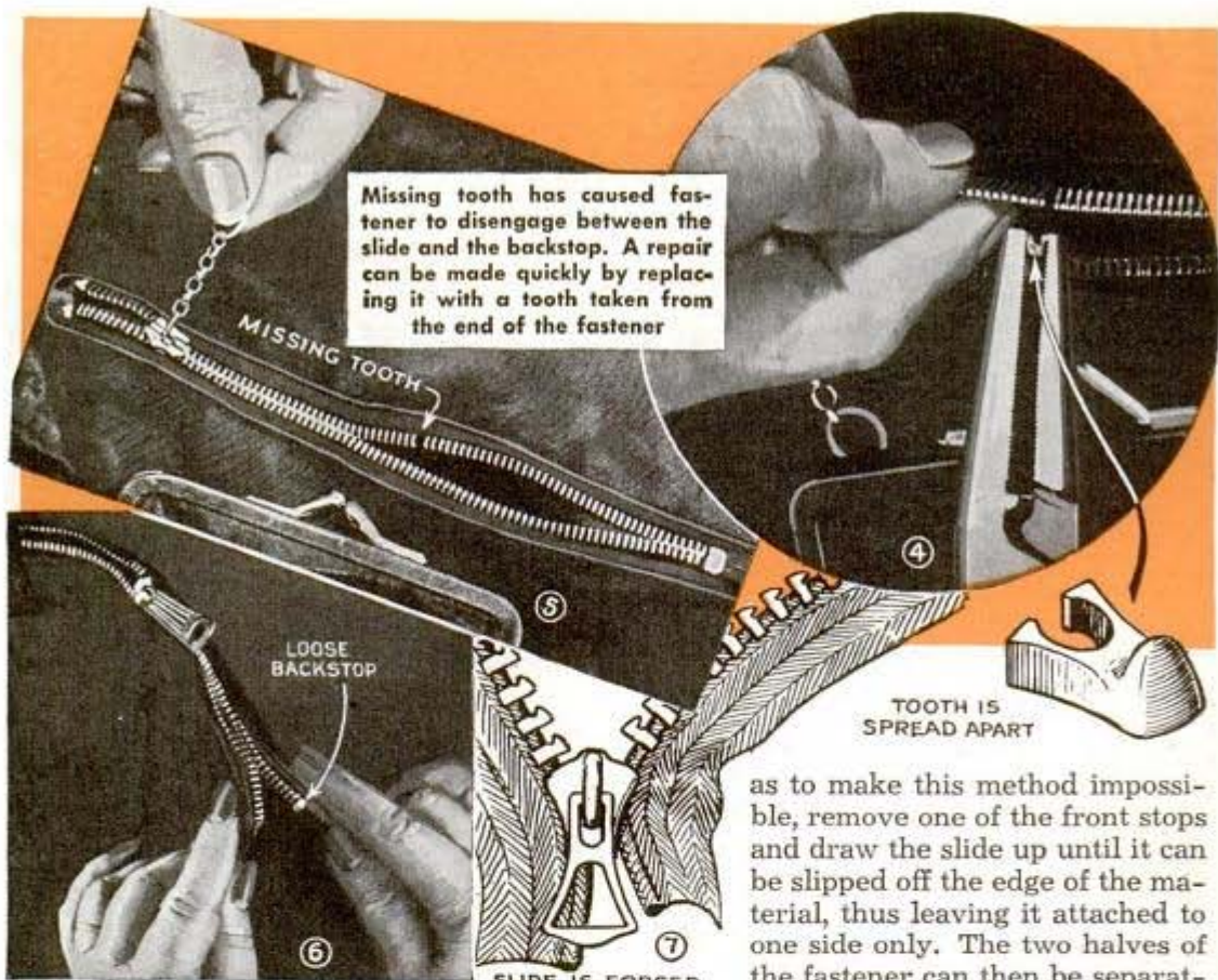
Loose backstop caused this fastener to open at rear. Repeatedly moving the slide against it will usually close it
