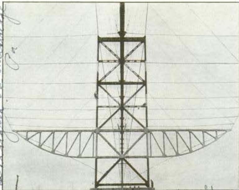
American Hoist & Derrick Co. Robert & Water St A 16-inch pipe line crosses Missouri river on half-mile suspension bridge
