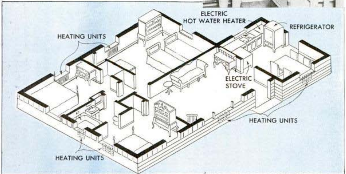
↓ Simplified drawing of Fonde house with roof removed to show the various electrical appliances and the location of electric heating units
