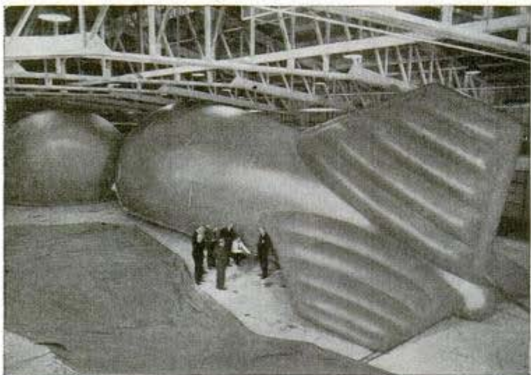
Four-fin balloon (above) inflated and ready for ascent after removal from hangar. Below, odd-looking barrage balloon of type being built for the Army by General Tire & Rubber Company
