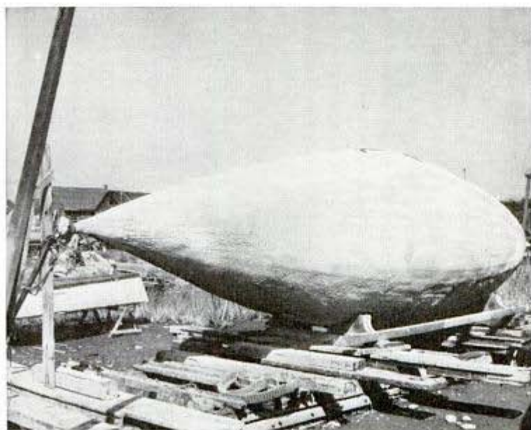
Concrete-coated submarine towed by warship, carries cargo under water
