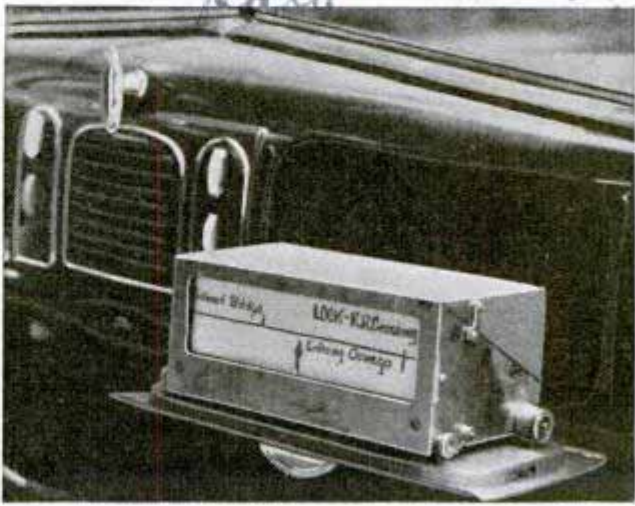
Highway map travels past window, keeping pace with progress of car by speedometer attachment
