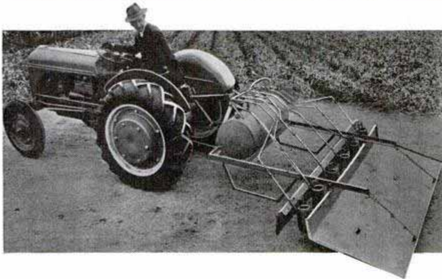
Burners fed by gas from kerosene tank throw intense flames beneath metal shield, creating an "inferno" to consume lice in the soil after harvest
