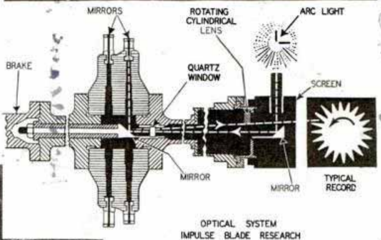
Diagram indicates how optical viewer peering into turbine (above and left) records vibration pattern. When the turbine turns without vibration, the light describes a circular path; when there is vibration, waves or notches appear in the circle
