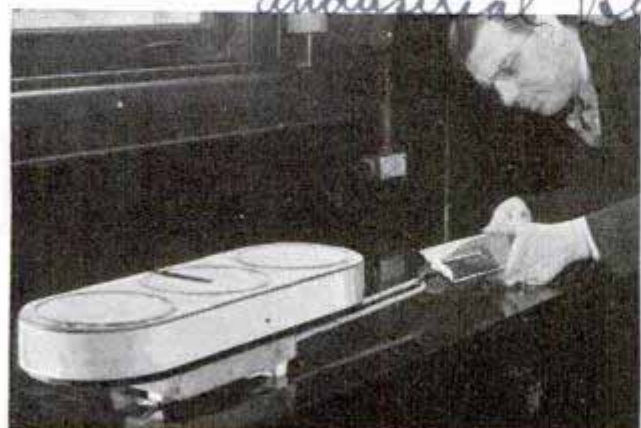
Effort required to pull 100-pound weight on "bobsled" over waxed surface is read on spring scale
