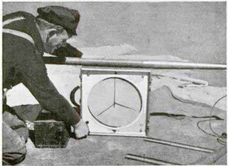
Top, timing an outboard speed trial. Bottom, brass tube resting on carrying case of clock contains "electric eye"
