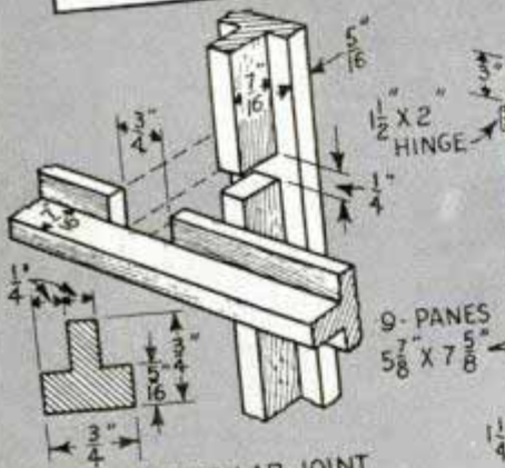
DETAIL OF HALF-LAP JOINT ON DOOR MULLIONS
