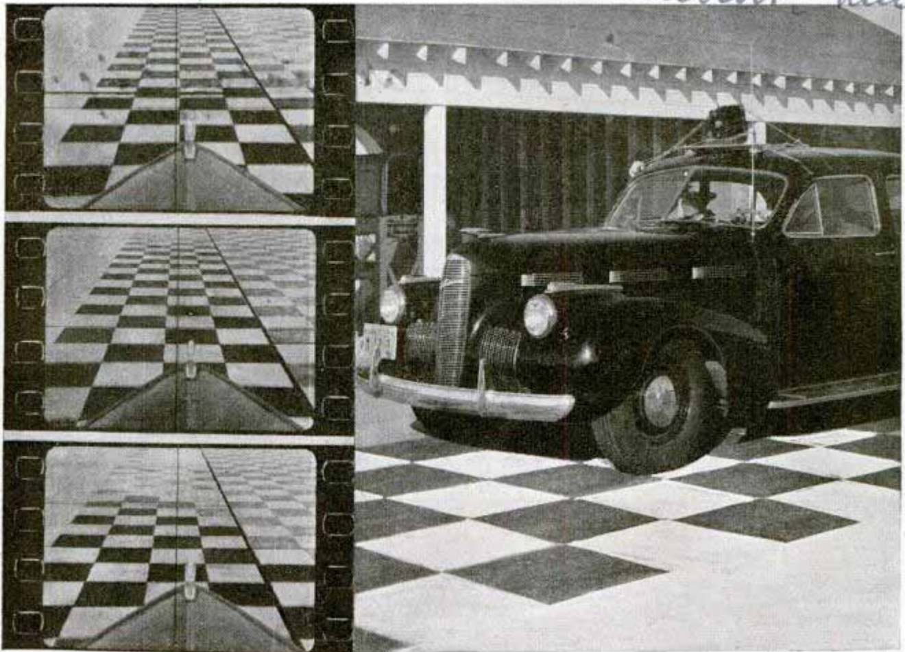
Views at left are taken from film made to analyze effect of side winds, shift of film center-line indicating extent of deviation from straight path. Right, camera on car roof is focused on checkerboard road
