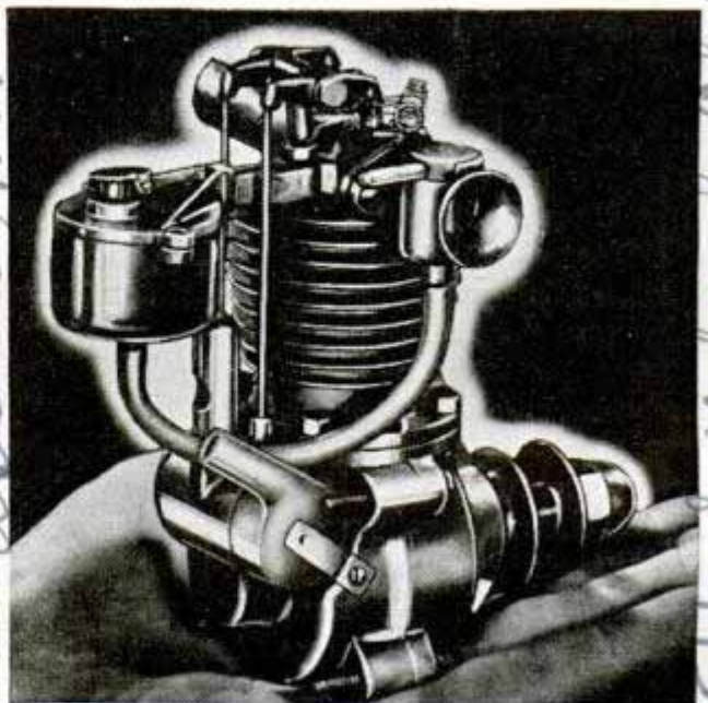
1516 W. Wash. Chevy 9151 Throttle control on model planes operated by radio is possible when this fifteen-ounce engine is used
