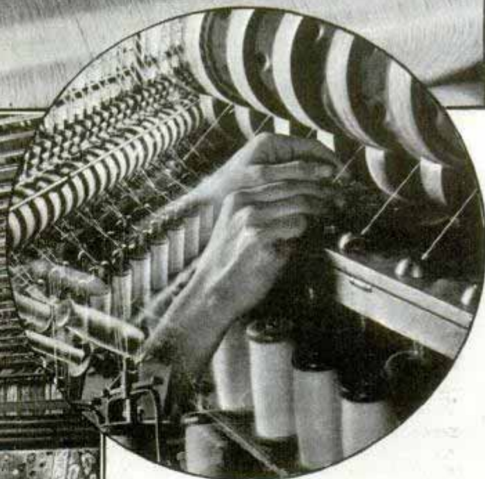
Modern engineering and scientific methods enable rug makers to meet the increasing demand. Top, right, operating cotton beamer, which combines several banks of warp threads and transfers them to the loom beam. Circle, how the long fibers are changed into yarn. Bottom, endless chain of spools which successively brings each spool into position in loom. Note the rug coming from the loom before which the worker stands
