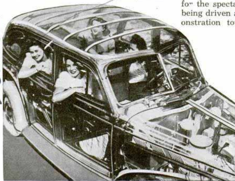
Automobile inclosed in transparent body exhibits structural bracing and mechanical features, also giving passengers unrestricted vision
