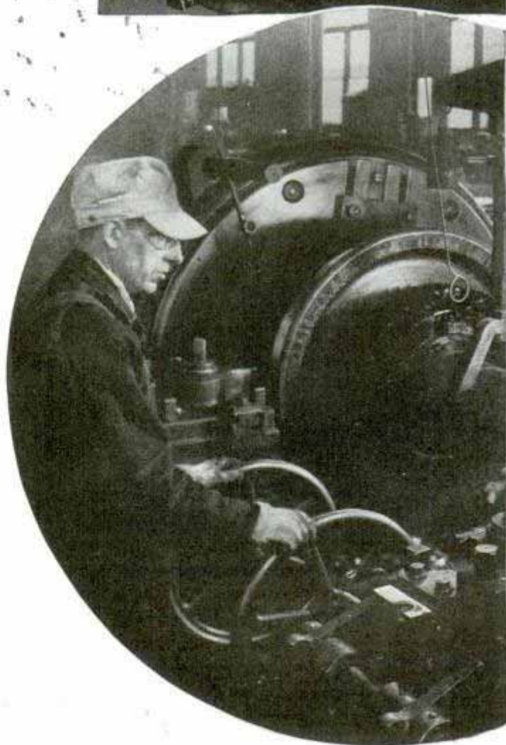
Diesel repairmen above, at left, remove piston assembly from 900-horsepower engine; right, roller bearings that smooth the streamliner's ride. Below, skilled lathe operator machines a pair of power wheels
