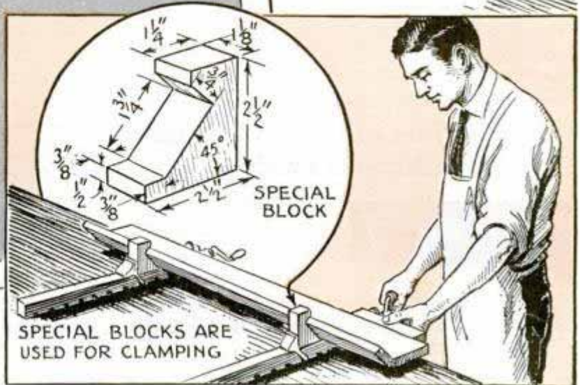
A GAUGE BLOCK IS CONVENIENT FOR SPACING SHELF PINS
