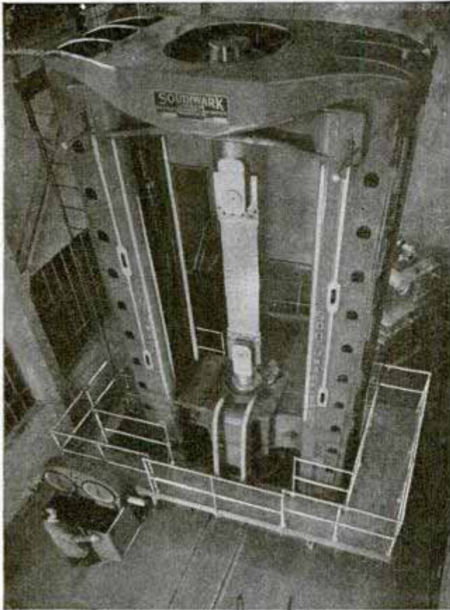
clerk At left is the research machine that can exert a 3,000,000-pound push; it was built to test fabricated aluminum products. At right, it uses a third of its muscle power to split a sturdy oak *
