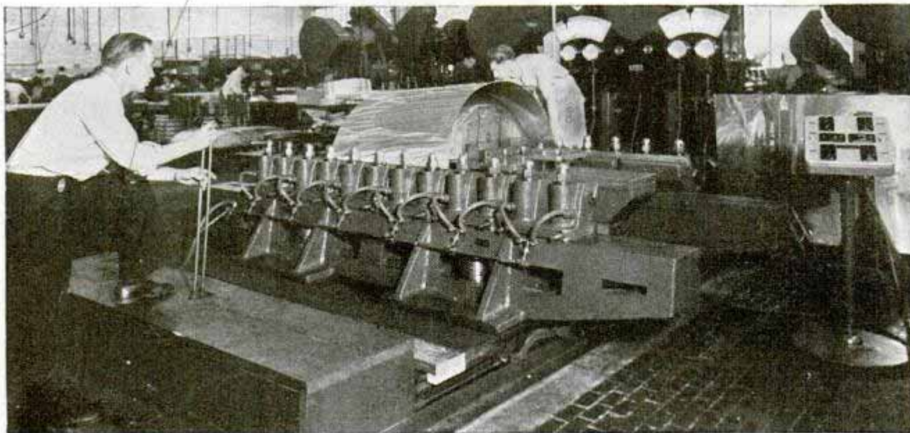
Hydraulic pressure applied to two cylinders under platen forces the form upward against sheet metal, stretching it into the shape of the form. Strong clamps grip the two ends of the sheet
