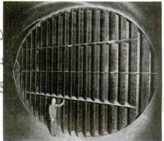
Nineteen-foot crescent-shaped vanes guide high-velocity wind around corners of wind tunnel
