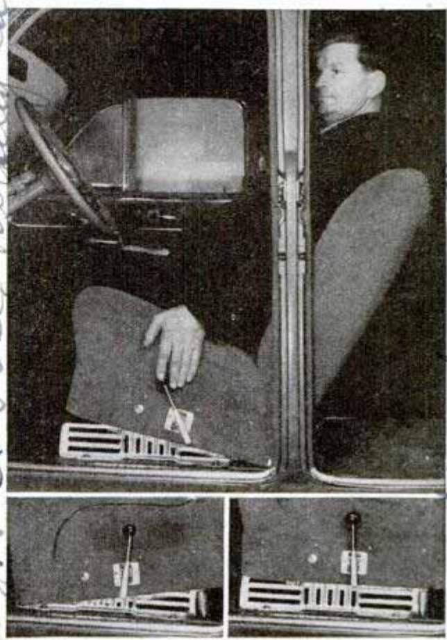
Tilting lever is reached easily by driver's left hand, above. Two bottom views show other seat positions
