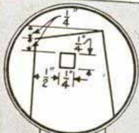
DETAIL OF TRAY ENDS
