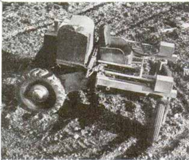
Tractor turns "pigeon-toed" to wheel around in its own length. Note forward position of driver's seat
