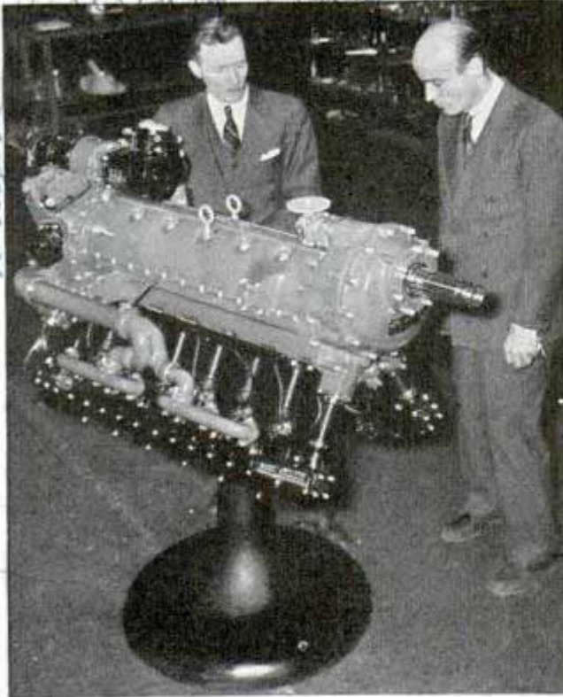
Inspecting twelve-cylinder airplane engine developing one horsepower for each 1.28 pounds of weight
