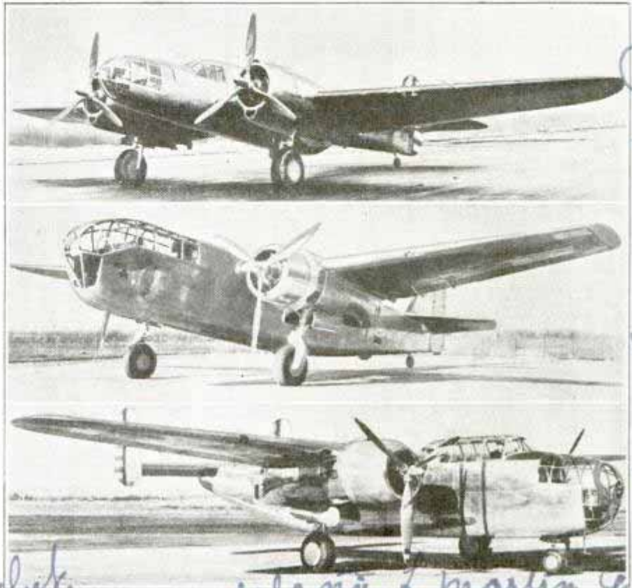
Photos U. S. Army Air Corps Top, the Martin attack bomber; center, Stearman Aircraft's entry, and below, the tricycle-type ship offered by North American Aviation
