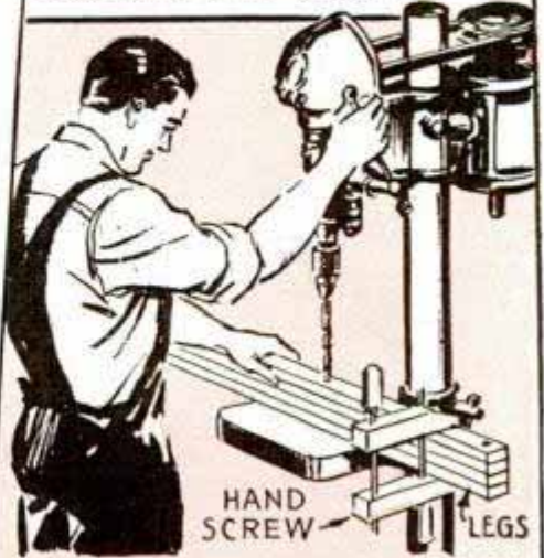
BORE THE DOWEL HOLES THROUGH FOUR LEGS AT THE SAME TIME
