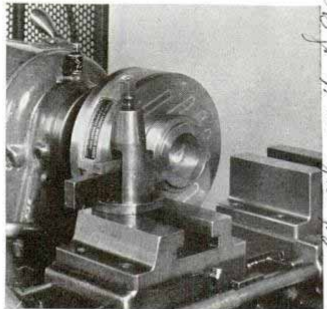
High-power magnet of this chuck obviates use of electricity, and magnetism lasts indefinitely
