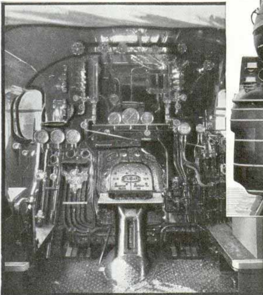
Wearing the name "American Railroads" because it is the pride of their New York World's Fair exhibit, this 140-foot steam locomotive is the largest ever built. Two of its four cylinders are visible at top. Left, the cab
