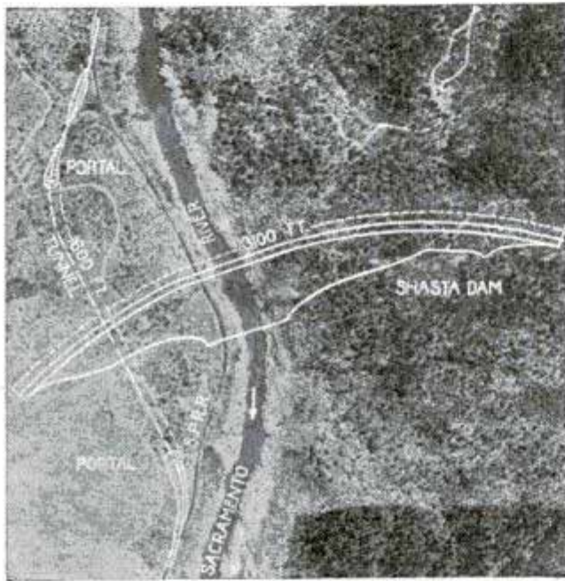
Showing how Shasta Dam will appear when completed. Note change in railroad route at left
