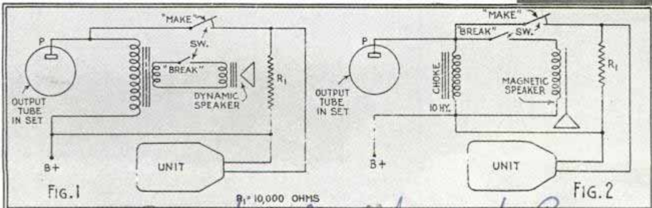
PILLOW-SPEAKER UNIT
