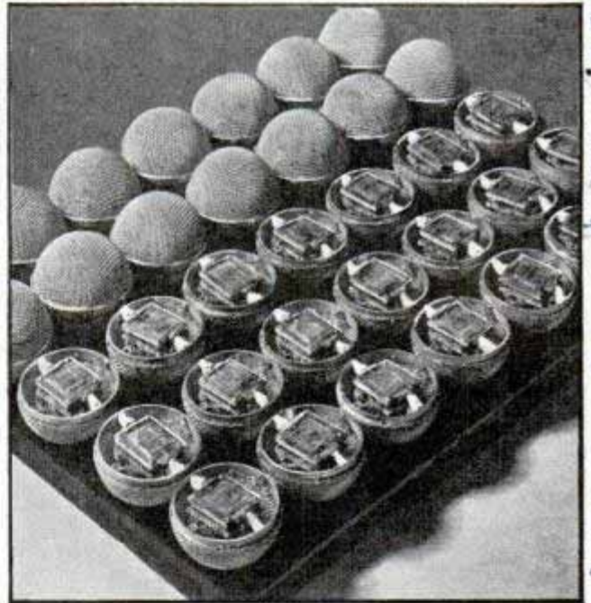
A tray of sound-cell microphones on the production line at the Brush Development company plant
