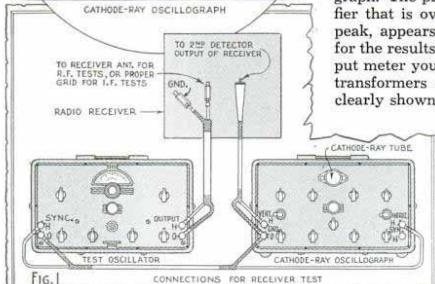
CONNECTIONS FOR RECEIVER TEST
