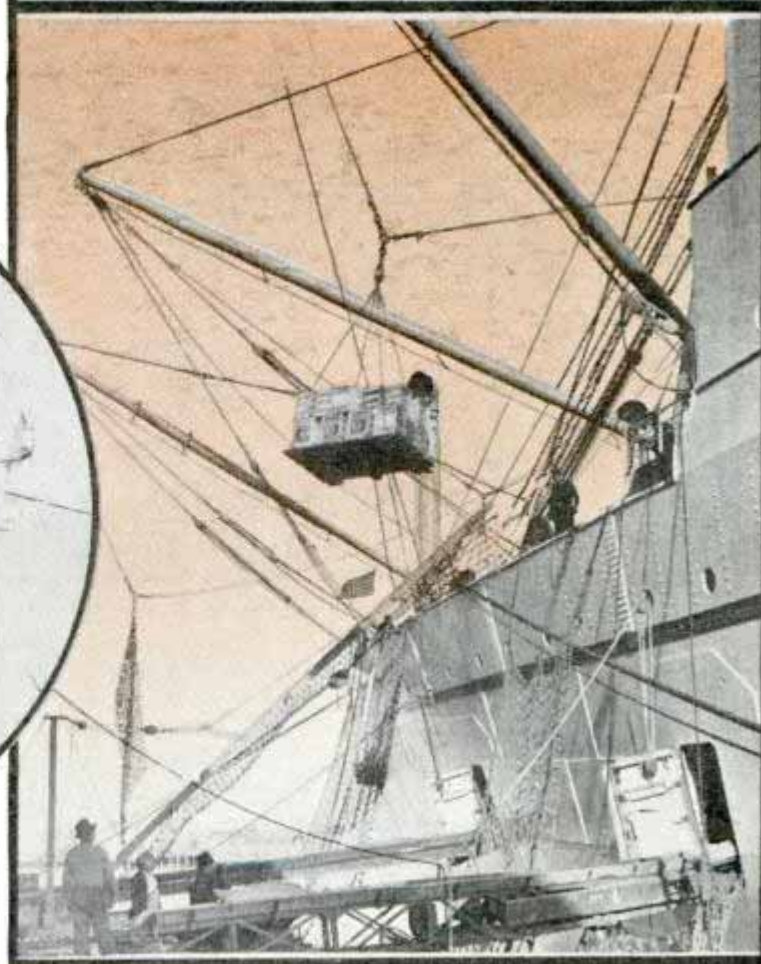
Top, engineer at throttle. Bottom, working cargo in port. Circle, opening valve to blow out tubes of boiler to remove scale
