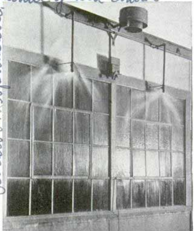
Automatic sprays in action to protect windows against heat from fire next door
