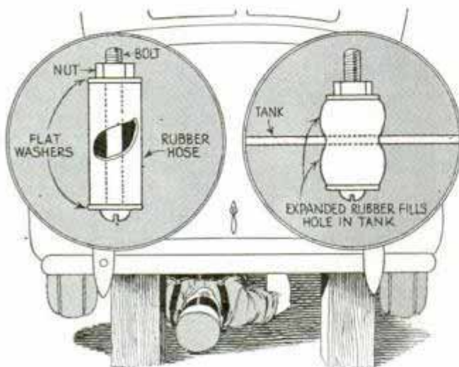
Expansive rubber plug seals puncture in gasoline tank until permanent repair can be made
