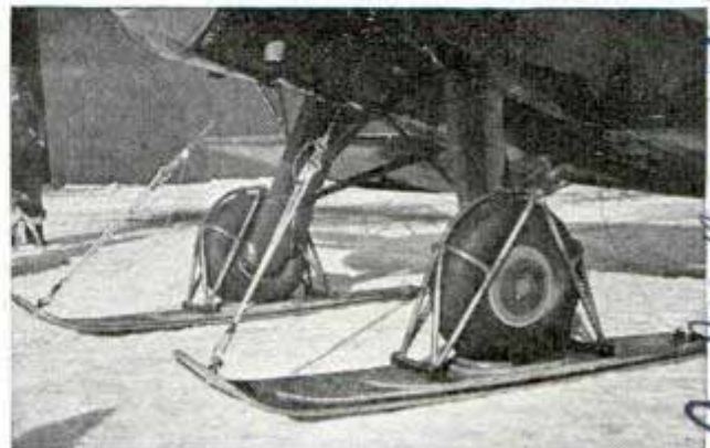
Frame of chrome alloy tubing, quickly installed, puts winter skids on plane without removing wheels
