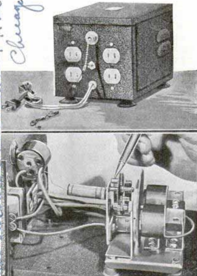
Top, flasher unit. Bottom, mechanism and wiring of handy sign lamp control
