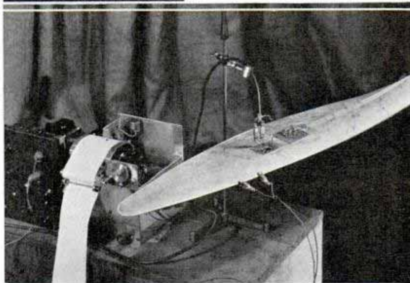
Apparatus, top, for calibrating and testing microphones. Center, sound-cell mounting in microphone. Bottom, measuring bending and torsional strains with aid of crystals and pen recorder
