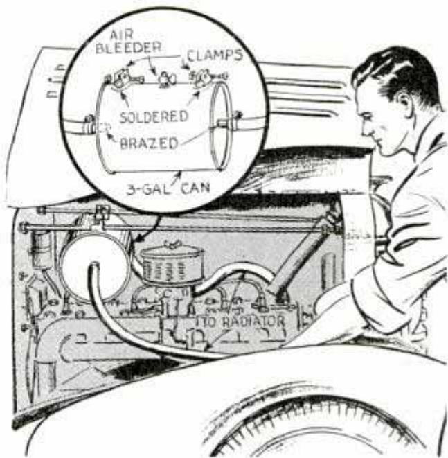
Auxiliary tank increases radiator capacity of car when pulling trailer over mountain roads
