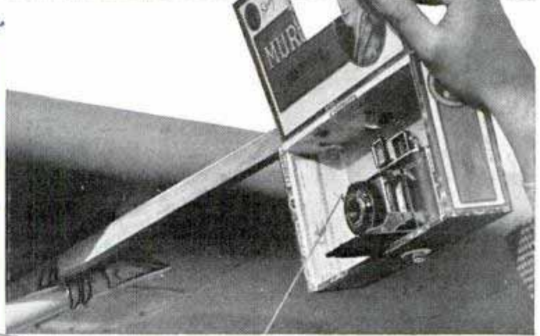
Top, pilot pulls cord tripping shutter of camera to take his picture. Below, camera mounted in cigar box fastened to wing
