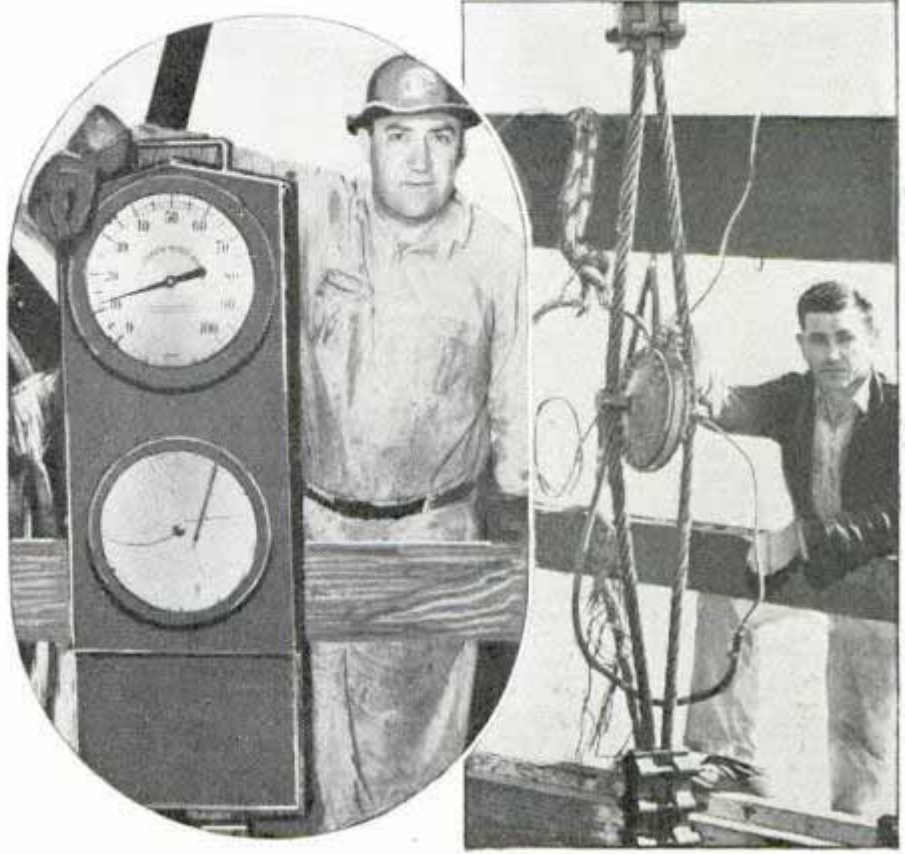
Tension on steel line and drum, right, is transmitted by hydraulic line to dial at left which shows pressure on drill in oil well
