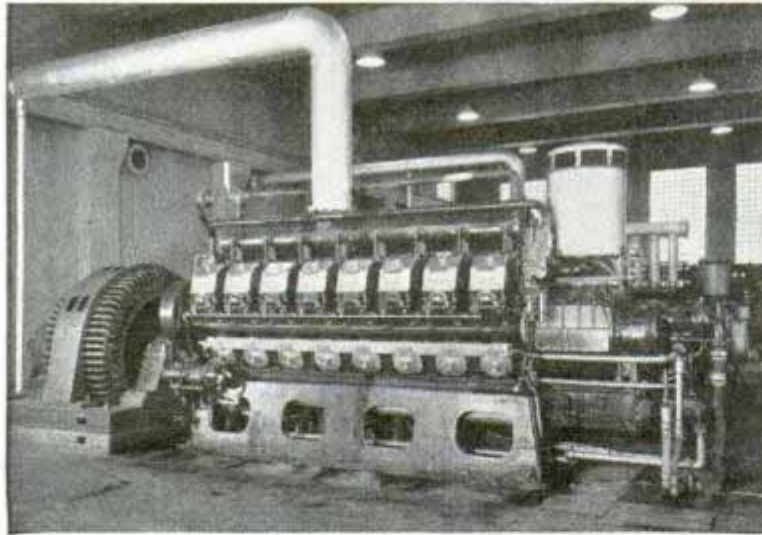
Top, Diesel engine assembly department in a General Motors plant. Bottom, sixteen-cylinder Diesel operating a 1,000-kilowatt generator
