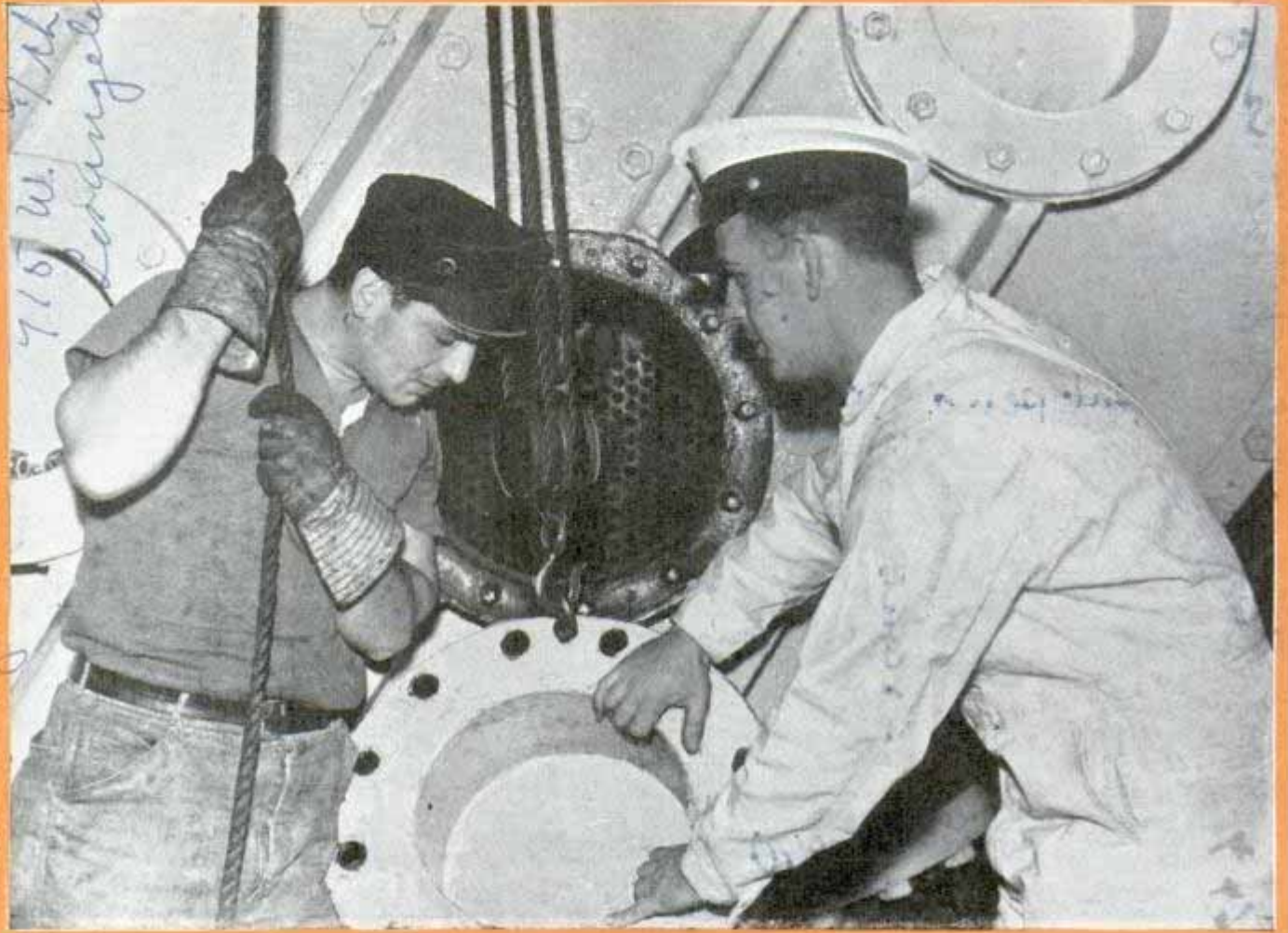
Removing heavy door from main condenser of ship's engine to inspect interior. Careful inspection frequently discloses trouble that might create an emergency at sea
