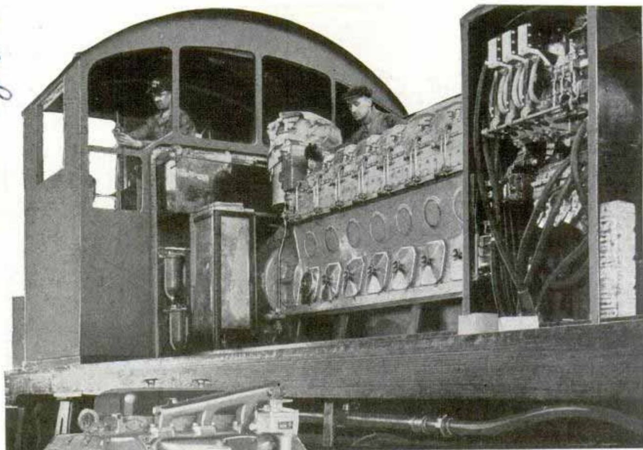
Top, closeup of Diesel-powered switch engine. Bottom, latest type of Diesel power plant, fully equipped
