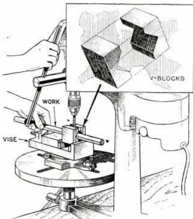
Two V-blocks clamped in vise hold rough work so it can be drilled through without damaging blocks
