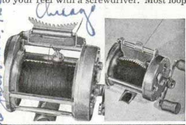
Right, the teeth set to catch snarls; left, in position for taking up slack after "brakes" are applied
