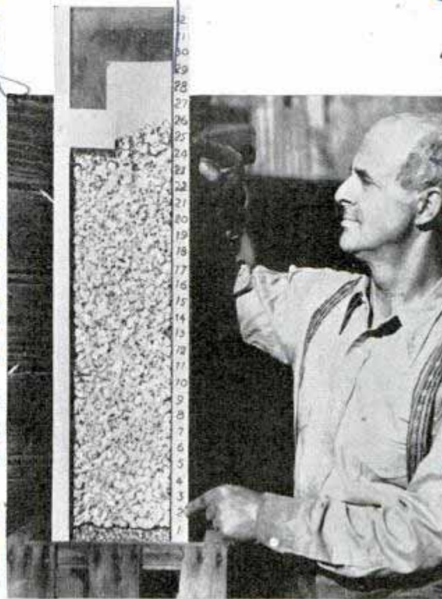
Popcorn measuring device which shows quality based on popping characteristics
