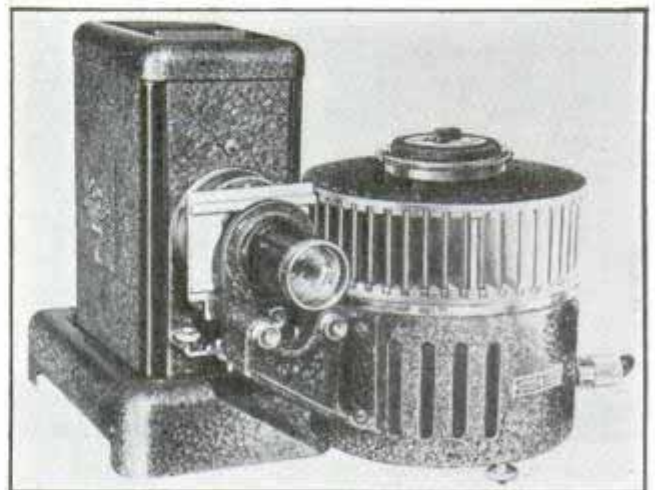
Forty-eight slides arranged in proper sequence in rotary magazine are fed automatically to projector
