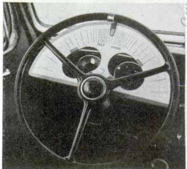
Curve meter mounted on dash aids engineers in surveying California highways
