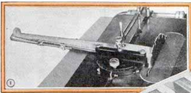
Miter gauge is set and table is tilted 2° for cutting upper end of leg
