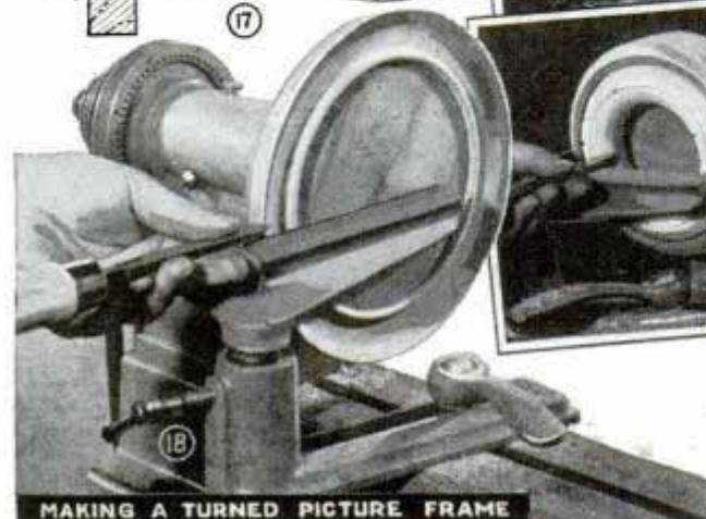
MAKING A TURNED PICTURE FRAME
