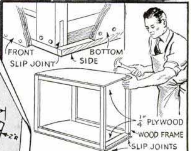
THE PLYWOOD HAMPER IS BUILT ON A FRAME
