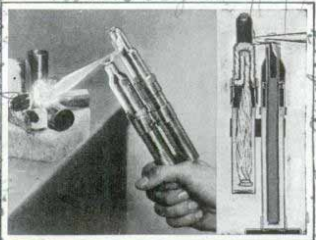
Pocket soldering lamp produces blue flame under high pressure, hot enough to melt copper or brass. Upper cylinder is "carburetor," lower is "heater"
