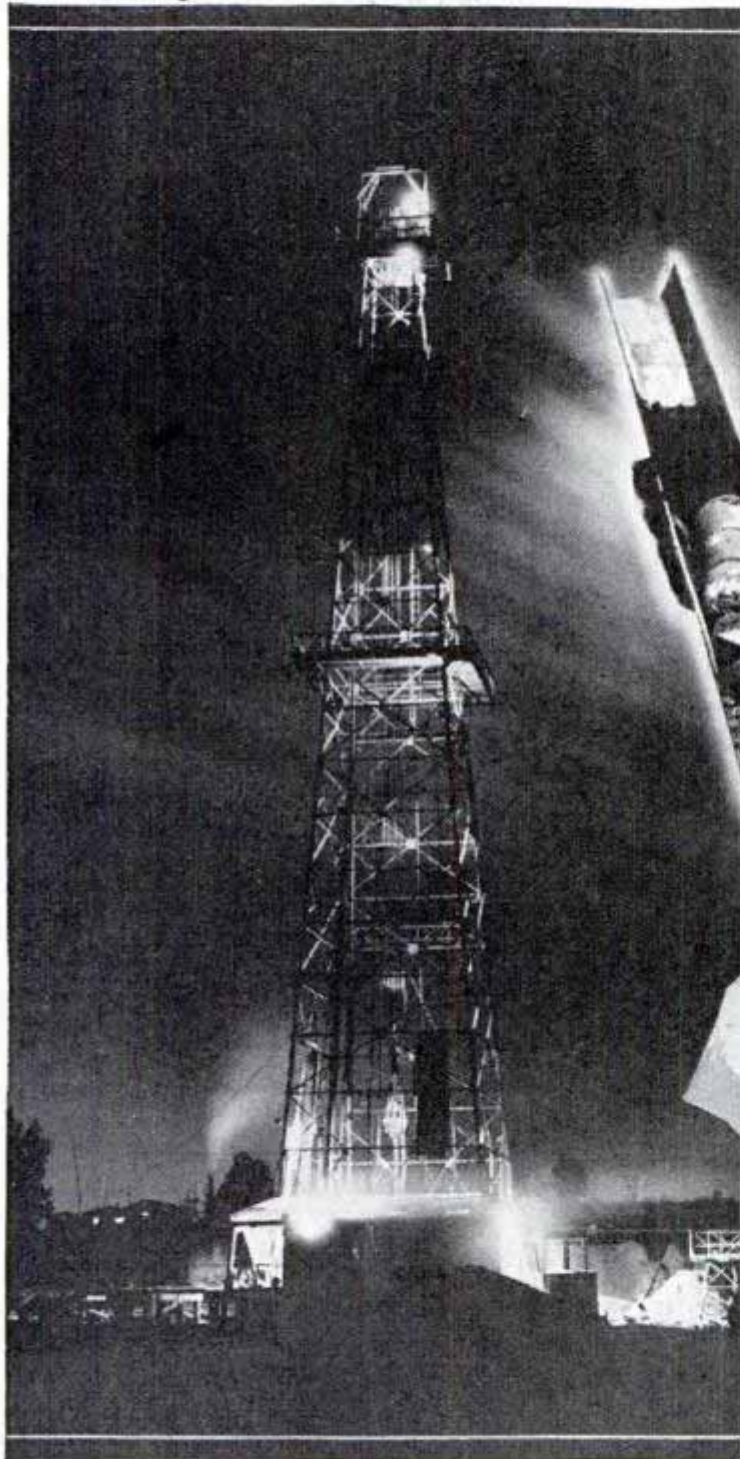
Left, night drilling scene. Right, samples of rock cut from bottom of well and brought to surface by coring machine that drops down inside drill pipe
