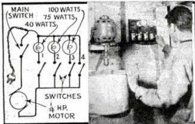
Rheostat consisting of three electric lamps used successfully to control speed of \frac{1}{4} -hp. motor
