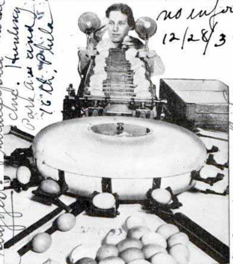
This woman operator finds it easy to grade eggs with the aid of this machine which turns out ninety per minute
