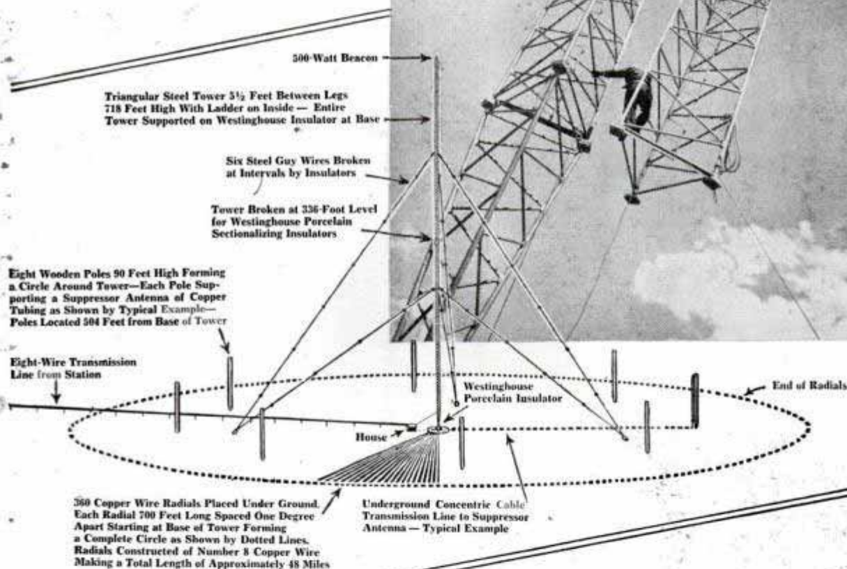
Top, section of lofty antenna being hoisted. Bottom, sketch of antenna system designed to improve radio broadcast service
