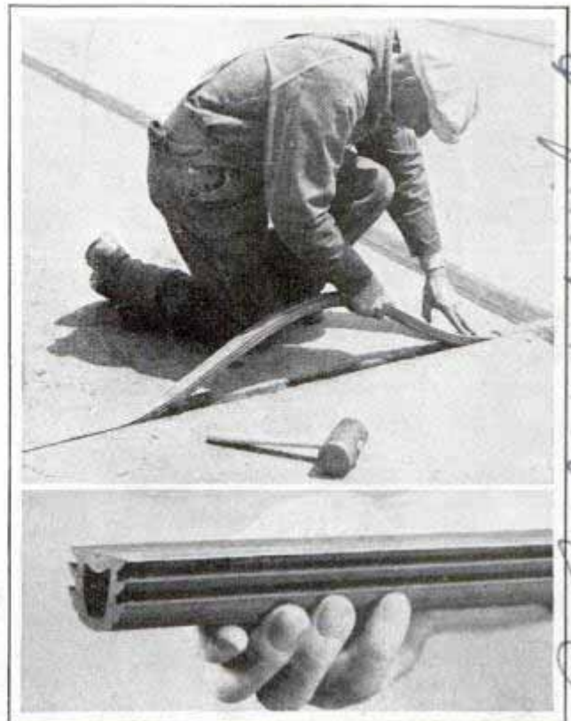
Laying the rubber expansion strip in joint of pavement, and closeup showing its moisture-proof design
