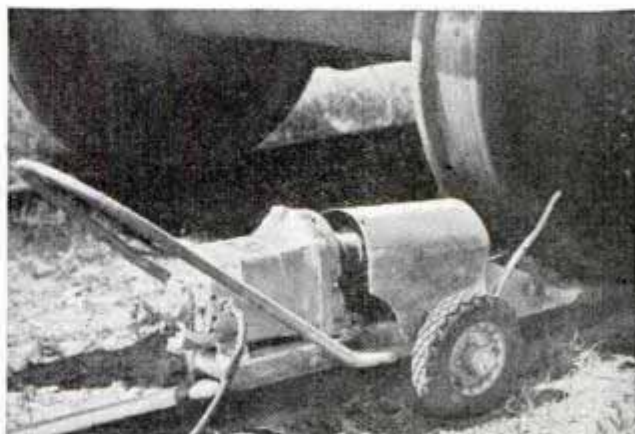
Small one-quarter horsepower device which easily shifts loaded freight cars in railroad yards by rooting under the wheel
