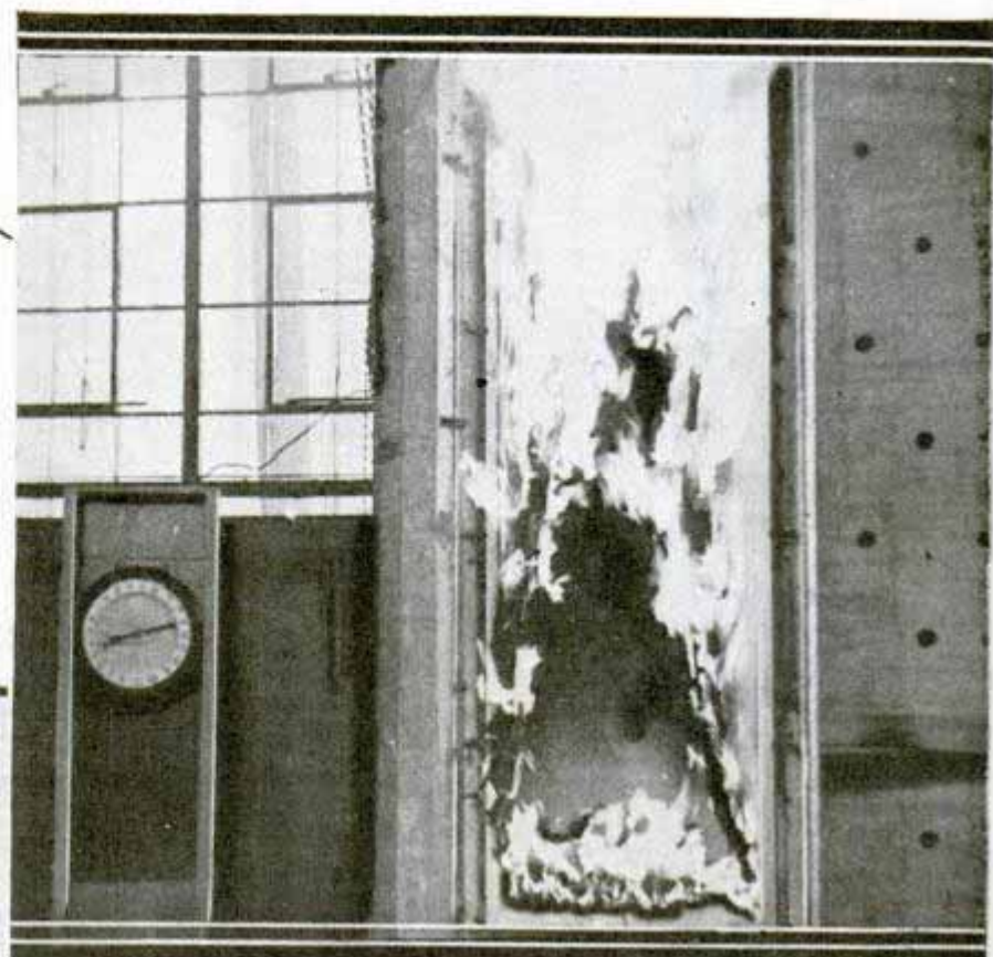
Left, testing door treated with fire-resistant chemicals. Ability of timber to withstand strain is important because intense heat exaggerates faults. Right, fire-treated wall panel fails in oven test
