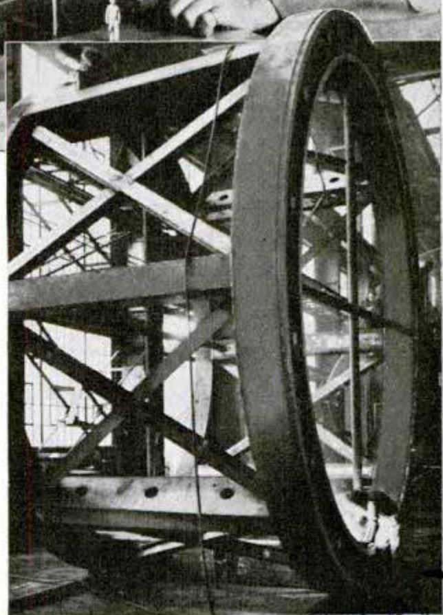
Mr. Tolmie Top, midget figure shows relative size of telescope mounting. Bottom, welding giant prime focus ring of telescope
