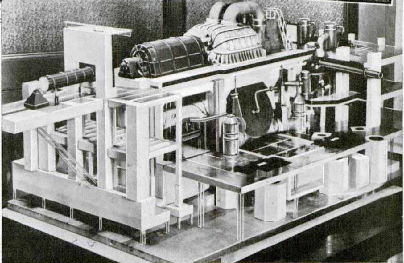
Top, turbo-electric generating plant built with aid of wood-and-celluloid model. Bottom, the model of turbo-electric generating unit, with celluloid used in floor to reveal structure of foundation
