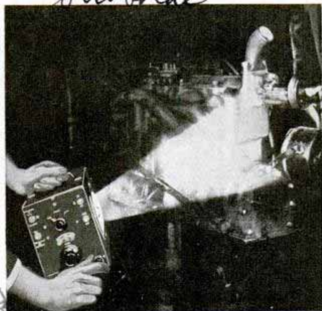
Portable stroboscope slows motion of engine fan for inspection while it really runs at full speed
