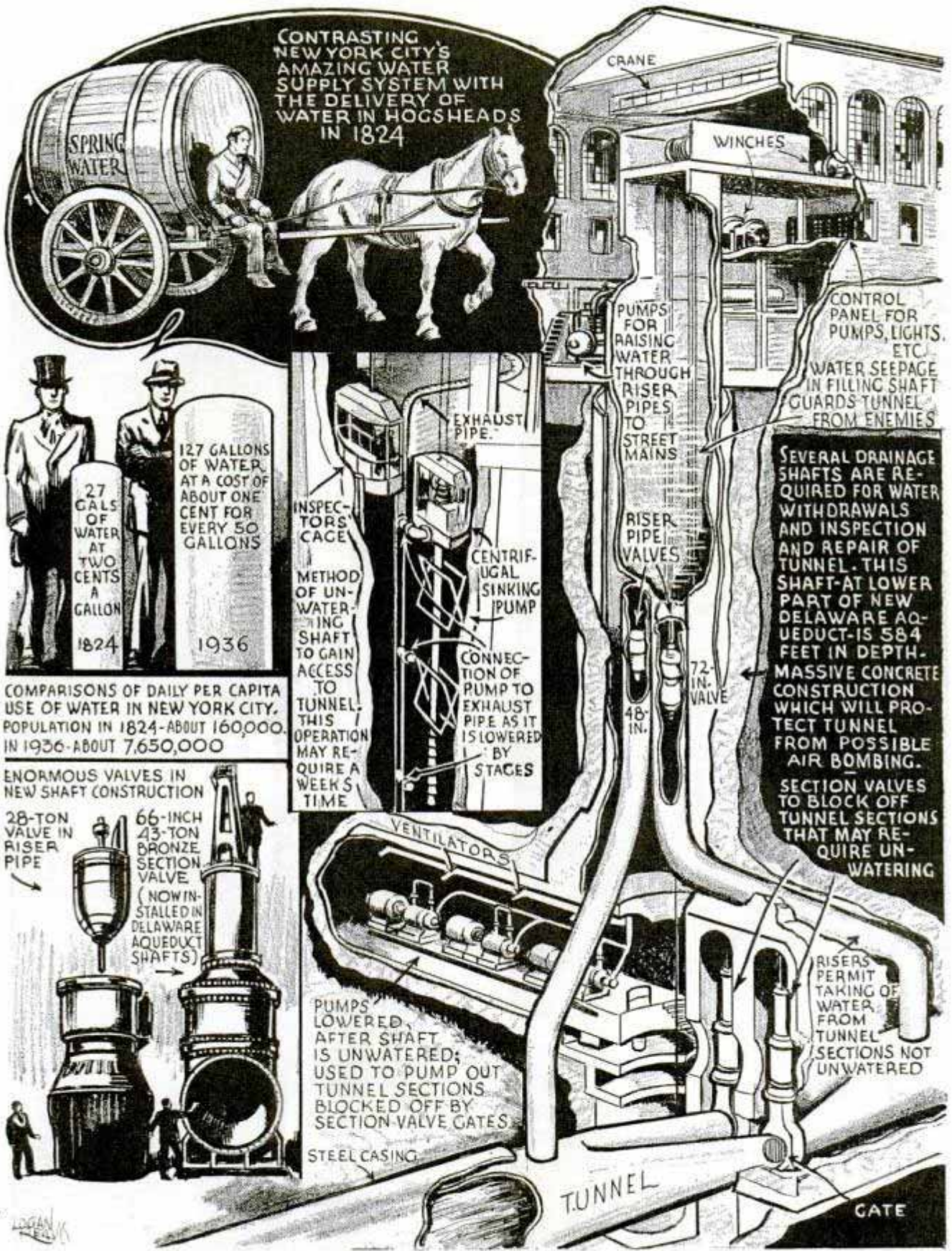
New York's $272,587,000 Delaware aqueduct, designed to supply ten million persons with water within ten years, is begun with driving of a shaft, fourteen feet in diameter, which pierces a mountain. Upper left, note how use of water increased as price dropped. Other drawings show features of the shaft which will tap the water supply in a giant tunnel. Massive concrete construction will protect water system from bombs dropped by enemy planes
