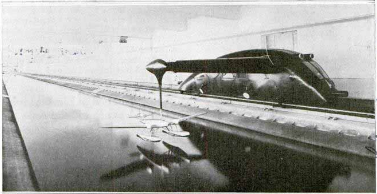
High-speed streamline car tows model seaplane in 500-yard test basin near Rome while instruments and observers check its performance in the water. Car is capable of eighty-five miles an hour
