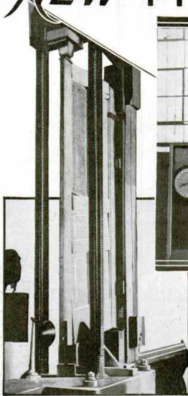
Left, testing door treated with fire-resistant chemicals. Ability of timber to withstand strain is important because intense heat exaggerates faults. Right, fire-treated wall panel fails in oven test
