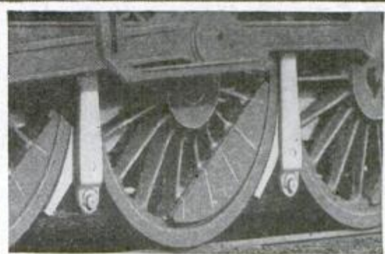
BRAKE SHOES are jammed against racing drivers by compressed air power for smooth, safe stops.
