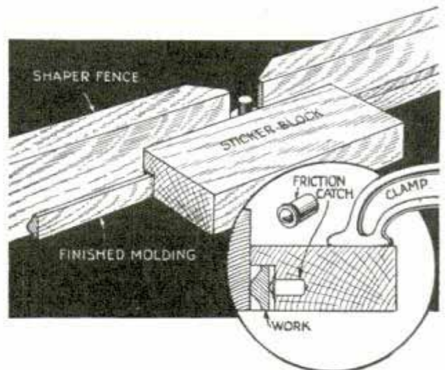
Friction catch in shaper sticker block takes up play caused by slight variation of thickness in stock
