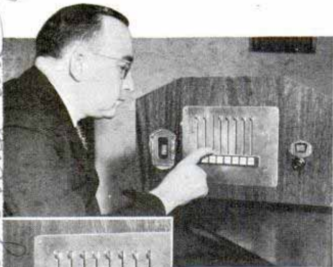
Levers select television and sound frequencies automatically; dials used only for adjusting levers. Left, set screws, under station name plates, for locking in desired frequencies
