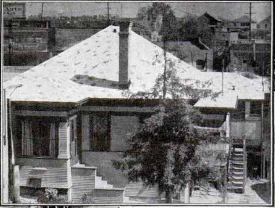
Blinds coated on outside with aluminum paint reflect the heat and help keep house cool, as does a light-colored roof
