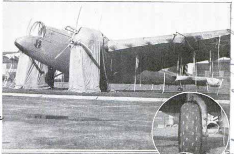
Stove under tent warms engine for quick takeoff. Steel cleats in tires at right aid traction
