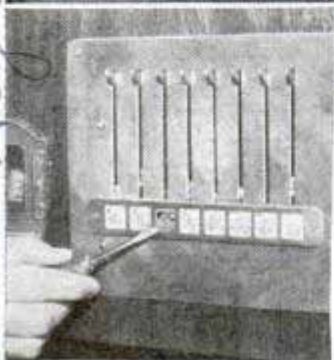
Levers select television and sound frequencies automatically; dials used only for adjusting levers. Left, set screws, under station name plates, for locking in desired frequencies
