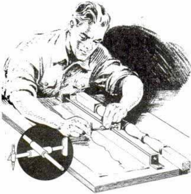
You can trace the profile of a turning on a piece of cardboard in a jiffy with this simple tool
