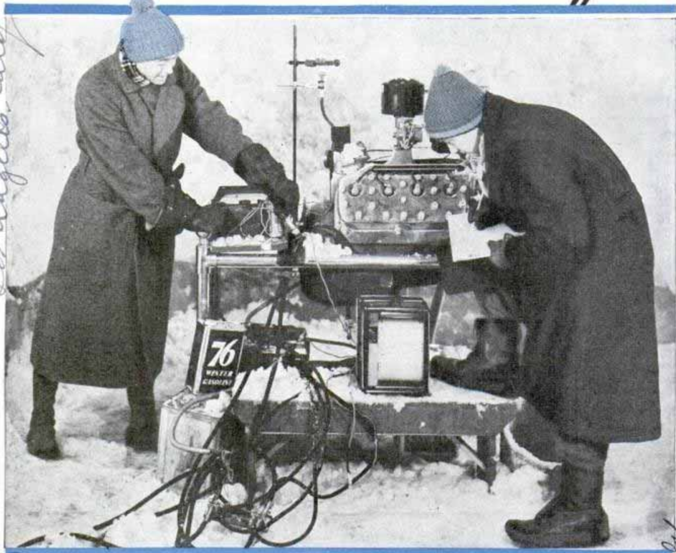
Union Engineers testing oil and fuels in sub-zero temperatures of a cold-weather laboratory. These tests show how lubricants will act in motor on severest winter days Courtesy Union Oil Co.
