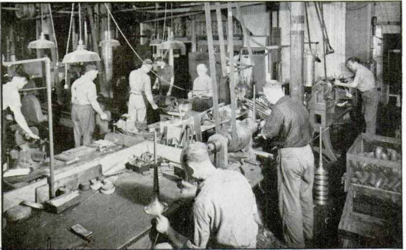
Briescher Here is another step in the manufacture of musical instruments. In this department the workers are shown forming bells for trombones.
