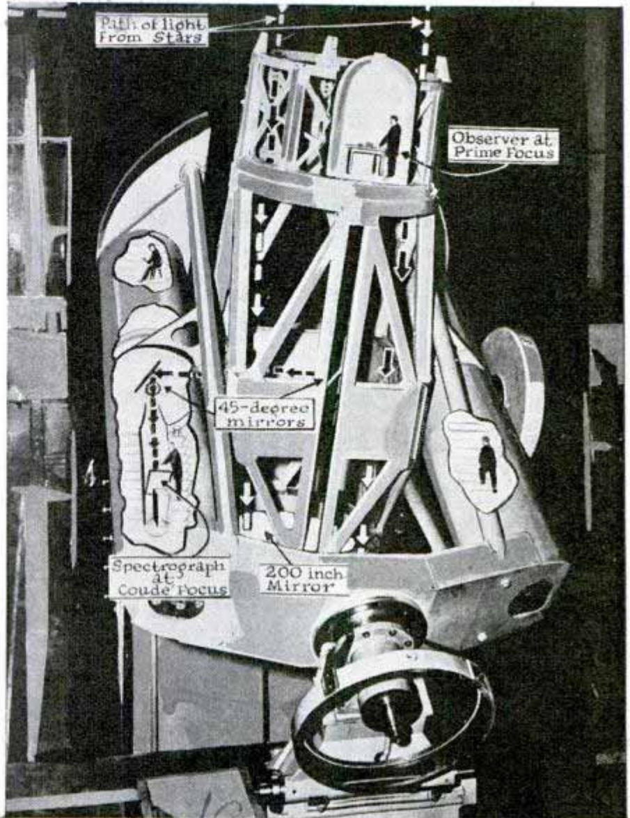
Right, diagrammatic view of model shows how observers will ride inside giant telescope
