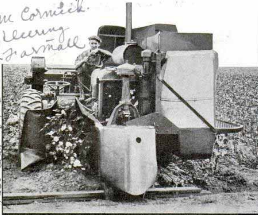
Here is the single-row cotton picker, undergoing tests in field. Its capacity is about one-half acre per hour, much faster than human workers
