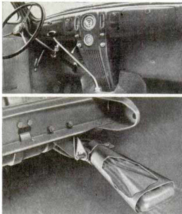
Top, grille extending from instrument panel to transmission housing in Lincoln-Zephyr. It houses radio and heater. Bottom, new exhaust pipe of Cadillac and LaSalle permits smooth flow of gases and reduces exhaust noise
