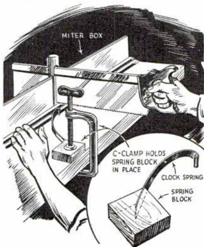
Small work is handled easily in a miter box without "jumping" when this spring is used
