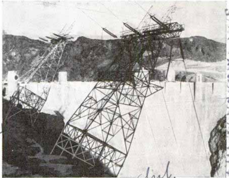
These leaning towers of steel perched over the brink of Boulder canyon shoulder the cables that start power flowing from dam to metropolis
