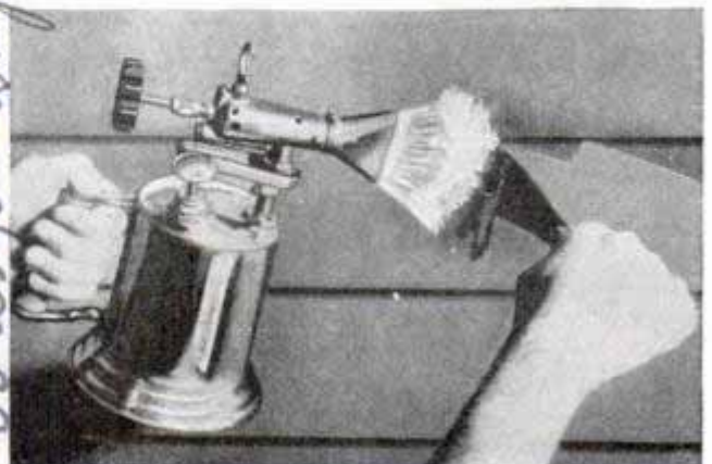
Burning paint with flame spreader on blowtorch
