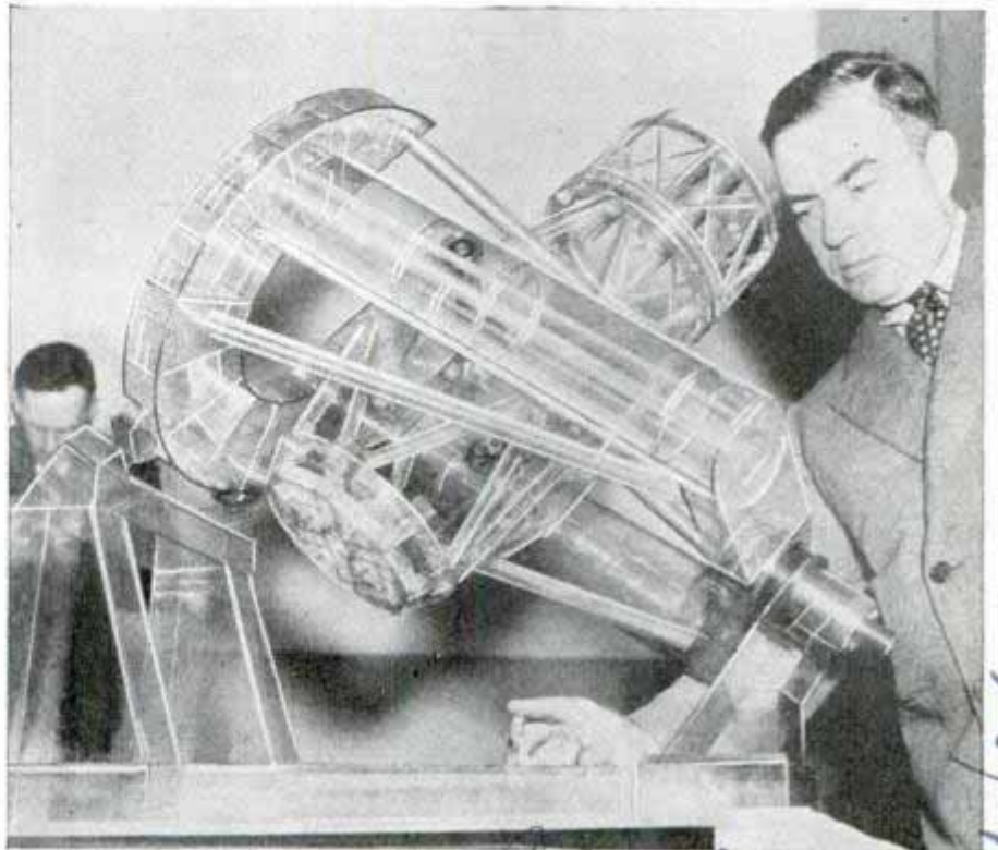
Scale model, made of glass, of the revolving frame for the world's largest telescope. The actual frame will be of steel, five stories high
