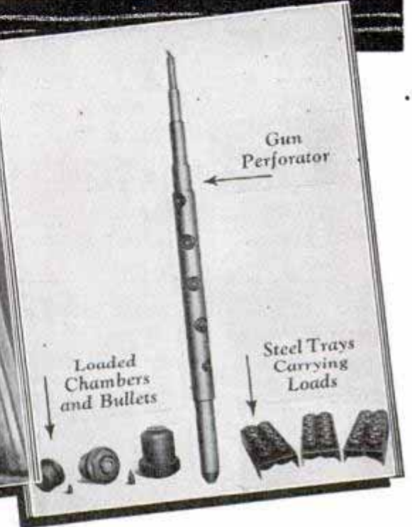
Sketch shows how bullets are fired from gun in well by remote control in truck. Photo, left, shows gun ready for lowering. Right, parts of the oil-well gun
