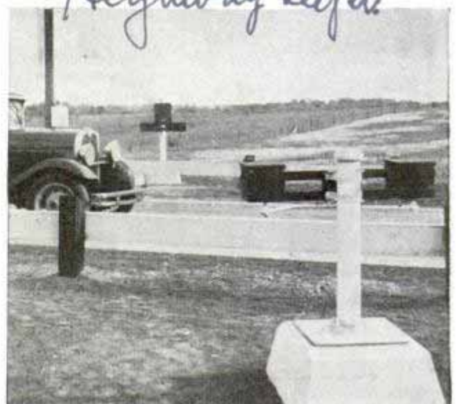
Passing vehicles are counted as they interrupt light beam focused on photo-cells on arms of post
