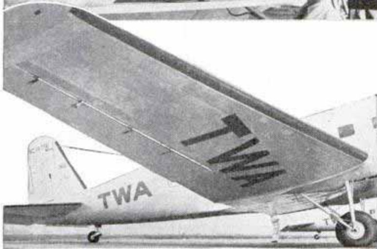
Left, three views of rubber overshoes attached to edge of wing, fin and stabilizer. Right, propeller guarded by cone-shaped spinner and by ring which distributes oil on blades to prevent ice formation
