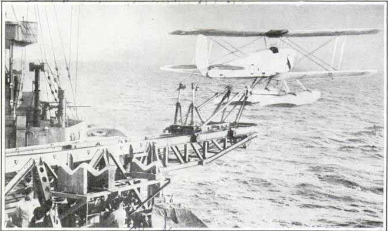
Here is the radio-controlled plane at the moment it was launched from British battleship by catapult. Note that the pilot is missing from the cockpit. Anti-aircraft fire failed to damage the robot craft
