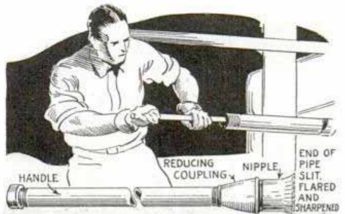
This flue cleaner "shaves" rust and corrosion from the pipes instead of scraping
