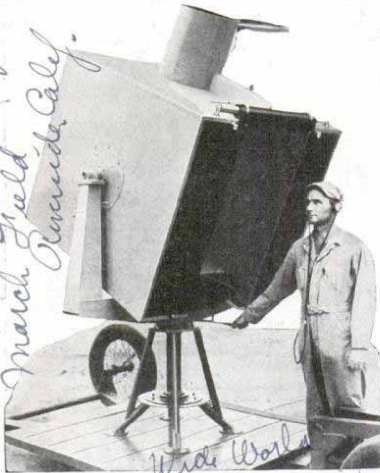
Camera obscura pointed at bombing plane in sky records its position when radio signal tells of missile dropped at target
