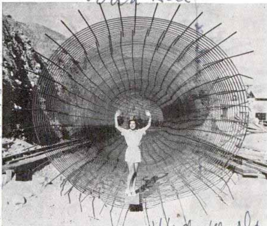
Figure of the girl helps to illustrate the size of iron-ribbed core of siphon which handles billion gallons of water per day
