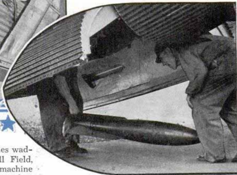
All photos by Harris and Ewing Loading bomb into Martin bomber, and machine gunner demonstrating mobility of his weapon
