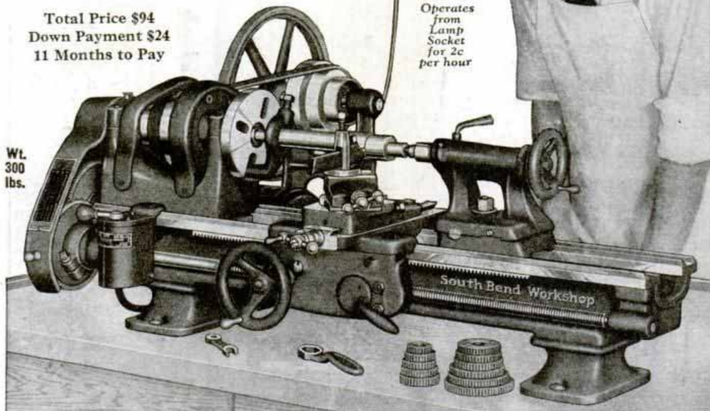
9 \frac{1}{2} " swing x 3' bed South Bend "Workshop" Bench Lathe, Complete with $94 Reversing Motor, Reversing Switch and Motor Drive, Wt. crated, 300 lbs.
