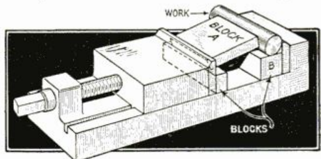
This Setup in a Milling Machine Eliminates Seating Work After Tightening It in a Vise
