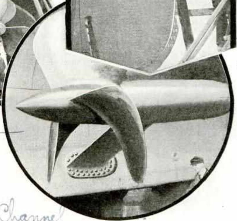
Streamlined Motorship, "Prince Baudouin," Which Carries Mail and Passengers between Dover and Ostend at Speed of Twenty-Seven Land Miles per Hour; Note Pointed, Trailing Stern and Two Rudders, One at Each End, Which Enable Craft to Make Complete Turn in Twice Her Length, or 720 Feet; Each of Her Streamlined Propellers Is Driven by a Twelve-Cylinder Diesel Engine of 8,500 Horsepower
