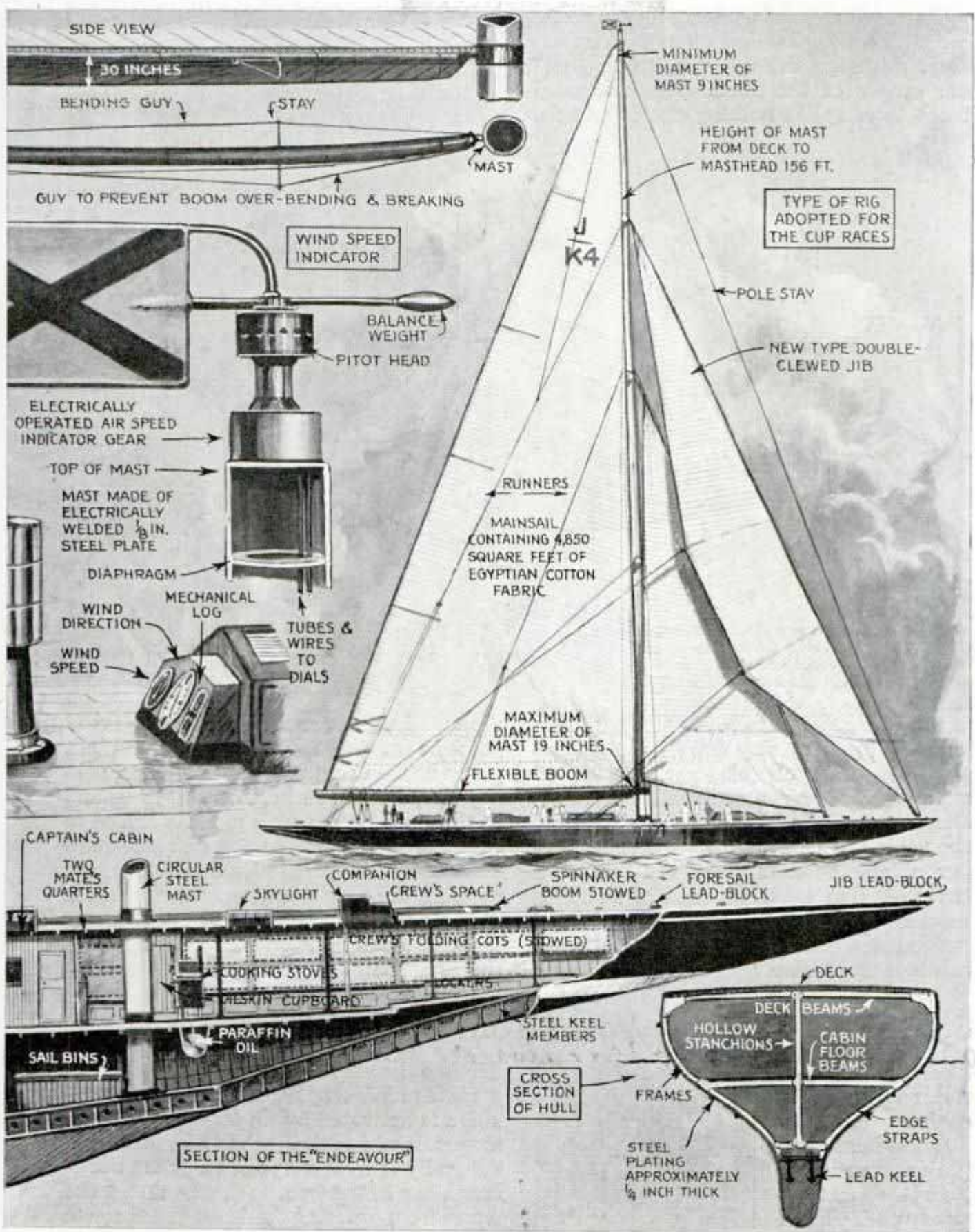
The "Endeavour's" Circular Mast, Weighing More Than 5,500 Pounds, Is Built Up of High-Tensile Steel Plating, One-Eighth Inch Thick and Electrically Welded; the Cutter Has a Racing Flag of Doped Canvas on a Tubular Frame and This Is Mounted on the Masthead on Ball Bearings and Connected with Recording Instruments Giving Wind Direction on a Dial Placed Before the Helmsman; There Is Also a Mechanical Log and a Wind-Speed Indicator Which Operates on Lines Similar to the Air-Speed Indicators with Which Aircraft Are Equipped
