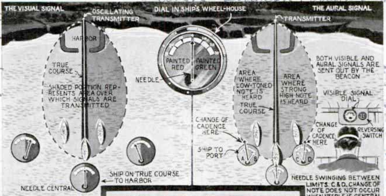
WITH THIS METHOD OF SIGNALING IT IS POSSIBLE TO NAVIGATE A SHIP IN THE THICKEST SEA FOG.
