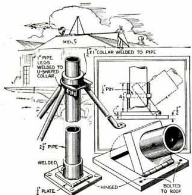
Wind-Sock Mast Attached to Hinged Base Is Lowered Easily for Adjusting the Sock
