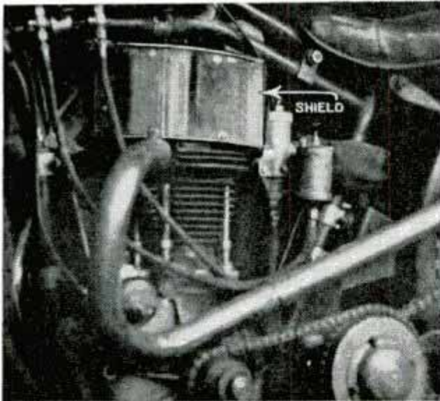
Fine Wire-Mesh Shield Keeps Dirt Out of Rocker-Arm Assembly on Motorcycle
