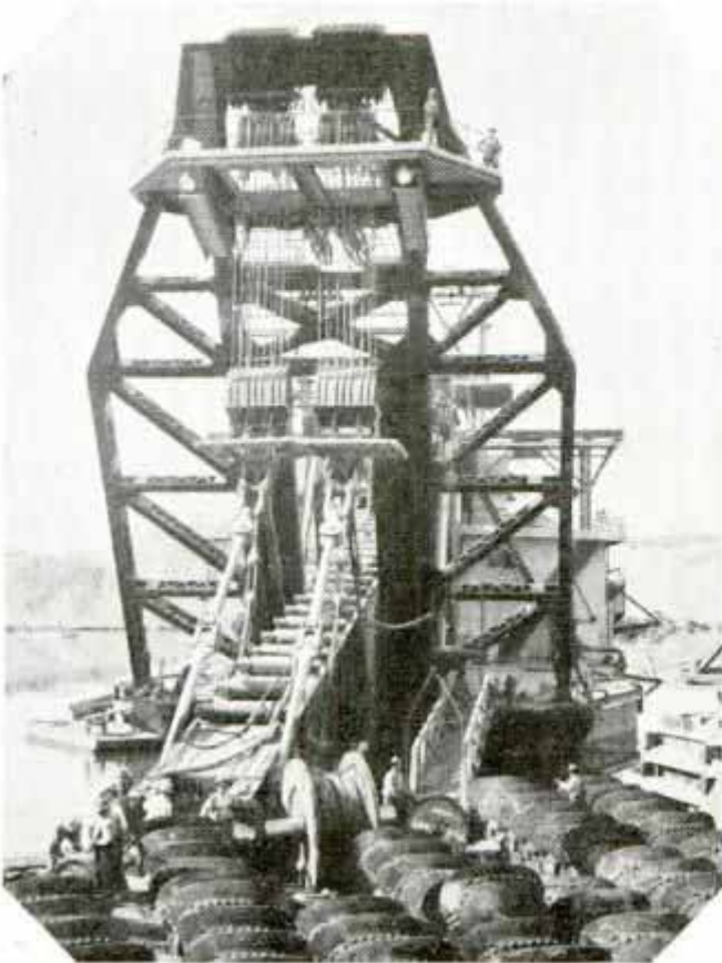
Left, Digging End of Dredge Before Buckets Were Attached; Fully Equipped, Dredge Weighs 3,500 Tons; Right, Endless Conveyor with Gold-Bearing Gravel Scooped from the Depths
