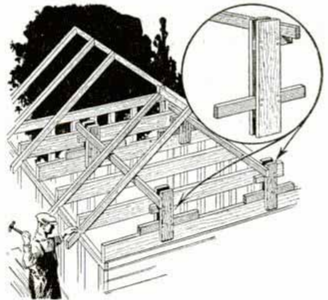
One Man Can Erect Rafters When Aided by These Wooden Supports
