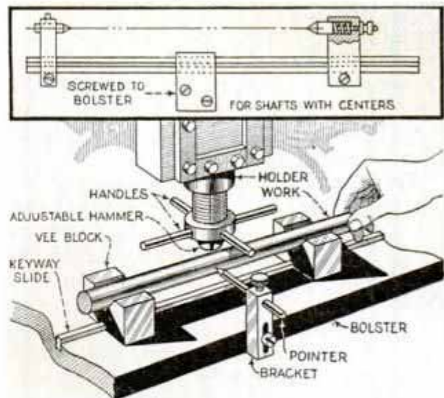
Simple Set-Up for Straightening Short Rods and Shafts in a Punch Press
