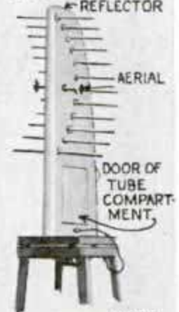
RECEIVER
