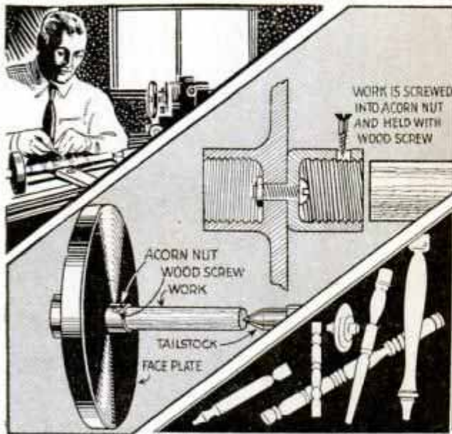
Acorn Nut Bolted to Lathe Faceplate Holds Small Stock When Turning Tiny Model Parts
