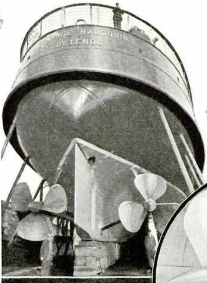
Streamlined Motorship, "Prince Baudouin," Which Carries Mail and Passengers between Dover and Ostend at Speed of Twenty-Seven Land Miles per Hour; Note Pointed, Trailing Stern and Two Rudders, One at Each End, Which Enable Craft to Make Complete Turn in Twice Her Length, or 720 Feet; Each of Her Streamlined Propellers Is Driven by a Twelve-Cylinder Diesel Engine of 8,500 Horsepower
