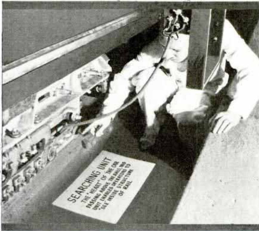
Top, Operator at Record Table in Detector Car Watches Tape for Flaws in Rail; Bottom, Operator Pointing to "Heart" of Detector
