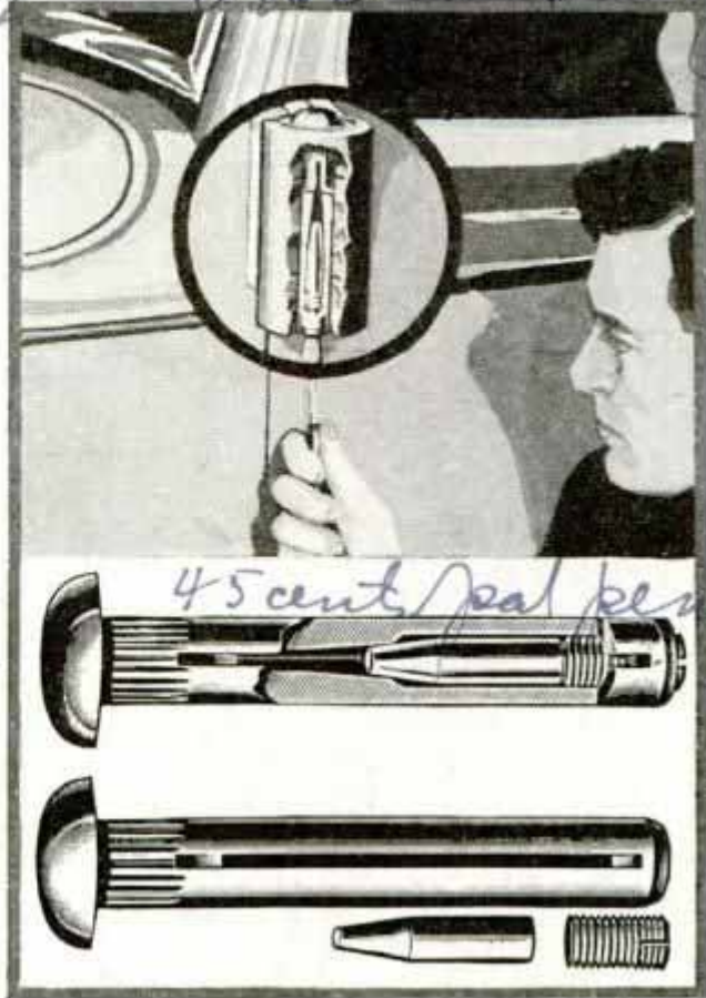
Cross-Section of Hinge Pin; Circle, Installation in Door of Automobile
