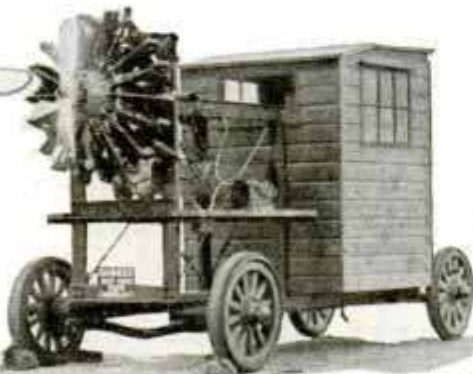
Wheeled Testing Block for Aircraft Motors Also Carries Small Mechanical Repair Shop
