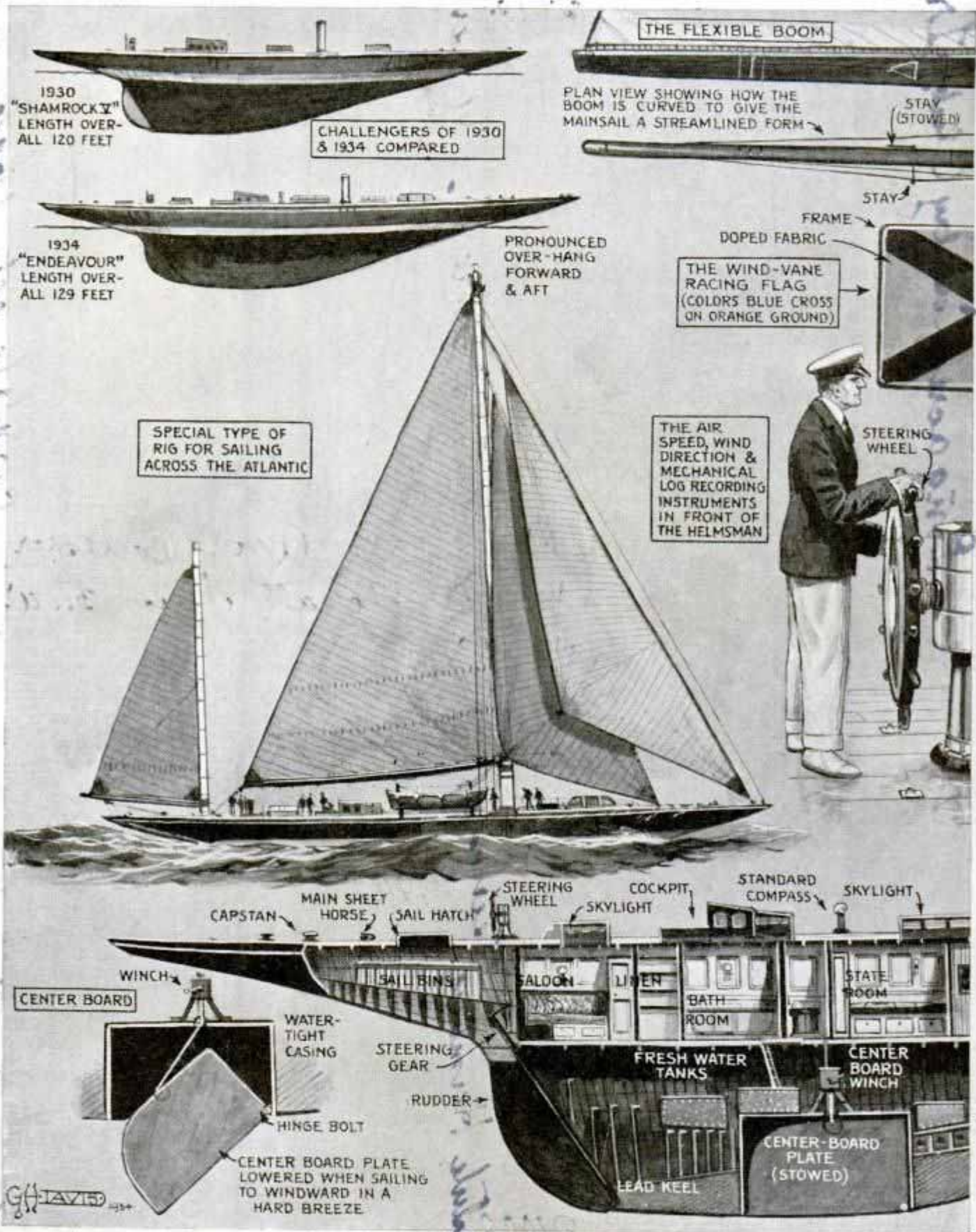
During More Than Eighty Years British Yachtsmen Have Made Fourteen Unsuccessful Attempts to Wrest the World's Premier Yachting Trophy from This Country; Diagrams Show Details of Construction of the "Endeavour," England's 1934 Challenger; Note the Pronounced Overhang Forward of the All-Steel Hull and the Flexible Boom Which Bends with the Curve of the Mainsail and Sets This Sail into a Streamline Form to Lessen Head Resistance; This Is the First British Challenger to Have an All-Metal Hull and the Construction Cost Was About $150,000
