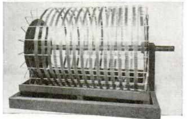
Reel Made of Tin Lids and Brass Rods Rotates Movie Film in Developing Fluid
