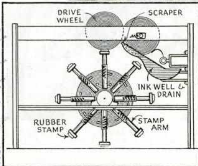
Stamping Machine Which "Walks" over Fruit and Diagram Showing the Method of Operation
