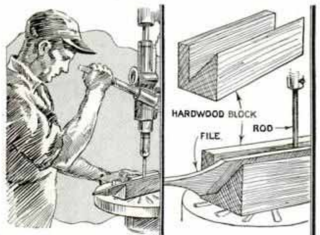
File Held at Angle in Hardwood Block Enables Use of Drill Press to Point Iron Rods
