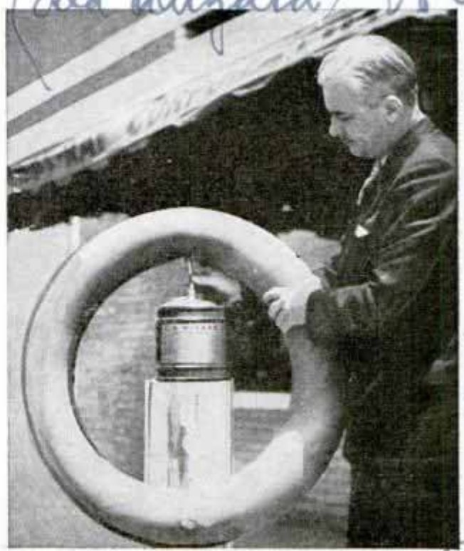
Equipment for Inflating Inner Tube with Reddish Vapor to Reveal Punctures
