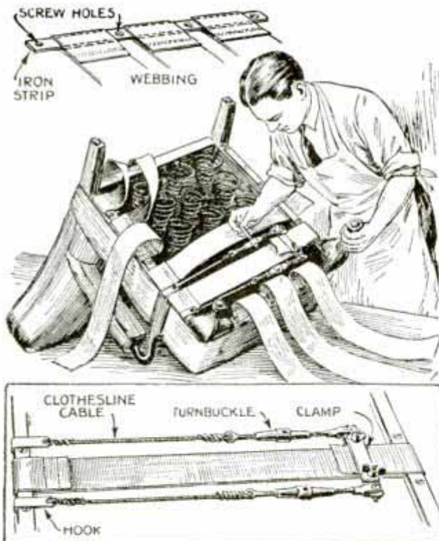
Iron Strips Hold Tightly Stretched Webbing on Frame of Upholstered Chair Seat
