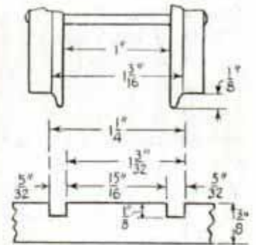
⑤ CROSS-SECTION OF FLANGE GROOVE IN CROSSING BLOCK
