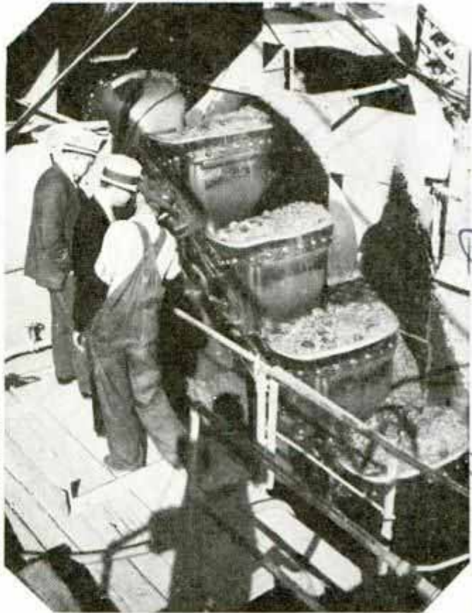
Left, Digging End of Dredge Before Buckets Were Attached; Fully Equipped, Dredge Weighs 3,500 Tons; Right, Endless Conveyor with Gold-Bearing Gravel Scooped from the Depths
