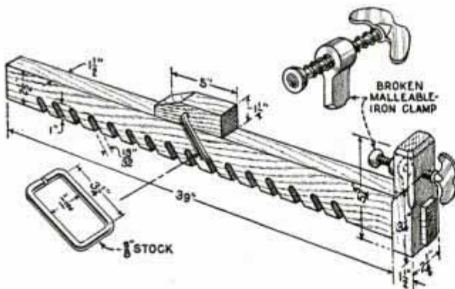
Woodworkers' Bar Clamp Made from Hardwood and Screw from Broken C-Clamp
