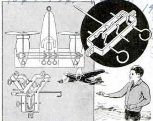
Circle, Transmission for Model Planes; Left, How Transmission Is Installed in Multi-Motored Craft
