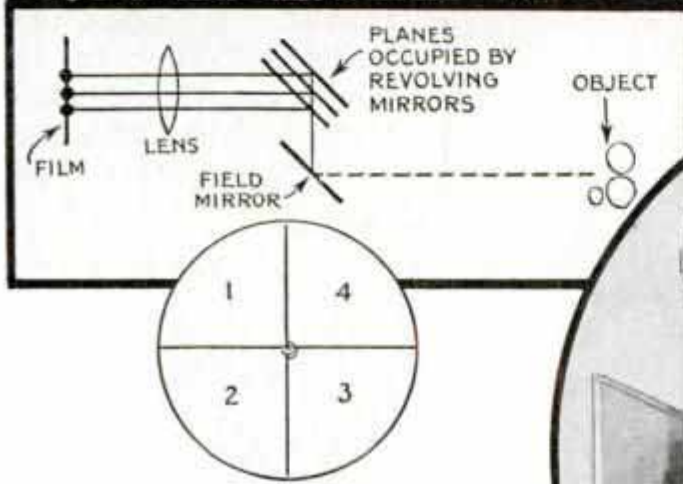
Circle, Three-Dimension Movie Camera; Bottom, Left, Illustrating Revolving Mirror Principle; Below, Strip Showing How Four Frames Snapped at Different Angles Take on Three-Dimensional Properties When Run through Projector
