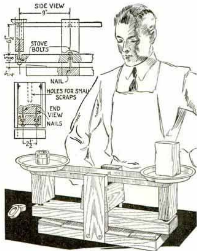
These Balance Scales Weigh Quite Accurately with Weights Made of Lead-Filled Pipe Nipples
