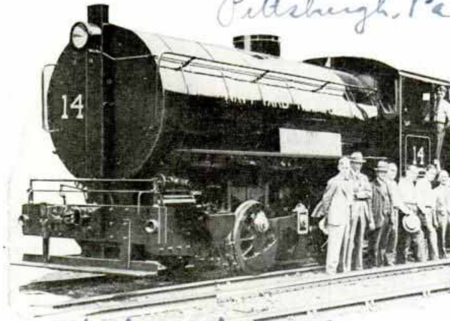
Fireless Geared Locomotive Whose Tank Is Charged with Enough Water and Steam from a Stationary Boiler to Operate for Several Hours
