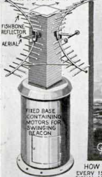
TRANSMITTING REFLECTOR AERIAL SYSTEMS SWING RIGHT & LEFT OVER A TOTAL ARC OF 6 DEGREES
