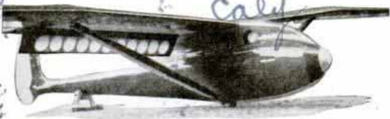
D10 Glider Equipped with "Air Brake" on Trailing Edge of Wing to Slow Down Craft for Safer Landing
