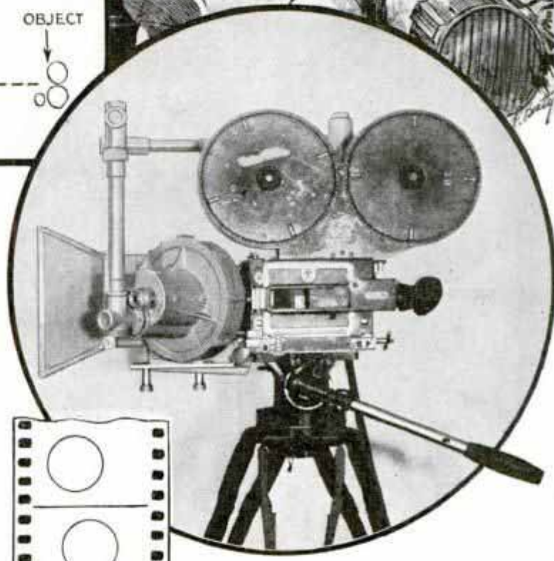
Circle, Three-Dimension Movie Camera; Bottom, Left, Illustrating Revolving Mirror Principle; Below, Strip Showing How Four Frames Snapped at Different Angles Take on Three-Dimensional Properties When Run through Projector
