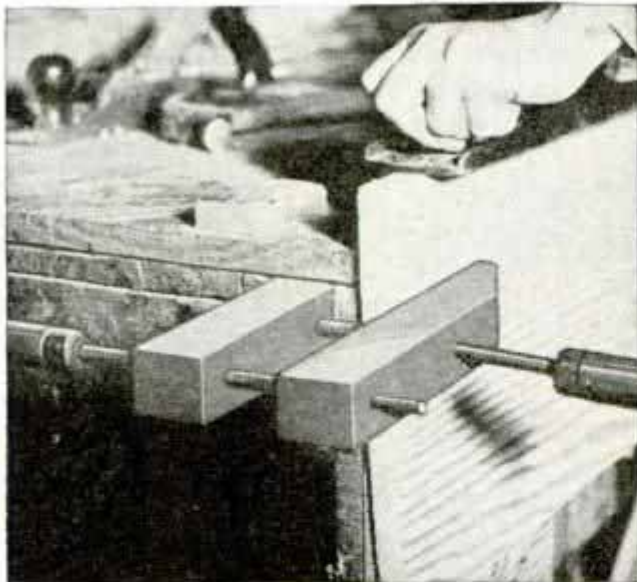
Woodworkers' Clamps Fastened to End of Workbench Serve as Emergency Vise for Large Panels
