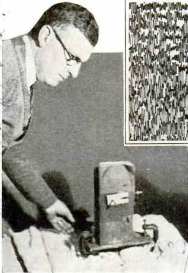
Seismograph Recorder and Lines Made by It from Which Weather Forecasts Can Be Made
