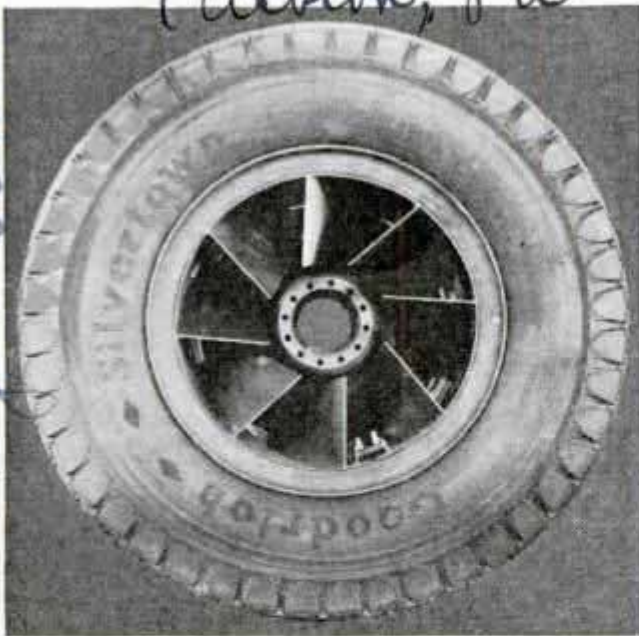
Fan Built Inside Auto Wheel to Lower Tire and Brake Drum Temperatures of Trucks and Buses
