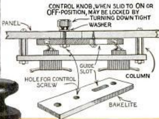
Above, Toggle Switch Ganged for Linking Two or More Experimental Circuits for Simultaneous Operation; They May Be Arranged to Close Together or to Close One Switch and Open the Other; an Escutcheon Plate May Be Made for Front-Panel Operation, and Many Other Variations Are Possible; Left, Isolantite Form for Winding Short-Wave Coils; the Handle at the Top Is Convenient for Inserting and Removing the Coil; the Flat Top Provides a Surface for Labeling; the Small Groove at the Bottom Is for Primary or Ticker Winding
