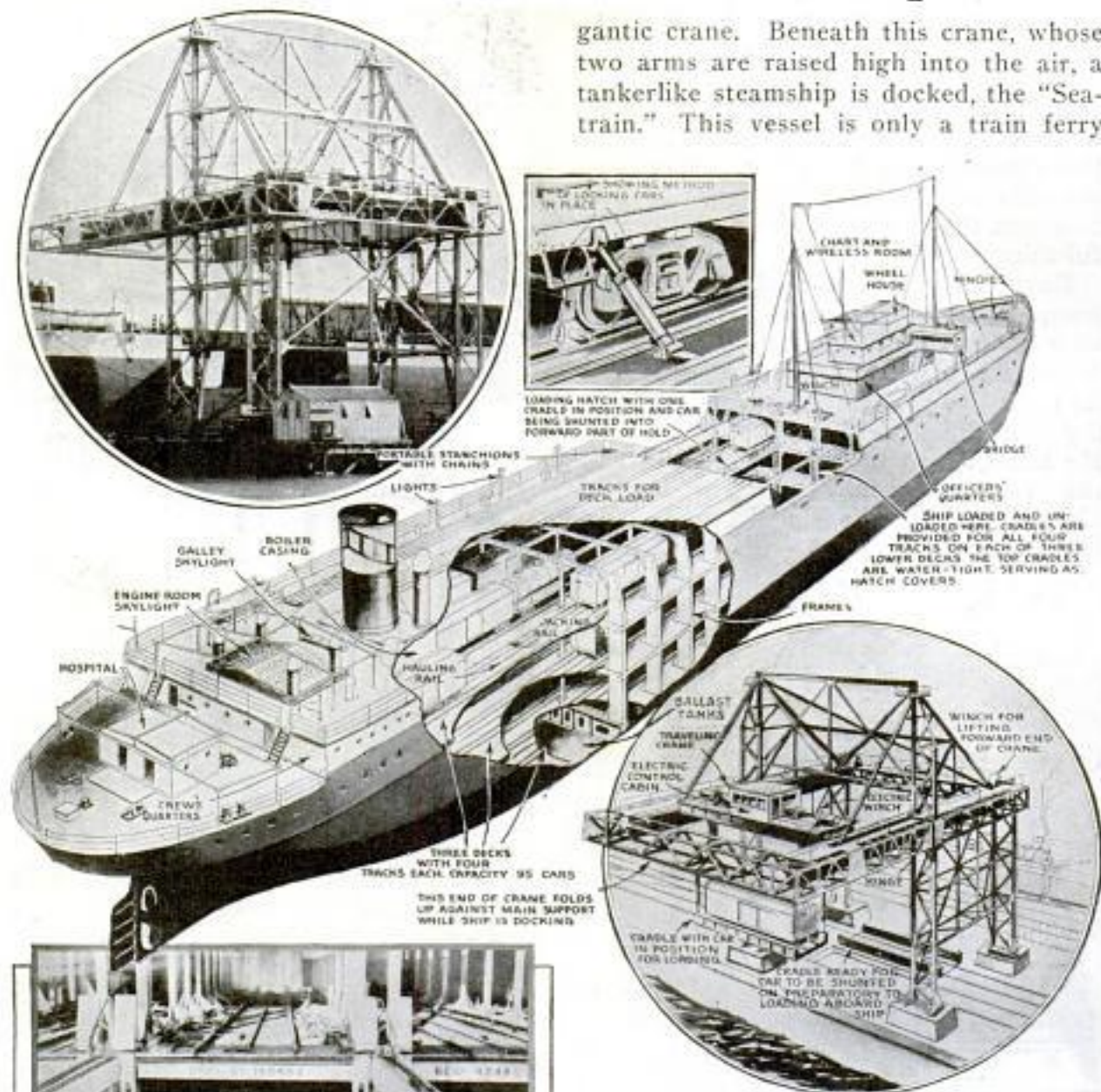
Diagram of Boat Which Carries Ninety-Five Railroad Cars, and Crane That Lifts Them; Left, One of Cars in the Hold
