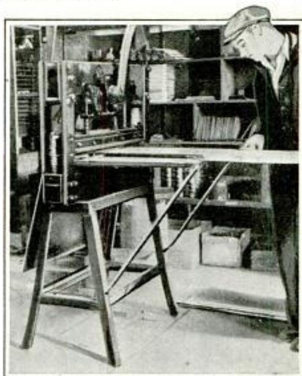
Machine Tables That Fold Down against the Legs Save Space in Crowded Shops
