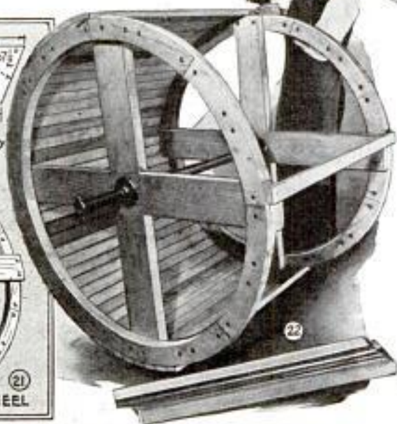
The Treadmill Makes Fun of Exercising; This One Is an Outside Wheel, but an Inside Tread Can Be Made by Increasing the Diameter
