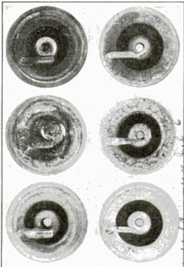
Inattention to Spark Plugs Results in Carbon Formations and Wearing Away of Side Wires
