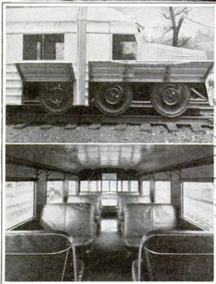
Top, Stainless-Steel Rail Car with Rubber Tires; Below, View of Front Trucks and Interior of the Coach
