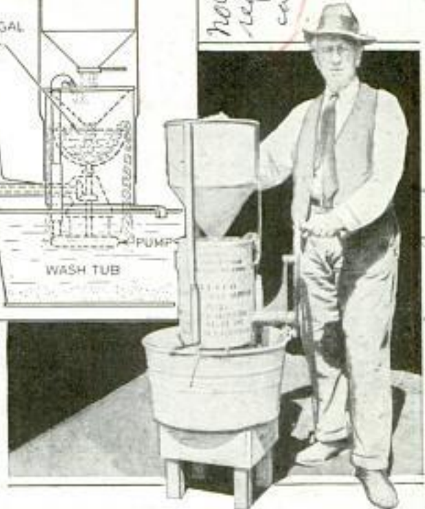
Little Water Is Required to Operate This Gold Washer Which Works Like a Cream Separator
