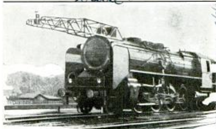
Frame Attached to Front of Locomotive Contains Wind Vane; Dial in Engine Cab Records Weather Conditions on Test Runs
