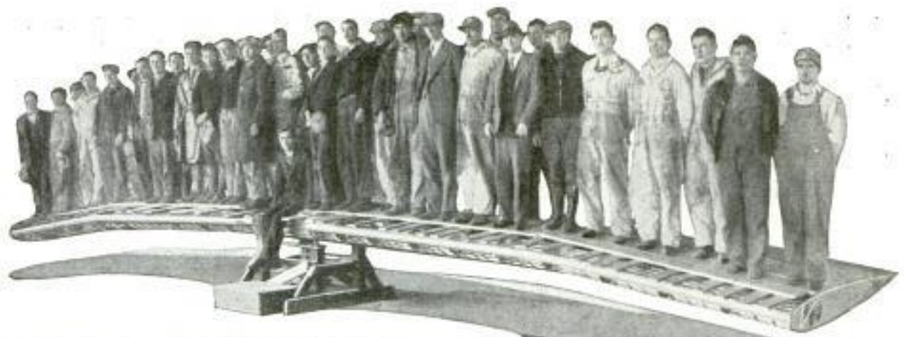
In Proportion to Weight, Airplane Structures Are the Strongest Known; This Wing Easily Carries the Load of Thirty-Eight Men without Evidence of Failure
