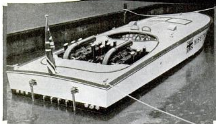
Diagram and Photo of "Miss England III." This Year's Challenger: Its Top Speed Is Estimated at 130 Miles an Hour
