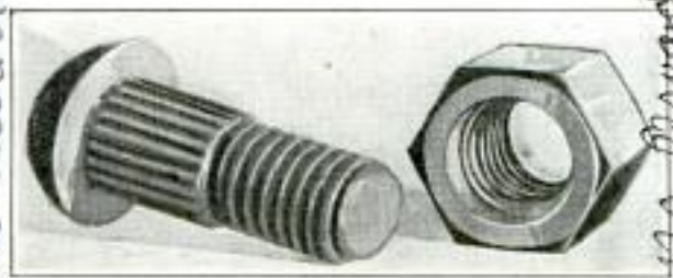
Rivet Is Driven In by Hand and Made Fast with Nut; No Heating Is Necessary
