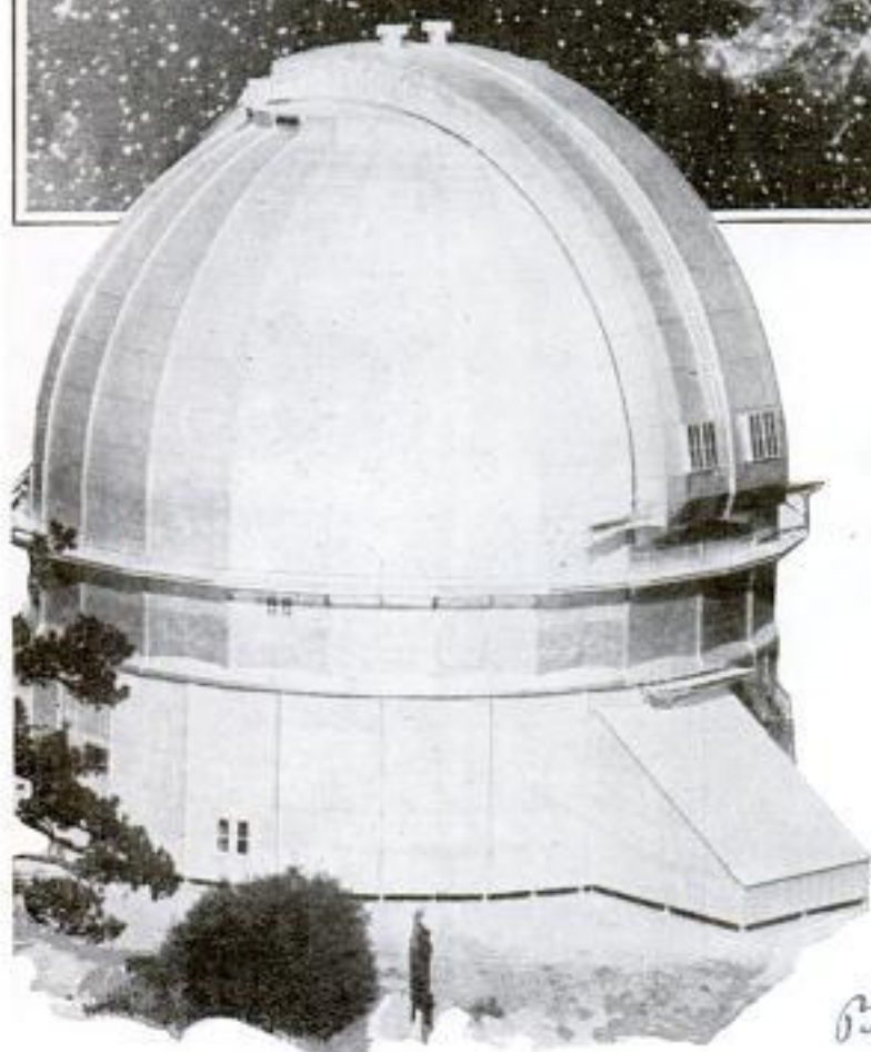
Above, Section of Sky Such as That in Which Stars Were Counted; Below, Mount Wilson Observatory
