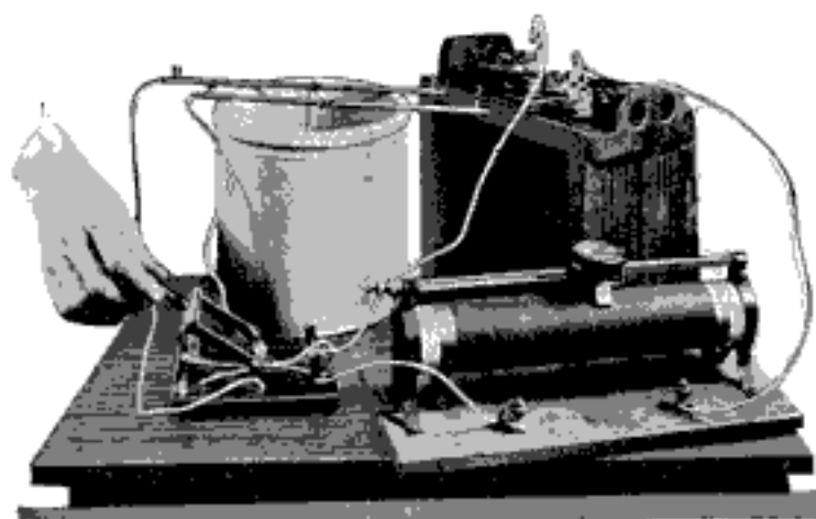
REVERSING CURRENT DURING ELECTRO-CLEANING PROCESS
