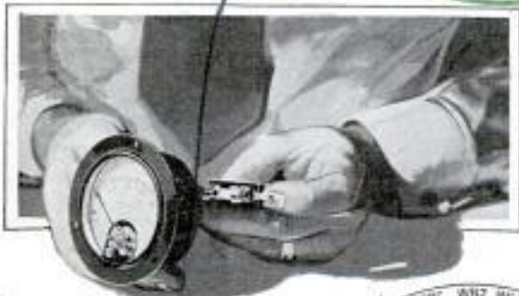
Above, 2 In. of Pencil Lead Makes Filament Resistor for 5-Volt Battery-Operated Tubes, Adjusted for Correct Voltage; Below, Small Fuse Protects Meter
