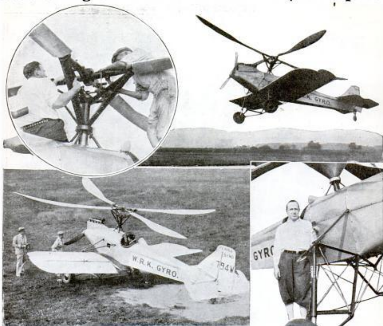
Gyroplane with Feathered Rotor Blades in Flight, Upper Right, and on Ground. Lower Left; Rigid Construction of Rotor, Improving Control, Is Pictured at Upper Left and Lower Right
