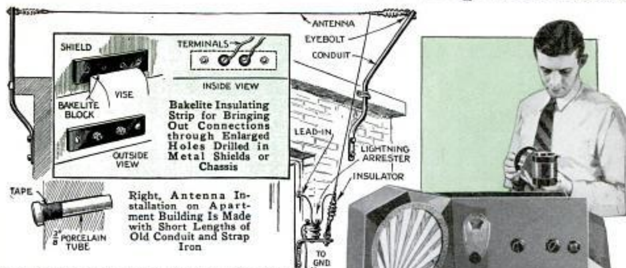
Insulating Tube for Bringing Lead-In Wire into Building Should Be Slanted Upward to Keep Out Rain; Tape Holds Tube in Position
