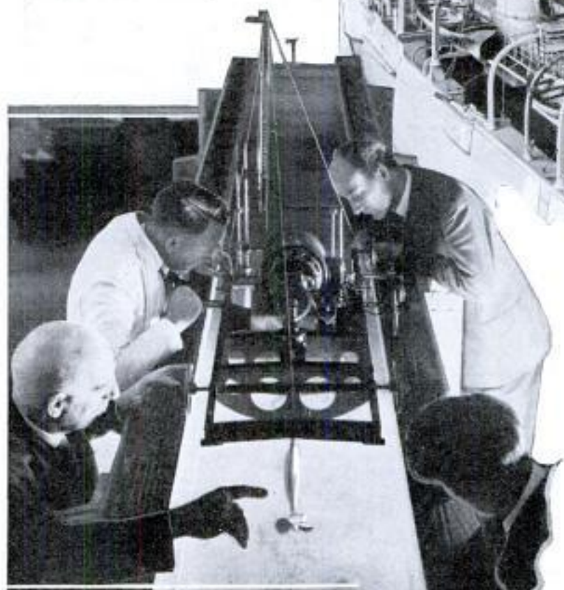
Above, Trial Car in Which the Propeller Is Installed under Water; the Propeller Is Moved by an Electric Motor on the Car Which Drives It Forward at Great Speed While Observers Watch the Action of the Blades in the Water
