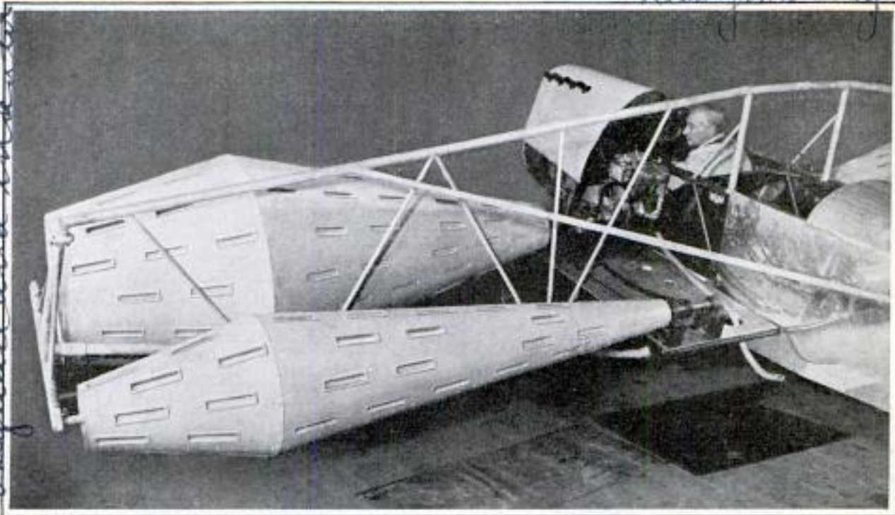
Left, Rotors of the Wingless Plane; Note Construction of Pockets in Rotor Surfaces Which Eliminate the Drag by Throwing the Air behind in Typical Slip Stream
