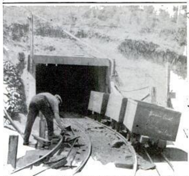
Rope Railways Are Built with the Tracks Tilted the "Wrong" Way on Curves. This One Is in Australia
