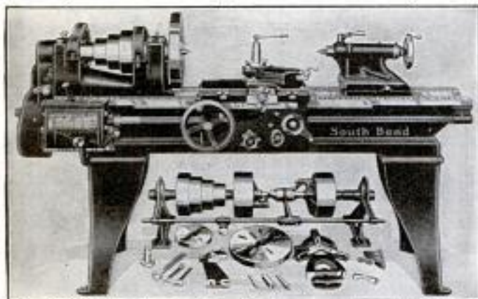
16" x 6" Quick Change Gear Lathe complete with Double Friction Countershaft and Equipment as shown, weight 1875 lbs. Price..... $540.00
