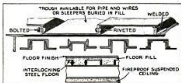
Methods of Fastening and Forming Interlocking Floors
