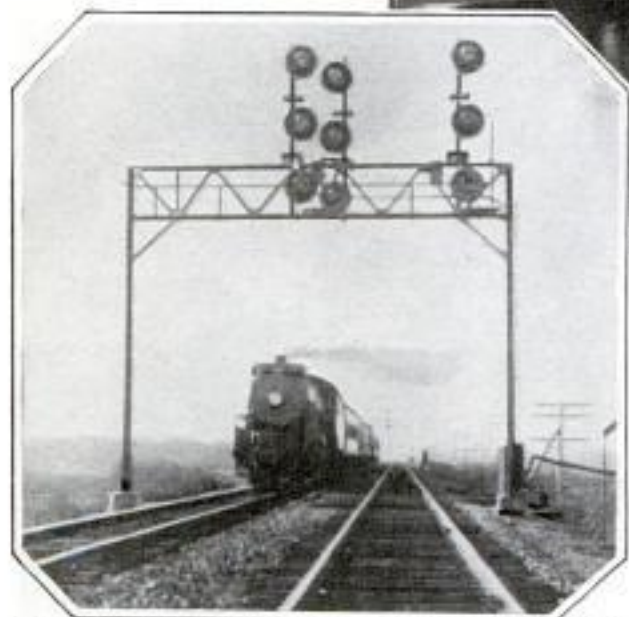
Top, Operator at the Remote Control Switchboard; Above, Signals Operated by Remote Control
