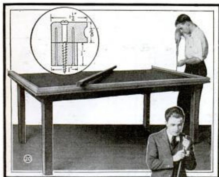
Simple Billiard Table Having a Wooden Bank Provided with a Length of Rubber Tubing Tacked On to Serve as Rebounding Strip; Pockets May Be Added or the Bank May Be Removable for Ping Pong
