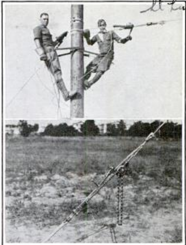
Guy Wires and Telephone Lines Are Easily Stretched with This Light-Weight Chain Hoist
