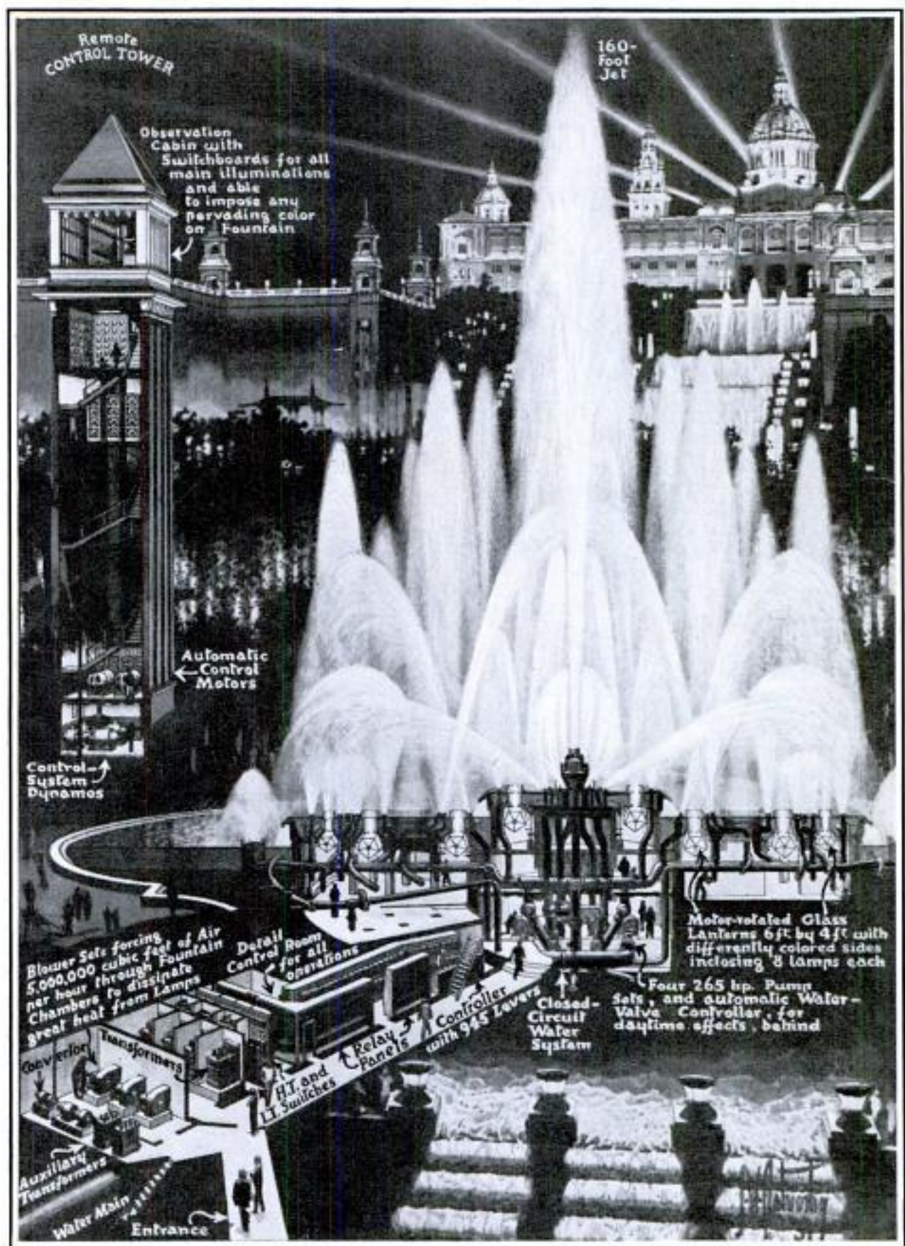
Operation of Giant Fountain at Barcelona; Pumps Force 2,000,000 Gallons of Water an Hour through 1,700 Jets to Form Forty Different Colored Patterns
