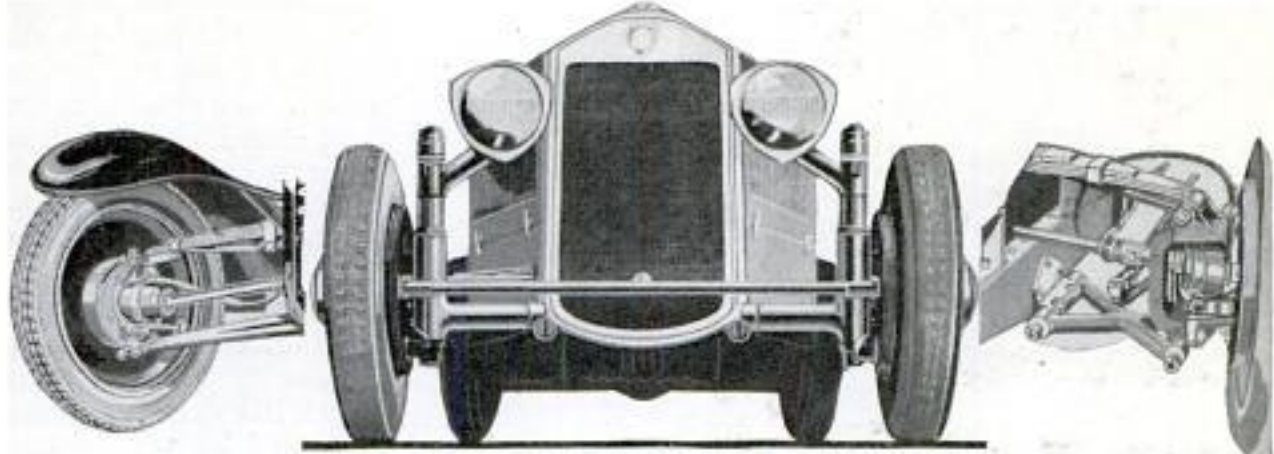
Above and Below, Individually Sprung Wheels; Right and Left, Two Different Spindles for Front-Wheel Drive
