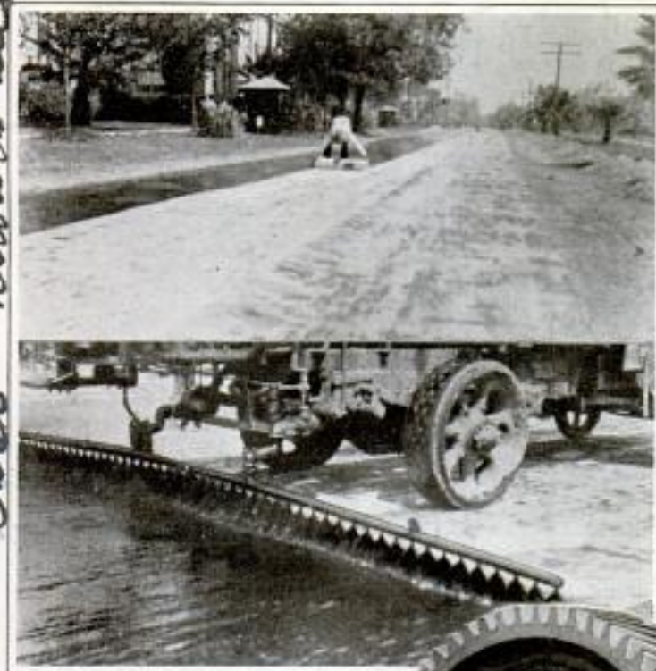
Courtesy Cotton Trade Institute Above, Laying the Canvas and Applying Asphalt in Making Cotton Road; Right, Timing Gear Made with Cotton
