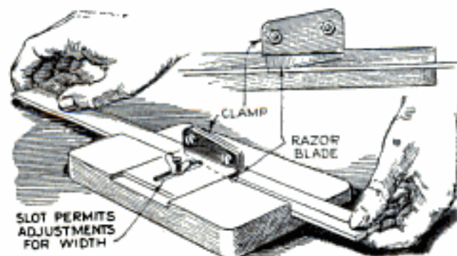
Balsa Wood Cut into Thin Strips with Tool Made from Razor Blade
