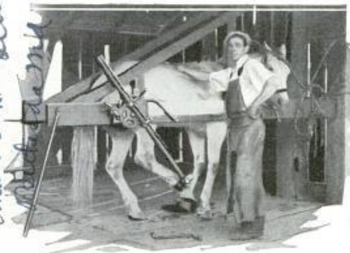
Courtesy U. S. Forest Service The Iron Man That Speedily Convinces the Wildest Outlaw Horse That His Struggles Are in Vain
