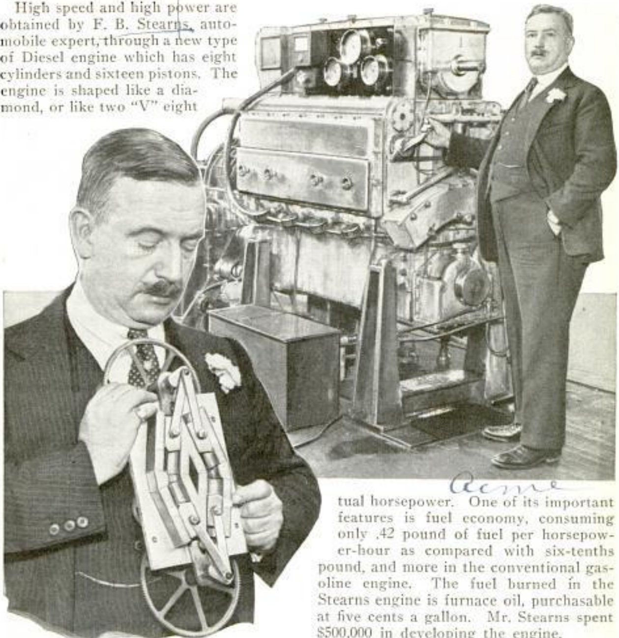
F. B. Stearns and His New Diesel. Above: the Inventor with a Cut-Away Model, Below
