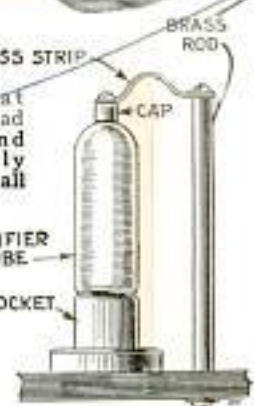
Above, Improved Terminal for Top of High-Voltage Rectifier Tubes; Copper Braid or Thin Brass Strip Holds Cap
