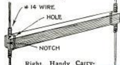
Right, Handy Carrying Strap for Testing Instruments Made from Old Belt; Below, Useful General-Purpose Clips and Jacks for Test Cords Made from Small Spring Clips
