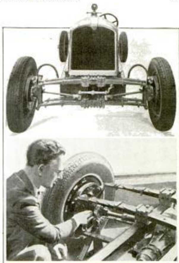
Top, Front Suspension, and, Below, Rear of Auto That Has No Axles
