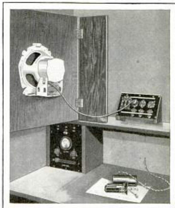
Baffle That Serves Also as Locker Door, and Method of Mounting the Speaker
