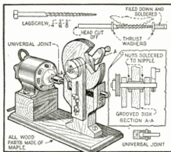
Made from Maple Parts, This Worm Gear Gives Wide Range of Speed for Moving Window Displays
