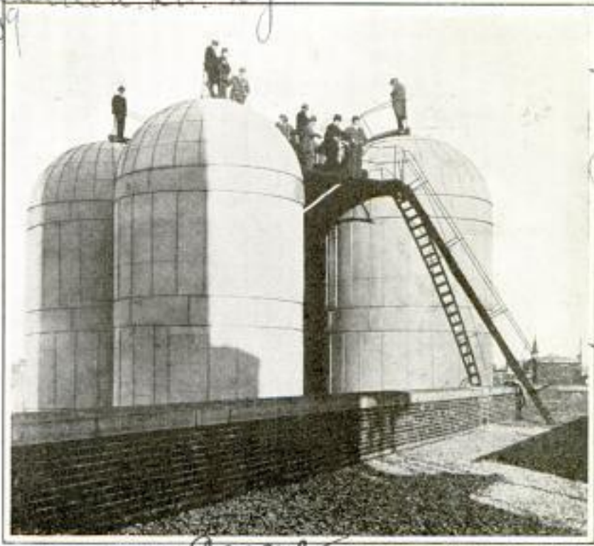
Steel Tanks of Special Design Are Used to Store Up Steam Generated in Slack Periods by Swedish Plants
