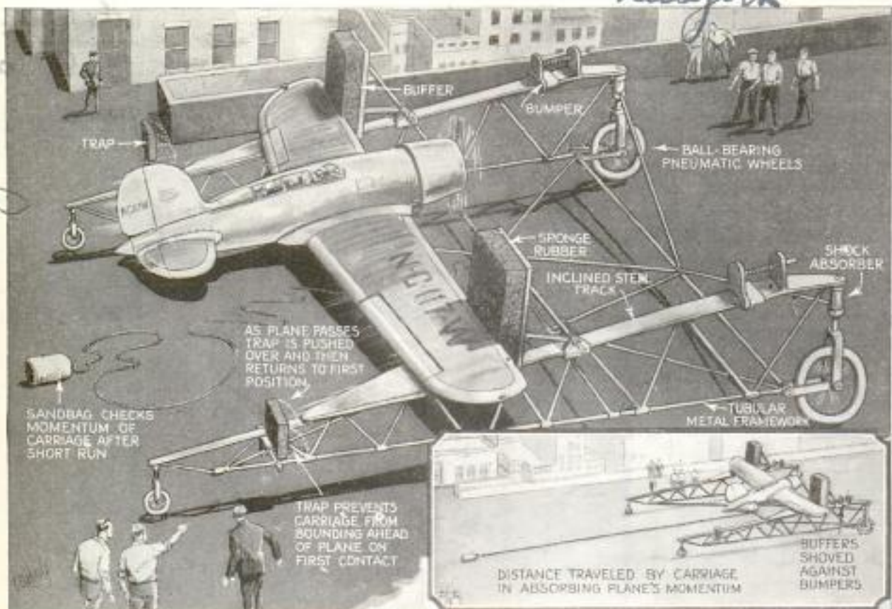
Planes Which Have Dropped Their Landing Gear Can Come to Earth Safely on a "Cradle"; Roof Landings Are Possible, Since the Cradle Stops Any-Size Aircraft after a Short Run
