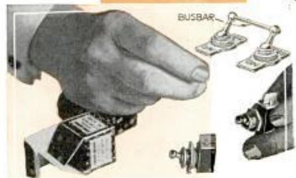
Left, Two or More Tumbler Switches May Be Ganged if Handles Are Insulated from the Circuit; Right, Pin-Jacks Used to Make Convenient Connector for Portable Receiver
