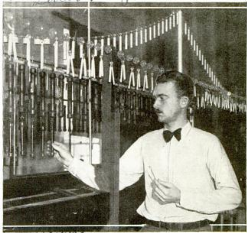
Small Weights Hung on This Bridge Model Reveal the Strain Which May Be Applied Before Collapsing Point Is Reached
