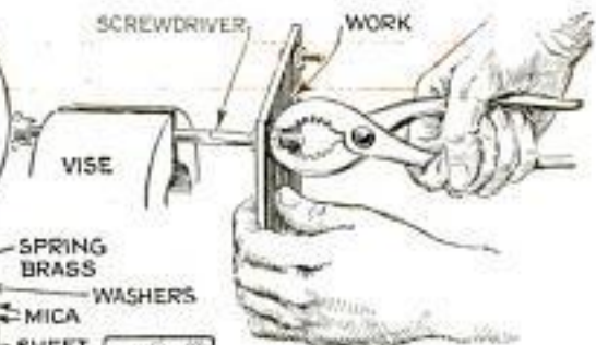
Screwdriver in a Vise Is Equal to Extra Hand When Tightening Hexagon Nuts on Panels
