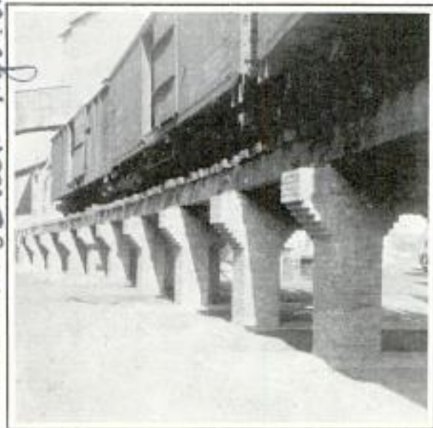
Railway Trestle Built in Fourteen Days of Steel-Reinforced Brick; There Are Twenty-One Piers
