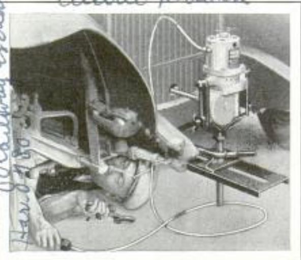
Electric Crank That Clamps to Front Axle and Turns Over Motor during Repairs to Car
