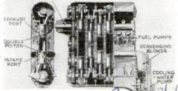
Airplane Motor That Uses Crude Oil for Fuel; Note Double Pistons for Each Cylinder
