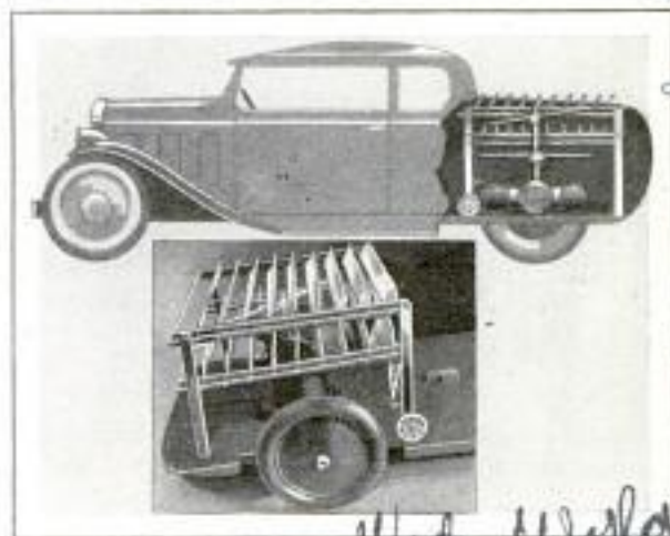
Auto Driven by Propeller at Rear, Which Sends Air Stream Upward through Movable Planes
