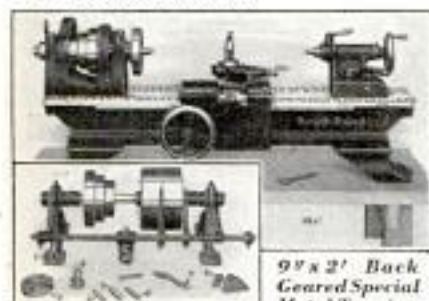
9' x 2' Back Geared Special Metal Turning Lathe. Weight 275 lbs. Price $100 Only $20 down; $7 monthly.
