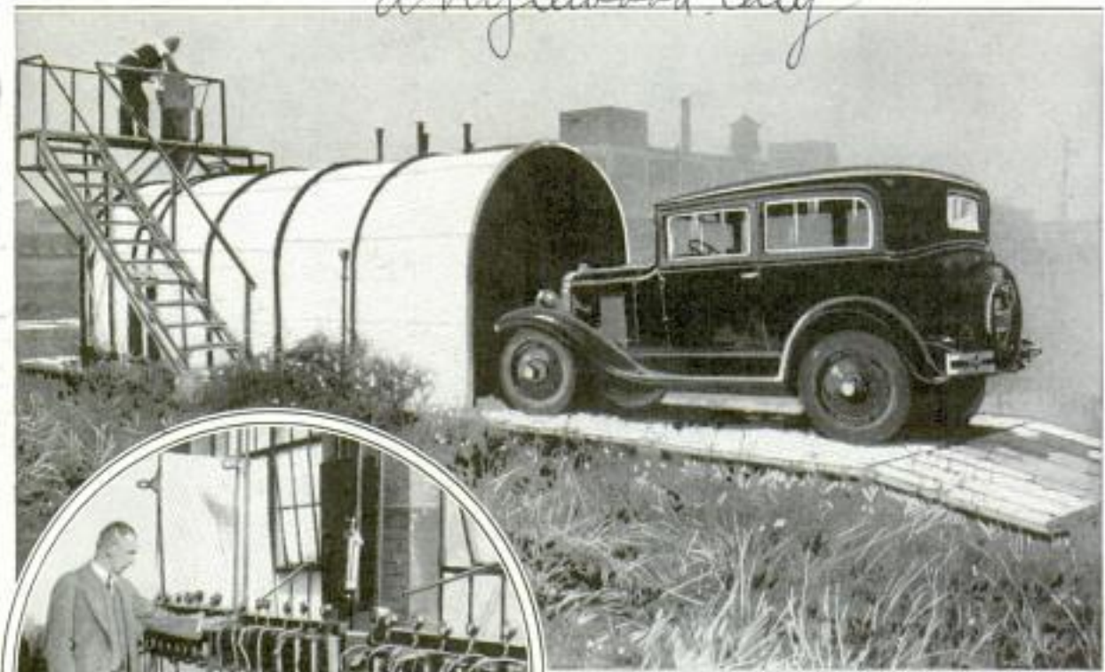
Above, Car Ready to Enter Wind Tunnel for Air-Cleaner Test; Left, Testing Oil Filters
