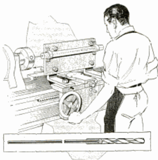
Improvised Holder on Lathe Carriage Forms Extension Drill for Hollow-Drilling Shafts
