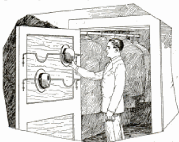
To Save Space, This Convenient Hat Rack Is Stapled to Inside of Closet Door
