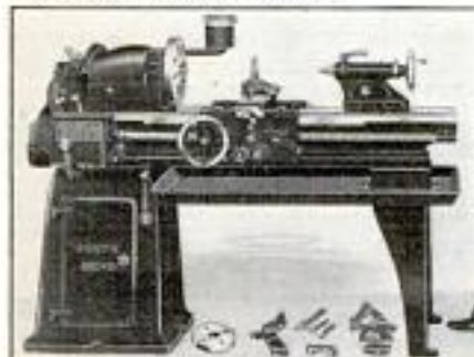
New Model Underneath Belt Motor Driven, Back Geared, Screw Cutting Lathes, available in two series, 96 sizes and types, 9' to 18' swing. priced from $283 to $1356 Can be bought on easy payments.
