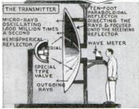
How Micro-Ray Receiver and Transmitter Operate, and Comparison of Small Power and Equipment Needed with That of Ordinary Station
