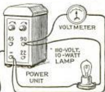
Lamp Used as an Artificial Load for Testing B-Power Units under Working Conditions; Below, Wall Plates Adapted for Switch Panel; Left, Phone-Tip Jack Arrangement
