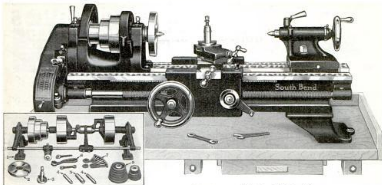
9' x 2' new model Junior Back Geared Screw Cutting Bench Lathe. Weight 325 lbs. Price $150. Only $30 down, $10.50 monthly.
