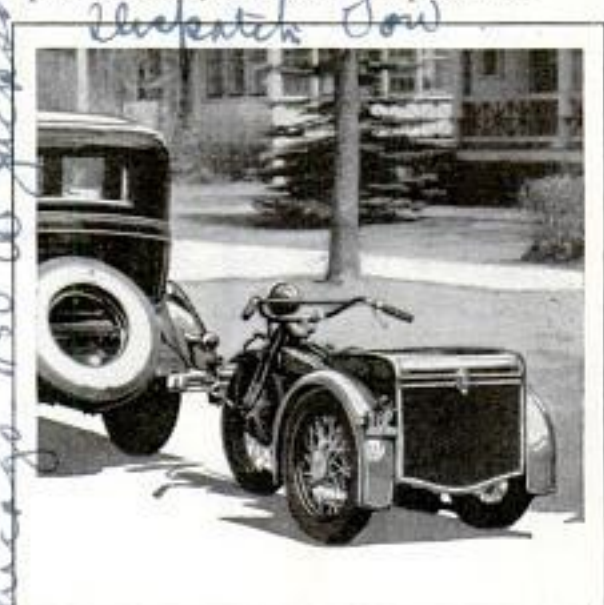
Motorcycle That Can Be Towed behind Auto, Enabling One Man to Call for or Deliver a Car
