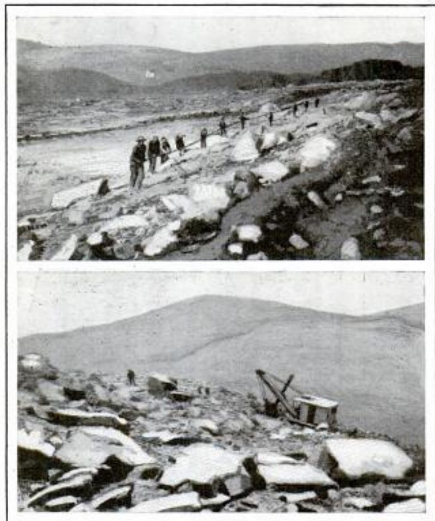
Above, Carrying 1,500-Foot Air Pipeline from One Switchback Up to Next; Below, Power Shovel Excavating Road after Dynamite Blast
