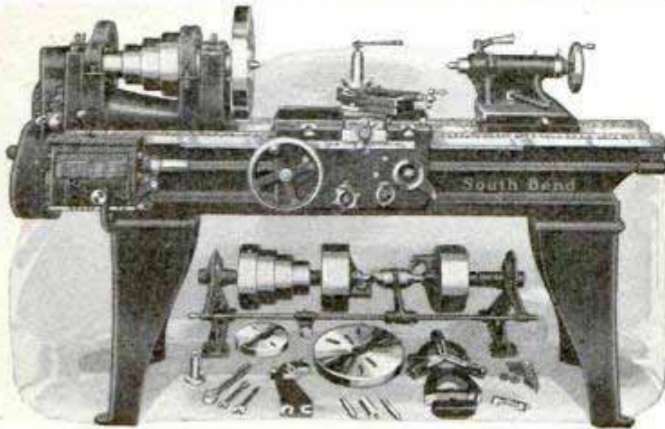
16" x 6' Quick Change Gear $598 New Model South Bend Lathe
