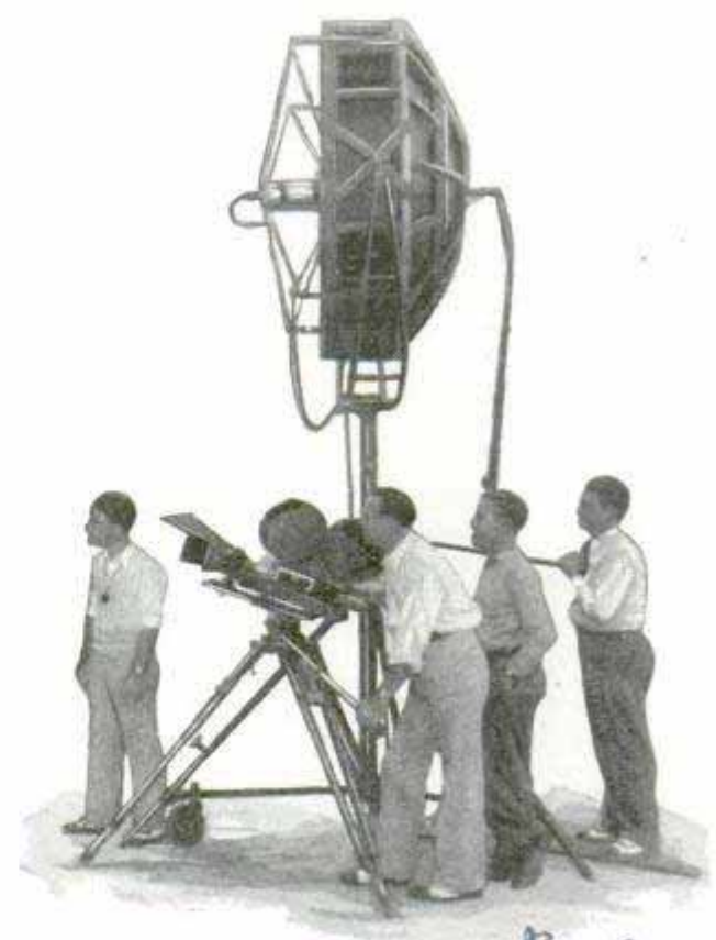
Directional Microphone, Used in Movies, Which Picks Out Only Sounds at Which It Is Pointed
