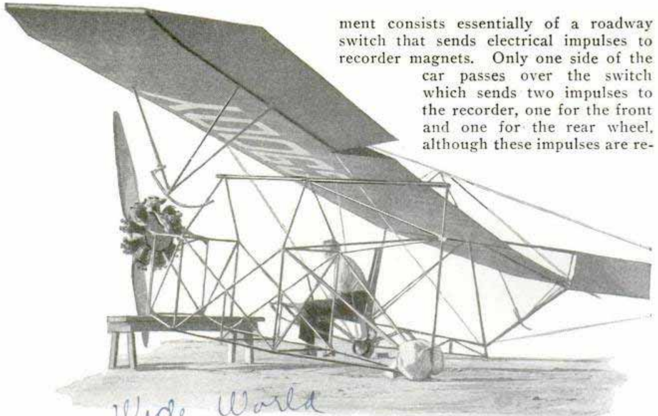
Interchangeable Plane Which Can Be Converted from a Glider to an Airplane by Attaching the Wings and Frame Forming the Glider to a Fuselage Which Contains the Engine
