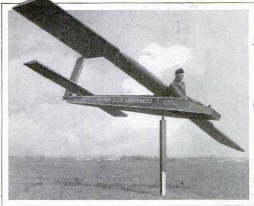
Glider Mounted on Post with Ball-Bearing Top, Which the Student Can Control Like a Real Ship without Fear of Accident
