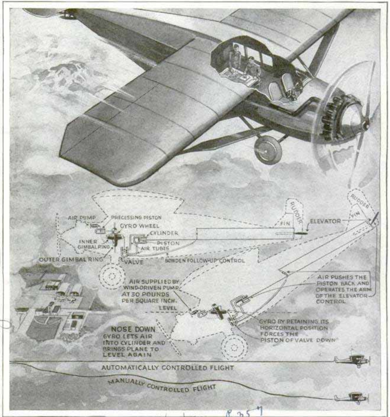
Drawing Showing How a Robot Air Pilot Keeps a Plane in Level Flight without Human Interference; a Gyroscope Is the Robot's Brain, and It Works the Controls by Compressed Air
