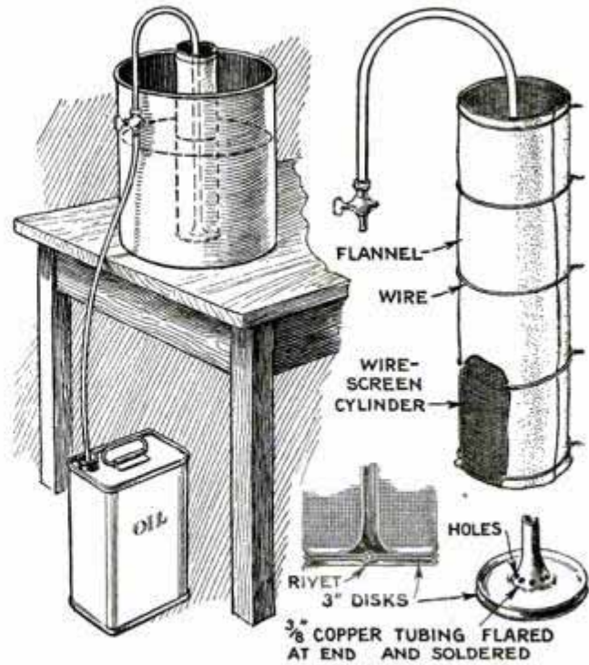
Easily Made Filter for Straining Dirty Gasoline and Old Oil and Even Homemade Beverages
