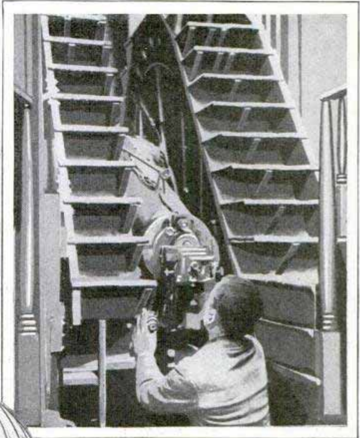
Upper Left, Tablet at Greenwich, England, Marking "Longitude 0"; from This Imaginary Line, the Rest of the Globe Is Marked into Units; Above, Telescope Facing Due South and Alined with Greenwich Meridian; by the Passing of Stars across a Thread in the Eyepiece, Greenwich Mean Time Is Computed
