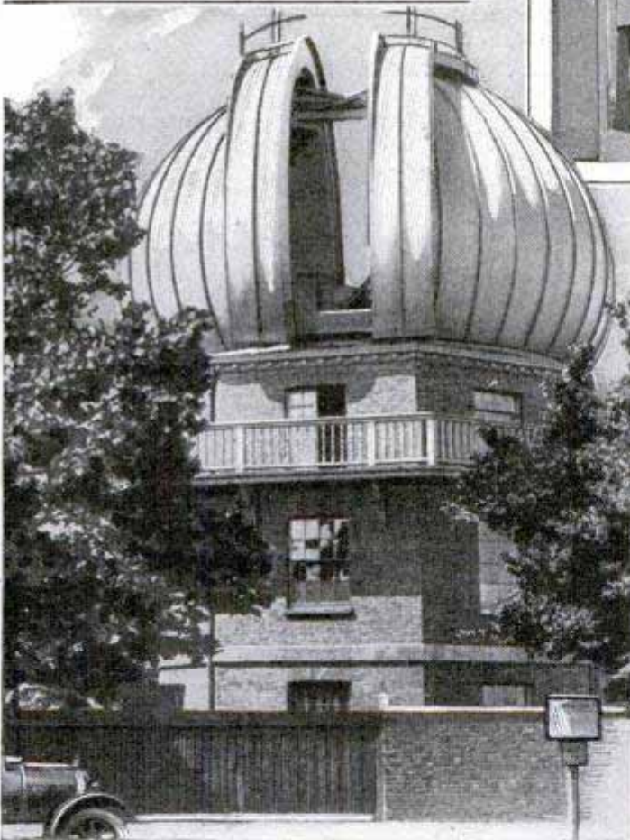
Above, Observatory at Greenwich, England, Containing a Great Telescope Which Is Part of the Elaborate Equipment Used by Scientists to Tell the Time of the World; Greenwich Meridian, Designated as "Longitude 0," Is the Official Starting Point of the Earth's Surface; from It Meridians Differing by Fifteen Degrees Each Have Been Marked Off on the Globe, East and West; Right, Standard Sidereal Clock at Greenwich Which Never Varies More than One-Fiftieth of a Second; It Is Kept in a Sealed Glass Case at an Even Temperature of Sixty Degrees
