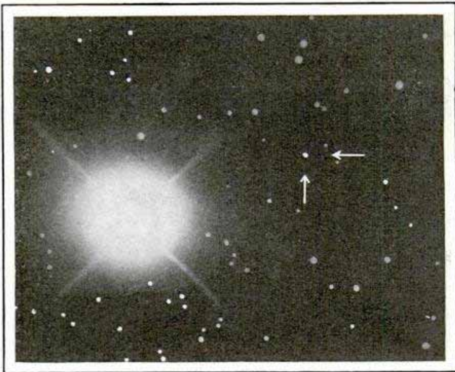
Arrows Point to New Planet Found in 1930, Although Its Existence Was Predicted Many Years Ago by the Late Percival Lowell
