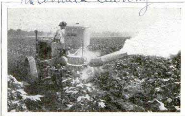
Cotton Duster Operated by Tractor, Which Sprays Sixty Rows at a Time and Covers Twenty-Five Acres an Hour
