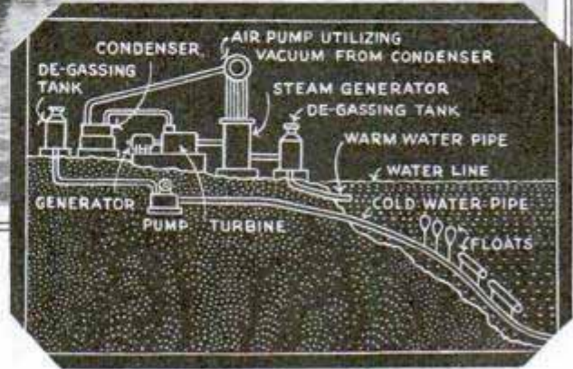
Floating a Mile of Pipe into the Sea, and Diagram Showing How Plant Works
