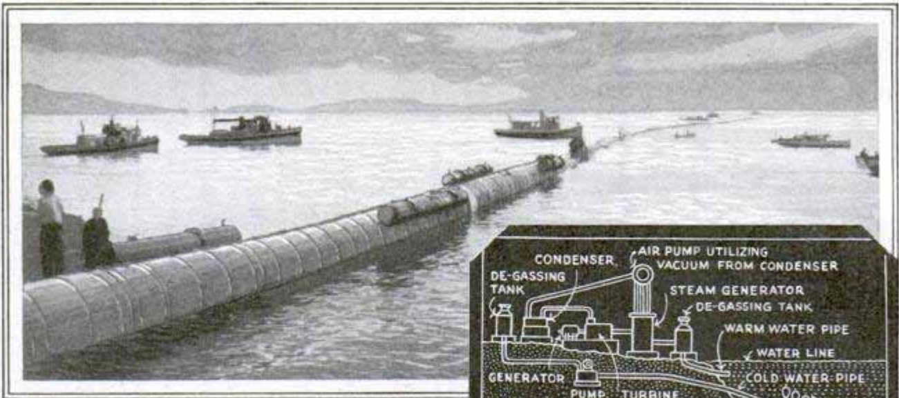
Floating a Mile of Pipe into the Sea, and Diagram Showing How Plant Works
