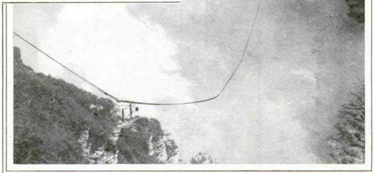
Above, One of Two Towers in the Swiss Alps between Which a Cable, Shown Below, Has Been Strung in an Effort to Trap a Charge of Lightning Powerful Enough to Smash an Atom
