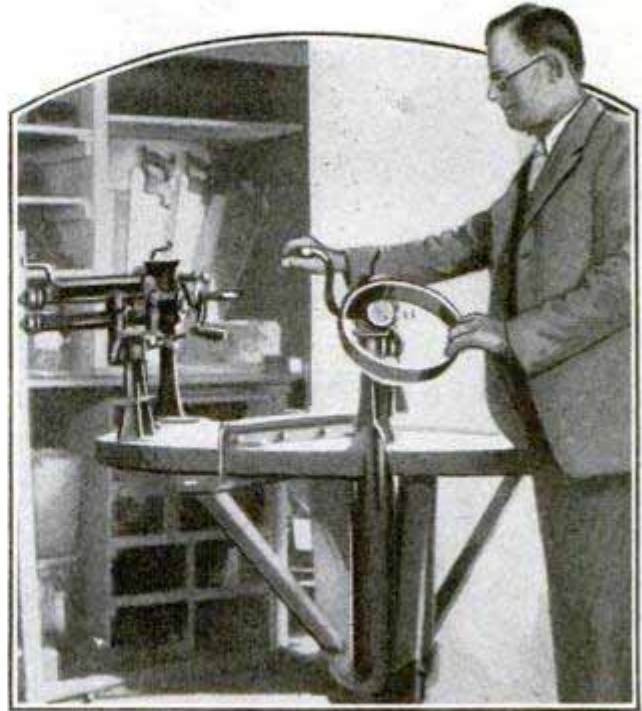
Revolving Table for Sheet-Metal Machines Saves Space in Small Shop
