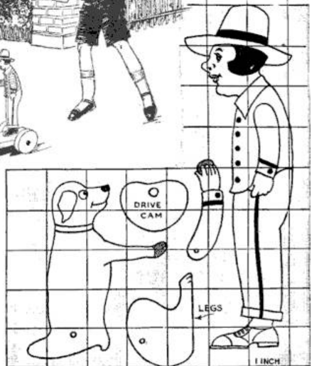
Here Is a Wooden Pup That Jumps Up for a Bite to Eat, Just Like a Real Dog
