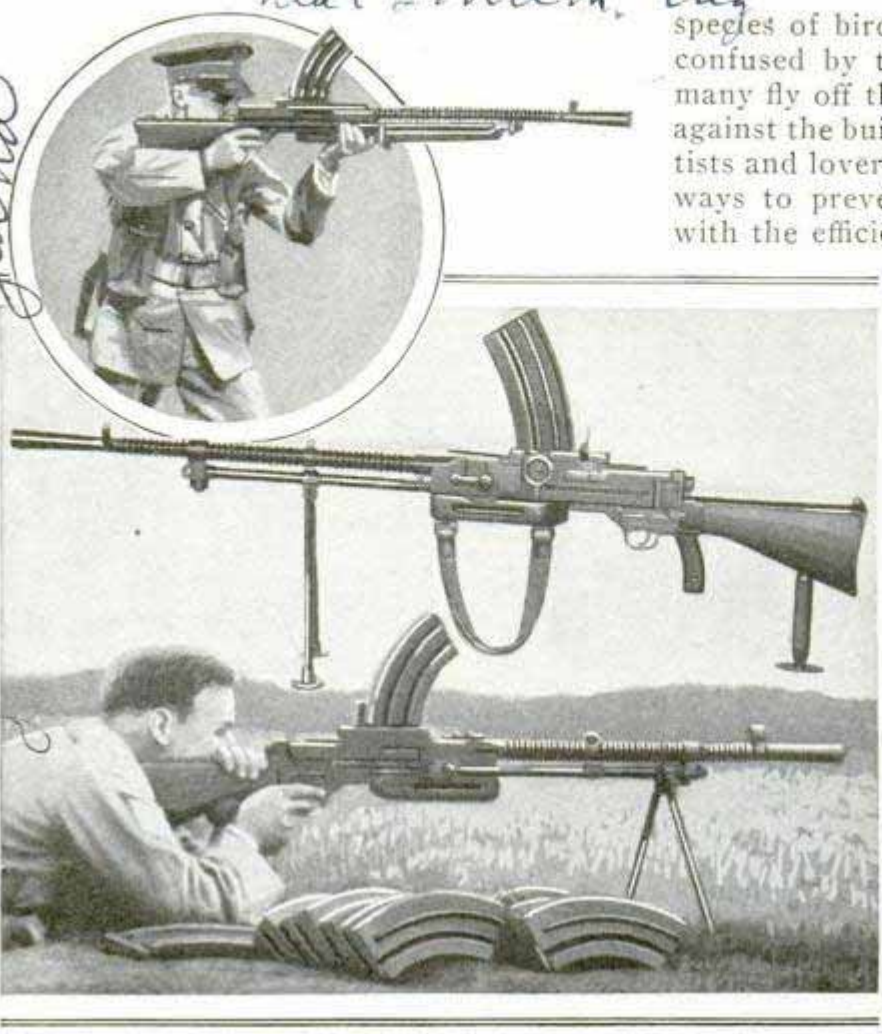
Combined Rifle and Machine Gun Converted from One Type to Another by Throwing a Lever; It Fires 300 Rounds a Minute
