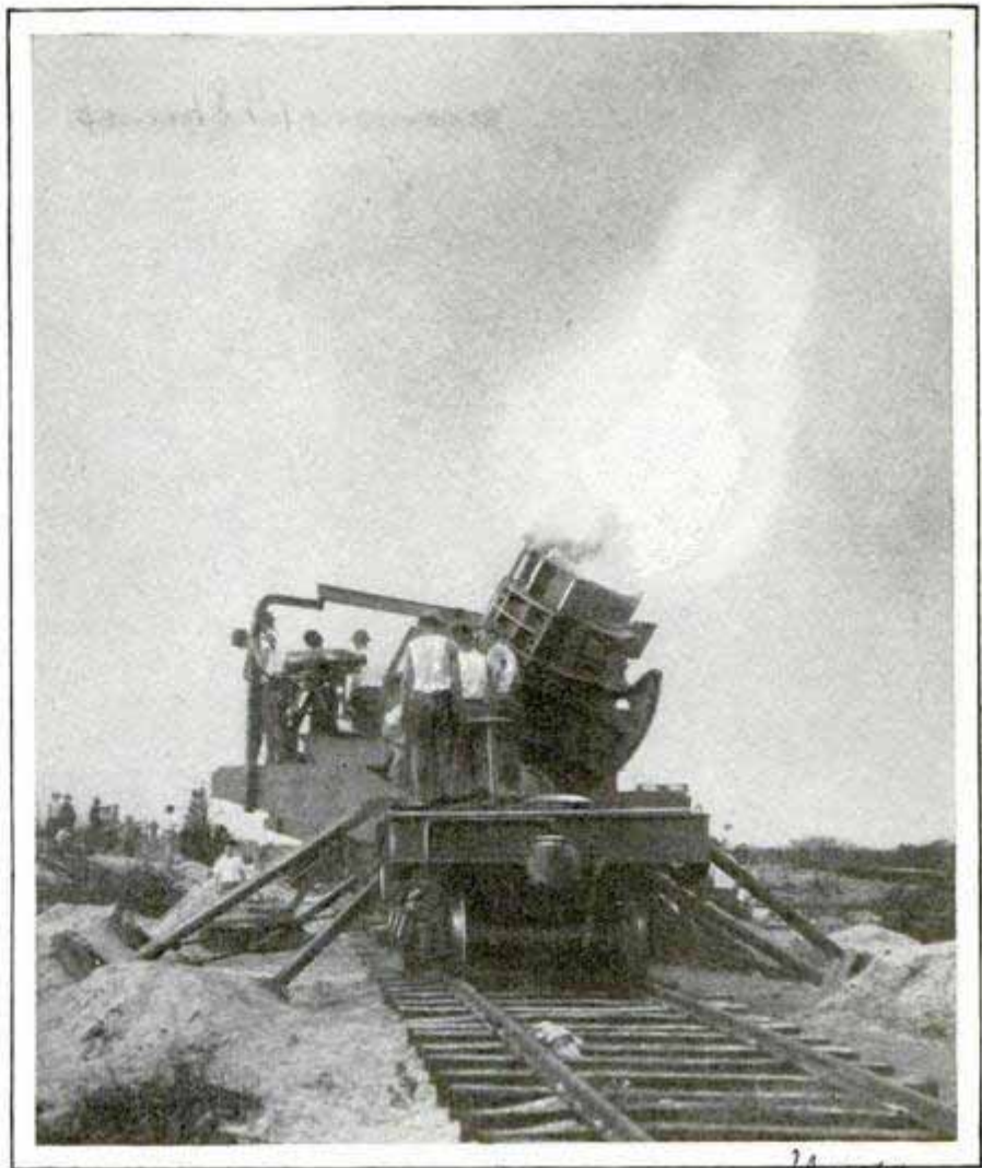
Twelve-Inch Mortar Railway Gun Which Can Fire a Projectile Nine Miles; It Is Intended for the Defense of the Atlantic Coast
