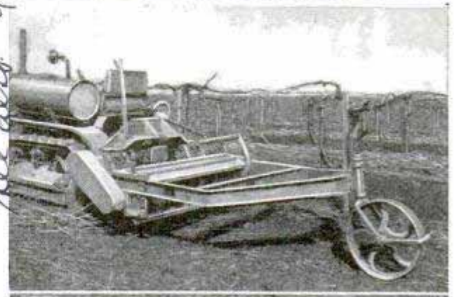
Grapevine Shredder Which Cuts Up Brush, Like That Shown Above, so It Can Be Plowed Under
