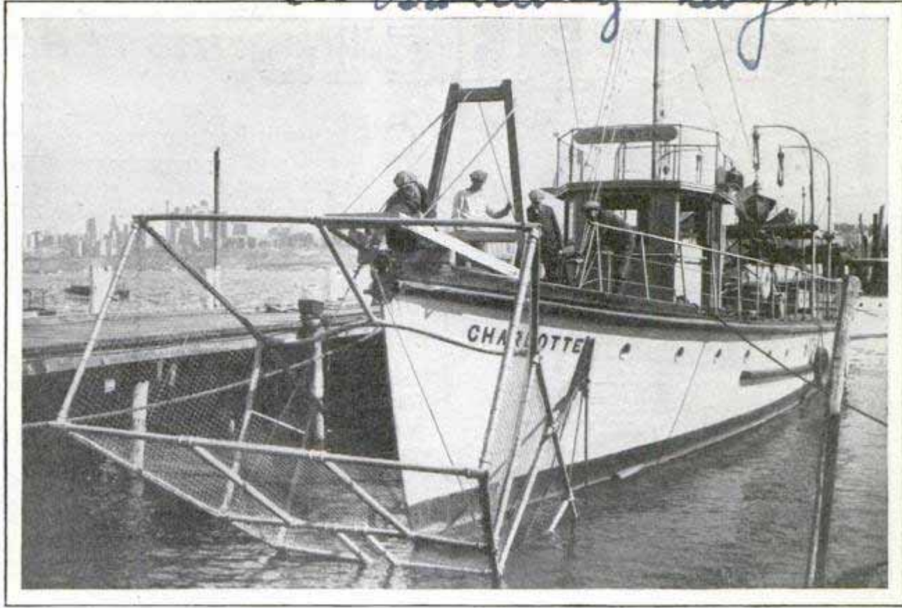
Boat Which Has Been Converted into a Fishing Machine and Pumps the Fish from the Water onto the Deck; in the Foreground Is a Net Which, When Lowered, Acts as a Chute for the Catch
