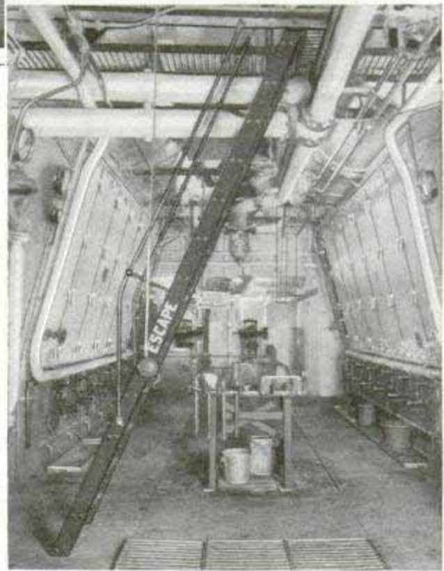
Above 8,500-Horsepower Motors in U.S.S. “Virginia,” and View of Vessel’s Boiler Room; the Motors Are Coupled Directly to the Driving Shafts
