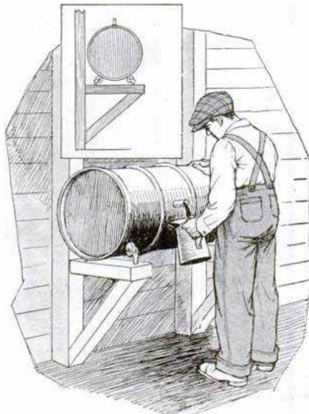
Simple Mounting for 15-Gal. Oil Drum Makes Dispensing Easy and Prevents Waste
