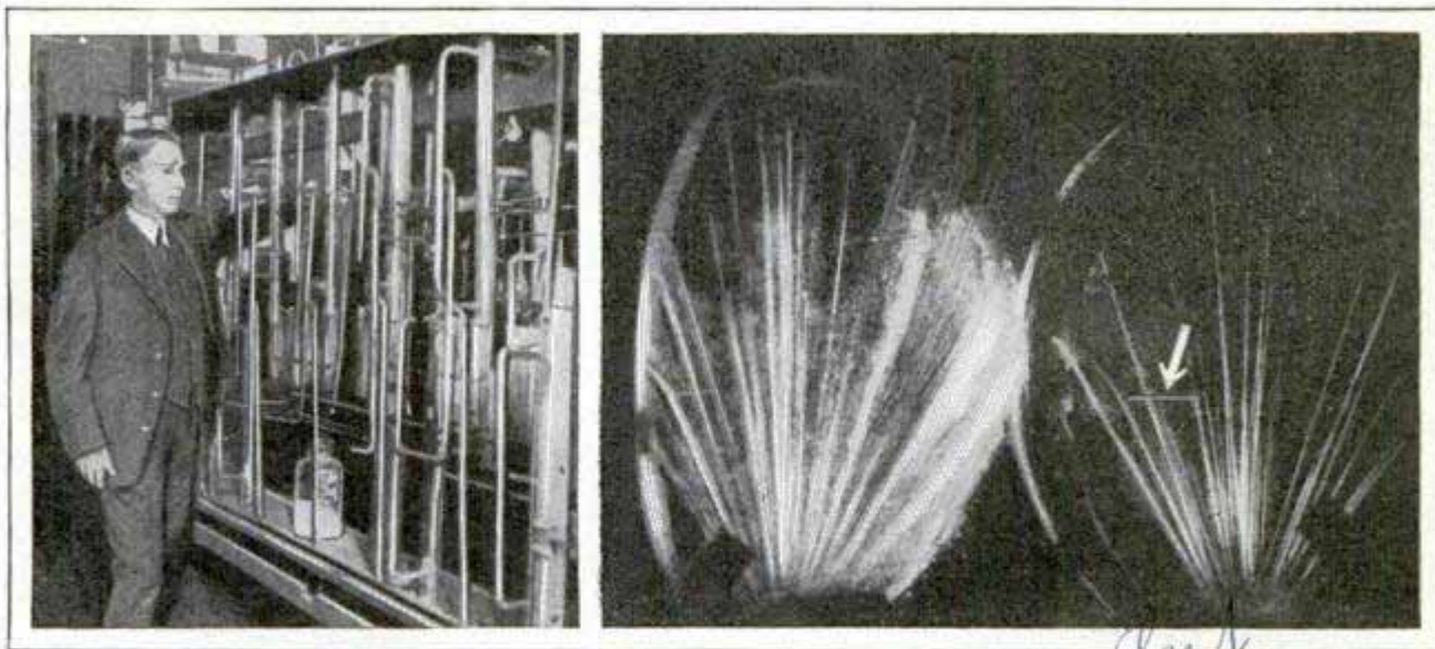
Left, Apparatus Which Fires Hydrogen "Bullets" at Atoms in Effort to Release Atomic Energy; Right, Arrow Points to Hydrogen Nucleus Traveling 10,000 Miles a Second
