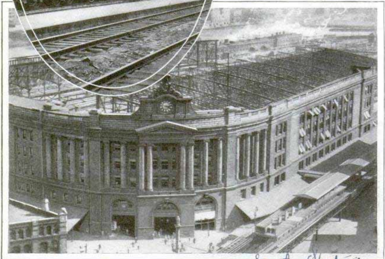
Above, Close-Up of Movable-Derrick Mount Used in Demolishing a Boston Train Shed without Interfering with Trains; Below, Station with Center Section of Train-Shed Steel Removed
