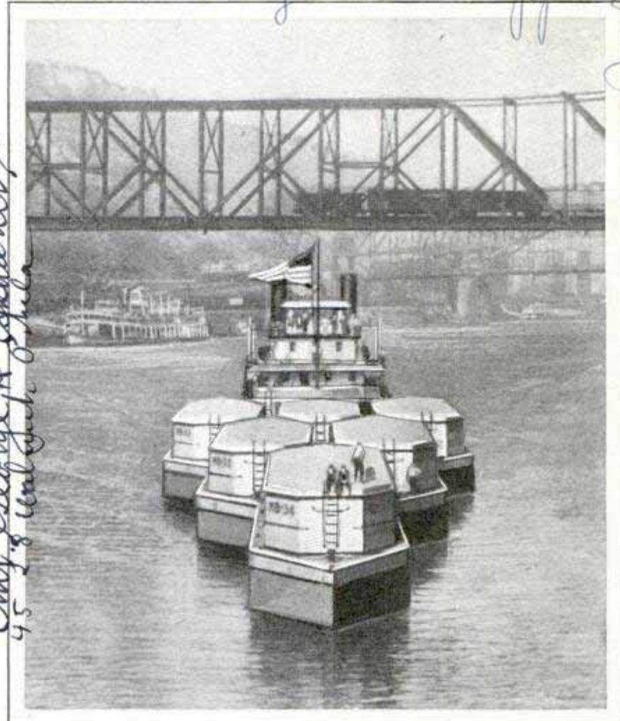
River Barges with Pointed Bows and Sterns Which Make It Possible to Tow Them in Clusters in Wedge-Shaped Formation
