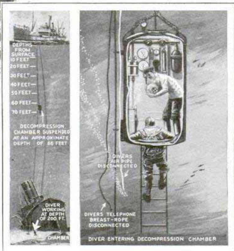
Views of the Compression Chamber Used by British Divers; Dives to Fifty-Eight Fathoms Have Been Made with It
