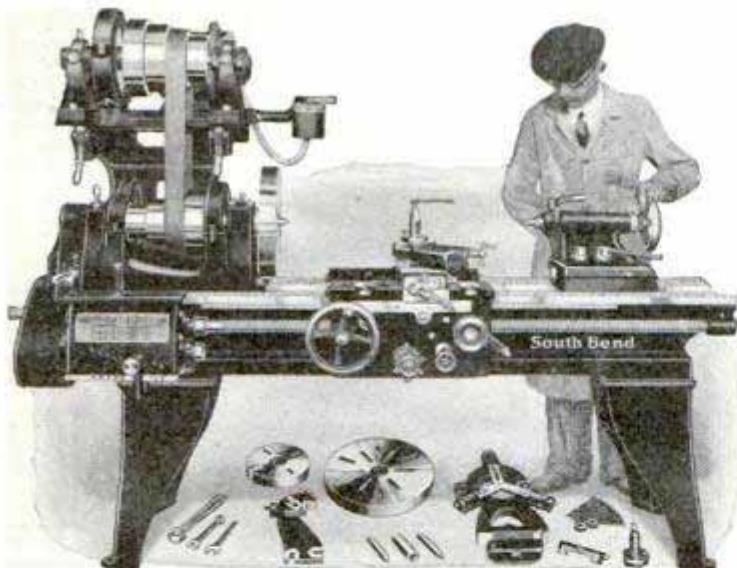
18" x 8' Quick Change Gear Silent Chain Motor Driven Lathe with Motor $997 and Equipment as shown . . .
