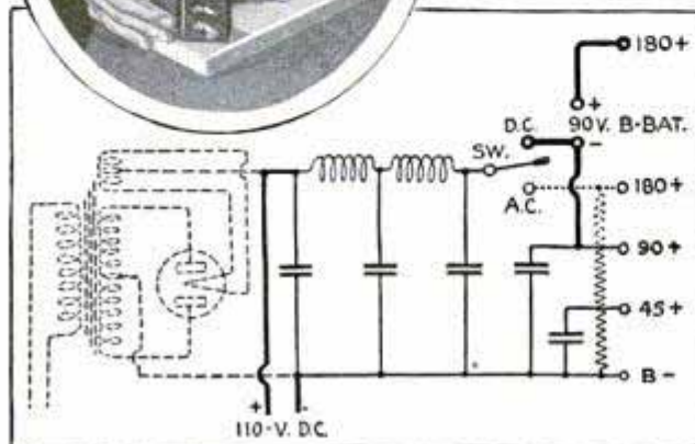
Power-Pack Eliminator Assembly for A.C. and, Below, Diagram Showing Connections for D.C. Operation
