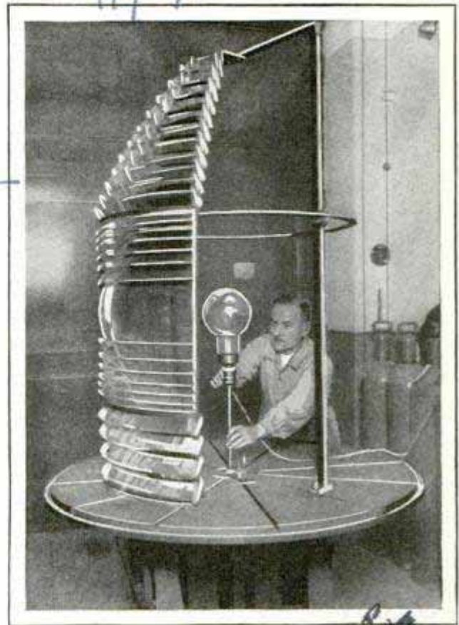
Four-Foot Searchlight Lens for a Lighthouse, and the 3,000-Watt Bulb Used with It
