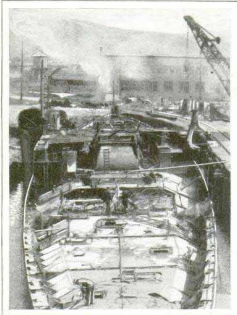
Obsolete Battleship Ready for Firing to Destroy All Woodwork, and, Below, Cutting Up a Metal Hull; Not a Pound Is Wasted
