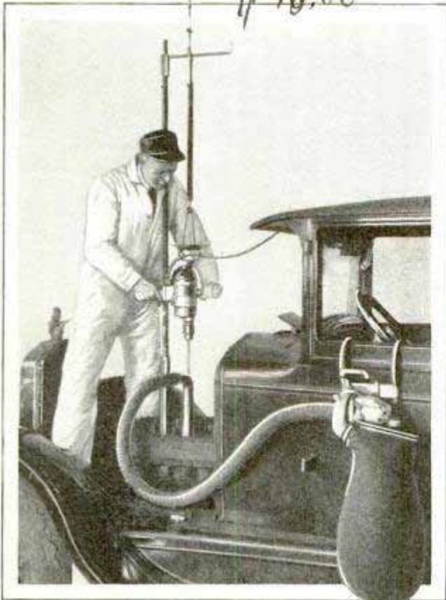
Portable Cylinder Grinder and Grit Remover, the Latter Operating Also as a Vacuum Cleaner
