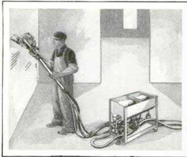
Plastering Machine Operated by Compressed Air, Which Mixes and Applies the Coating
