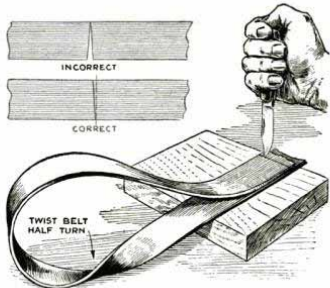
Cutting Both Ends of a Belt at the Same Time Insures Accuracy of Joining Line
