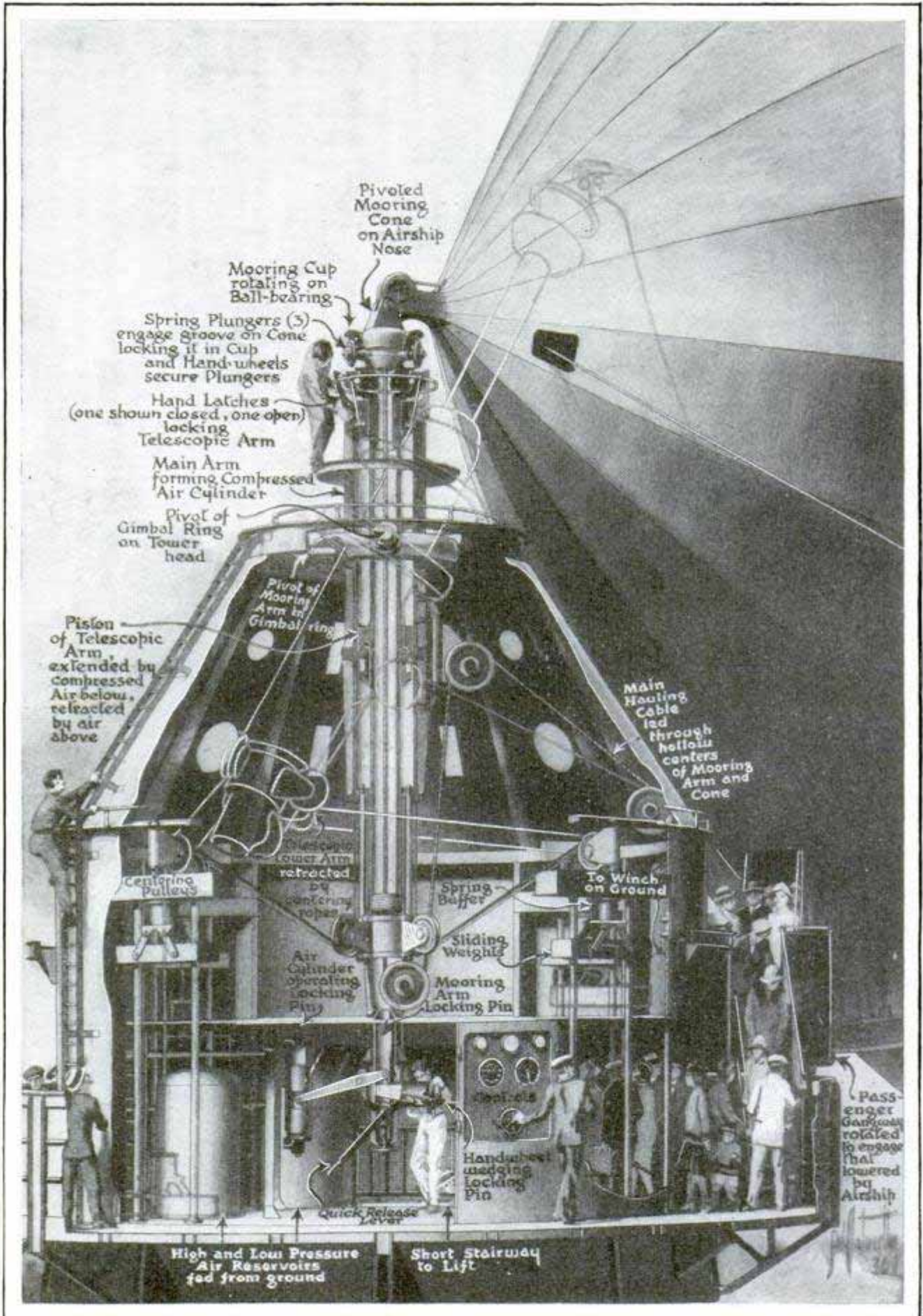
Where the "R-100" Rested When in Montreal; Artist's Drawing of the Mooring Tower Head at St. Hubert; the Mechanism Is Operated by Compressed Air—See Page 630
