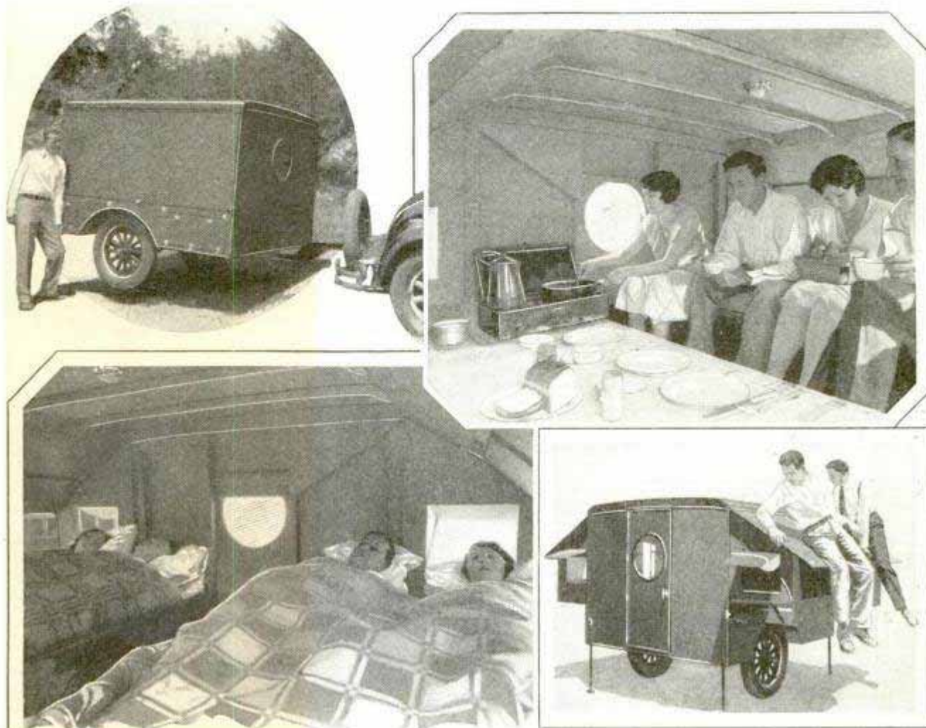
Interior and Exterior Views of an Auto Trailer Which Expands into Commodious Living Quarters; Compact Equipment Transforms the Trailer into Kitchen, Dining Room or Bedroom
