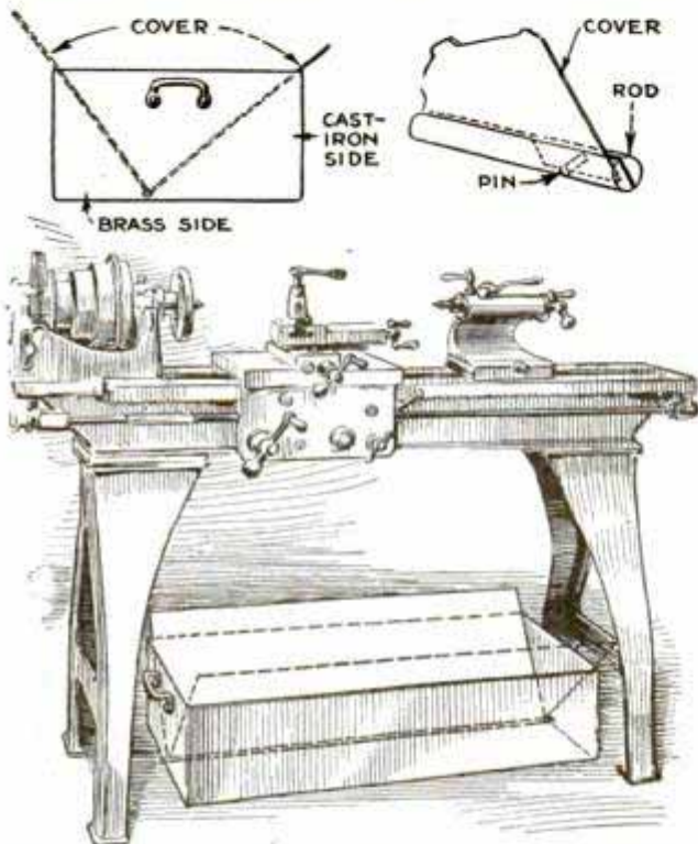
Cover of Cutting Pan, Pivoted at the Bottom, Separates Brass and Cast-Iron Cuttings
