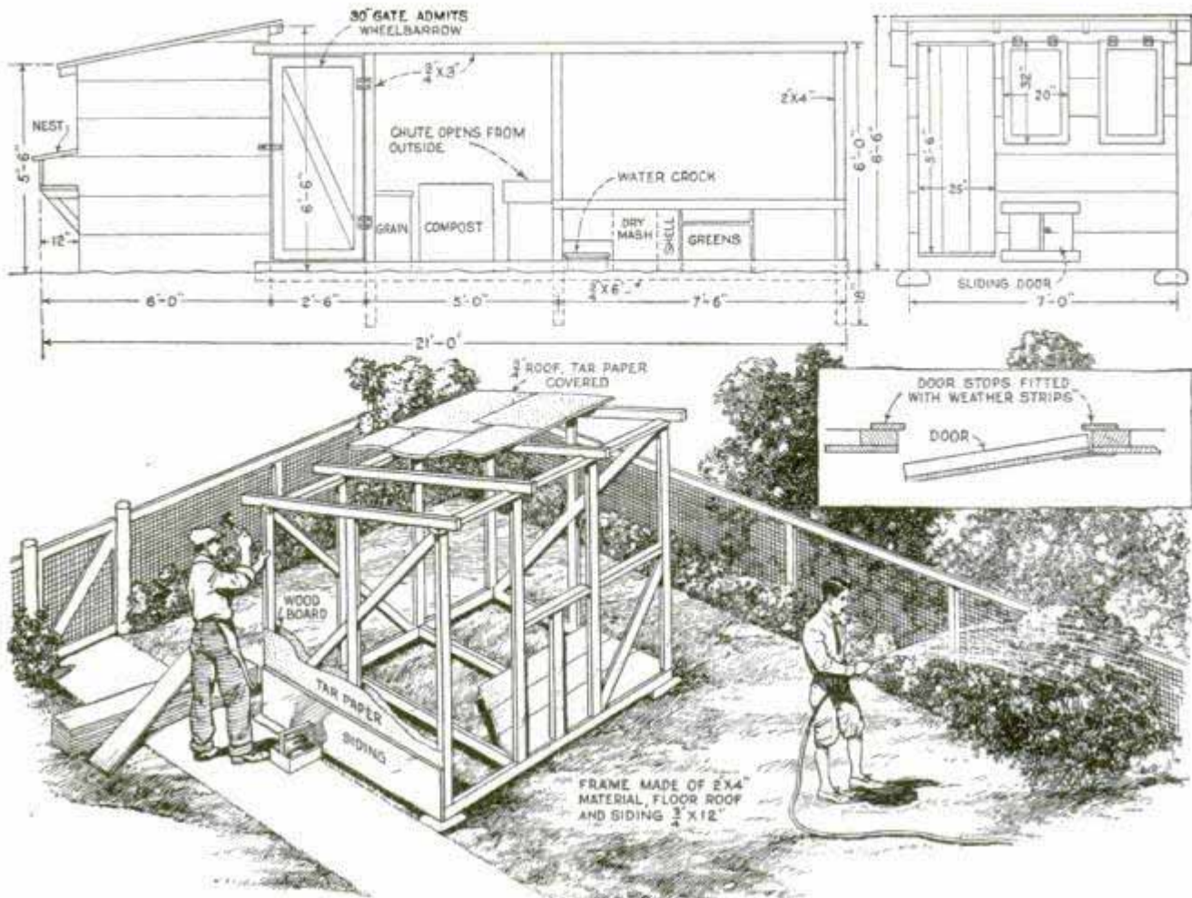
Constructional Details and Dimensions of the Hen House and Run, Showing How Easy It Is to Build One; Vines and Shrubbyery Can Be Used to Conceal It and Provide Shade
