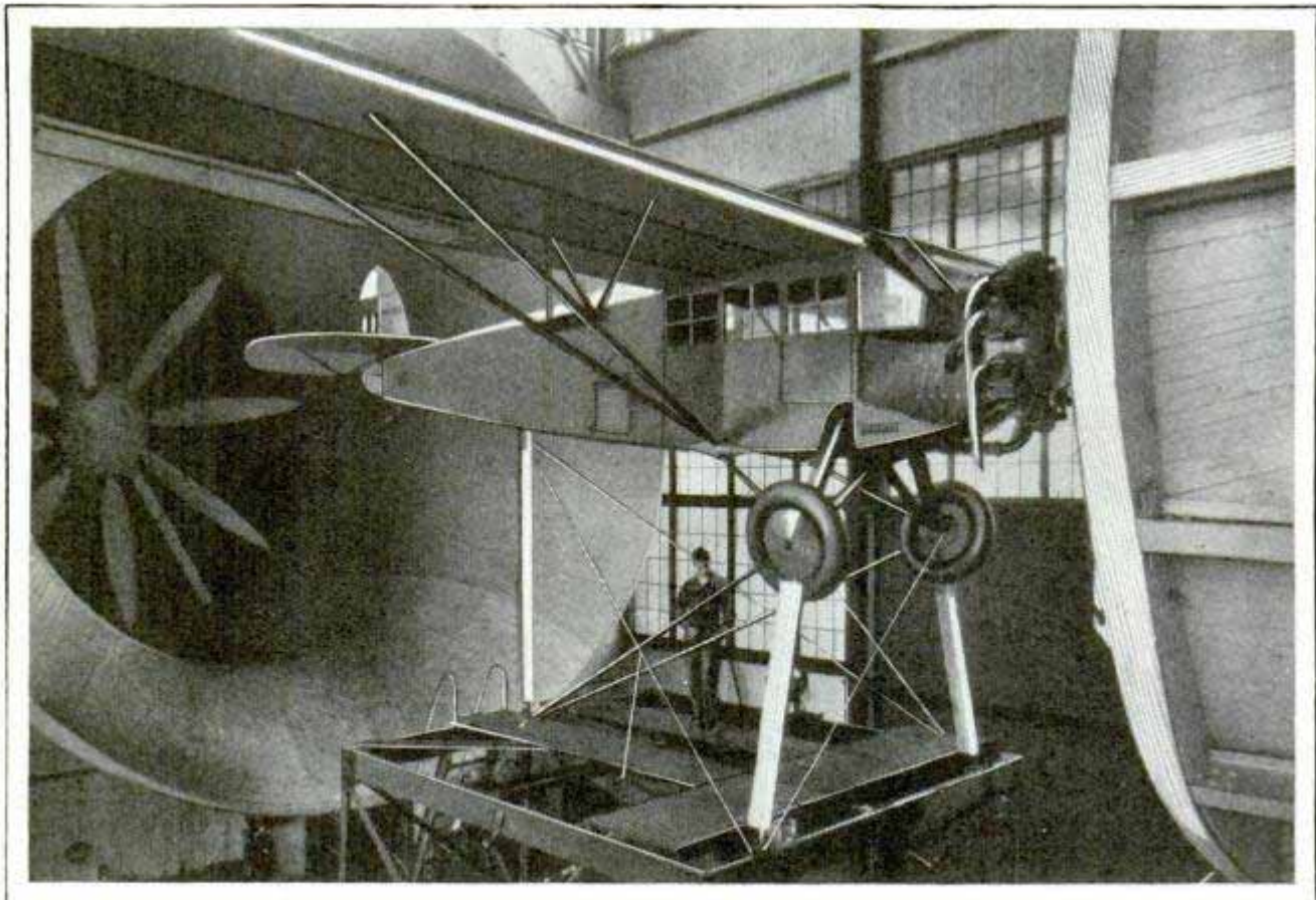
Accurate Tests of a Plane's Performance Are Obtained before Flights in the Wind Tunnel, Where Flying Conditions Are Simulated; Experiments Here Have Done Much to Develop Streamlining
