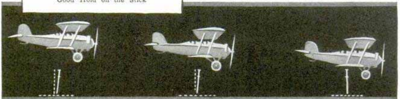
Critical Stages of a Landing; Gliding Down to a Height of Thirty Feet, Then Leveling Off by Pulling Back Slightly on the Stick
