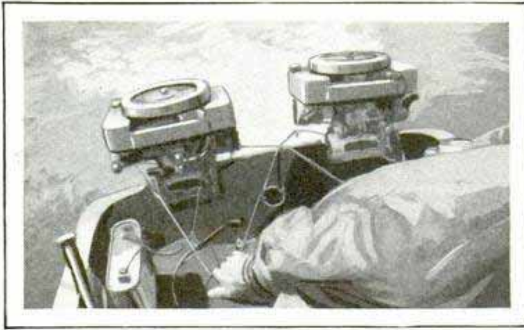
Hooking Up Two Outboard Engines So That They May Be Turned, for Steering, at the Same Time and to the Same Degree
