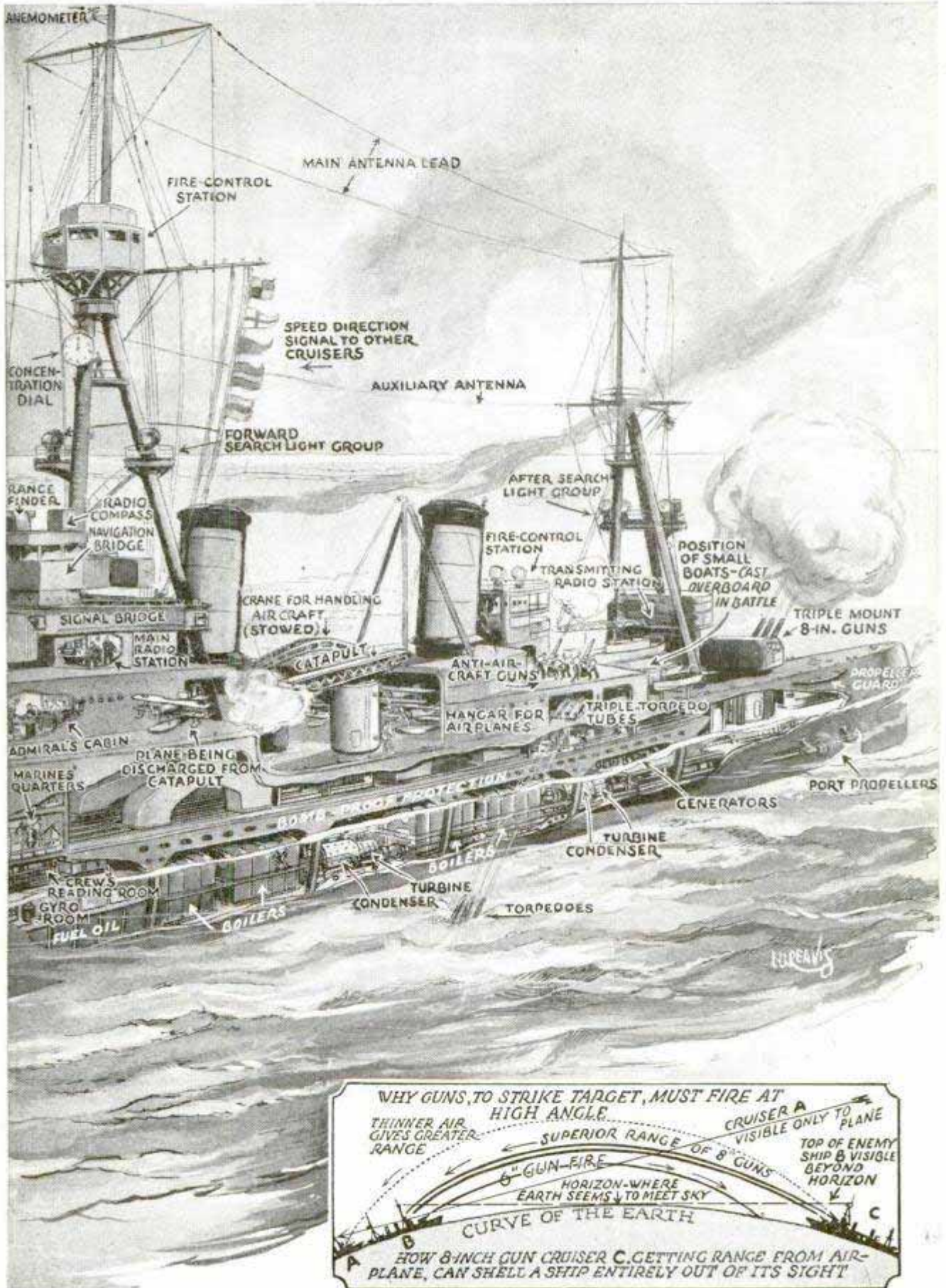
This Cruiser Develops in Excess of Thirty-Five Miles an Hour; It Is Longer and Has a Broader Beam than Other Ships of Its Type; the Diagram Explains the Effectiveness of Its Eight-Inch Guns
