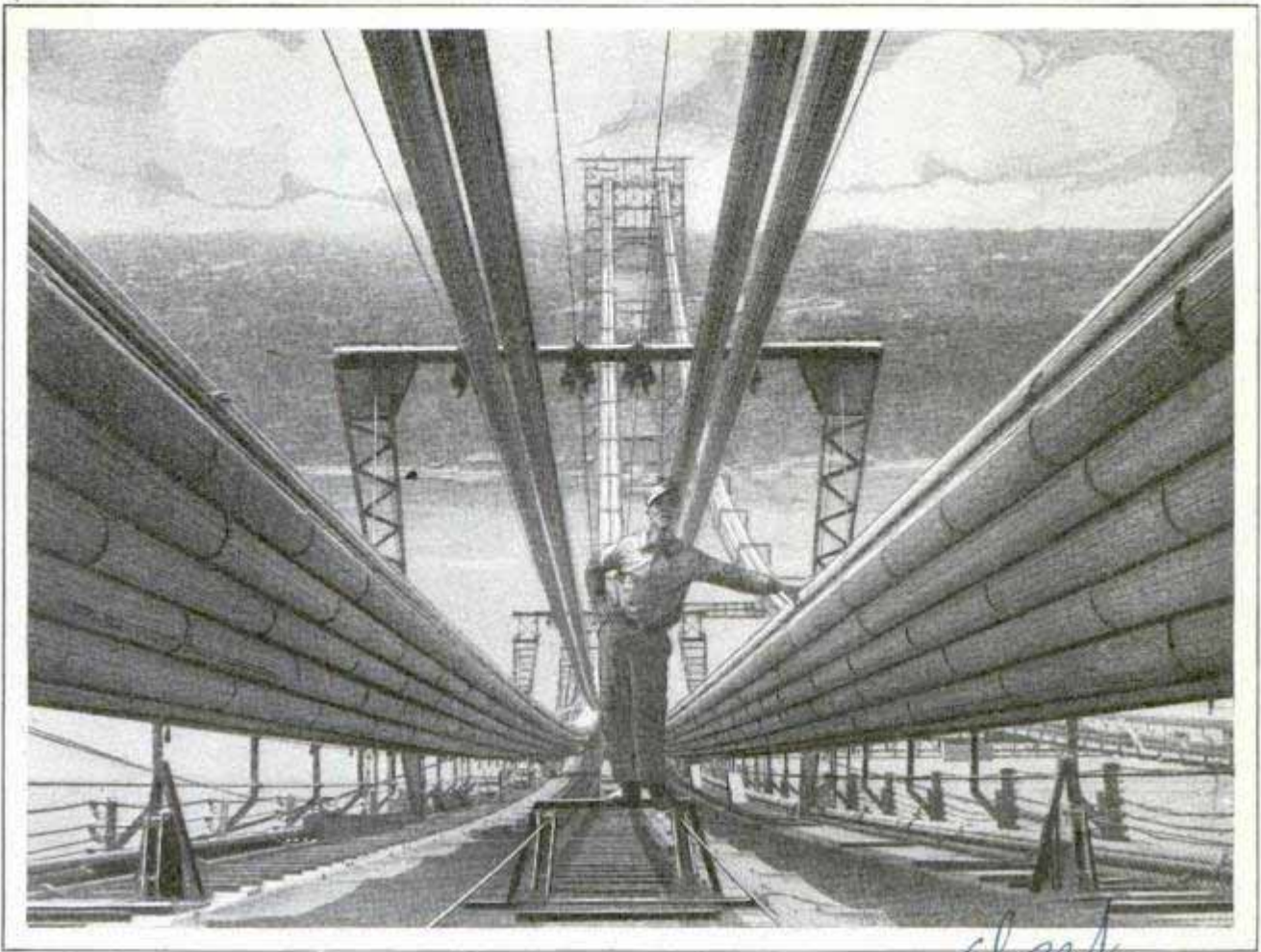
Two of the Great Cables That Will Support the Hudson River Bridge at New York, the World's Longest Suspension Span; More Than 107,000 Miles of Wire Are Spun into These Cables
