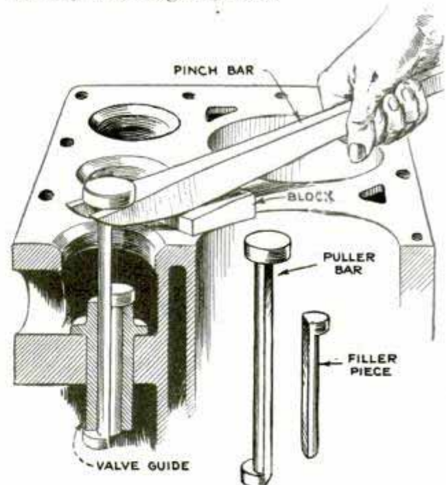
Pulling Rod and Pinch Bar Are Effective in Removing Valve Guides
