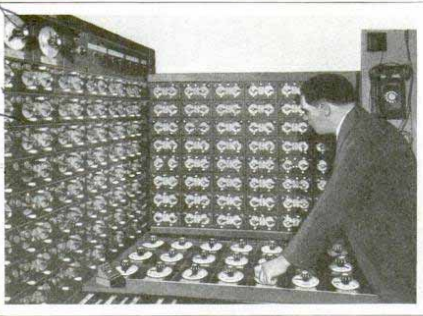
Part of Stage-Lighting Control Board, Used in Chicago Civic Opera House; It Is beneath and in Front of Stage
