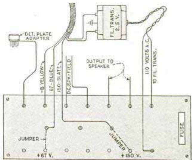
AMPLIFIER TERMINAL BOARD
