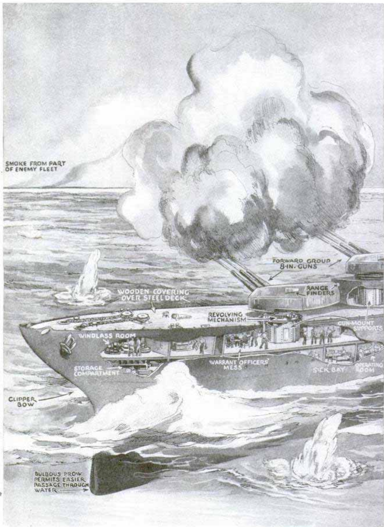
Artist's Drawing of Recently Completed Cruiser "Northampton," Showing Inner Details and How It Would Look in Battle; Note the Two Smokestacks Instead of the Usual Four
