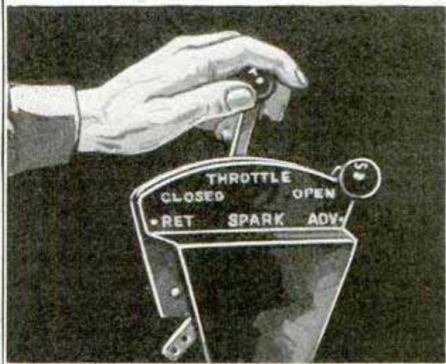
Throttle in "Fledgling" Is Operated with the Left Hand; Here It Is Shown at Cruising Position; the Spark Is Fully Advanced for Flying
