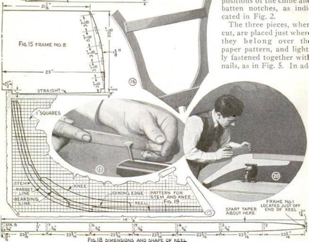
FIG. 18 DIMENSIONS AND SHAPE OF KEEL
