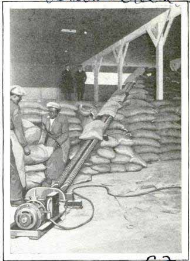
Twin-Screw Electric Conveyor Whose Revolving Spiral Tubes Move Bulky Articles Quickly
