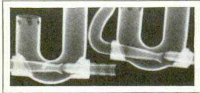
X-Ray of a Die Casting, and Incorrect Assembly of Hard-Rubber Siphons Shown by X-Ray; Right, X-Raying a Camera
