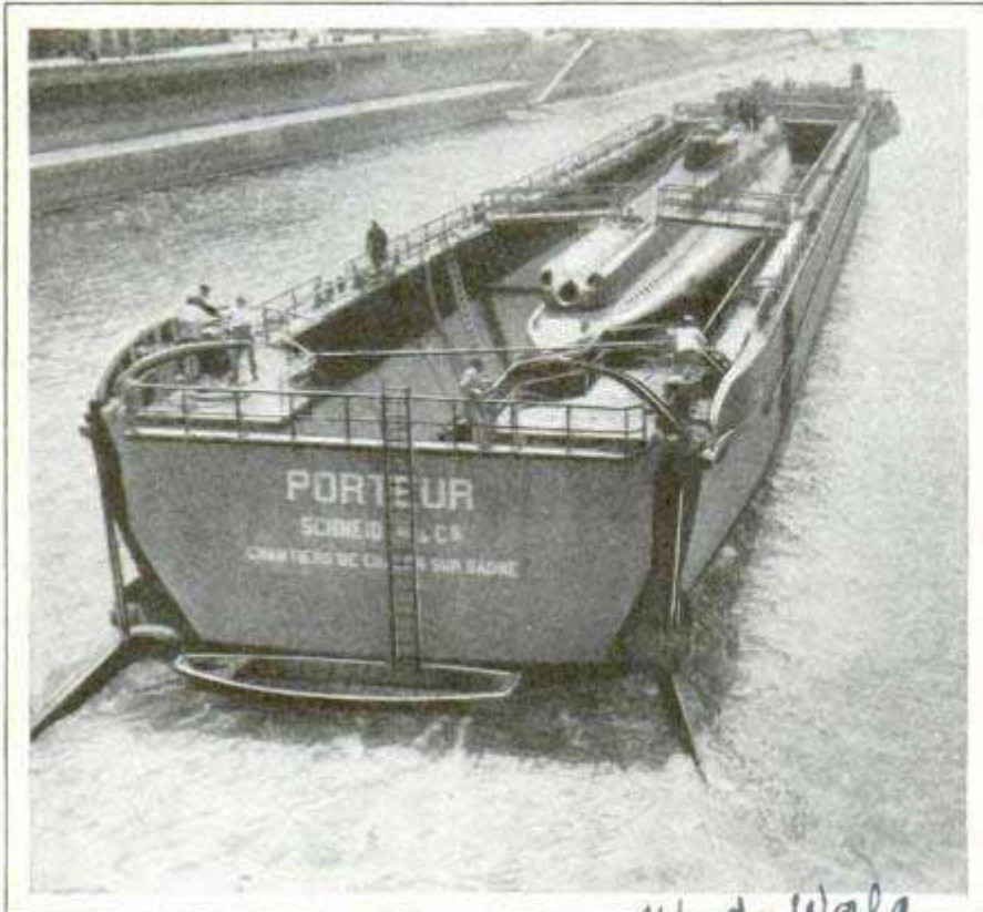
Submarine Carrier Which Was Used to Transport the Undersea Craft from the Ocean across France to the Mediterranean Sea
