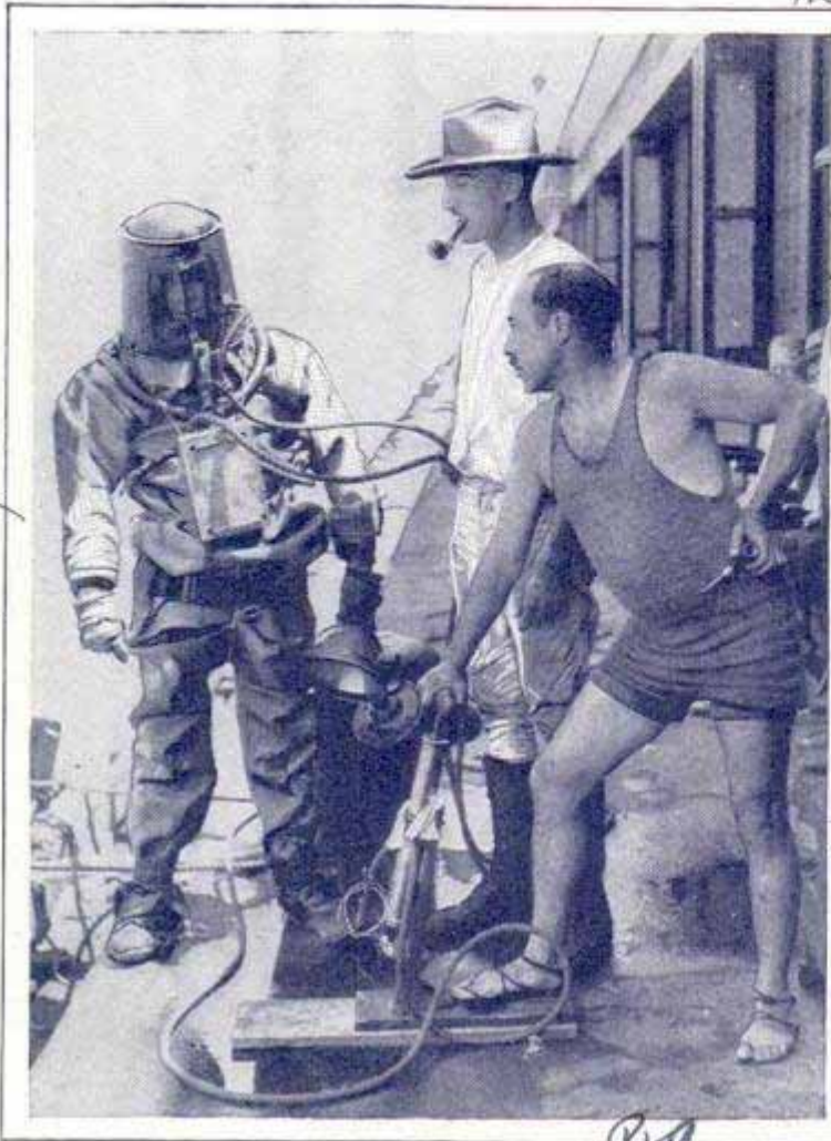
Homemade Diving Suit Constructed from Old Automobile Inner Tubes and a Few Other Odds and Ends of Material
