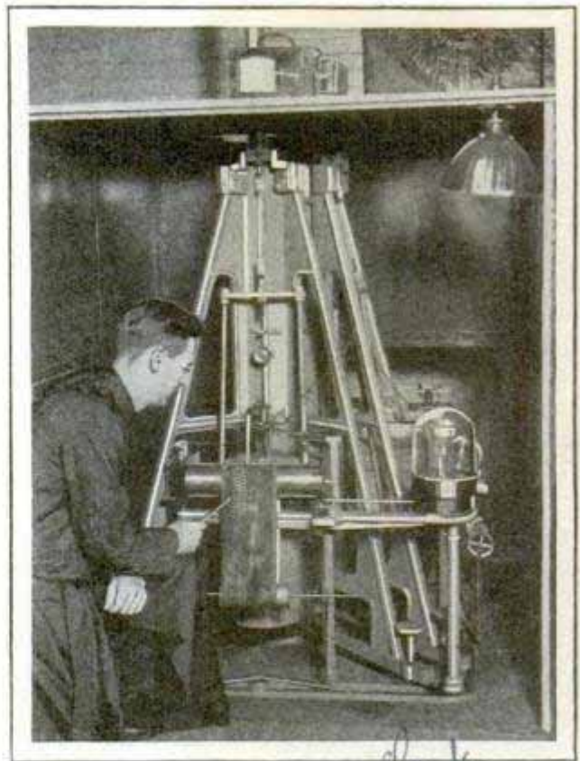
Seismograph at Georgetown University, and Chart Showing the Record of an Earthquake
