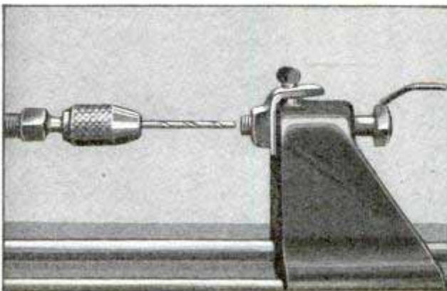
Improved Screw-Feed Attachment on Small Lathe for Feeding Work to Drill
