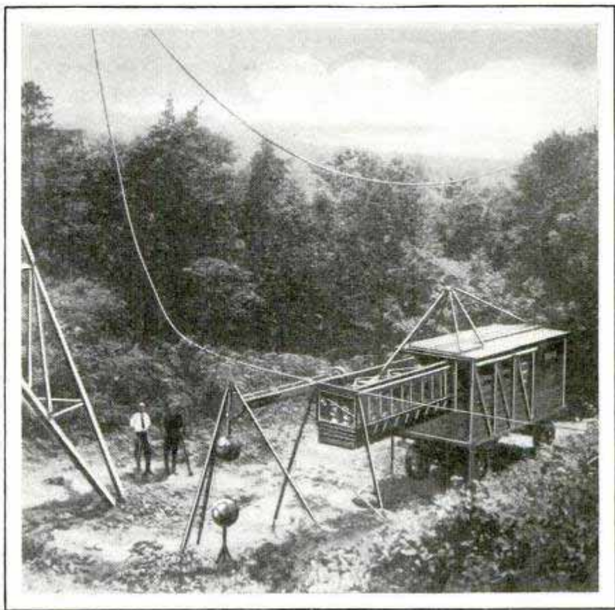
Portable Lightning Generator Capable of Developing 1,000,000 Volts, Used to Determine Effects of Lightning on Power Lines
