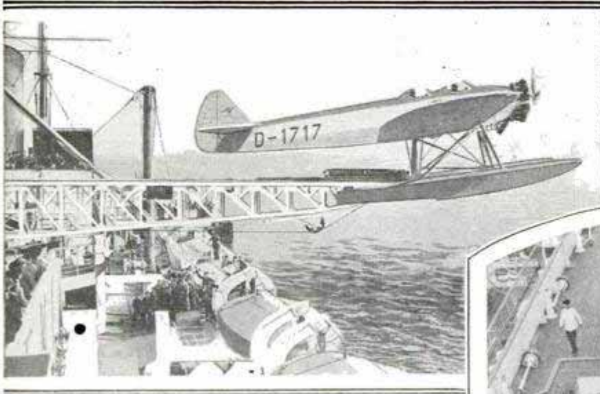
Two Views of a Catapult for Launching Airplanes from a Ship; It Is Light in Weight, but Has Unusual Strength and Dependability
