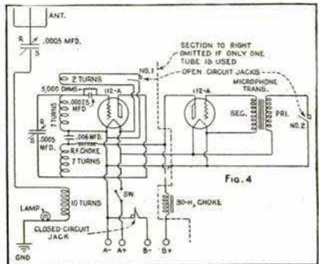
Top, Details of R.F. Choke and Homemade Microphone; Center, Assembling Parts; Bottom, Schematic Diagram of Complete Two-Tube Transmitter
