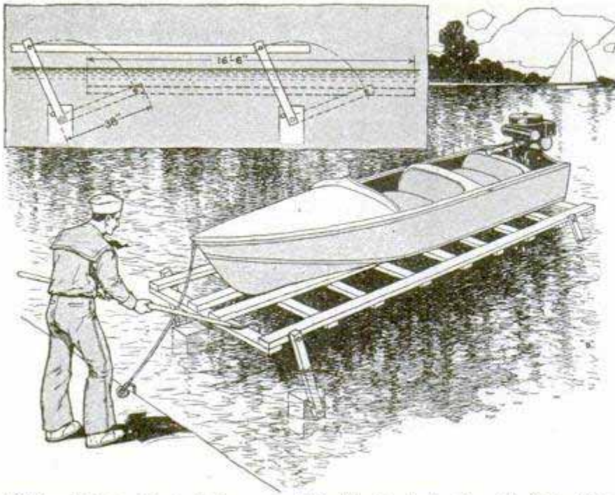
Outboard-Motor Boat, Driven over This Sturdy Rack, Can Be Pulled Out of the Water Easily
