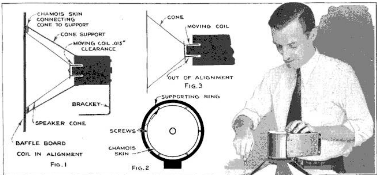
Right, Removing Retaining Ring Holding Chamois Skin to Rim; Left, Section Diagrams Showing Coil In and Out of Alignment
