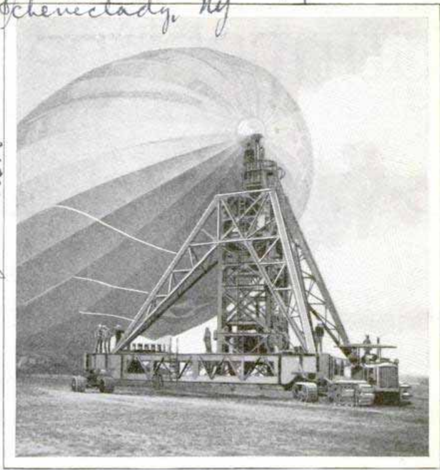
Portable Mast for Dirigible in Use; It Can Be Hauled About by a Tractor and Requires a Smaller Ground Crew
