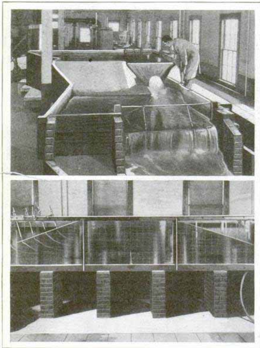
Above, Model of Dam in River Hydraulic Laboratory with Conditions at the Site Duplicated; Below, Model Section of a Proposed Dike
