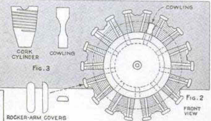
This Radial Engine for Model Airplanes Looks Realistic and Can Be Used on Flying Models
