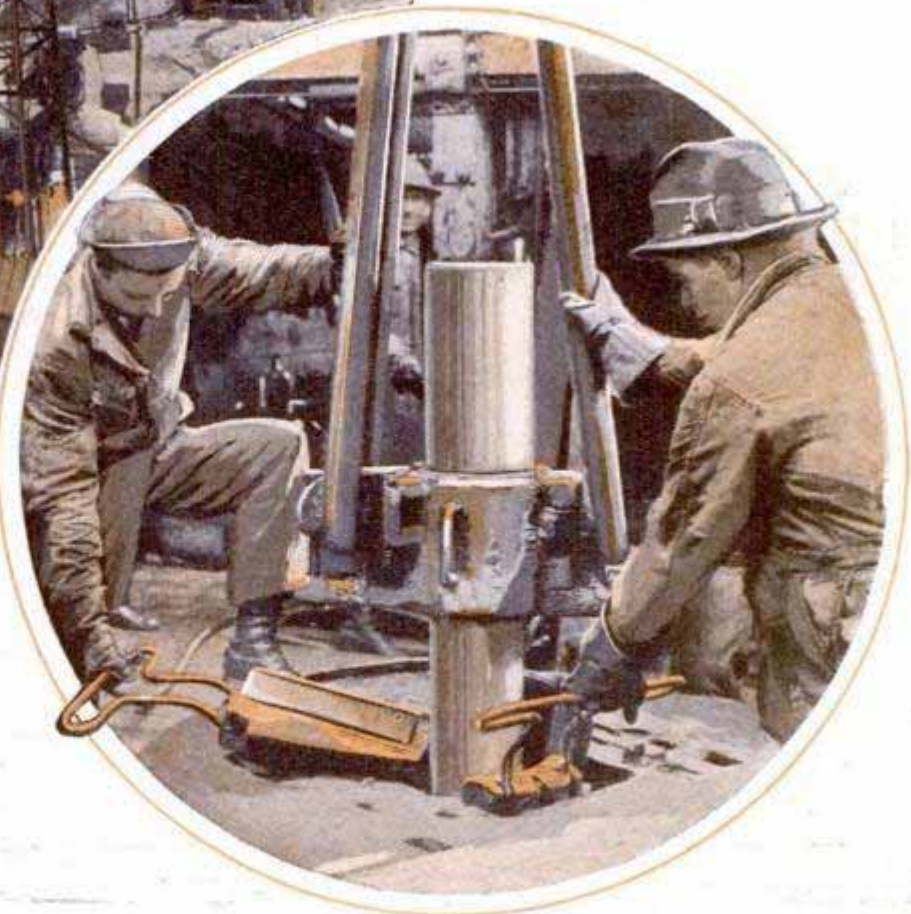
Members of the Drilling Crew Holding the Slips Which Wedge against the Drill Pipe, Preparatory to Joining New Lengths to It; They Are Getting Ready to Pull the Pipe; When One Stand Is Pulled, the Elevator Is Loosened and the Pipe Stacked against One Side of the Rigging; When Wells Descend More Than a Mile in Depth, as Many of Them Do, the Problem of Handling the Casing for So Deep a Hole Is an Expensive One
