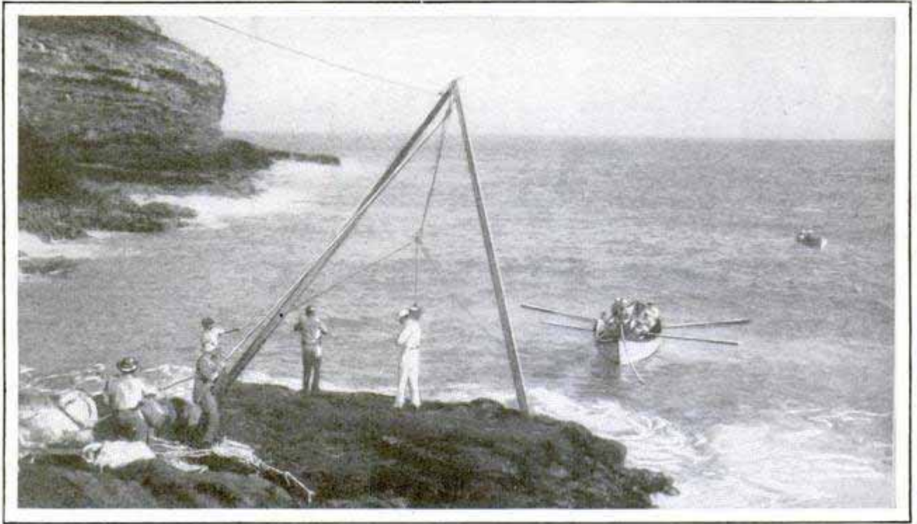
Landing the Apparatus for the Gravity Survey on Nihoa Island, Hawaii; Tests Have Been Made on Mountain Peaks, at the Equator and near the Poles, to Establish a Universal Gravity Standard
