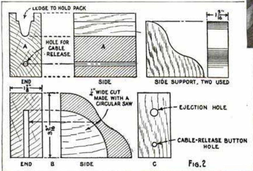
The Hole for the Cable Release May Be Drilled through Blocks A and C at the Same Time, as Shown Above, Using a Hand Drill if a Press Is Not Available
