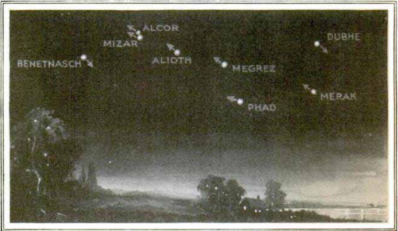
Scientists Have Found That the Big Dipper in the Sky Is Gradually Breaking Up, the Stars Composing It Moving in Different Directions as Indicated by Arrows
