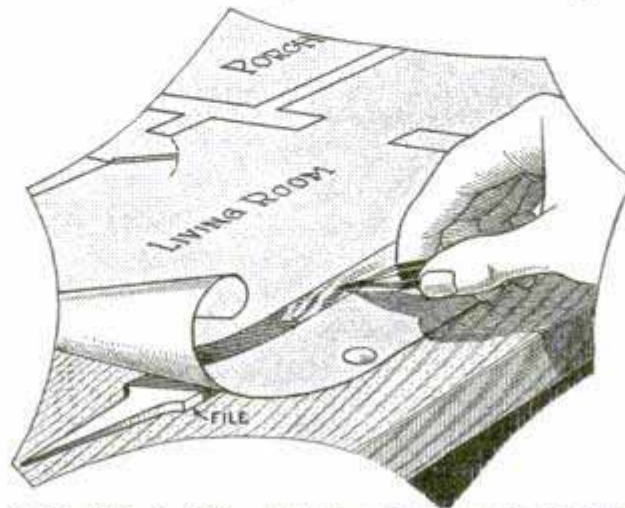
Quick Method of Crosshatching Partitions in Drafting Building Plans
