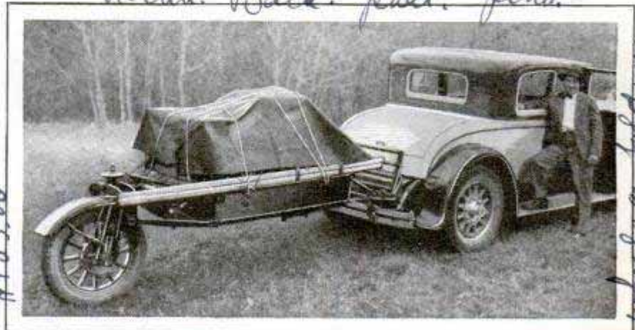
One-Wheeled Trailer Loaded and Attached to Car; the Single Wheel Adjusts Itself to Backing or Forward Travel
