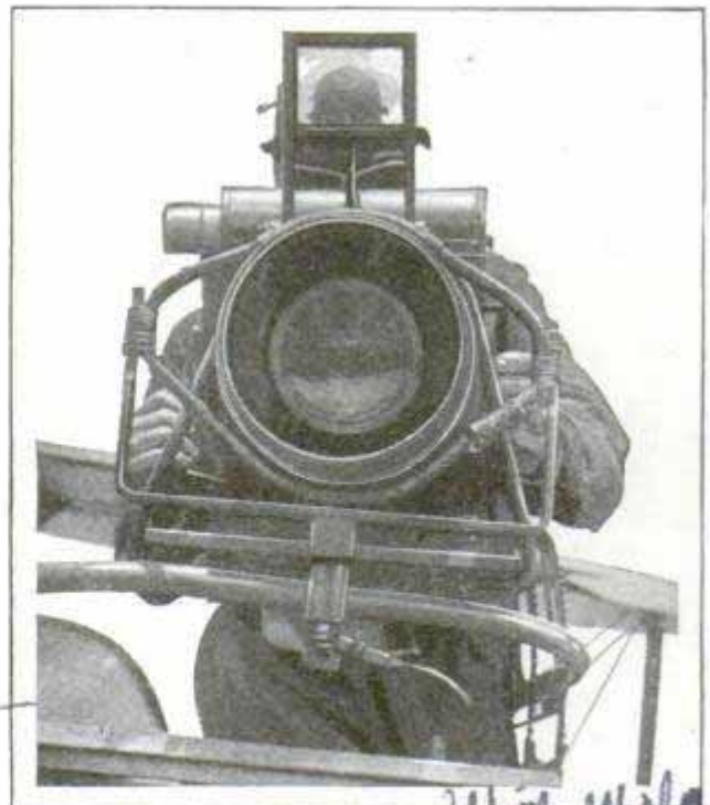
Aiming One of the Monster Aerial Cameras Developed Especially for Army Use
