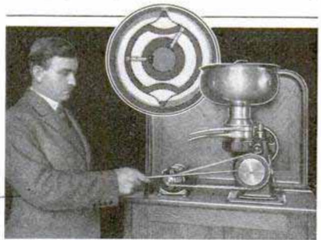
Sectional View of the Gear-Shift Substitute, and Device Employed on Cream Separator
