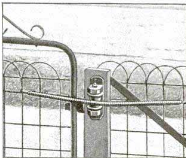
Effective Method of Attaching Coil Spring to Gate to Obtain Necessary Leverage
