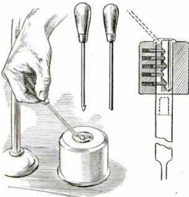
Broken Keys in Auto Locks Can Be Removed with the Aid of These Tools
