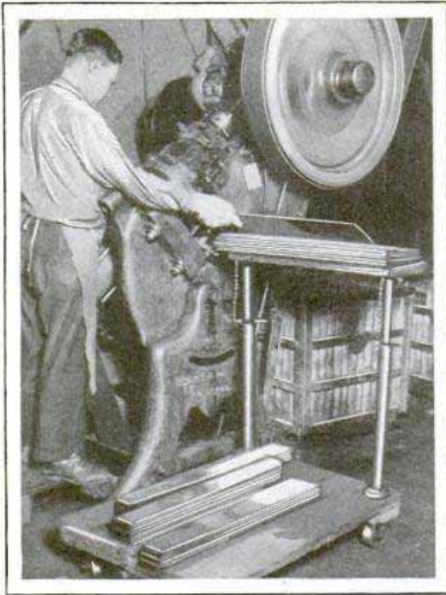
Work of Punch-Press Operator Made Easier by This Adjustable Table Attached to Truck
