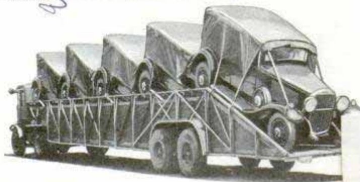
Cars Loaded at an Angle on Frames in Auto Trailer, Thus Allowing Five Autos to Be Hauled Instead of Three
