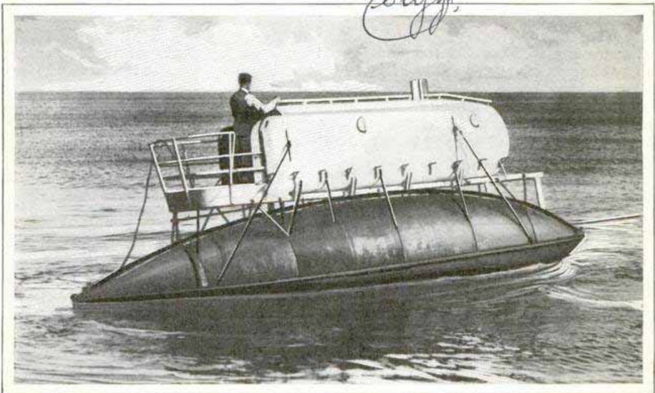
Queer Motorboat German Engineer Has Built for a Possible Trip across the Atlantic; It Has a Water-Tight Compartment or Cabin Mounted on the Torpedo-Shaped Hull
