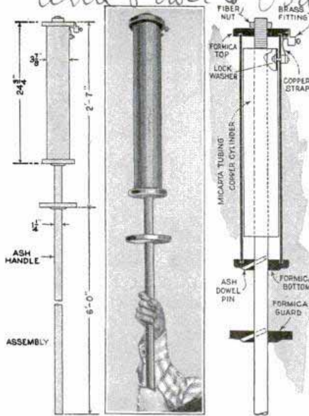
This Indicator Stick Protects Linemen from Dangers Involved in Working on High-Tension Lines
