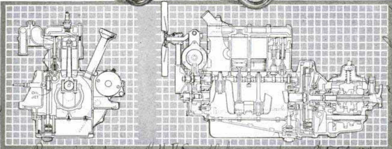
The Austin Two-Passenger Coupe, and Two Views of Its Power Plant; the Squares in the Background Represent Inches, Showing, for Example, That the Cylinder Block Is Only About a Foot Long
