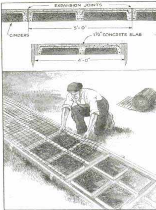
Reinforced Cement Sidewalks Require Less Material and Are Stronger Than Walks of the Usual Kind
