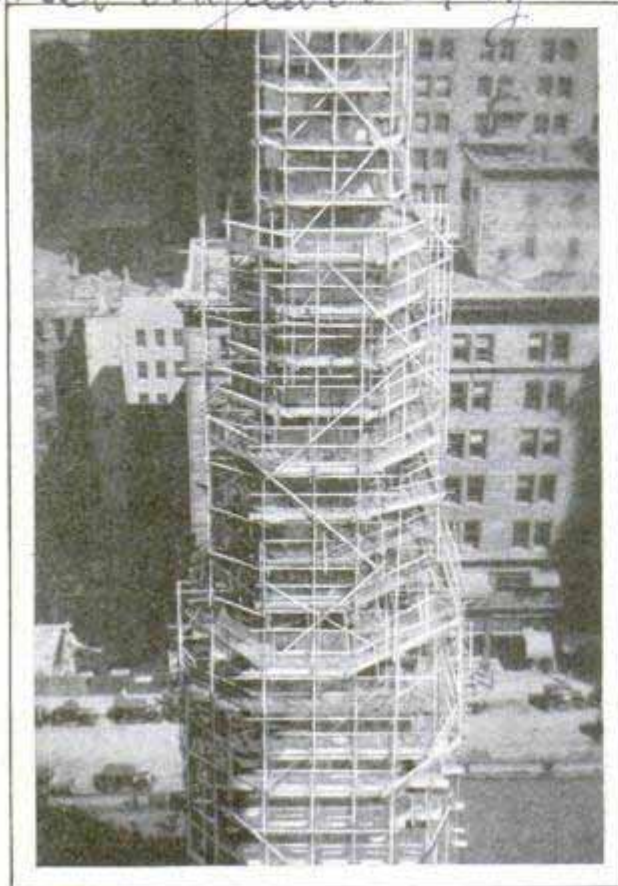
Steeple of St. Paul's Church, New York, as It Appeared Surrounded by Scaffolding during Repairs
