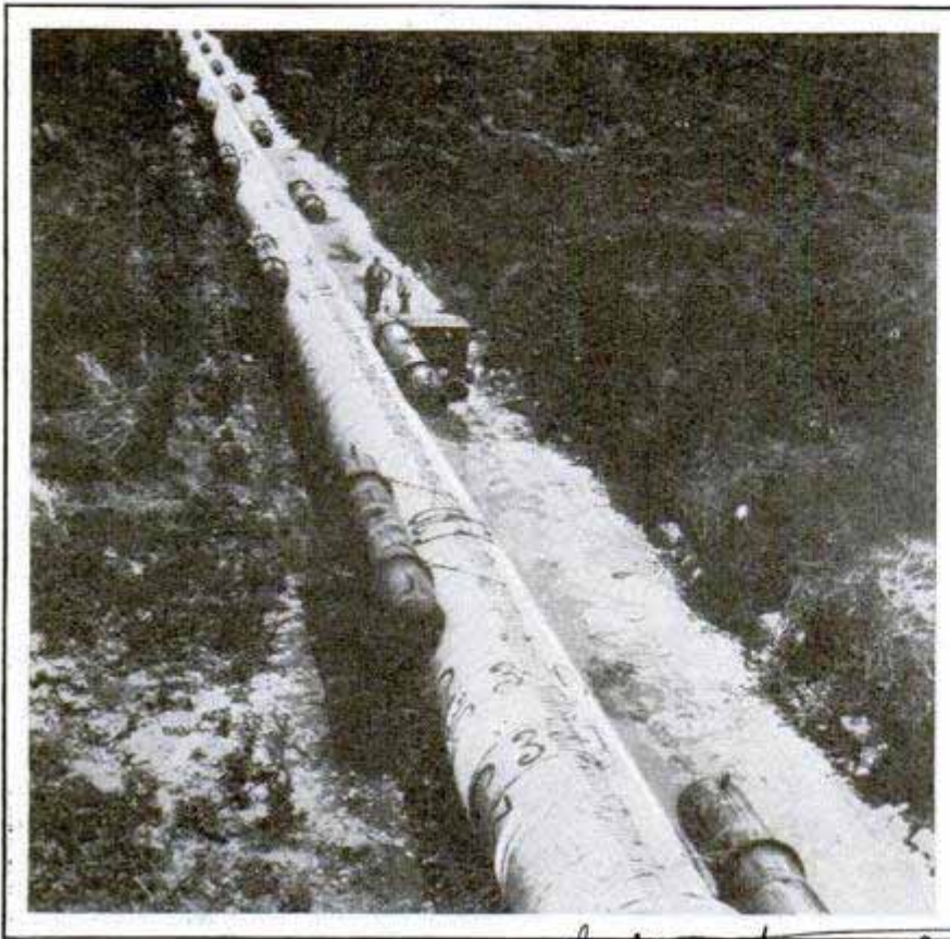
Section of Mile-Long Pipe as It Was Being Towed on Pontoons to a Position in the Gulf Stream; It Sank Before It Was in Place
