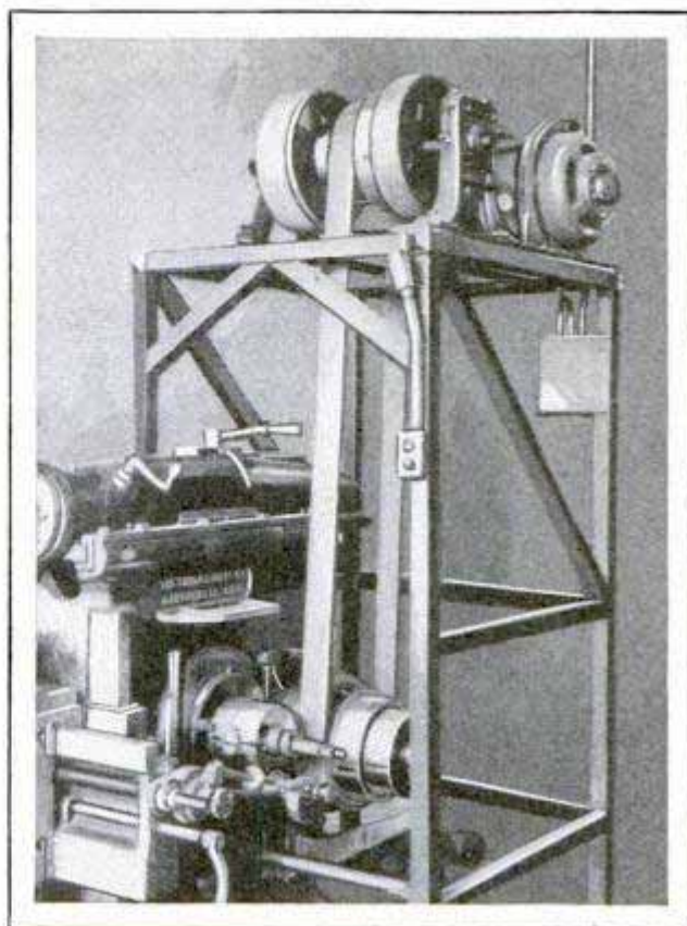
Individual Motors for Machines Supported on Frame Made of Steel Tubing
