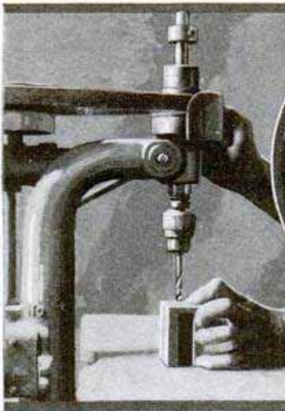
The Hole for the Cable Release May Be Drilled through Blocks A and C at the Same Time, as Shown Above, Using a Hand Drill if a Press Is Not Available
