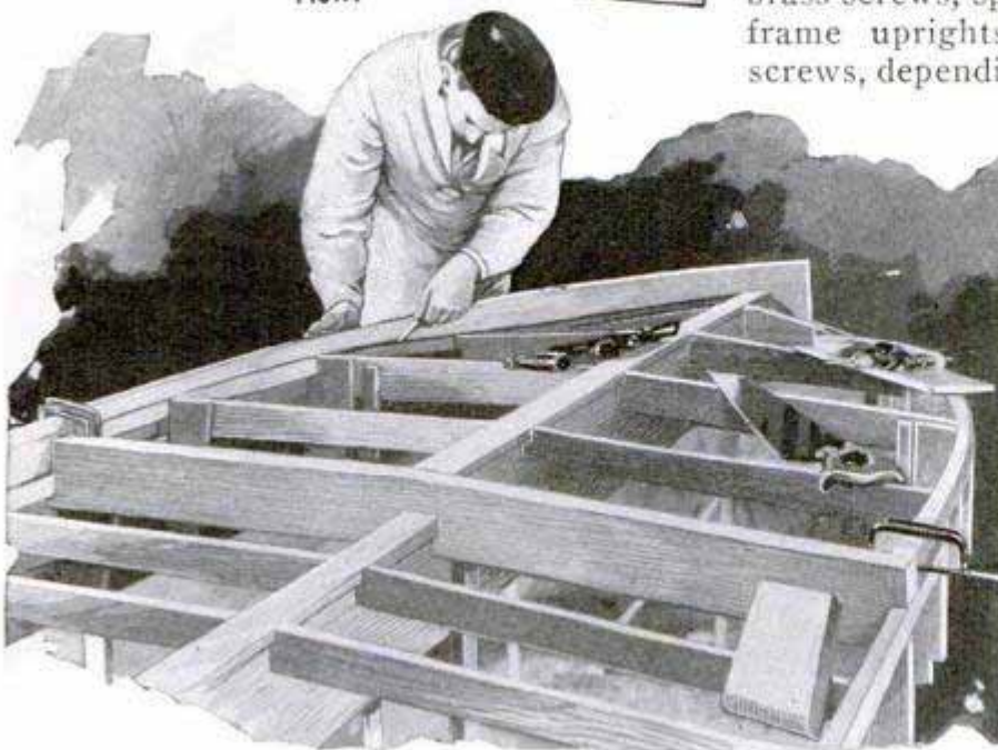
Side Planking Clamped On to Be Marked for Sawing. After Which Marine Glue and Tape Are Applied to the Frame Members
