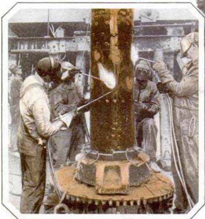
Below, Welders Riveting Twenty-Inch Stovepipe Casing before Lowering It into the Hole; This Casing Serves as a Guide for Later Drilling; at Right, Setting the Slips, the Wedges That Support the Pipe Temporarily While It Is Being Pulled Upward from the Hole
