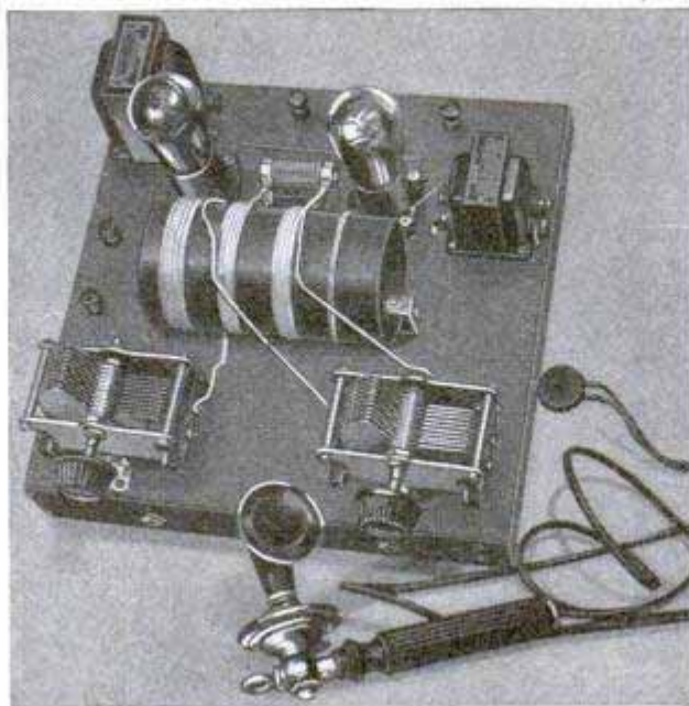
Completed Short-Wave Radiophone with Hand Microphone Plugged in at Phone Jack No. 2
