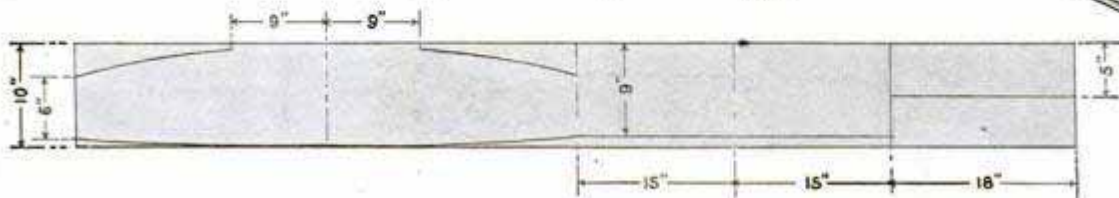
FIG. 13 HOW STERN IS CUT FROM 8 FT. BOARD
