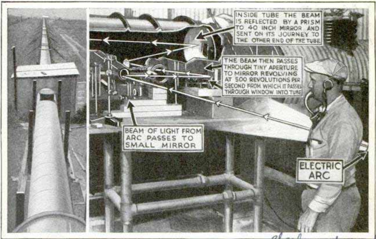
Photo-Diagram of the Mile-Long Pipe "Runway" Where Speed of Light Is Being Checked, and Arrangement of Mirrors for Reflecting the Rays
