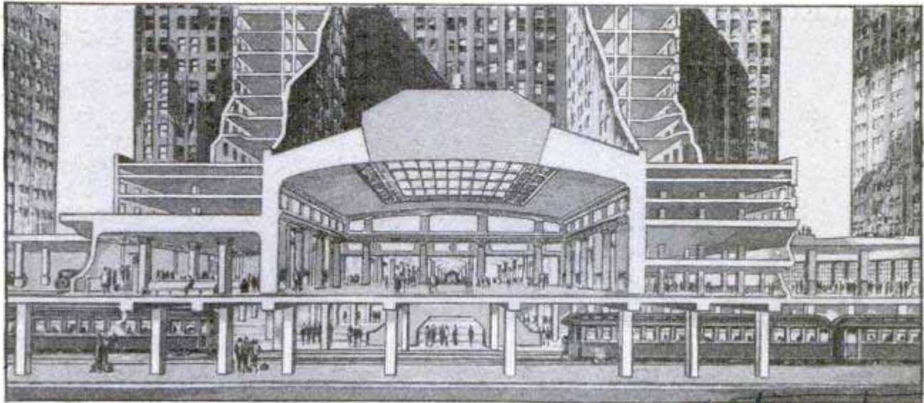
Cross-Section Drawing, Showing How Trains and Other Conveyances Pass under Union Terminal Building in Cleveland; a Hotel, Bank, Office Building and Station Are under One Roof.
