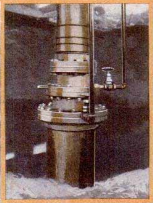
From a Roaring Deluge of Flame, an Oil Well Is Transformed to a Harmless-Looking Pipe in the Ground, as Shown Above; the Mouth of a Well That Had Blazed for More than Seven Weeks Before It Was Successfully Capped with the Fittings Illustrated; Below, a Gas Well on Fire in the Santa Fe Springs Area, California; While a Blazing Well Alone Often Means a Loss of Fortunes, the Fire Is Particularly Feared for What It May Do to the Surrounding Derricks and Buildings
