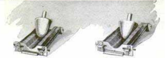
Courtesy The Sphere Enlarged Point of Phonograph Needle at Various Stages of Wear and Model of Record Groove
