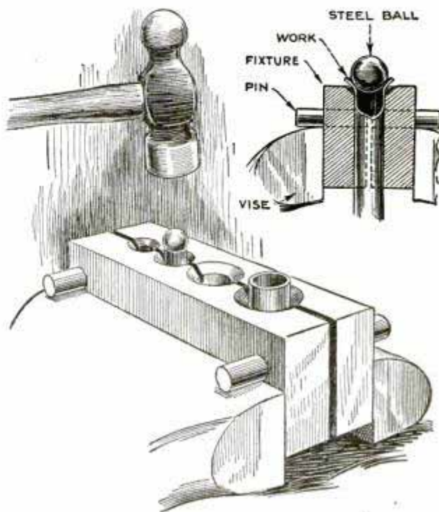
Fixture Holds Tubing While Flaring Out End with a Steel Ball
