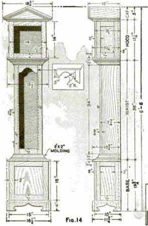
side view of the clock case assembled, and the names of the different units. In general, the various parts of the units are
