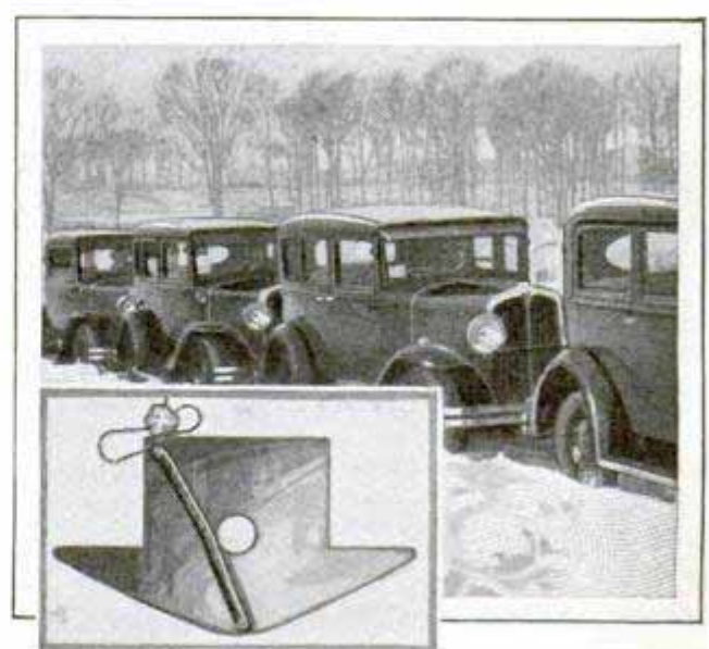
Autos En Route from Factory to Dealer Are Equipped with This "Hobble," Limiting Their Speed
