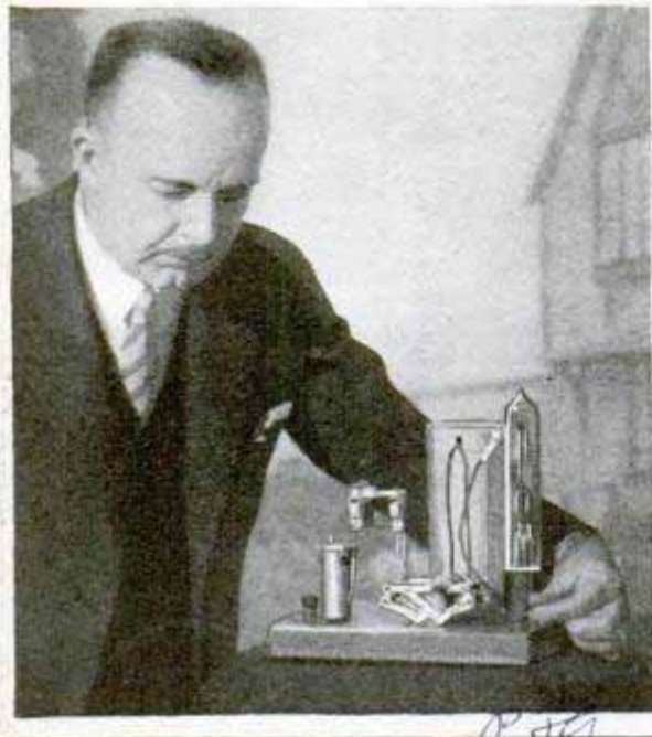
Model of Ultraviolet-Ray Burglar Alarm; Interruption of the Invisible Rays Rings an Alarm
