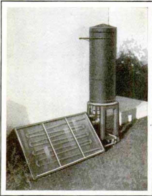
Actual Installation of Solar Heater Which Has Given Satisfactory Results
