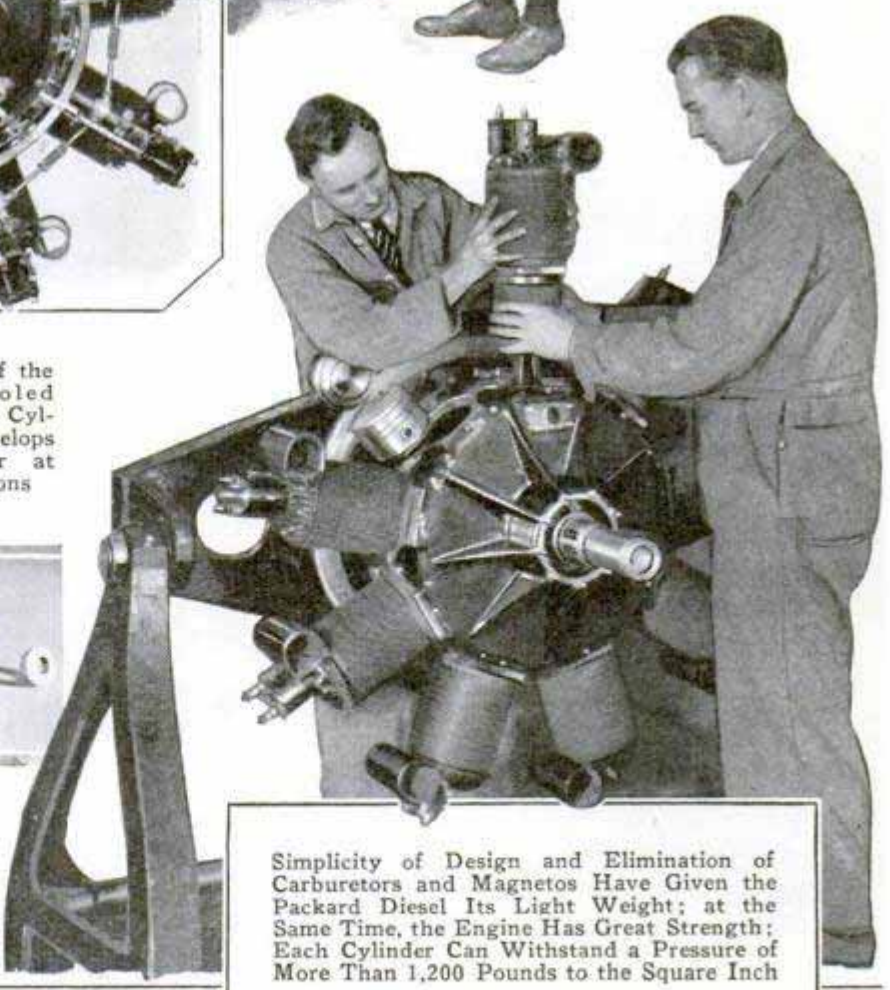
The Engine Weighs Only 510 Pounds or 2.26 Pounds per Horsepower, Exceptionally Light for Diesels; Each Cylinder Weighs Eleven and Three-Fourths Pounds
