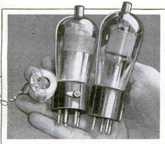
Right, Old Type Screen-Grid Tube; Center, New Five-Element Tube; Left, Tube with Glass Removed
