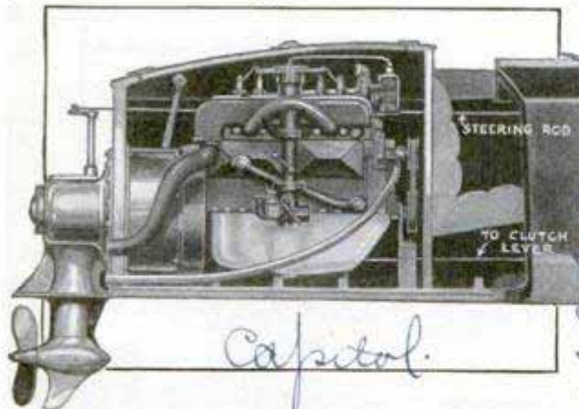
Stern Drive and Reverse Gear Arrangement for the Small Motorboat
