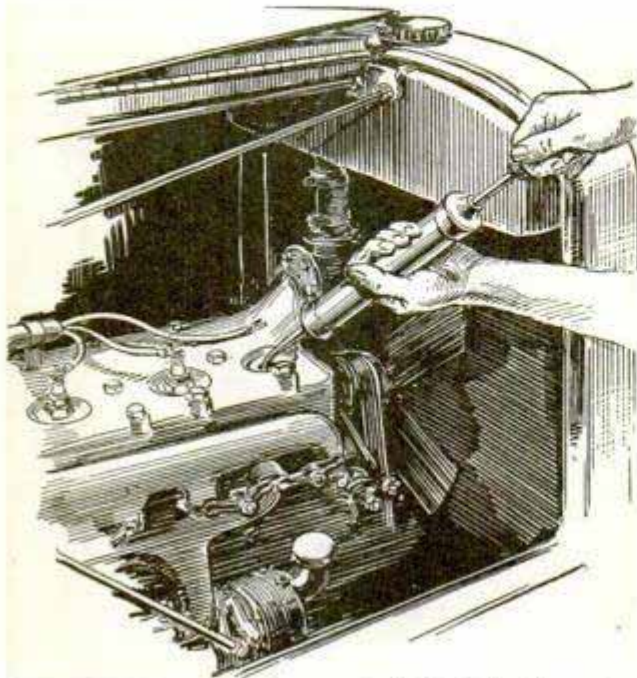
Using Oil Gun and Denatured Alcohol for Removing Carbon in Auto Motors
