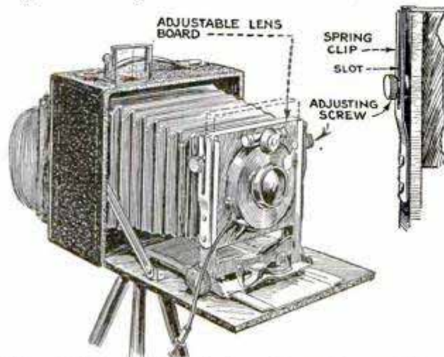
Clips Made from Clock Springs Prevent Loss of Lens-Board Thumb screws
