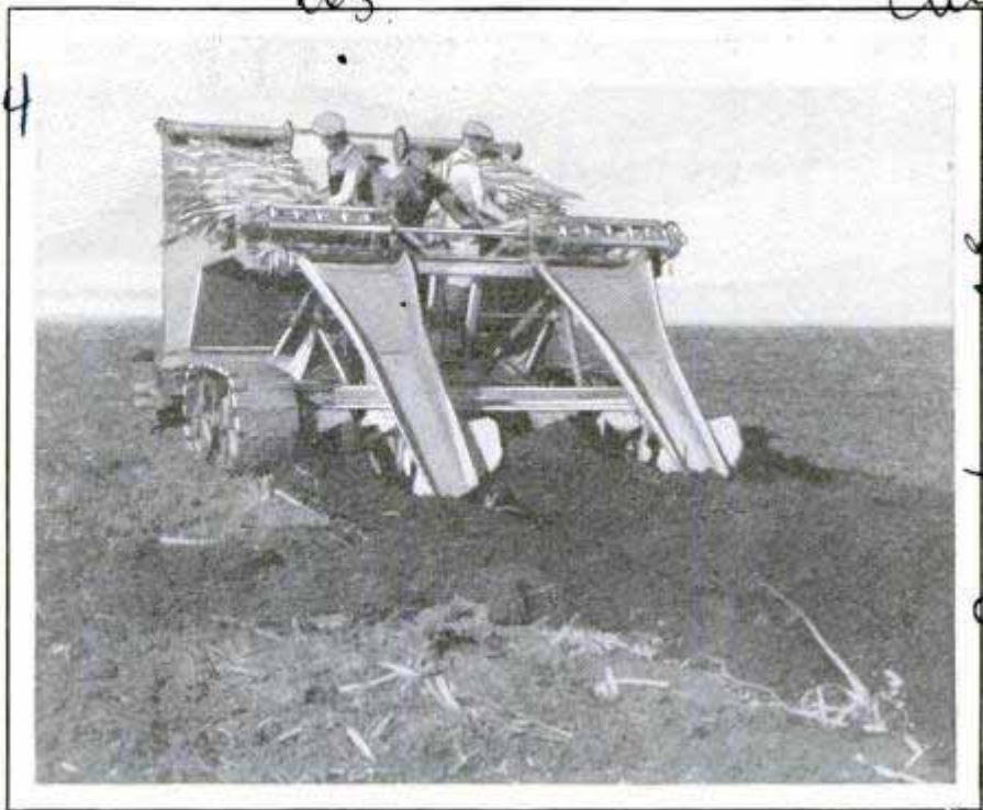
Sugar-Cane Planter Which Plows and Sets Two Furrows of Seed Stalks Simultaneously, Work That Formerly Required Twenty Men
