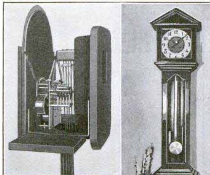
Above, Grandfather-Clock Movement Fitted with Westminster Chimes, Ready for Installation; Right, the Finished Clock, Made as Described in This Article
