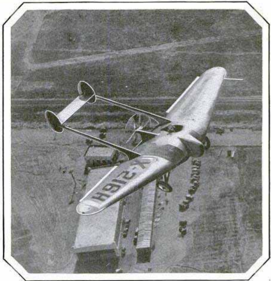
"Flying Wing" Airplane Which Is Virtually All Wing and without Fuselage; Cockpit and Landing Gear Are Fitted in the Big Wings
