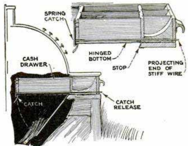
Bills in Cash Register Dumped into Lower Box Foils Holdup Attempts
