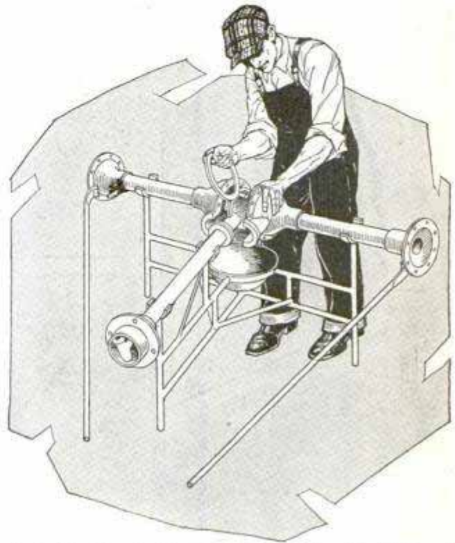
Rack for Overhauling Rear Ends Can Be Made of Half-Inch Pipe, Welded at the Joints
