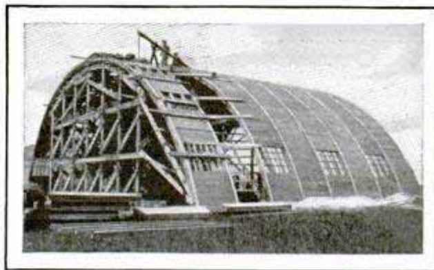
Sections of a Continuous Arch Hangar Which Is Constructed without Either Beams or Girders
