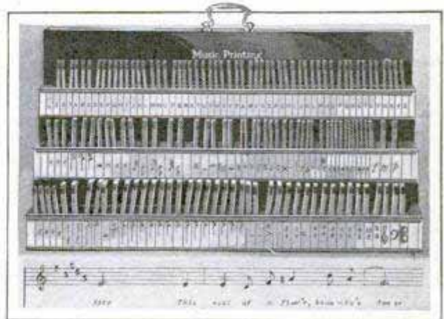
Machine for Printing Music Which Is Simple in Operation and Intended for the Novice
