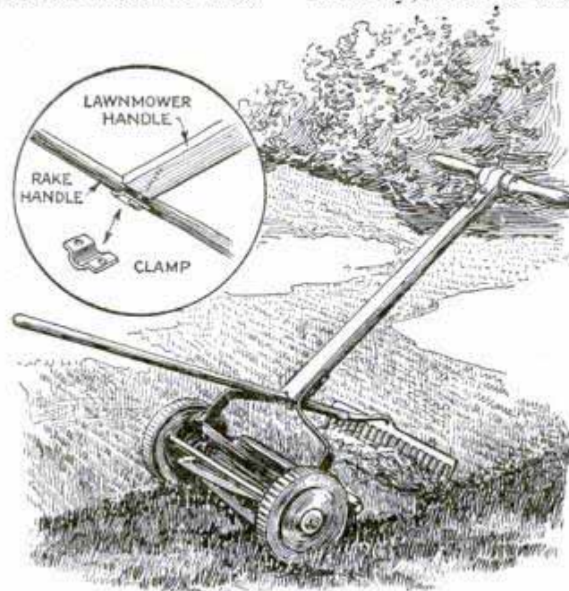
Rake Attached to Lawn Mower Picks Up the Grass While Mowing
