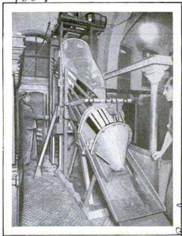
Apparatus in a German Packing Plant Which Electrocutes Hogs at the Rate of 200 an Hour
