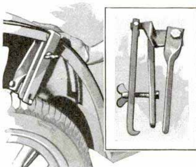
Simple Clamp Made of Bar Stock Holds Broken Fender in Position for Welding
