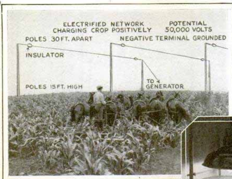
Diagram Showing Wiring High above Plants to Permit Cultivation, and Apparatus for Growth Experiments with Electric Lamps
