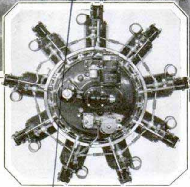
The Engine Is of the Radial Air-Cooled Type with Nine Cylinders; It Develops 225 Horsepower at 1,900 Revolutions
