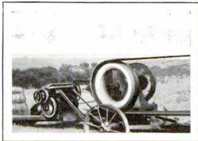
Old Tractor Tire Slipped on Flywheel of Gasoline Engine Prevents Belt from Coming Off
