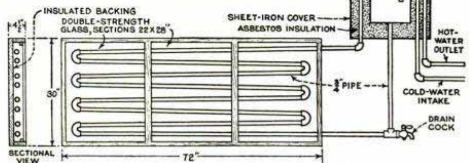
Storage Tank and Heating Coil of the Solar Heater, Showing Arrangement of Piping and Dimensions
