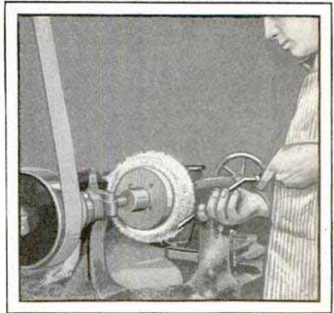
Buffer Made of Canvas Disks Puts a Keen Edge on Woodworking Tools
