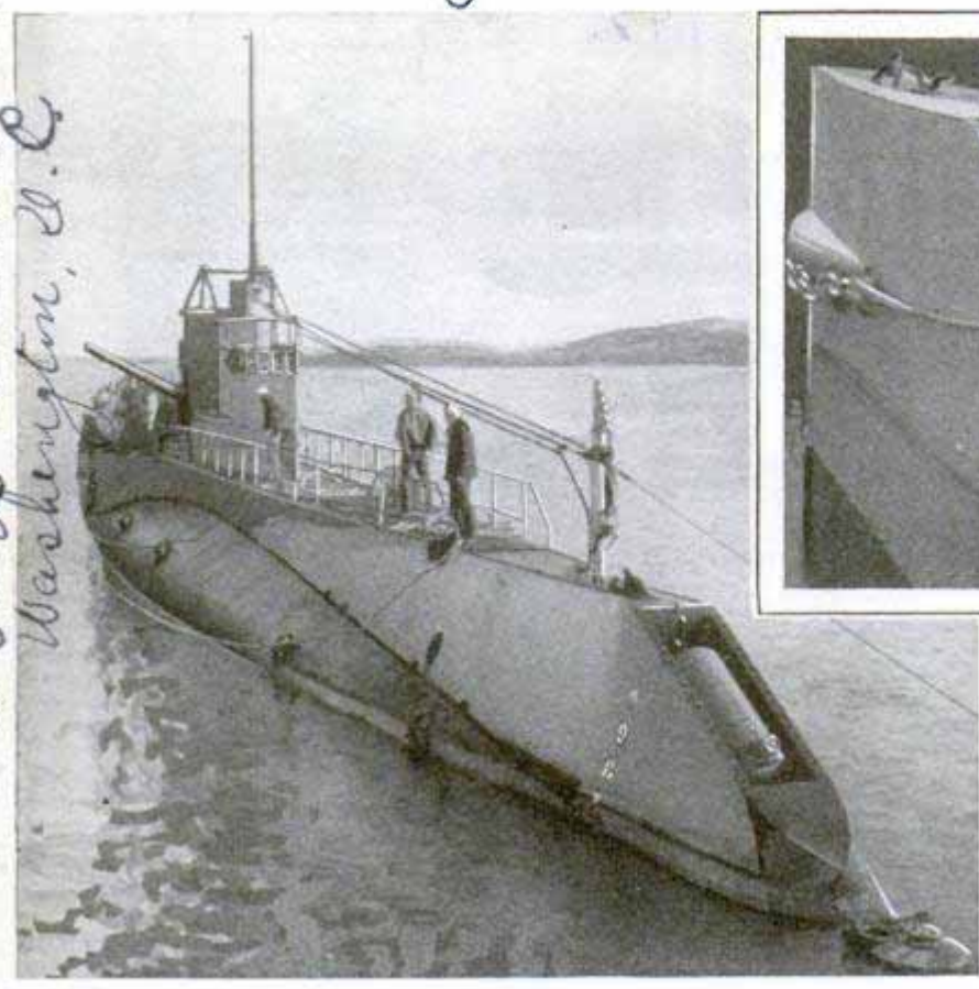
Above, Testing Undersea Telephone on a Submarine; at Right, Front View of Sub, Showing How the Telephone Buoy Is Housed
