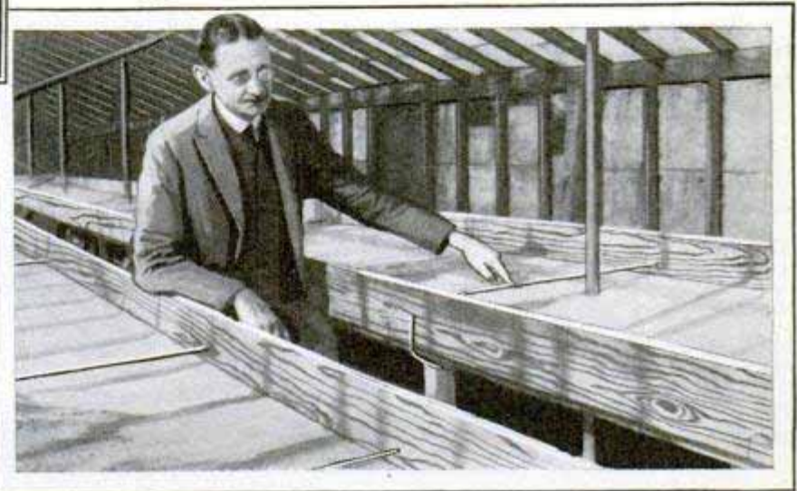
Concrete Potting Benches Supported by Pipe Uprights; the Side Boards Are Held in Place by Means of Heavy Tie Wires
