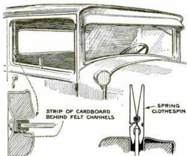
Simple Methods Are Effective for Stopping Car Windows from Rattling
