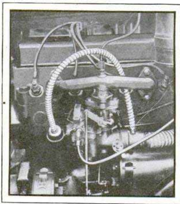
Metal Tubing from Breather-Pipe Cap to Carburetor Intake Conducts Oil Fumes into Motor
