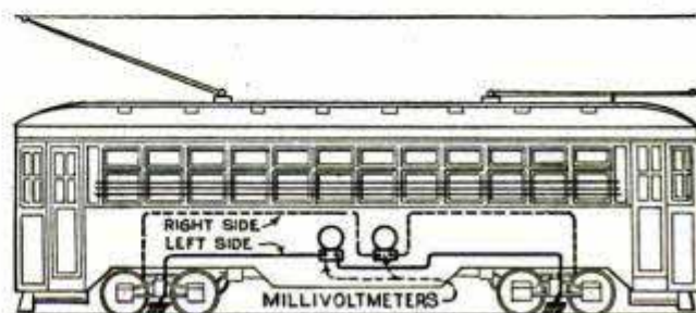
Street Car Equipped with Meters and Brushes Detects Radio Interference Caused by Track Breaks
