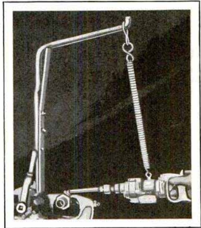
Holder for Air Tools, Made of Steel Rod and Coil Spring, Relieves Worker of Strain
