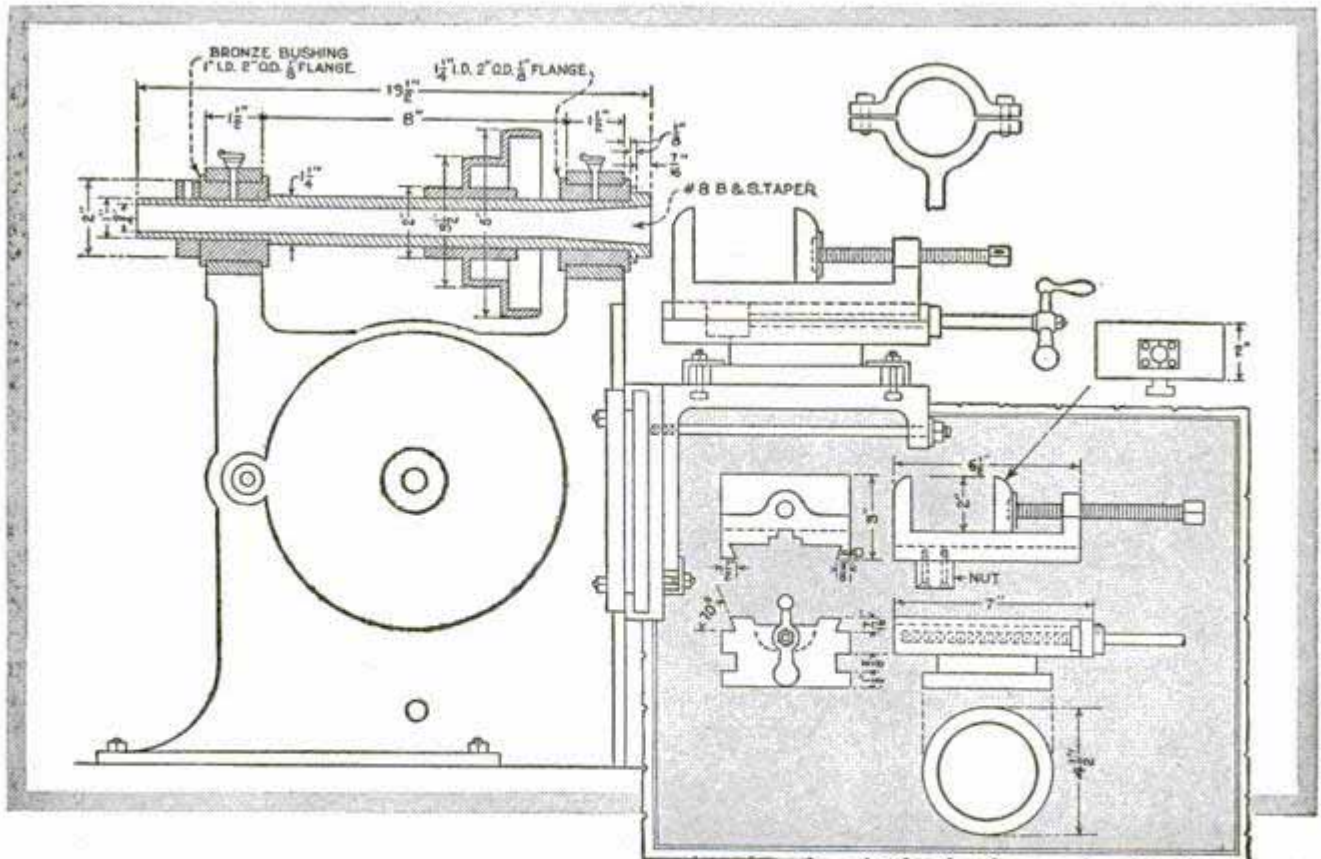
Adapted from the Sturdy Shaper Designed for Popular Mechanics by J. V. Romig, This Milling Machine Has Proved Very Useful in a Small Shop; the Change from Shaper to Miller Is Made in a Few Minutes
