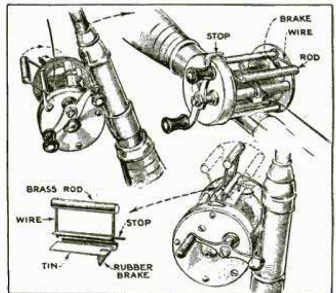
Two Variations of a Reel Backlash Stop to Prevent Tangled Lines When Fly Casting
