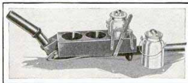
Sheet-Metal Stove Uses Exhaust Gas for Heating Motorists' Food While Driving
