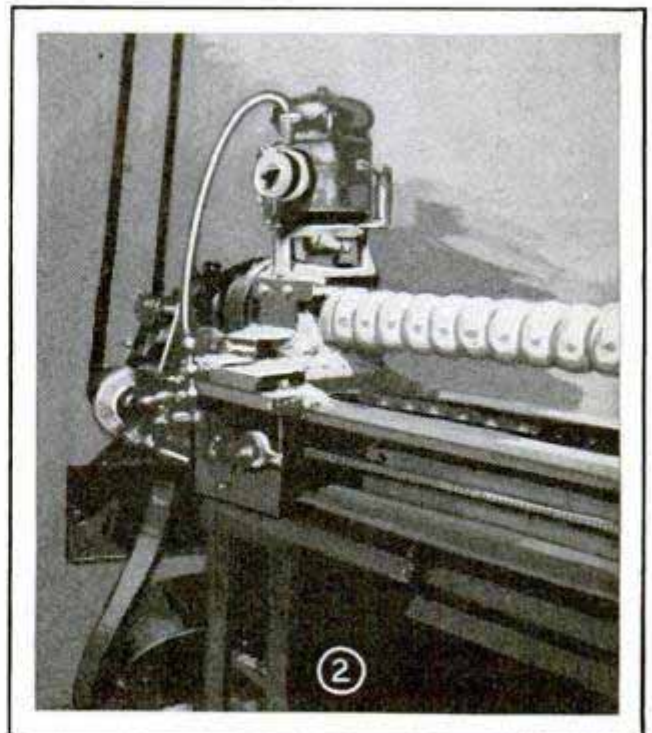
Completely Finished Spiral after Making Two Cuts with the Router
