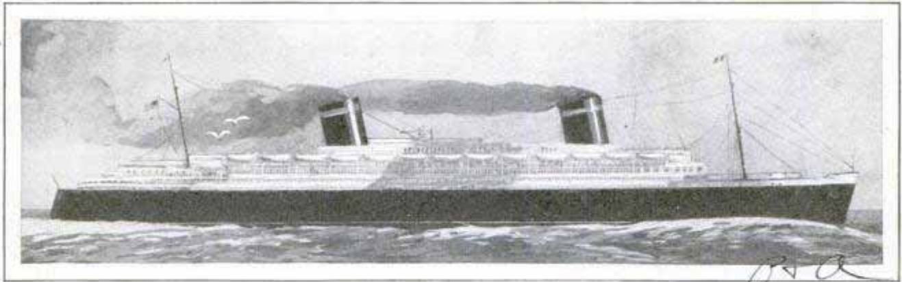
Drawing of One of Two Giant Liners Which United States Lines Will Build in Struggle for Transatlantic Trade; It Will Be Faster Than the "Bremen" and Longer Than the "Leviathan"
