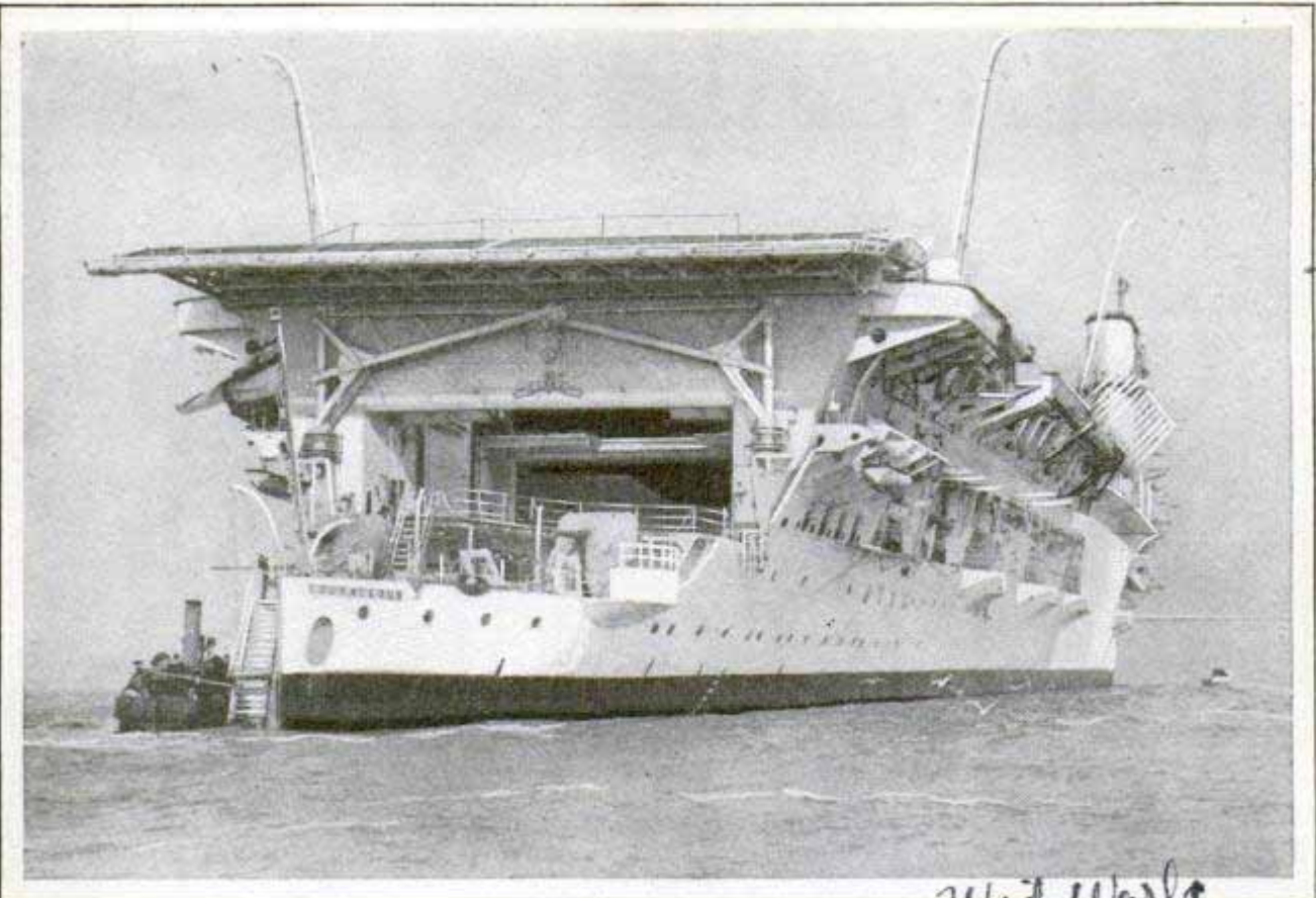
One of the Most Striking Vessels Afloat Is This Airdrome, the British Aircraft Carrier "Courageous"; It Is Mother Ship for Dozens of Seaplanes Attached to the Fleet.
