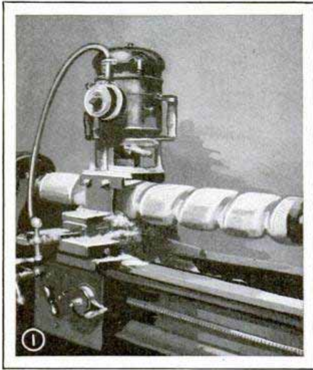
Cutting Spirals of Considerable Pitch by Using a Portable Router on a Machine-Shop Lathe
