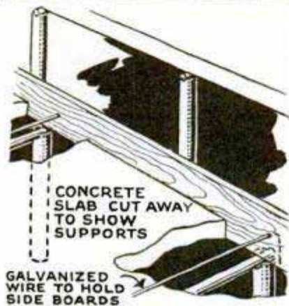
Concrete Potting Benches Supported by Pipe Uprights; the Side Boards Are Held in Place by Means of Heavy Tie Wires
