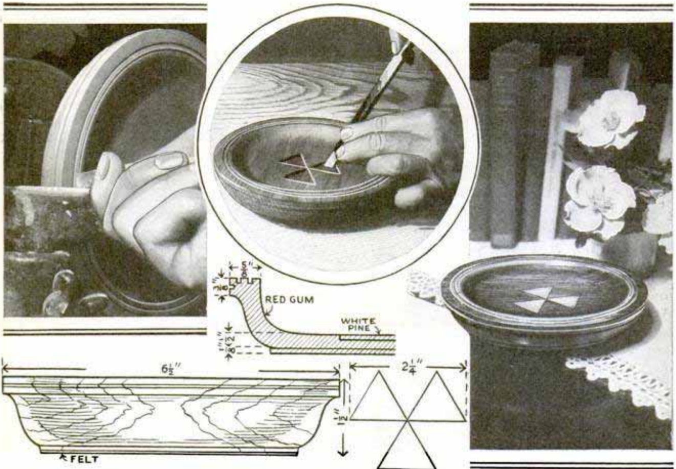
Left, Cutting the Grooves for the Line Inlays; Center, Cutting Out for Triangle Inlays; Right, the Completed Tray; Below, Sketch and Section of Tray, Showing How Grooves Are Cut
