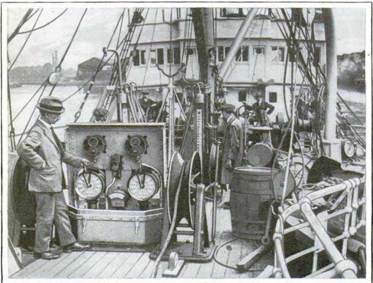
Equipment on the Deck of a Cable-Laying Ship Which Controls the Paying Out of a Cable, a Task Requiring Much Skill and Care
