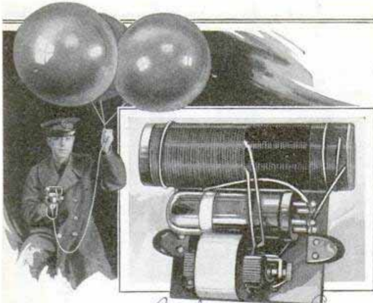
Three Balloons to Which Are Attached Radio Instruments for Recording Weather Conditions, and Recording Apparatus
