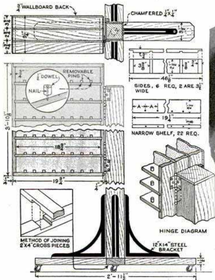
With This Cabinet, All Small Parts Are Easily Found When Wanted and the Cabinet May Be Moved Close to the Job, If Desired
