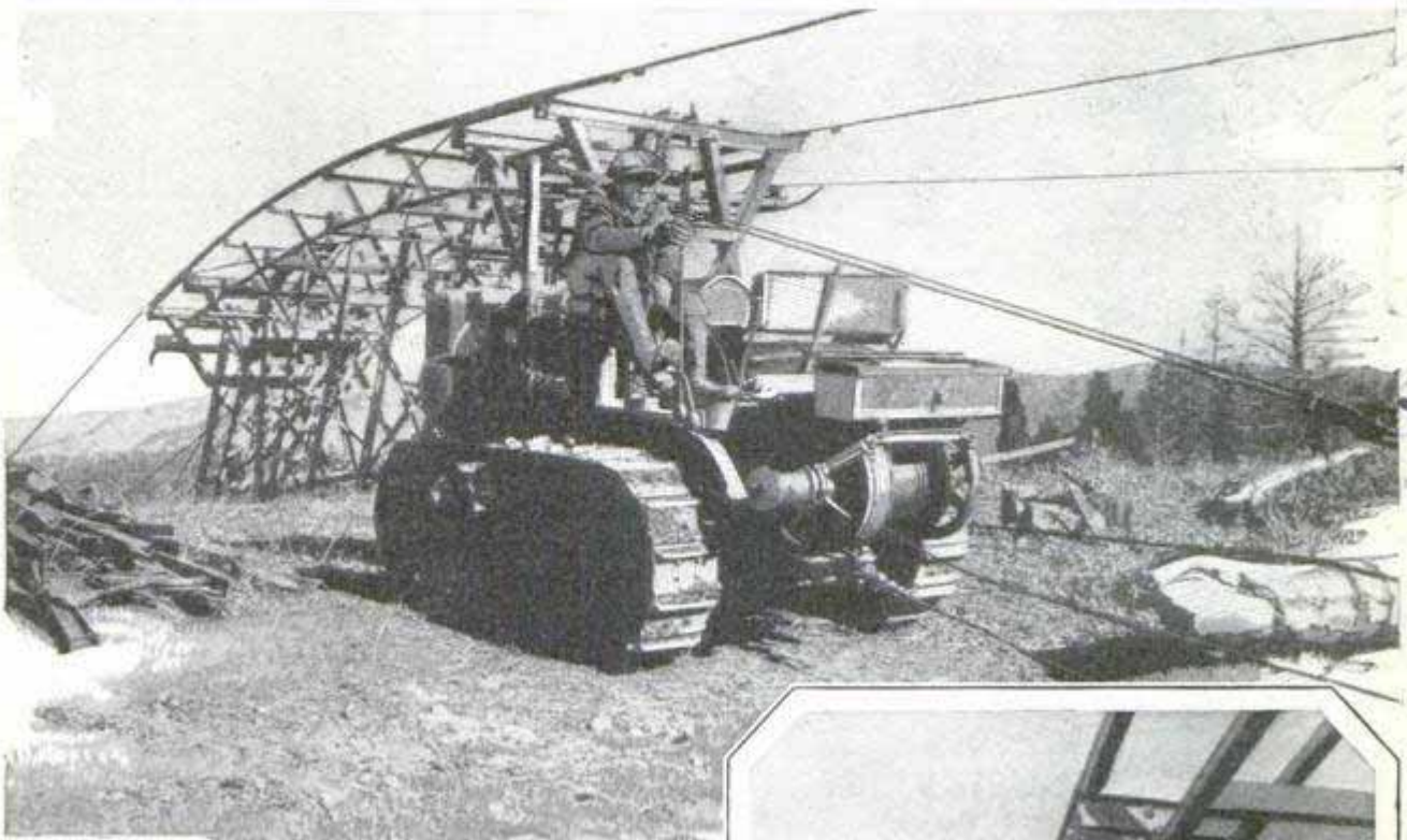
Single-Drum Winch Attached to a Tractor Used to Operate Mining Tramway over a Canyon When the Machinery Failed
