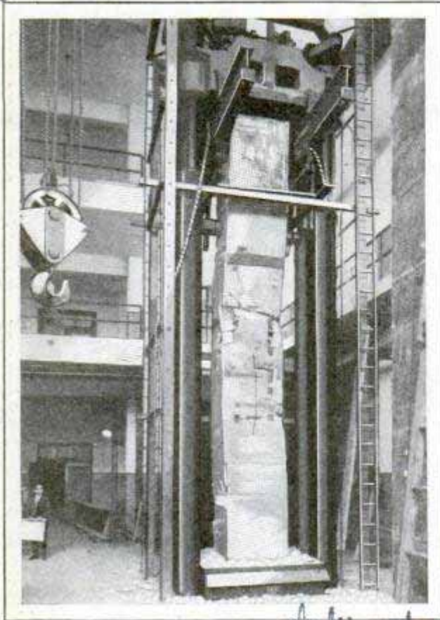
"Nutcracker" Which Tests Bridge Columns, and a Column Which Has Crumpled from Its Impact
