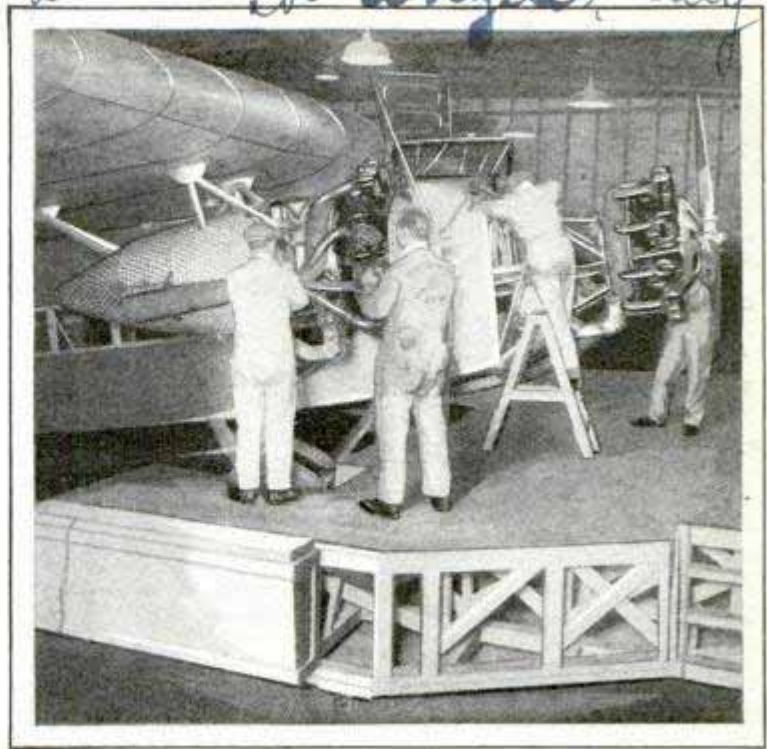
Portable Service Platform for Airplanes Which Gives Mechanics Easy Access to All Parts of the Engine
