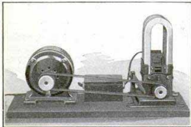
Magneto Driven by Motor Used to Furnish A.C. Source for Step-Up Transformer
