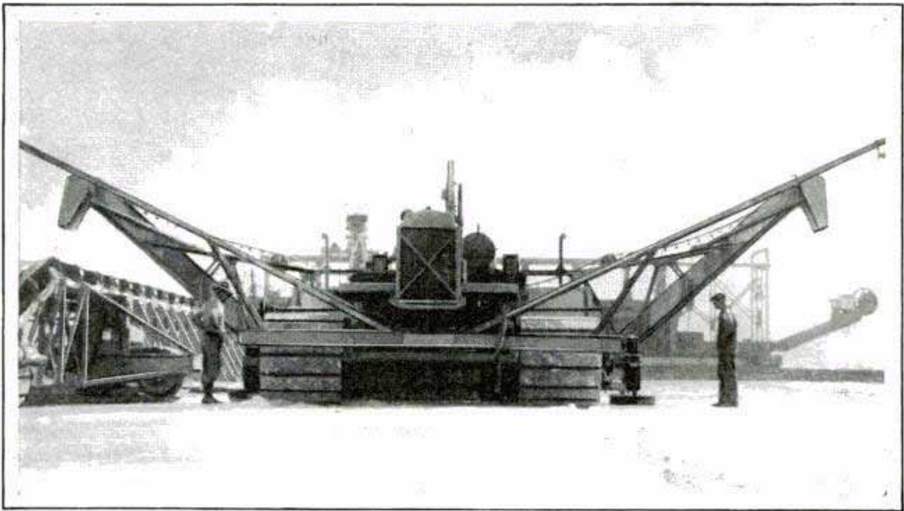
* Tractor with Rotary Digger Used on Salt Farm; the Salt Is Elevated to Conveyors and Carried to a Barge, Another Tractor Towing the Barge by Canal to the Cleaning Plant
