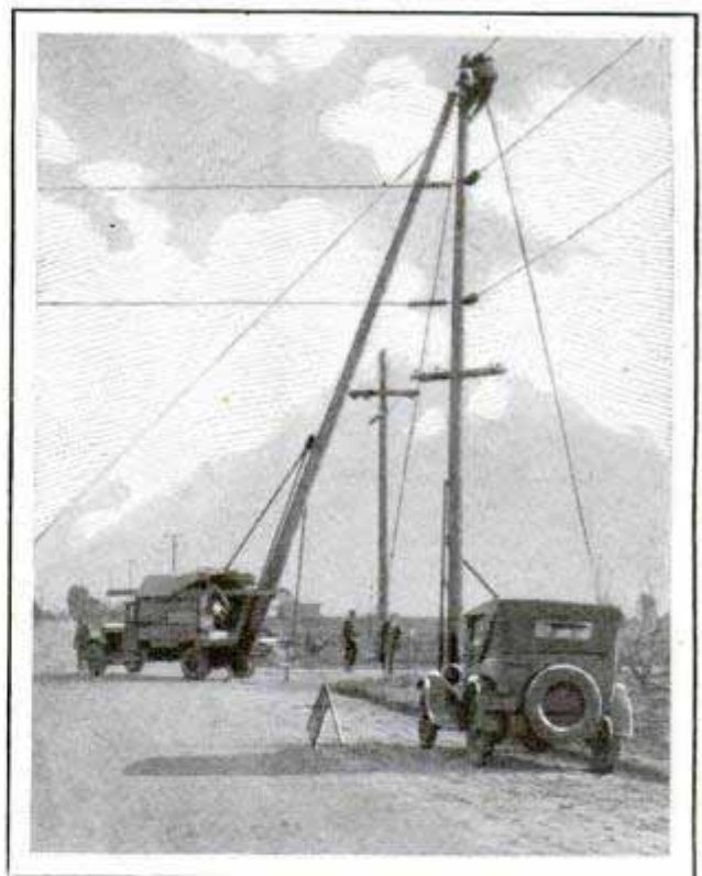
Pole Lashed to Truck, Enabling Repair of Power Line without Shutting Off Power on Other Lines
