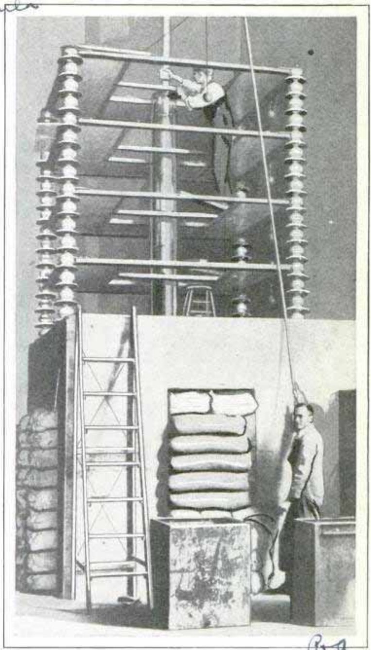
Million-Volt X-Ray Machine, Most Powerful in the World, Which Is Capable of Penetrating an Inch of Lead
