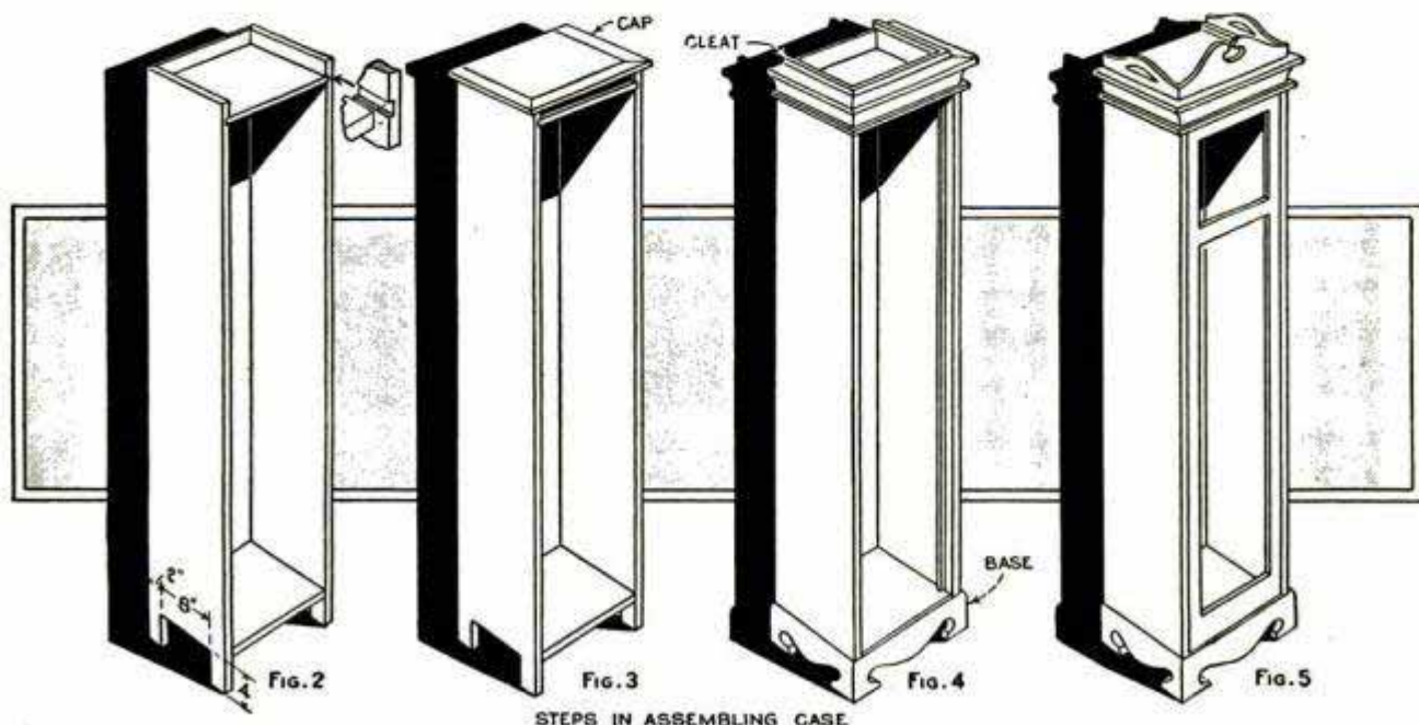
STEPS IN ASSEMBLING CASE
