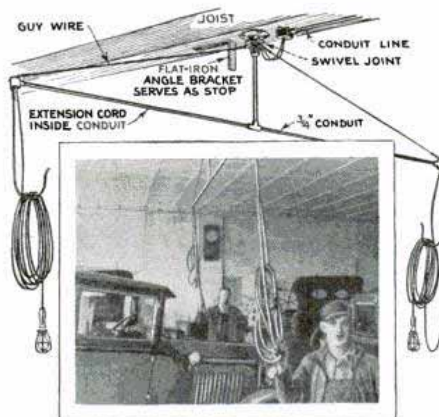
Convenient Holder for the Garage Extension Cord Serves Wide Radius
