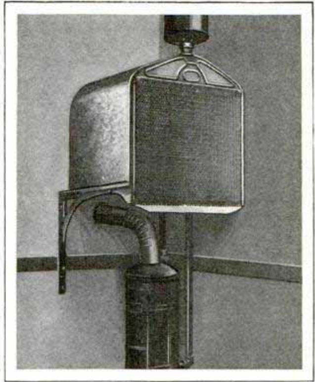
Photo of the Original Heater as Installed in a Restaurant; It Takes Little Room, and Is Economical
