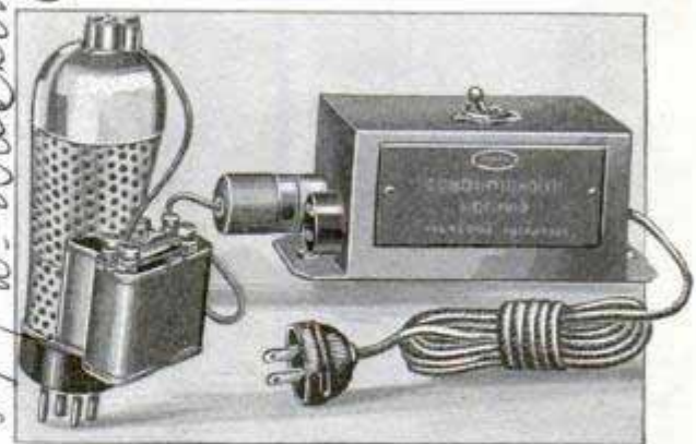
Screen-Grid Unit Ready for Plugging into Power Line
