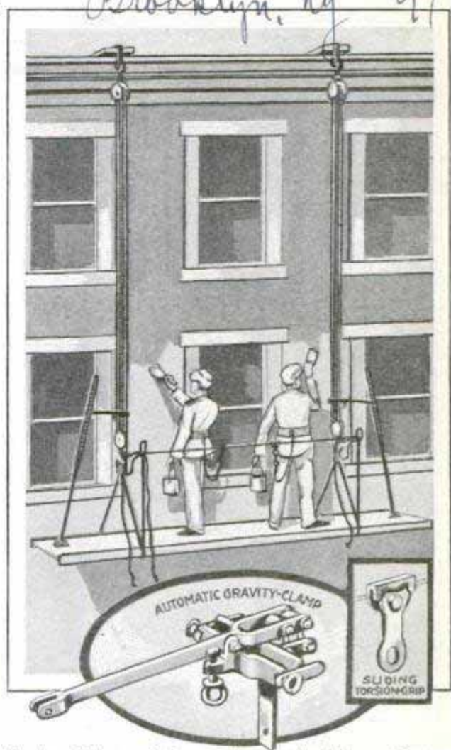
Torsion Grips and Automatic Gravity Clamps Protect Workmen on This Scaffold from Accident
