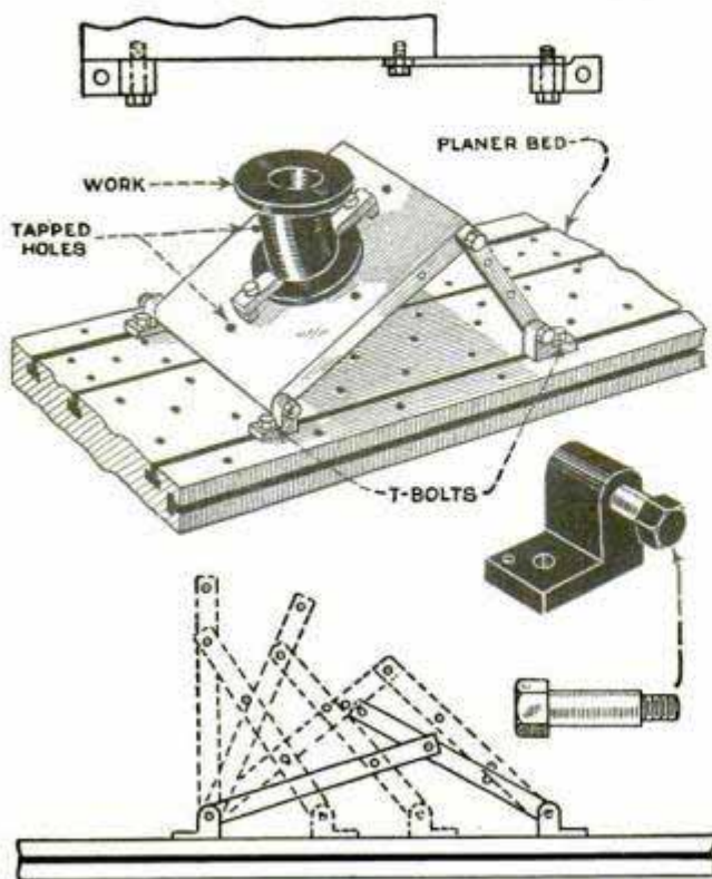
Universal Angle Plate Which Can Be Used on Any Planer or Shaper
