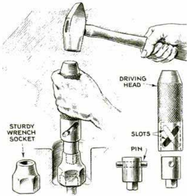
Simple Tool for Starting Nuts and Bolts in Places Difficult of Access
