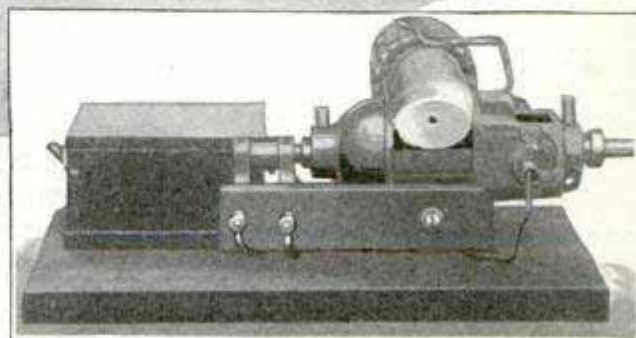
Upper Left, Armature Removed from Frame; Lower Right, Complete Converter-Unit Assembly, Showing the Transformer in Position
