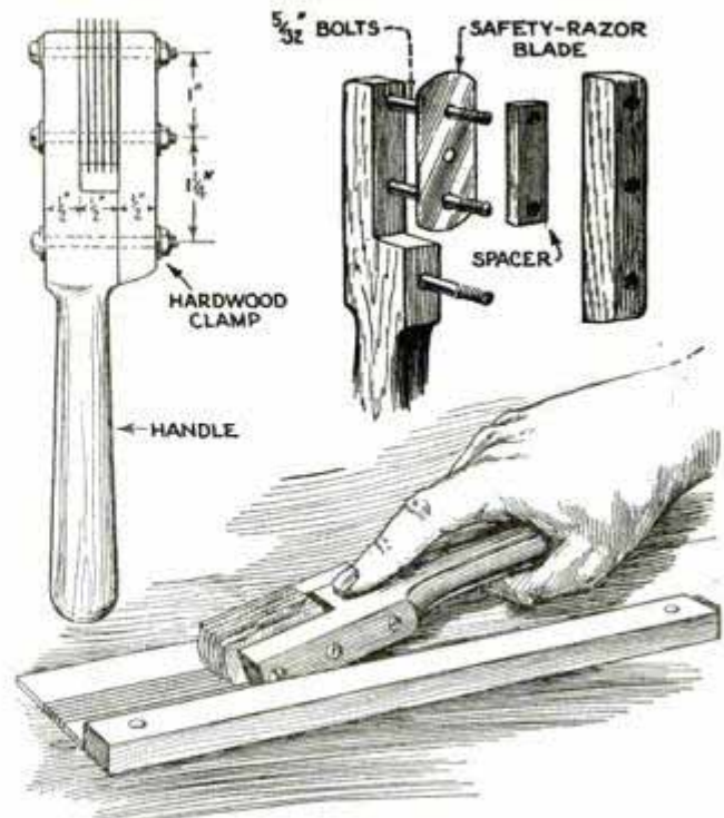
Handy Tool for Cutting Strips of Balsa Wood of Any Desired Width
