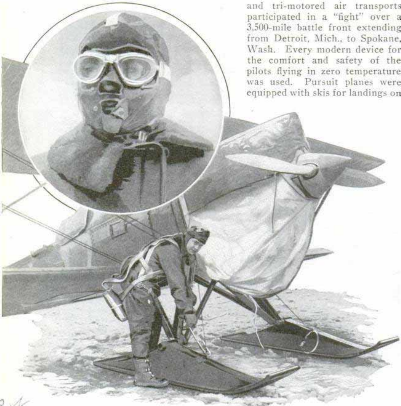
Top, Electrically Heated Face Mask and Goggles for Pilot Flying in Zero Weather; Below, Plane on Skis Equipped with Canvas-Covered Heating Element to Keep the Engine Warm
