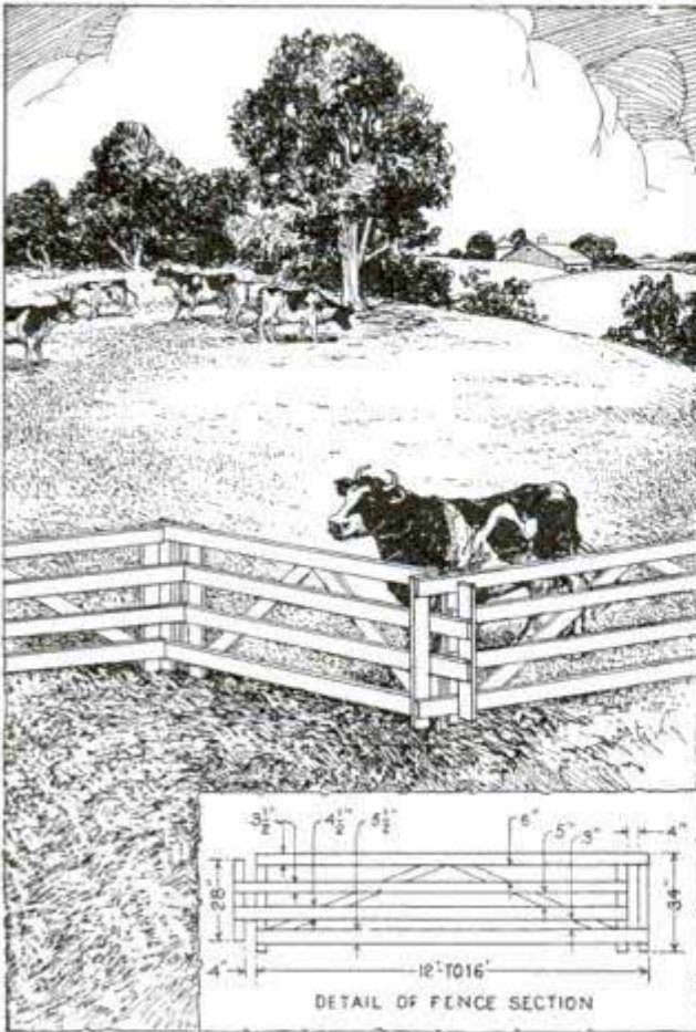
Zigzag Fence Made of One-Inch Stock Useful for Making Temporary Corrals
