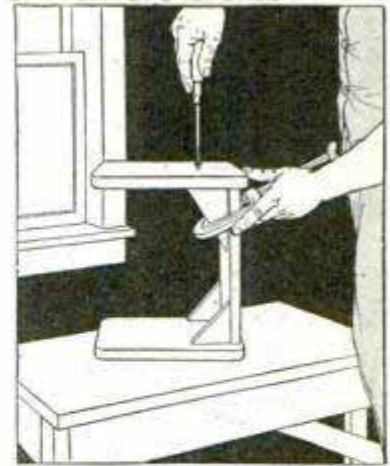
ASSEMBLING FRAME
