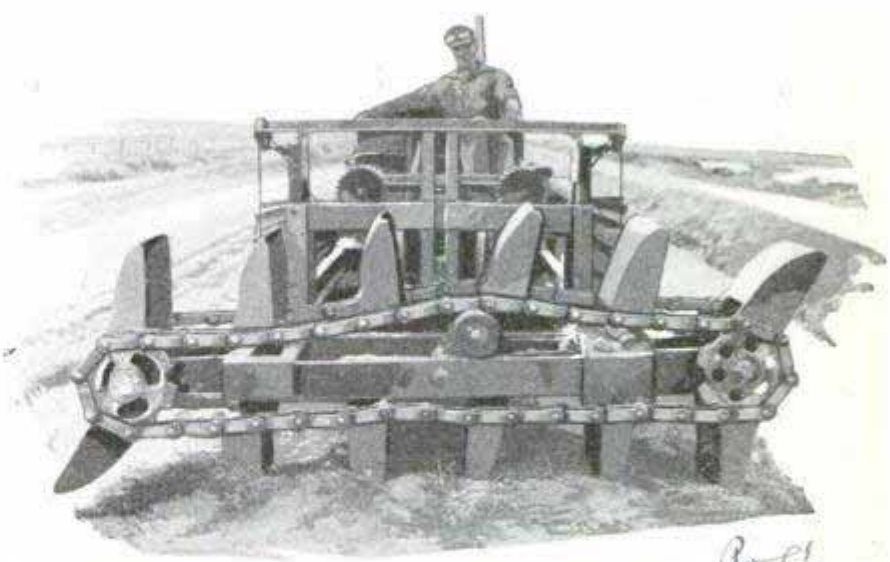
Rotary Grader Used to Reclaim Farm Lands Laid Waste by Floods; the Shovels Move at Right Angles to the Path of the Machine
