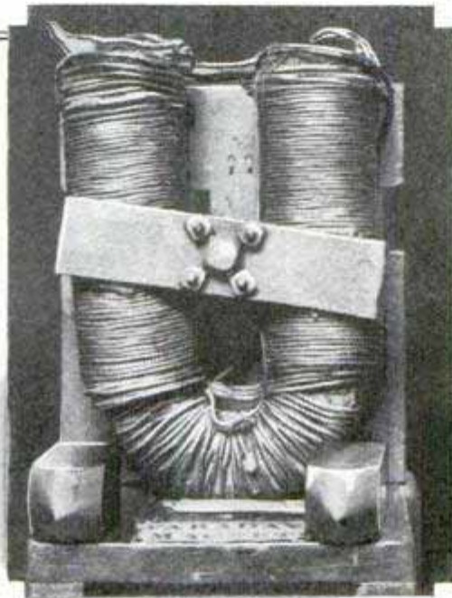
Michael Faraday's Original Electromagnet, Made in 1845 and Recognized Today as an Important Step in the Development of Wireless
