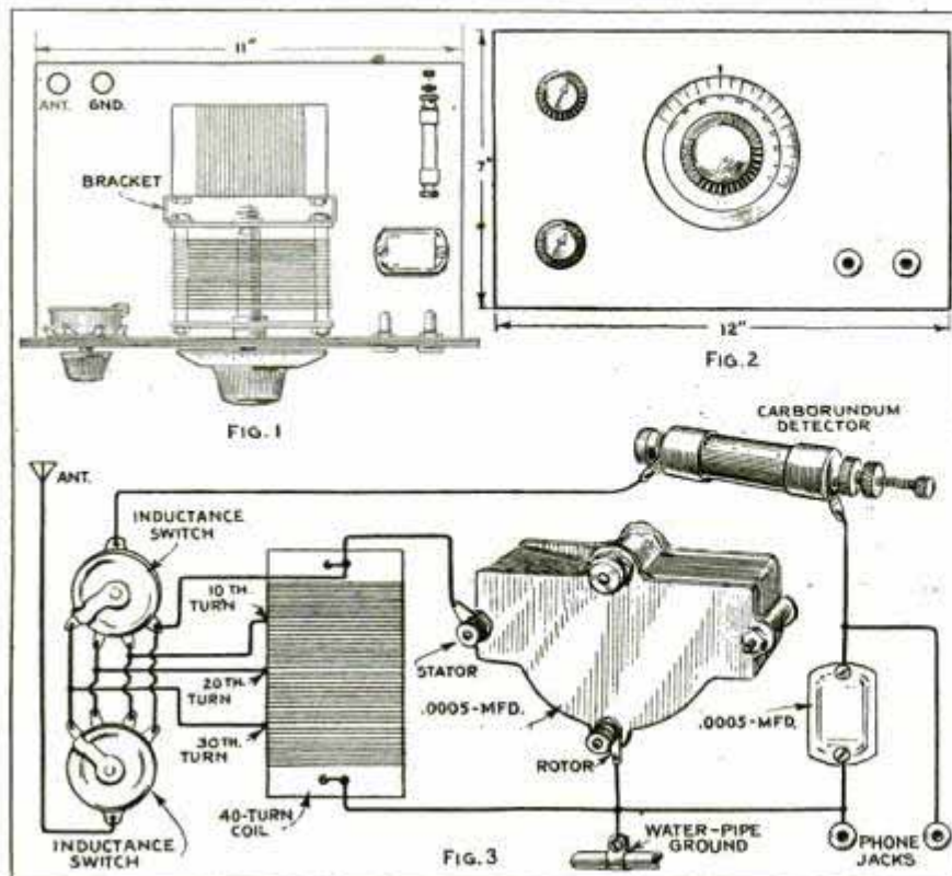
Upper Left, Instrument Assembly Showing Coil Mounted on Variable Condenser; Right, Front Panel Layout; Below, Simplified Wiring Diagram
