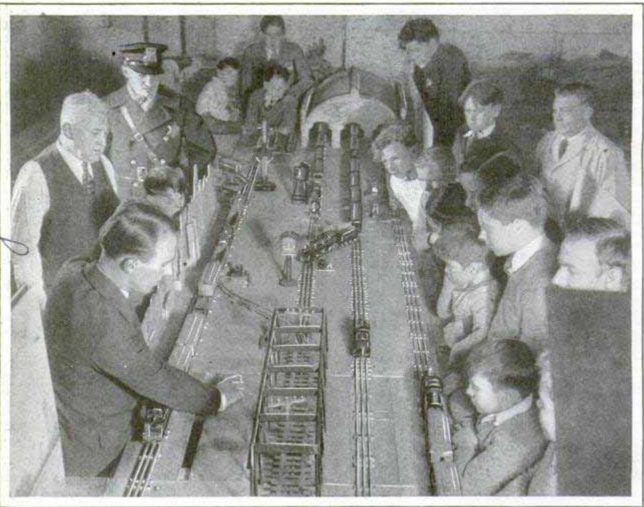
Perry A. Ball, at Left in Foreground, Teaching Class of Boys and Men Some of the Principles of Railroad- ing by Means of Miniature System That Closely Duplicates a Real Railway
