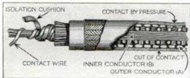
Cross Section of Cable Which Makes an Electric Contact When It Is Pinched at Any Point
