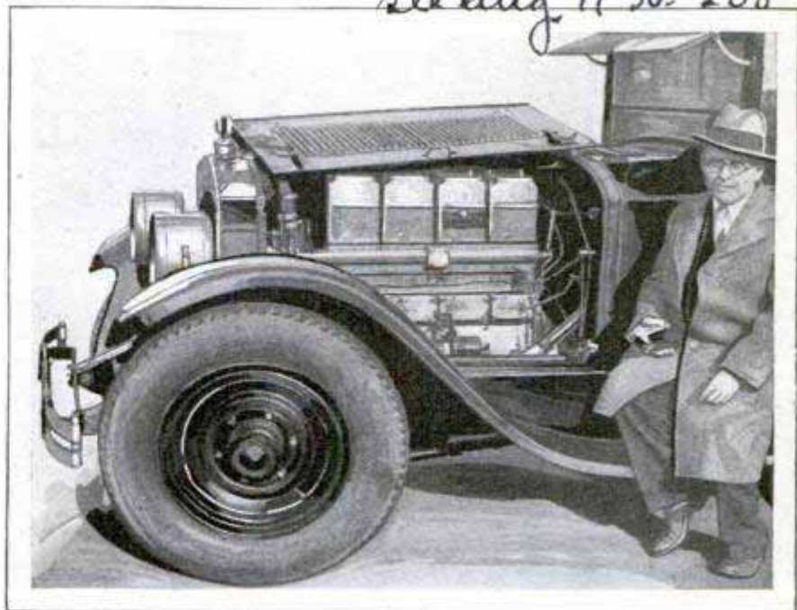
Diesel Engine in Standard Car Chassis; the Auto Traveled 792 Miles with This Motor at a Fuel Cost of $1.38
