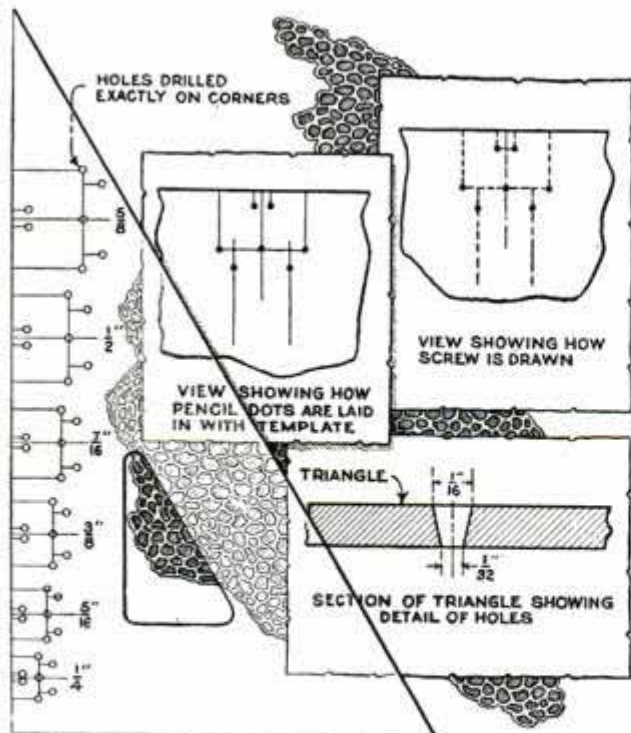
Laying Off Fillister-Screw Heads on Triangle Saves the Draftsman's Time
