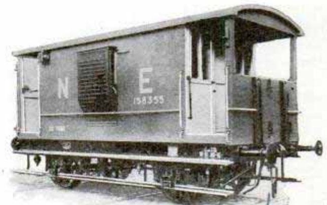
Railway Car of Concrete, Built on a Steel Framework, Which Is Being Tested in England
