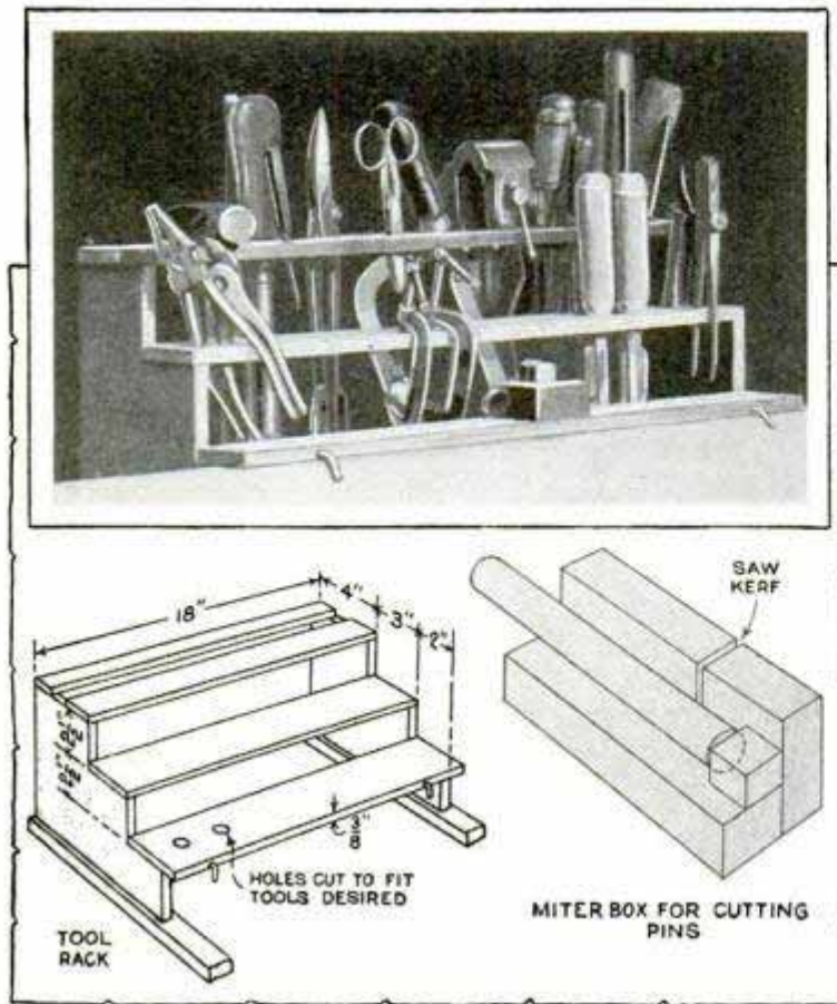
This Convenient Tool Rack Hooks onto the Back of the Bench, Keeping Tools Out of the Way, Yet Instantly Available
