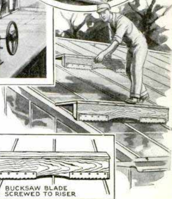
Above, Vermin-Proofing the Greenhouse with Screen without Interfering with the Window-Raising Arms; Below, Non-Slipping Platform for Use When Replacing Window Panes
