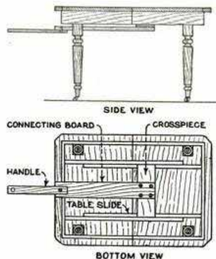
Arm Attached to Extension Table Makes It Possible for One Person to Open or Close It Single-Handed
