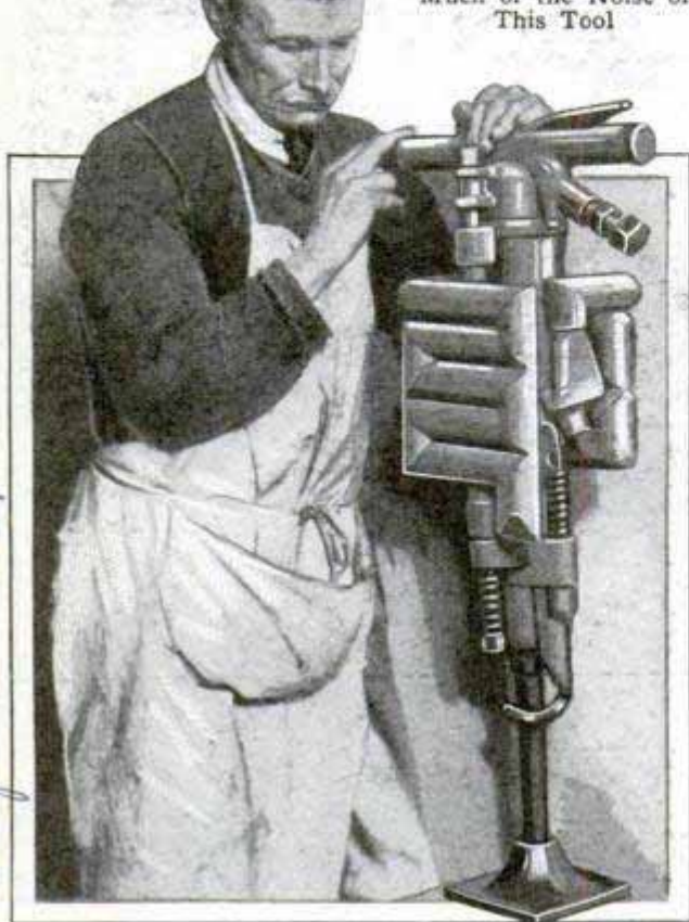
Pneumatic Road Drill Equipped with Silencers Which Deaden Much of the Noise of This Tool
