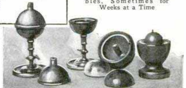
Faraday's Specific Inductive-Capacity Apparatus of 1837, Used in Experiments That Blazed the Way for Important Industries
