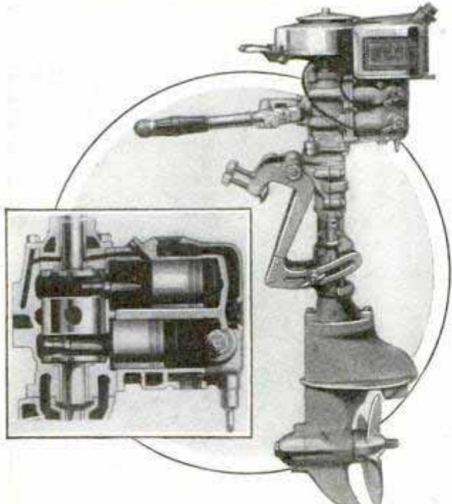
Outboard Motor with Alternately Firing Twin Cylinders, Producing Two Impulses Per Revolution
