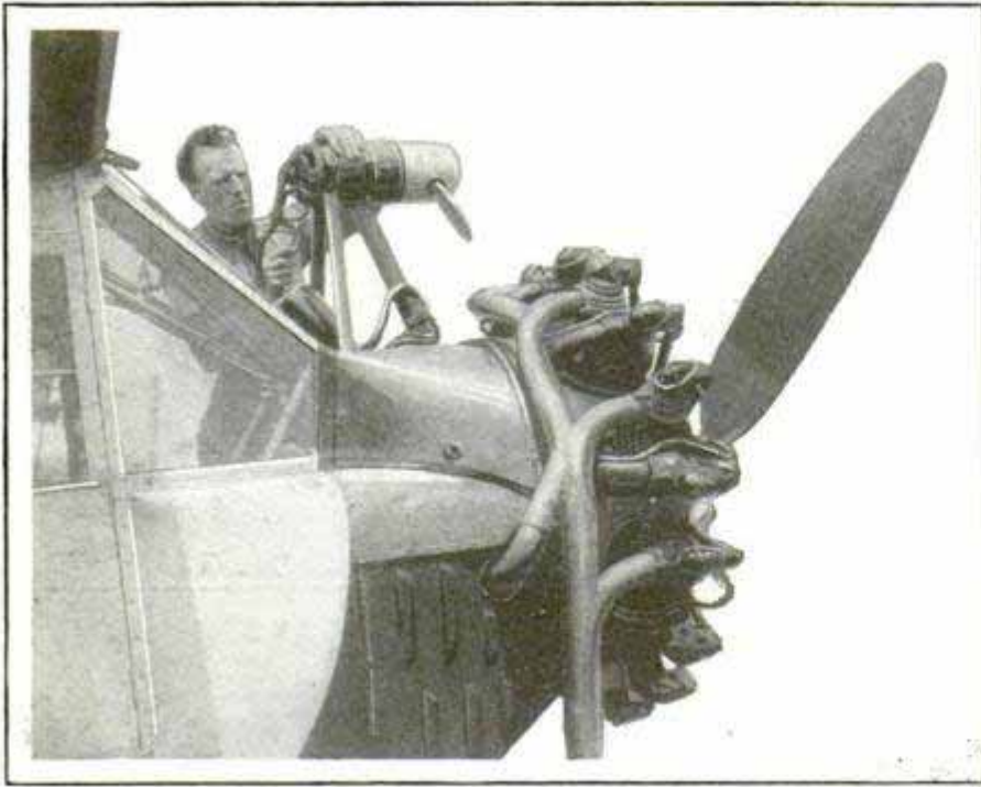
Wind-Driven Generator Which Supplies Filament and Plate Current for the Plane's Radio Transmitter and Receiver
