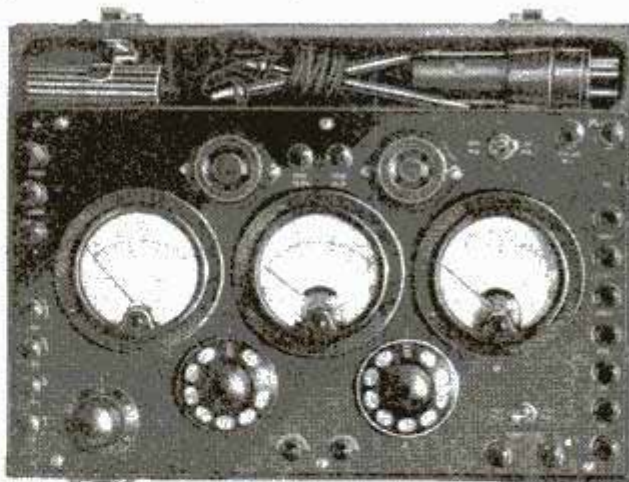
Combination A.C.-D.C. Set Tester for the Service and Repair Man
