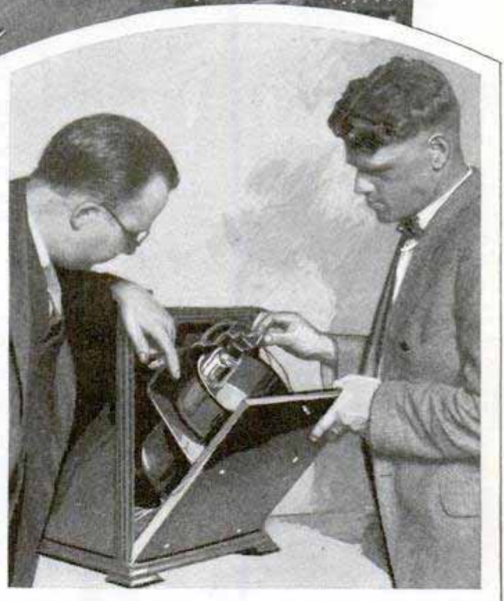
Television in the Home; Lower Left, Scanning Drum, Motor and Selector-Shutter Assembly; Right, Engineers Examining the Installation by Opening the Rear Door of the Cabinet
