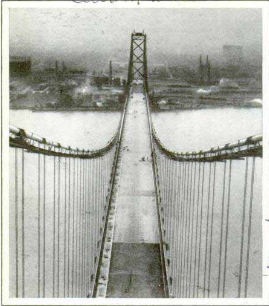
The 1,850-Foot Free Span of the "Good Will" Bridge between Canada and the United States, the World's Longest Suspension Span.
