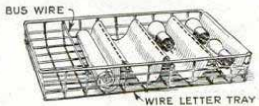
A Wire Letter Tray Converted into a Vacuum-Tube Holder; Busbar Wire Forms the Partitions and the Covering Material Is Felt or Woolen Cloth; the Holder Should Be Fastened to the Bench
