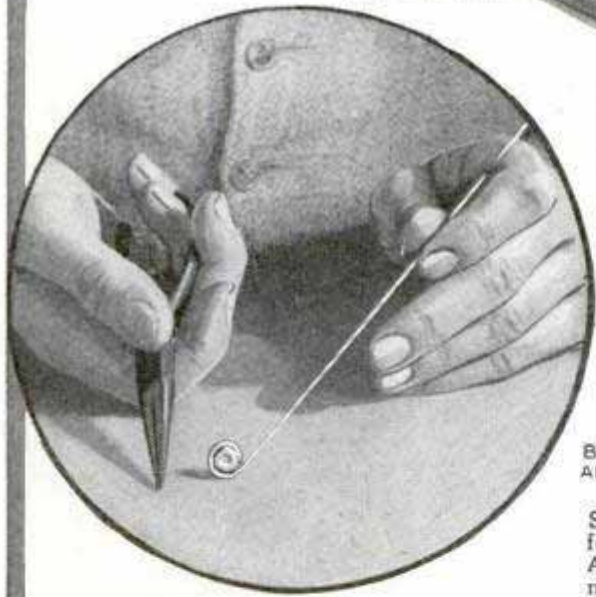
Threading Nuts behind Panels and under Instruments Is Simplified by Bending a Length of Busbar Wire to Hold the Nut
