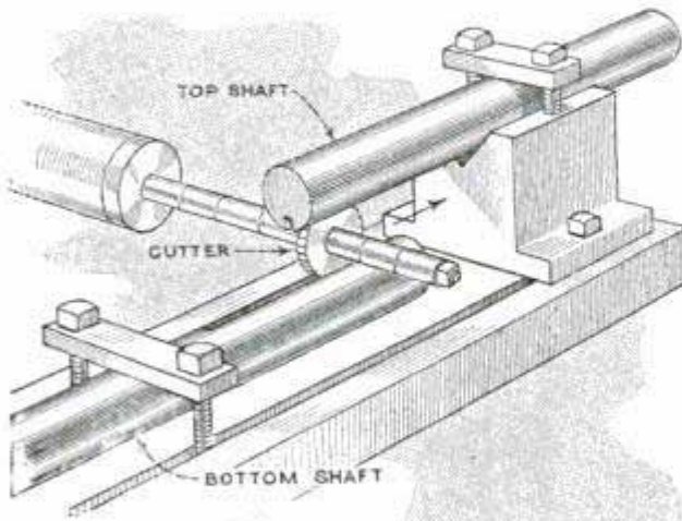
Milling Keyways in Two Shafts at One Set-Up Increased the Production Speed in a Small Shop
