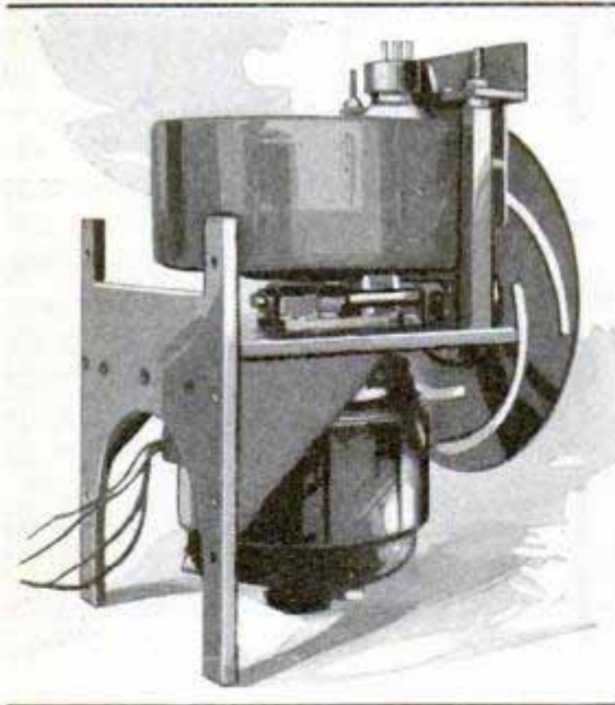
Television in the Home; Lower Left, Scanning Drum, Motor and Selector-Shutter Assembly; Right, Engineers Examining the Installation by Opening the Rear Door of the Cabinet
