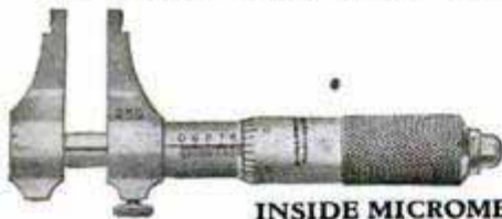
INSIDE MICROMETER CALIPER NO. 250 With a range .200" to 1" by thousandths of an inch, this micrometer is especially adapted for accurately measuring small internal dimensions.
