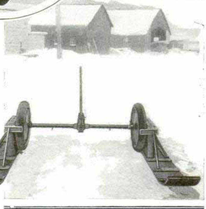
Combination Ski-Wheel Landing Gear for Alighting on Snow after Take-Off from Bare Ground
