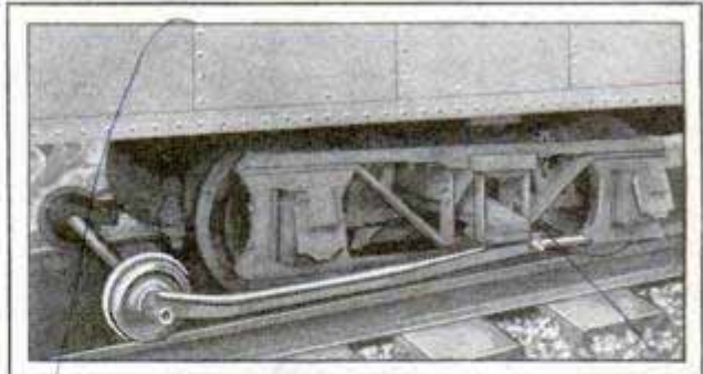
Truck Placed under Street Car with Broken Axle, Enabling It to Proceed under Own Power
