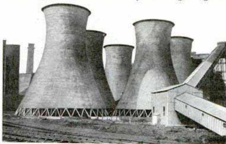
They Look Like Huge Milk Bottles, but These Concrete Structures Are Cooling Towers for an Electric Generating Station
