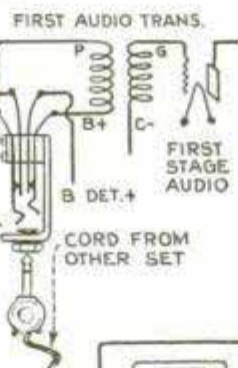
Left, a Handy Jack Assembly for Making Amplifier Unit in Broadcast Receiver Available for Use with Short-Wave Adapter or Phonograph Pick-Up; the Double-Circuit Jack Is Mounted at the Rear of Subpanel and the Diagram, Showing All Connections, Is Given Below
