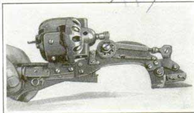
Pair of Shears Operated by Electric Motor for Cutting Many Layers of Cloth at Once
