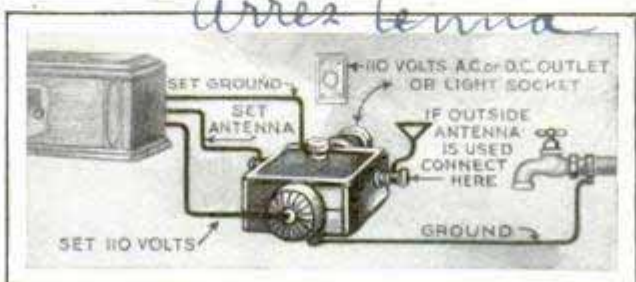
Lightning Arrester for Radio Which Protects from Charge through Antenna or Light Wires
