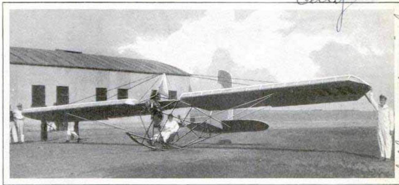
Glider Equipped with a Forty-Horsepower Motor Which Gets into the Air More Quickly Than an Airplane and Lands at a Safe Speed of About Fifteen Miles an Hour
