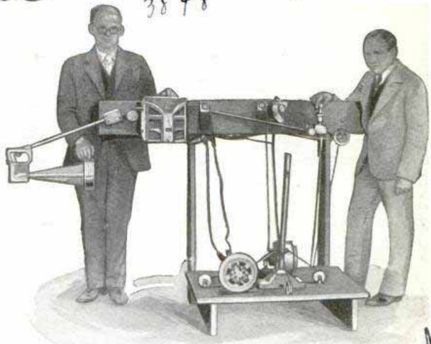
Automatic Plane Stabilizer, Embodying the Principles of the Vane and Pendulum, to Keep the Ship in Level Flight Constantly.
