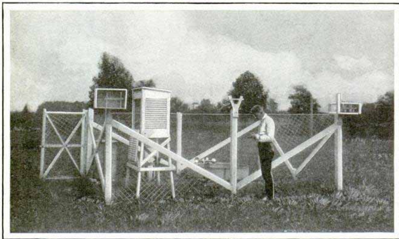
Evaporation Station of the United States Weather Bureau; the Pan Is Seen in the Middle of the Inclosure with the Wind, Rain and Other Gauges
