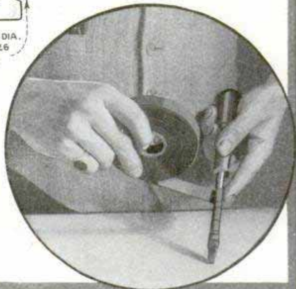
Above, Handy Kink for Cutting Resistors in Series and Condensers in Parallel In and Out of Experimental Hookups
