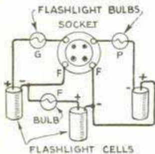
To Test Radio Tubes for Short Circuits, Insert Tube; if Bulb F Lights, Bulbs G and P Should Not Light; G Lighted Indicates Grid-Filament Short; P Lighted Shows Grid-Plate Short; to Clear Short in Either Case, Tap Tube, and if Lamp Continues to Burn Discard Tube; Many Elaborate Tube Testers Do Not Indicate Shorts
