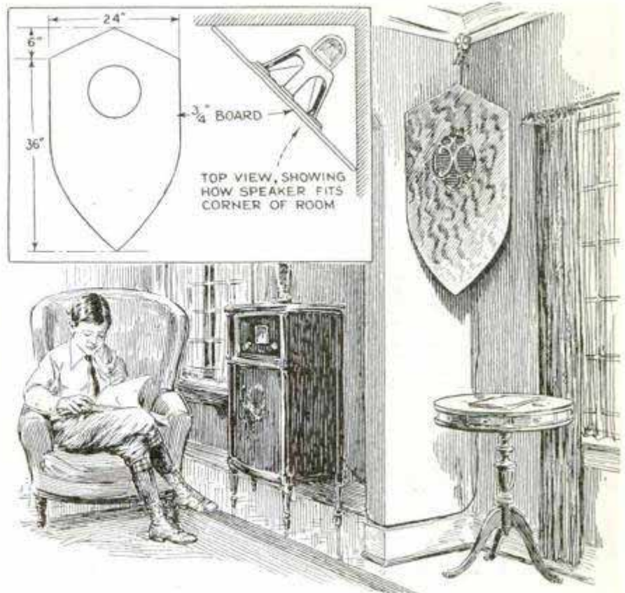
Upper Left, Construction Details of Baffle; Right, Completed Unit Showing Method of Installation
