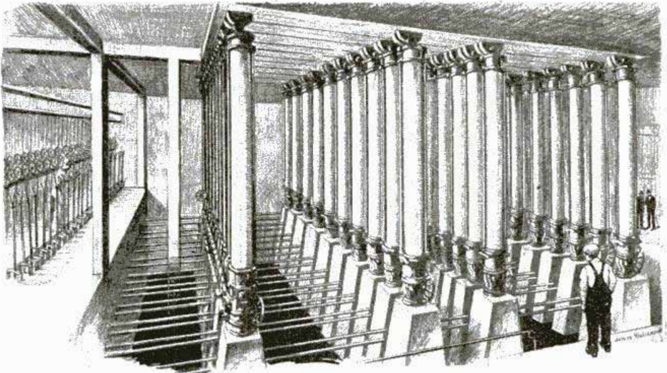
Drawing of the Forty Hydraulic Plungers That Raise or Lower the Twenty Stage Sections Above a Total Distance of Twenty-Four Feet to Make Possible Varied Setting Effects
