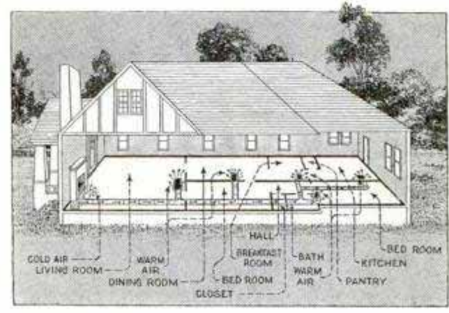
Diagram Showing How Heat from a Fireplace May Be Conveyed to Other Rooms of the House
