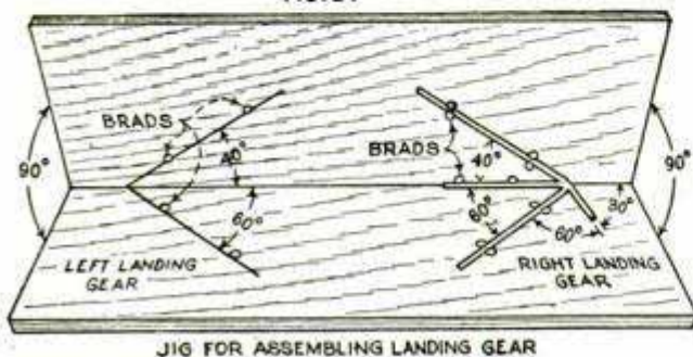
LANDING-GEAR DETAILS FIG. 27
