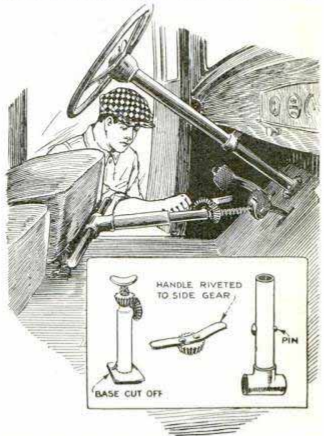
Pedal Depressor, Made from Old Auto Jack, Helps When Adjusting Brakes Single-Handed
