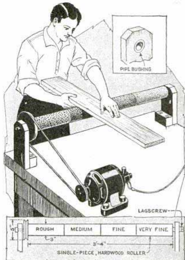
Four Different Grades of Sandpaper Are Mounted on This Cylindrical Sander
