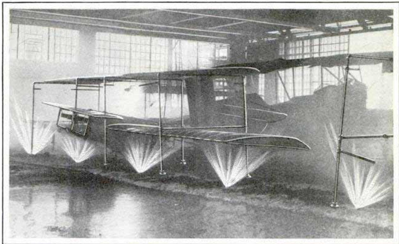
Hangar Equipped with Both Overhead and Ground Sprinklers for Protection of Planes; Heat Starts a Shower of Water from Above and Also Sends Powerful Sprays Upward
