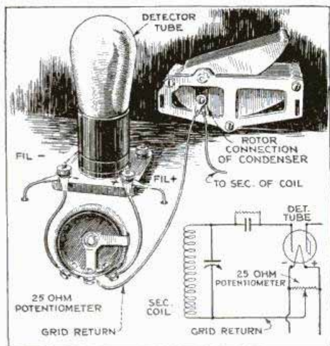
Left, Picture Diagram Showing All Connections; Right, Schematic Circuit Diagram
