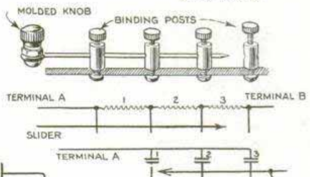
Above, Handy Kink for Cutting Resistors in Series and Condensers in Parallel In and Out of Experimental Hookups
