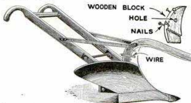
Wooden Guard Block Attached to Plow Beam Keeps It Free from Rubbish
