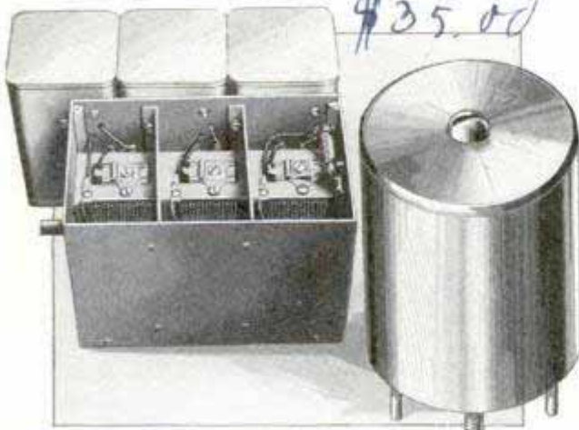
Three-Stage Screen-Grid Amplifier with Cover Removed from Triple Condenser Shield; Right, Shielded and Polarized R.F. Choke Coil
