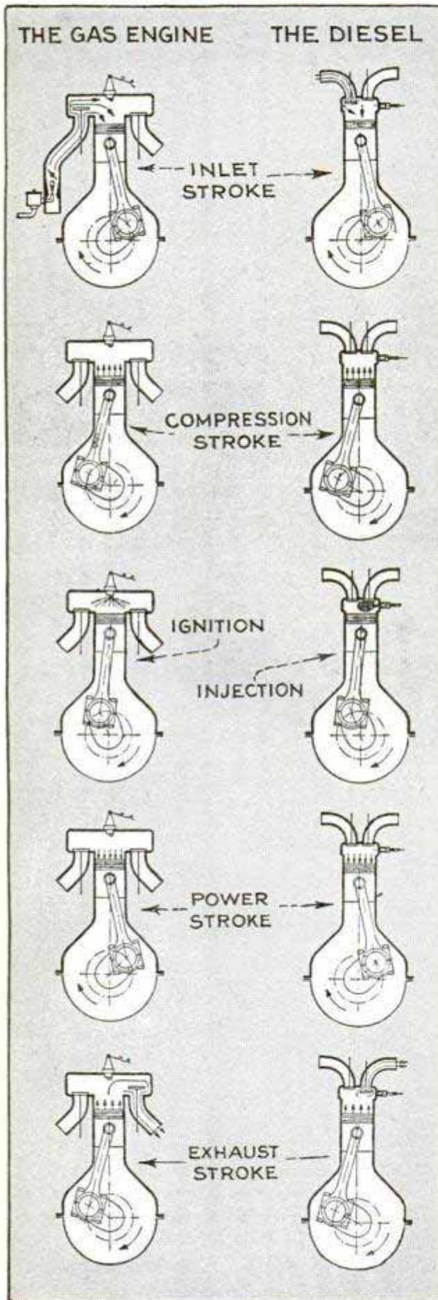
Drawing Illustrating Difference in Principle Between the Gas Engine and Diesel Engine; Absence of Ignition Is the Chief Characteristic of the Latter
