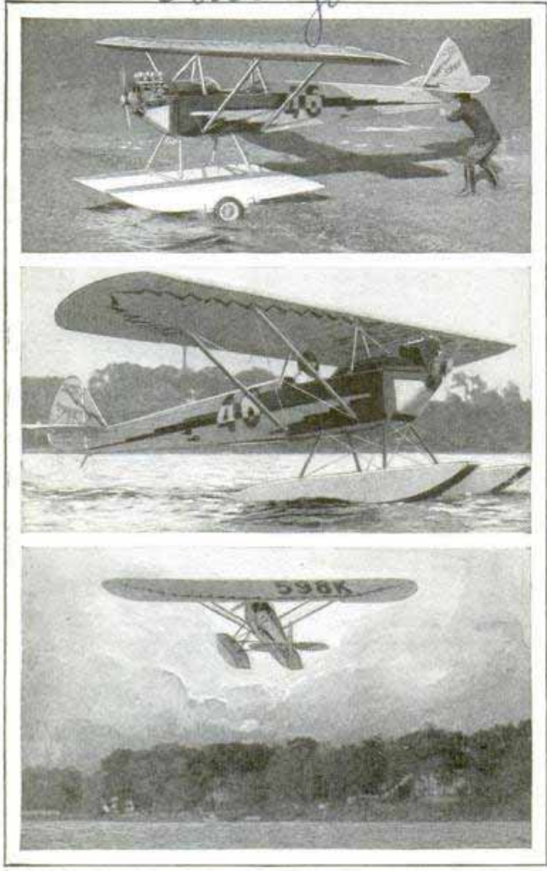
Three Views of an Airplane with Detachable Pontoons beside the Landing Gear to Transform It into a Seaplane
