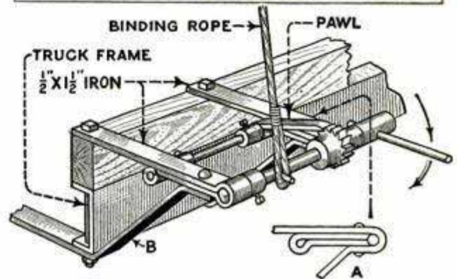
Winch Attached to Rear End of Truck for Holding Down Heavy Loads
