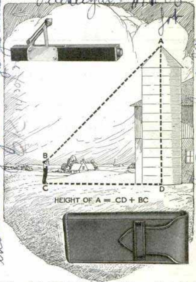
Views of the Height Finder, and Diagram Illustrating the Principle of Its Operation
