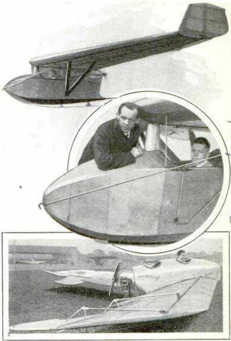
Views of the Motorized Tailless Gliders Tested in Germany; the Engine Is Seen behind Rear Cockpit in Lower Photograph
