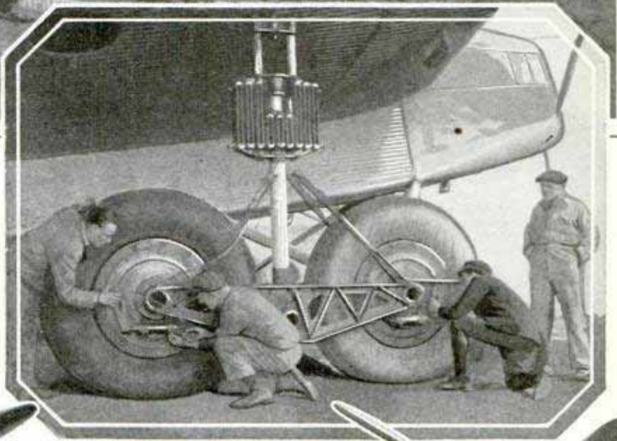
The Junkers Plane "G-38" in Flight, and a Close View of the Landing Wheels, Which Are Five Feet in Diameter; the Ship Has Four Motors, Developing a Total of 2,400 Horsepower, and Carries Forty Persons
