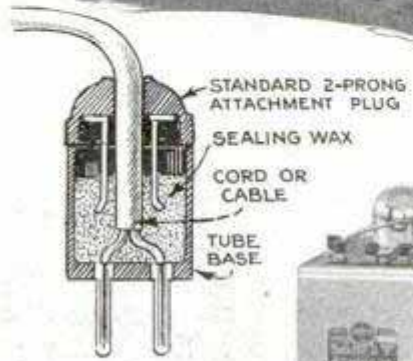
Connector Plug for Tube Testers or for Short-Wave Adapters
