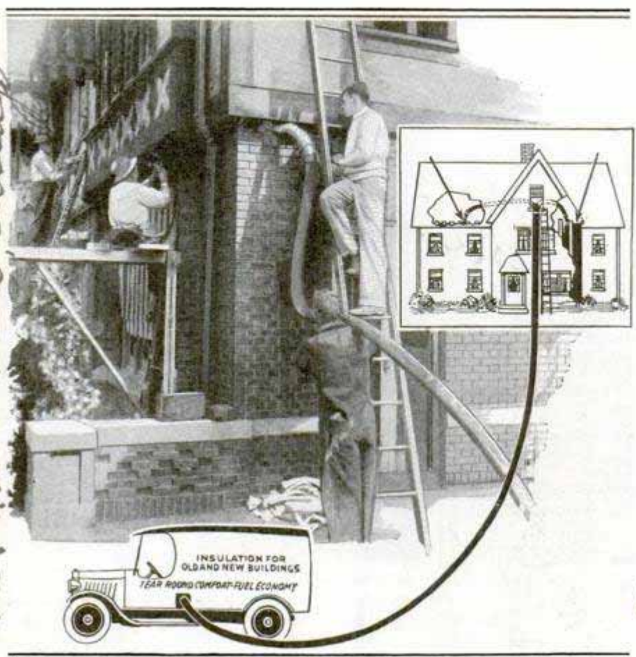
Photograph of a Typical Filling and Insulating Job and, Drawing to Show How Material Is Pumped between the Walls of a House
