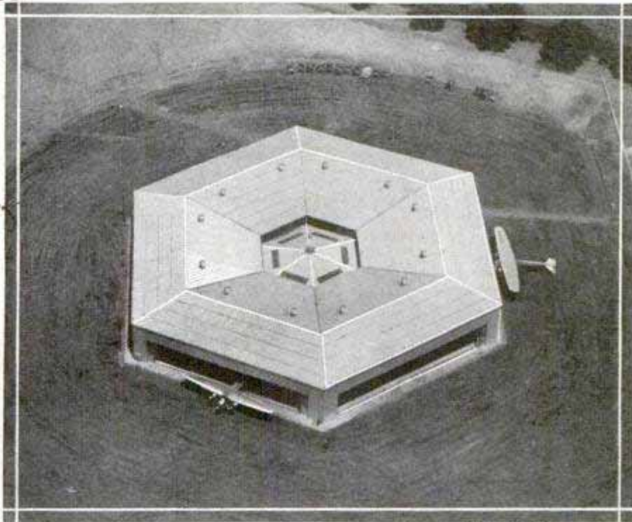
Emptying This Huge Hexagonal Airplane Hangar, with 54,000 Square Feet of Floor Space, Requires Only Thirty Seconds
