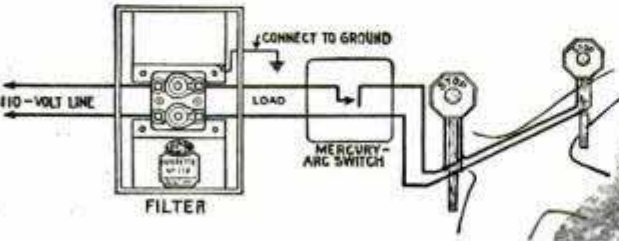
Upper Left, Bridge Approach Showing Location of Flasher Signal; Below, Diagram of Filter Installation; Right, Signal at Through Street
