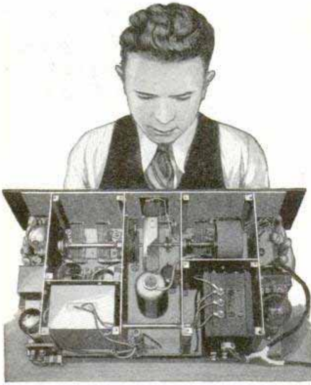
Above, the Completed A.C. Screen-Grid Receiver Ready for Testing
