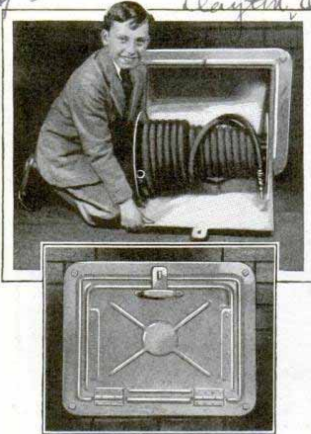
Above, Disappearing Hose Reel Which Fits in Coal-Chute Door; Below, the Door When Closed
