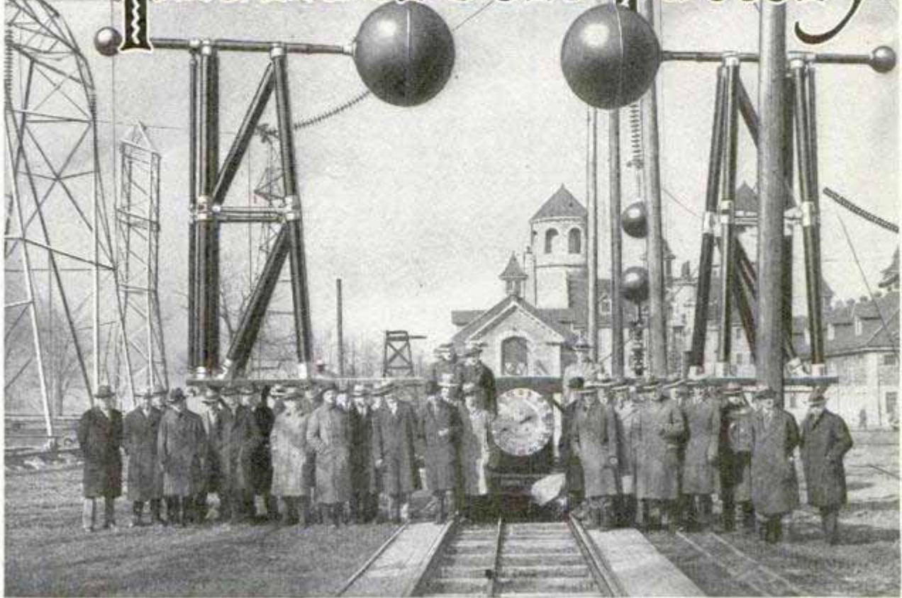
Sphere Gap Used for Controlling and Measuring Artificial Lightning at the Outdoor Laboratory; the Upright Supports Are Special Insulators and the Dial Records Distance between the Spheres
