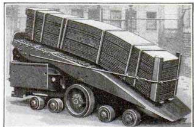
Self-Loading Truck with Tilting Platform Which Handles Ten Tons of Steel at a Time
