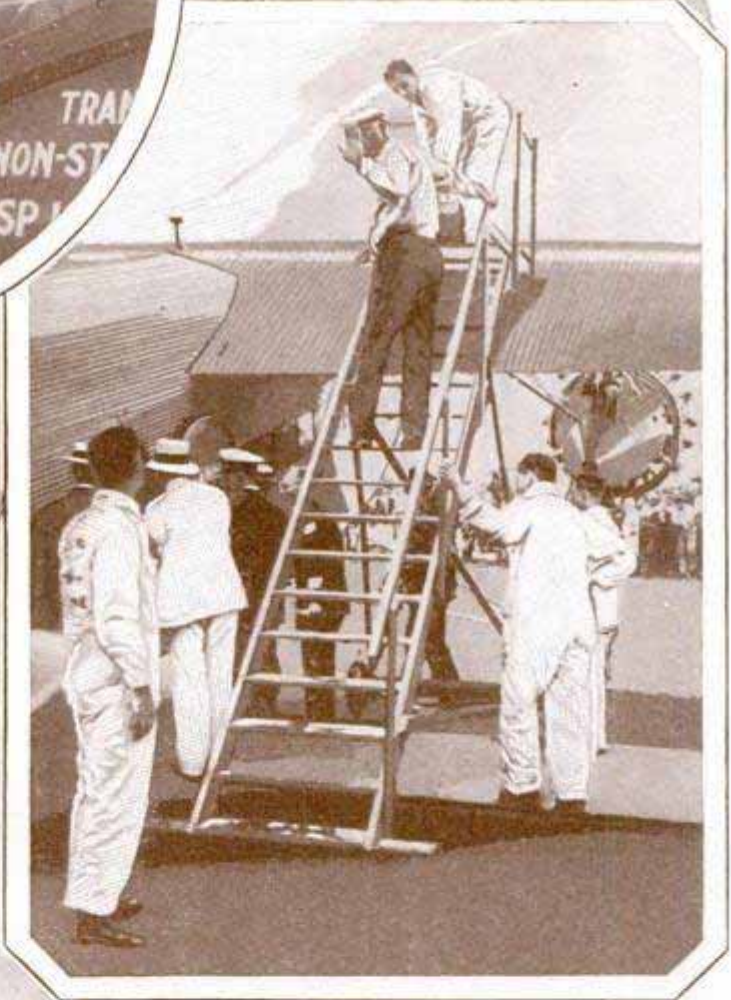
Space Is Ever at a Premium in Passenger-Carrying Ships, Particularly When It Comes to Baggage; the Transcontinental Air Transport Planes, Carrying Passengers on the Coast-to-Coast Rail-Air Route, Solved the Baggage Problem by Providing Space for It in the Wings; Above, Transport Employees Are Loading Bags into the Wing of the "City of Columbus" before the Initial Rail-Air Trip
