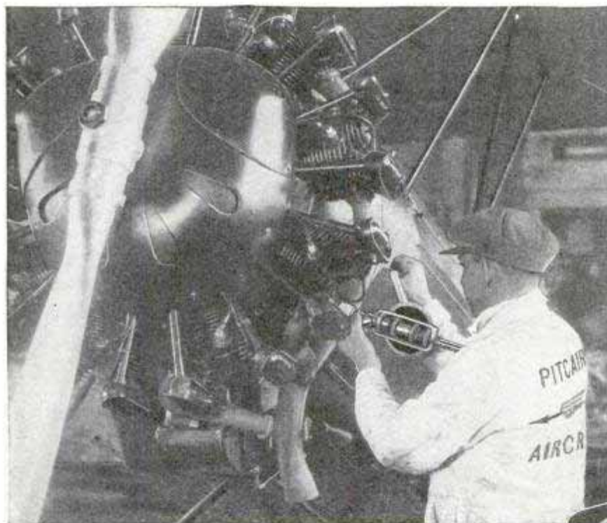
Photograph by permission Pitcairn Aircraft Inc. “Yankee” Ratchet Drill in use, on Pitcairn Super-Mailing, by John Van Winkle, who says, “I have used ‘Yankee’ Drills and Screw-drivers for eight years in Aircraft Work and found them very satisfactory; and convenient in close quarters.”
