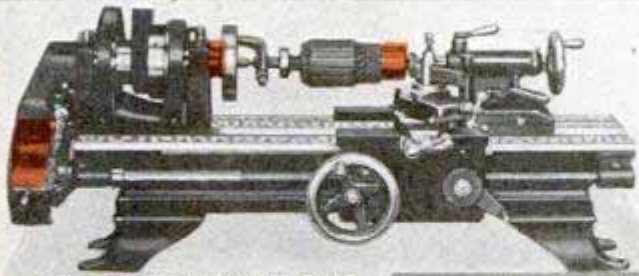
9' x 3' New Model South Bend Jr. Back Geared Screw Cutting Lathe (Weight 375 lbs.) Complete with Countershaft and $169 Equipment shown only
