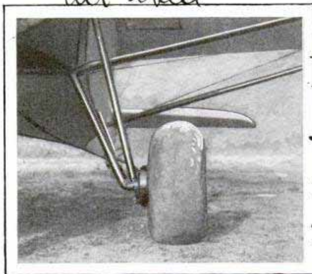
This Airplane Tire Fits Directly onto the Hub, Acting as Wheel and Shock Absorber
