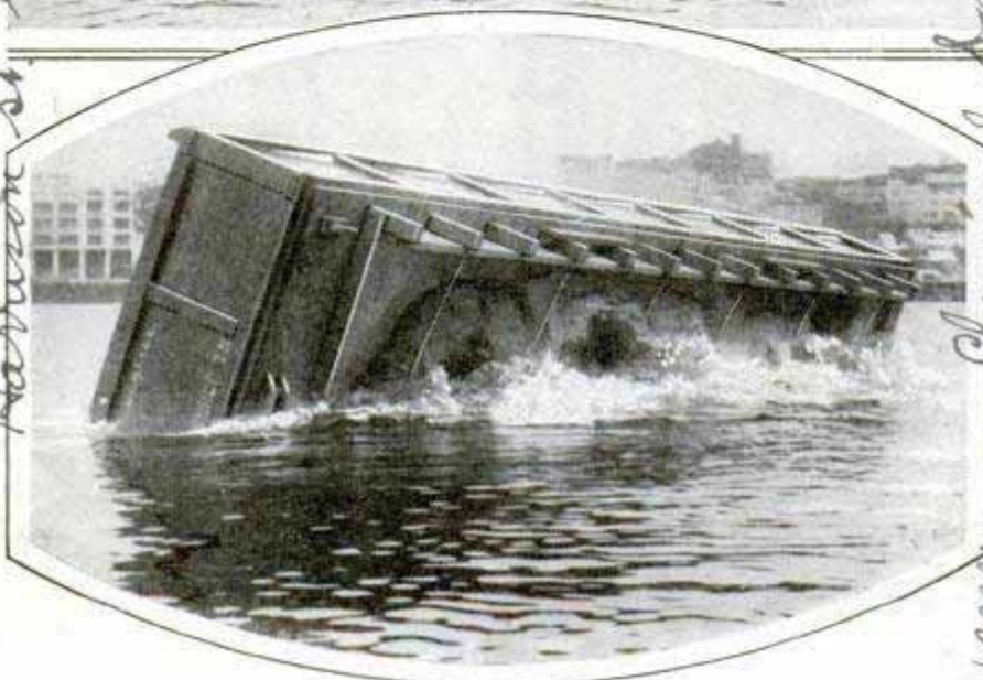
Two Views of a Self-Dumping Scow Operated by Flooding Air Chambers, Whereupon the Bottom Becomes the Top for the Next Load
