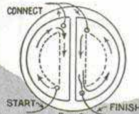
Fig. 9 DIAGRAM FOR WIRING AND CONNECTING "D" COIL UNIT
