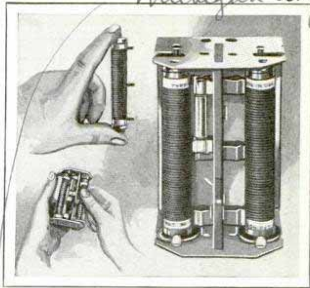
Rectifying Unit Being Placed in the Double Mount; and Complete Rectifier Ready for Installation
