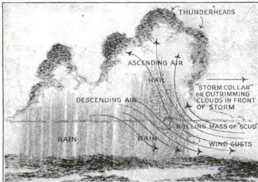
Cross Section of a Typical Thunderstorm, According to Dr. W. J. Humphreys of the Weather Bureau, Showing Ice or Hail "Factory" in Clouds
