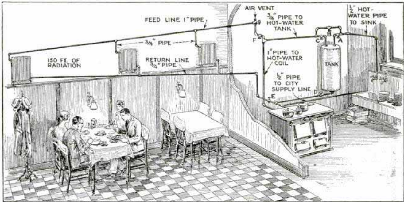
Small Cafe, Formerly Using Stove Heat, Made More Modern by the Installation of Hot-Water System Using the Excess Heat from the Kitchen Range
