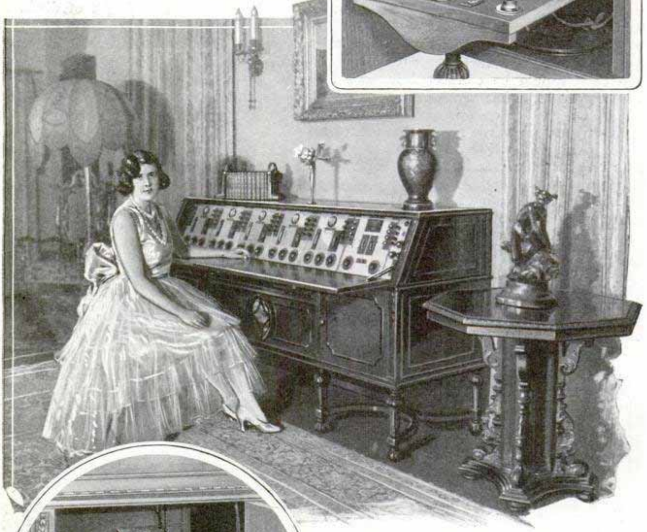
Top, Phonograph Turntable Located in Lower Compartment; Center, Complete Installation; Left, Power Pack and Amplifier
