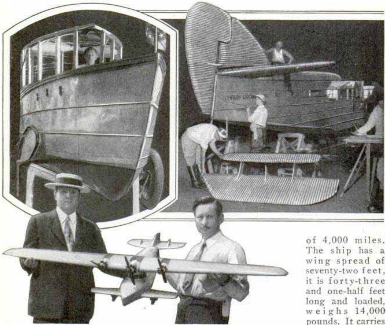
Views of the Amphibian under Construction and, Below, Erwin Greer, at Left, and J. H. Wendt, Designer of the Craft, Holding a Small Model
