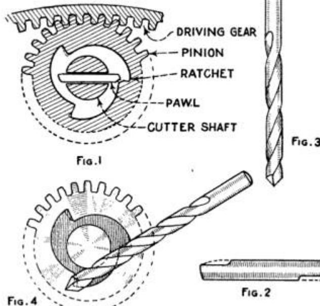
Fig. 1, the Ratchet Mechanism, Showing Wear; Figs. 2 to 4, How the Parts Are Repaired
