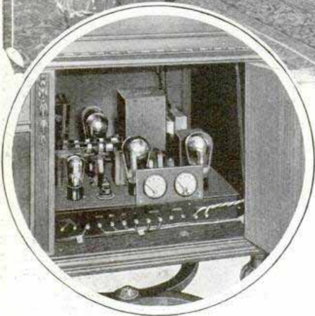
Top, Phonograph Turntable Located in Lower Compartment; Center, Complete Installation; Left, Power Pack and Amplifier
