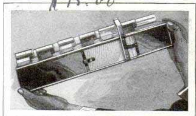
Sand Passes Successively Through a Graded Series of Screens in This Simple Sand Tester
