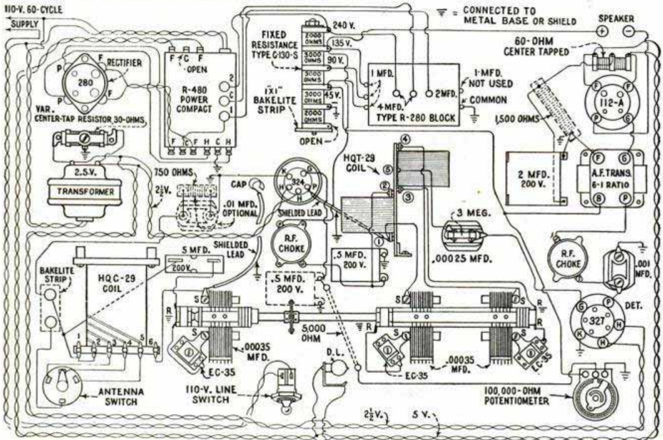
Upper Left, Underside View of the Completed Receiver Showing the Location of the Biasing Resistors and By-Pass Condensers; Below, Simplified Wiring Diagram Showing the Various Instruments in Approximately the Same Positions They Occupy in the Assembled Set
