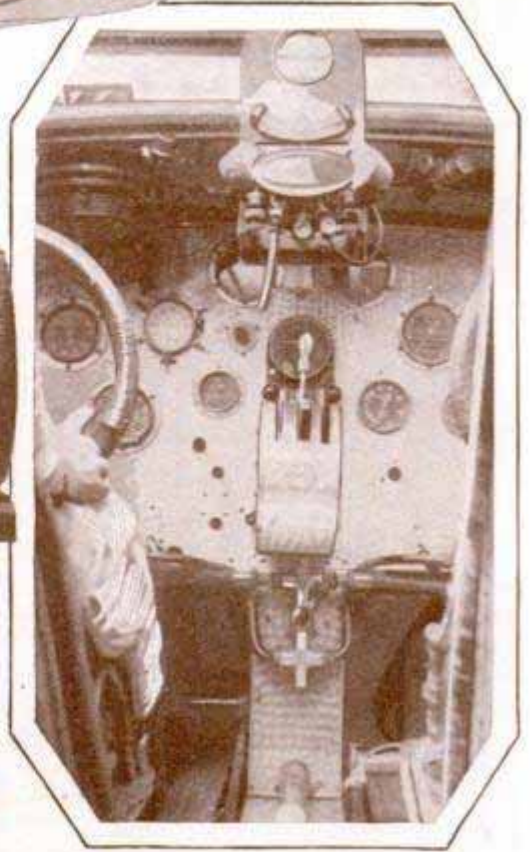
Above, the Instrument Board of the Single-Motored "Yellow Bird" on Which the French Aviators, Jean Assolant, Rene Lefevre and Armeno Lotti, Jr., Relied for Their Successful Transatlantic Flight; Left, Mechanics Repairing a Dump Valve Which Was Damaged during the First Attempt of the Frenchmen to Get Away, Necessitating a Return for a Second Start
