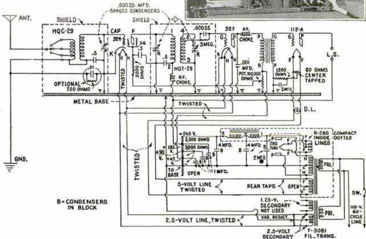
Upper Left, Panel Template for One-Half-Inch Subpanel; Right, Placing Shield over Screen-Grid Tube; Below, Schematic Diagram of Three-Tube A.C. Screen-Grid Receiver and Power Supply
