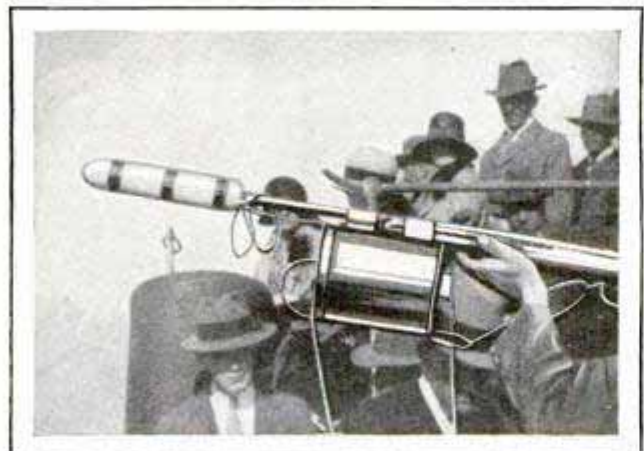
Life-Saving Rifle, Fitted with Rocket Which Throws Line and Float for 250 Yards
