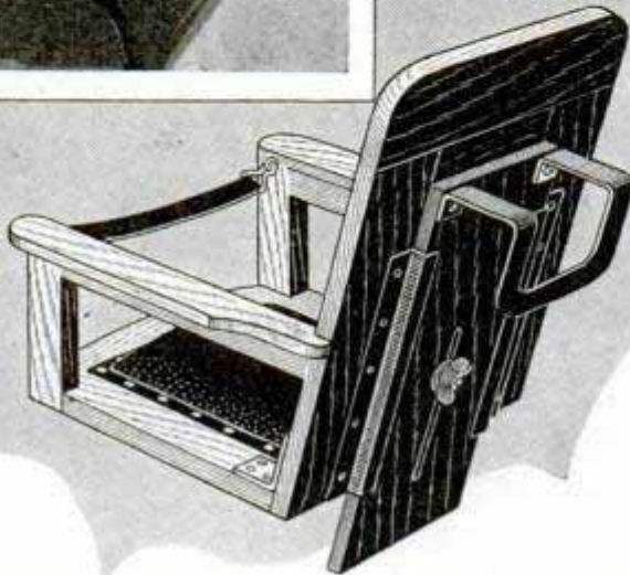
Small Adjustable Baby Seat Hooks over the Front Seat of Any Make of Car
