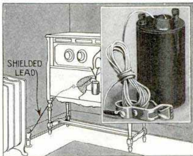
Antenna Eliminator, Showing Shielded Ground Lead and Clamp; Left, Sketch Showing Installation
