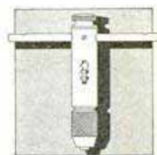
Tap hole with “Yankee” Tap Wrench No. 250. Ratchet adjustments and sliding cross-bar make awkward jobs easy. Price, $1.85.
