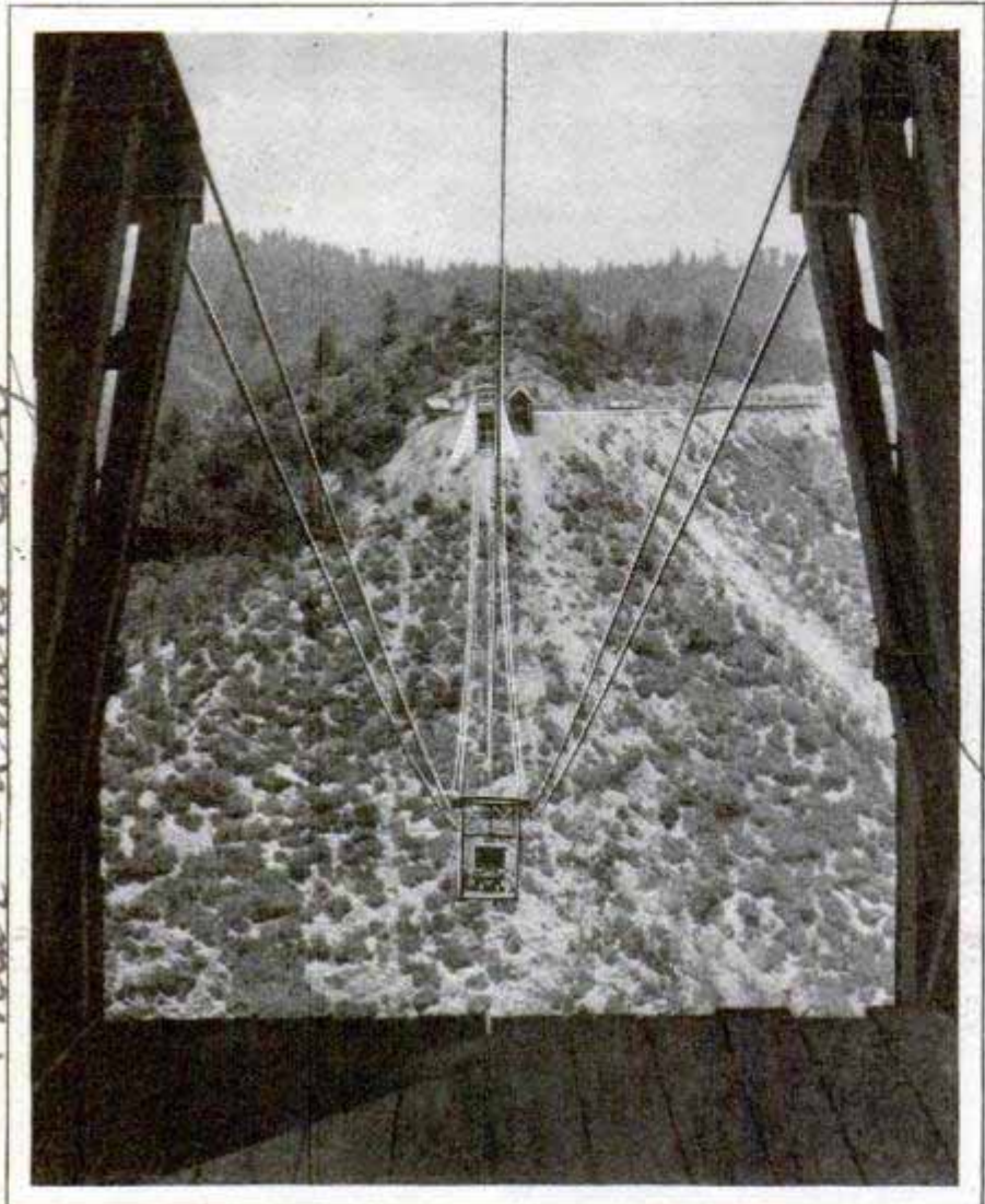
Courtesy General Electric Co. An Electric Cableway Which in Six Minutes Transports 24,000 Pounds of Lumber a Half Mile over a 1,200-Foot Canyon
