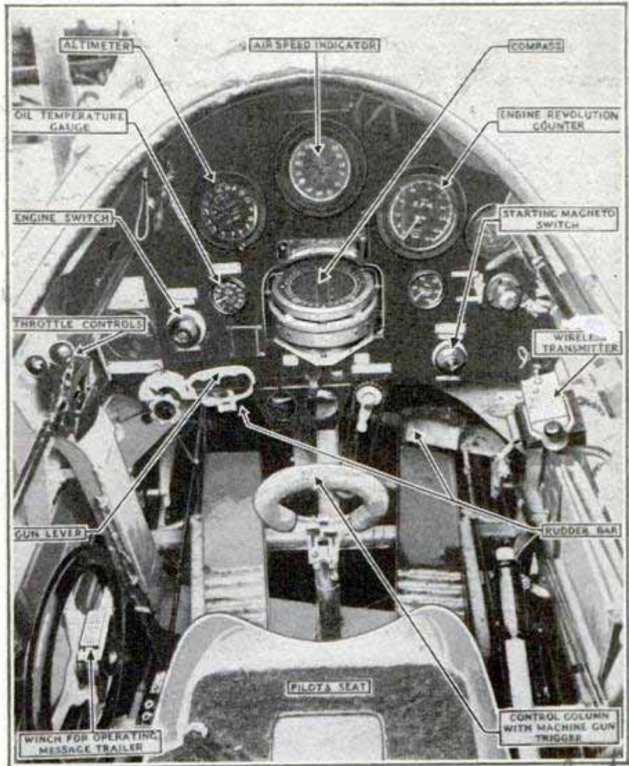
Pilots of the Australian Air Force Face This Maze of Controls When They Fly One of the Combat Planes Recently Purchased
