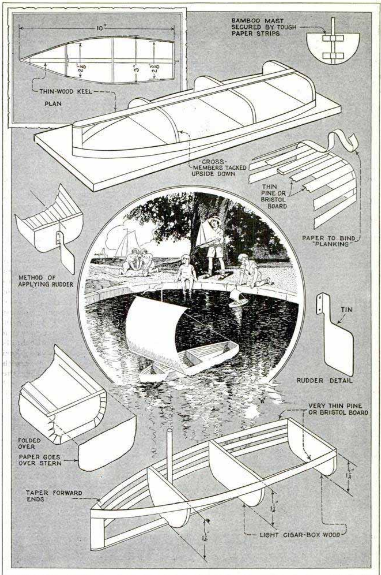
This Ten-Inch Paper Boat Is So Light That It Draws Only One-Eighth Inch of Water and Develops a Surprising Speed
