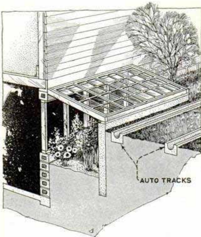
Hotbed Which Is Accessible from the Basement Keeps the Flowers Blooming during Winter
