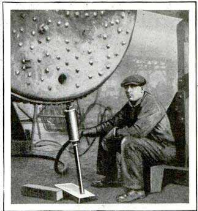
Air Bucker Used in Riveting Can Be Suitably Adjusted under Heavy Tank with Wood Blocks
