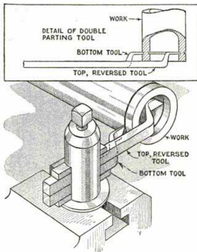
Two Offset Parting Tools Cut Collars from Both Sides of the Tubing
