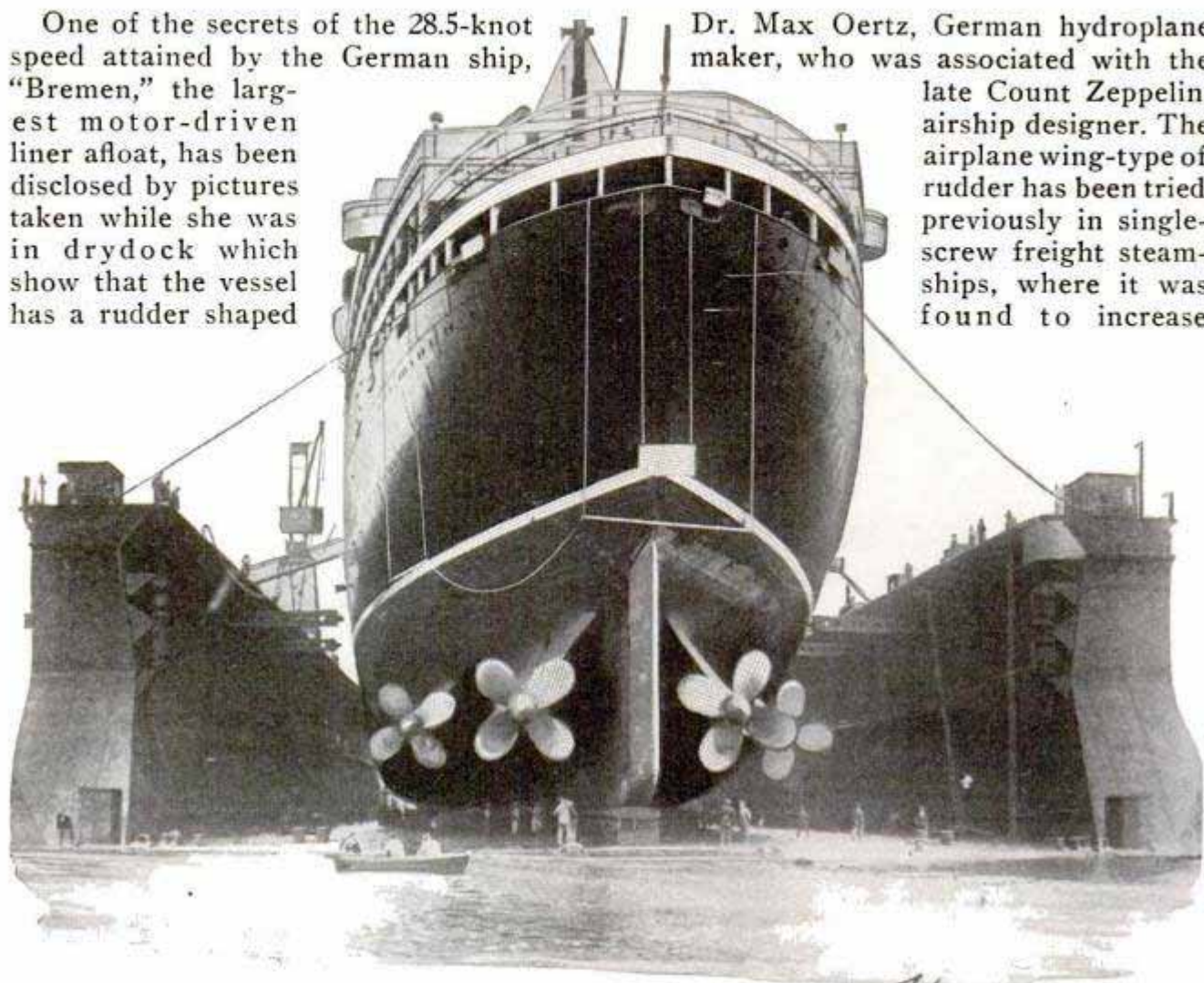
Here is the German Liner, "Bremen," Fastest Steamer Afloat, in Drydock Before Her Record-Breaking Trip to America; Note the Propellers, and the Rudder Shaped Like an Airplane Wing
