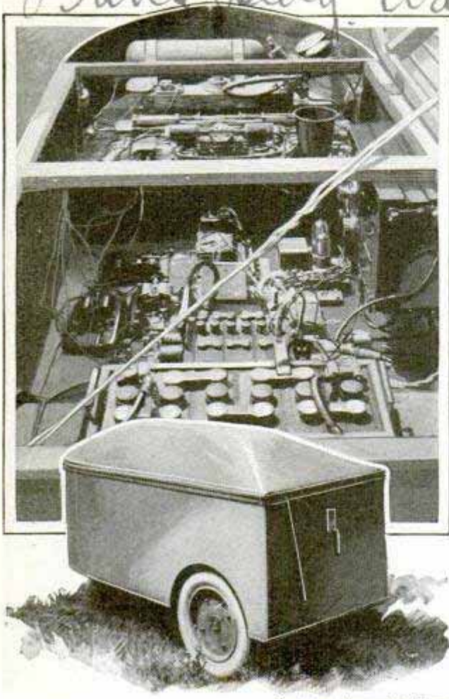
Courtesy Army Air Corps Close View of the Radio-Controlled Tank and of Its Interior Equipment
