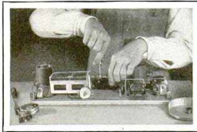
Top, Sawing Off Unused Length of Shaft at Rear of Ganged Condenser Unit; Above, Mounting Flexible Coupling for Shaft Extension
