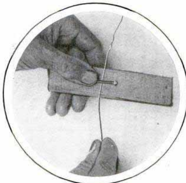
Using a Stovebolt and a Piece of Wood for Straightening Fine Wire
