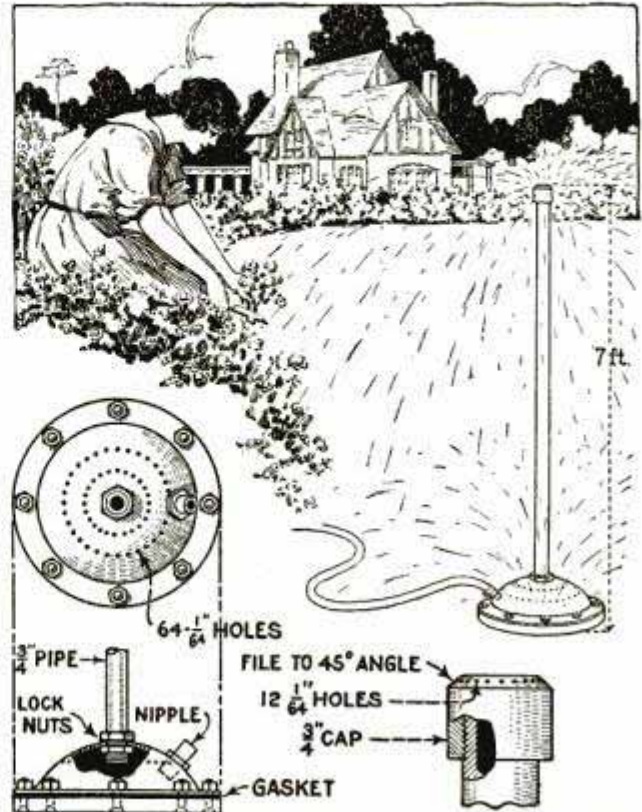
Simple Lawn Sprinkler Which Can Be Made from Pipe and Fittings
