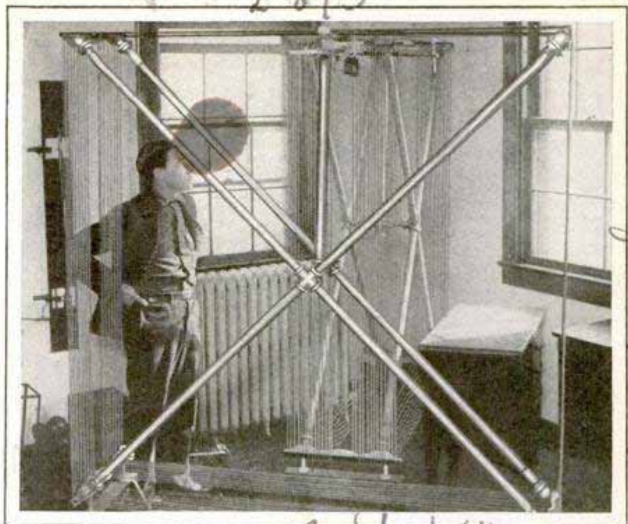
Courtesy Harris & Ewing View of the Static Apparatus Which Gives Weather Experts Indication of the Approach of Storms
