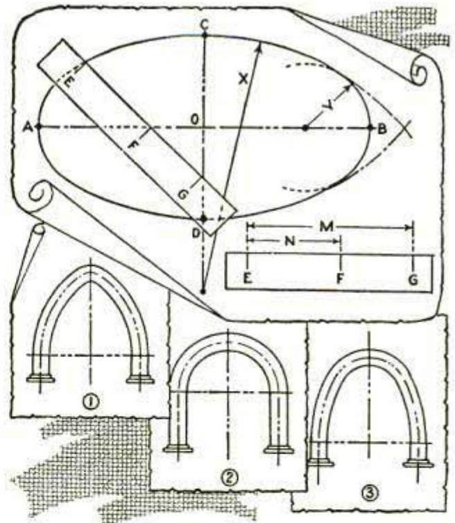
Method of Laying Out Ellipses; Applied with Care, It Produces an Accurate Curve
