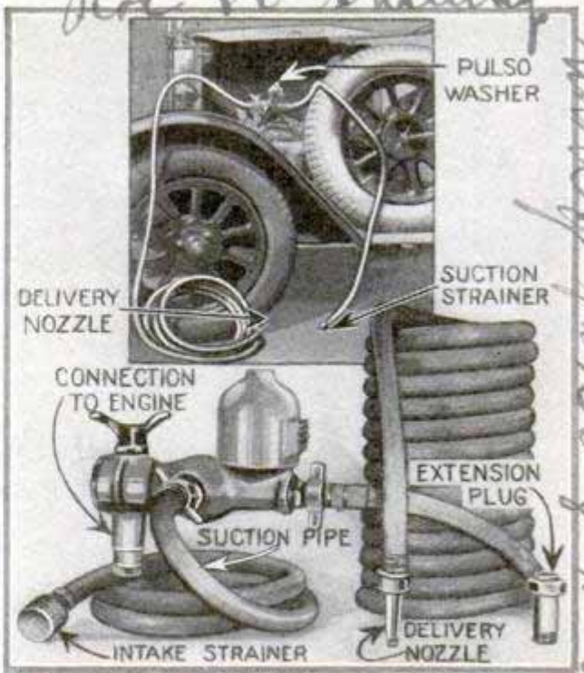
Attached in Place of One Spark Plug, This Water Cleaner Gets Pressure from Suction in the Cylinder
