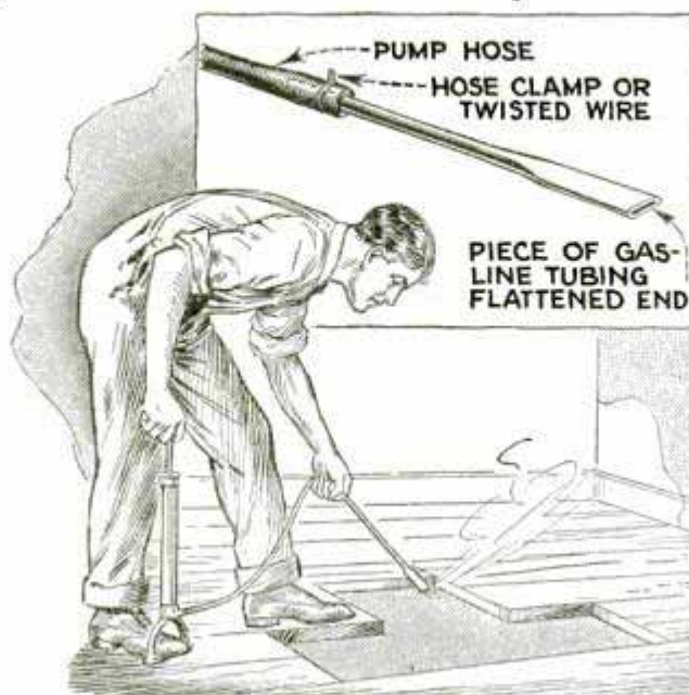
Auto-Tire Pump, Hose and Nozzle Make a Good Chip and Dirt Remover
