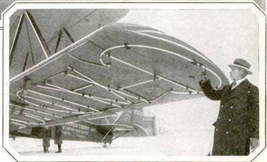
The Tri-Motored Bomber Rebuilt with an Enormous Lower Wing, to Carry the Neon Sign, and a Close-Up of the Glass Tubes
