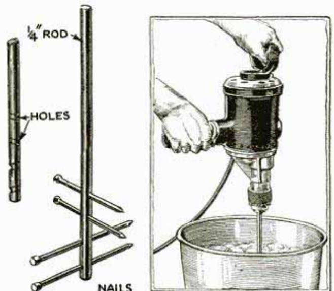
Large Quantities of Glue Can Be Quickly Mixed with the Aid of an Electric Hand Drill
