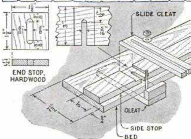
Fig. 1, Details of the Construction of the Molding Board; Fig. 2, Working a Rabbet on the Edge of a Piece Held in the Molding Board
