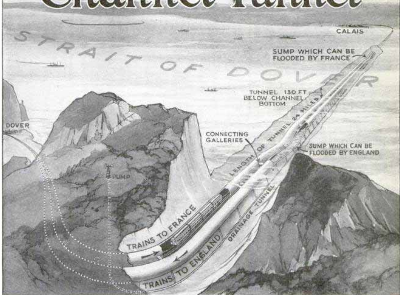
Artist's Diagram of the Proposed English Channel Tunnel, with Sumps near Either Shore to Permit Flooding against an Invasion, if France and England Should Ever Fight
