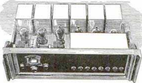
Right, Six-Tube A.C. Screen-Grid Receiver Has Automatic Control; Automatic Tuning Is Made Possible by a Mechanical Device Arranged So That the Dial Condensers Are Automatically Removed Whenever a Selection Is Made on the Automatic Finder
