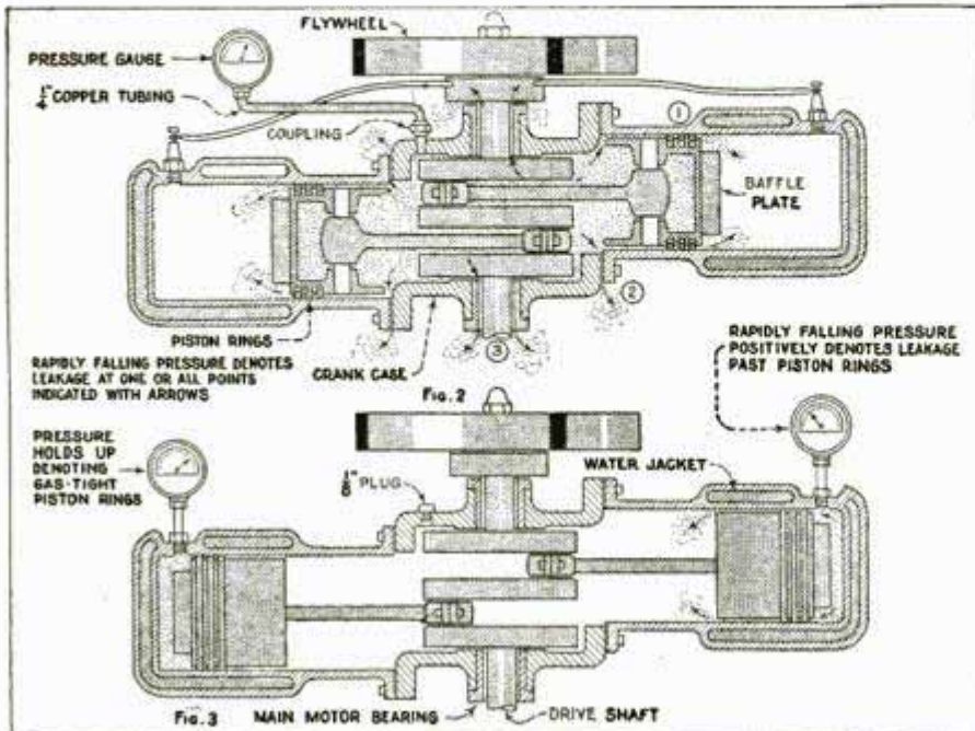
Old Auto Oil-Pressure Gauges Used for Checking Compression of Cylinder and Crankcase
