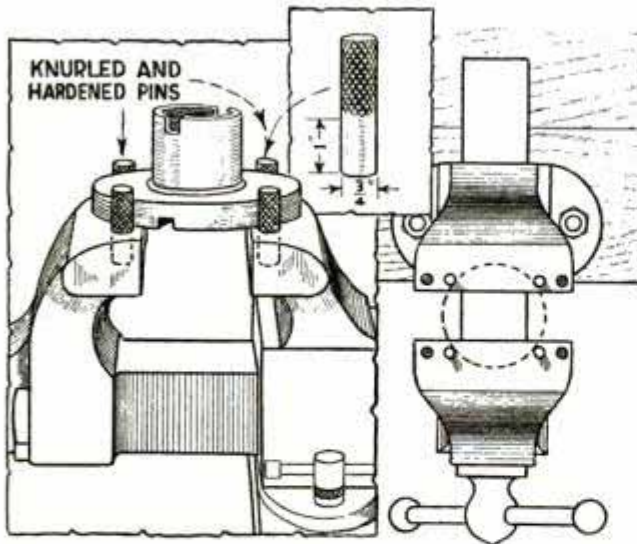
Knurled and Hardened Pins, Set in Holes in Vise Jaws, Hold Disk-Shaped Parts Securely
