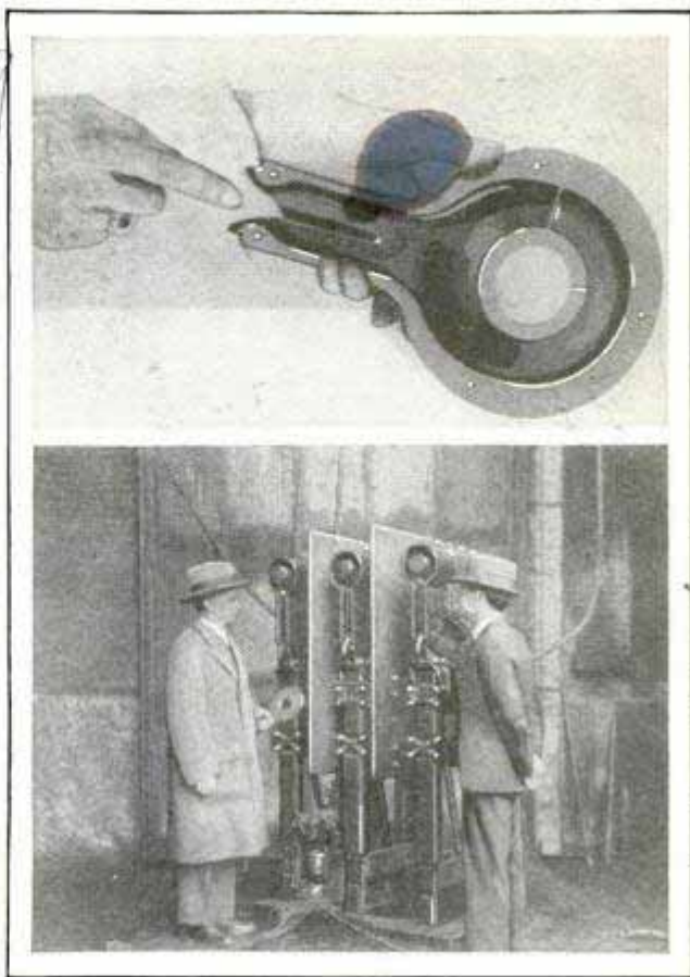
Circuit Breaker Which Stops Flash and Saves the Electric Fuses by Absorbing the Heat
