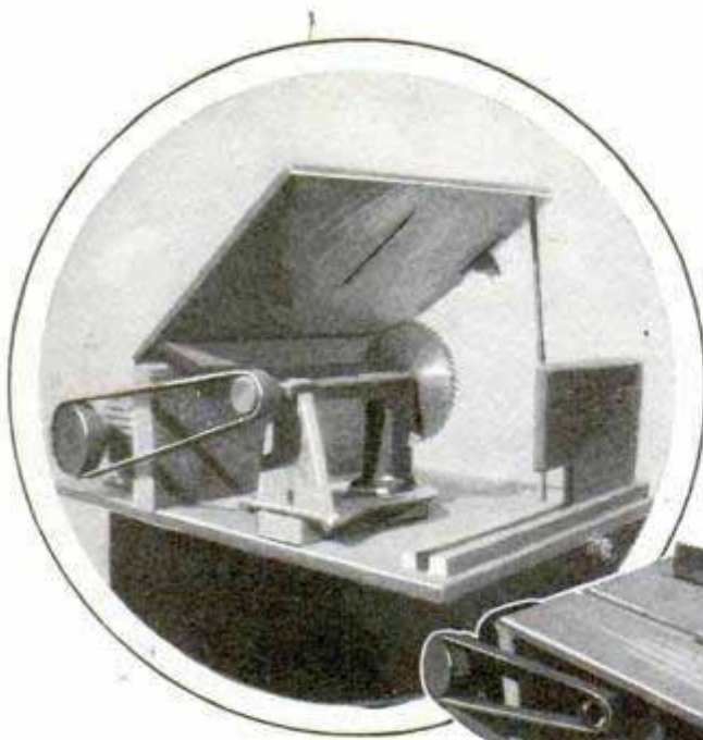
An Old Sewing-Machine Head and a 1/4-Hp. Electric Motor Were Used to Make This Handy Circular Saw
