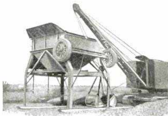
Dirt Holder Provided with Wheels to Facilitate Its Transportation
