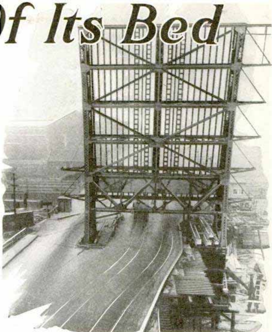
This Bascule-Bridge Leaf and Its Mate Were Built over a Busy Street; Then a River Was Dug beneath Them
