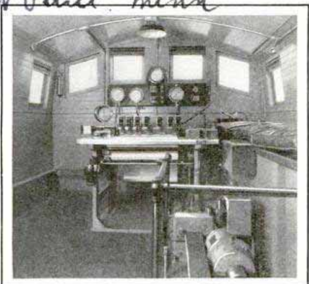
Interior of the Engine-Testing Railroad Car, Showing Chief Parts of the "Mechanical Man"
