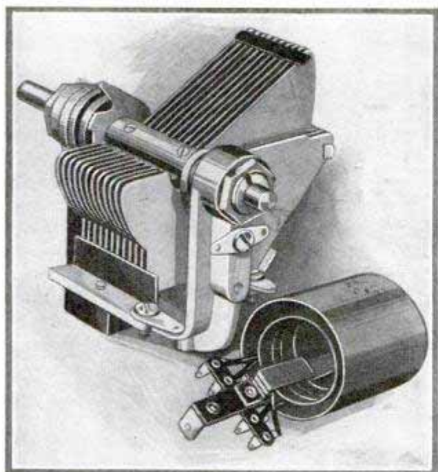
Above, Variable Condenser with Removable Shaft for Tandem Coupling; Below, Specially Designed R.F. Coil
