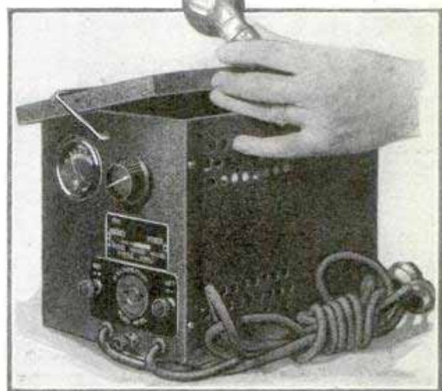
Dry A-Power Unit Showing Three-Ampere Full-Wave Tungar Bulb
