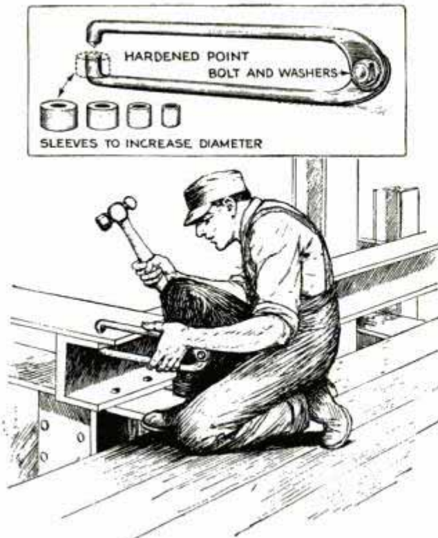
Tool Which Facilitates Transferring Hole Locations from Channels and I-Beams
