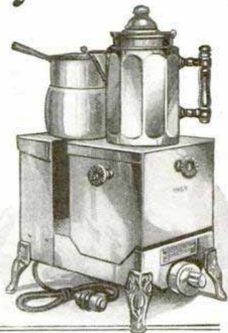
Electric Stove for Use on Table Has Burner Plate and Oven; It Will Cook, Bake or Roast and Keeps Foods Hot; Operated from 110-Volt Direct or Alternating-Current Socket
