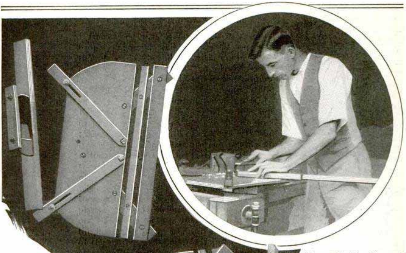
Upper Left, Top View, and Below, Bottom View of the Shooting Board; Note the Plane Clamped to the Side
