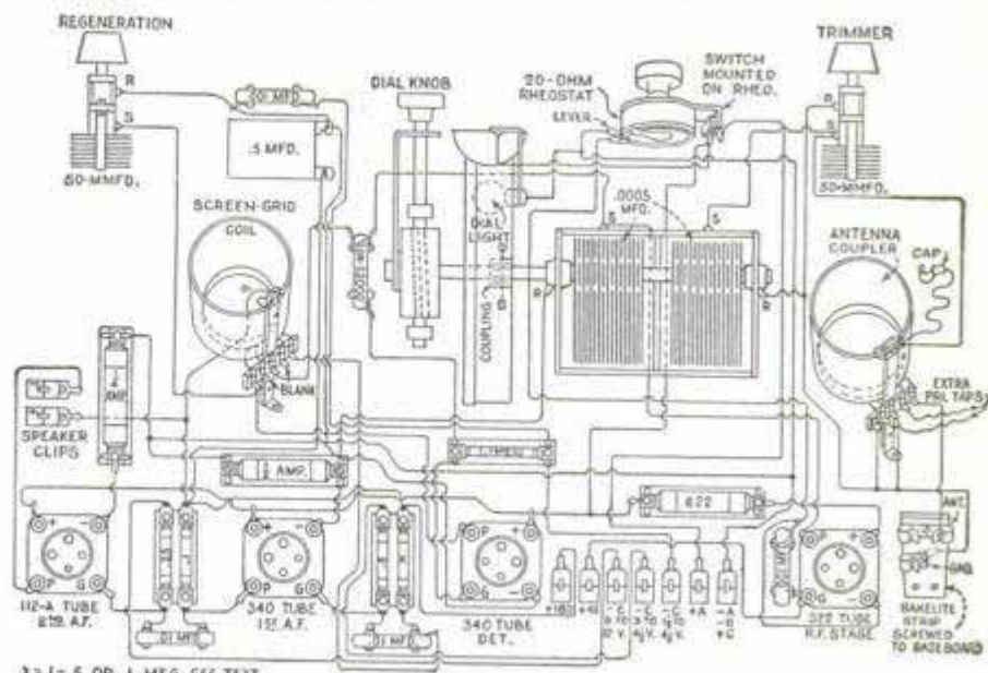
Simplified Wiring Diagram Showing the Various Instruments in Their Relative Positions
