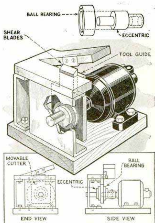
Small Electrically Operated Bench Shear for Cutting Light Sheet Metal
