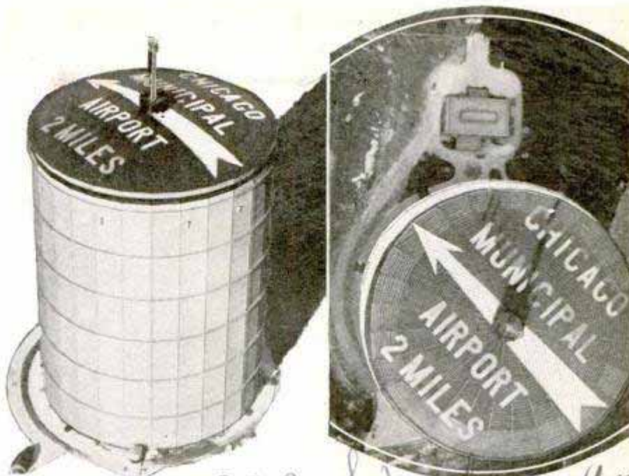
© Chicago Aerial Survey, 332 Michigan Ave. Converted into an Aircraft Beacon, a Huge Gas Holder in Chicago Now Guides Flyers to the Airport
