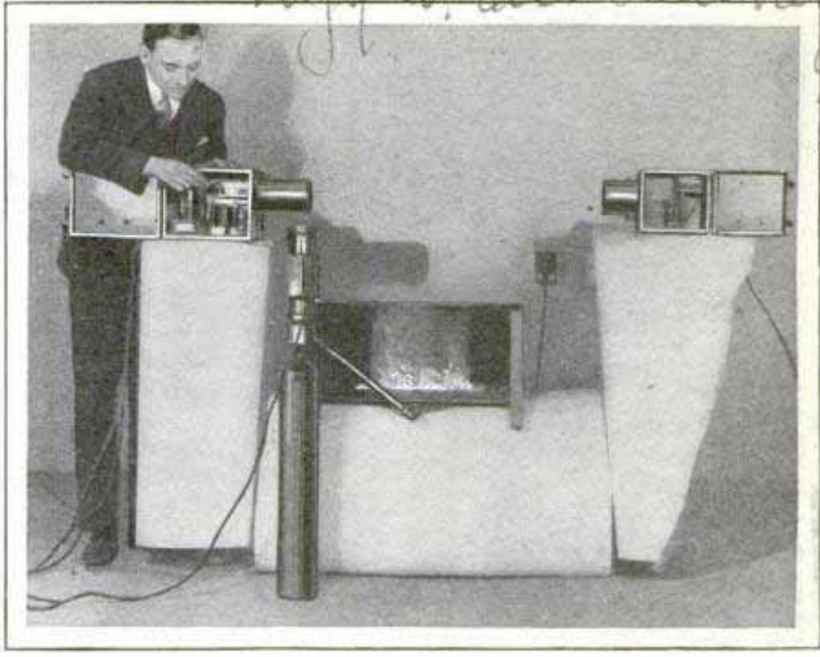
Testing Outfit Used to Demonstrate How Photo-Electric Cell Was Used to Extinguish a Fire; Smoke Caused It to Function
