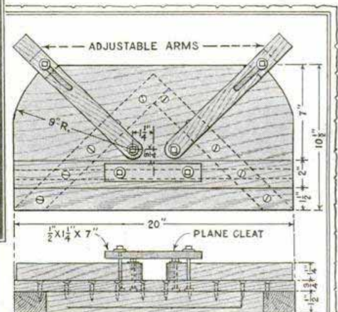
Fig. 4 PLAN AND ELEVATION OF SHOOTING BOARD
