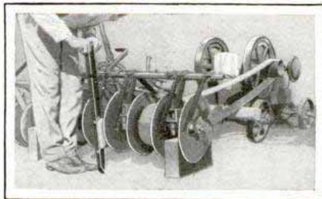
Sharpening Disk-Harrow Blades with Engine Rig and Stone Held against Them as They Revolve
