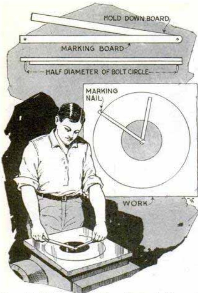
Improved Device for Scribing a Circle, the Center of Which Is over a Hole
