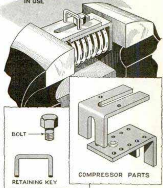
Practical Adjustable Holder for Keeping Coil Springs Compressed
