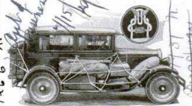
Ropes Tied to Clamps and about Luggage, and Close View of One of the Clamps
