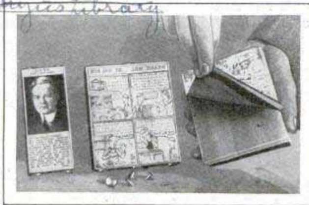
New Kind of Plate for Printing; It Can Be Sent Cheaply by Mail Because of Light Weight
