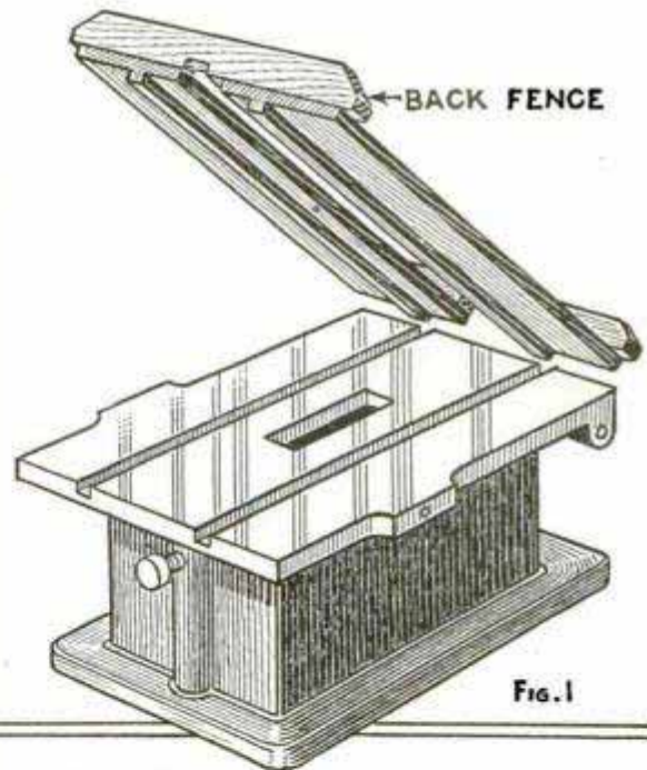
Fig. 1. Saw Table with Finished Auxiliary Table above It; Left, Dadoing with the Table; Note the Lines Squared across the Work
