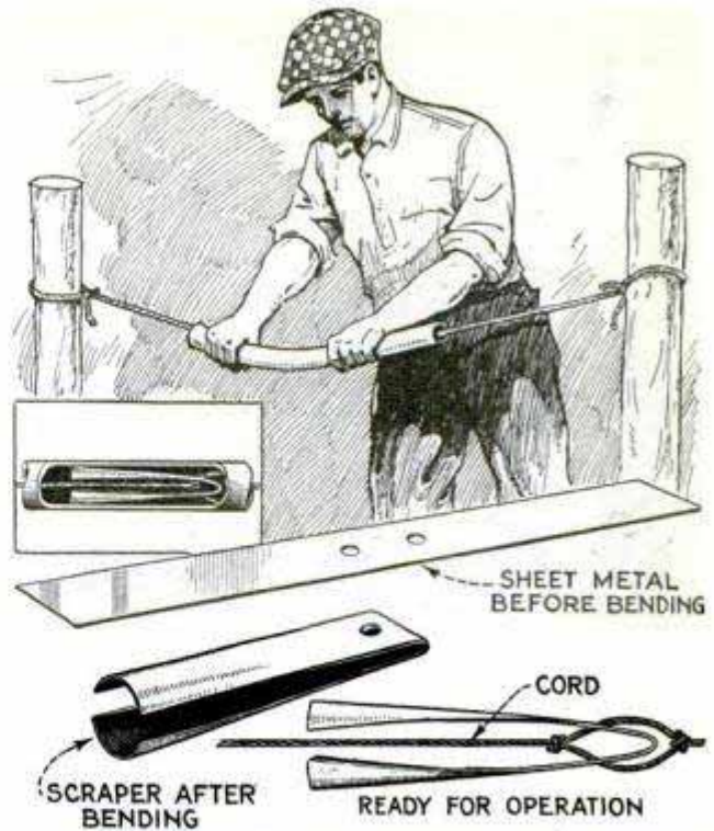
Clogged Automobile Exhaust Pipes Can Be Easily Scraped Clean on This Handy Device
