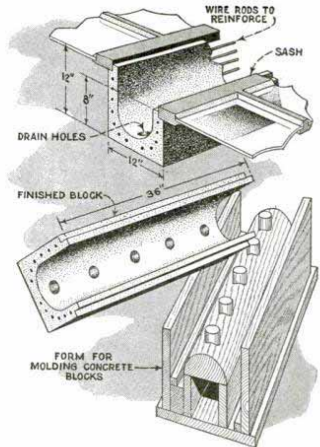
Concrete Frames for Hotbed Sashes Are Easy to Make and Neat in Appearance
