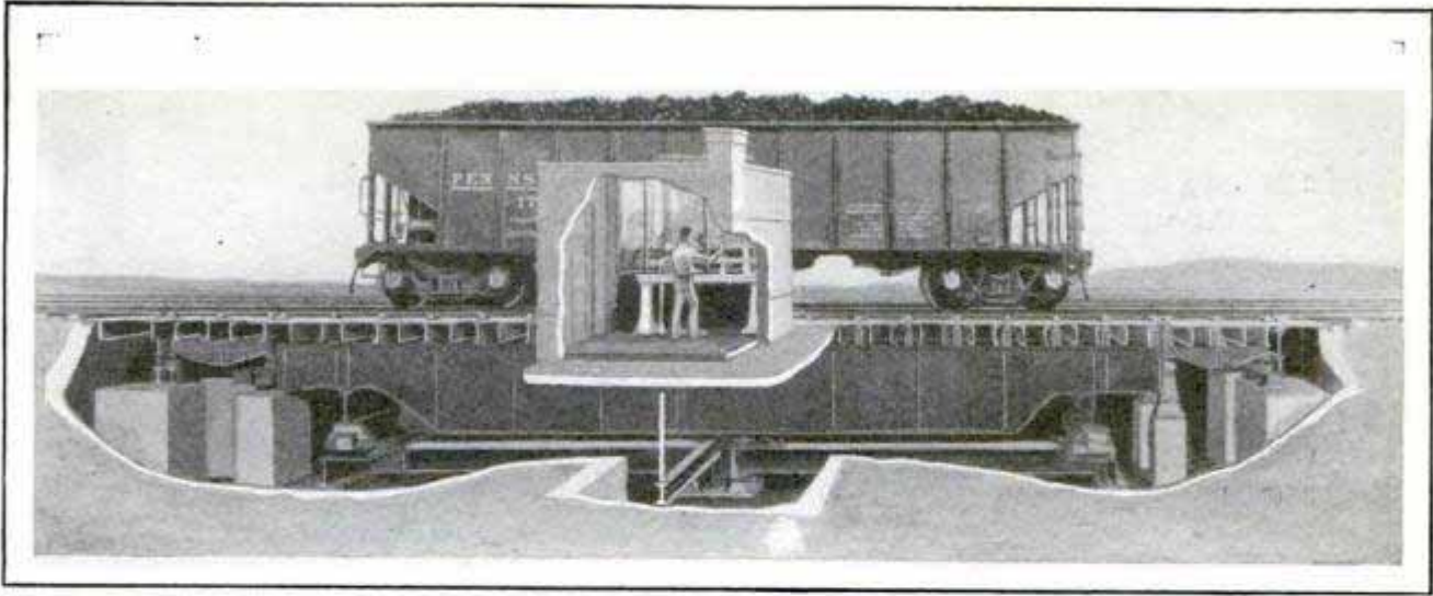
Weighing a Car Load of Coal on the Giant Balance of a Pennsylvania Railroad Fulcrum Track Scale; the Cut-Away Scale House Shows the Operator Adjusting the Balance
