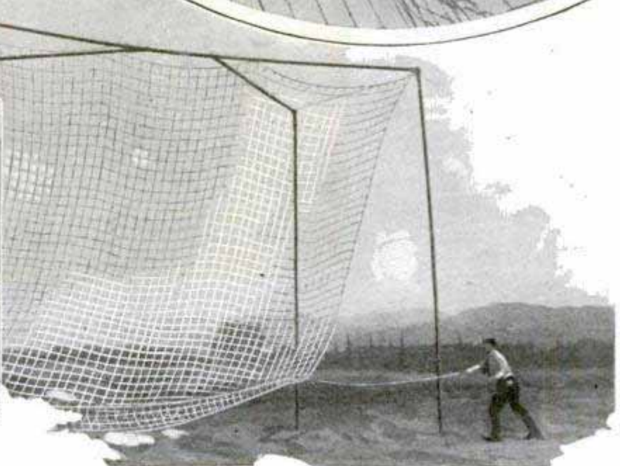
Bag in Cage Showing Teeth That Cut the Rope; the Lowering Reel on Side of Fuselage near the Pilot and Net Ready for Catching a Bag from Approaching Plane; the Trap Can Be Set Up in Any Part of the Field and Is Taken Down or Assembled in a Few Moments; Side Arms Direct Rope against the Knife
