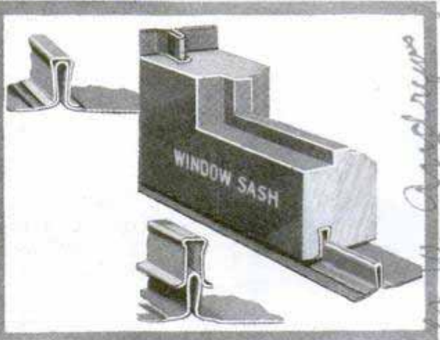
Adequate Weather Stripping, When the Old House Is Rebuilt, Can Eliminate Drafts; This Is a Metal Strip
