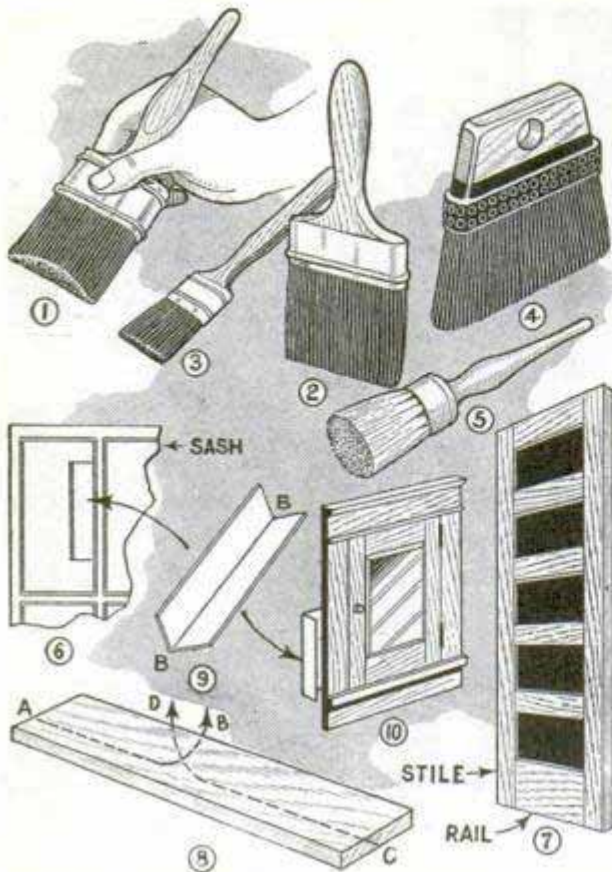
Every Home Owner Should Know What Kind of Paint Brushes to Have and How to Use Them Properly
