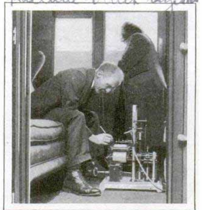
How Smooth Is the Ride? This Gauge Tells by Waving Lines When the Railway Car Sways
