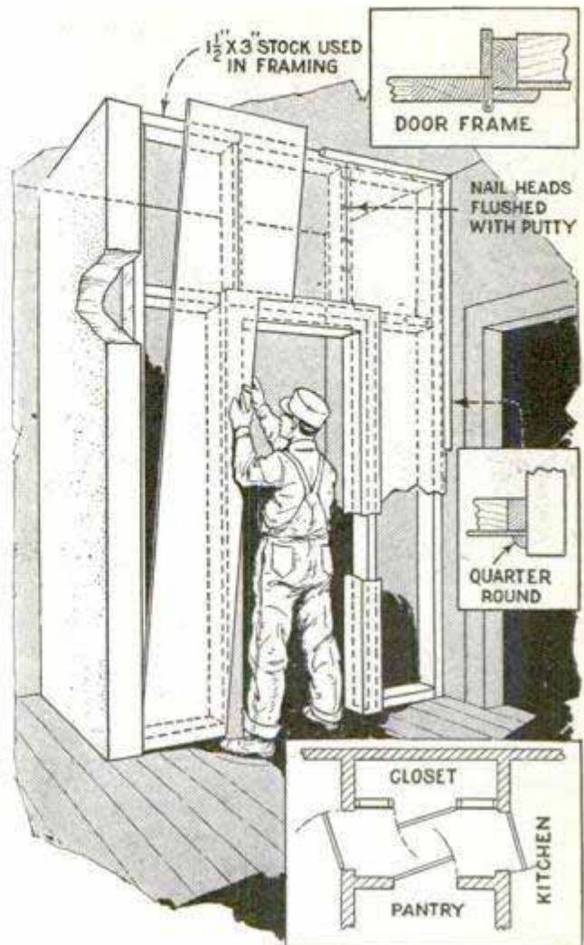
Closets Made of Wallboard and Light Studs Are Cheap and Easy to Put Up
