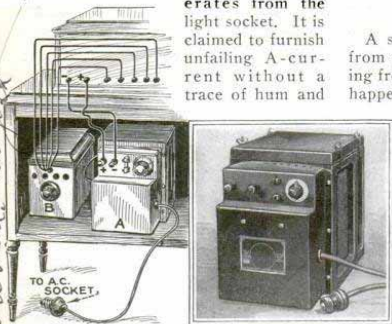
Left, A-Power Unit, Showing Installation with B-Eliminator, for Complete A.C. Operation of D. C. Sets
