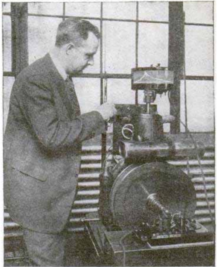
This is Thomas Midgley, Jr., the inventor of Ethyl Gasoline, and the Midgley Optical Indicator, the machine which played such an important part in the development of Ethyl. The Midgley Optical Indicator, mounted on an engine, took a picture of what occurred inside the combustion chamber and enabled Mr. Midgley and his associates to establish the cause of the "knock."
