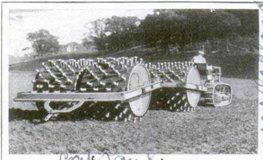
Roller with Feet That Help Tamp the Soil and Break Up Clods; the Rollers Are Weighted with Water
