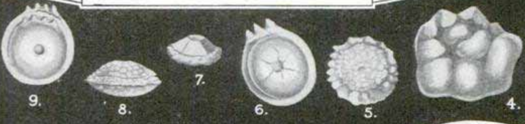
Hailstones of Curious Shapes Gathered after a Storm in Central Europe, and False Dew on Clover, Drops Exuded by the Plant Itself and Not Condensed from the Atmosphere; How Large Are the Largest Hailstones, Is a Frequent Question; One, Weighing Four and One-Half Pounds and Ten Inches Long, Fell through the Roof of a House in Germany in August, 1925; Other Larger Stones Have Been Reported but Are Not So Well Authenticated; the Various Layers of the Stones Are Formed by the Irregular Fall of the Lump from the Sky to the Earth
