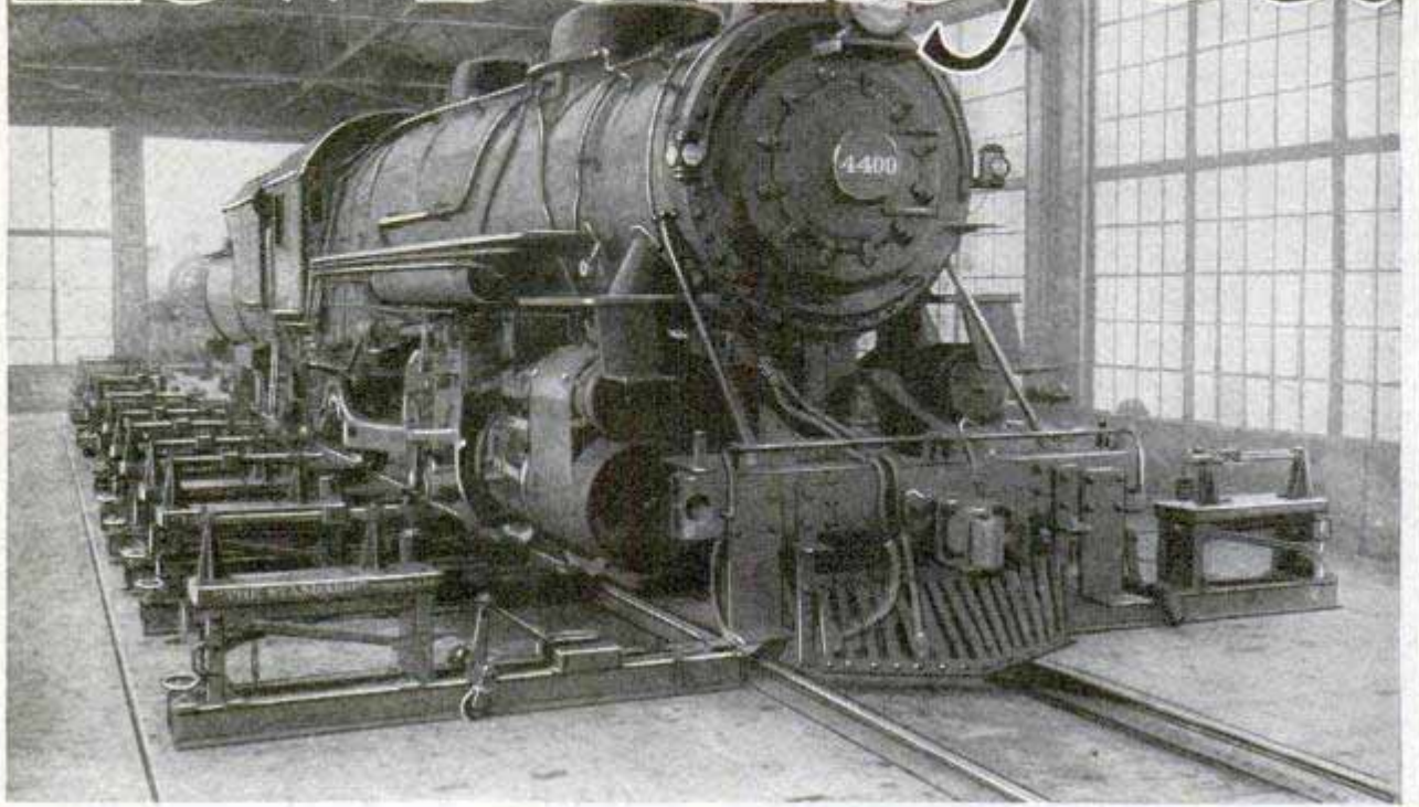
Weighing a New Locomotive in the Shops of the Baldwin Locomotive Company, at Philadelphia; Separate Track Sections and Scales Catch the Weight on Various Parts
