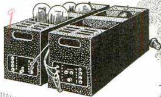
Left, an A and B-Eliminator Which Supplies All Required Voltages from D. C. Supply Lines, Ranging from 110 to 250 Volts, and Is Suitable for Sets Employing from 1 to 14 Tubes; Right, a Powerful Three-Stage Push-Pull Audio Amplifier, for Radio Set, Phonograph Reproducer or Microphone, Employs the New 250-Type Power Tubes
