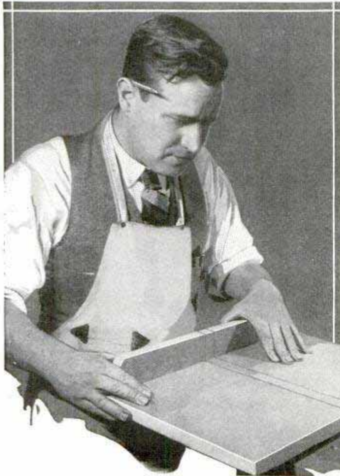
Fig. 1. Saw Table with Finished Auxiliary Table above It; Left, Dadoing with the Table; Note the Lines Squared across the Work
