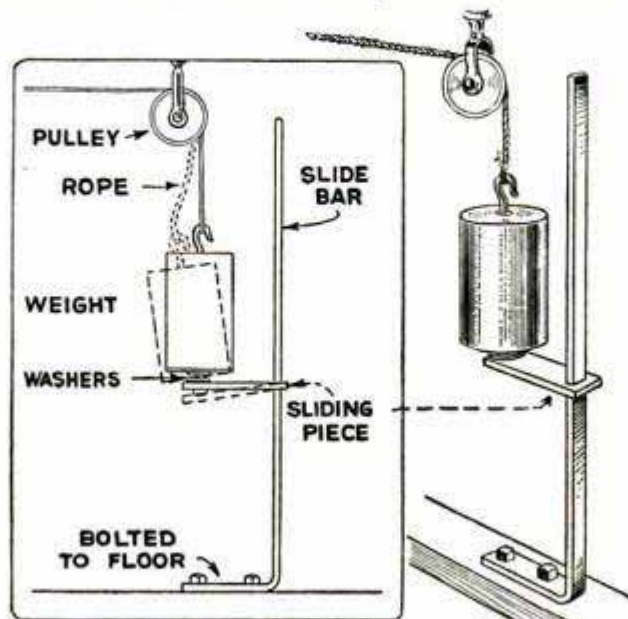
Device for Arresting the Fall of a Counterweight in Case the Rope Breaks
