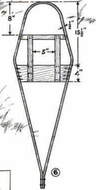
The Rawhide of the Traditional Snowshoe Is Replaced by Galvanized Screening, or So-Called "Hardware Cloth," Cut to Shape with Tin Snips and Tacked in Place
