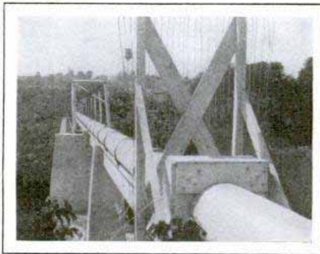
Aerial Sewer, Built of Concrete, Suspended across a River, Found Better Than Tunnel beneath Stream
