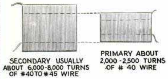
Disassemble the Burned-Out A. F. Transformer as Shown Above; the Parts Are Laminations, Secondary, Primary and Shield
