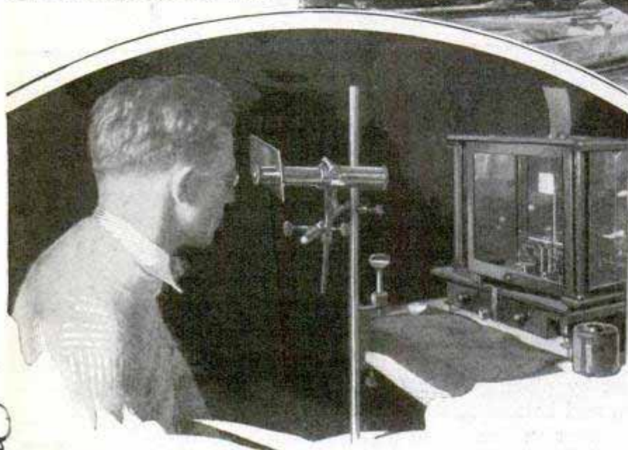
Lowering the Seventy-Five-Foot Fulcrum-Scale Bridge into a Scale Vault on the Pennsylvania Railroad; the Completed Scale Bridge, Including Rails and Ties, Weighs 143,000 Pounds; at Left, Examining at Close Range the Cabinet-Inclosed Precise Test Scale at the U. S. Bureau of Standards; This Machine Will Weigh Objects Down to the Thousandth Part of a Milligram; Some Laboratory Scales Weigh the Millionth of a Milligram
