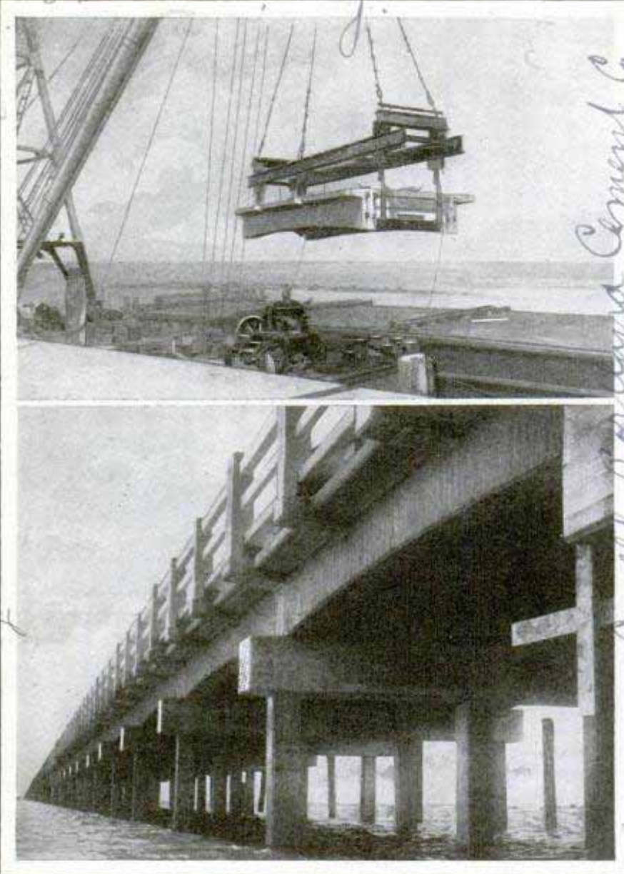
Swinging a Load of Bridge Sections into Place, and View of Part of the Structure, Showing Method of Assembly
