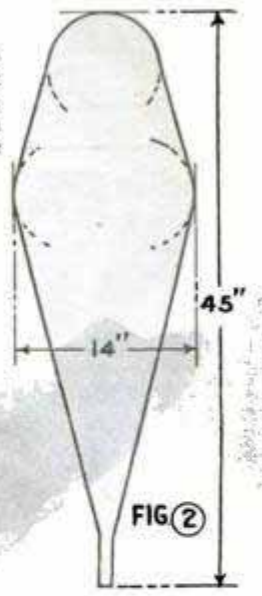
Fig. 2. How the Shape of the Snowshoe Frame Is Laid Out on the Boards; Fig. 3, Tin Cans and Wood Blocks Make the Form around Which the Frames Are Bent
