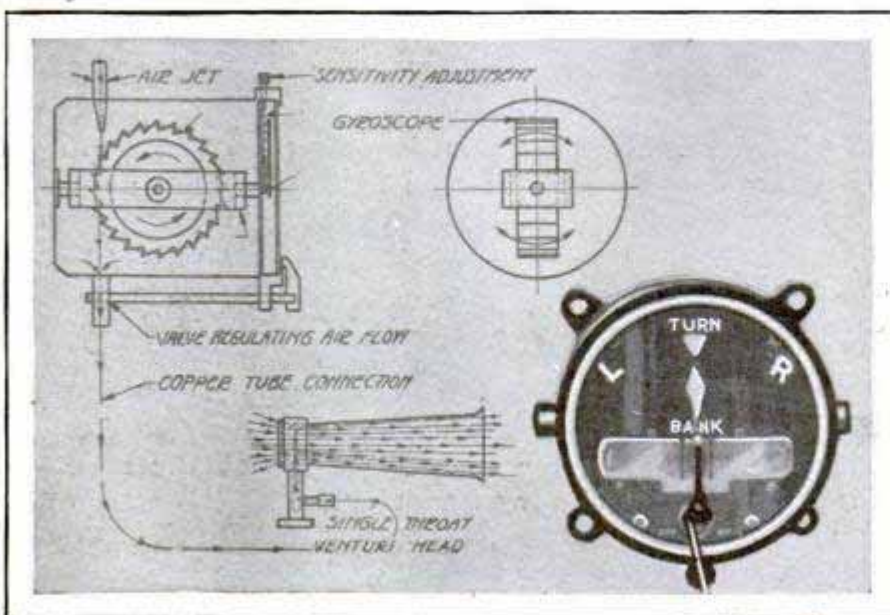
Diagrams Showing the Working of the Gyrostatic Turn Indicator and the Flight Guide, or Inclinometer
