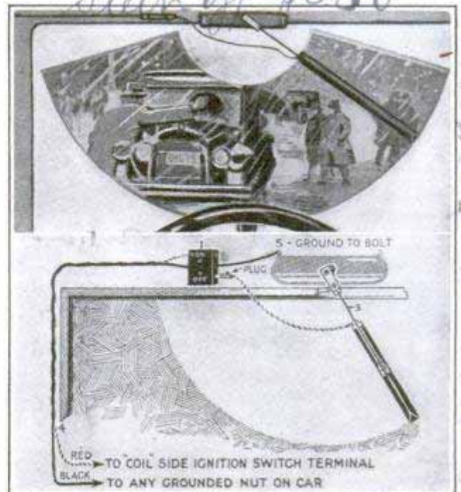
Drawings to Illustrate the Effect of the Heated Windshield Wiper and the Method of Connecting It
