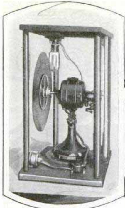
Left, Homemade Television Receiver Showing Fan Motor in Position; Right, Front View of the Apparatus Showing Radio Receiver and Loud Speaker Mounted Above
