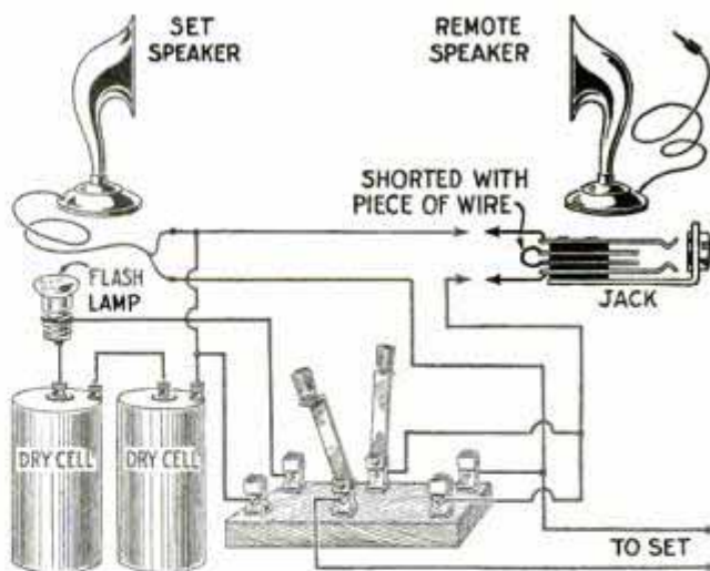
Remote-Speaker Control, Showing the Jack and Lamp Arrangement for Checking the Distant Speaker
