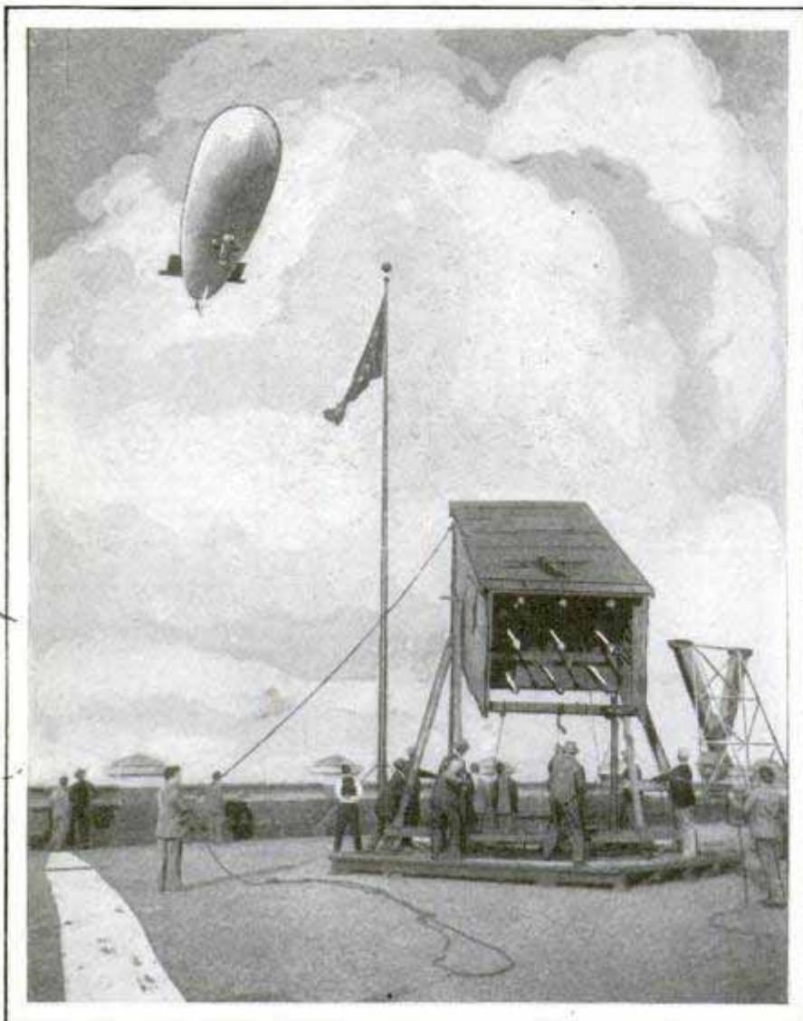
Special Horn That Projects a "Beam of Sound" for the Guidance of Aircraft; It Is Effective at 1,500 Feet and More
