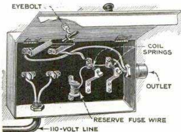
Safety Switch and Fuse Box Which Throws Out the Switch Automatically
