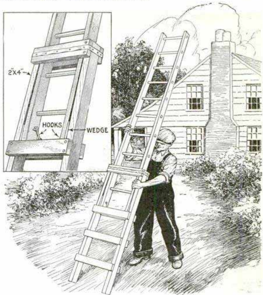
Five-Foot Extension for the Ladder Which Permits the Worker to Reach Otherwise Inaccessible Places
