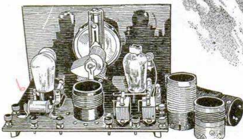
A Simple Short-Wave Receiver Now Available in Kit Form for Long-Distance Broadcast Reception and Experimental Television Signals; Easily Assembled from Standard Parts, This Receiver Employs a Screen-Grid Tube and Specially Designed Plug-In Coils
