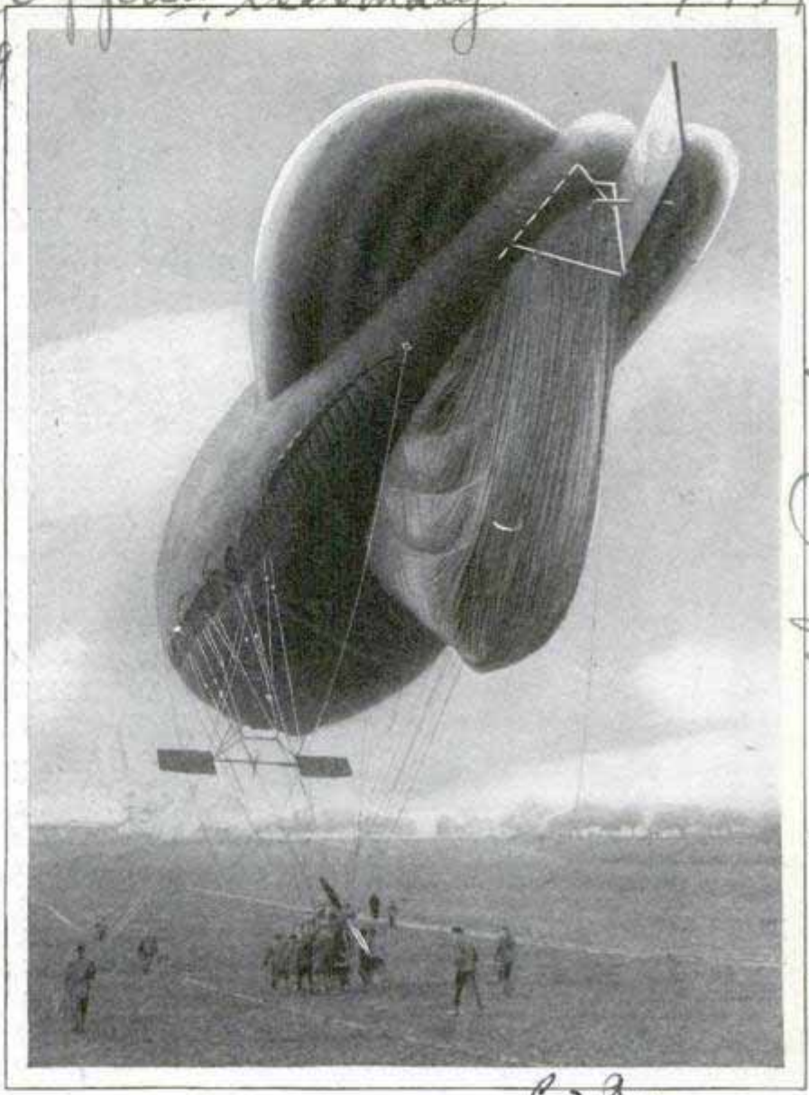
With a Rudder at the Tail, Elevators Forward and an Outboard Motor and Propeller on the Basket, the Balloon Becomes a Dirigible
