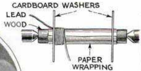
Above, Coil Mounted for Winding; Count Turns on First Layer and Multiply Layers for Total Count; Cover Each Layer with Paraffin Paper; Dry Coils in Slow Oven before Re-assembling
