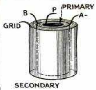
Above, Primary and Secondary Assembled; P and B Are the Primary Leads, a Negative and Grid the Secondary
