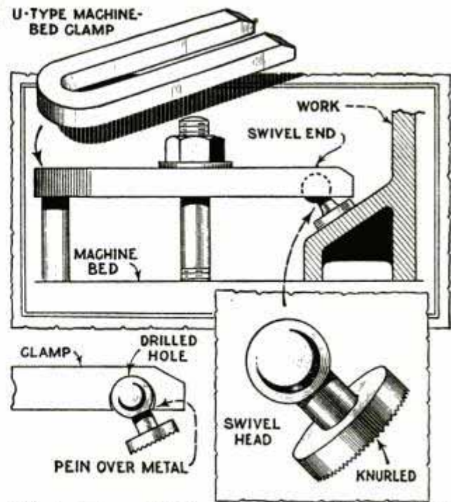
Swivel End on Machine-Bed Clamp Helps to Hold Non-Parallel Work Securely
