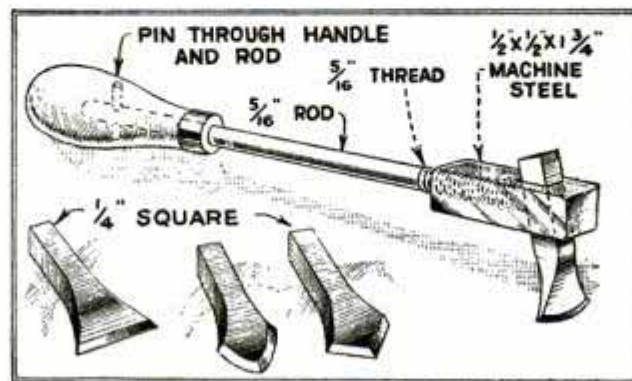
Adjustable Scraper with Tips of Different Shapes Facilitates Carbon Scraping
