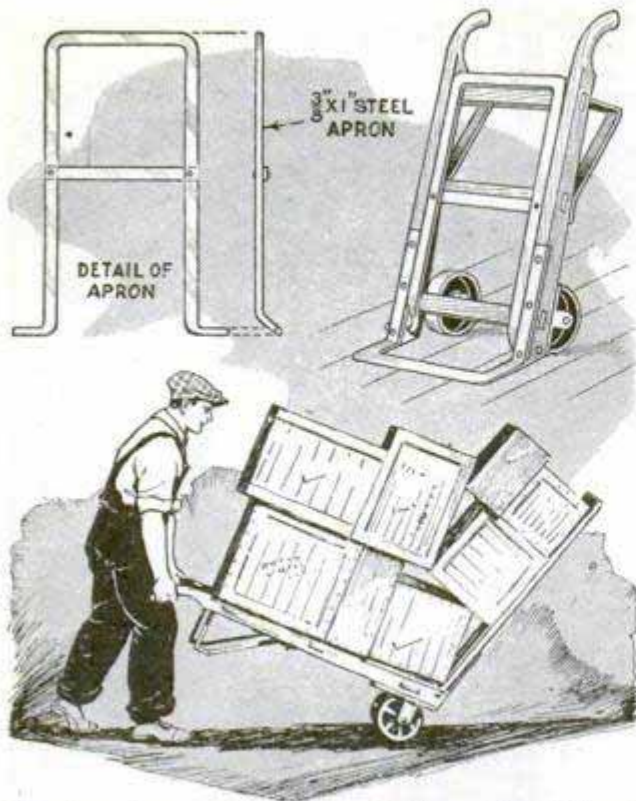
Flat-Iron Apron, Attached to Ordinary Hand Truck, Increases Its Capacity
