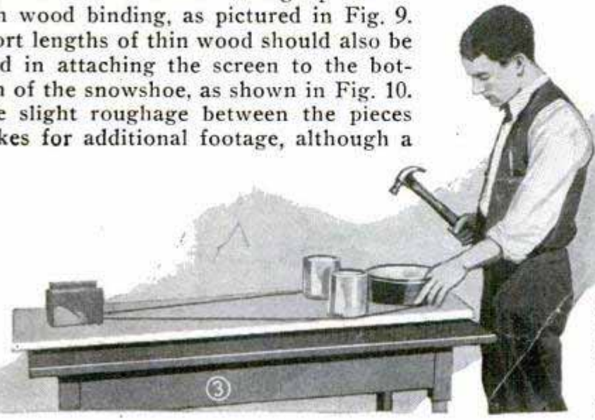
Fig. 2. How the Shape of the Snowshoe Frame Is Laid Out on the Boards; Fig. 3, Tin Cans and Wood Blocks Make the Form around Which the Frames Are Bent
