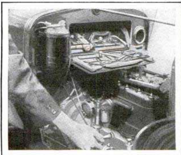
Tool Kit Open for Easy Access; Its Installation Does Not Interfere with the Wiring
