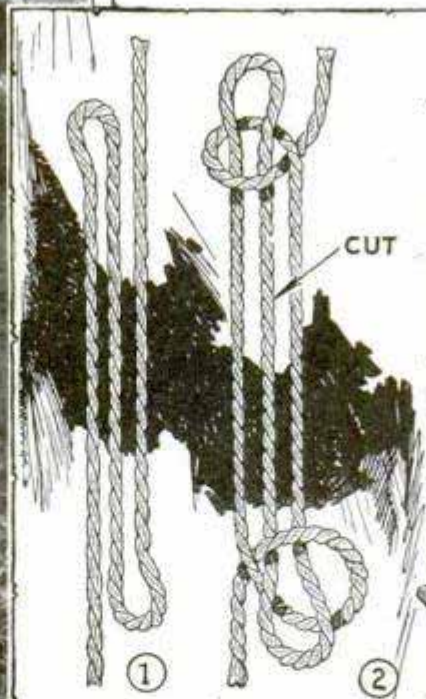
DIAGRAMS SHOWING CONSTRUCTION OF SHEEPSHANK
