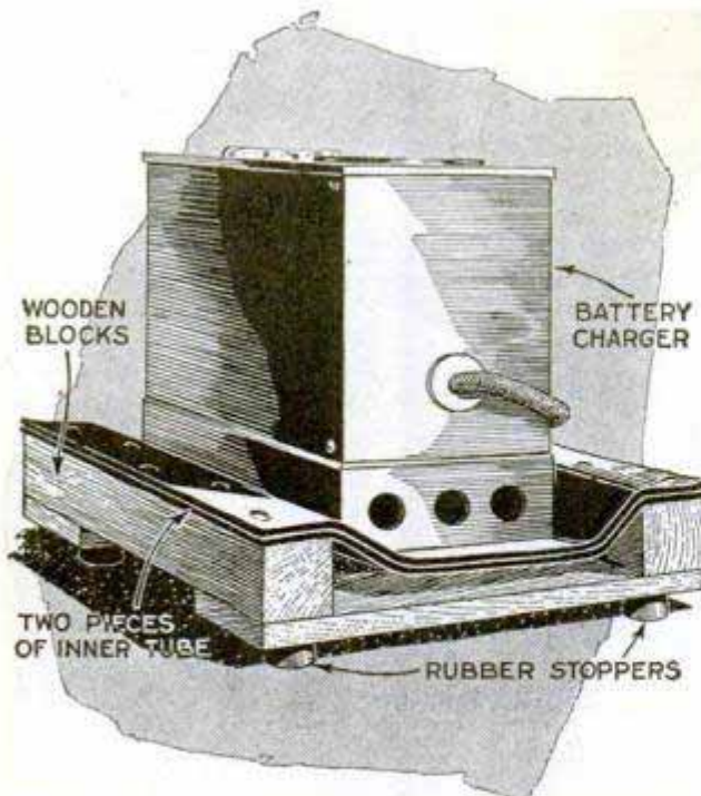
Details of Support for Reducing Noise of Operation, Showing Charger in Position
