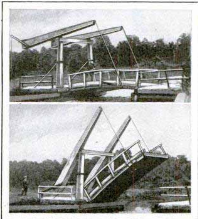
Old-Style Balanced Bridge Still in Use over a Canal within Twenty Miles of London, England
