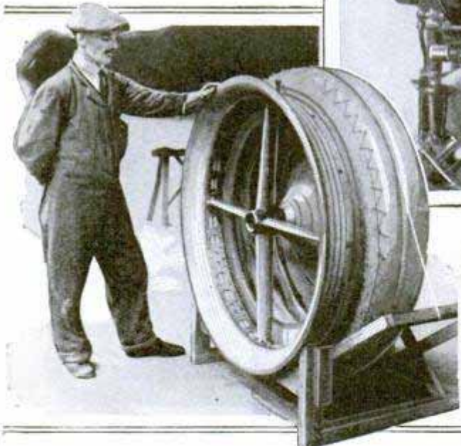
Above, a Rim of One of the Big Wheels of the "R-101," to Be One of the World's Largest Airships, Now near Completion at Cardington, Eng.; It Is for Service on the England-Egypt-India Route; Right, View of a Gas Valve of the "R-101"; This Ship Is 750 Feet Long and the Gas Bag Has a Capacity of Almost 5,000,000 Cubic Feet
