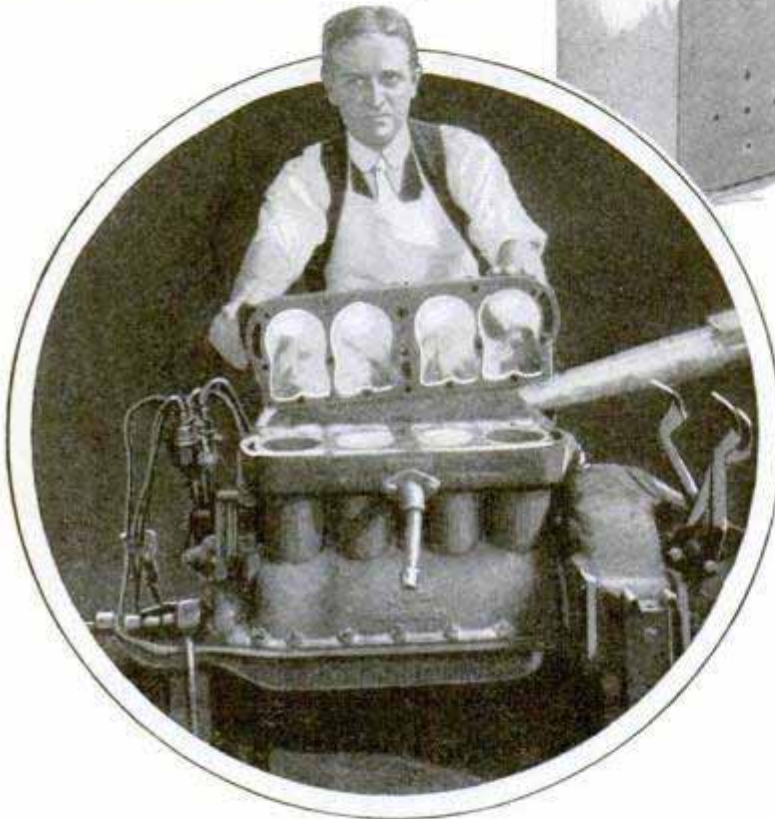
Sheet-Metal Box Used to Mix the Corn Flour and Air to Form an Explosive Product, and the Auto Engine, with Head Removed, Showing, at Right, the Pipe through Which the Mixture Is Sucked
