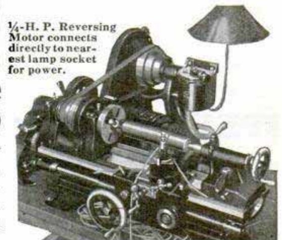
Only $18.64 per month 9"x3' New Model Junior Self-Contained Motor Driven Bench Lathe, complete.
