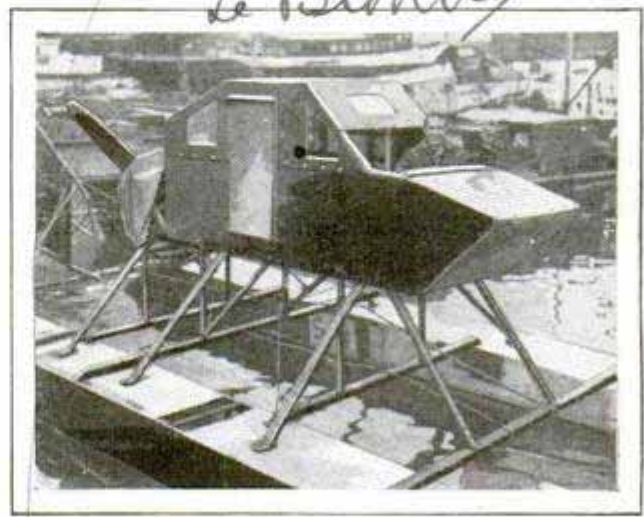
Speed Boat Built like Wingless Seaplane, for Which Eighty-Five Mile Speed Is Claimed
