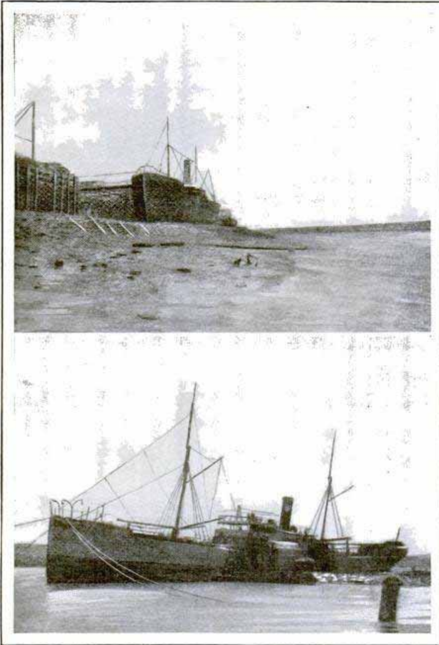
Courtesy U. S. Coast and Geodetic Survey High and Low Tide in the Bay of Fundy, Showing a Ship on Dry Land at the Low Stage and Afloat at High
