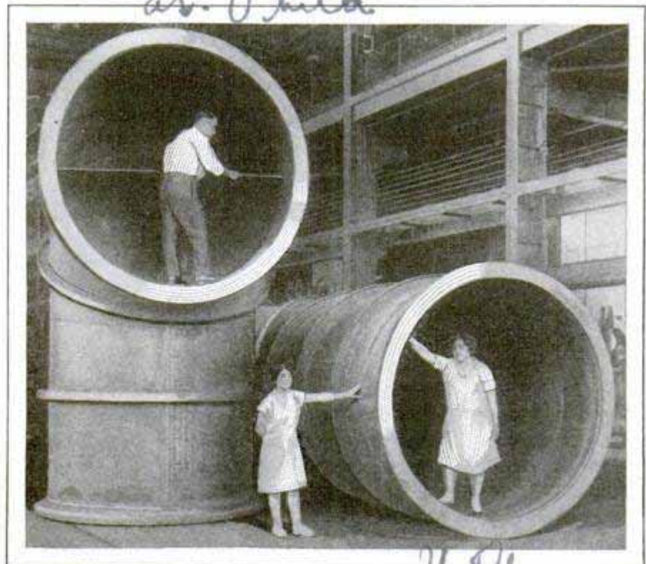
Giant Steam Pipe, Seven Feet in Diameter, Formed by Arc Welding of Steel Plates, a New Time and Money-Saving Method
