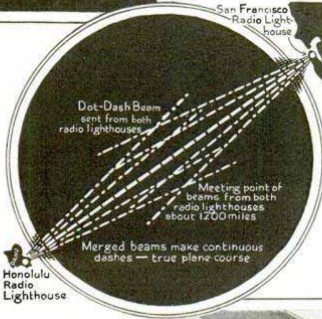
Diagram of the Radio-Beacon System, Which Sends Code Signals That Blend in a Central Path into a Continuous Chain of Dots, and, Above, Arrangement of the Visual Signal Lights Which Convert the Beacon Signals into Green and Red Lights on the Plane's Instrument Board
