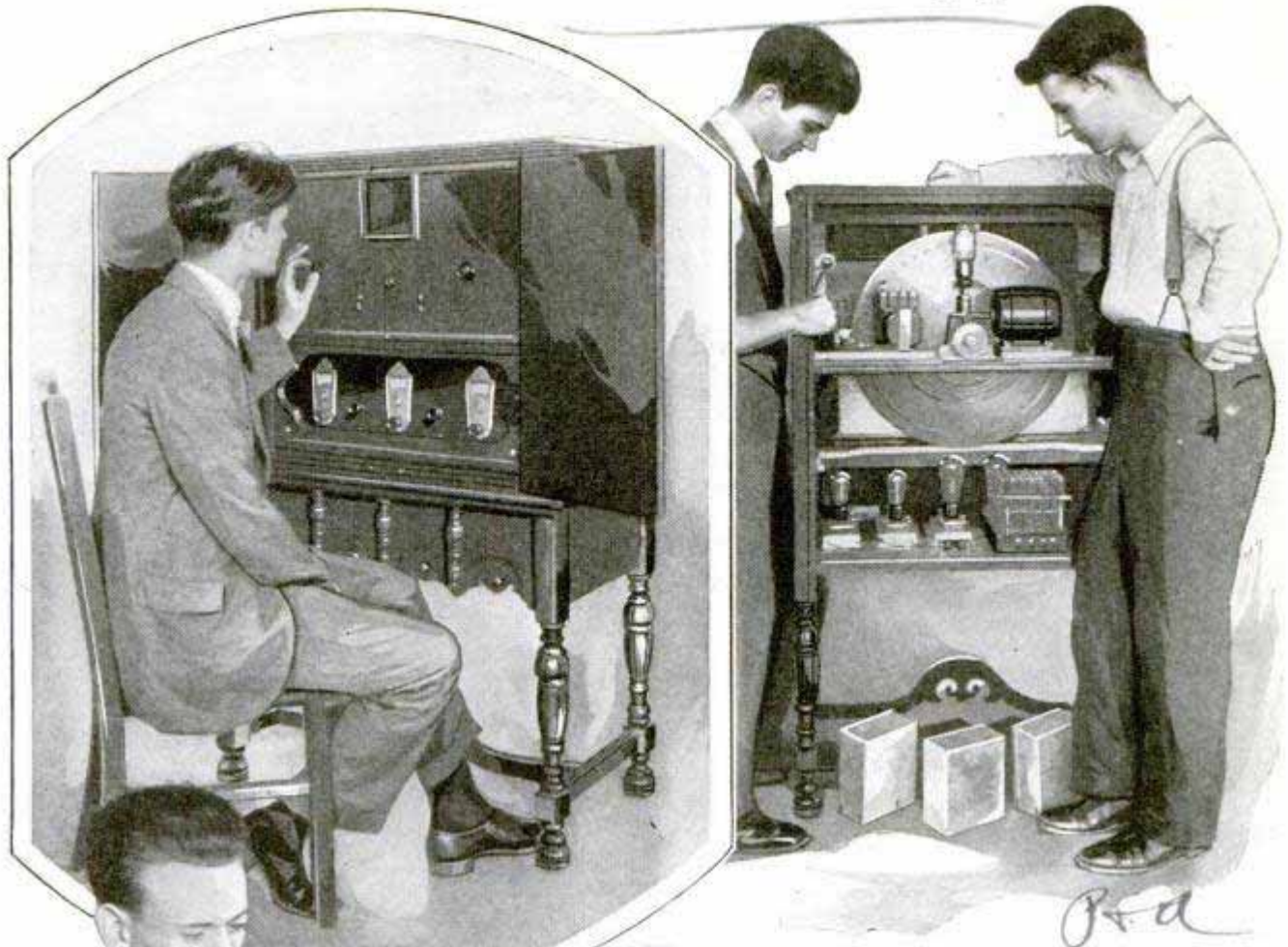
Above, Left, John Gelso, of the Pilot Electric Mfg. Co., Adjusting His Complete Television Receiver and Observing a Test Picture; Right, Rear View Showing the Arrangement of the Apparatus
