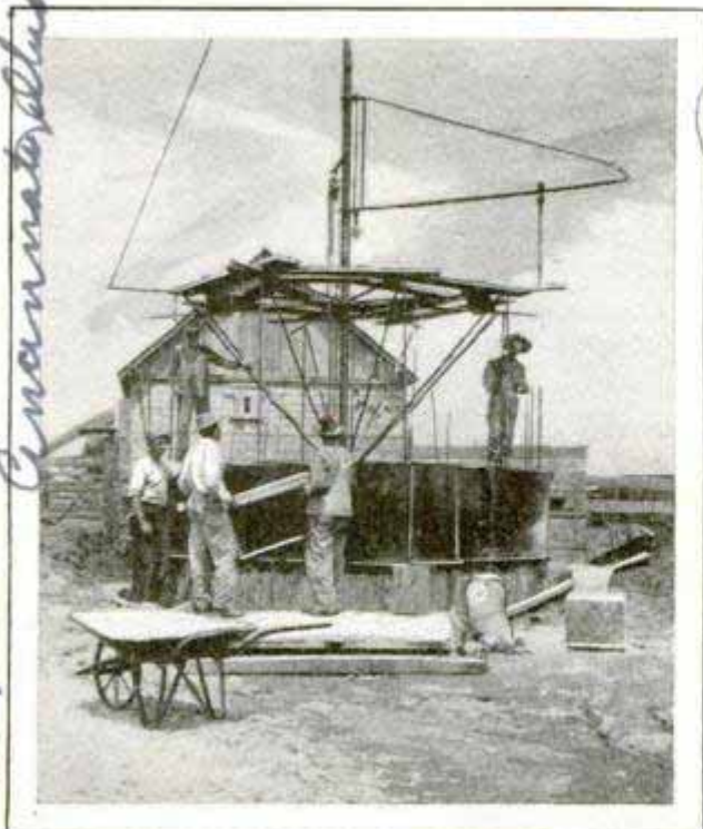
Mast and Movable Forms Which Speed Building of Circular Storage Bins of Reinforced Concrete
