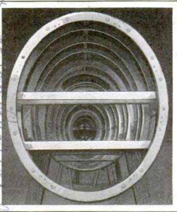
Looking into the Fuselage Framework of the Airplane Constructed for Wilkins' Proposed South Pole Flight
