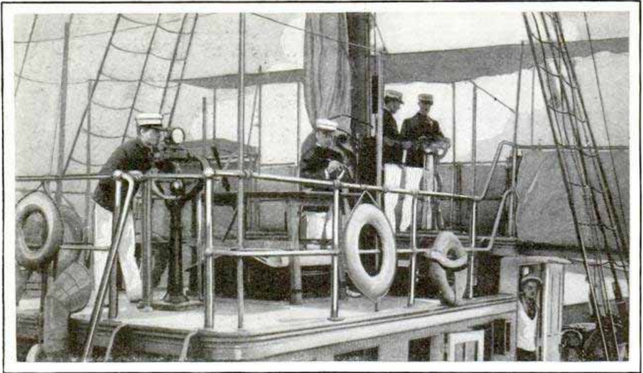
Scientists of the Carnegie Institution Making Magnetic Observations Aboard the Famous Ship "Carnegie," Which, Because of Its Construction, Is the Only Non-Magnetic Vessel Afloat
