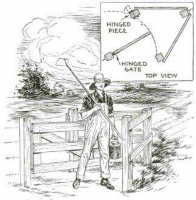
Hinged Gate for the Farm Is Convenient and Cannot Be Left Open by Mistake
