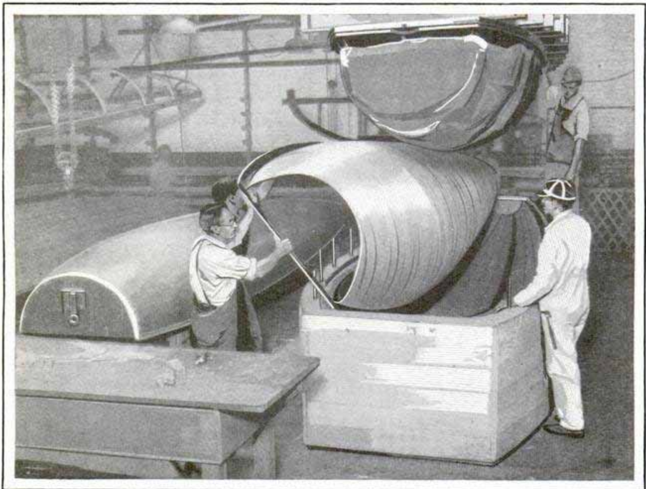
Sheets of Vincer Are Glued Together, Then Placed in This Concrete Mold and Formed into Fuselage Halves under a Pressure of Fifty Tons; Two Halves Are Then Joined
