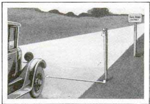
Warning Bell at Crossing and Trap Bar by Which It Is Rung as Auto Passes
