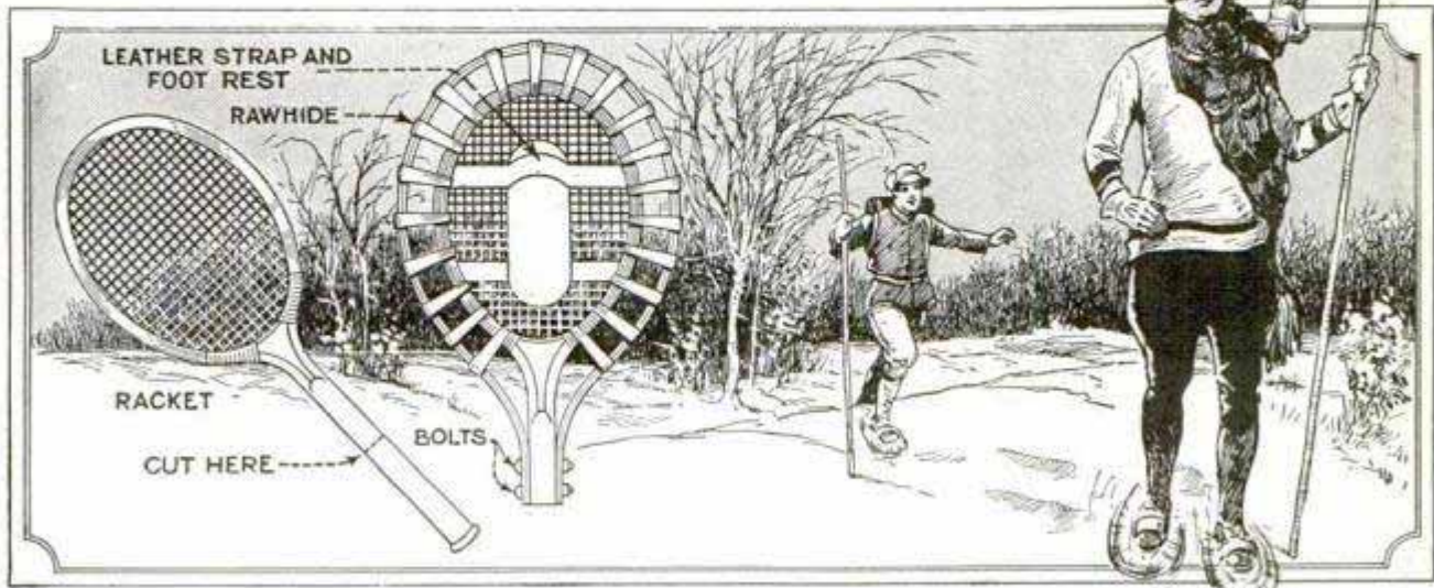
Tramping over Loose Snow Is Great Sport. These Snowshoes Were Made from Old Tennis Rackets and Anyone Handy in the Home Workshop Can Duplicate Them
