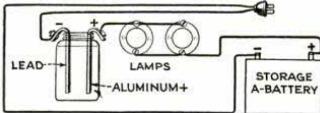
Completed Trickle Charger Mounted on Wood Base, and Wiring Diagram Showing Connections
