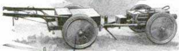
Light Mortar as It Is Packed on Mule Back, and the Truck Outfit Which Also Carries Ammunition
