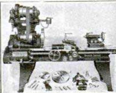
18" x 8' Quick Change Gear Motor Driven Lathe - $908
