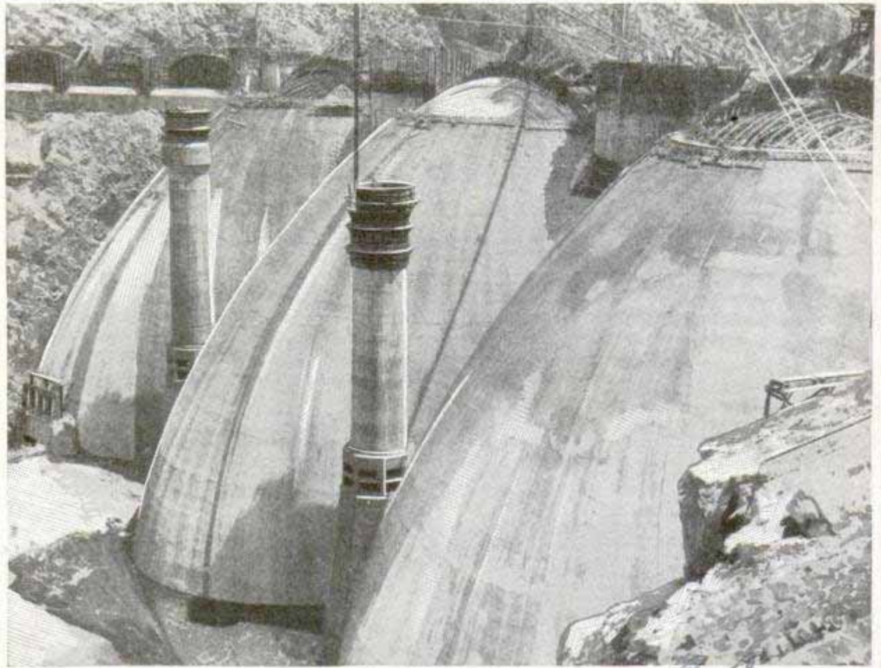
Constructed to Withstand Severe Strains; the Multiple-Dome Coolidge Dam across the Gila River, near Phoenix, Ariz.; It Has Been Built at a Cost of Almost $3,500,000
