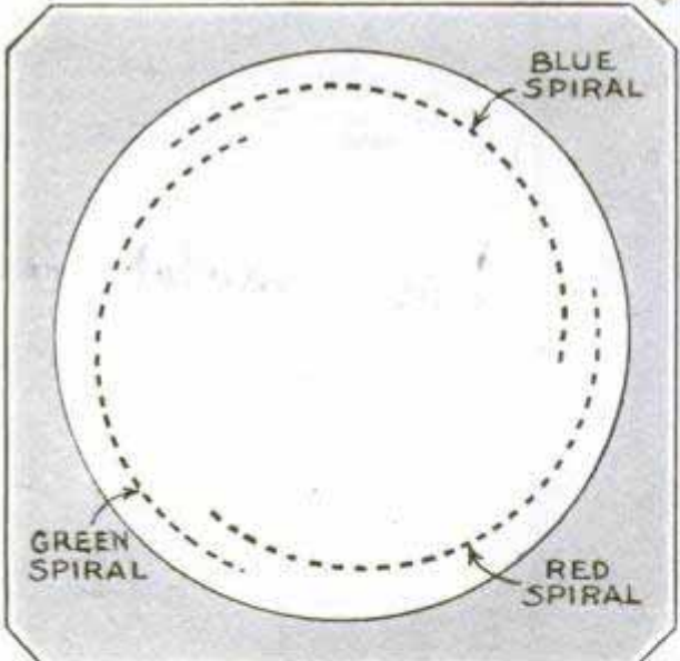
Transmitting a Daylight Television Picture; Drawing to Show the Perforated Transmitter Disk That Helps Produce Color Effects, and Demonstrating Receiver
