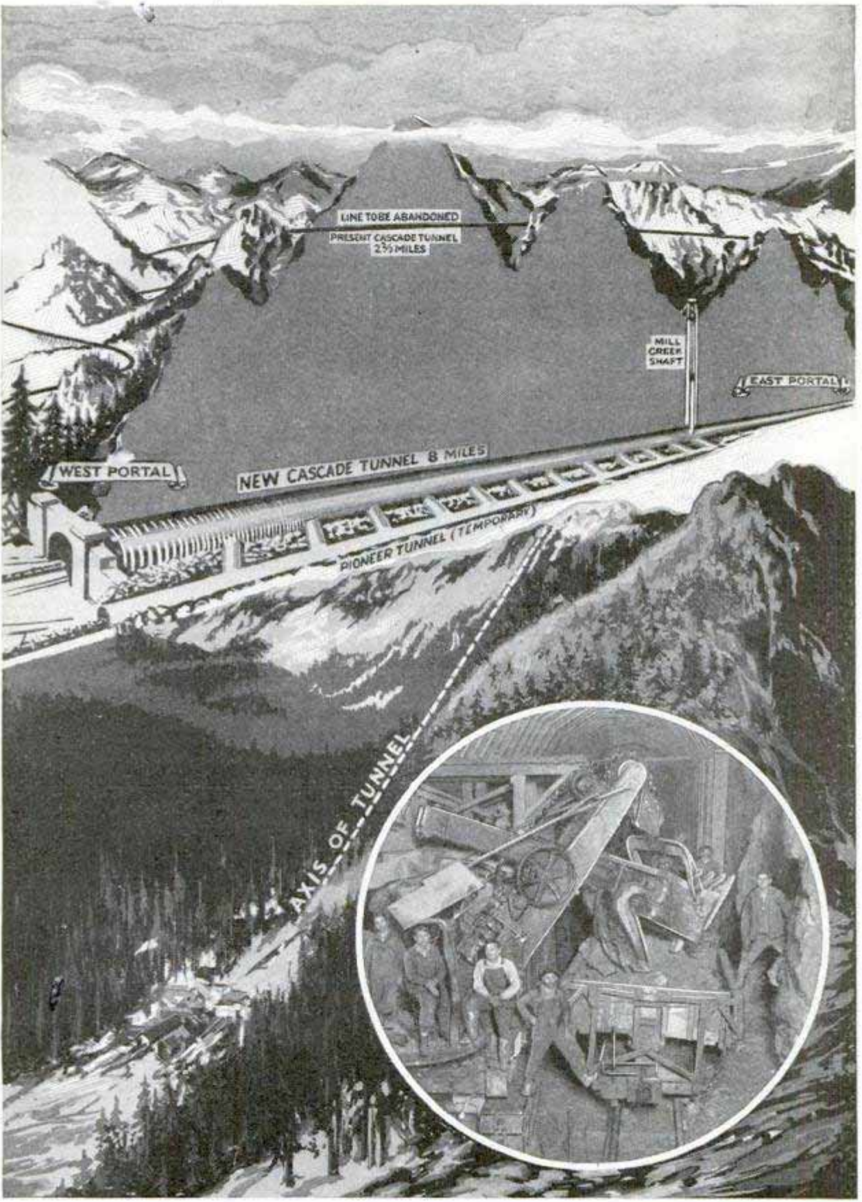
Cross Section of the Cascades, Showing the New Tunnel 500 Feet Below the Present Railroad Line; Photograph of the Range under Which the Big Bore Passes, and, in Circle, One of the Compressed-Air Shovels That Works in Limited Quarters to Clear Away the Rock
