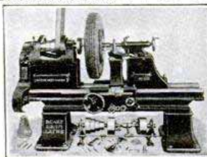
18" x 8' Quick Change Gear Motor Driven Lathe - $908
