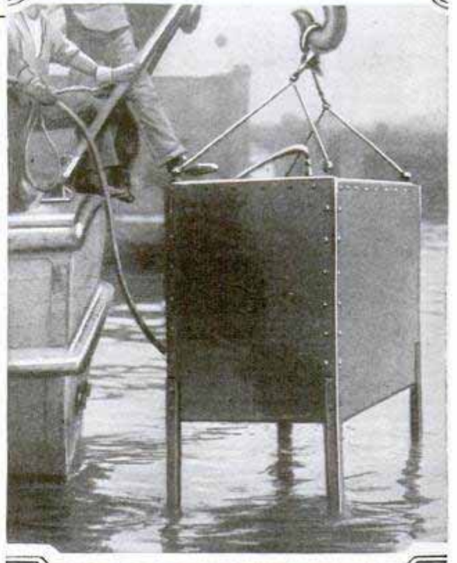
Close View of the Bell That Aided in Rapid Descents during Breathing-Mask Tests by the Navy; Note Air Hose and Connection
