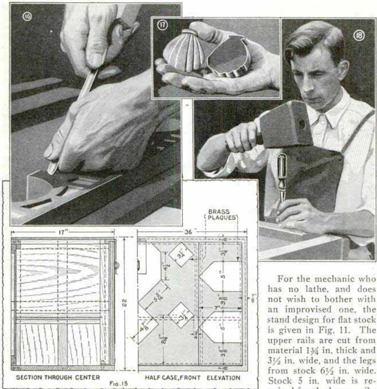
Fig. 16, Carving the Flower Ornaments; Fig. 17, Shell Ornaments in Process of Carving; Fig. 18, Outlining the Carving
