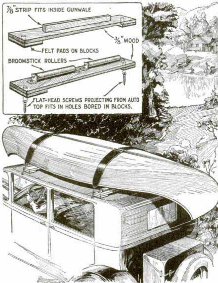
This Easily Made Canoe-Carrying Rig Will Not Spoil the Appearance of Your Sedan; Insert, Details of Holding Blocks
