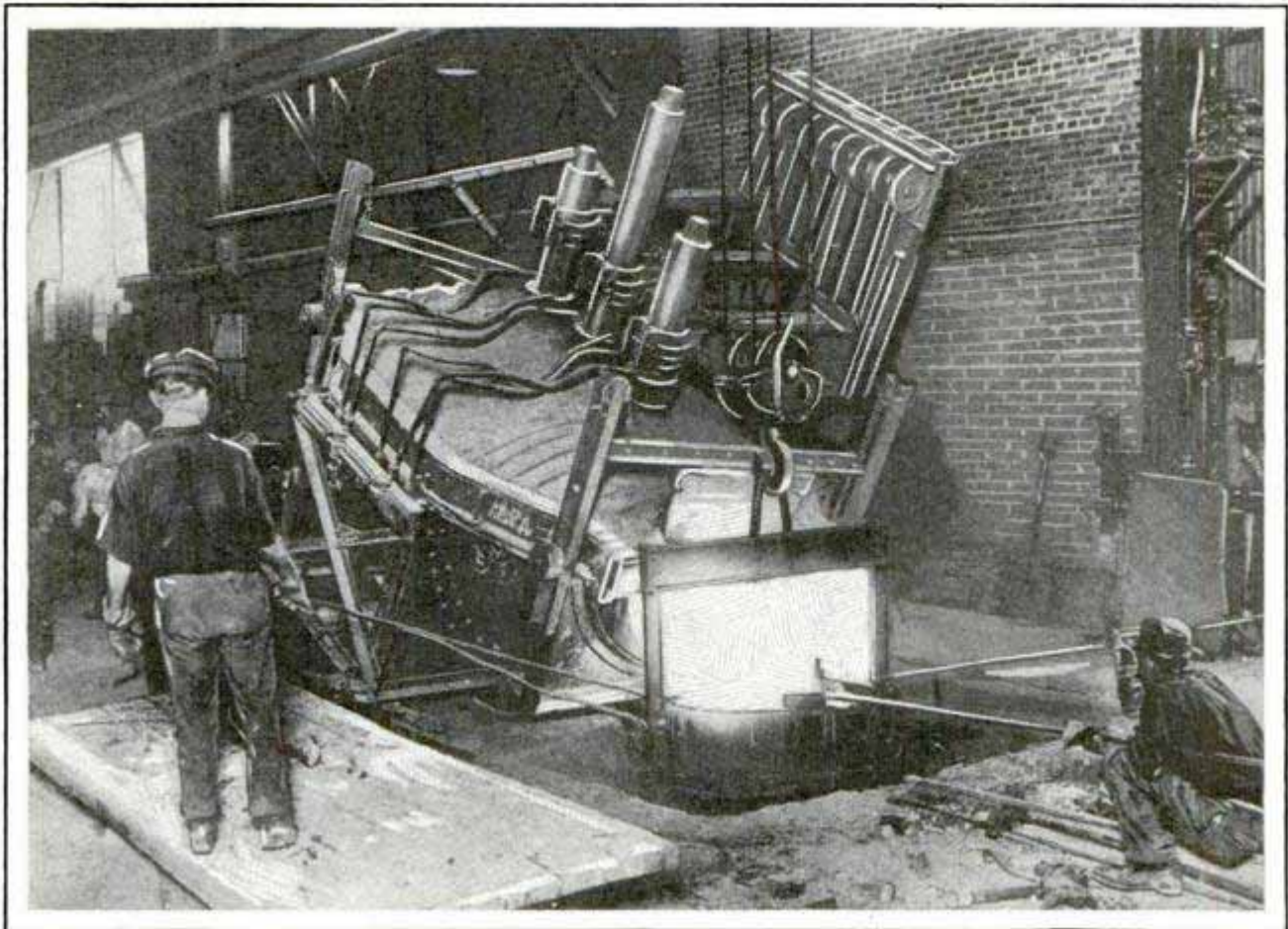
Pouring the Molten Charge from an Electric Steel Furnace; a Large Percentage of All the Energy Generated at Niagara Falls Is Used as Heat in Various Manufacturing Processes
