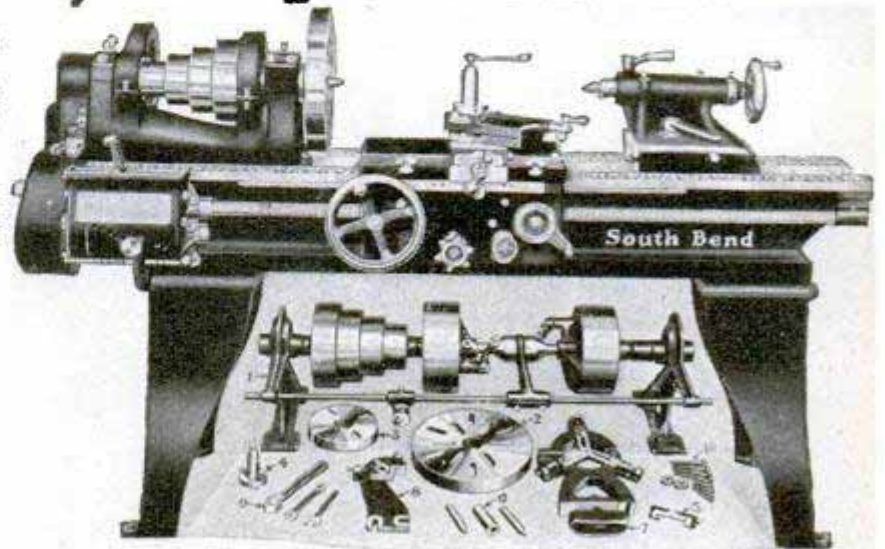
16" x 6' New Model South Bend Quick Change Gear, Back Geared Screw Cutting Lathe - $540
