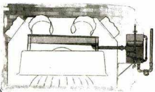
Drawing of the Moistening Outfit Installed in Hot-Air Furnace; Note Supply Chamber at Right
