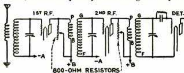
Diagram Showing the Variable Resistors Shunted across the Primaries
