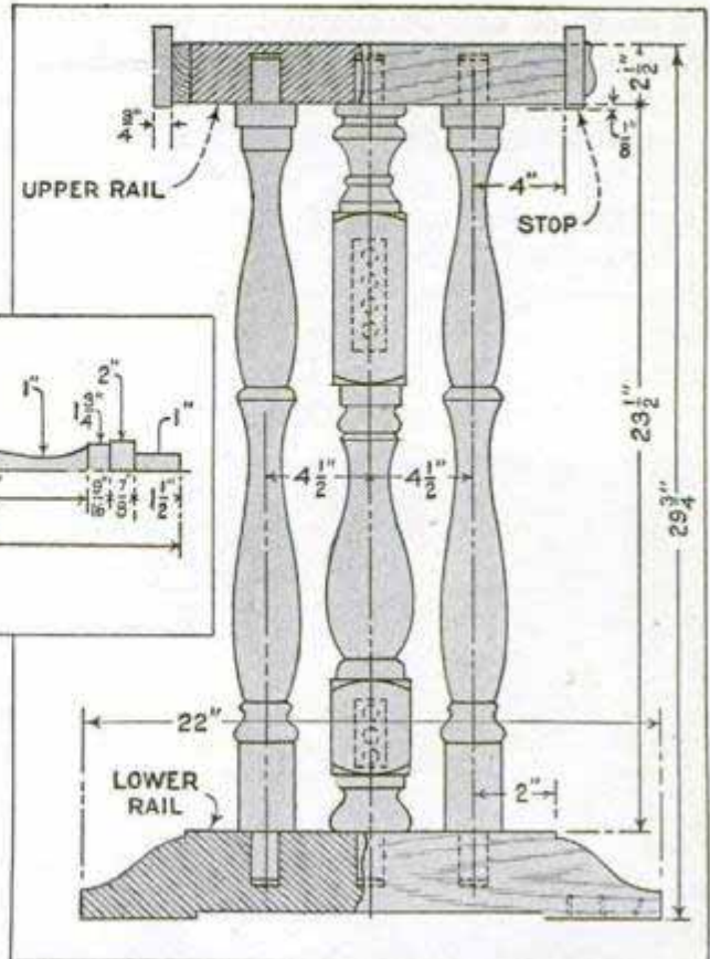
FIG. 2 CORNER SPINDLE, 4 REQUIRED
