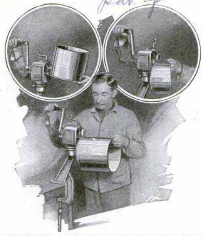
Metal-Working Unit and Three of Its Operations; Note the Inclosed Gears
