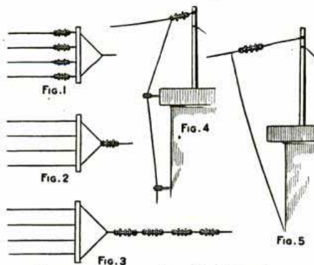
Proper and Improper Use of Aerial Insulators
