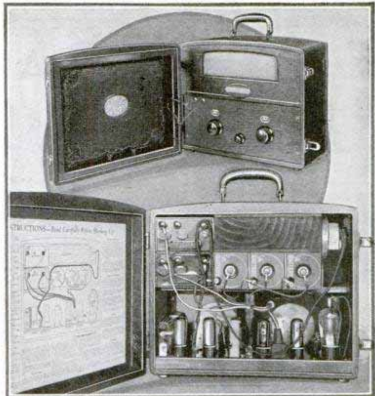
Front View Showing Portable Receiver Ready for Use; Below, Back Opened Showing Arrangement of Tubes and Batteries
