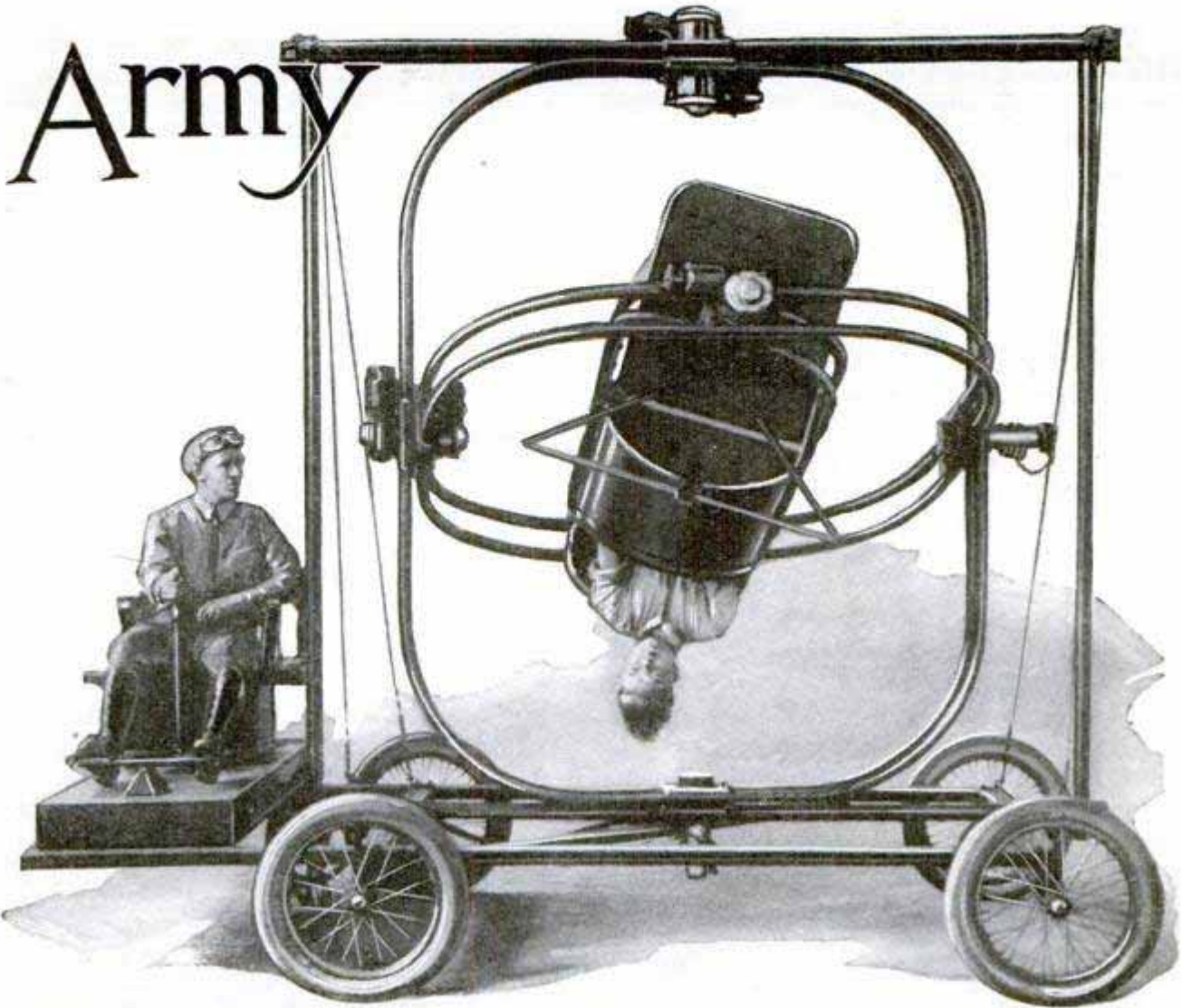
Testing Future Flyers on the Ground; the Pilot of the Ruggles Orientator Has Put the Student in an Upside-Down Position and Is Watching His Efforts to Right the "Ship"
