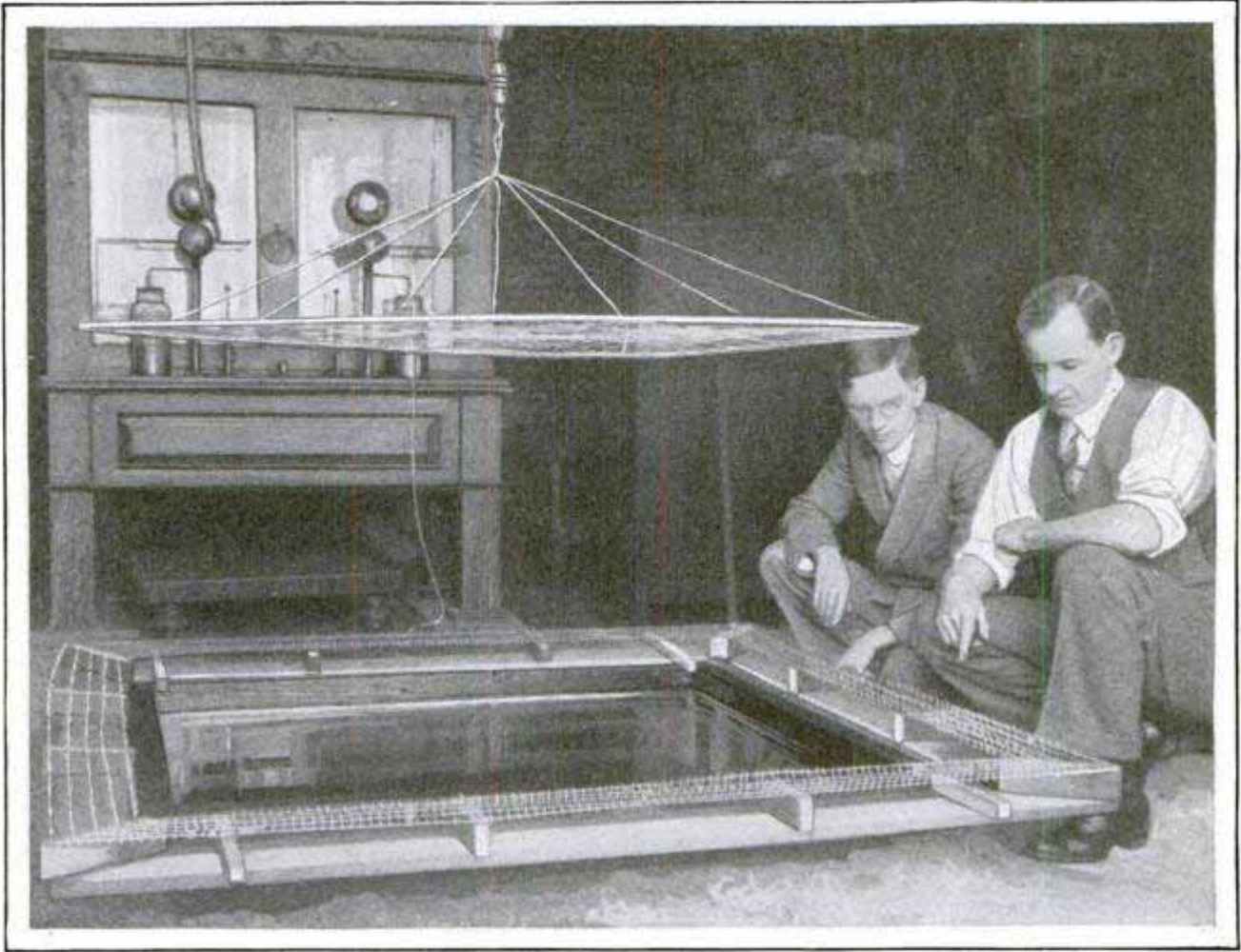
A Variation of the Birdcage Theory Being Tested in a Los Angeles Laboratory as a Means of Protecting Oil-Storage Tanks from Being Fired by Lightning
