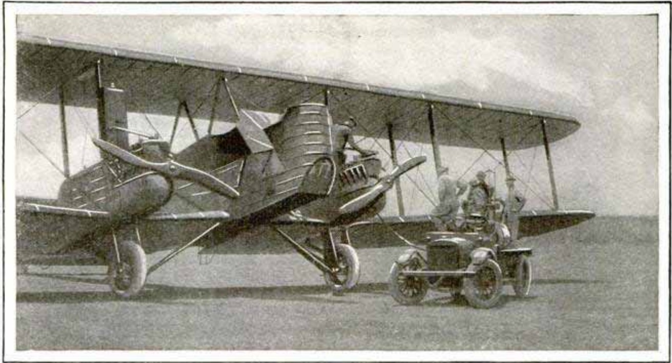
Filling the Gas and Oil Tanks of a Two-Engined Martin Bomber, One of the Biggest Planes the Cadets Learn to Fly; the Cockpit in the Nose Is the Forward Machine-Gun Nest
