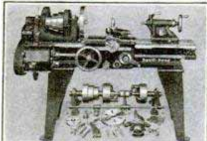
11" x 4' Quick Change Gear Lathe, Straight Bed - - $335
