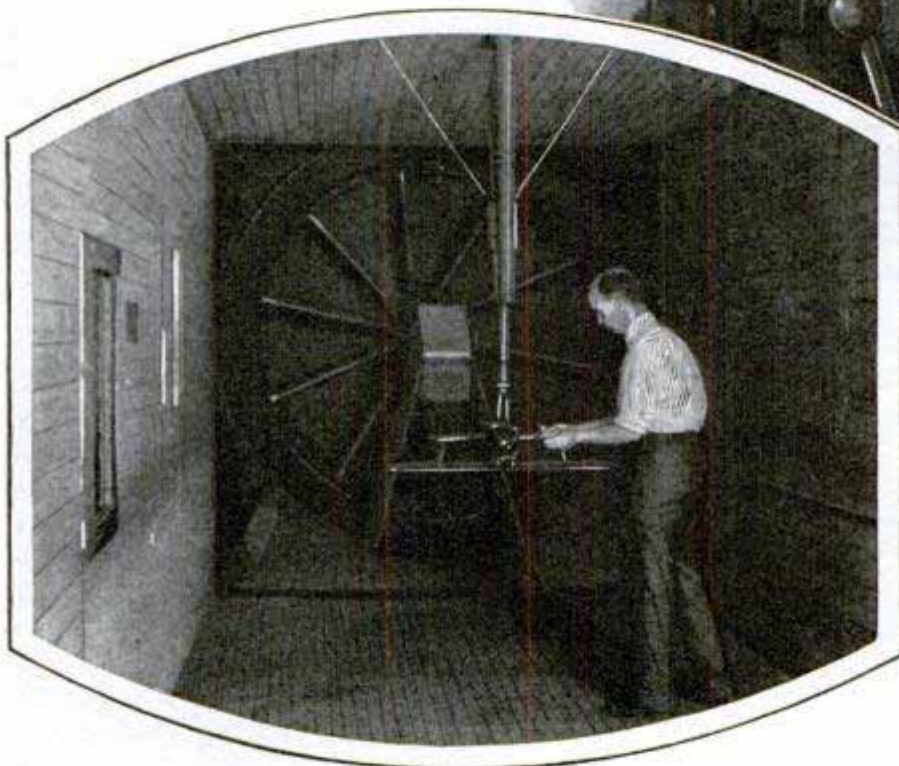
Preparing a Model for Test, Top, and Mounting One in the Wind Tunnel; in the Background Is the Blower
