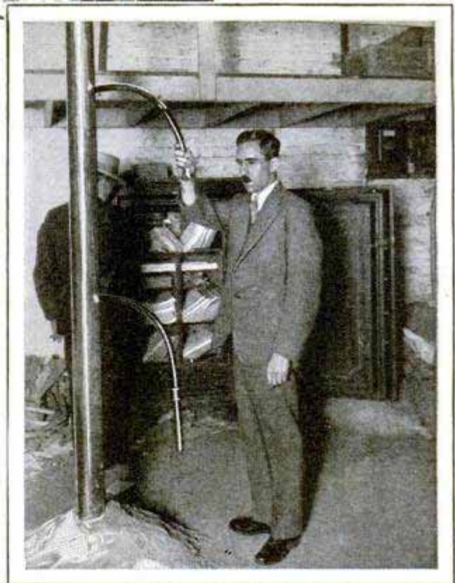
Rigging the Thermocouples, Setting an Alarm Clock in One of the Safes, and, Bottom, the Basement-Debris-Temperature Takers
