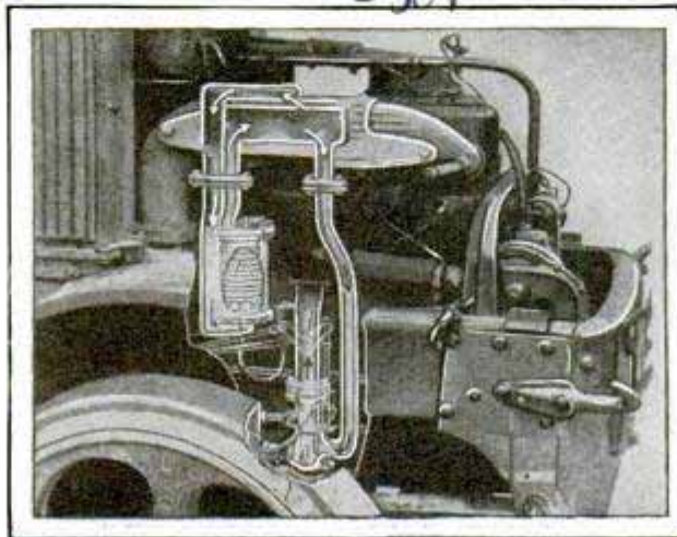
Drawing to Show the Vaporizer Installed
