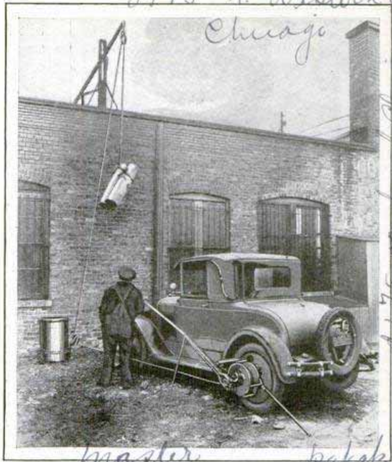
Auto Harnessed as a Hoist; Lowering of the Bucket without Reversal Is Done with the Lever Control
