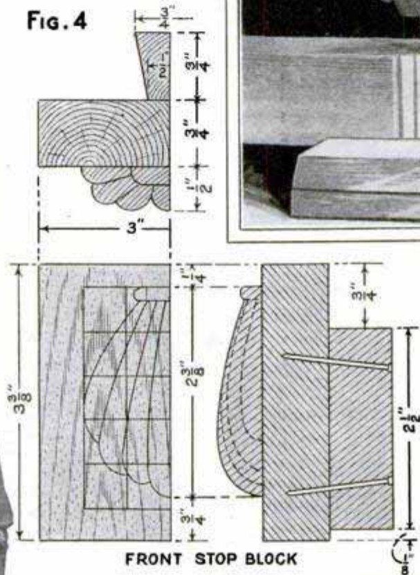
Above, End Veneer Clamped in Vise, Showing the Method of Lacing the Veneer to the Curves for Gluing; Below, Smoothing the Stretcher-Rail Arches with a Half-Round File; Right, Details of the Stop Blocks and the Carved Seashell Ornaments for the Stand Ends; Upper Right, Shaping the Lower Rail Ends, Chipping Out the Waste and Trimming Smooth with a Chisel
