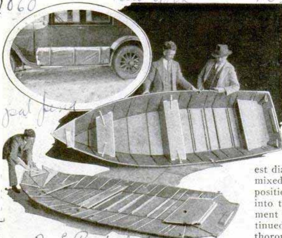
Boat on Auto Running Board, Ready for Use, and Partly Set Up; It Is Made of Mahogany Pieces Joined by Canvas
