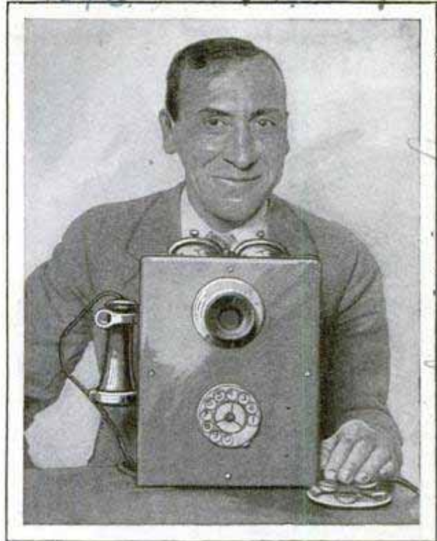
Automatic Telephone Box That Conceals a Motion-Picture Camera for Trapping Criminals
