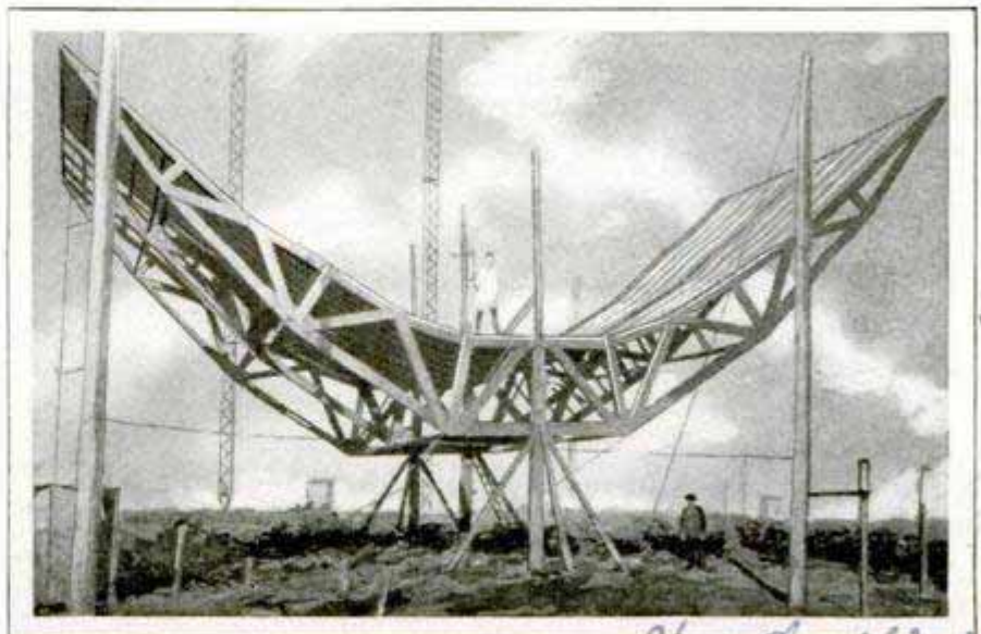
Incline at Radio Station in Germany, Where Experiments Are Being Made in Directing and Focusing Wireless Waves
