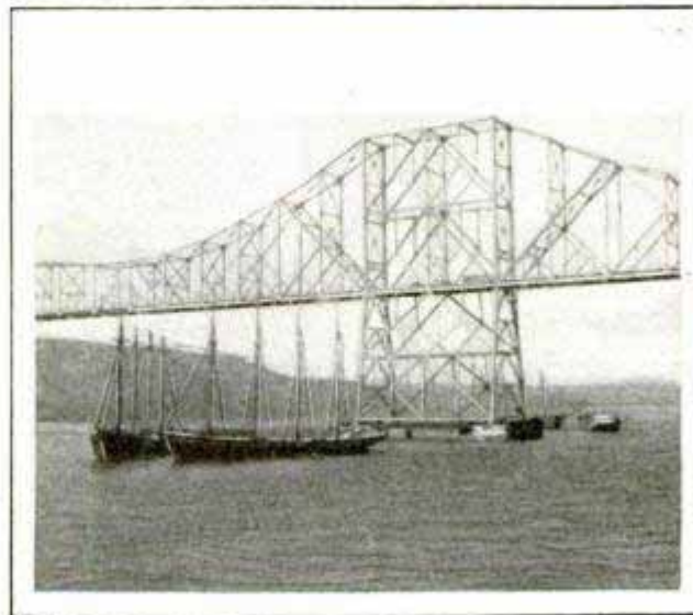
Old Wooden Ships Guarding the Central Pier of Big Steel Bridge from Damage by Collisions
