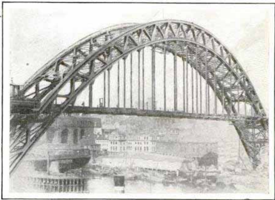
Long Span of the Tyne Bridge between Newcastle and Gateshead, England; the Structure Cost Nearly $5,000,000 824
