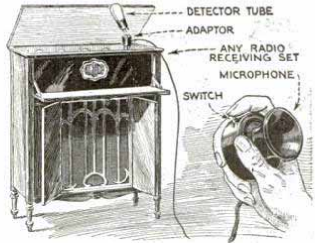
Microphone, Showing the Adapter Inserted in the Detector Socket of the Set
