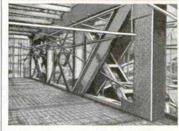
Details of Truss Bracing, and Model Showing How Japanese Builders Are Fortifying against Quakes
