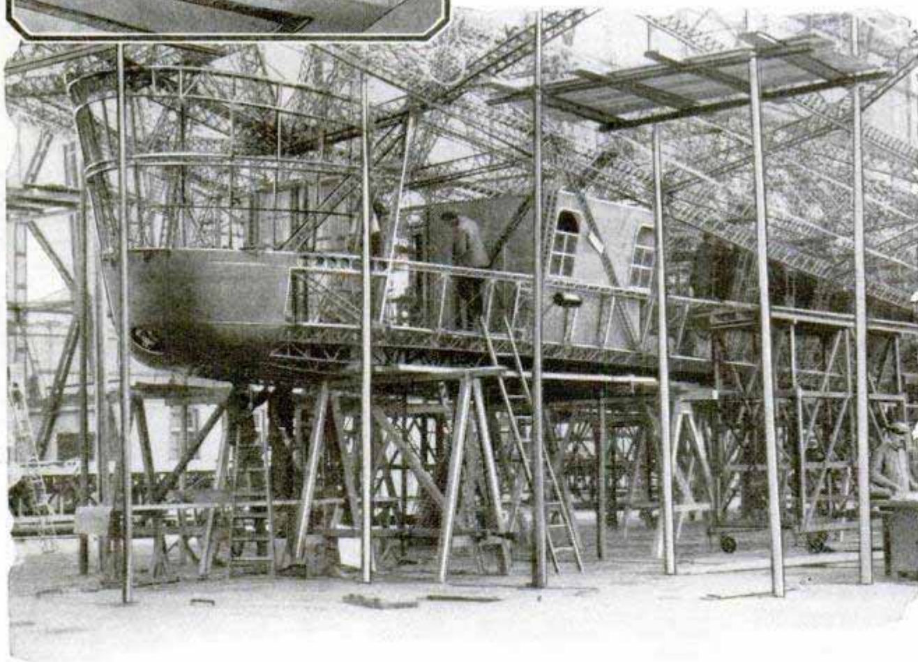
One of the Staterooms of the "LZ-127" and the Passenger and Control Gondola under Construction; the Walls in the Center Inclose the Radio Operator's Compartment
