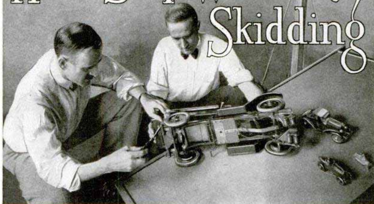
Tuning Up Midget Models for Spins down an Inclined Plane; the Bureau of Standards in This Way Studied the Cause and Effects of Skids and Discovered the Remedies
