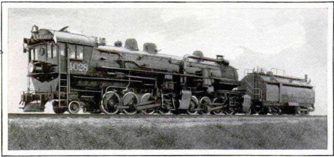
Remodeled Locomotive, with the Cab in Front for Easier Control of the Engine, Weighs 322 Tons and Is More Than 104 Feet Long
