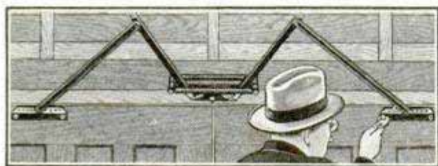
Close View of the Gear Control for Garage Doors, Showing Method of Installation
