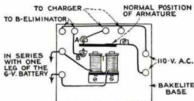
Layout and Wiring Diagram for Control Relay
