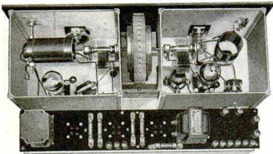
Completed Receiver with Tops of the Compartment Shields Removed, Showing the Screen-Grid and Detector Tubes in Position, and at the Right, Schematic Diagram of the Circuit
