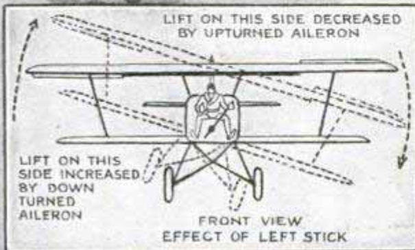
THE EFFECTS OF AILERONS
