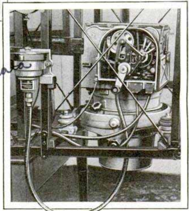
Single Exposure of a Hundred Square Miles of Ohio, Made with a New Five-Lens Mapping Camera, Above, and, at the Right, a New Electric Mapping Camera Which Is Used in England
