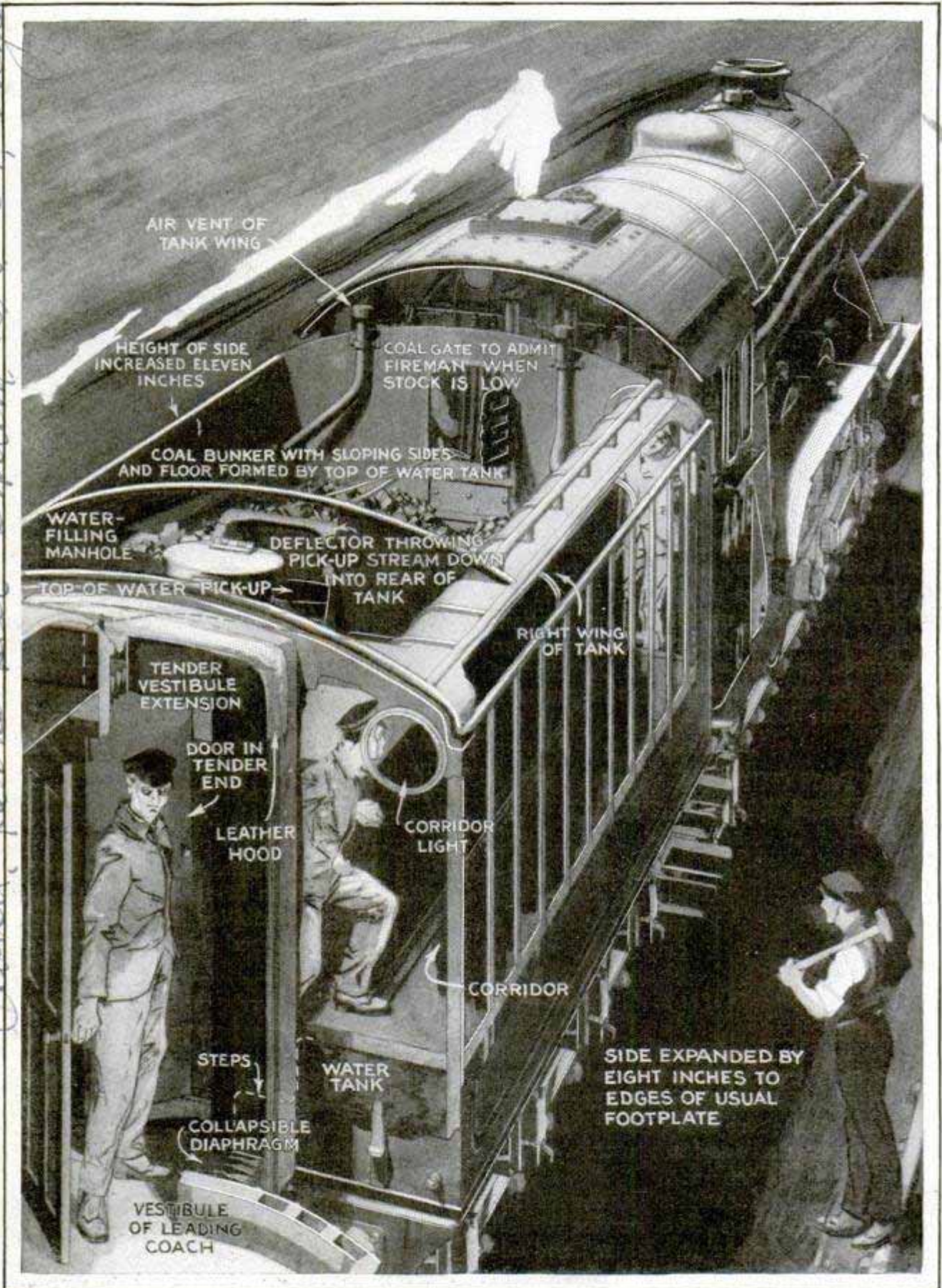
The Famous "Flying Scotsman," Which Runs from London to Edinburgh, Now Makes a 392-Mile Non-Stop Run between the Two Cities; Crews Are Changed Midway by Means of a Corridor through the Tender, the Spare Crew Riding as Passengers in a Baggage-Car Compartment
