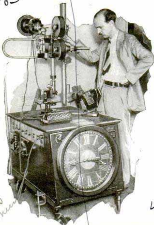
Combination Motion-Picture Camera and Microscope Operated by Clockwork for Filming Germ Life
