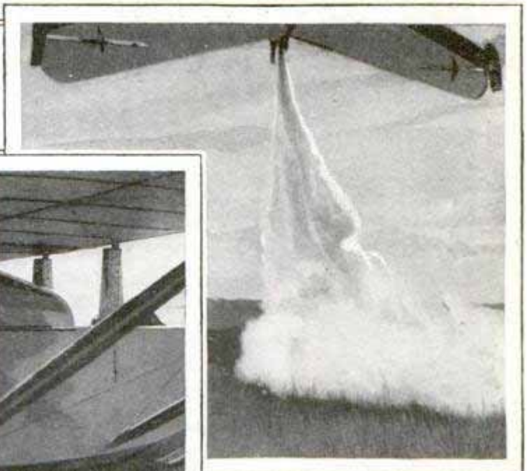
New Opel Rocket Plane in Full Flight, and, Below, the Rear of the Fuselage, Which Carries Its Tail in Front; the Arched Shield Protects the Pilot from Heat and Possible Premature Explosion of the Rockets
