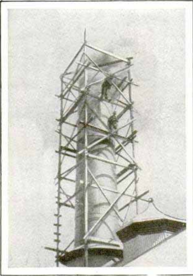
Adding Section to Big Smokestack While Fires Burned Below; Workmen Completing Second Half of a Joint
