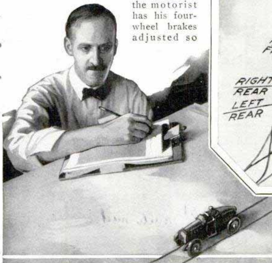
Above, with Rear Wheels Locked on a Steep Grade, the Model Skids and Comes to a Stop Facing in the Opposite Direction, Whereas, with the Braking Force Mostly on the Front Wheels and the Rear Ones Free to Revolve, It Continues in a Straight Line Until It Stops
