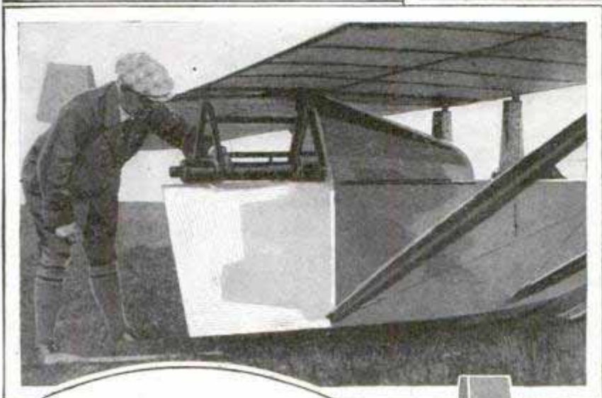
New Opel Rocket Plane in Full Flight, and, Below, the Rear of the Fuselage, Which Carries Its Tail in Front; the Arched Shield Protects the Pilot from Heat and Possible Premature Explosion of the Rockets
