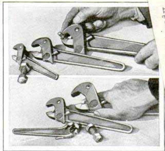
Three Wrenches Equal to Thirty; the Different Sizes and Method of Adjusting to Fit the Nut
