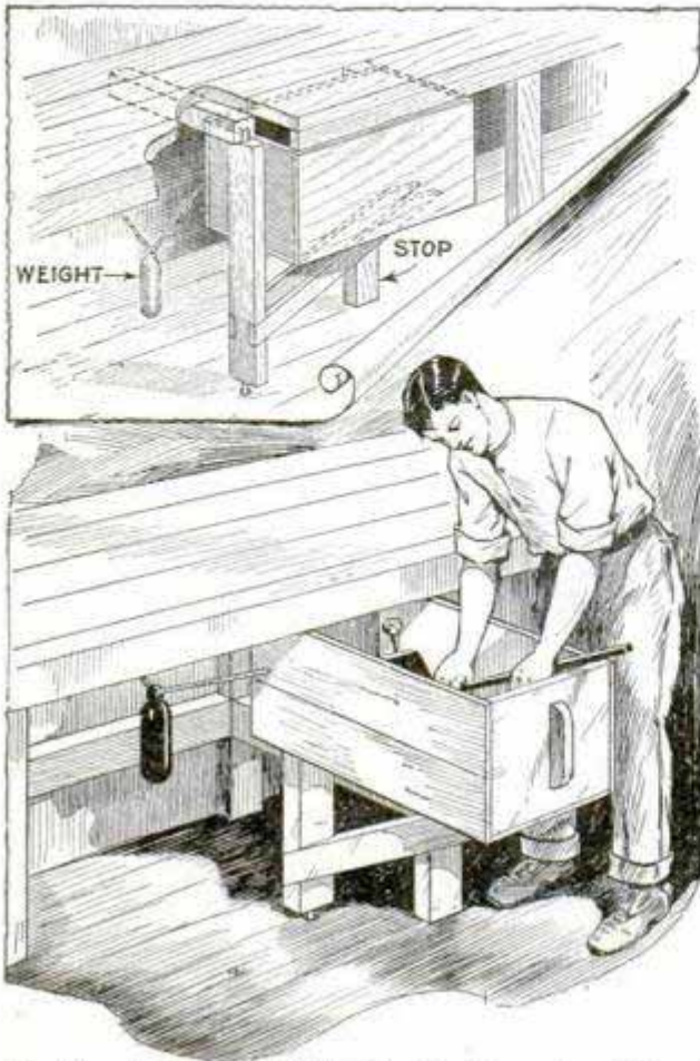
Workbench Drawer Which Can Be Opened and Closed Easily, No Matter How Heavily Loaded
