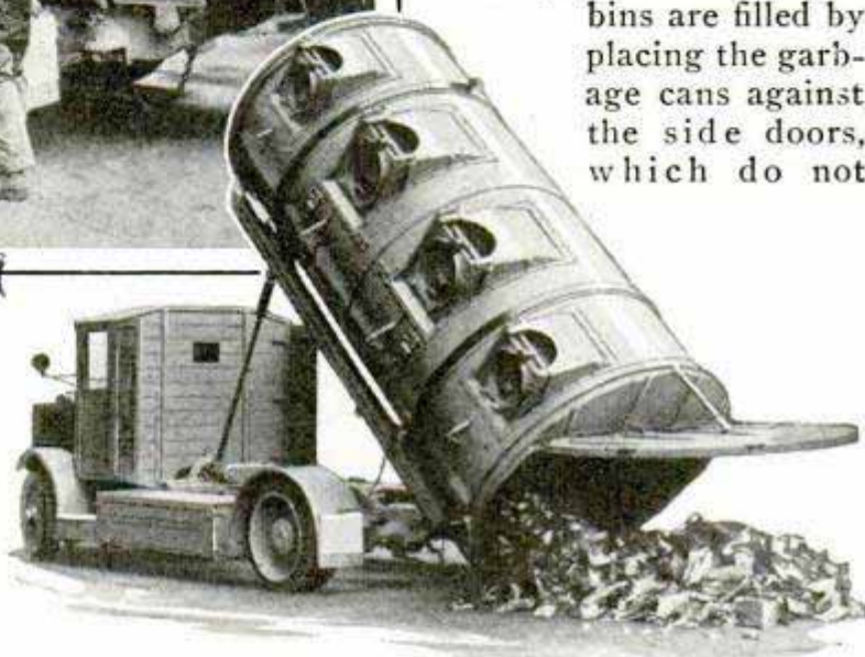
Filling the Garbage Truck through the Side Doors and Emptying a Load; the Tank Is Elevated by Hydraulic Mechanism
