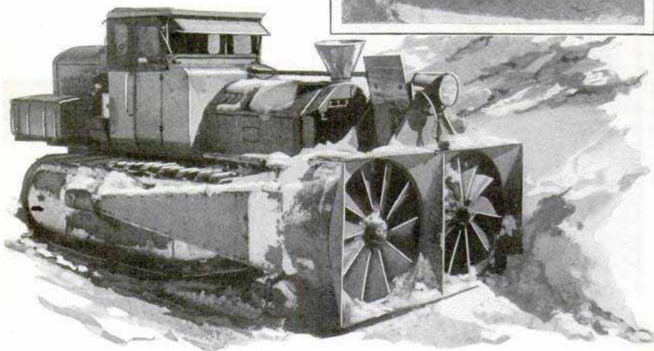
Huge Road-Clearing Rig to Combat Snowdrifts in the Alps; It Has Two Fifty-Horsepower Motors and Can Be Operated in Difficult Places with Endless-Tread Drive
