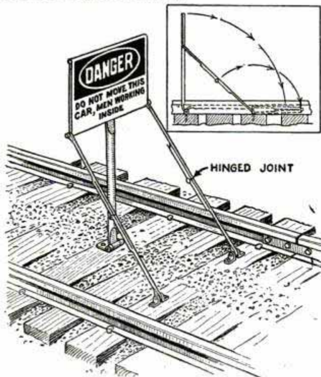
Collapsible Stop Sign on Railroad Sidings Is Always Ready for Use
