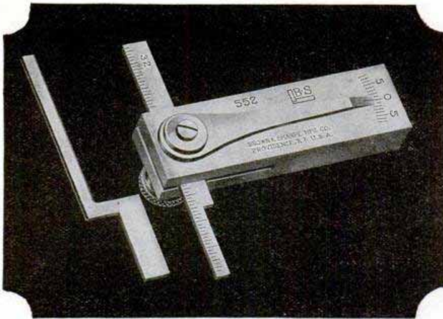
Die Makers' Square No. 552 is a typical Brown & Sharpe Tool made to do the specialized work of the die maker and pattern maker.
