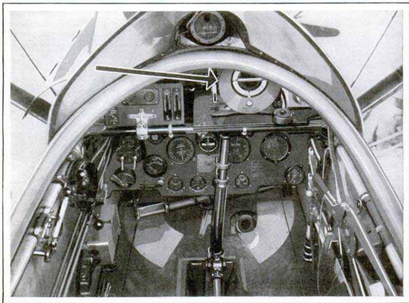
Cockpit of a Douglas Transport Plane; the Arrow Points to a German Bank-and-Turn Indicator Loaned the U. S. Government in Exchange for Avigation Information from This Country
