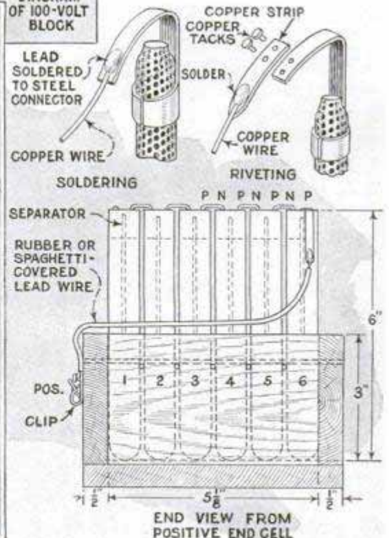
Upper Left, Sectional Diagram of the 100-Volt Block, Showing the Cell Arrangement; Bottom, Left, Two Completed Cells with Positive and Negative Elements and Separators between Them; Right, Sectional View from Positive End Cell; Above, Methods of Connecting Lead Wire to Elements
