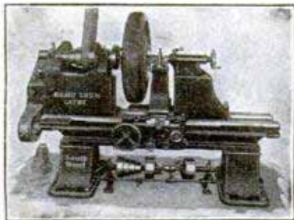
Brake Drum Lathe Handles all Brake Drum work without removing tire or rim, up to 33" diameter..... $425
