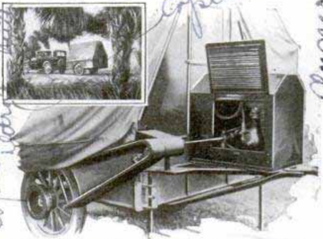
Trailer and Car on Journey, and Method of Connecting Ice Machine to the Axle
