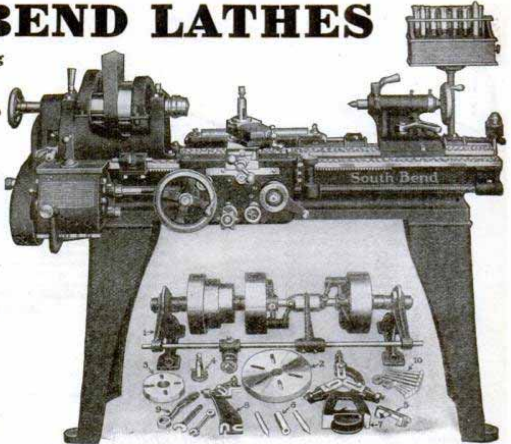
11" x 4' New Model Precision Tool Room Lathe with Counter-shaft and Regular Equipment..... $335
