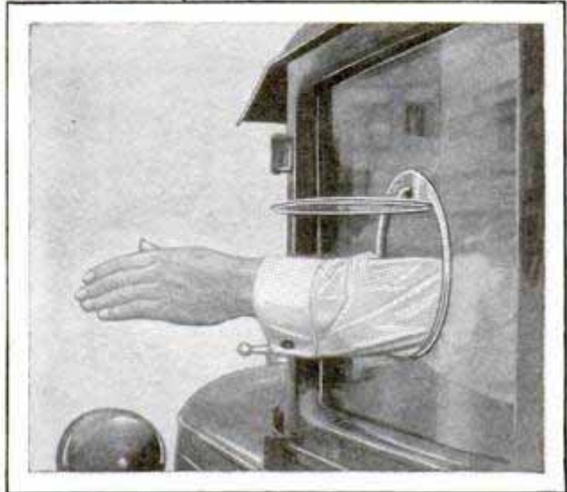
Hinged Section in Auto Door for Making Arm Signals; Opening Also Is Aid to Ventilation
