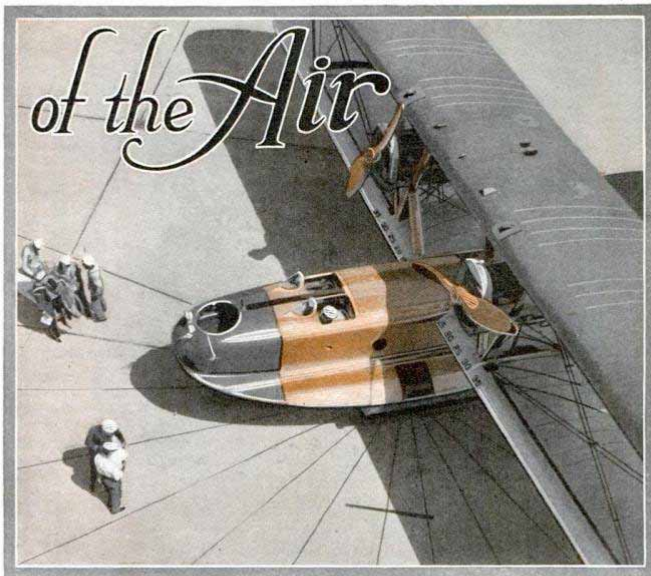
Swinging Ship to Correct the Compass of a Huge Twin-Motored Flying Boat; Note the Compass Points Laid Out in Radiating Lines on the Concrete Base to Guide the Correctors
