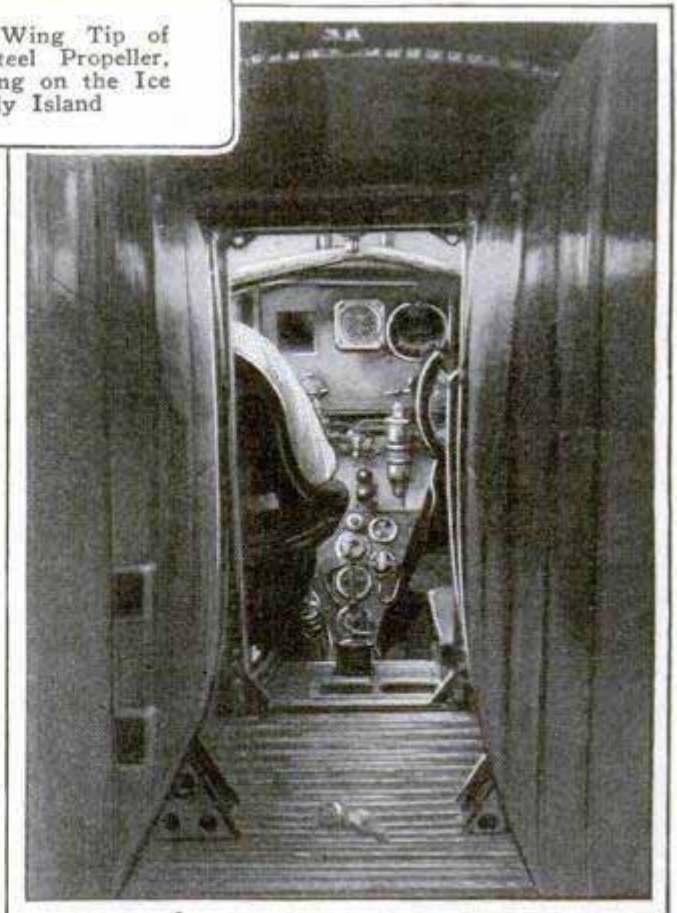
Looking Forward past the Huge Gasoline Tanks Built into the Cabin Walls; the Two Pilots Rode Side by Side at Dual Controls
