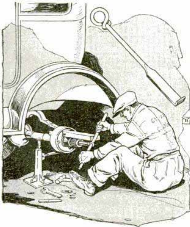
Roller Bearings on Ford Axles Can Readily Be Removed with This Simple Tool
