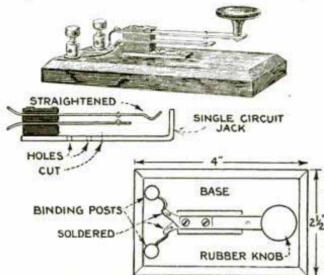
Above, Sketch Showing Completed Key; Below, Construction Details and Top View of Assembly
