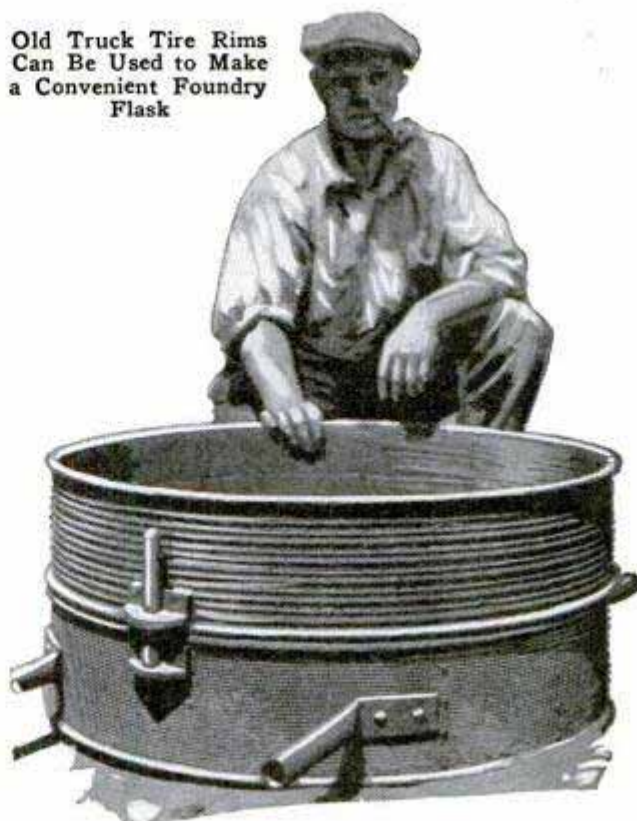
Handy Foundry Flask Made from Tire Rims
