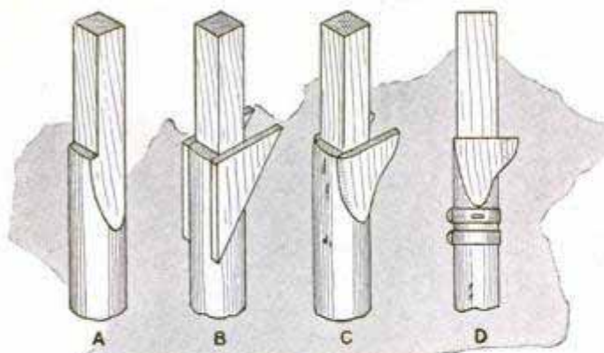
SQUARING LOWER MASTHEADS AND FITTING CHEEKS
