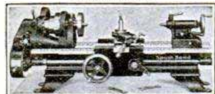
9" x 2 1/2' Junior Back Geared, $150 Screw Cutting Bench Lathe... Shown complete in Booklet 22K
