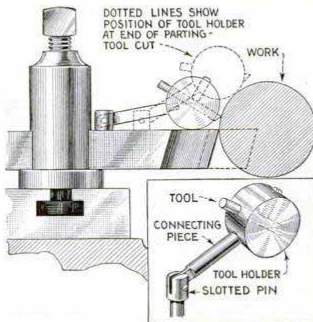
Automatic Chamfering Attachment on the Parting Tool, Useful in Absence of Double Toolpost
