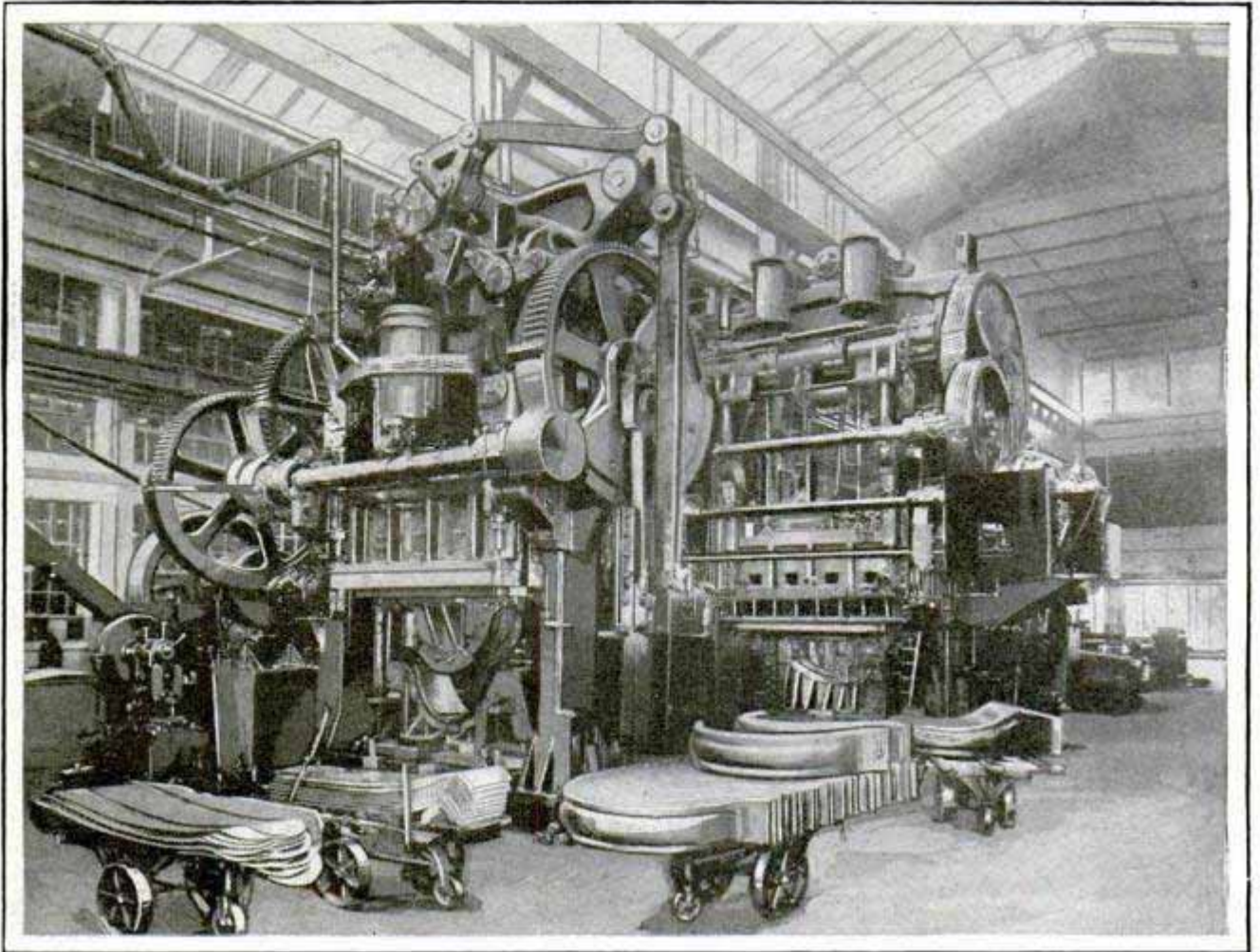
Fender Press in a Detroit Automobile Factory, Which Takes Flat Sheets of Steel and Presses Them into the Intricate Shapes of Full-Crowned Auto Mudguards
