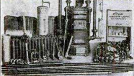
Complete Hot Water Heating Plant ready for shipment with set of installing tools, diagrams, and New Easy Method of self-installing instructions.
