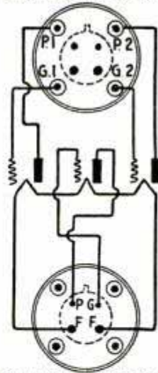
BOTTOM PIN CONNECTIONS
