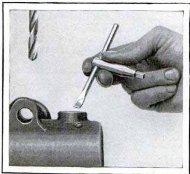
Handle of Lathe Chuck Wrench Ground Down to Spoon Shape Adds to Its Usefulness
