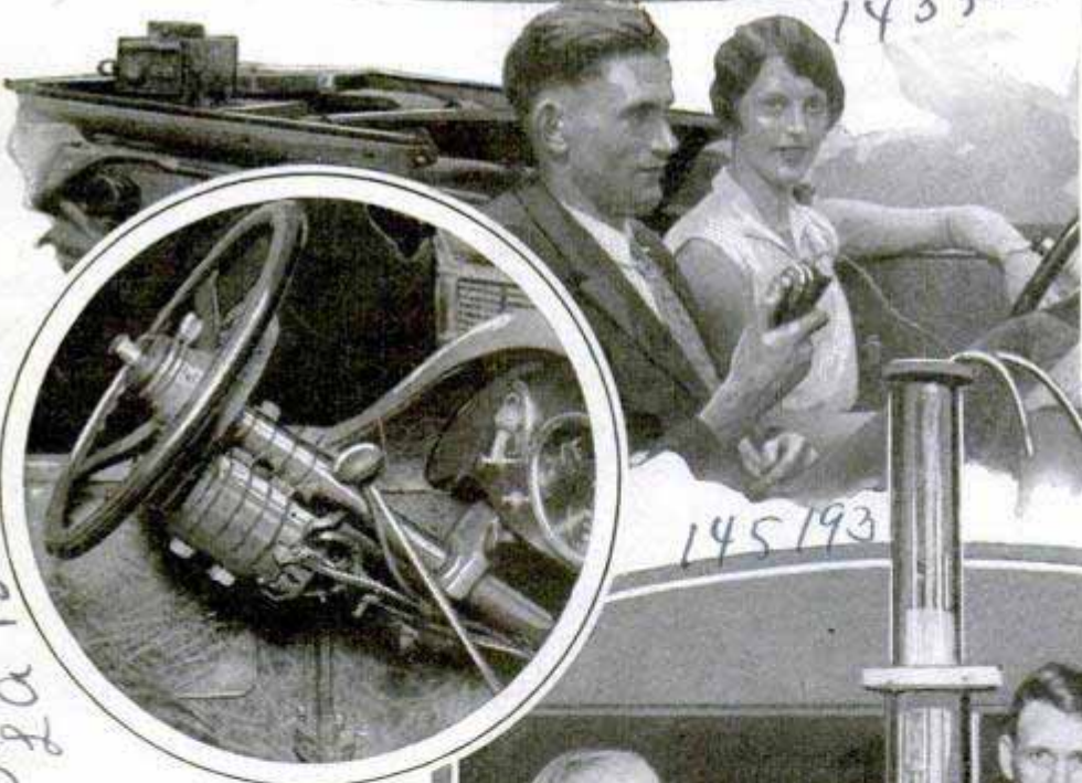
Above, R. L. Mack, Former Naval Radio Operator, Directing a Driverless Car by Means of Radio Control; the Inventor Claims the Control Mechanism is Adaptable to Any Car; Insert, Close-Up of Steering-Column Mechanism in a Second Car, Actuated by Remote Control; at Right, Comparing the New 100-Kilowatt Transmitting Tube with One of the Old Types; These Tubes Were Exhibited at the New York Radio Show
