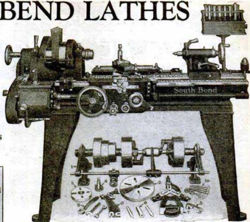
11" x 4' New Model Precision Tool Room Lathe with Countershaft and $335 Regular Equipment..... One of the types illustrated in Special Booklet No. 11
