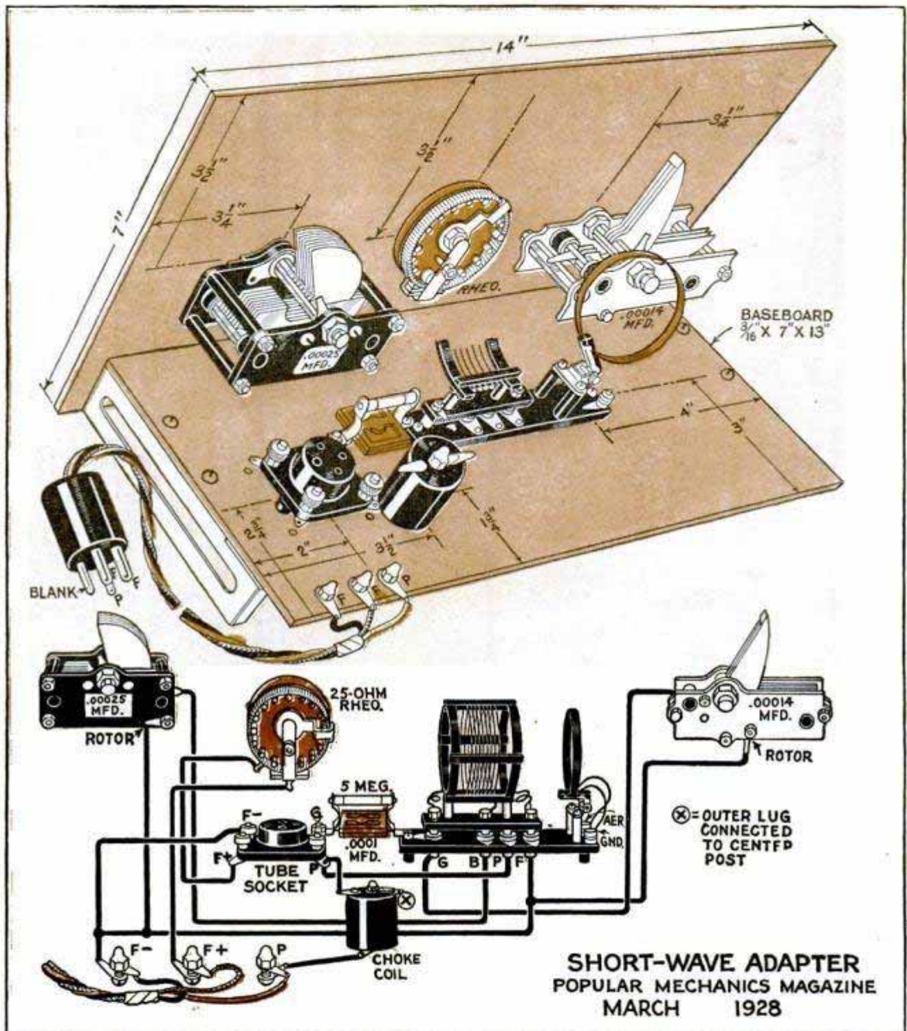
Above, Front and Subpanel Layouts, Showing Instruments in Position; Below, Simplified Wiring Diagram, Showing Original Instrument Layout with Point to Point Connections
