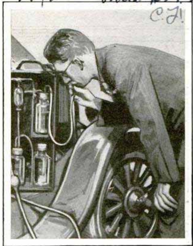
Testing Auto's Exhaust Fumes, to Determine if the Carburetor Has Been Adjusted Properly
