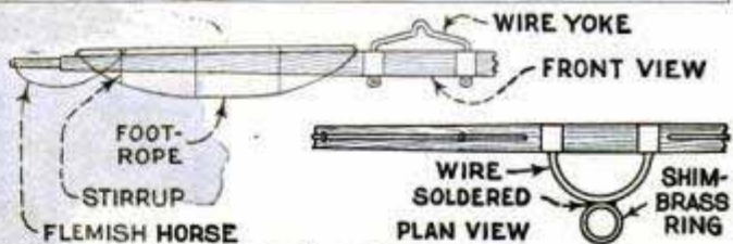
TOPS'-WARD DETAIL Fig. 95
