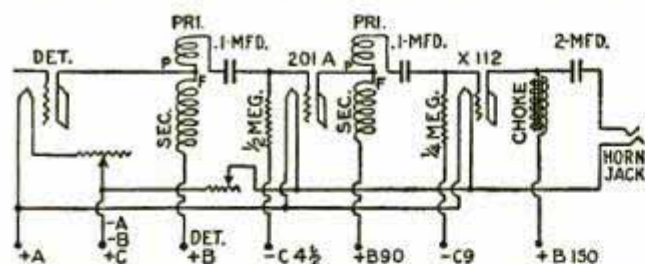
Diagram Showing Completed Audio Changes and Speaker Filter
