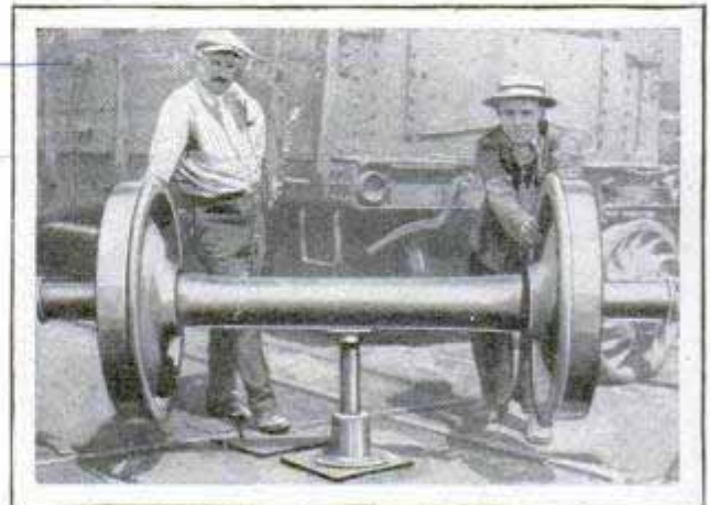
Air-Operated Jack Which Raises Car Wheels So They Can Be Shifted to Different Tracks
