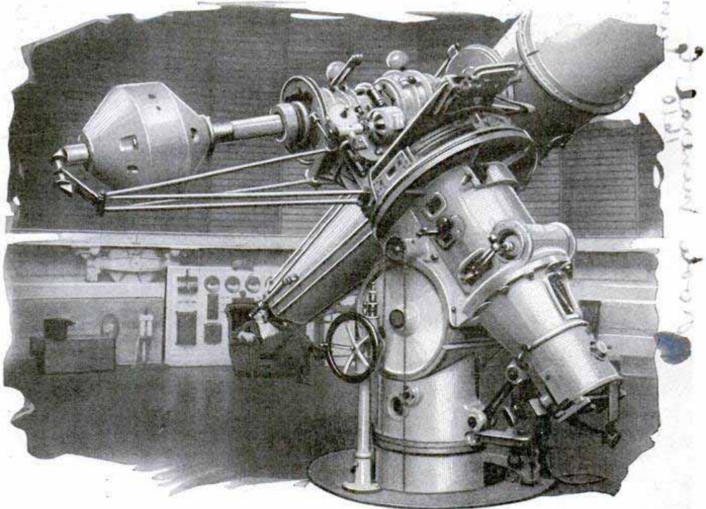
Seated in His Comfortable Armchair, This German Astronomer Views the Heavens through His Giant Telescope, Moving the Ponderous Mass at Will with the Controls behind Him
