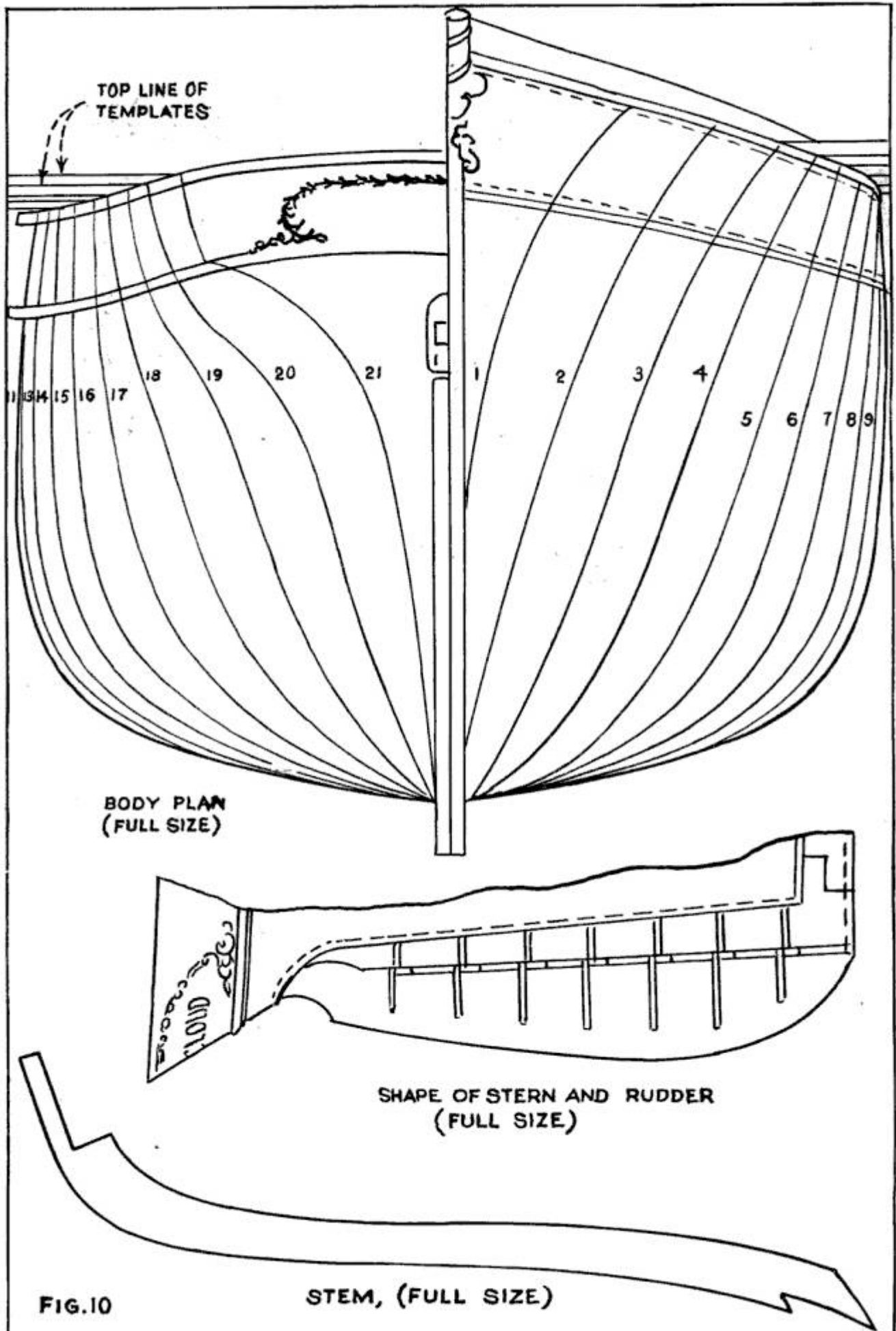
Full-Size Drawings for Making Body Molds, Stem and Stern Templates
