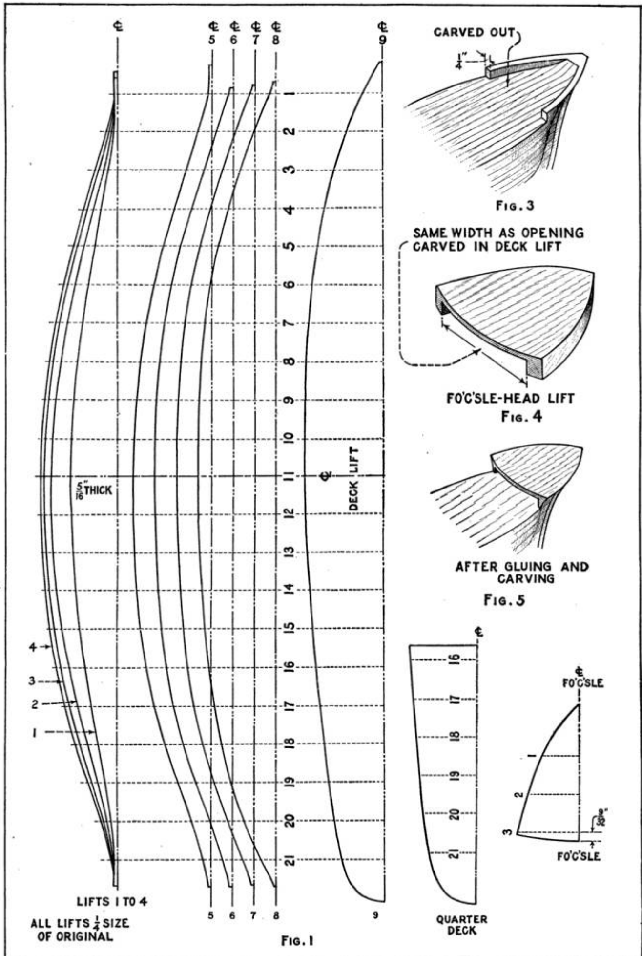
Quarter-Size Drawings for Making Hull, Deck, Quarterdeck and Fo'c'sle Templates
