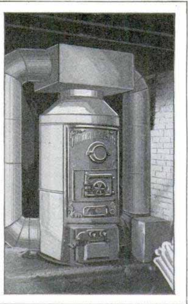
Left, How the Pipe Collars on the Dome Are Closed by Pieces of Sheet Iron; Right, Completed Installation, Showing the Pipes That Return the Air for Reheating
