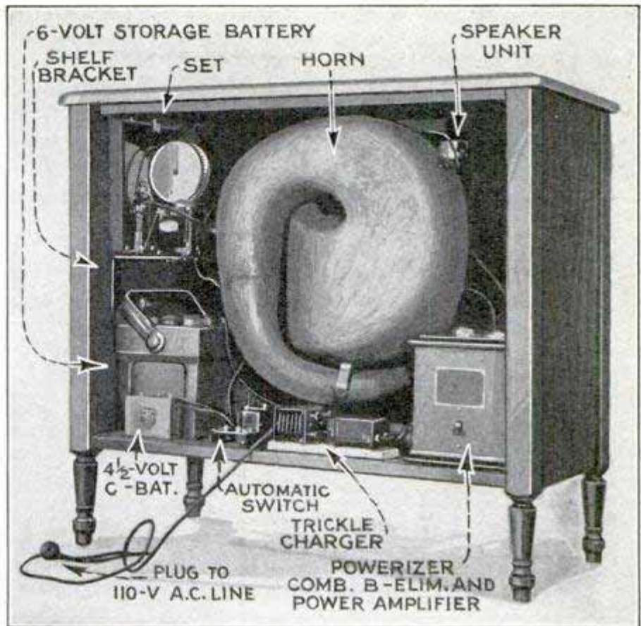
View of Cabinet Speaker with Back Removed, Showing the Location of the Various Instruments
