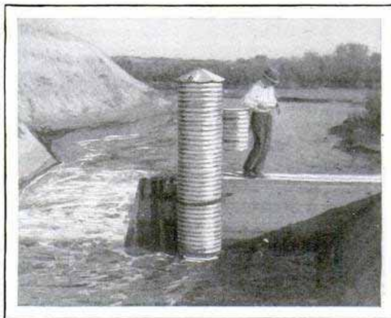
Water-Stage Recorder Mounted in a Section of Old Culvert Pipe
