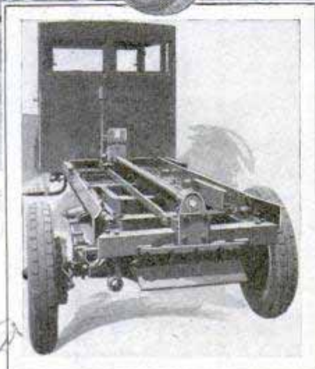
Sliding Body from the Auto Truck for Easy Unloading, and Rear View Showing the Gear That Moves the Body
