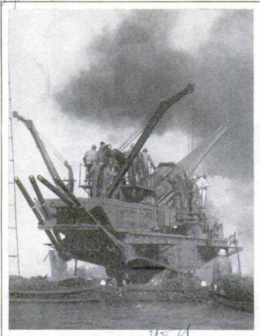
Big Coast-Defense Rifle in Action during Marksmanship Test; the Gun Is Mounted on Railway Carriage for Easy Transportation
