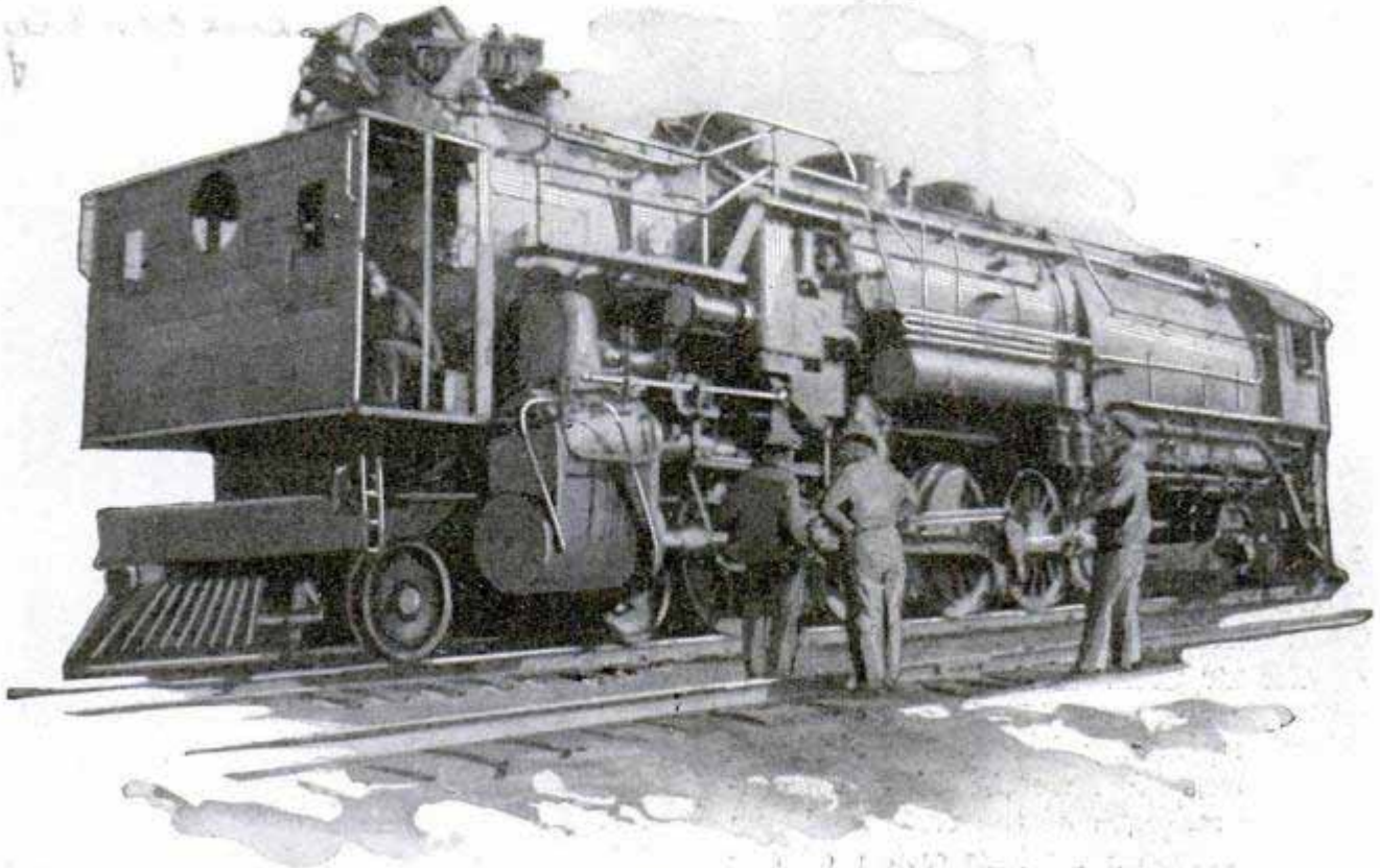
Testing Apparatus, Installed in Booth on Front of Engine, Enabled Mechanics to Obtain a Complete and Accurate Record of the Locomotive's Performance on Trial Run.
