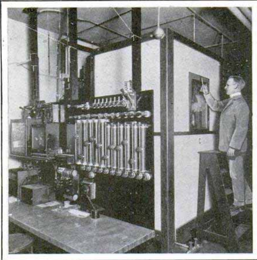
In This Air-Tight Chamber, the Body Heat and Energy Developed by Measured Amounts of Food Products Are Determined
