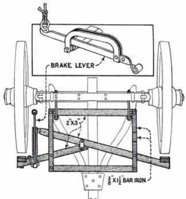
Homemade Brake for Heavy Wagons Which Has Been Found Very Effective
