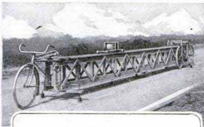
Two Types of Meters That Register the Bumps in Cement Pavings, and, at Right, Illustration of the Familiar Straightedge for the Same Purpose
