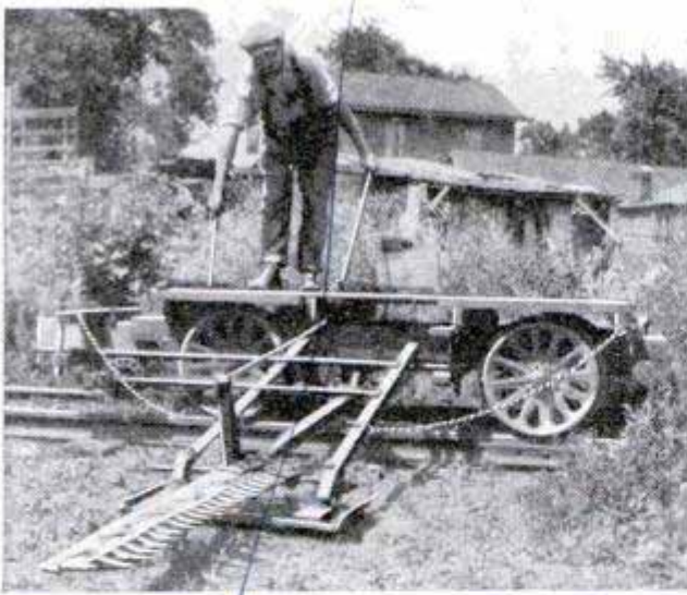
Mowing Weeds along Railroad Tracks with Push-Car Cutter, Made by Foreman at Little Expense
