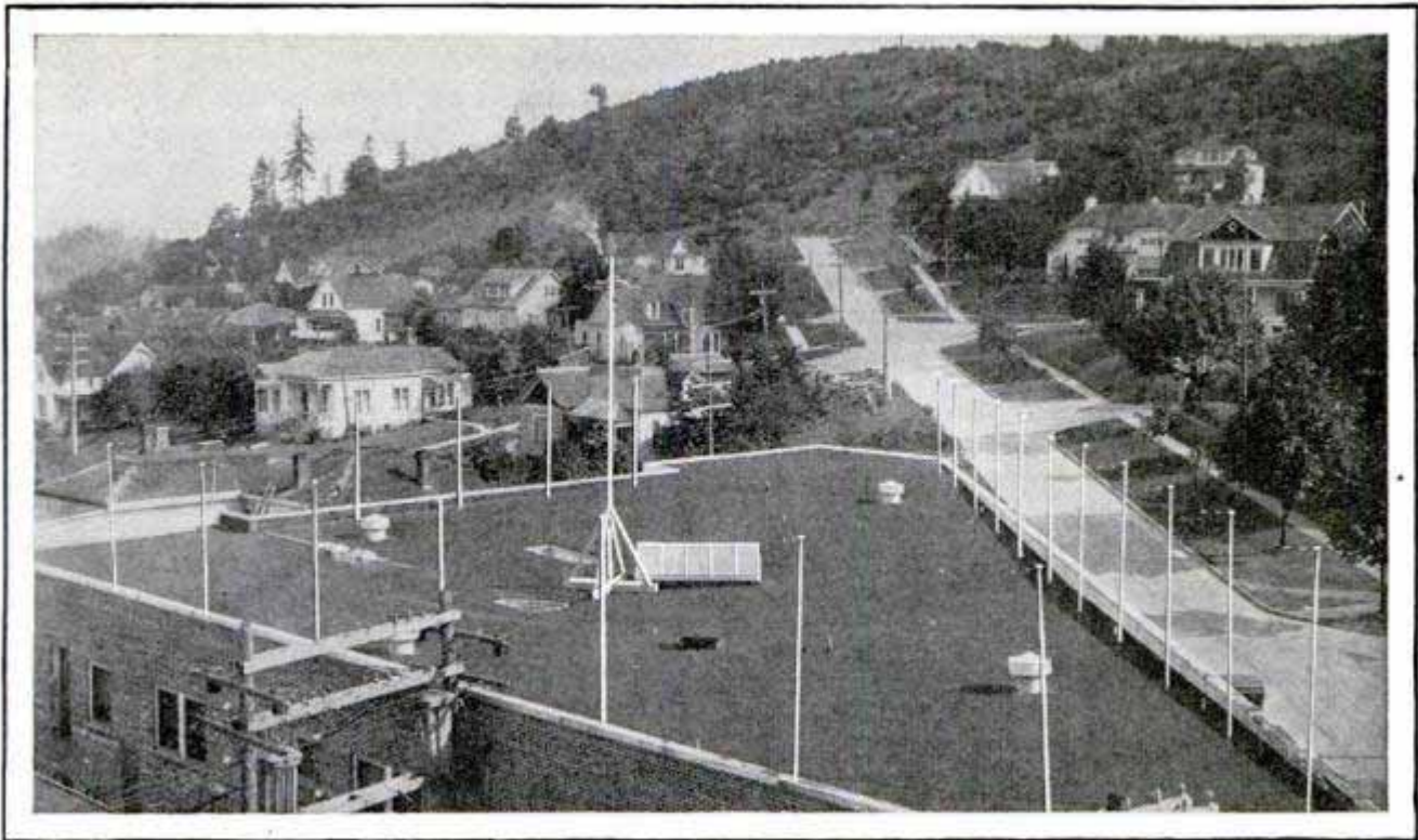
Washington Apartment House Has a Neat Installation for 32 Aerials, Consisting of a Large Central Mast and a Number of Small Masts
