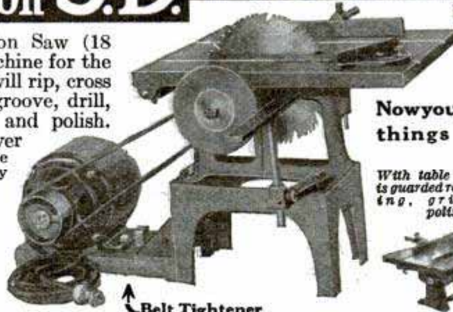
↑ Belt Tightener
