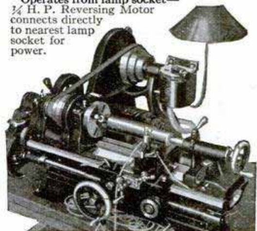
9" x 2 1/2" New Model Junior Self-Contained Motor-Driven Bench Lathe, complete as shown .....$228
