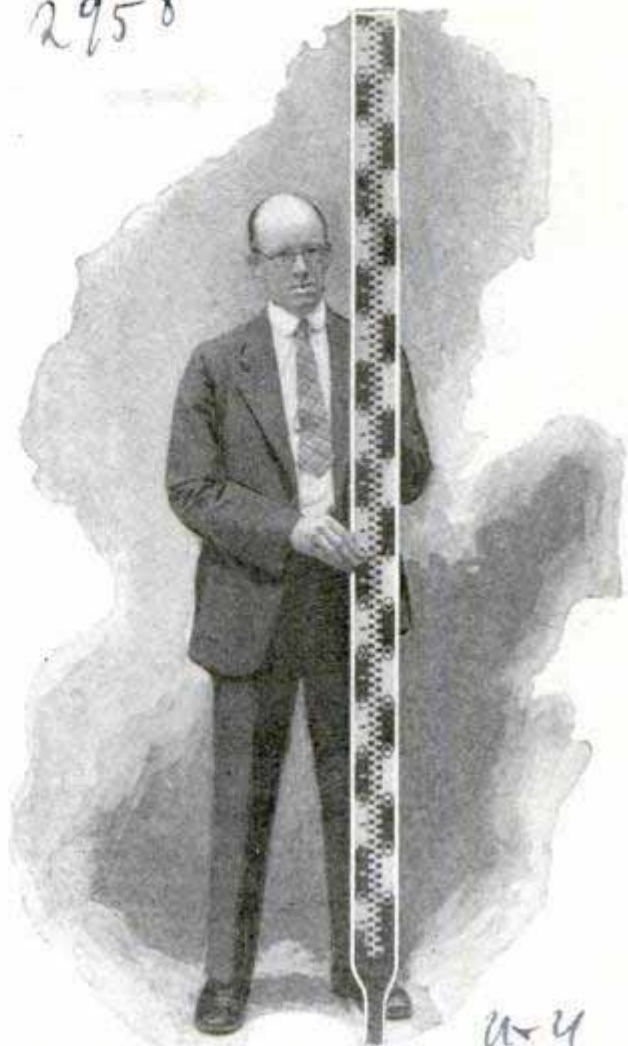
For Accuracy in Surveys; Rod Is Little Affected by Temperature Changes and Has Thermometer
