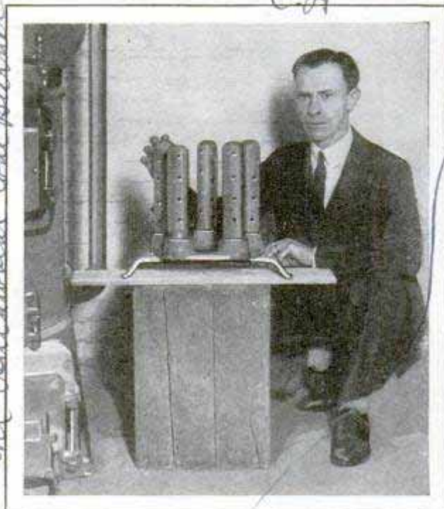
Air Tubes for the Furnace, to Permit Burning of Small-Size Coal; They Increase Oxygen Supply
