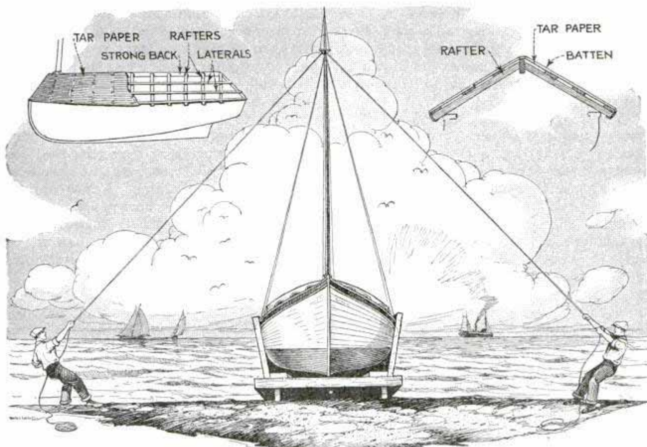
How Sailboats Are Kept Upright When Shoring Them; Details Show Method of Covering the Boat with Tar Paper in Order to Keep Out the Rain and Snow
