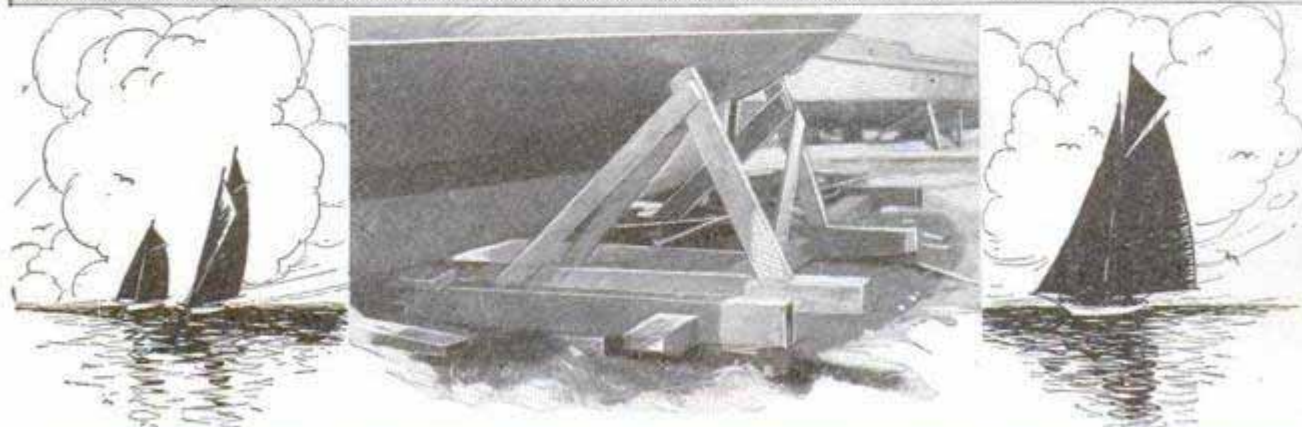
Top, This Boat Is Well Covered with Canvas; Center, Details of the Cradle and Way Used to Haul the Boat; Bottom, One Method of Cradling a Boat, Showing Props, Braces and Cross Bearers
