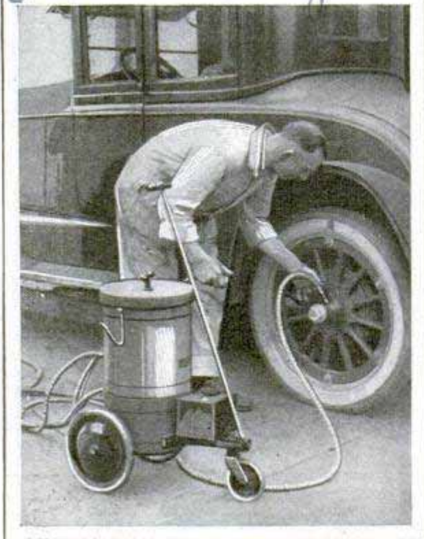
Greasing the Car with the Gun; Compressed Air from the Tank Forces Lubricant into Parts
