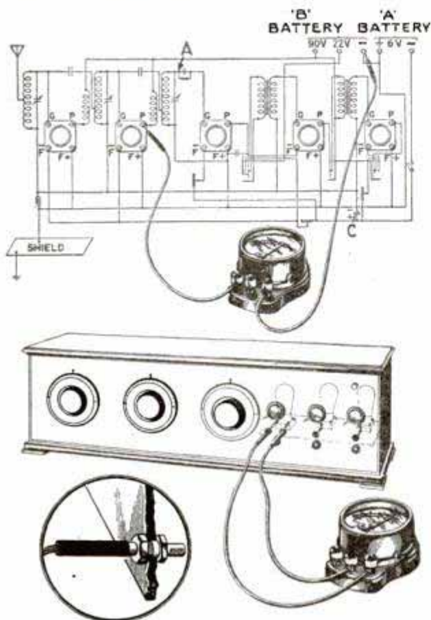
Suggested Tests Obtained with Dual-Range Voltmeter
