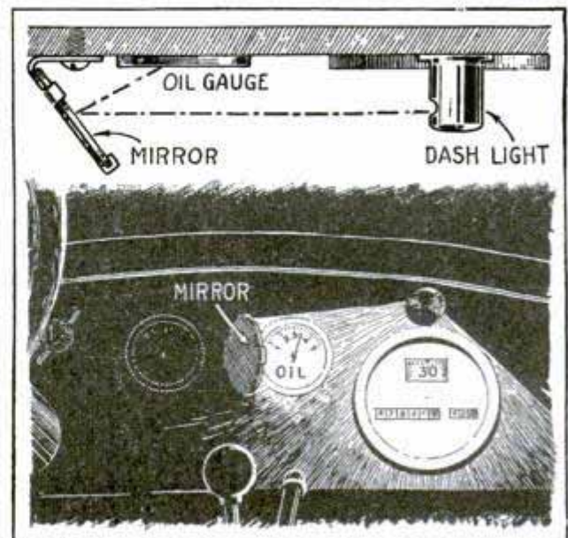
Reflector to Illuminate the Oil Indicator on the Auto Instrument Board
