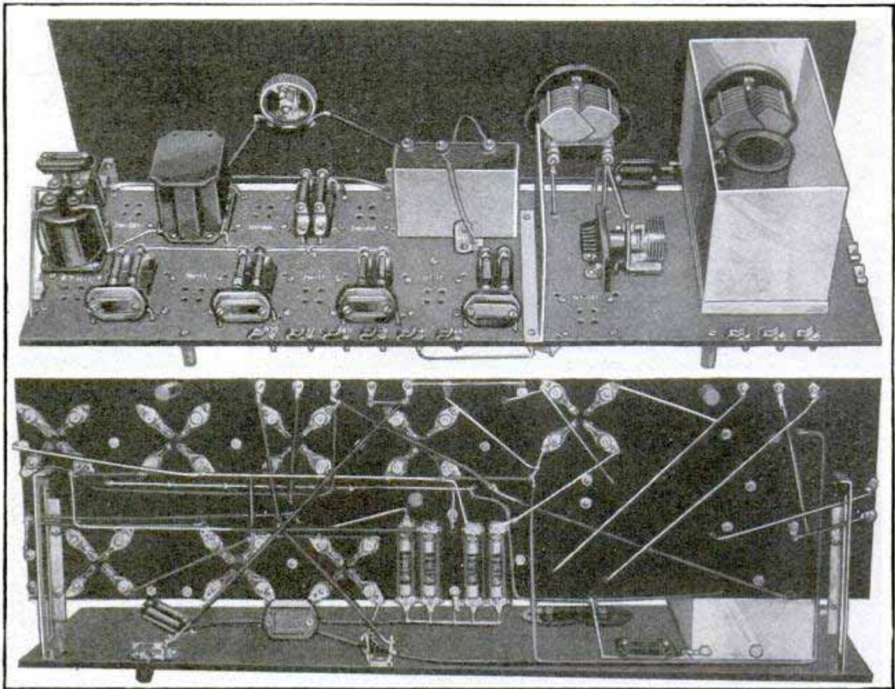
Top, Rear View of Completed Set with Lid of Oscillator Shield Removed; Center, Undersubpanel Showing Method of Wiring and Instrument Assembly There; Left, Side View of First-Detector Shield
