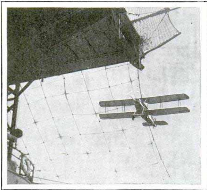
Plane Landing on the U. S. S. "Langley"; the Big Wire Net Protects the Lower Deck, and the Small Net Is for the Landing-Deck Crew to Dodge Into
