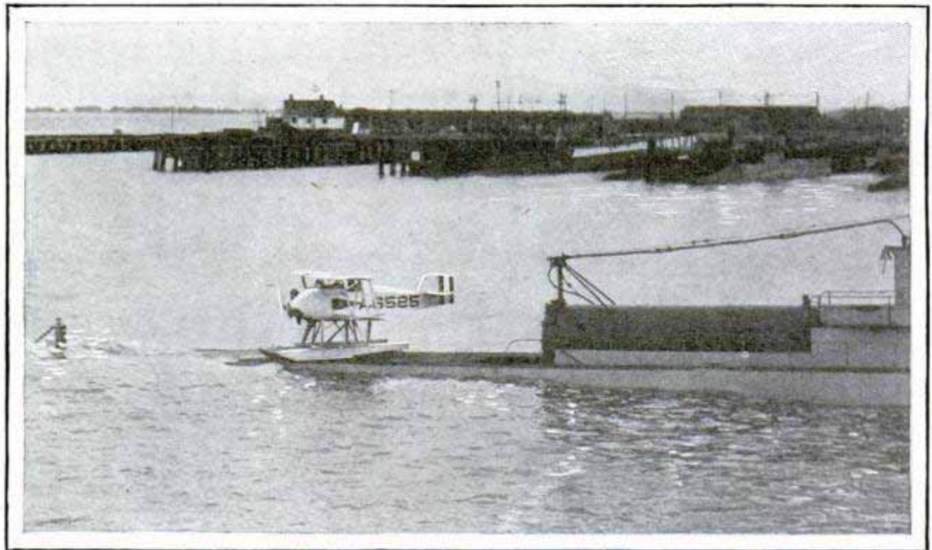
Assembled in Five Minutes from Parts Carried in the Big Steel Tank on the Deck of the Submarine "S-1," This Tiny Plane Is Ready to Take the Air as Its Mother Ship Submerges
