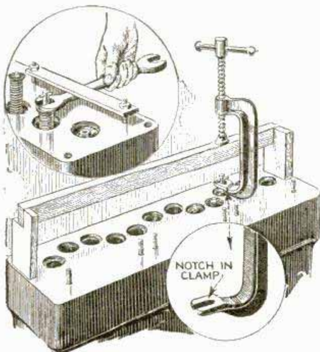
Easy Method of Removing Overhead-Valve Cages without Special Tools
