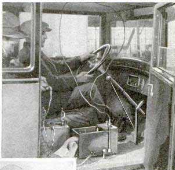
Duplicate Steering-Wheel Device Used to Measure Steering Effort, Top; and an Electrical Brake-Pedal Pressure Recorder, Center
