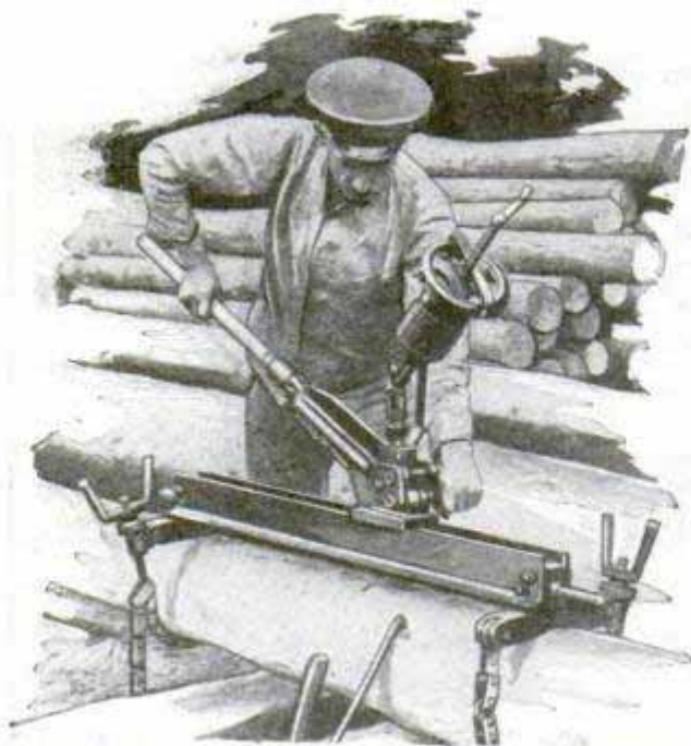
Injecting Charges of the Preservative in Timbers to Prevent Decay; Material Applied with Great Force
