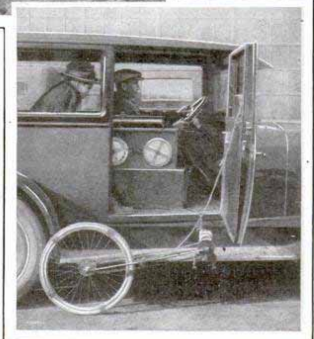
Bicycle Wheel and Chain Drive Operating the Electrical Apparatus That Makes a Written Record of Acceleration Tests at the Proving Grounds
