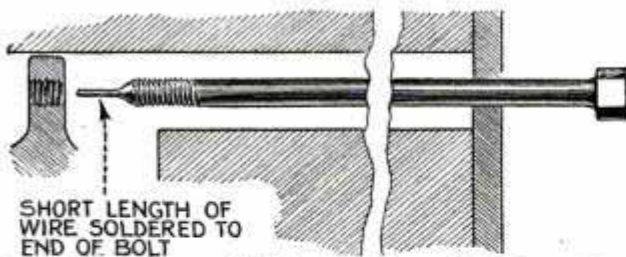
Finding the Tapped Hole for a Long Bolt in a Door Lock
