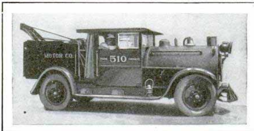
Auto-Wrecking Car like Locomotive; Fumes from the Exhaust Are Passed through the Smokestack
