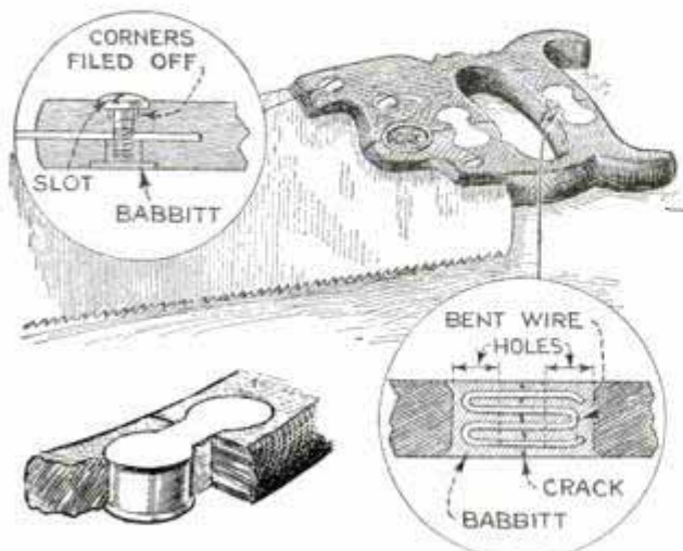
How to Make a Simple and Efficient Repair on Cracked Saw Handles
