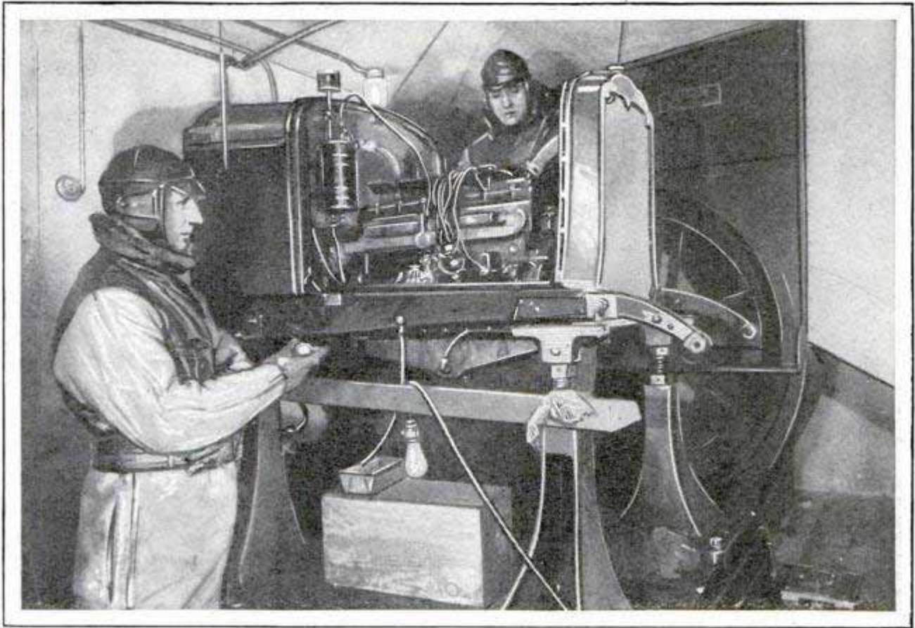
Clad in Aviator's Fur Suits, Testers in the Subzero Room of Automobile-Test Grounds Operate Sample Engines under the Most Trying Conditions to Which They Can Be Subjected
