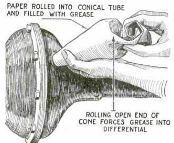
Filling Auto Differential with an Emergency Paper Grease Gun
