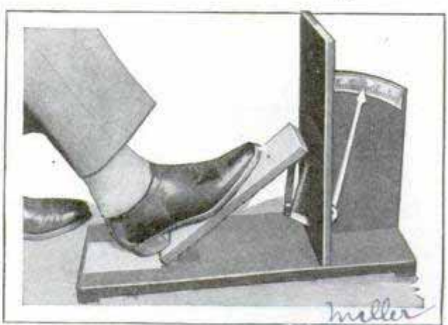
Gauge Used in Testing Foot Action of Automobile Driver License Candidates
