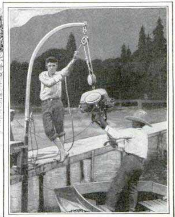
Left, Ordinary Baggage Truck Fitted with Wooden Support Facilitates Carrying Outboard Motor; Right, the Small Hoist Eliminates the Hard Task of Lifting the Motor from Boat to Wharf or Vice Versa
