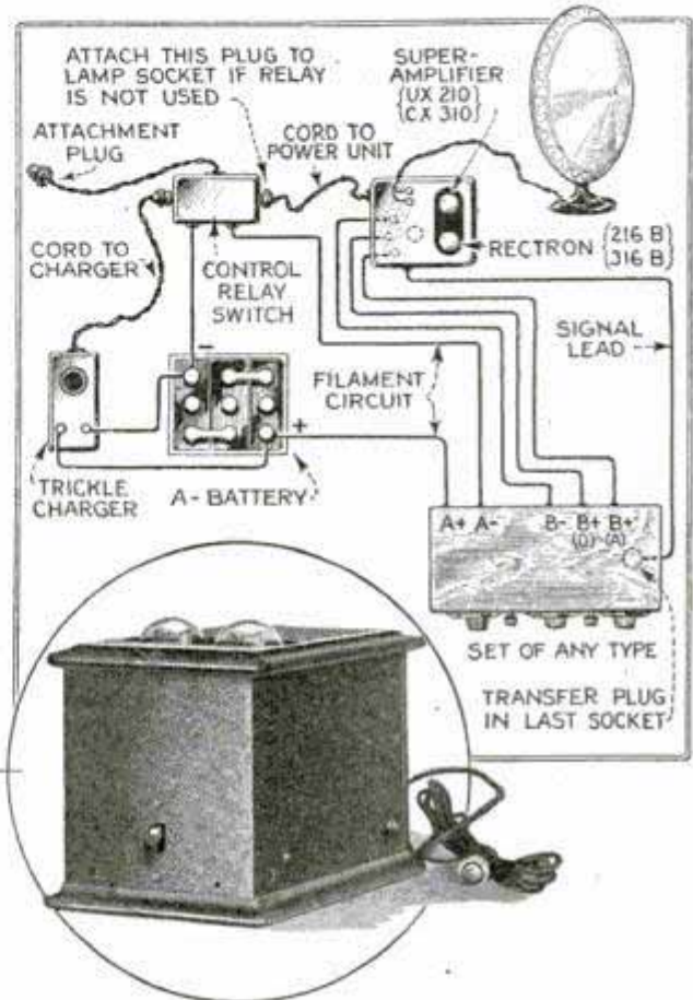
Amplifier and Diagram of Connections for Power Amplification and B-Elimination
