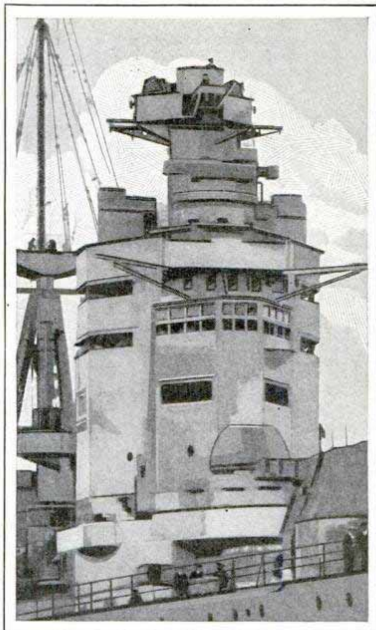
Eight Stories High and Violating, Because of Its Vulnerability, All the Accepted Rules of Naval Architecture, the Armored Control Tower of the "Nelson," England's Newest Warship, and, with Her Sister Ship, the "Rodney," the Biggest Battleship Afloat
