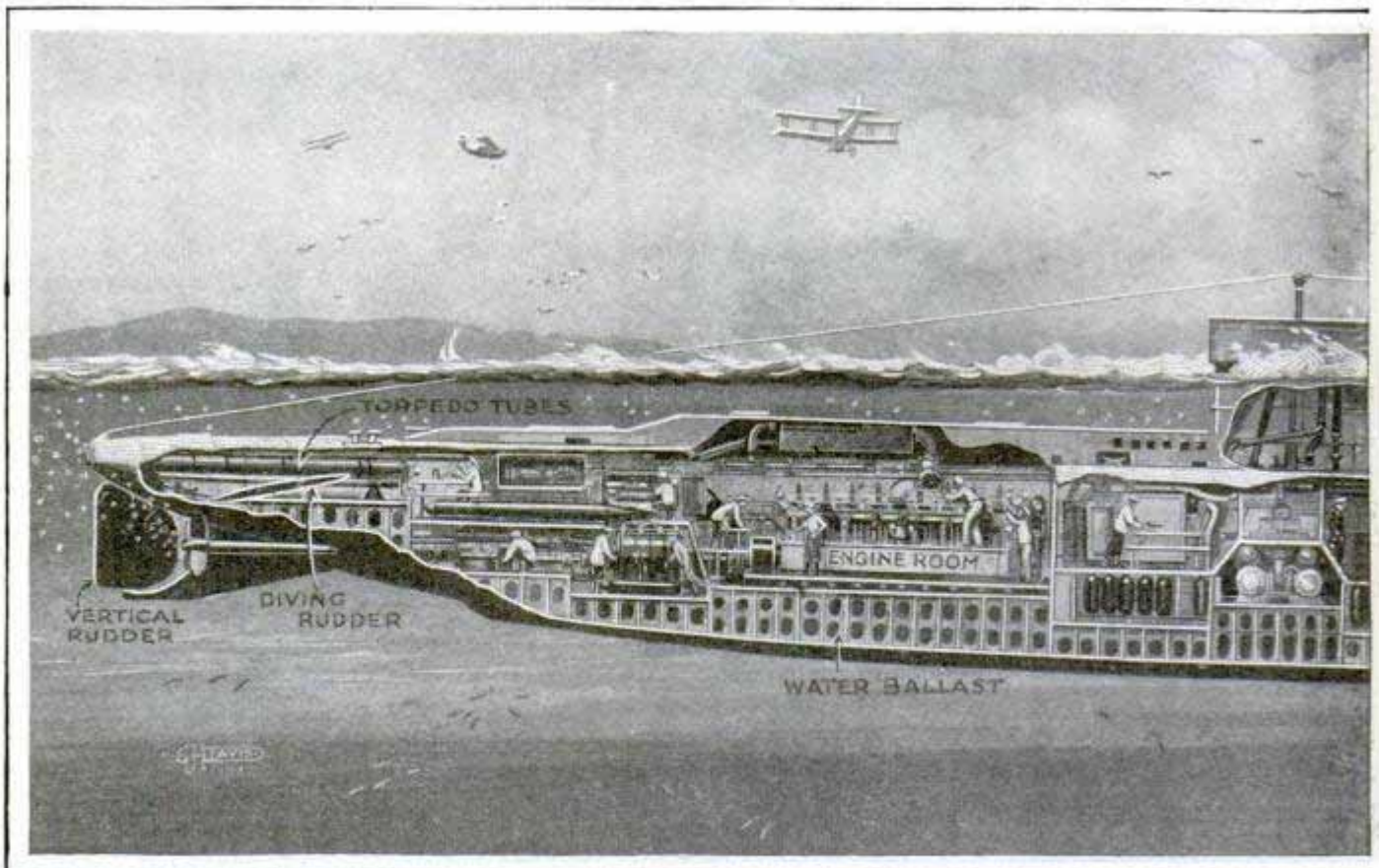
Cross Section of a British Submarine in the Act of Diving, Showing the Entire Crew at Stations, the Diving Rudders Set to Force the Ship Down and a Torpedo Being Shoved into Its Tube
