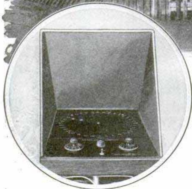
Ferry Slip Fitted with Beacon Transmitter to Guide Ships, and, Left, the Sound-Compass Dial
