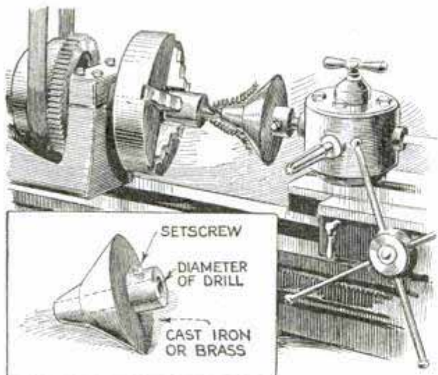
Cone-Shaped Device for Turning Away Long Chips on Automatic Machines
