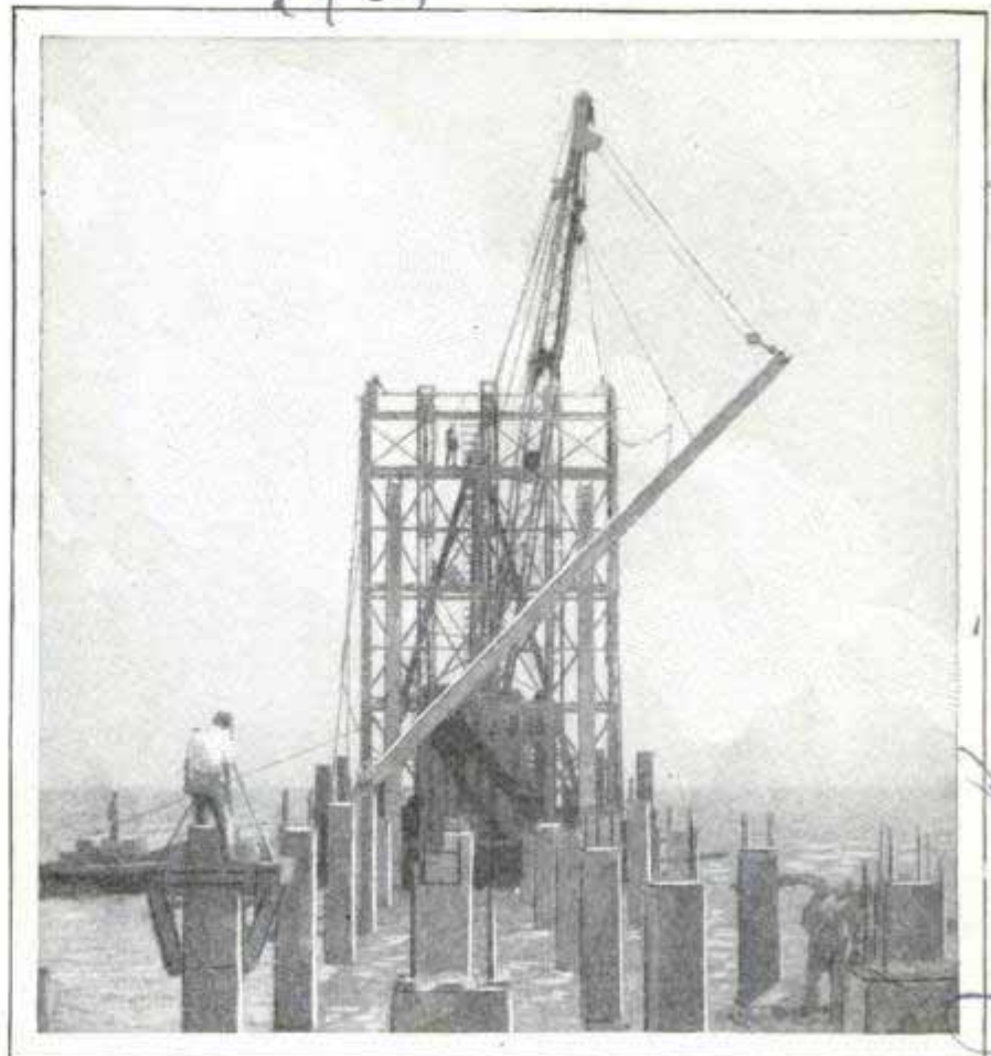
Swinging Eighty-Foot Concrete Pile into Place for Driving; Part of the Equipment That Did Rapid Work on New Orleans Bridge
