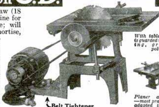
Belt Tightener
