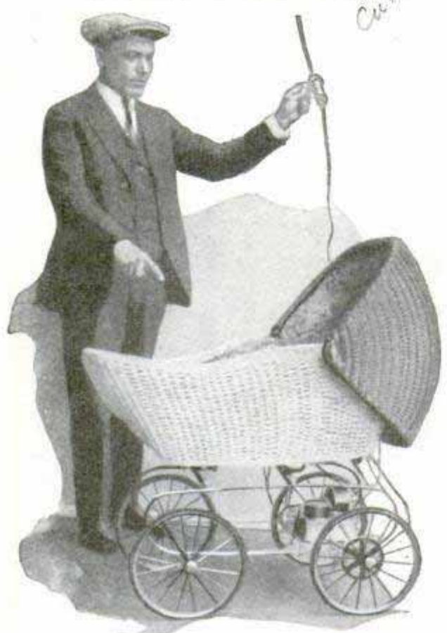
Rocking Apparatus Installed under Baby Buggy and Connected to a Lighting Socket for Operation
