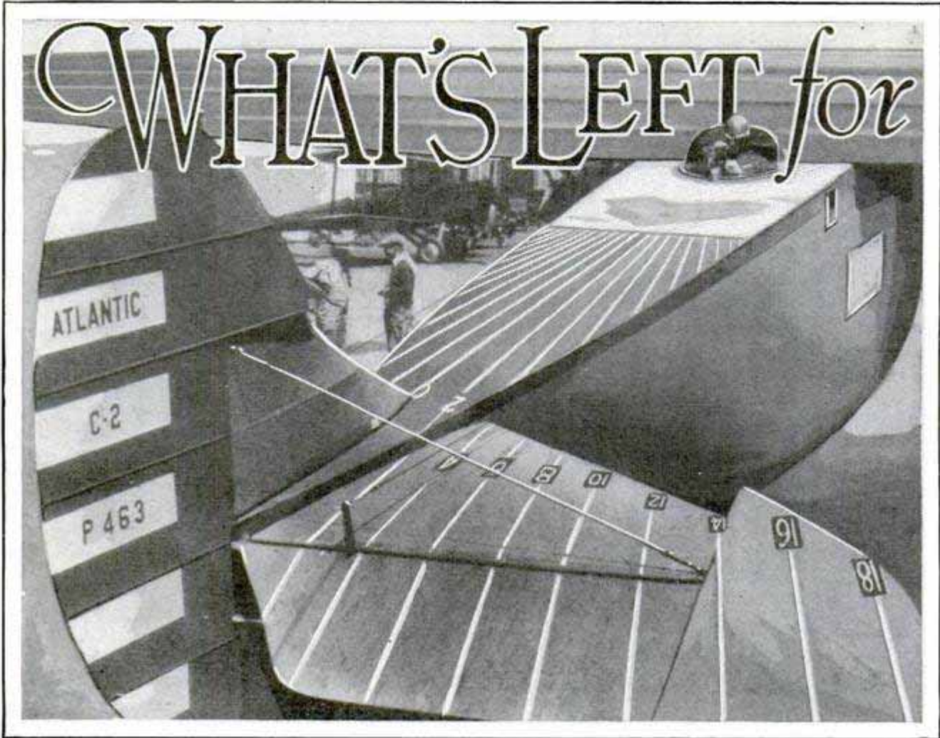
The Army Fokker Which Flew to Hawaii, Showing the Radial Lines Painted on the Ship to Help the Navigator in Dead Reckoning, Aided by the New Sun Compass
