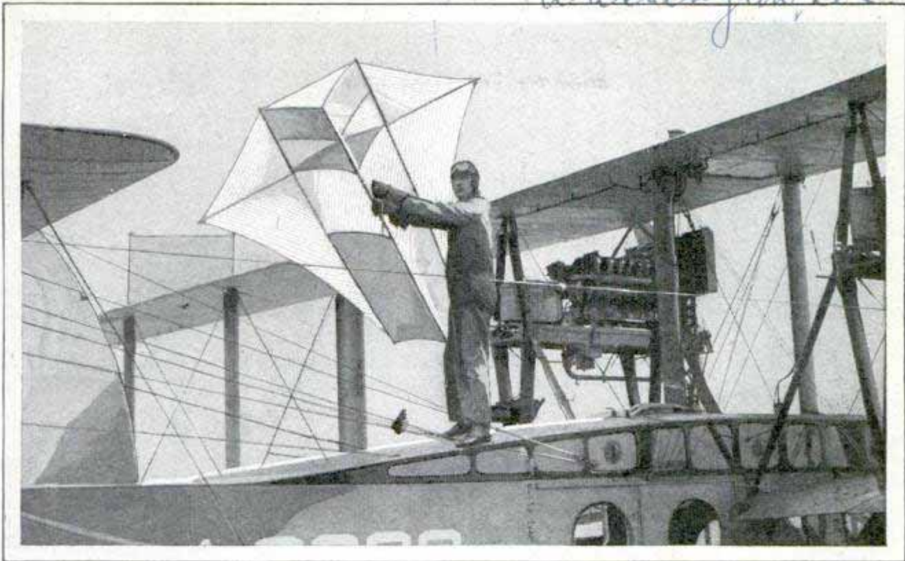
One of the Types of Kites Being Used on Naval Planes to Support Radio Antenna in Case of an Emergency; Besides This Service, the Kite May Be Used as a Visible Signal of Distress
