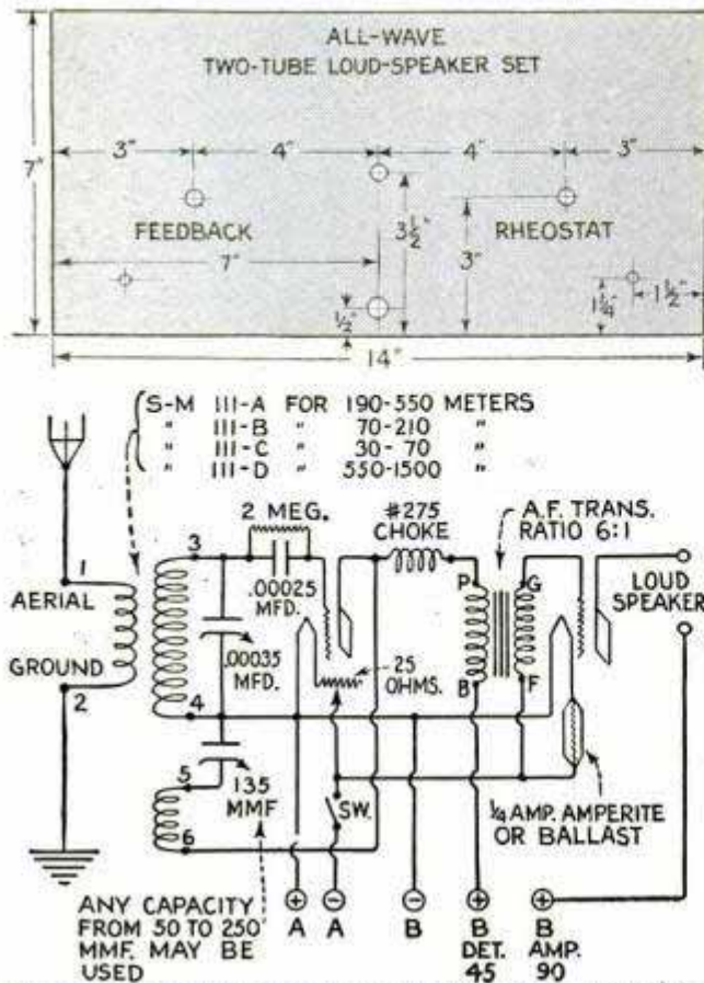
Above, Front-Panel Template; Below, List of Coils for Various Wavelengths, and Diagram of Circuits
