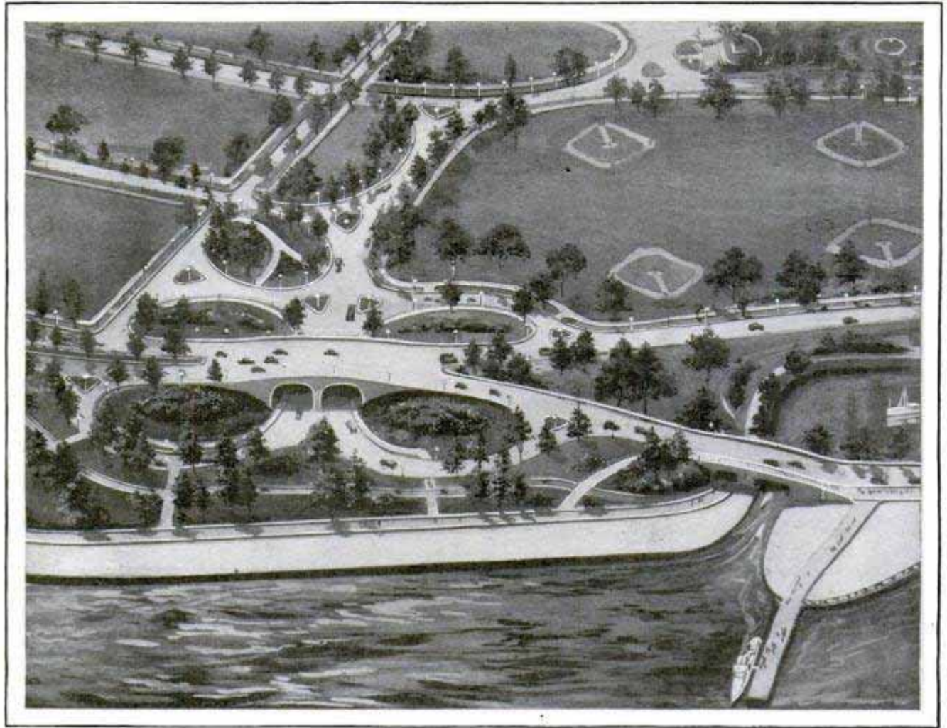
How a Busy Traffic Center at Entrance to Lincoln Park, Chicago, Has Been Arranged to Avoid Congestion by the Construction of Overhead Crossings, Permitting Safe Passages and Eliminating Delays
