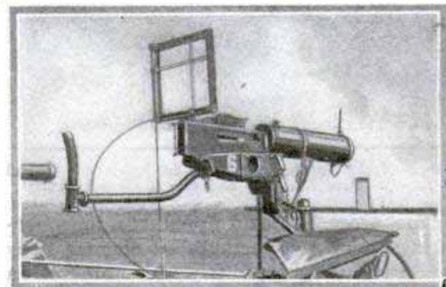
Mechanically Set Sight on Anti-Aircraft Gun, to Improve Accuracy of Fire at Moving Planes
