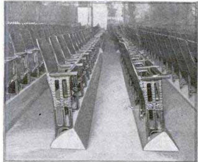
Theater Chairs on Concrete Ridge, Which Serves as Anchor and Footrest and Simplifies Task of Sweeping
