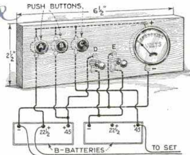
Wiring Diagram Showing Test Board Connected to the B-Batteries and Location of Apparatus
