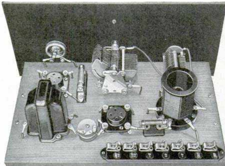
Rear View of the Completed Set, Showing Simple Arrangement of Parts
