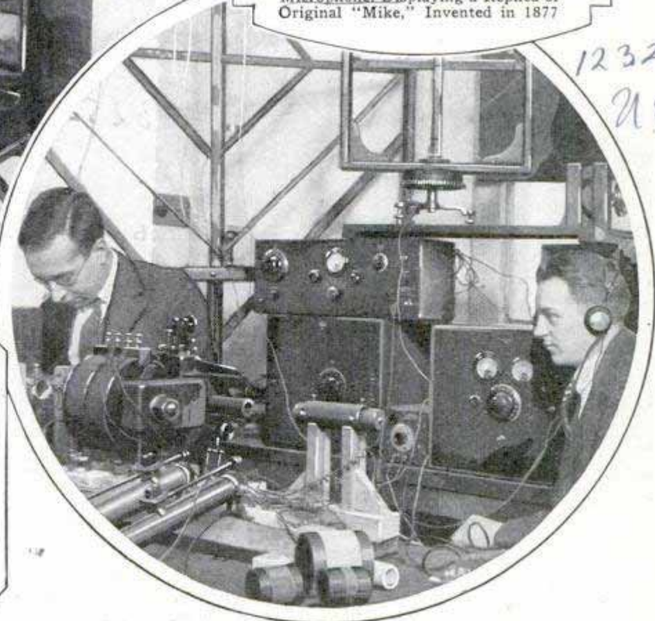
Above, an Attractive Radio Cabinet Copied from the Modern Baby-Grand Piano; Right, Dr. G. Breit and Dr. M. A. Tuve, Research Investigators of the Carnegie Institution at Washington, Conducting Experiments Verifying the Existence of a Layer in the Upper Air Which Bends Radio Waves Back to Earth; Changes in the Layer Are Said to Cause the Phenomenon Known as Fading
