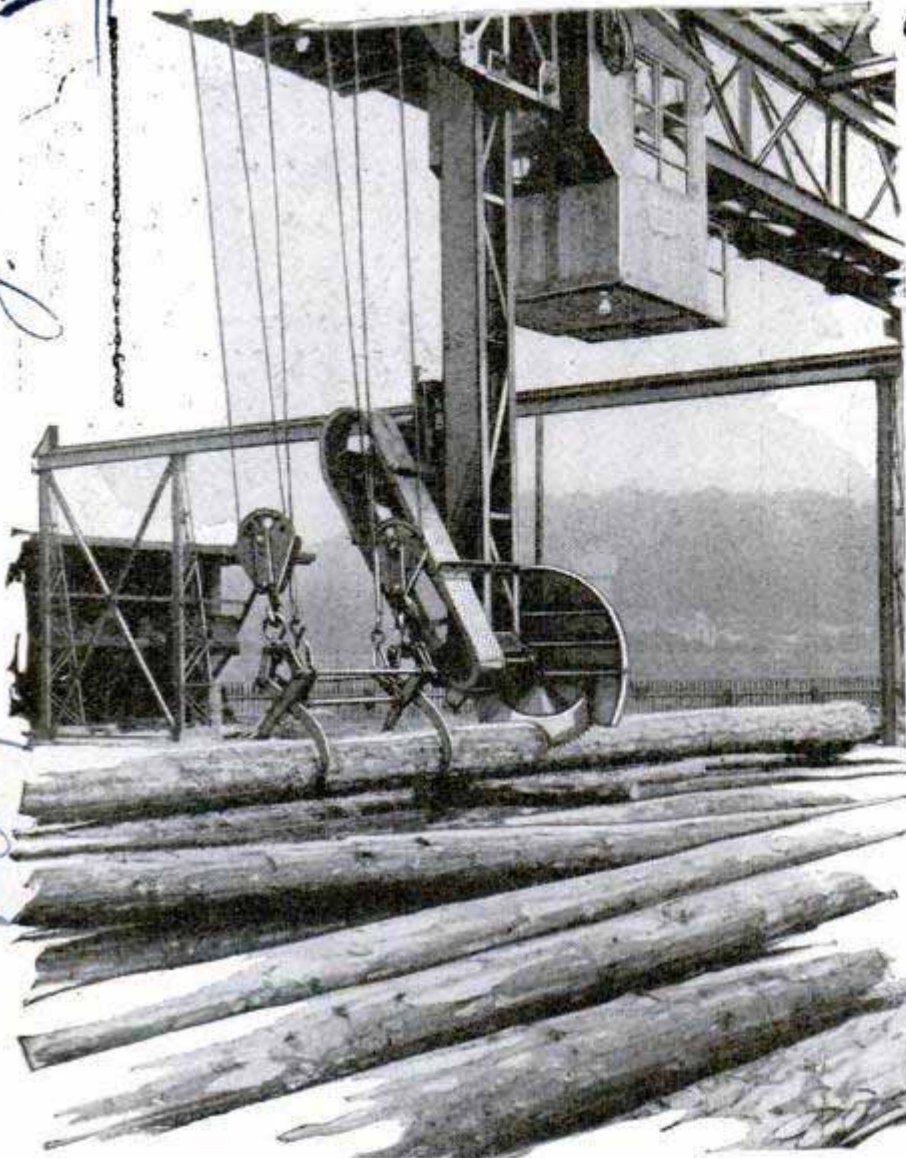
Circular Saw and Lifting Crane, to Speed Cutting and Handling of Logs at a European Lumbering Plant
