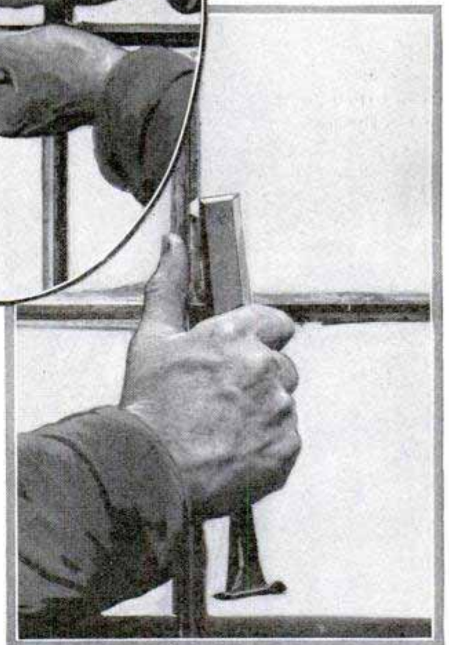
Top, Painting Frame before Setting Pane; Center, Putting On Layer of Bedding Putty; Bottom, Method of Forcing In Glazing Points
