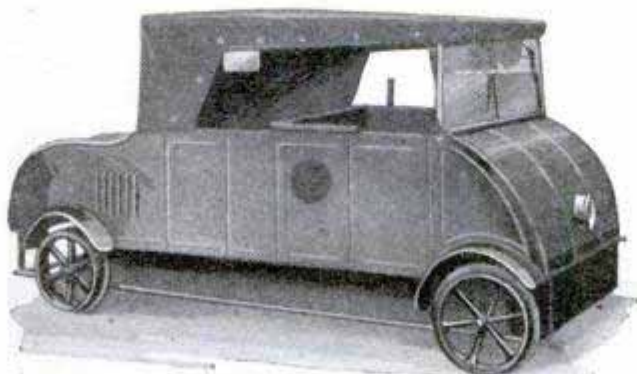
Railroad Track-Inspection Auto on German Lines; Car Has Speed of Fifty Miles an Hour with Load
