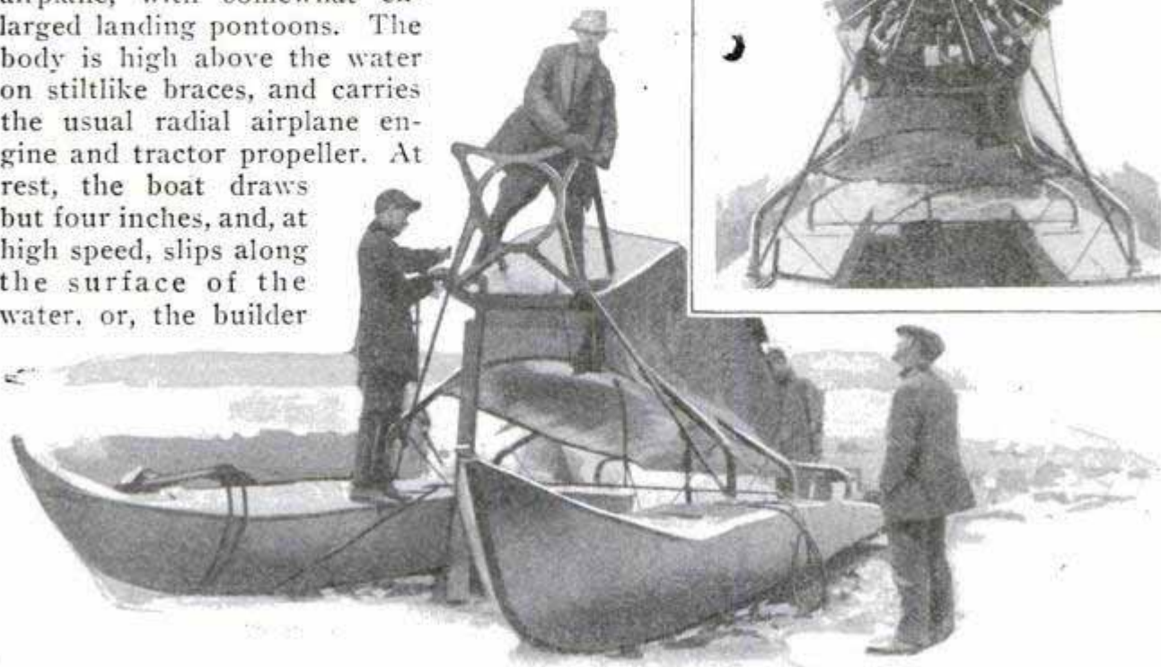
The Radial Aviation Engine of the Pontoon Boat, and the Craft Itself Ready to Have the Power Plant Mounted; It Follows Airplane Design, But Is Much Sturdier
