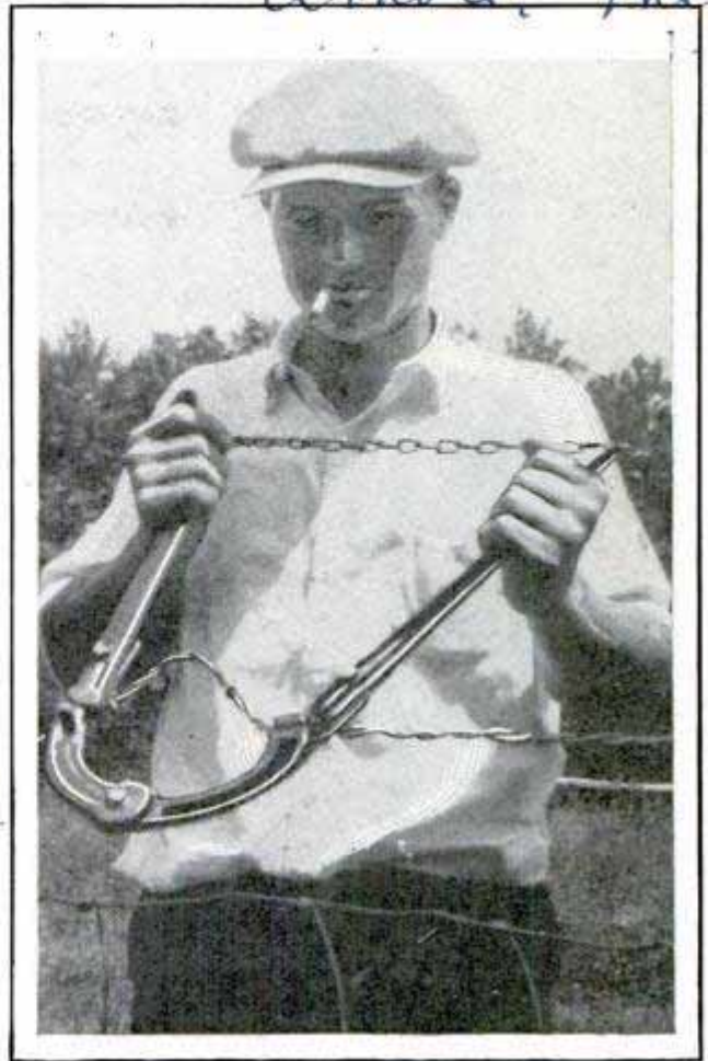
Stretcher in Use; the Chain at Ends of Handles Holds It When Desired Tautness Is Attained
