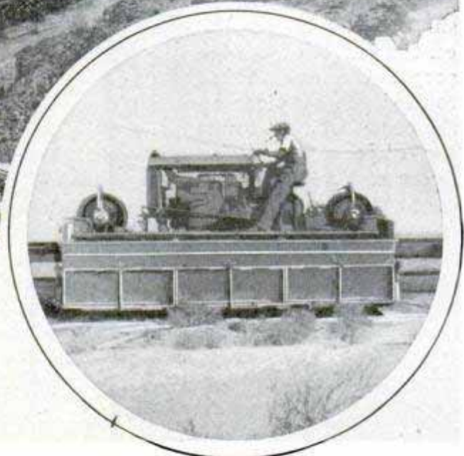
Front and Side Views of the Monorail Car. Showing Bunkers That Hold the Ore, and a Winding Track
