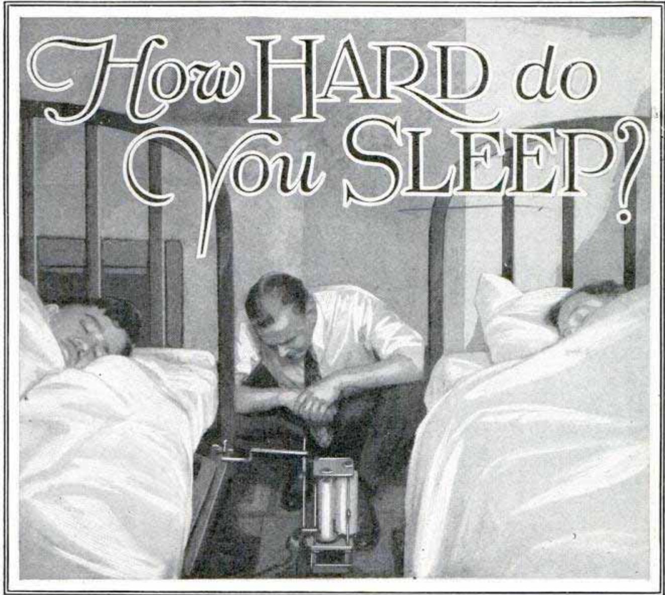
Clockwork-Driven Chart Used to Record Every Restless Movement of Sleepers Undergoing Tests at the Mellon Institute; It Also Charts the Exact Time of Each Movement
