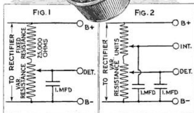
Resistor Having Several Taps to Obtain Various Voltages for B-Eliminators
