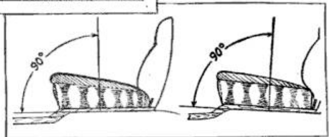
Sloping the "Kick-Up" of the Frame, as at Right, Keeps the Rear-Seat Rider from Being Bounced Forward, as at Left
