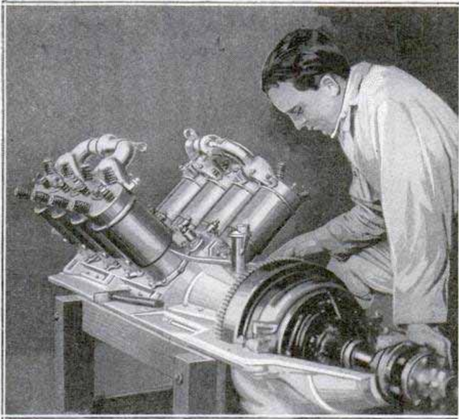
Curtiss Airplane Engine Being Dismantled to Be Rebuilt as a Marine Motor for High-Speed Boat
