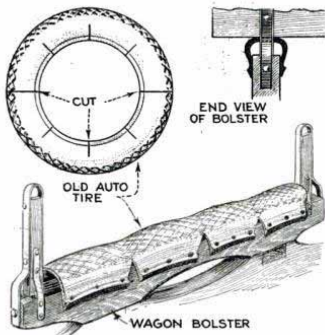
Old Auto Casing Nailed to Bolster Makes a Good Shock Absorber for Wagon
