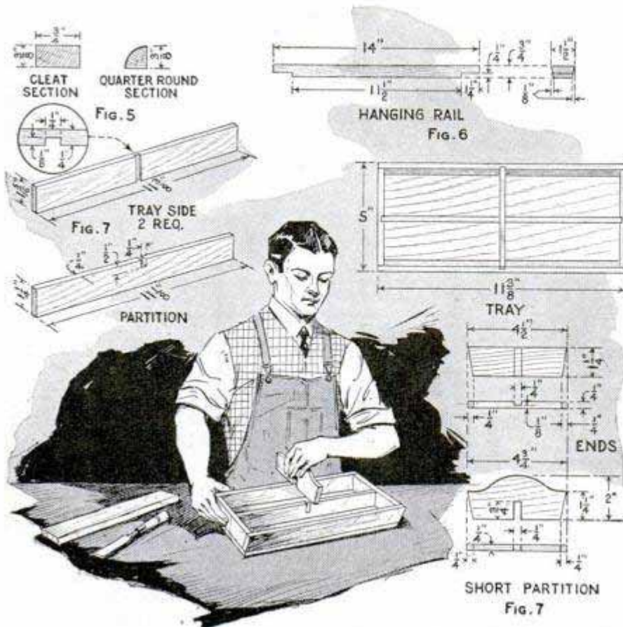
Details of Tray Construction, Cleat and Hanging Rail; the Bottom View Shows How the Tray Is Assembled
