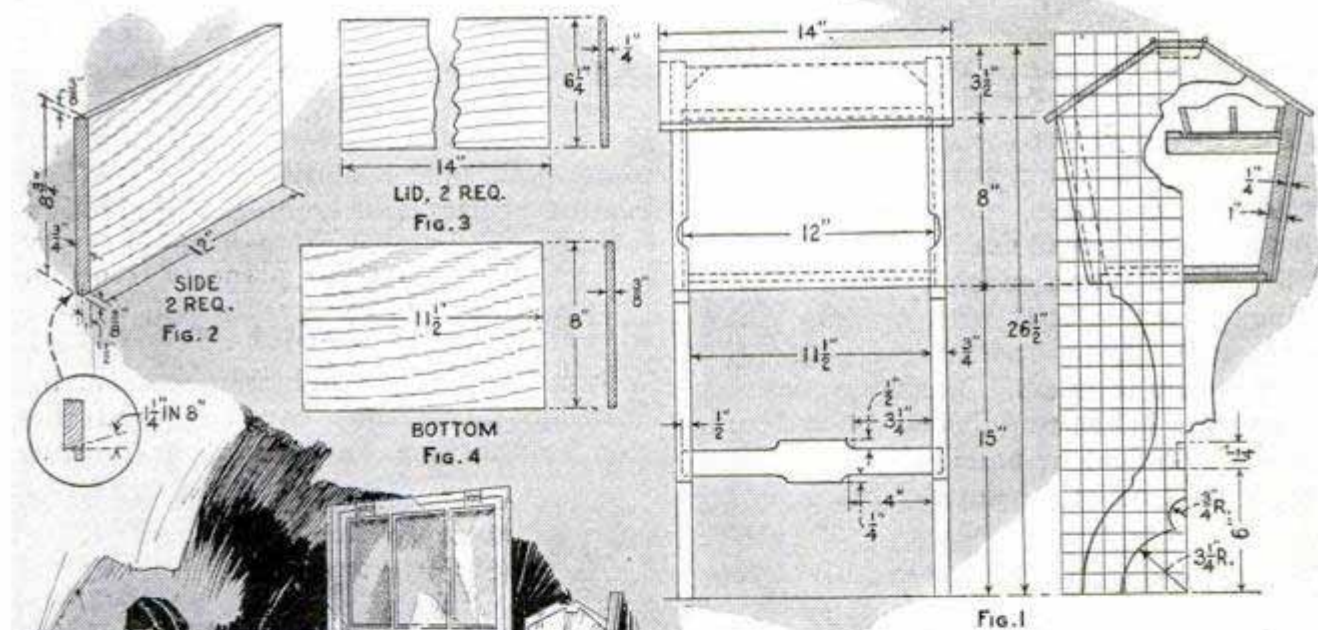
Details of Side, Lid and Bottom of Priscilla Sewing Cabinet; Also Front Elevation, and Layout of End, with Part Section
