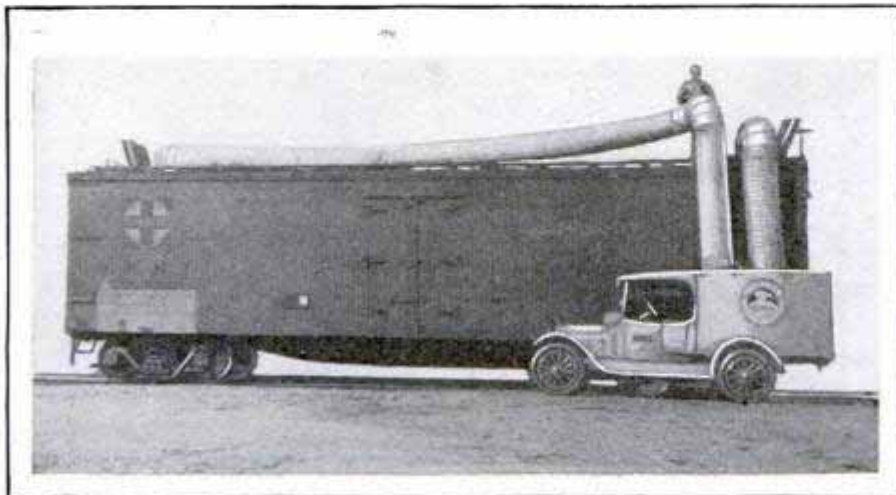
Blowing Air over Ice in Refrigerator Car, to Speed Cooling of Contents; Outfit Is Quickly Set Up at Different Cars
