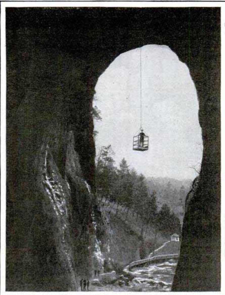
Examining the Underside of Virginia's Natural Bridge, at Staunton, to See if Traffic on Top Is Damaging It
