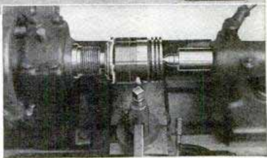
A close-up view of the lathe tool making a finishing cut across the piston
