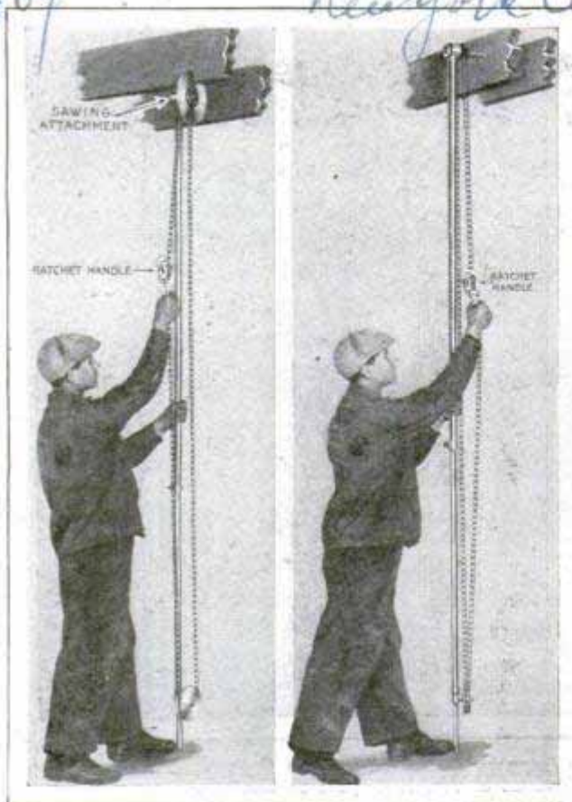
Chain Rig for Sawing and Boring; It Saves Both with a Ladder and Permits Easy Working Position
