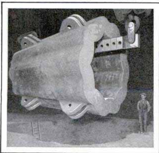
Monster Unit at Eastern Steel Mill; the Mold for Making Ingots That Weigh Over 200 Tons
