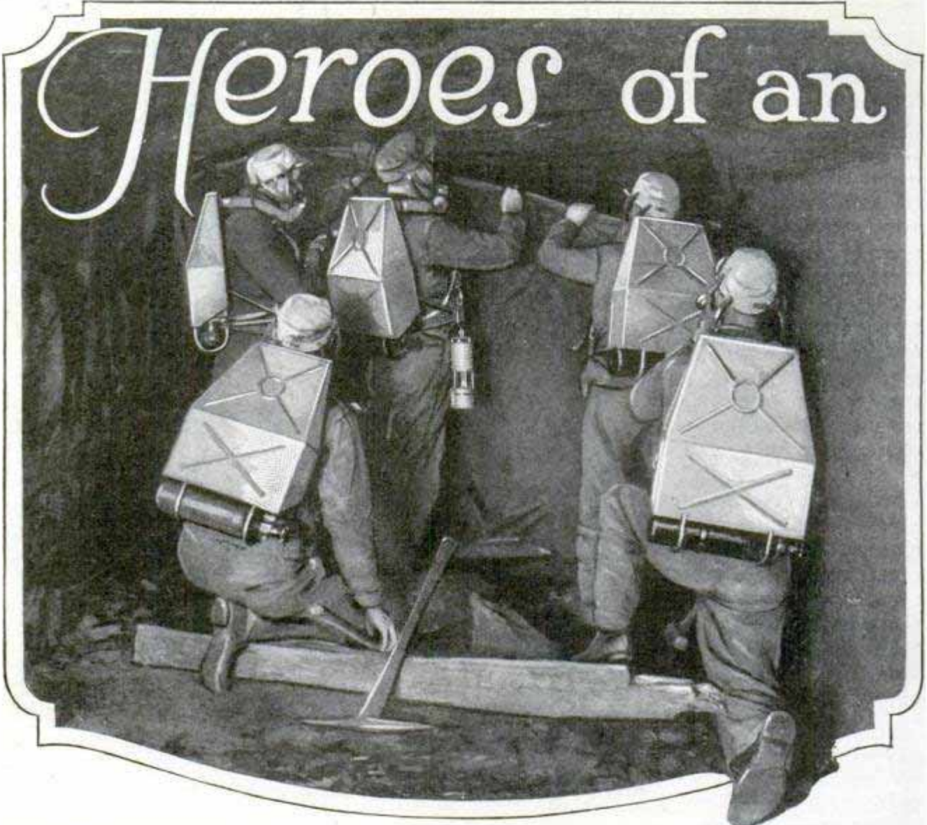
Mine-Rescue Crew Erecting Works to Control and Direct the Fresh-Air Current to Clear a Mine of Dangerous Gases after an Explosion; They Carry Large Oxygen Tanks on Their Backs
