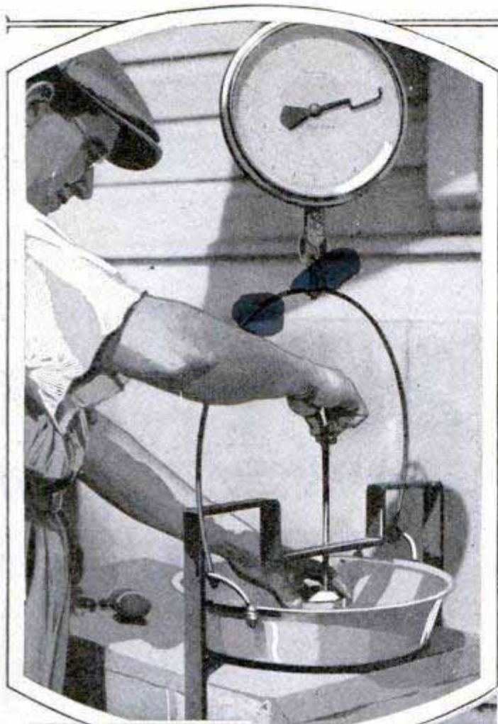
Strong Eggshells Are Necessary to Stand the Rigors of Shipment, and Fowls Are Especially Bred to Produce Them; Above Is the Test by Which the Strength Is Determined
