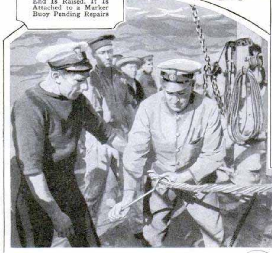
Huge Grappling Iron, Above, Which Has Been Broken by Contact with Rocks on the Sea Bottom, While Trying to Find the Cable; at Left, Workmen Repairing the Armored Sheath, the Last Step in Making a Splice in the Cable before Returning It to the Ocean, Ready Again to Transmit Messages
