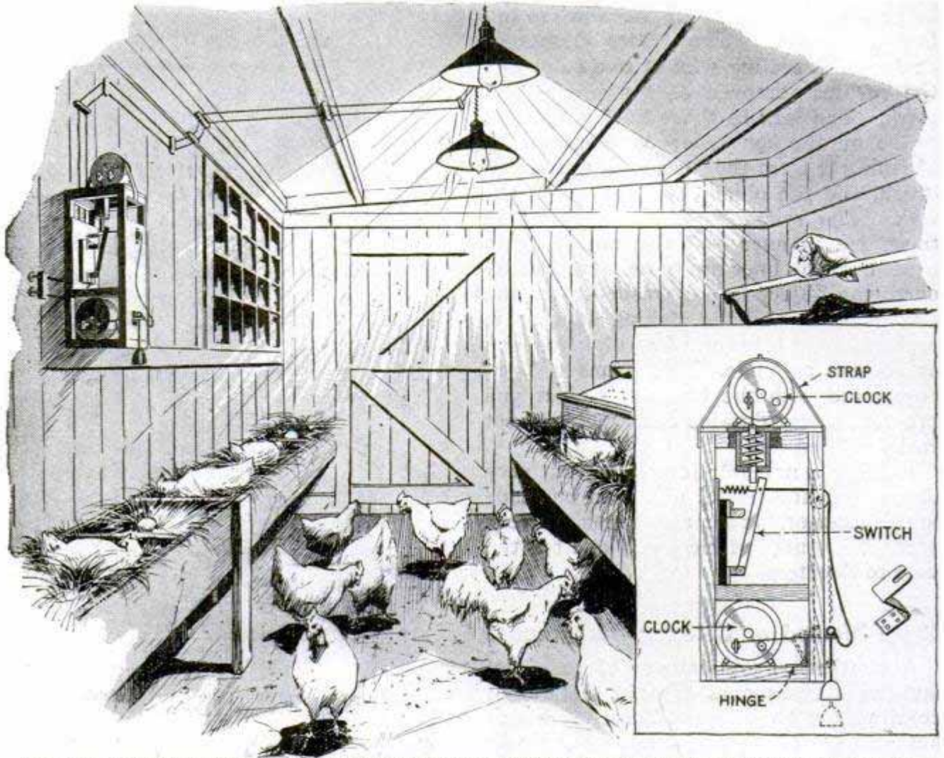
Any Poultryman Who Has Two Extra Alarm Clocks Can Readily Construct This Automatic Switch for Turning the Hen-House Lights On and Off to Increase the Hen's Working Day
