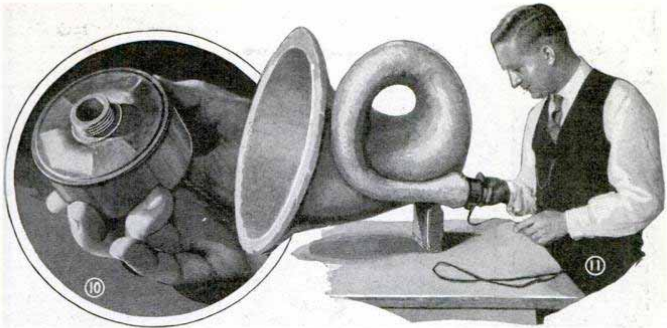
Left, Type of Loud-Speaker Unit Suggested, Which Is Easily Mounted in a Small Brass Bushing, or Sealed in Plaster in the Position Shown in the Photo at Right
