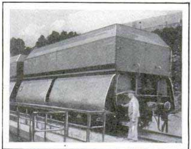
Freight Car, Dumped from Sides by Pulling Levers at End in Few Seconds, Holds Fifty Tons
