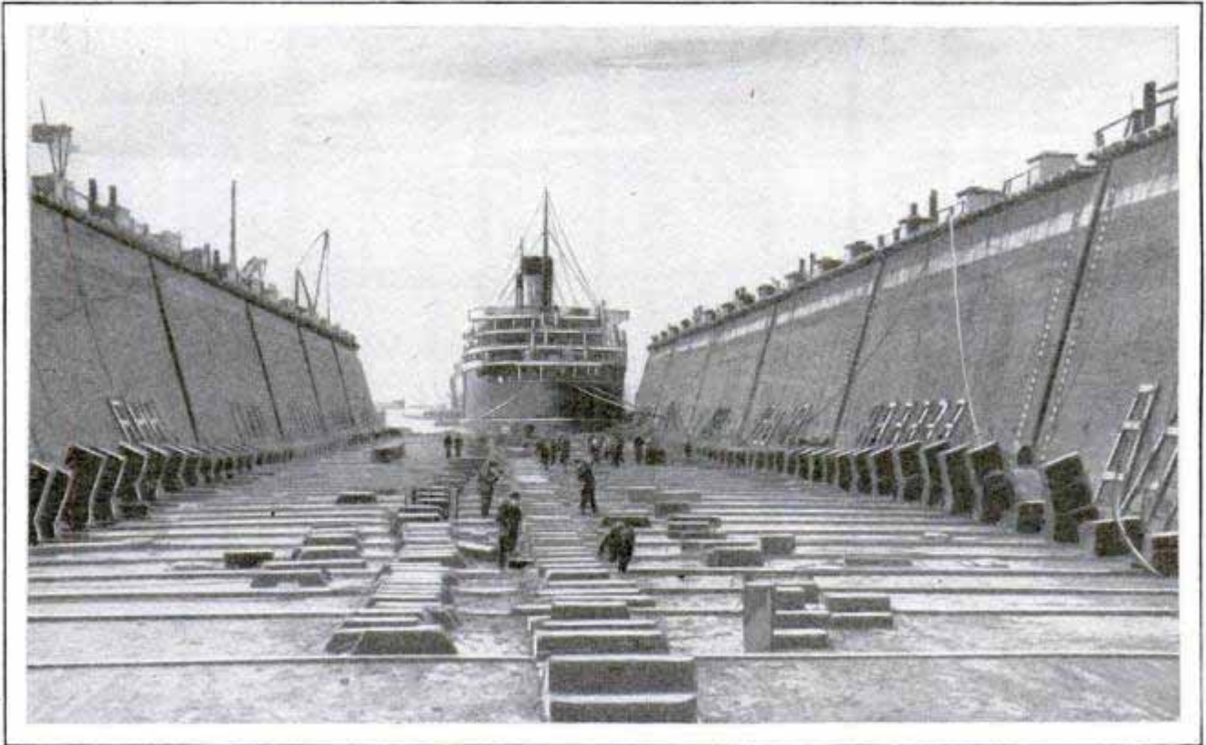
Docking the "Malolo," Biggest Passenger Ship Ever Built in the United States; Although the Vessel Was Rammed during a Speed Trip, Its Water-Tight Bulkheads Prevented Sinking
