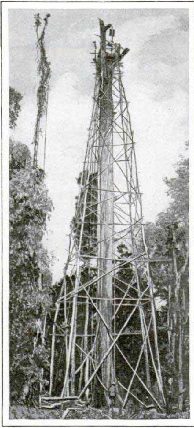
Signal Tower in the Philippines, Utilizing a Tree to Lift the Signal Light above the Jungle
