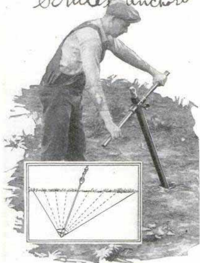
Setting the Anchor, and Diagram Showing How It Grips Wide Area When in Place
