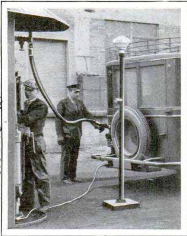
Filling Gasoline Tank on Motor Bus in Safety; Note Cable at Bottom, Making Ground Connection
