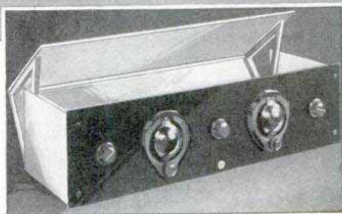
Above, Completely Assembled Set Mounted on Aluminum Chassis with Front Shield in Position; Below, Sides in Position, Back and Top Assembled in One Piece
