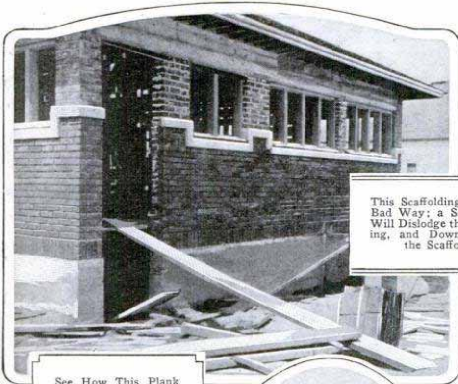
See How This Plank Sags under Its Own Weight; It Is More Than Likely to Break When a Man Carries a Load over It
