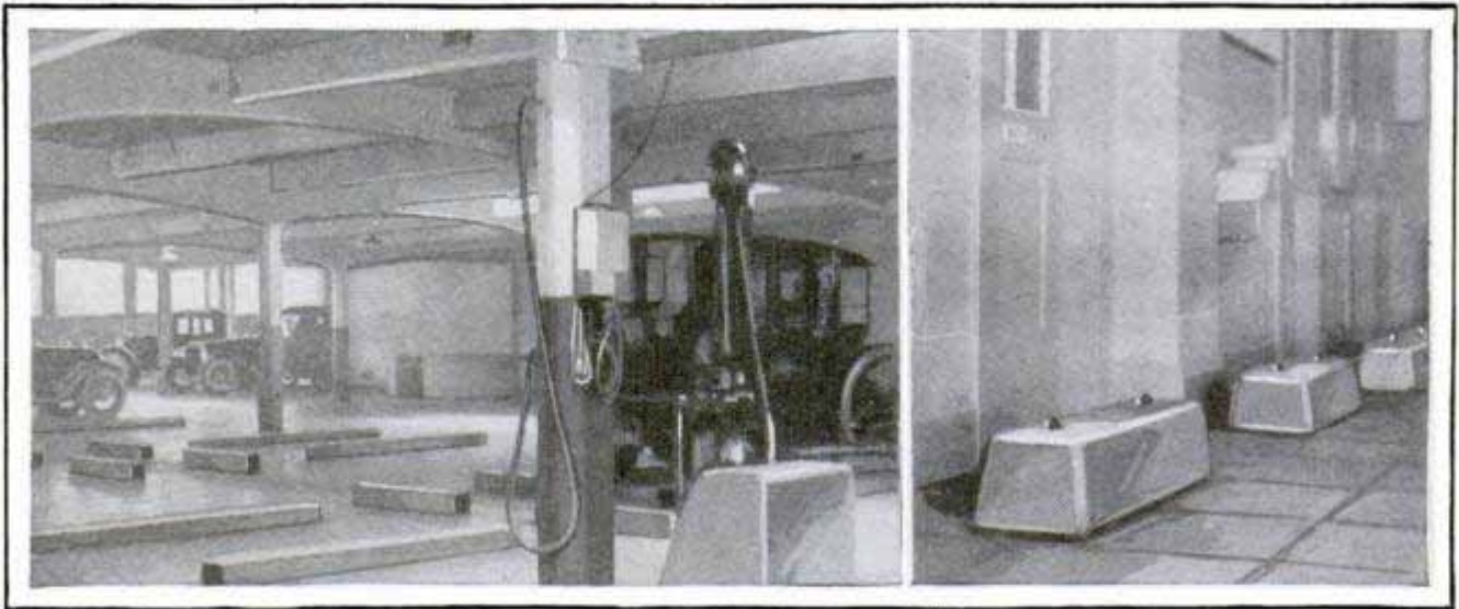
Concrete Bumpers in a Large Garage Are Heavy Enough to Withstand Abuse and Can Readily Be Moved from Place to Place
