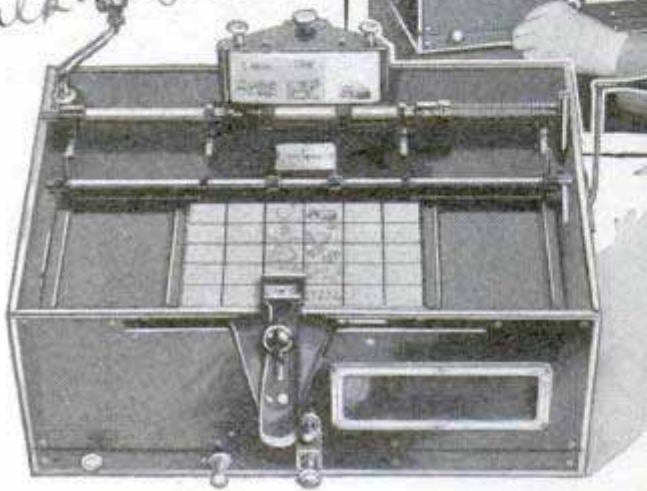
Machine Showing Index Chart and Record Tape, Synchronizing Knob above Operator's Left Hand and Cabinet Open for Removing Record
