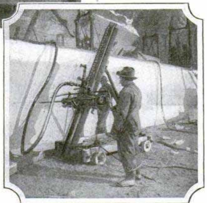
Courtesy Vermont Pneumatic Chisels and Electric Drills Do Much of the Work; Center, Gang Saws Cutting Layers
