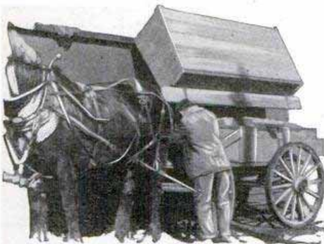
Dumping Box for Loading Sand or Gravel into Wagons from Freight Cars
