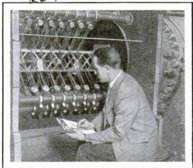
Reading Gauges That Tell Where Duralumin Girder Is Weakening; Piece Being Squeezed by Big Plunger
