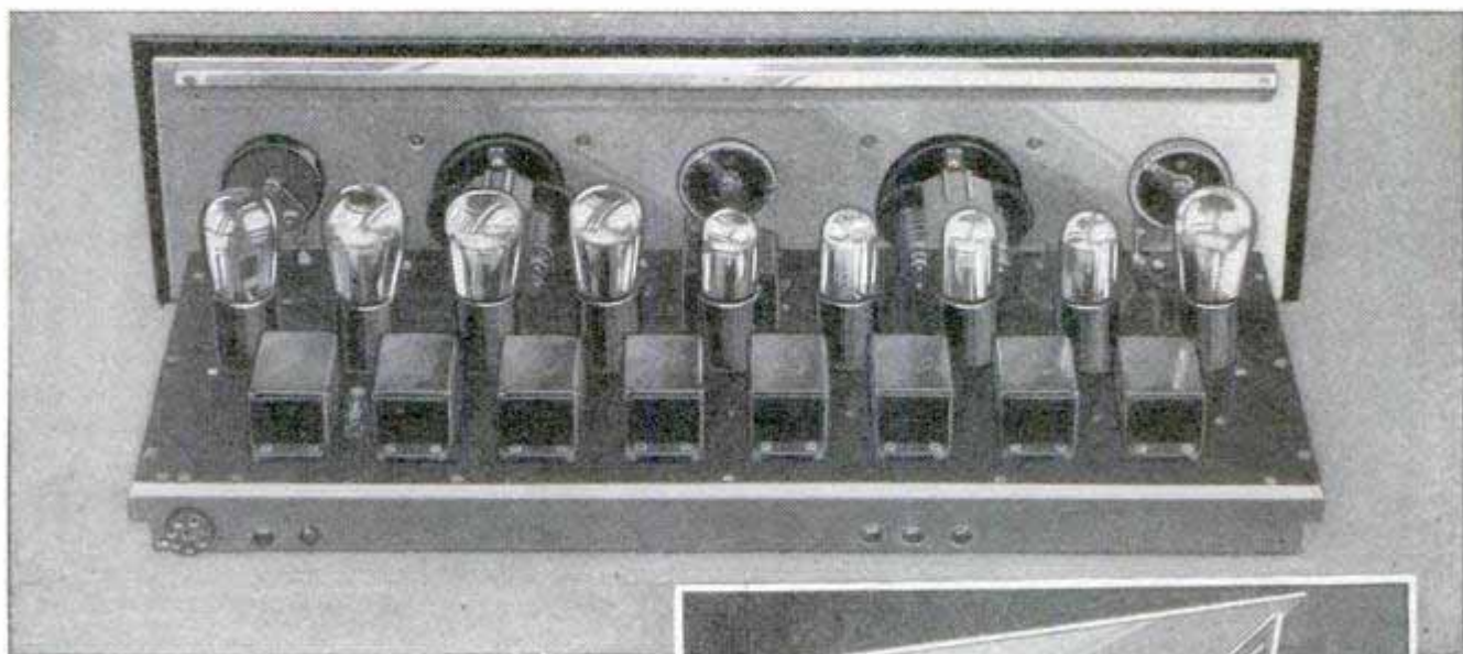
Above, Completely Assembled Set Mounted on Aluminum Chassis with Front Shield in Position; Below, Sides in Position, Back and Top Assembled in One Piece
