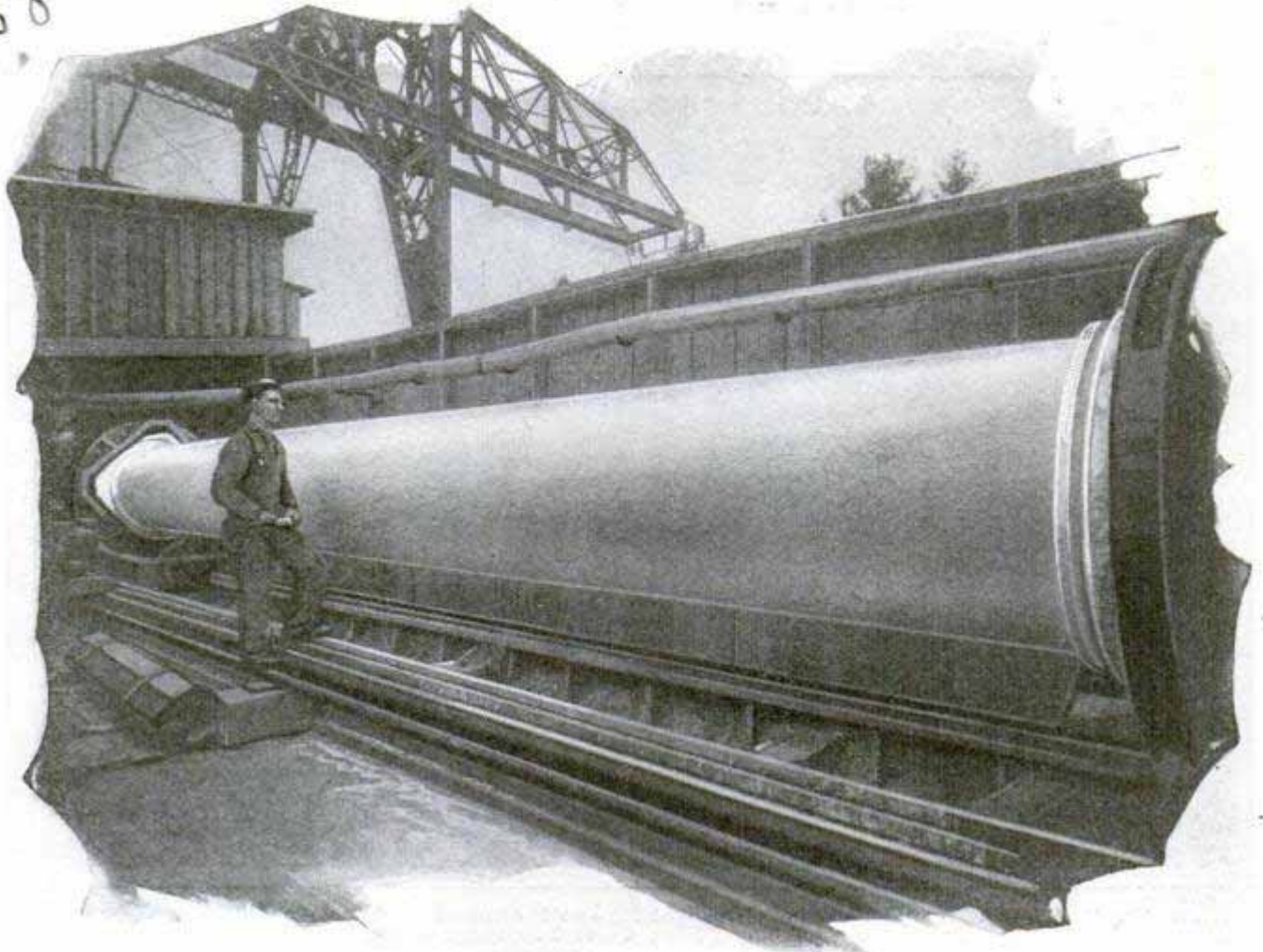
Turning a Marble Column, Thirty Feet Long and Four Feet in Diameter, in a Giant Lathe; Smooth Columns Are Often Made in One Piece, While Large Fluted Ones Are in Sections
