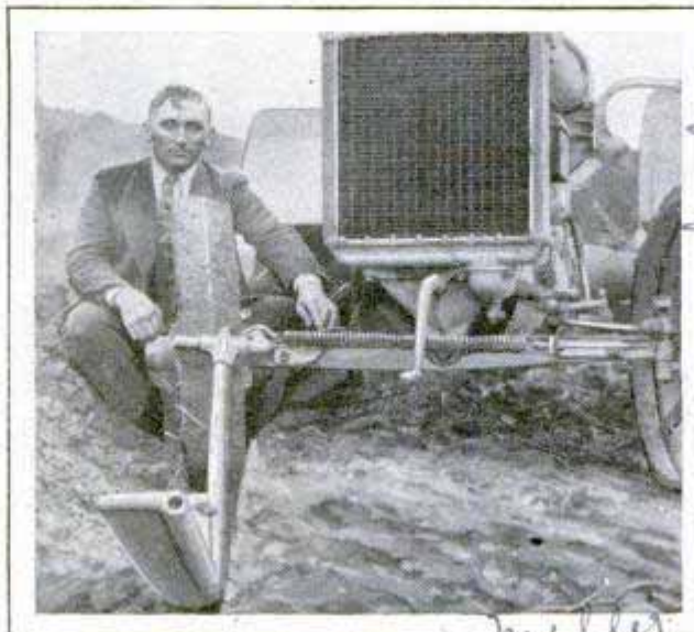
Steering "Foot" That Guides the Tractor
