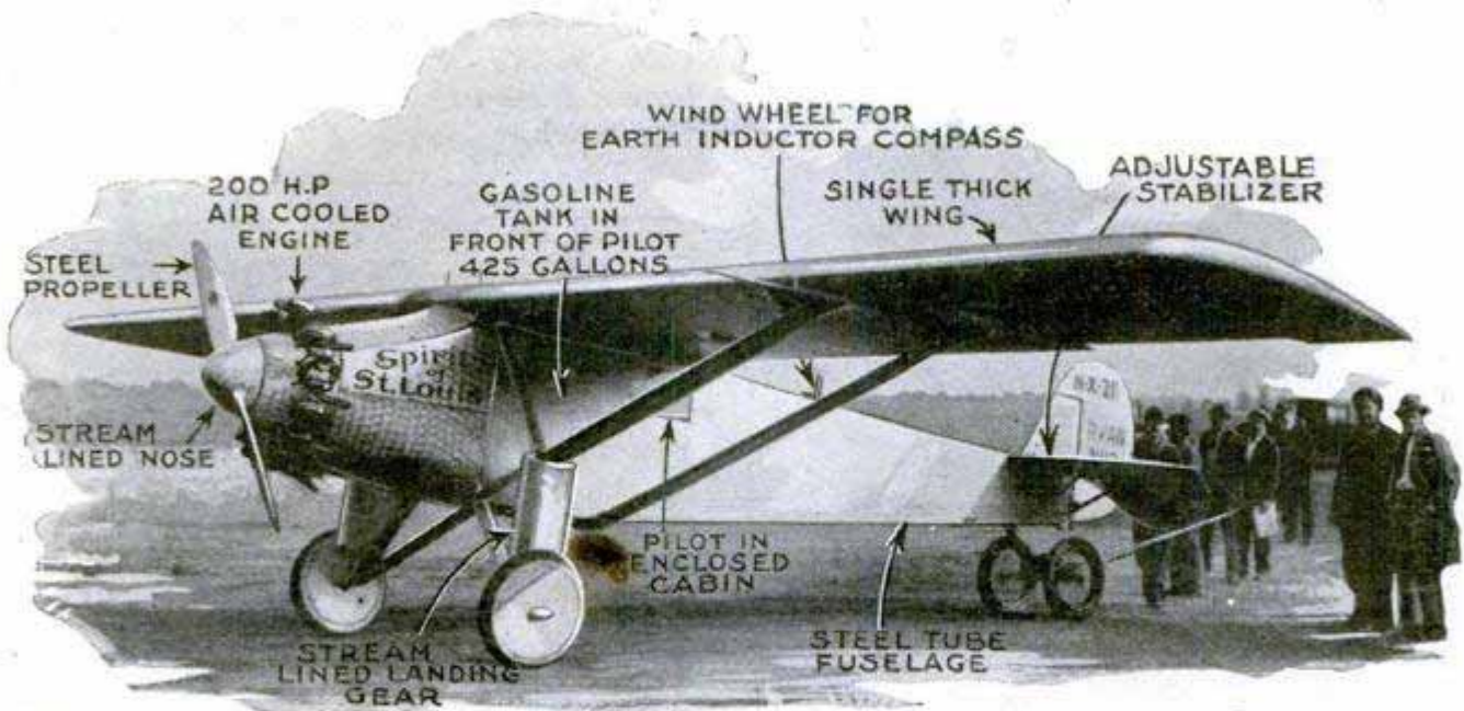
The "Spirit of St. Louis" in New York, and Some of the Principal Features of the First Airplane to Bridge the Gap between Two Great Cities on Opposite Sides of the Atlantic in One Flight
