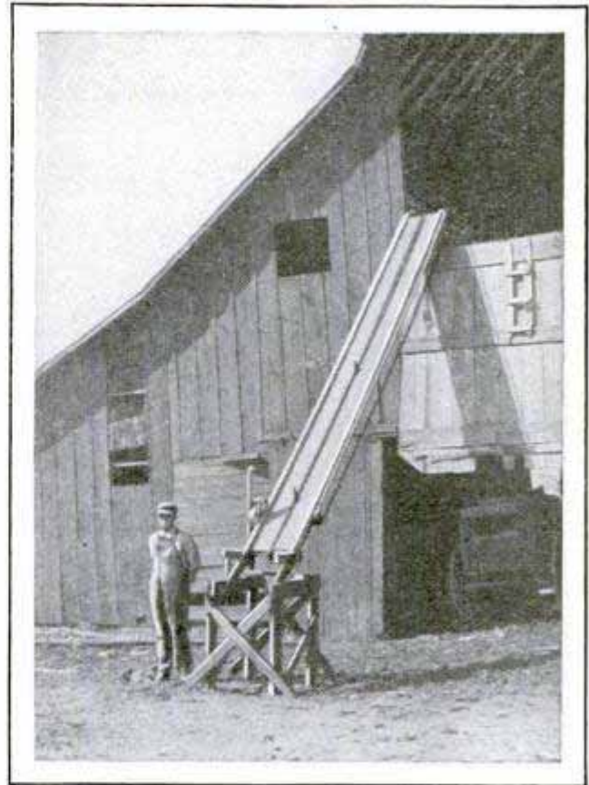
Convenient Homemade Apparatus for Hoisting Baled Hay into Barn Loft
