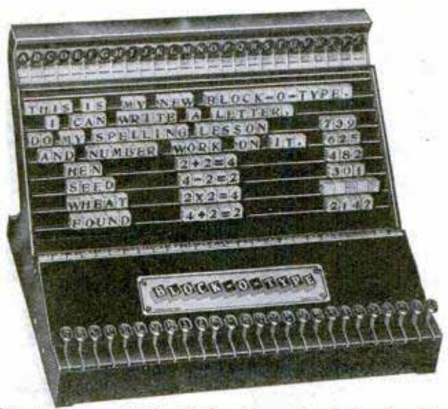
Blocks Arranged after Lifting Them from Magazines by Pressing Keys at Bottom; Feeder Openings at Top
