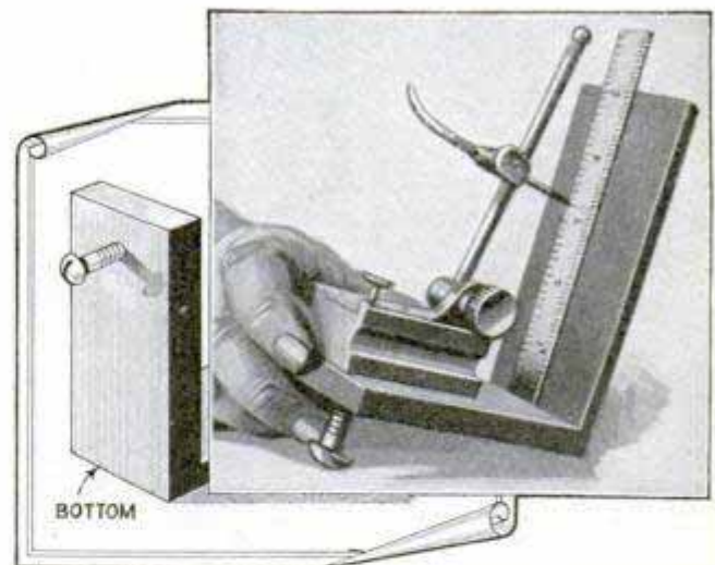
Practical Method of Setting the Mechanics' Surface Gauge Also Makes Reading Easier
