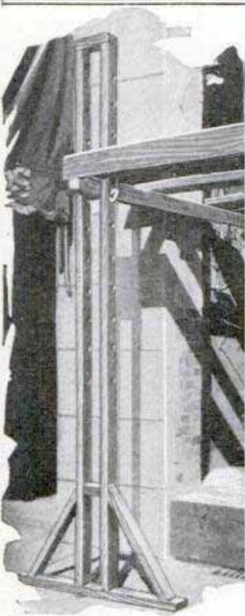
Simple Adjustable Scaffold for Store-Front Erection
