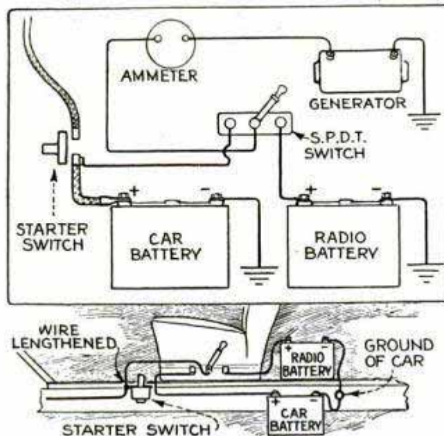
Method of Charging a Radio Battery in an Automobile and Connections to Be Made for the Purpose
