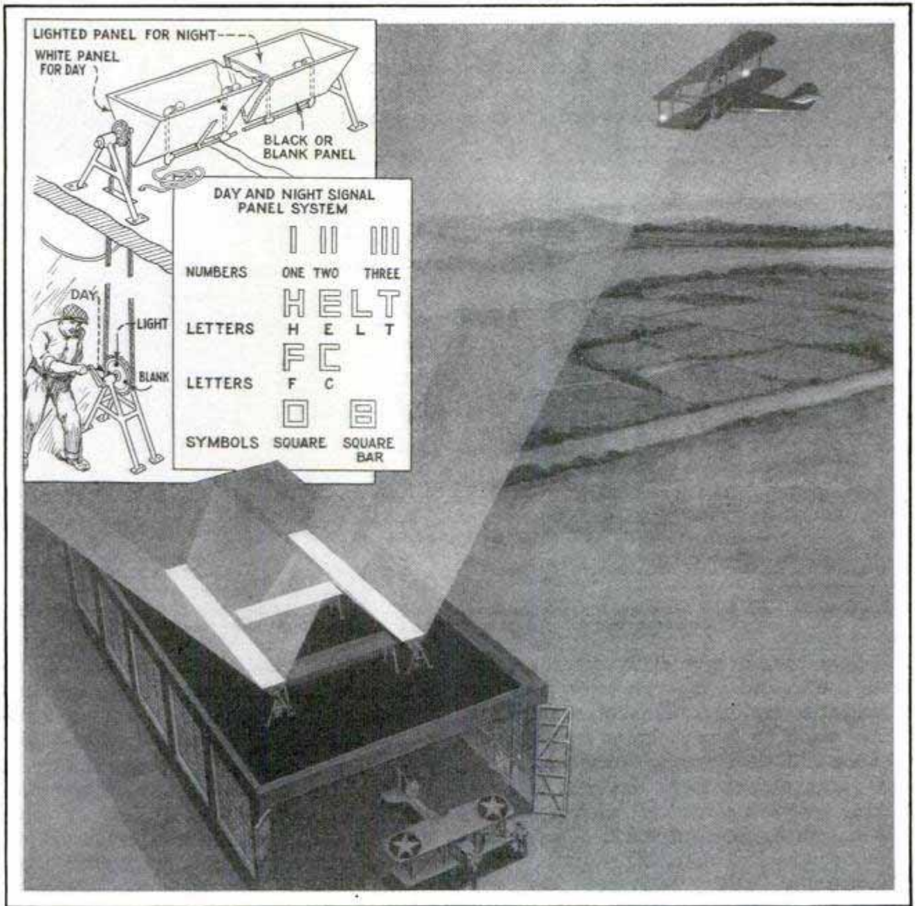
Guiding Airplane Pilots with Troughs of Light; Drawing of the Signal Apparatus as Installed on Top of Hangar, How Signs Are Operated, and Drawings of the Eleven Characters
