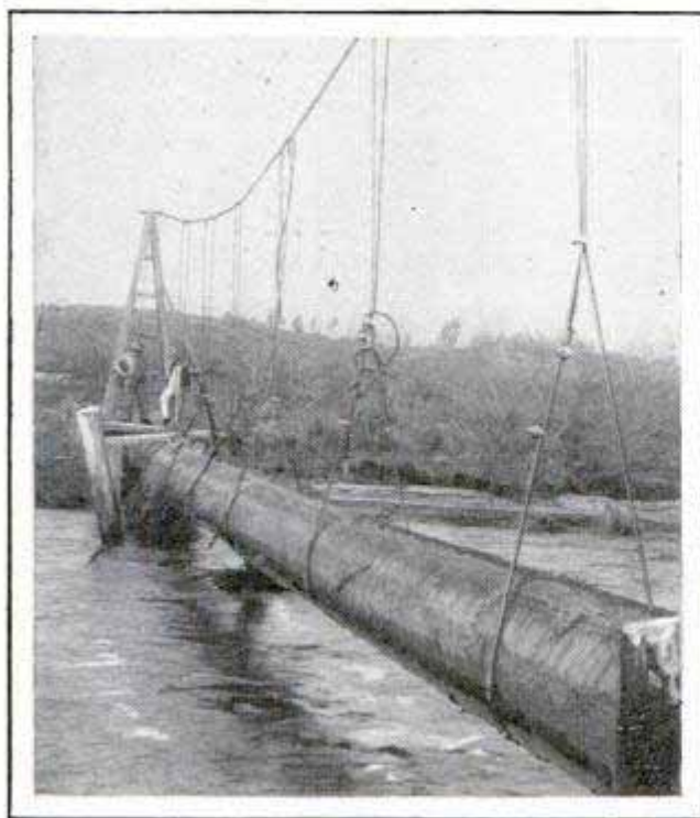
Sling Suspenders for the Pipe Line; It Failed to Break Although Unsupported for Some Time
