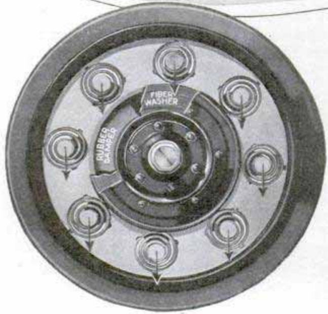
Car Equipped with Spring Wheels, and Another with Spring Bumper; the Inserts Show, Top, the "Spider" Which Distributes the Load to the Springs, and, Bottom, the Outer Side
