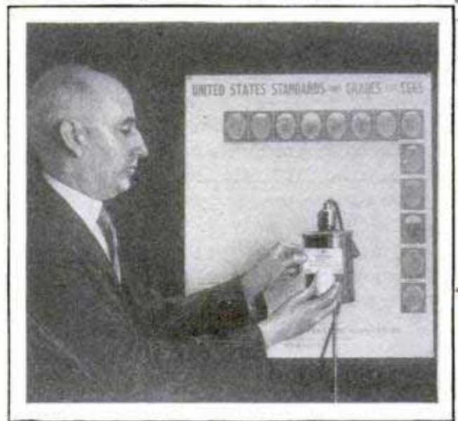
Grading an Egg by Measuring Its Air Space; Chart Behind Gives Diagrams of Different Qualities
