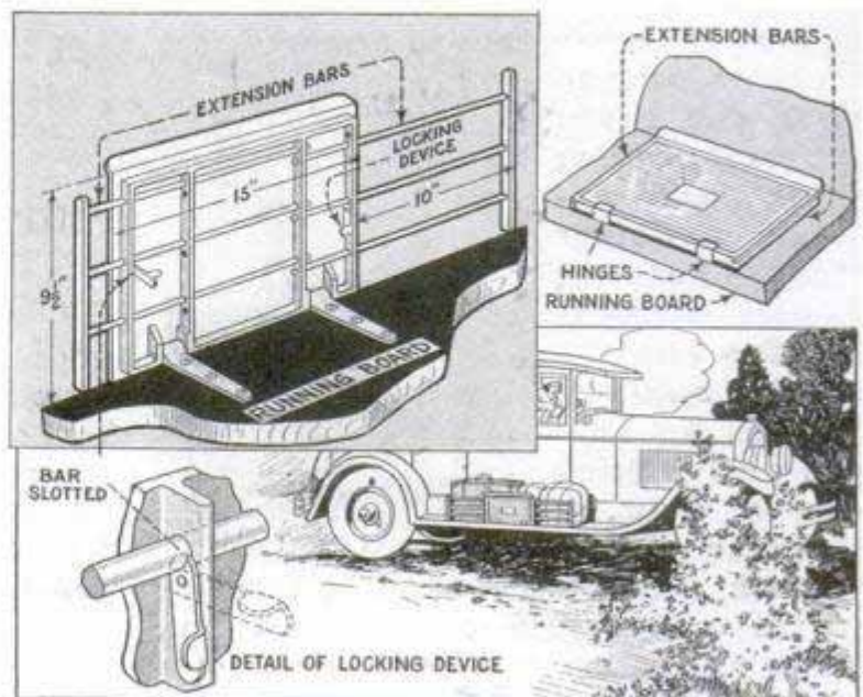
Diagrams of the Luggage Carrier Folded and Extended, and in Use on Auto Running Board
