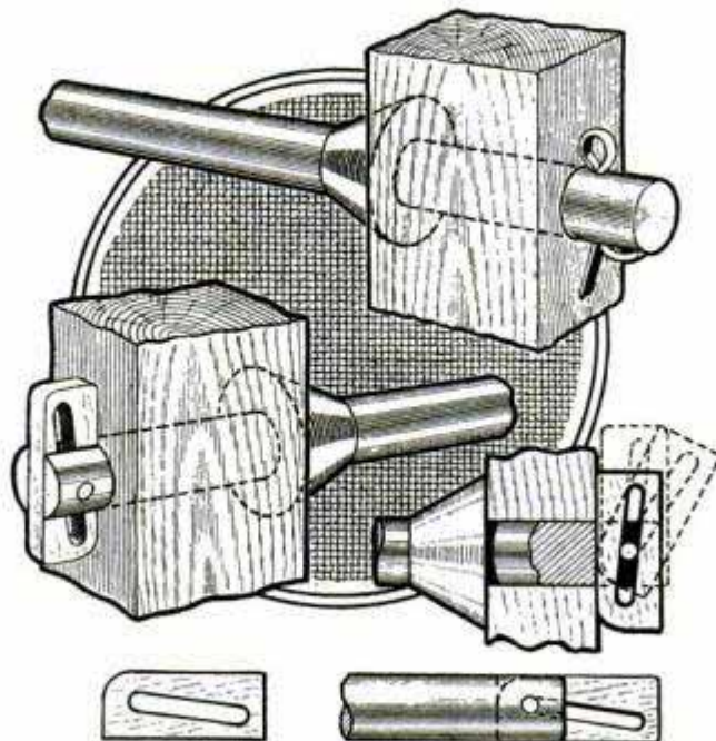
Quick-Acting Wedge Is Better Than Cotter Pin for Use with Portable Equipment
