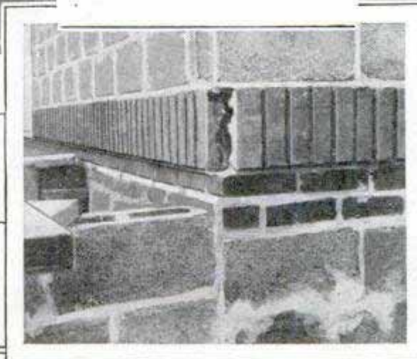
Right, the Correct Way to Corner a "Soldier" Course; Below, Difficulty Encountered When a "Soldier" Course Is Carried On to the Corner
