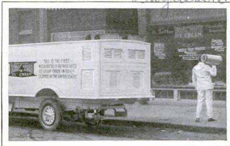
Ice-Cream Delivery Truck with Own Refrigerating Plant
