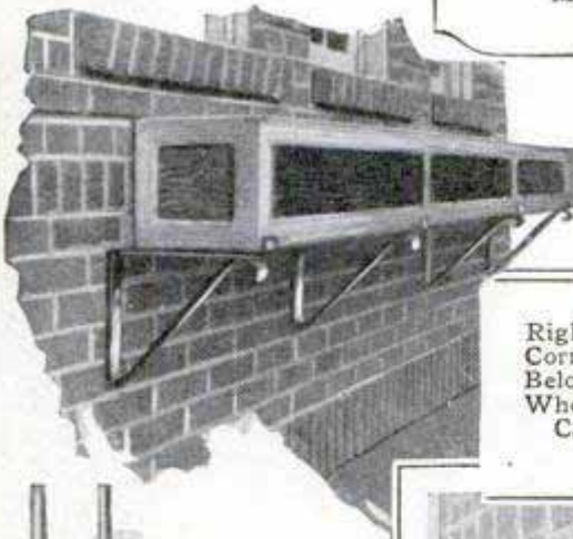
Simple Adjustable Scaffold for Store-Front Erection
