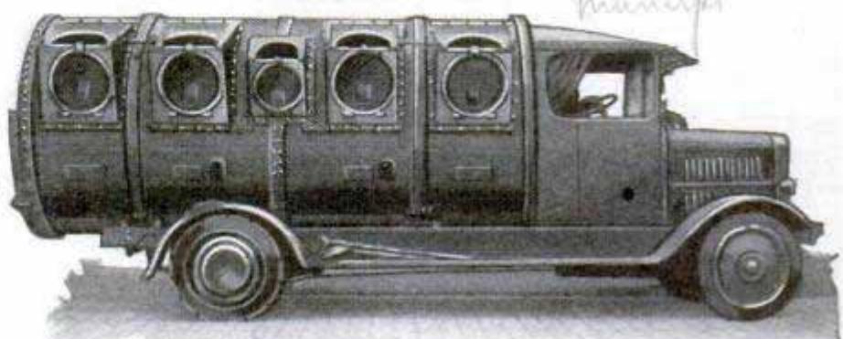
Armored Car for Hauling Street Rubbish; the Compartments Are Tightly Closed, to Prevent Scattering the Contents
