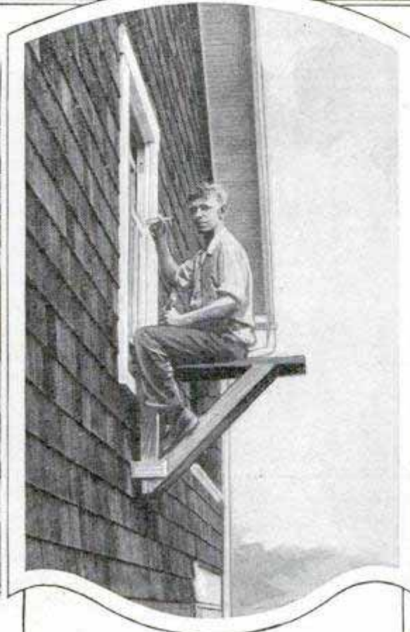
A Painter's "Cripple" That Makes the Painting of Trim Easier; a Couple of Lengths of Pipe Pass through the Members Projecting Inside
