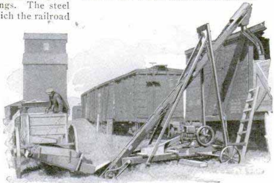
Unloading Grain from Wagon Directly into Freight Car with the Portable Elevator Outfit, a Useful Aid to the Farmer
