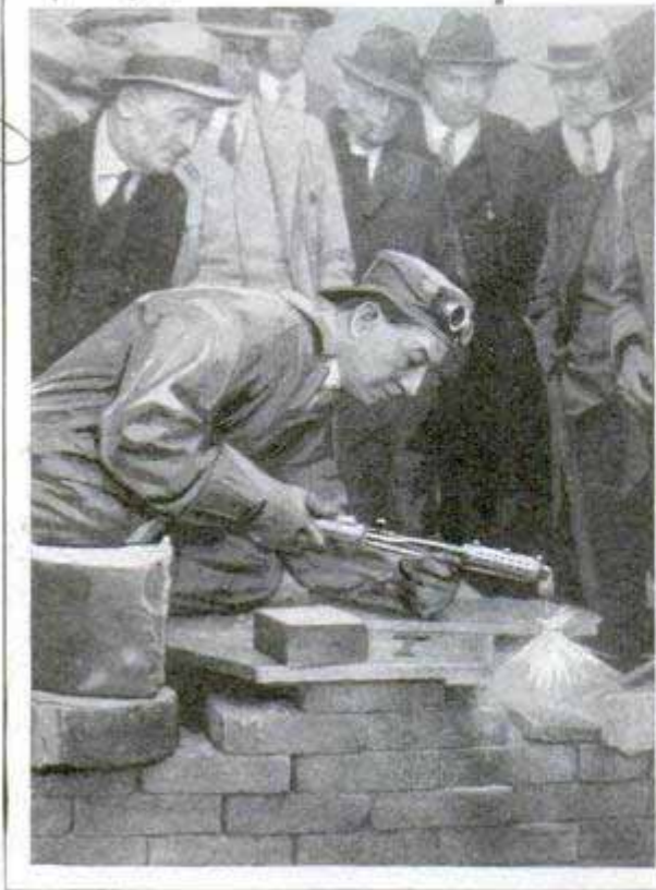
Demonstrating the Cutting Torch Which Uses Natural or Manufactured Gas; It Has a "Superheating" Unit
