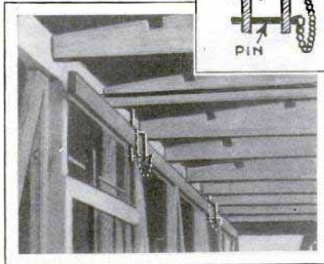
Handy Forked Hook Holds Support, Which Facilitates Fastening of Overhead Joists
