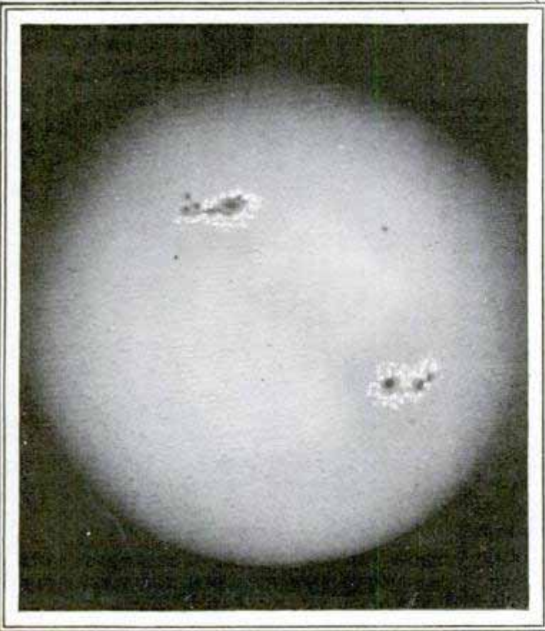
Enlarged Picture of a Sunspot, Above, Showing a Giant Whirling Tornado of Fire, Brighter than Any Flame on Earth, but So Dull Compared to the Rest of the Sun's Surface That It Photographs Black; the White Line across Its Center Is a Bridge of Calcium Flame, 20,000 Miles Long; at Left, a Pair of Sunspot Storms as They Appear in Relation to the Entire Disk
