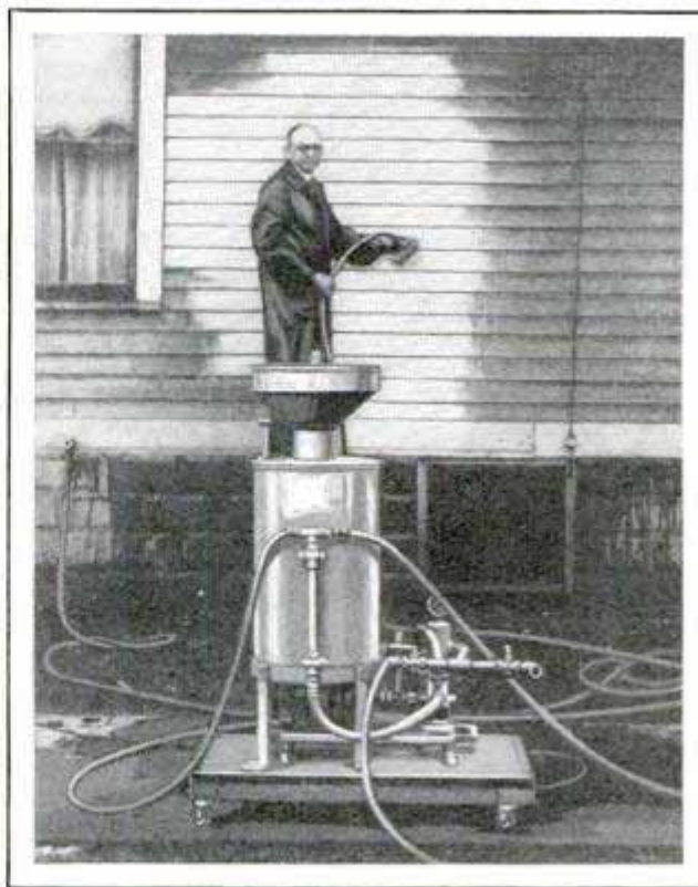
House-Washing Outfit and Sample of Its Work; Rinsing Is Done through Cleaning Nozzle
