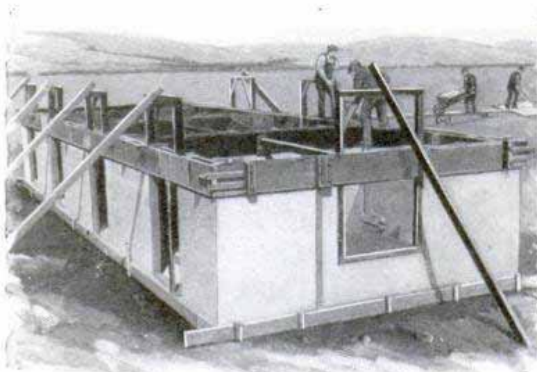
Where Lumber Is Scarce and a "One-Course" Concrete Form Has to Be Used
