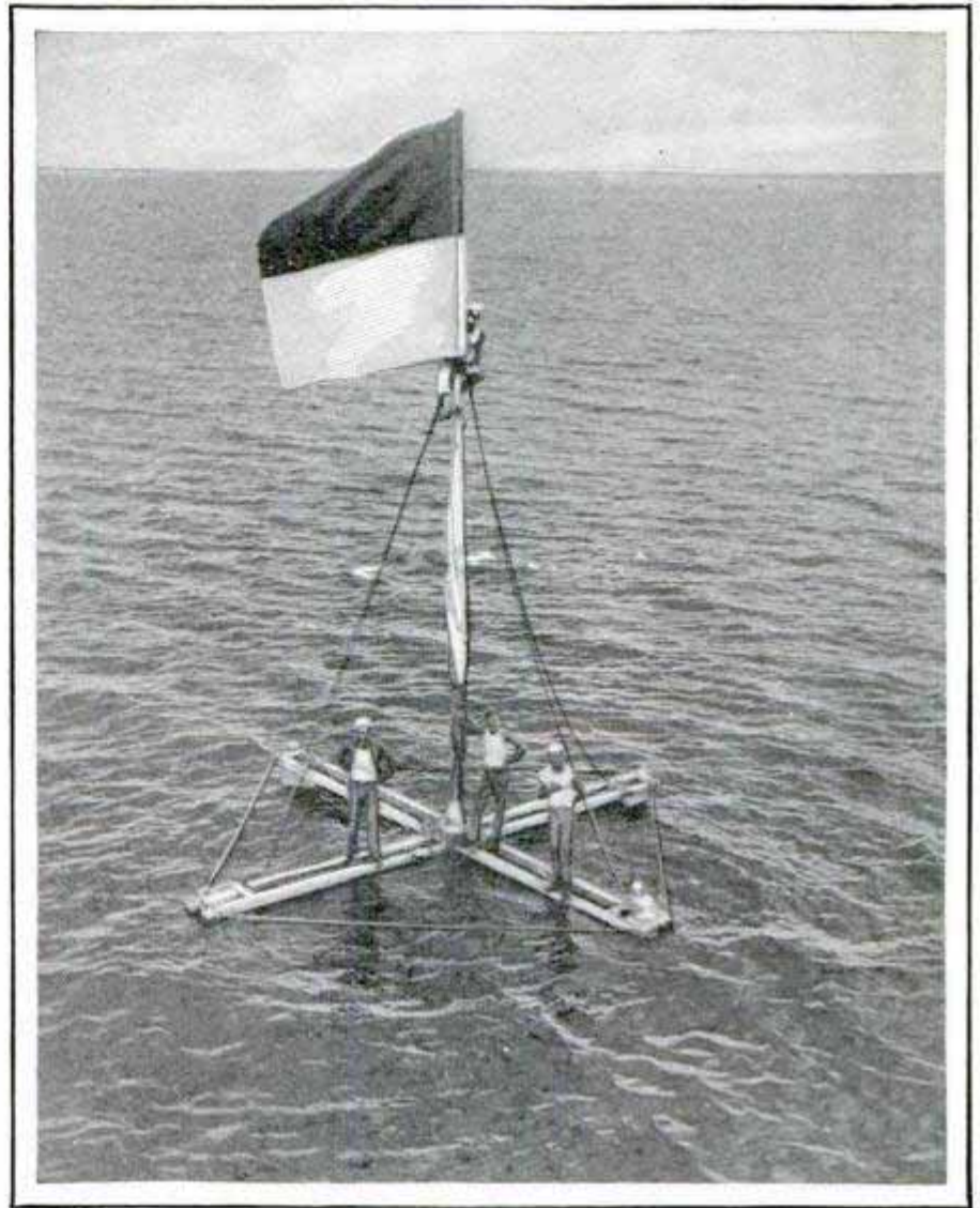
Floating Signal Launched and Anchored; the Survey Boats Get Their Exact Bearings from It for Several Miles Around
