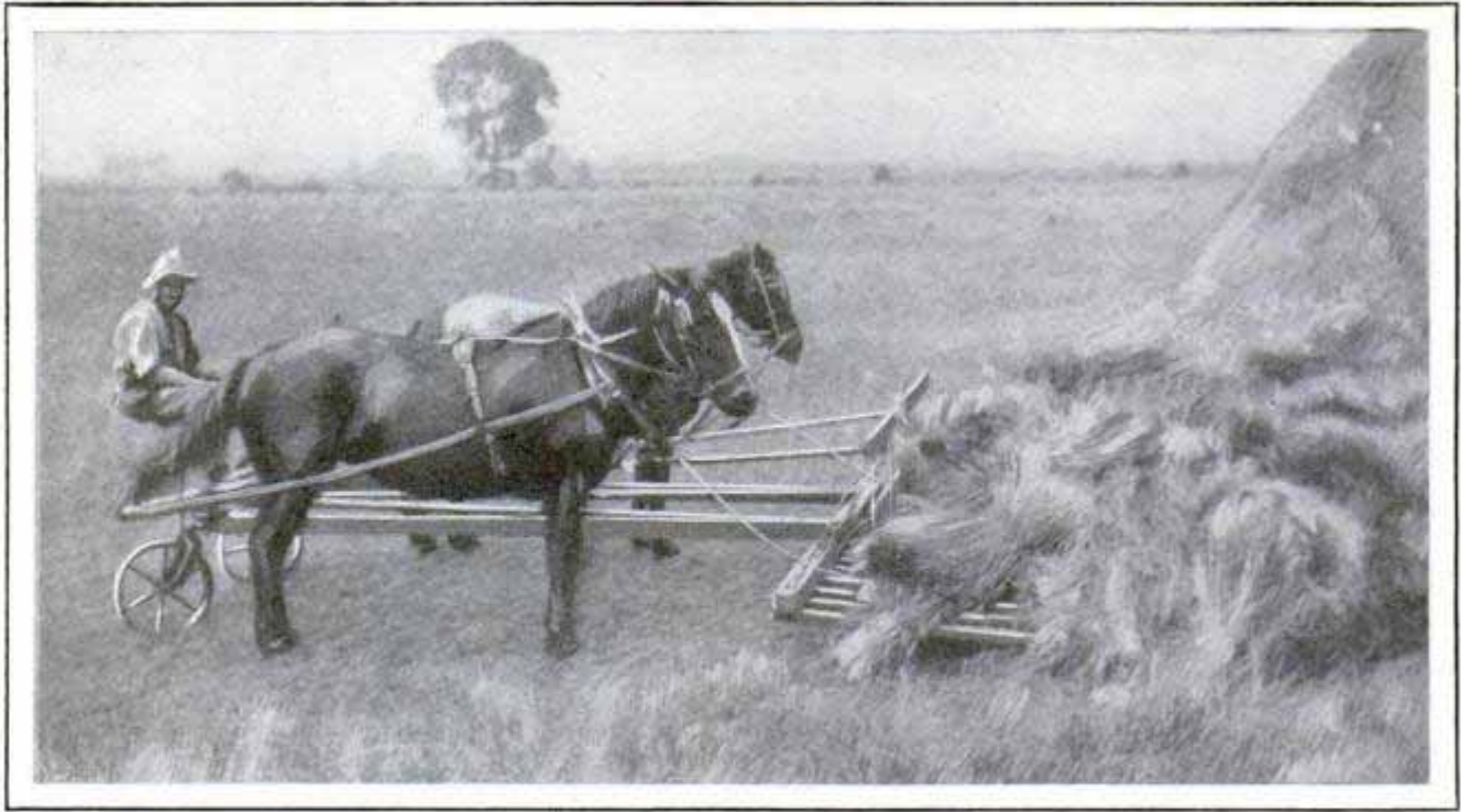
Improved Buck Rake, Attached to Tongue of Horse-Drawn Rig to Project in Front of Horses, Facilitates Raking Bundles to Thresher
