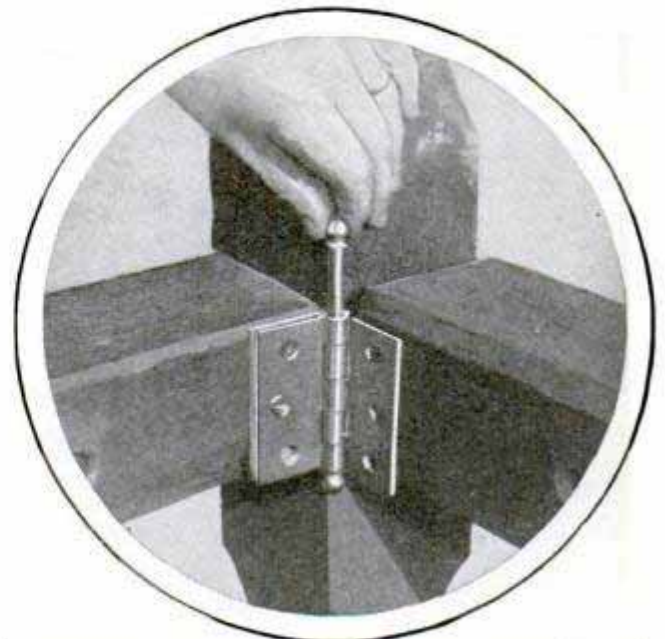
Loose-Pin Hinges on Old Beds Hold Sidepieces in Place Securely
