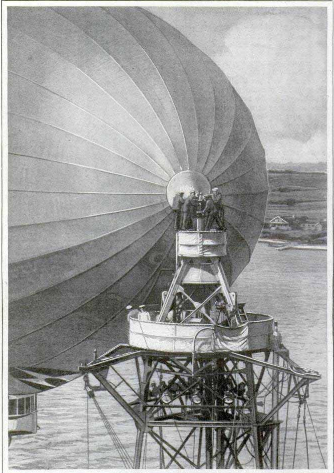
Anchoring the Nose Cone of the "Los Angeles" to the Cup on the Mooring Mast of the "Patoka," the World's Only Floating Landing Field for Airships; the Lofty Mast Is Ascended by Elevator
