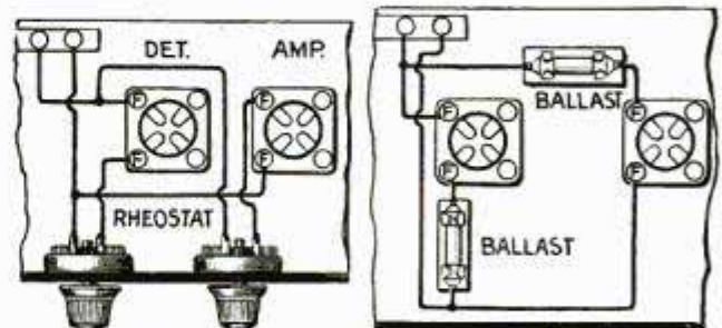
Left, Detector and Amplifier Tubes Controlled with Rheostats; Right, Automatic Filament Control
