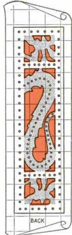
Patterns for the Lead Overlays of the Chinese Box; the Squares Are One-Fourth the Size of Those in the Finished Job
