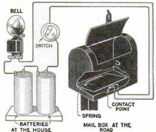
Electric Bell Rings in House When Mail Is Deposited in the Box
