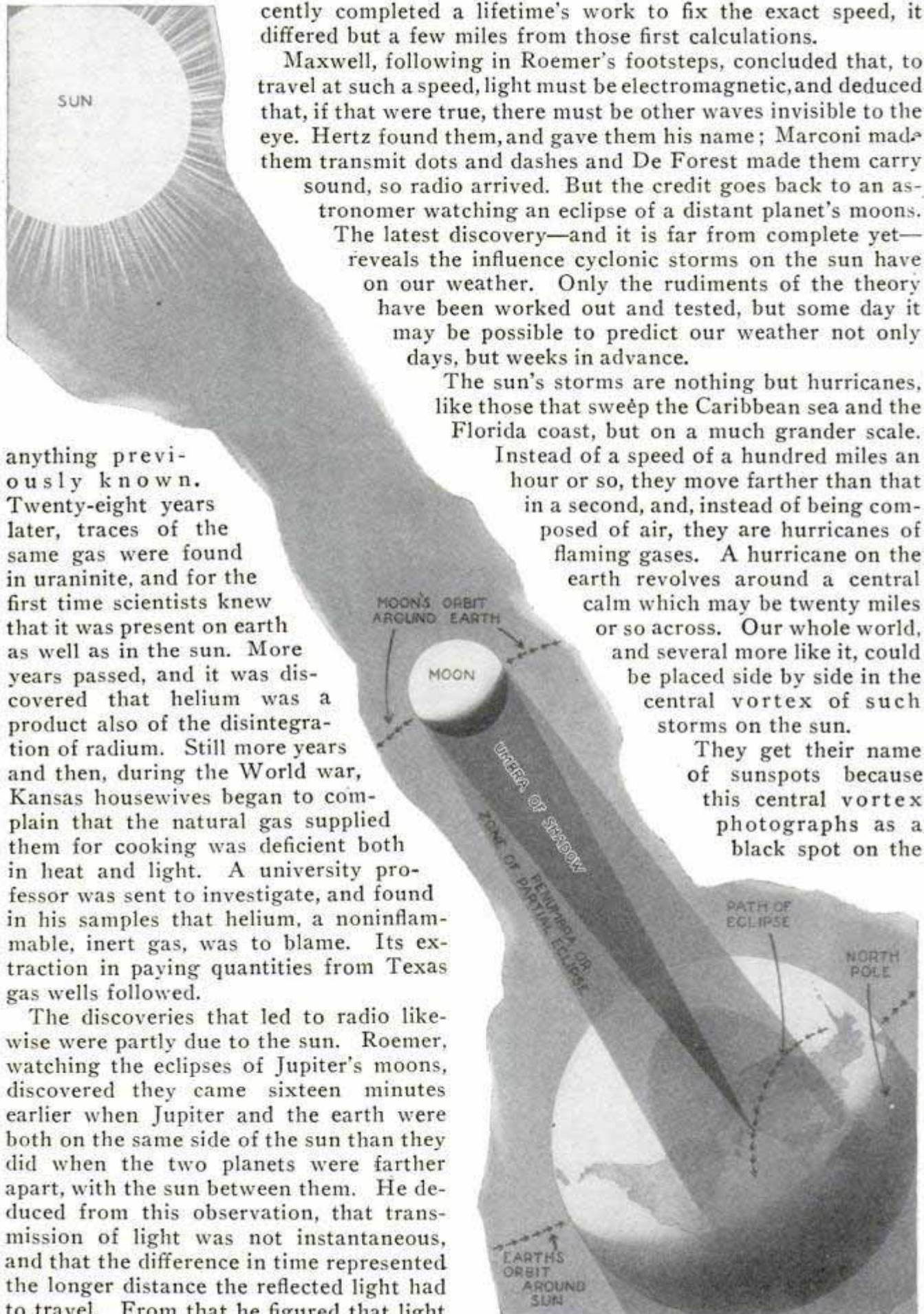
What Happens When the Moon Passes between the Sun and the Earth, and Eclipses the Former; the Zone of Total Darkness Is About Fifty Miles Wide
