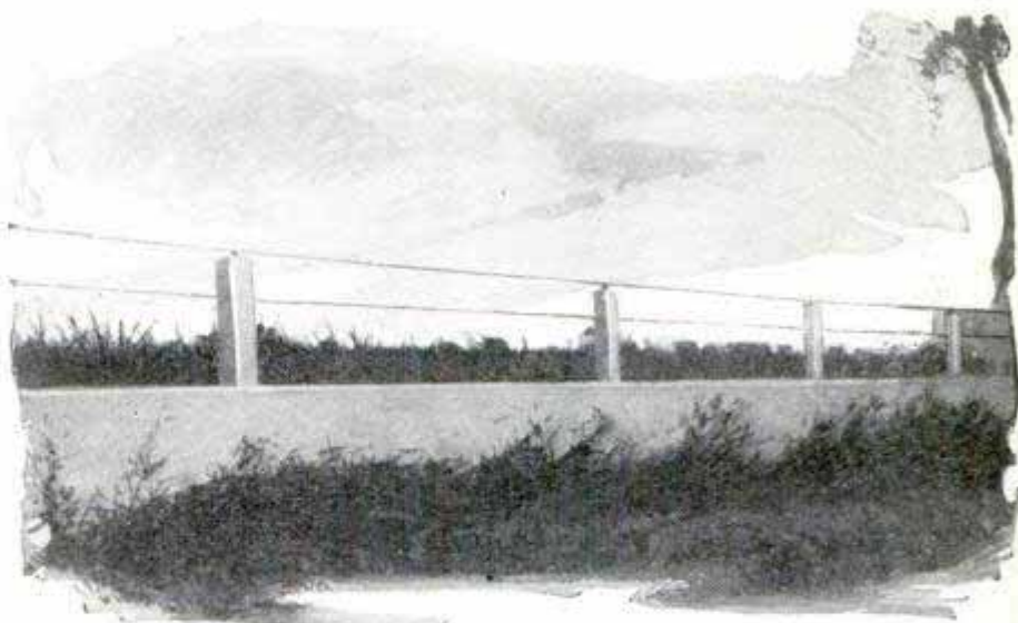
Lower Part of Fence around Pasture Field Built of Concrete to Keep Sheep and Hogs from Getting Through
