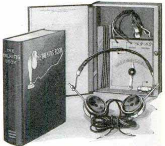
Small Crystal Set Contained in a Cloth-Bound Box Made to Resemble a Book
