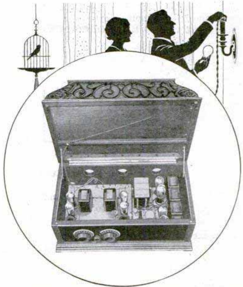
Power Unit and Receiver Combined; the Loud Speaker Is Built into the Lid of the Cabinet
