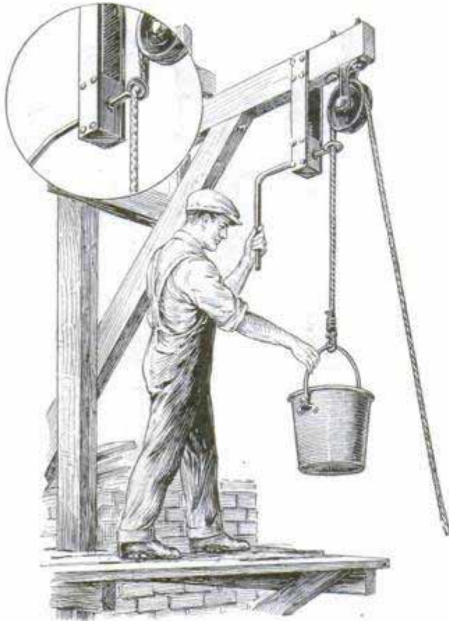
Emergency Brake on Hoisting Rope Helps Avoid Accidents in Building Construction
