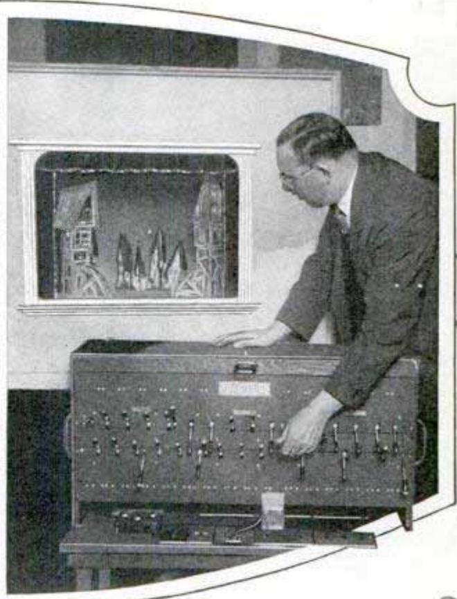
Miniature Stage and Lighting System Save Time and Expense in Planning Effects for Real Plays; a View behind the Scenes and the Control-Switch Box
