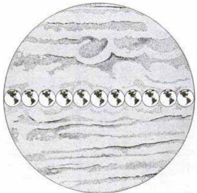
Our Earth Is a Tiny Thing Compared with Jupiter, Also a Satellite of the Sun
