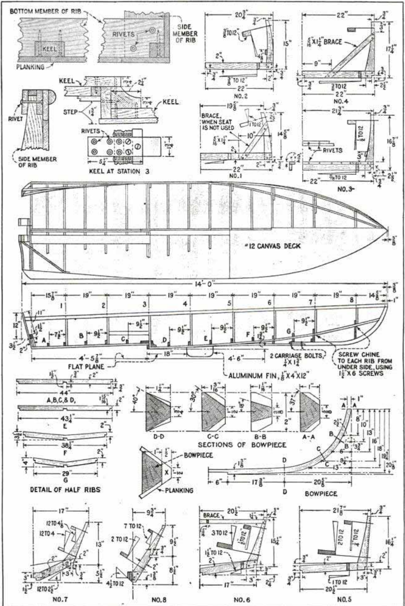
Constructional Details of the Hull of the Hydroplane; Any Boatbuilder Can Assemble a Speed Boat from These Plans, and Even the Amateur Will Not Find It a Difficult Task
