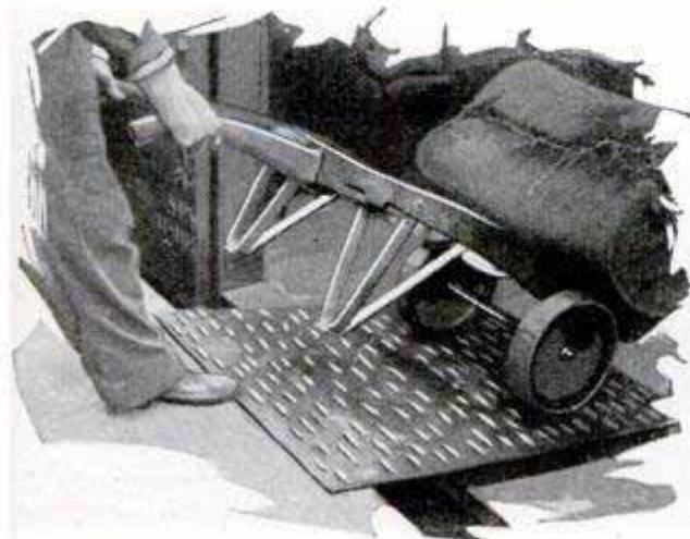
Ribs Welded on Surface of Loading Plate Prevent Trucks from Skidding on It
