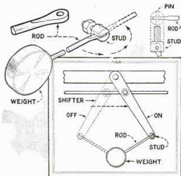
Safety Device for Shifter Handle That Prevents Machine from Starting Too Easily
