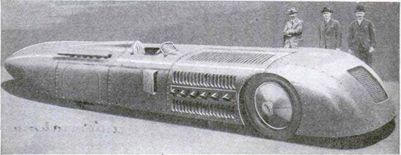
More Than Thirty Feet in Length, This Double-Engine, 1,000-Horsepower Racer Is Expected to Travel Faster Than 200 Miles an Hour over the Sands at Daytona Beach
