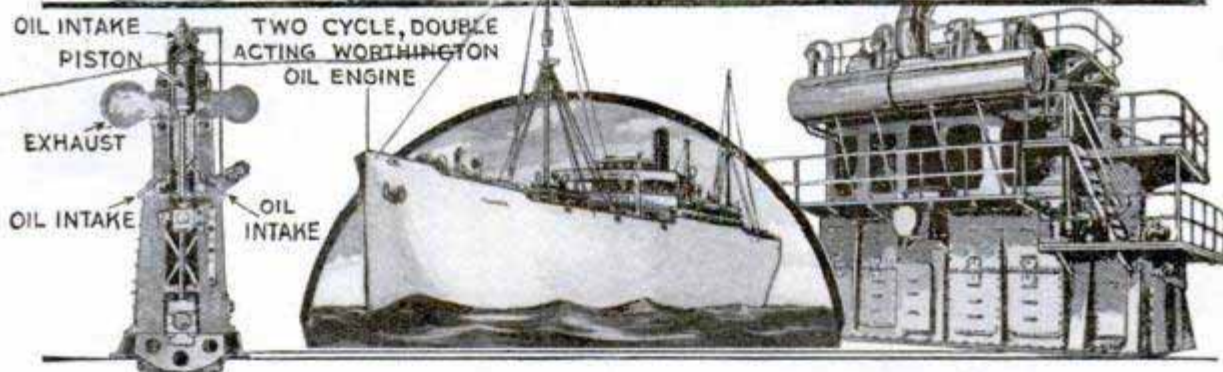
The "Tampa," First Motorized Shipping-Board Vessel with Its All-American Diesel Engine, and Sketch Explaining the Worthington Principle, with Designer's Idea of Car Using It
