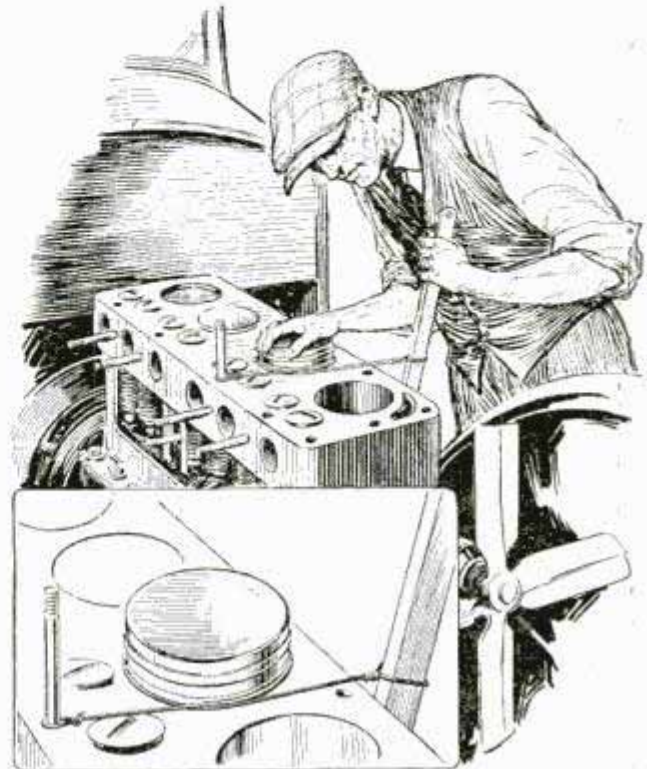
Effective Method of Compressing Piston Rings with Length of Baling Wire
