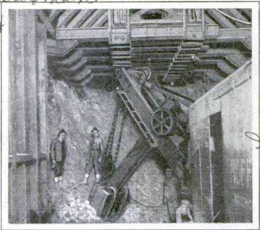
How the Steel "Rib" Holds Up Mountain While Men Pierce Continent's Backbone; Scene in Moffat Tunnel
