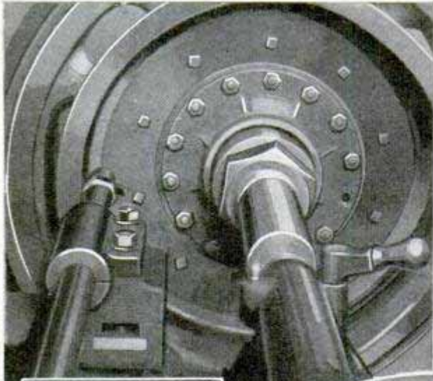
Close-Up of Job at Right, Showing the Type of Tool and Arbor Used
