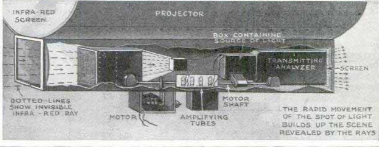
Copyright, The Illustrated London News Using Invisible Infra-Red Rays and a Fluoroscope as a Receiving Screen, an English Inventor of Television Apparatus Has Developed an Invisible Searchlight for War Use
