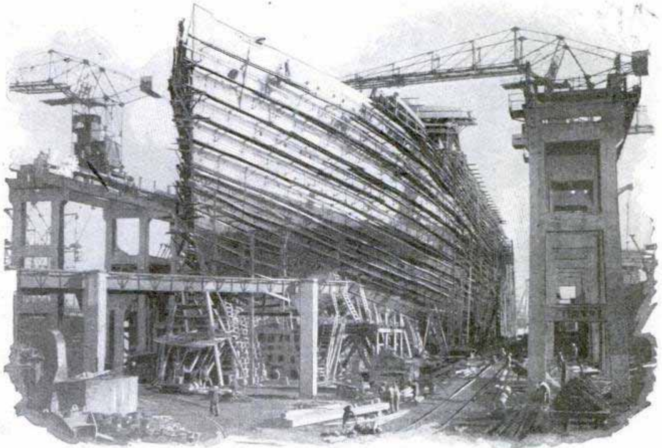
Shortly before the Launching, the Giant Hull of the Steamer "Vulcania," on the Ways at Monfalcone, Italy; Special Steel of High Elastic Properties Was Used in Constructing the Boat
