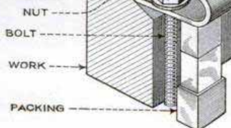
Simple Strap Used to Hold Tapered Work on Machine Table
