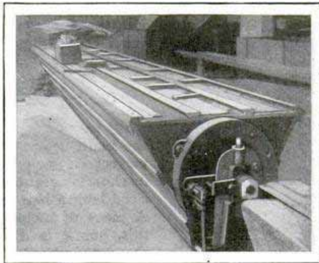
Triangular Gluing Table Rotates on a Horizontal Shaft and Triples Output
