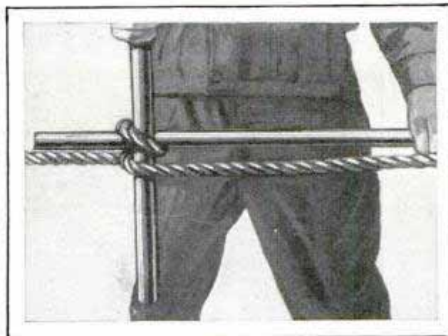
Considerable Force Can Be Exerted with This Improved Windlass
