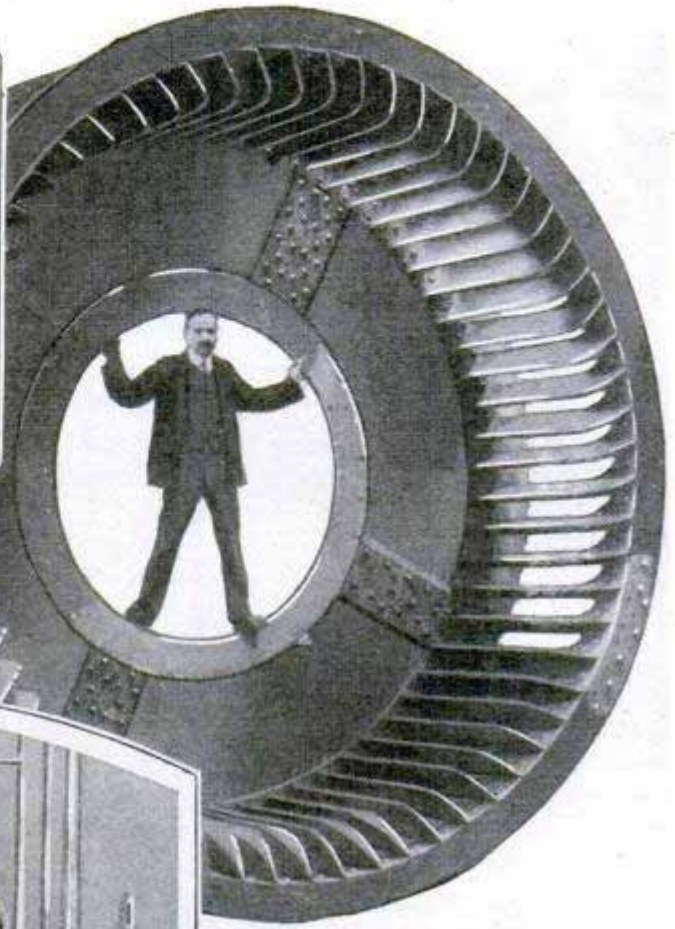
Part of a Fan Capable of Pumping Twenty-Five Tons of Air a Minute, Built for a South African Coal Mine, Is Shown Above, and Below Is Its Huge Rotor Being Assembled Previous to Factory Test
