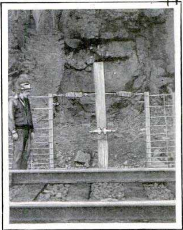
Alarm Fence on Union Pacific Railroad, Which Sets Signal When Rock Slides Strike It
