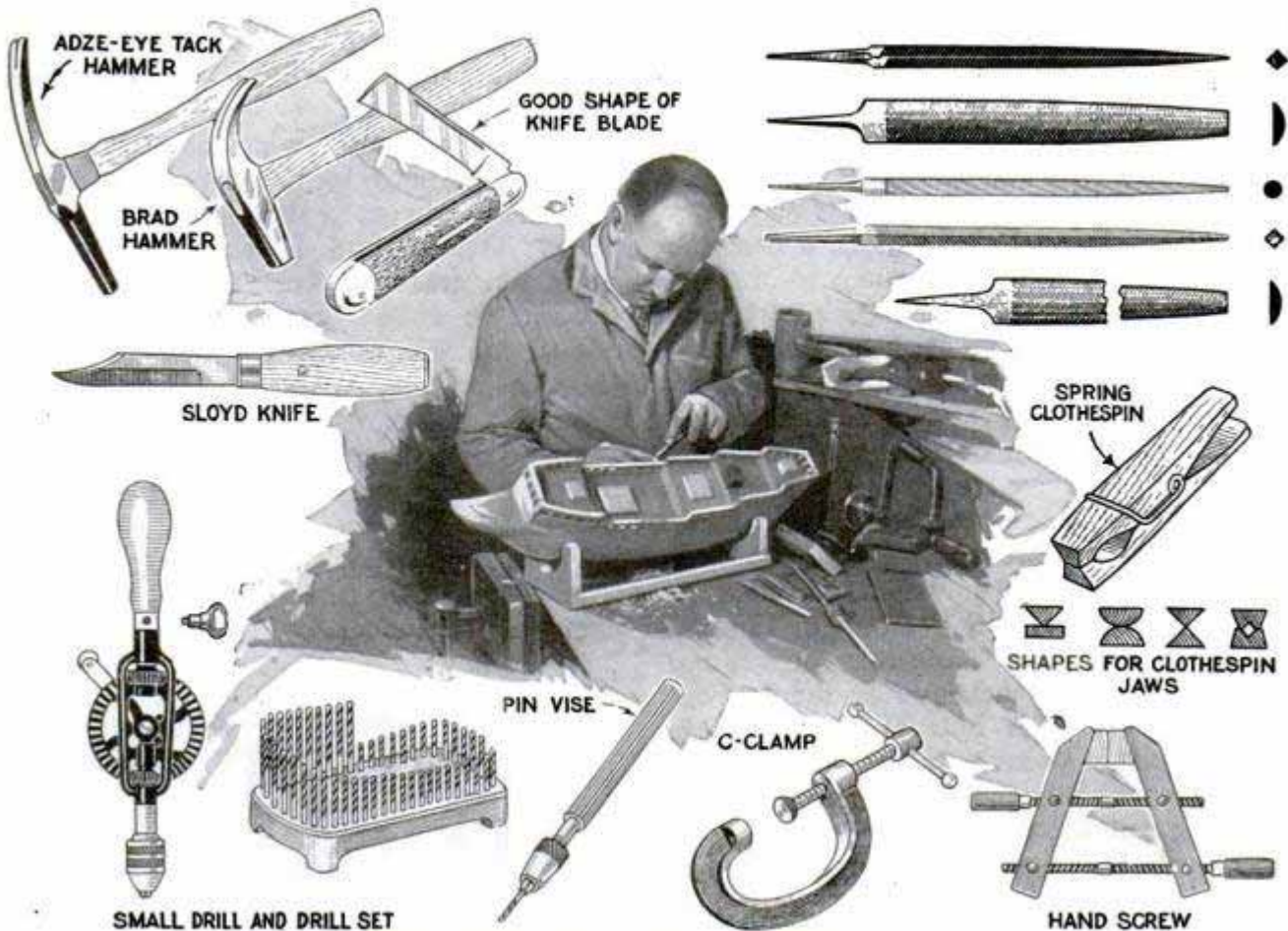
The Pin Vise and the Homemade Clothespin Clamps Are Indispensable in Gluing and Drilling Small Parts; the Knife Blade Will Also Be Found More Useful When Honed to the Shape Shown
