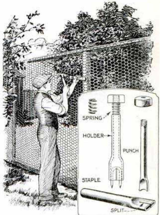
Staple Driver Made from Bolt and Pieces of Metal Tubing Saves Time and Sore Fingers
