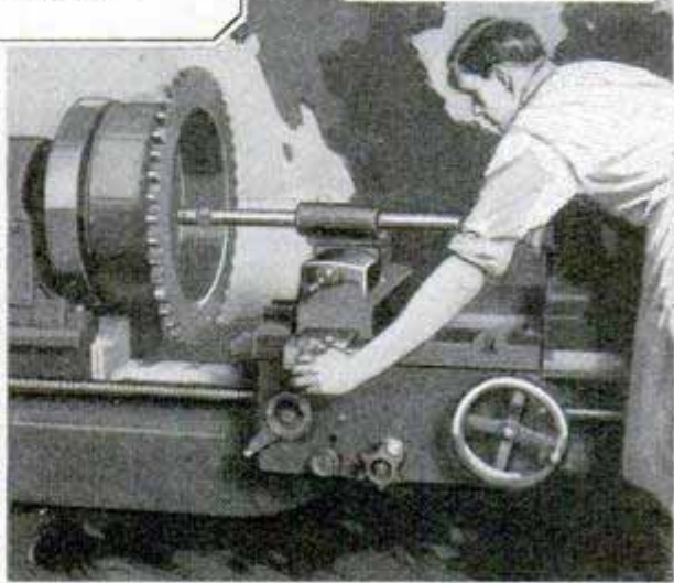
Truing Brake Drum on a Chain-Drive Truck Wheel
