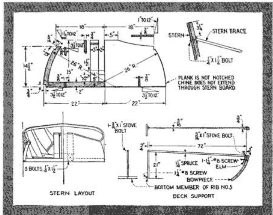
Layout of Stern, Showing Frame and Bracing; Right, Support for Canvas Deck, Which Extends over Forward Part of Hull
