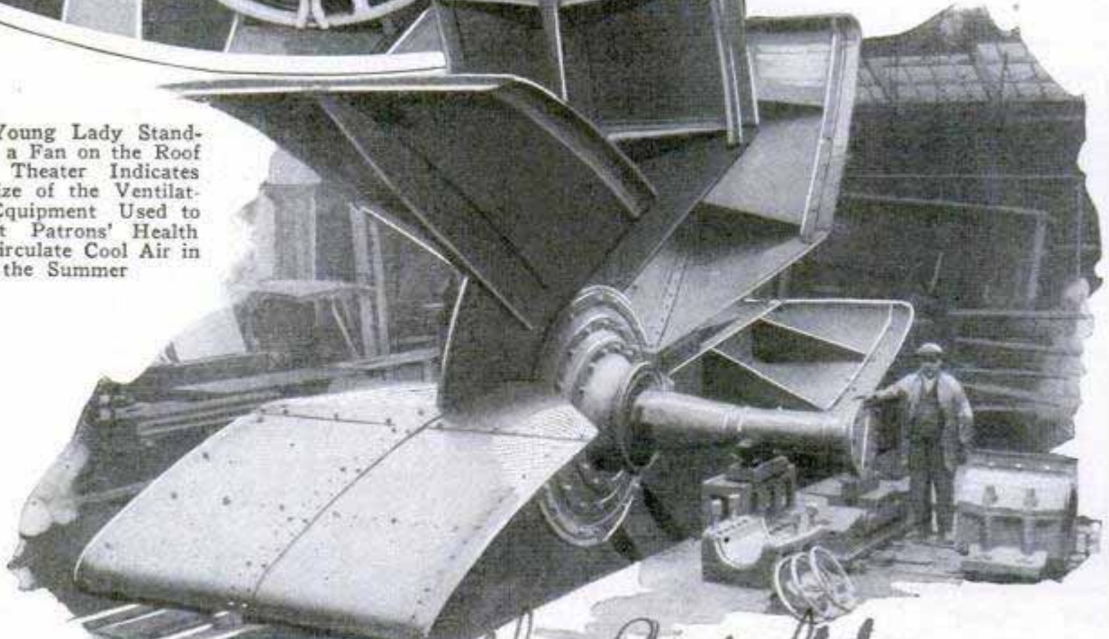
Part of a Fan Capable of Pumping Twenty-Five Tons of Air a Minute, Built for a South African Coal Mine, Is Shown Above, and Below Is Its Huge Rotor Being Assembled Previous to Factory Test
