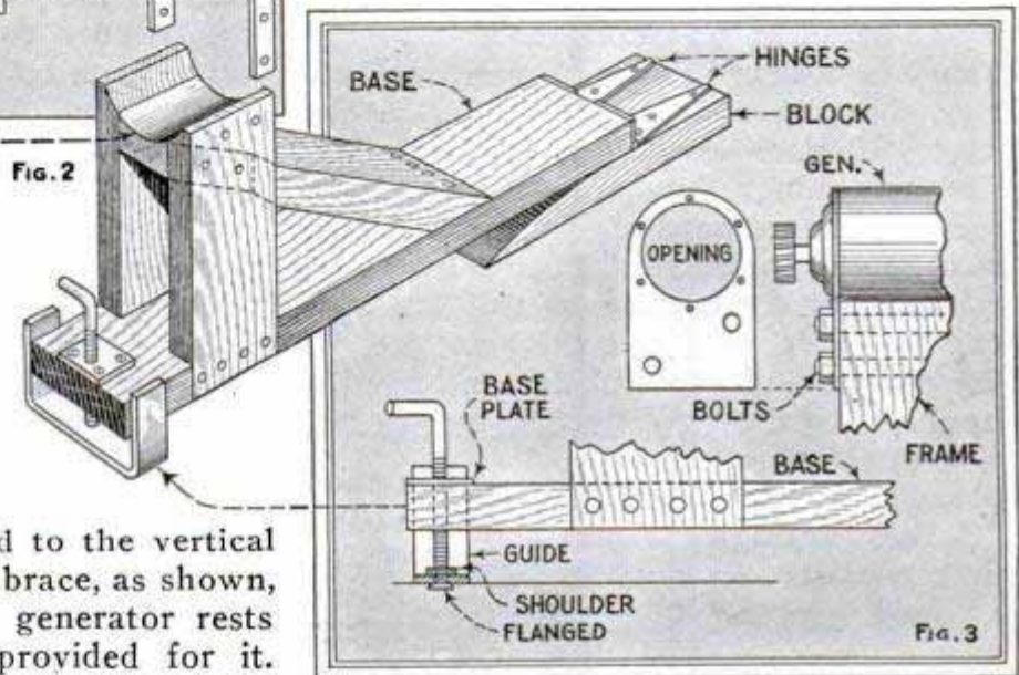
Details of Generator Mounting and Fitting for Disengaging Drive When Generator Is Not Wanted
