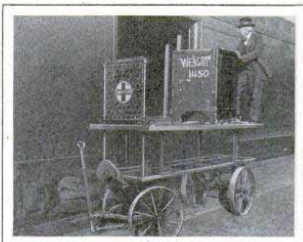
Safe Lifted to Level of Baggage Car on Elevator Truck for Easy Loading
