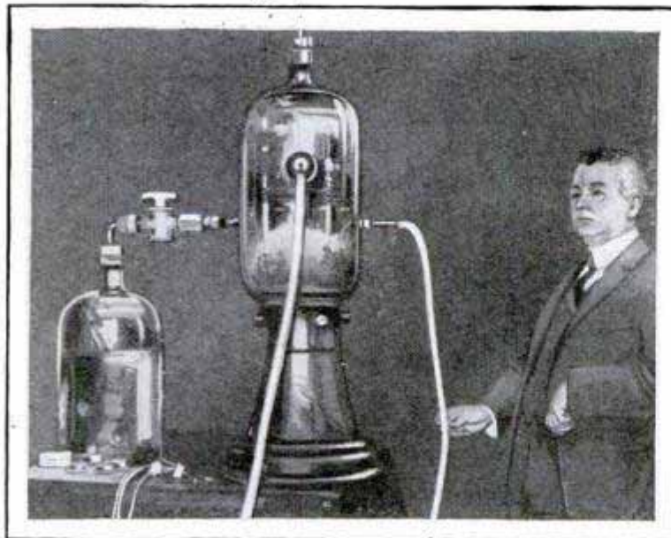
© Herbert Photos Test Apparatus Which Produced Steam to Run Turbine and Light Small Electric Lamps for a Few Minutes
