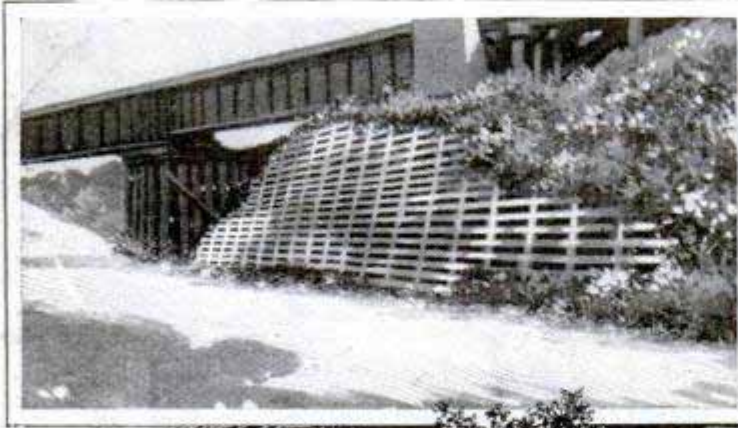
New Type of Concrete Wall, Used on Highways to Prevent Earth Embankments from Washing Out or Breaking Down over the Road, Is Built Up of Slabs, Which Provide Strength and Insure Proper Drainage
