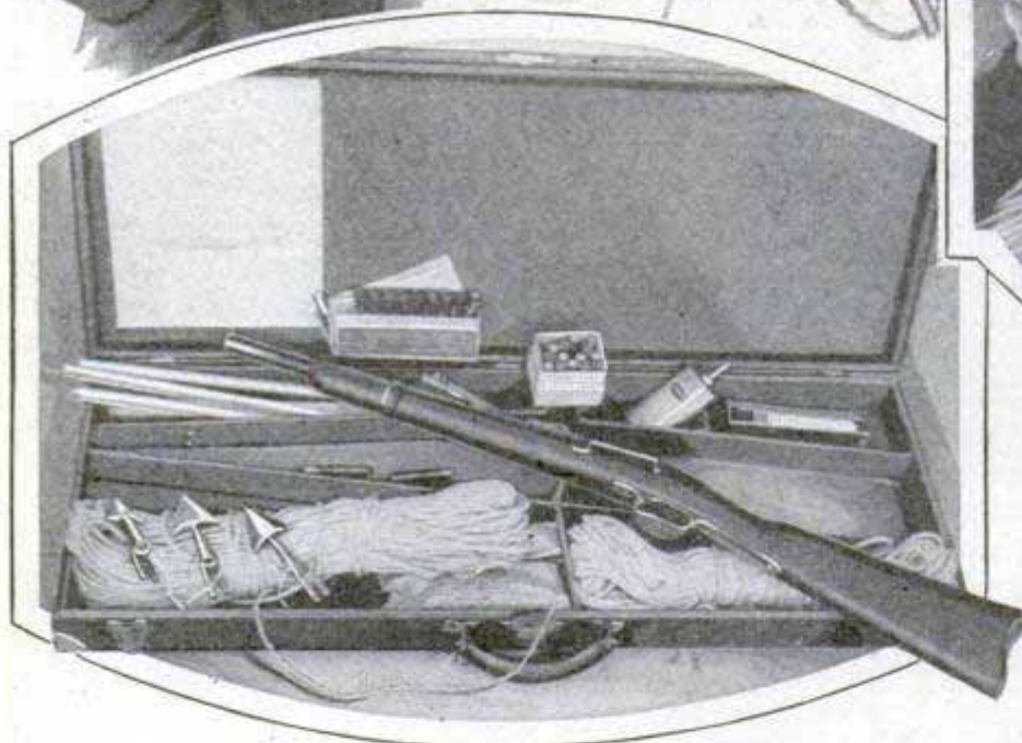
Old Army Carbine Converted into Harpoon Gun for Fishing; Close View of Dart and the Entire Outfit
