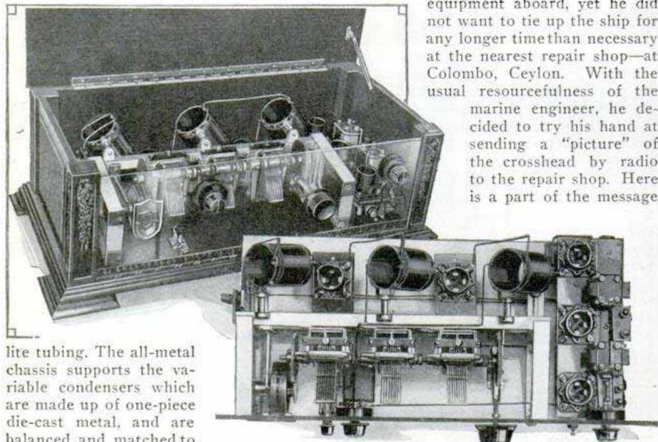
Above, Set as It Appears in the Display Cabinet with Glass Front Panel; Below, Complete Unit Assembly Removed from the Cabinet
