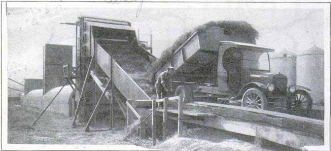
Dumping a Truck Load of Hay onto the Conveyor Which Carries It to a Cutter, and Then Delivers the Shredded Fragments to a Belt Moving through the Drying Tunnel, from Which It Emerges Cured
