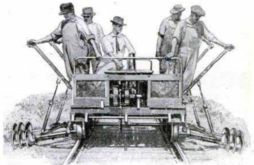
Disk Weeder and Ballast Shaper in Operation on Railroad; the Cutters Are Adjustable to Different Angles and Lengths
