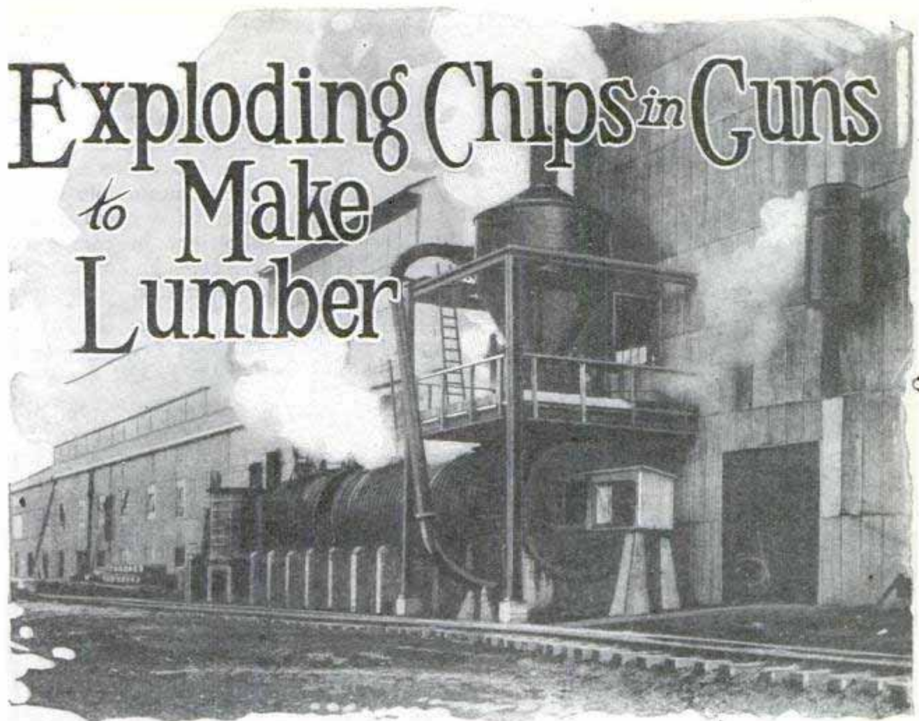
Where the Steam Is Allowed to Escape from the Pulp Material after "Firing" from the Guns; the "Cyclone" at the Wood-Waste Salvage Plant
