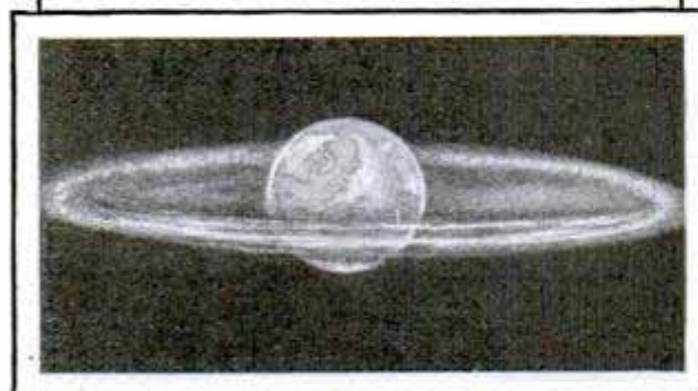
German Scientists Are Interested in a New Theory That Our Earth May Have a Luminous Ring like Saturn's, an Idea That Explains the Ghostly Zodiac Light
