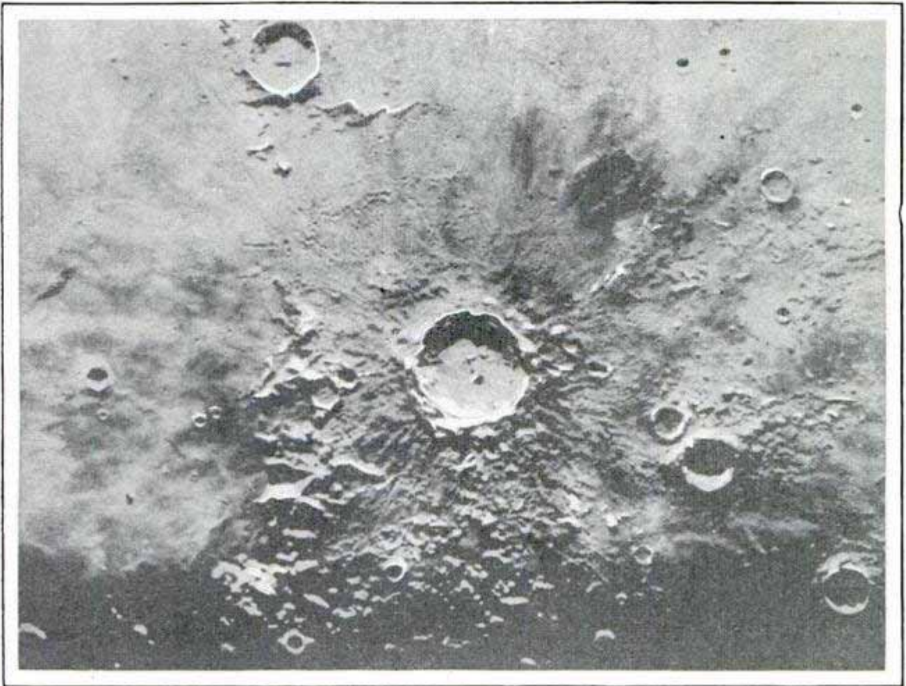
The Crater Theophilus on the Moon Is the Central Depression; the Vast Hole Is 18,000 Feet Deep, and the Central Mountain, Which Casts the Black Shadow, Stands 10,000 Feet High
