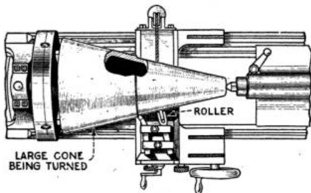
Simple Method of Turning Large Cone on a Lathe
