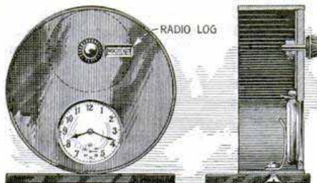
Left, Front View of Completed Unit, Station-Logging Disk Indicated by Dotted Lines; Right, Section
