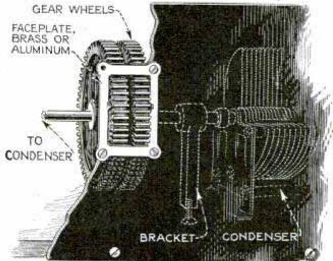
Homemade Back-Mounted Dial That Can Be Easily Made at Small Cost
