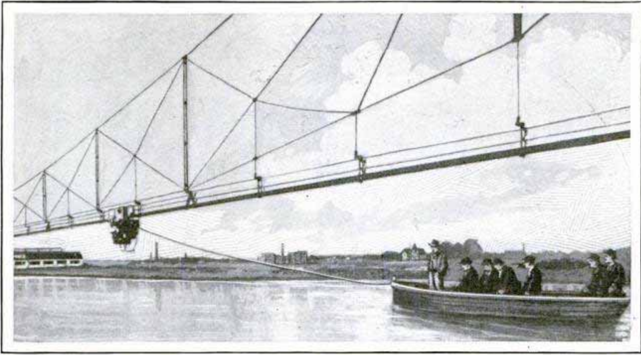
As the Monorail Tug Would Appear over Water; the Experiments Were Conducted with a Boat Load of Persons on a Grass Plot, and Proved Successful
