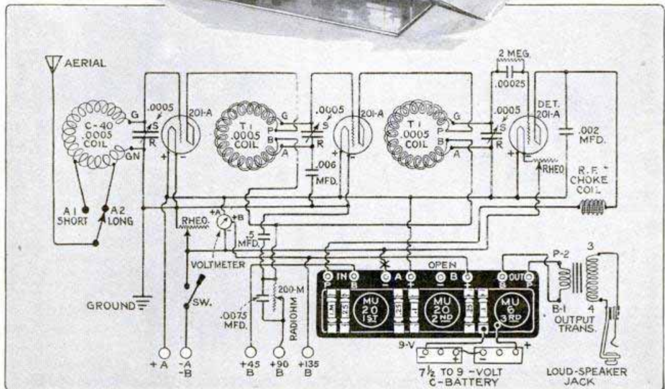
Above, Partly Assembled Panel and Subpanel; Below, Schematic Diagram of Set for Those Who Prefer to Work from One of This Type
