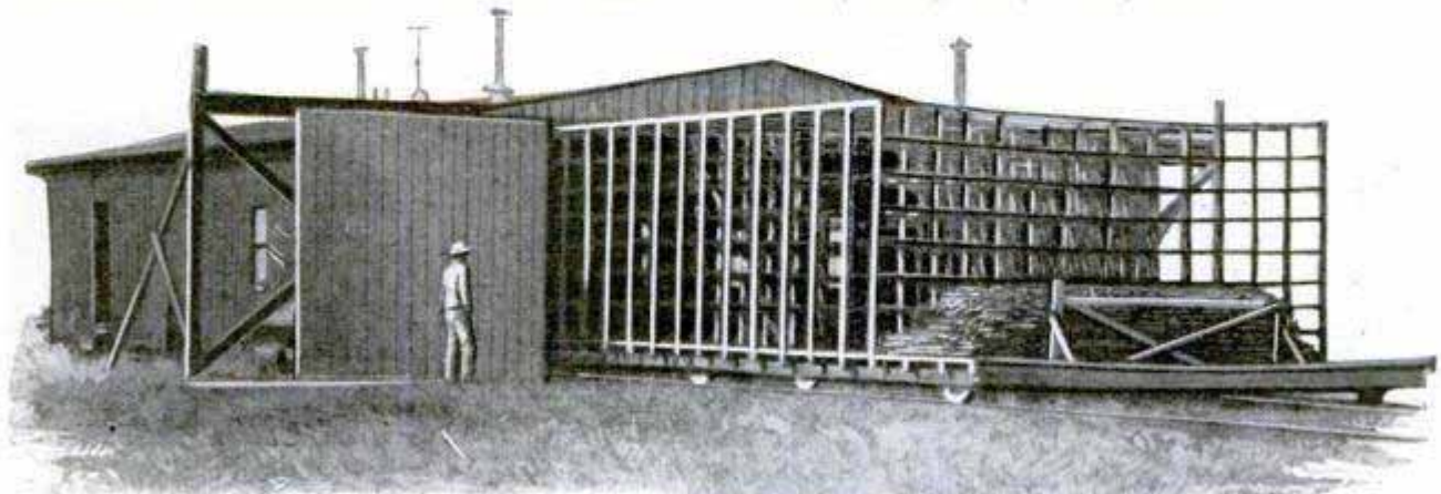
Drying Sheds Are Built like Huge Aircraft Hangars, with Racks That Run on Railroad Wheels and Track, and Each Capable of Holding Many Thousand of the Pelts
