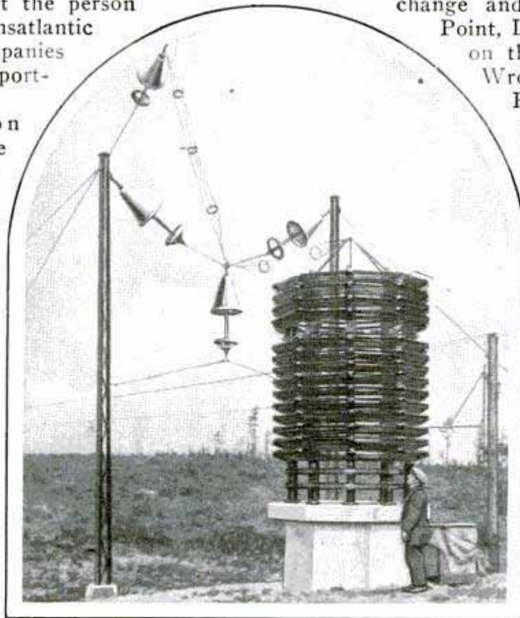
Where American Words Take the Air; the Outdoor Tuning Inductance at the Rocky Point Transmitting Station on Long Island
