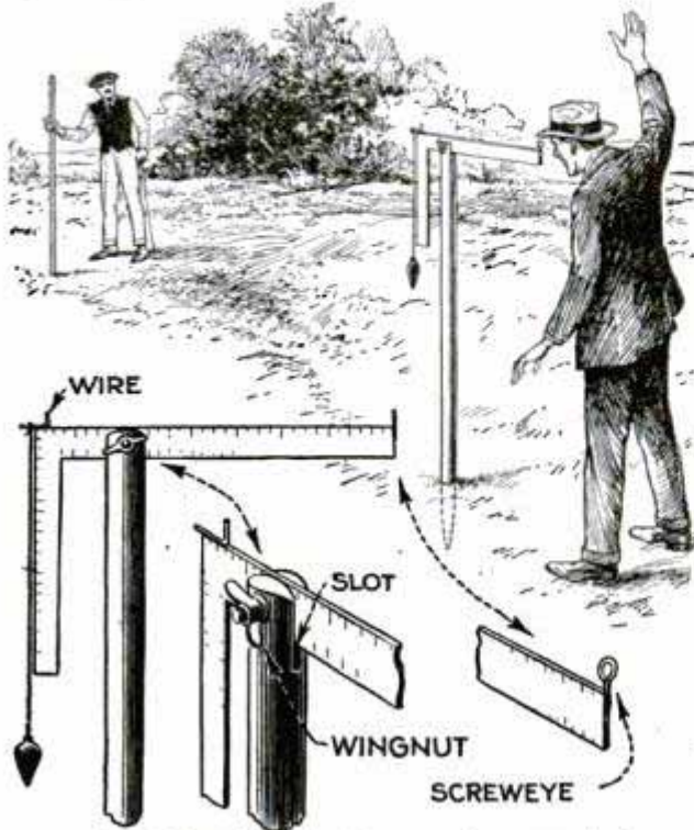
Improved Level Made from a Carpenters' Square Proves Satisfactory for Farm Use
