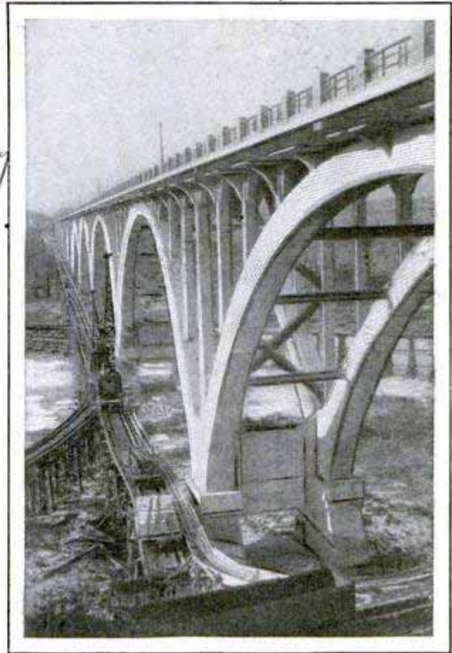
Concrete Arches of the Memorial Bridge between Fort Snelling and Mendota, Minnesota
