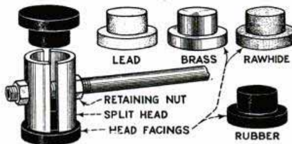
Shop Maul Fitted with Interchangeable Head Facings for Different Uses
