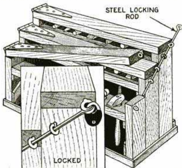
A Padlock, a Steel Rod and Some Screweyes Securely Lock This Tool Rack
