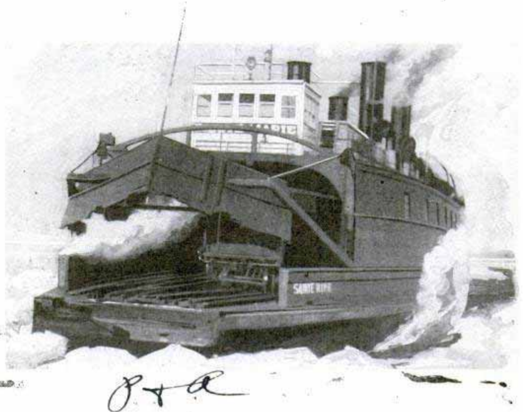
Car Ferry "Sainte Marie" with Its Plow Raised Ready for an Attack on the Ice Jam in the St. Mary's River; for a Time, the Blockade Threatened to Trap the Crusher
