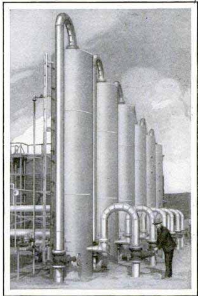
Big Plant Where Gasoline Is Absorbed from Domestic Gas; General View of Extracting Units
