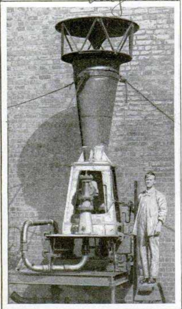
Fog Horn That Produces the World's Most Terrible Noise and Can Be Heard Forty Miles
