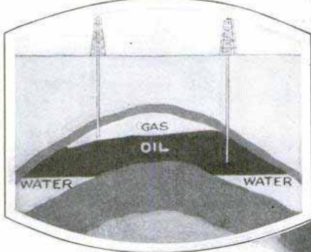
Showing How Gas Can Be Forced down the Well at the Left to Increase the Subterranean Pressure and Drive the Oil up the Well at the Right; at Right Is a New Style Drill That Sinks and Reams a Twenty-Four Inch Hole, While the Top Rollers Enable It to Cut Its Way Back Up through a Cave-In
