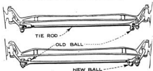
Repair on Ford Tie-Rod Eliminates Expense of Purchasing a New One
