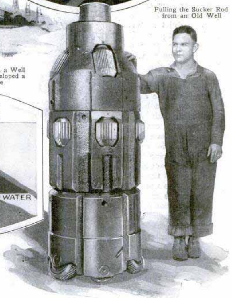
Showing How Gas Can Be Forced down the Well at the Left to Increase the Subterranean Pressure and Drive the Oil up the Well at the Right; at Right Is a New Style Drill That Sinks and Reams a Twenty-Four Inch Hole, While the Top Rollers Enable It to Cut Its Way Back Up through a Cave-In
