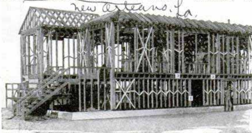
Specially Braced Framework Intended to Reduce Damage in Case of Severe Winds; an Outcome of Recent Hurricanes
