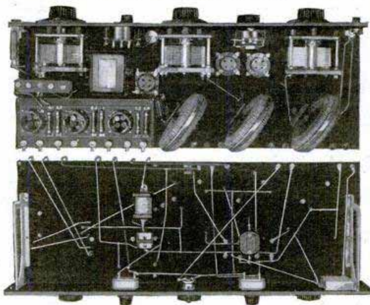
Top and Bottom Views of the Completed Receiver; Note the Angle at Which the Coils Are Set
