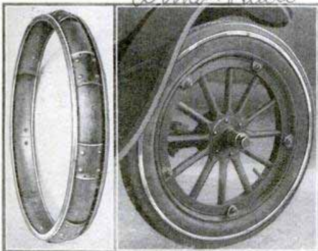
Tire Armor at the Left and Assembled at Right, Showing Outer Strip of Hard Rubber
