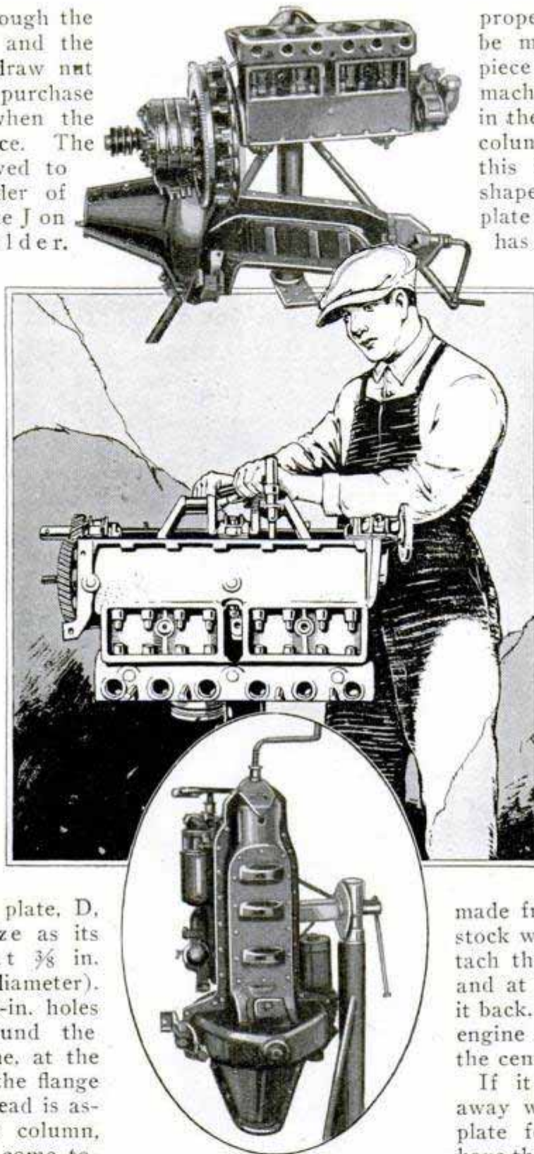
Two Views of the Stand in Use, Showing How the Engine May Be Swung
