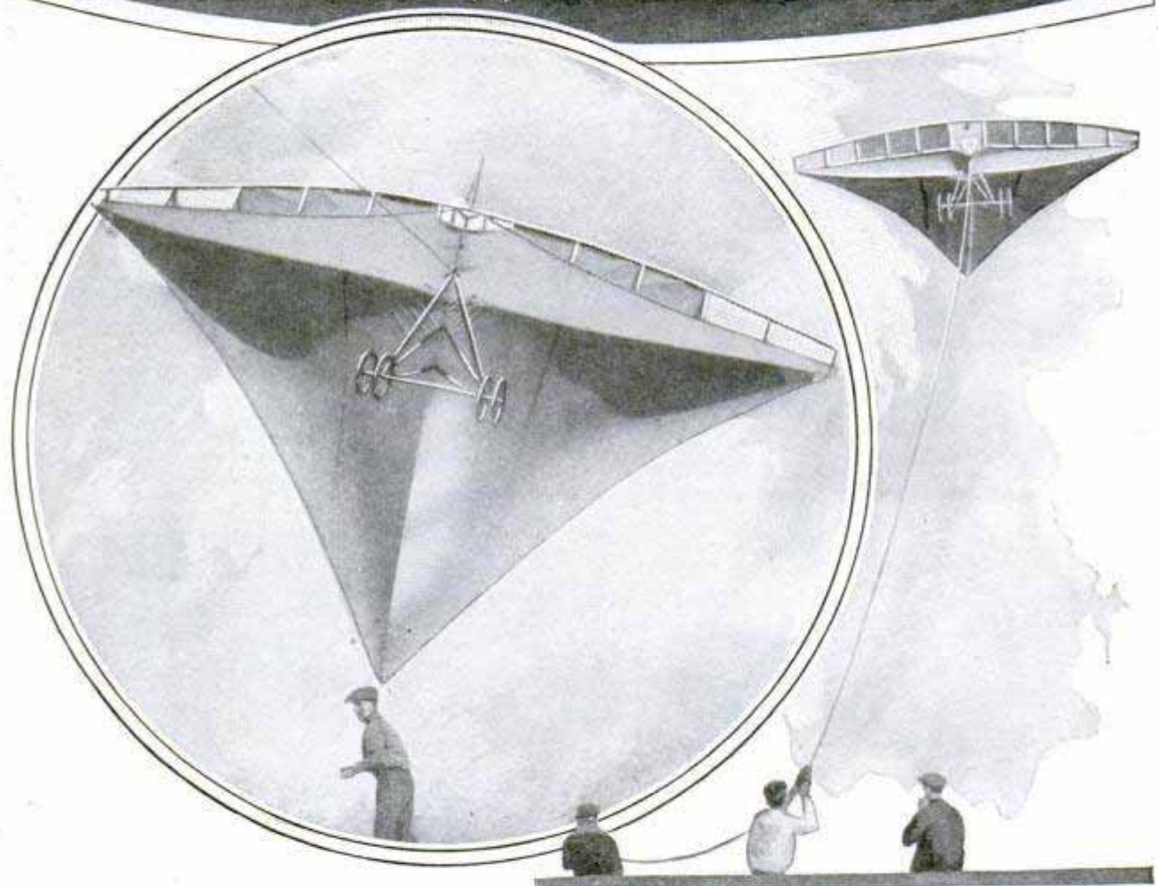
Demonstration of the Kite's Strength and Views of It in Flight; More than 200 Successful Trials Have Been Made with It, Lifting 186 Pounds
