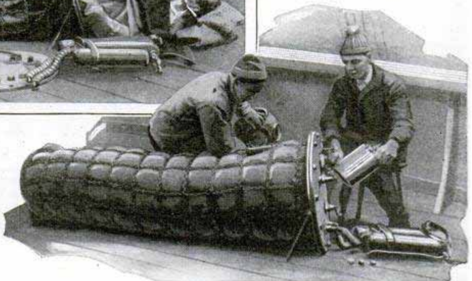
Placing Diver in the Chain Sack and Administering the Compressed Air and Oxygen After Bag Has Been Sealed
