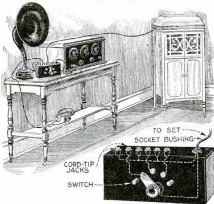
Above, Switch Box in Use, Showing Leads Run to Speakers of Various Types; Lower Right, X-Ray View of the Box
