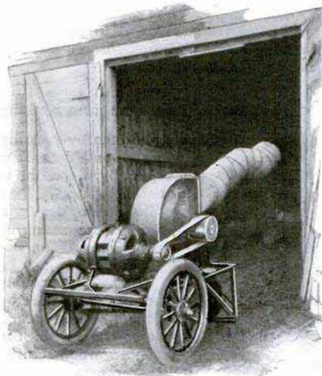
Portable Blower Provides Forced Ventilation for Tobacco Shed and Prevents Shed Burn
