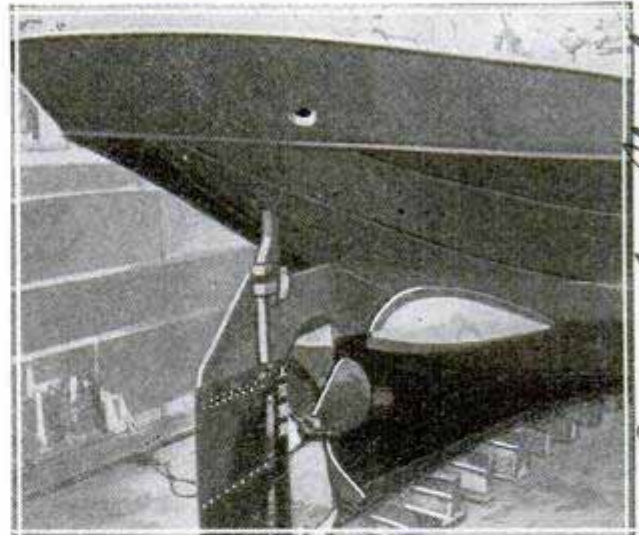
Deflecting Fins Attached near Propeller Are Said to Reduce Fuel Consumption and Increase Speed
