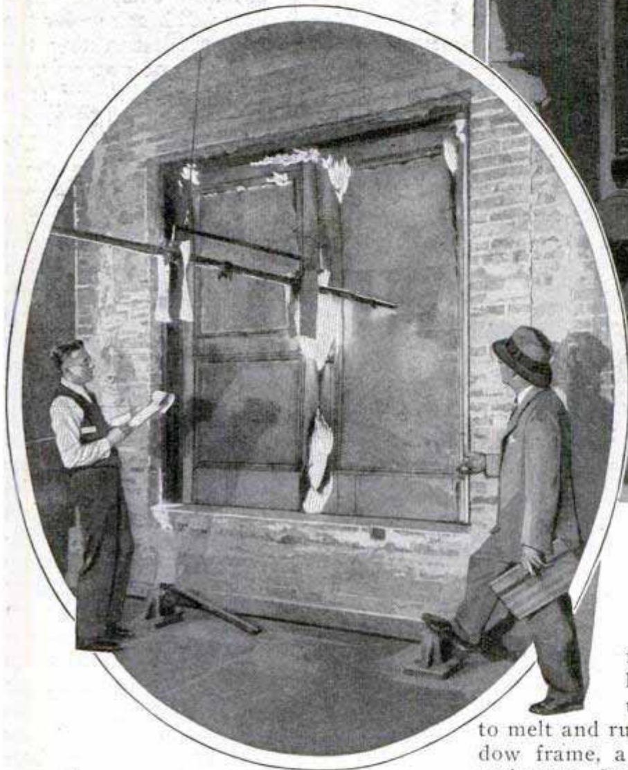
Expanding on the Side Next to the Fire First, a Huge Steel and Wire-Glass Window Slowly Bends In to the Flame; Left, Metal-Covered Fire Doors Flicker with Wood-Gas Flames as the Interior Carbonizes
