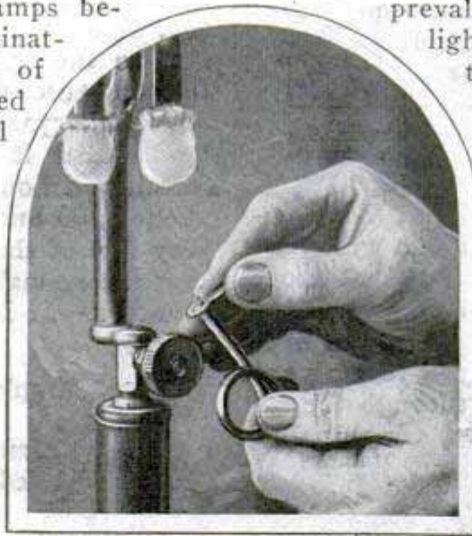
Unscrewing Generator Tip; Right, Inspecting Lead Washer on the Filler Plug
