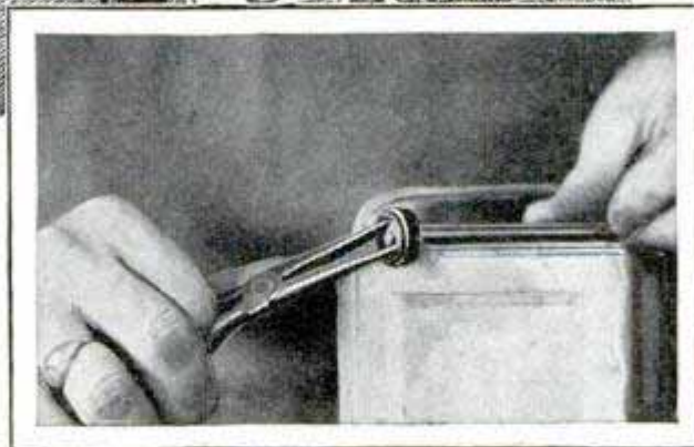
Removing the Nut That Holds the Washer on the End of the Pump Rod
