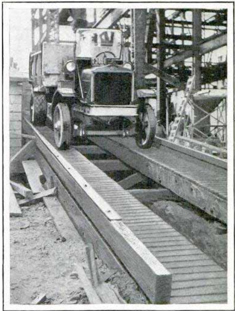
Inclined Runway to Concrete and Sand Bins Which Feed a Mixer Located in Excavation
