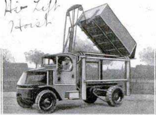
Body Elevated for High Dumping from End; It Also Empties from Sides or Bottom
