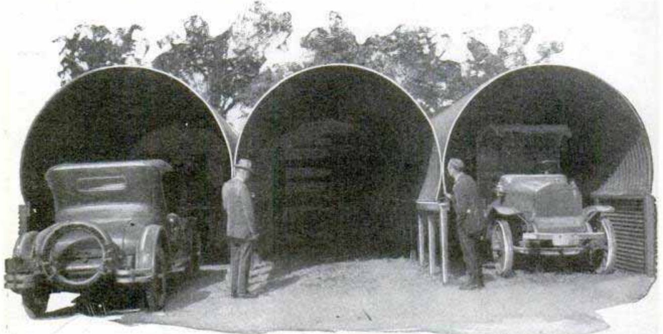
Intended for Bomb-Proof Shelters but Adapted to Garages for Government Automobiles; Steel Roofs Arranged to Harbor Cars at the Plant-Testing Farm in Virginia
