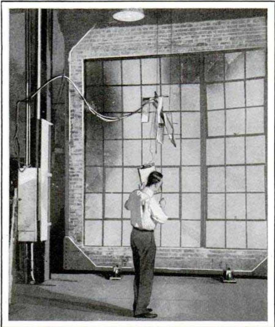
Heat, So Intense It Will Melt the Wired Glass, Is Raging behind This Big Fire Window during the Test
