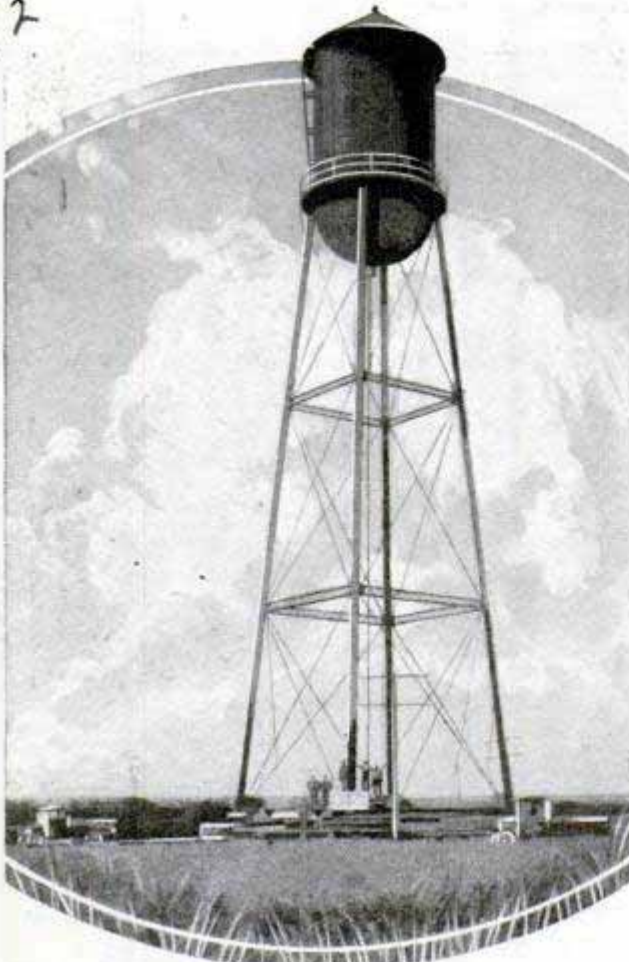
Pulling the Tower across the Prairie; after a 630-Foot Journey, It Was Only One Inch Out of Plumb
