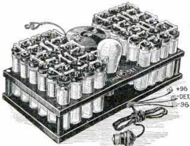
Storage B-Battery Showing Built-In Charging Unit permanently attached to a light socket. Leads for the set connections are also provided, and the unit is a complete source of B-battery supply that is easy to keep at maximum efficiency.
