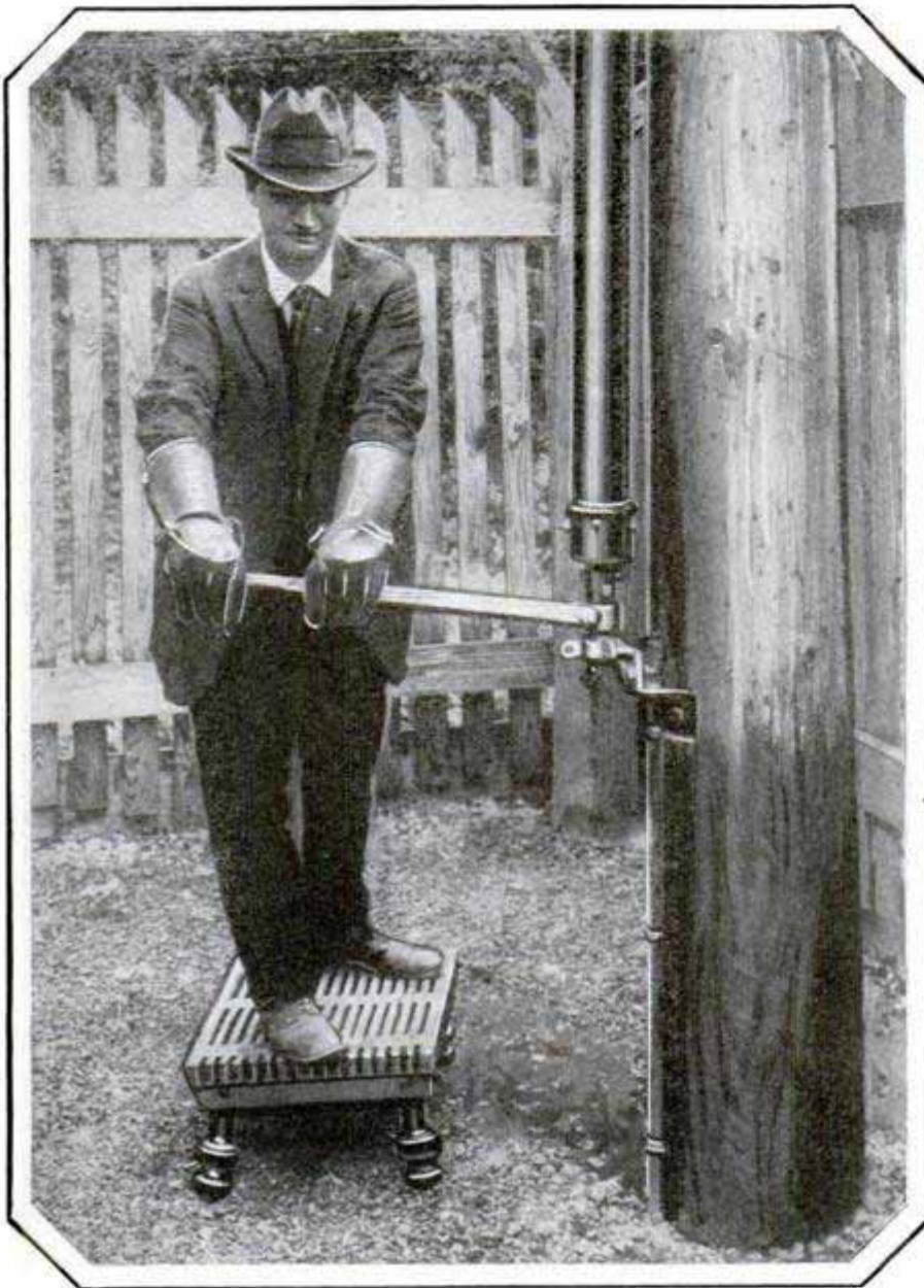
Guarding against Injury in Manipulating a Grounding Switch by Standing on Insulated Platform and Using Gloves
