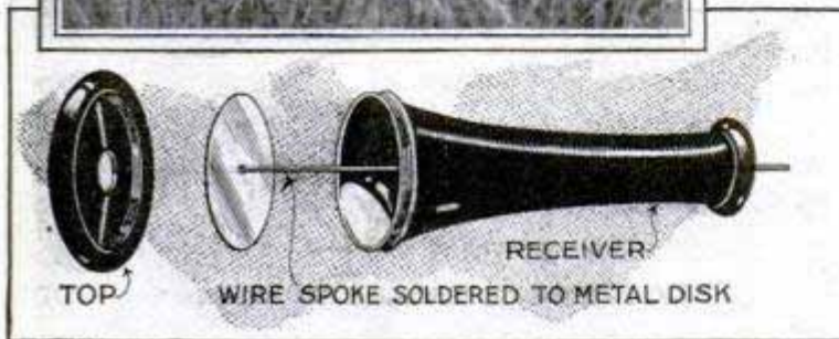
Simple Device for Detecting Leaks in Water Pipes, Made from an Old Telephone Receiver
