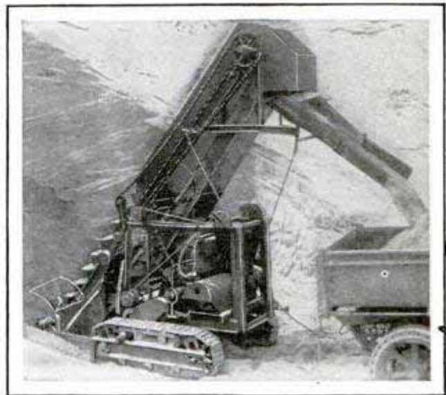
Sand Loader in Action; It Can Be Moved to New Position by Its Own Power
