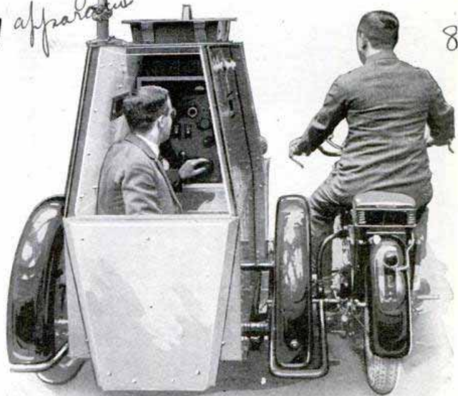
Radio Sidecar for Police Work in Berlin; It Can Be Disconnected and Run on Own Power
