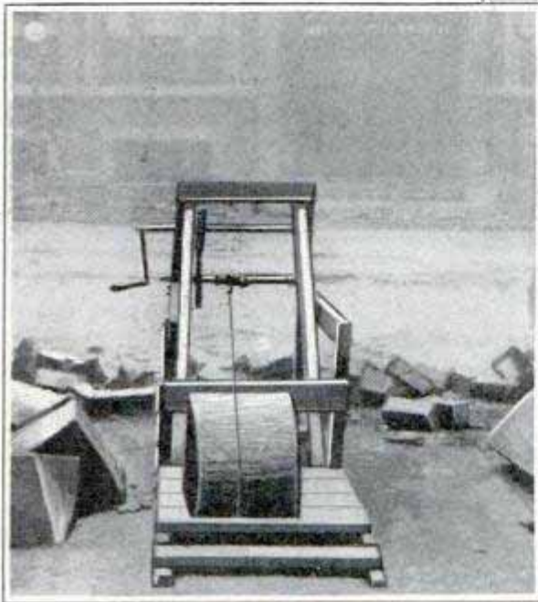
Platform and Mechanism for Cutting Large Cakes of Tar with Little Effort and at a Considerable Saving of Time
