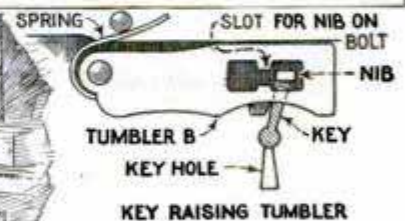
Details of Common Rim and Mortise Locks; Also Interior View of Front-Door Lock with Split Handle and Locking Pins
