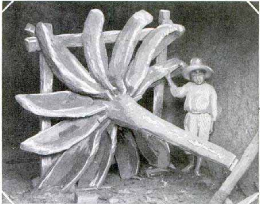
Turbine Water Wheel, Cut from Wood Nearly Four Centuries Ago for Mill in Mexico; It Still Operates
