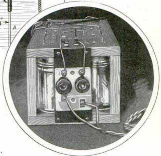
Above, Section Diagram Showing Method of Mounting the Electrodes; Left, Front View of Completed Eliminator; Right, Rear View Showing Fuse Block in Position
