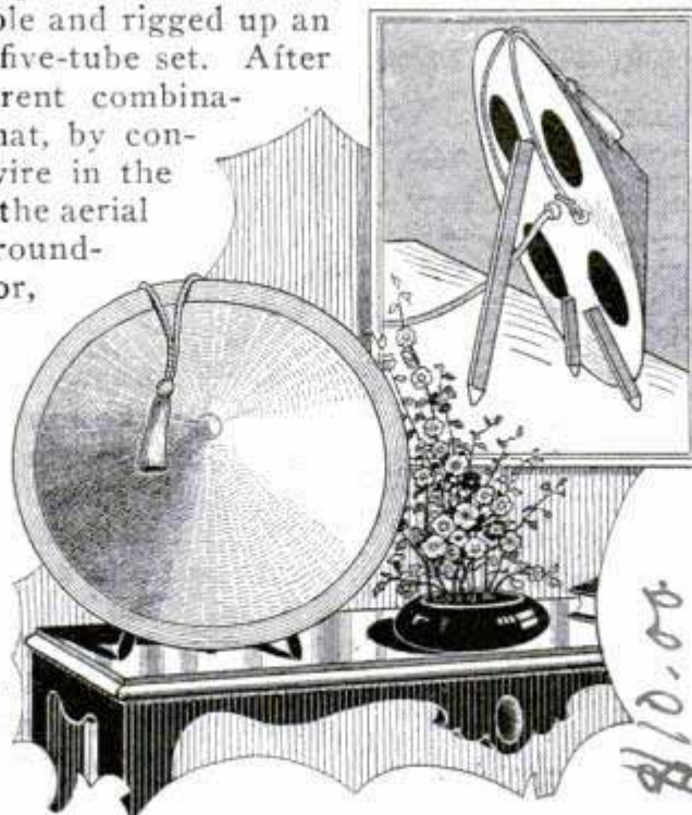
Cone Speaker That Can Be Mounted on Sturdy Easel, Or Suspended from Picture Molding
