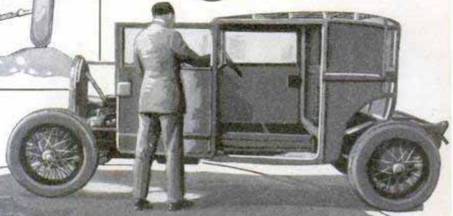
Built without a Front Axle, the Car Above Is Said to Have Unusually Easy Riding Qualities; at Right Is a European Type of Low Body
