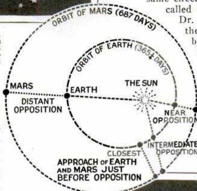
Map of the Orbits of Earth and Mars, Showing Why They Are Nearest at Certain Periods, and, at Right, a Sketch from a Photograph Showing Canals
