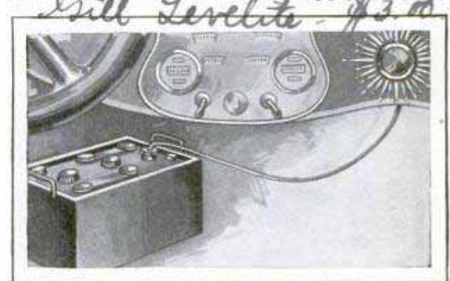
Battery Water-Gauge Light Installed on Dashboard; It Goes Out When Water Gets Too Low
