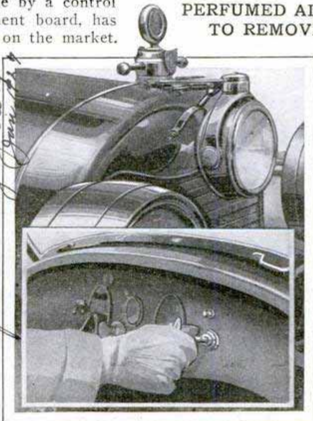
Auto Spotlight Mounted on the Radiator and Swung in All Directions by a Dash Control
