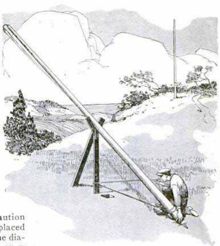
Aerial Mast Resting in Crotch, Ready to Be Raised
