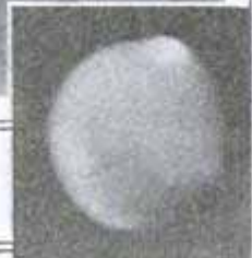
Valley of San Jose, Above, and Right, Mars, Photographed through Ultraviolet Filters
