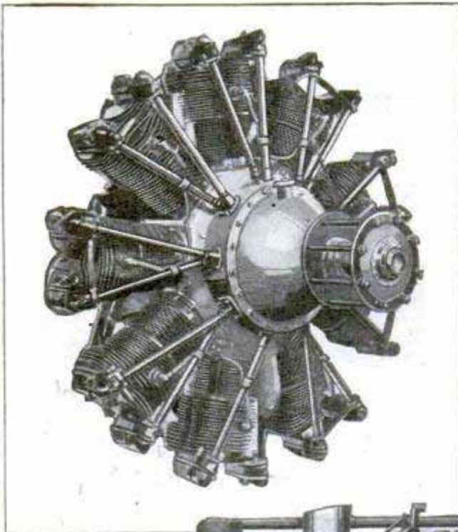
Air - Cooled Radial Engine; Engine, Radiator and Tanks of an Observation Plane; Bottom, End View of an Inverted Motor
