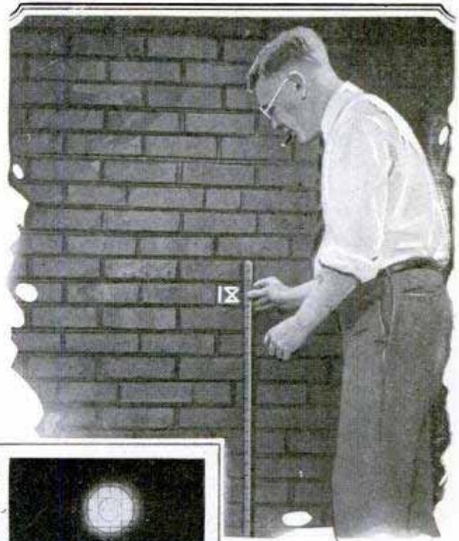
Top, Marking Center Height on Wall; Left, Correct and Incorrect Focusing; Bottom, Marking Center-to-Center Distance
