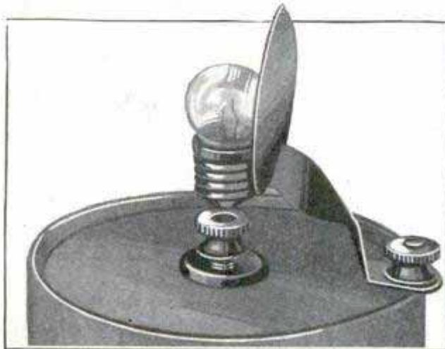
Bulb Attached to Dry Battery; Circuit Is Completed by Pressing Bracket against Center Post
