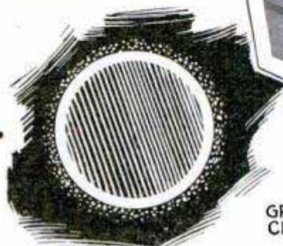
CROSS SECTION ENAMELED-COPPER WIRE
