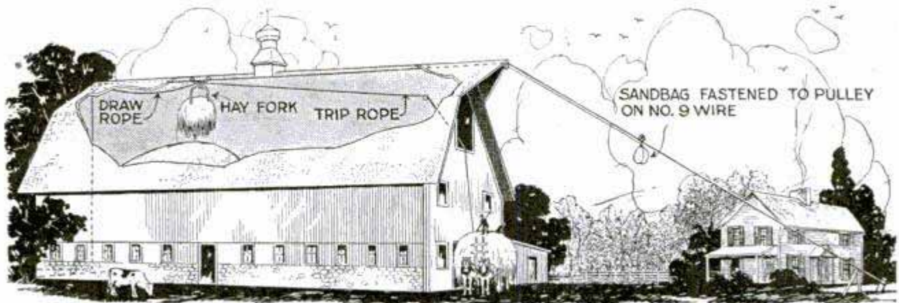
Sandbag Fastened to a Pulley on Wire, Which Is Run from the Barn Gable to a Stake in the Yard, Pulls the Hay Fork Back the Entire Distance in a Long Dairy Barn
