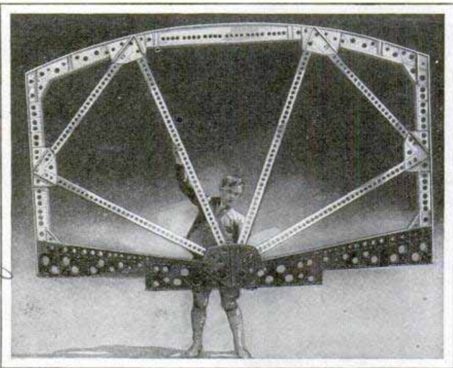
Demonstrating Light Weight of Metal Being Used for Huge Airplane; Whole Span Easily Lifted by One Man
