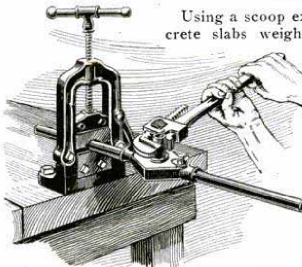
Method of Threading Short Lengths of Pipe
