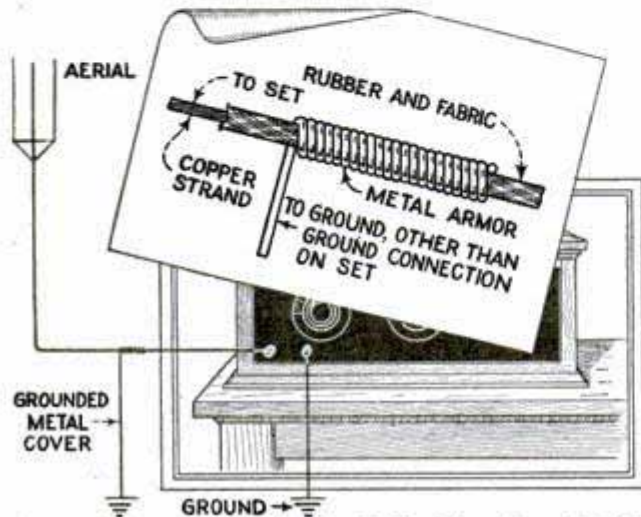
Armored Automobile-Circuit Cable That Proved Efficient Aerial, and Diagram of Installation
