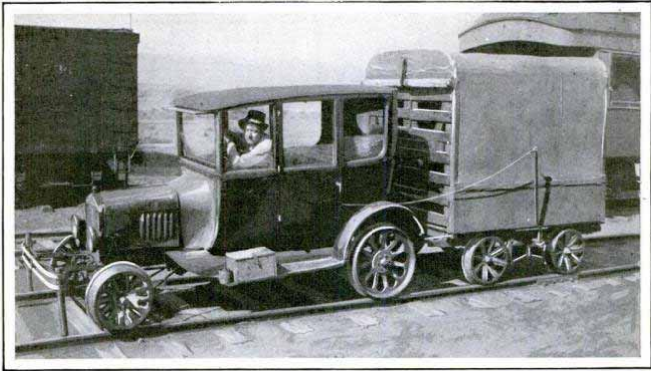
Handcar Wheels Attached to Automobile Enables It to Run over Railroad Tracks with Considerable Speed; Lengths of Hose Hanging from Bumper Brush Away Small Obstructions from Rails
