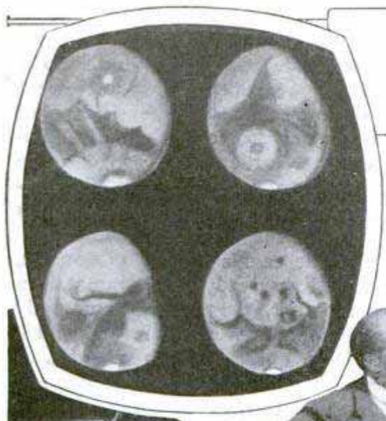
Four Drawings, at Different Times, Showing the Entire Surface of Mars, at Left, and Below, the Forty-Inch Lens of the Yerkes Telescope
