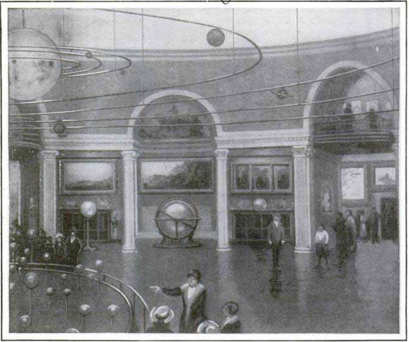
Miniature Indoor Universe, Planned for Astronomical Hall of the American Museum of Natural History, Will Enable the Layman to See the Sun, Stars and Planets Revolve
