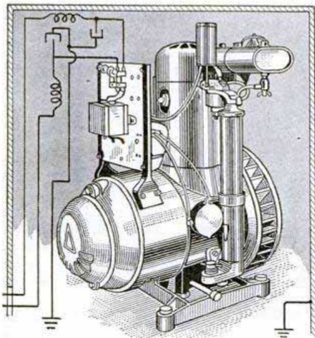
Lighting Plant, Showing Suggested Methods of Eliminating Radio Interference
