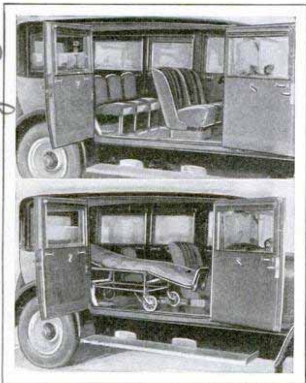
Seats Arranged for Eight Passengers and Adjusted as Wheeled Stretcher; Note Absence of Door Post
