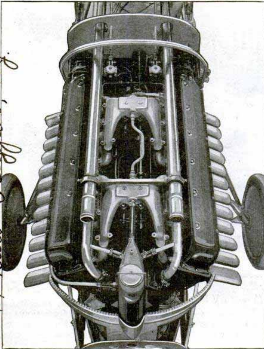
Looking Down on the Motor of the Curtis "Hawk," an Army Pursuit Plane Noted for Its High Speed and Fast Climbing Ability
