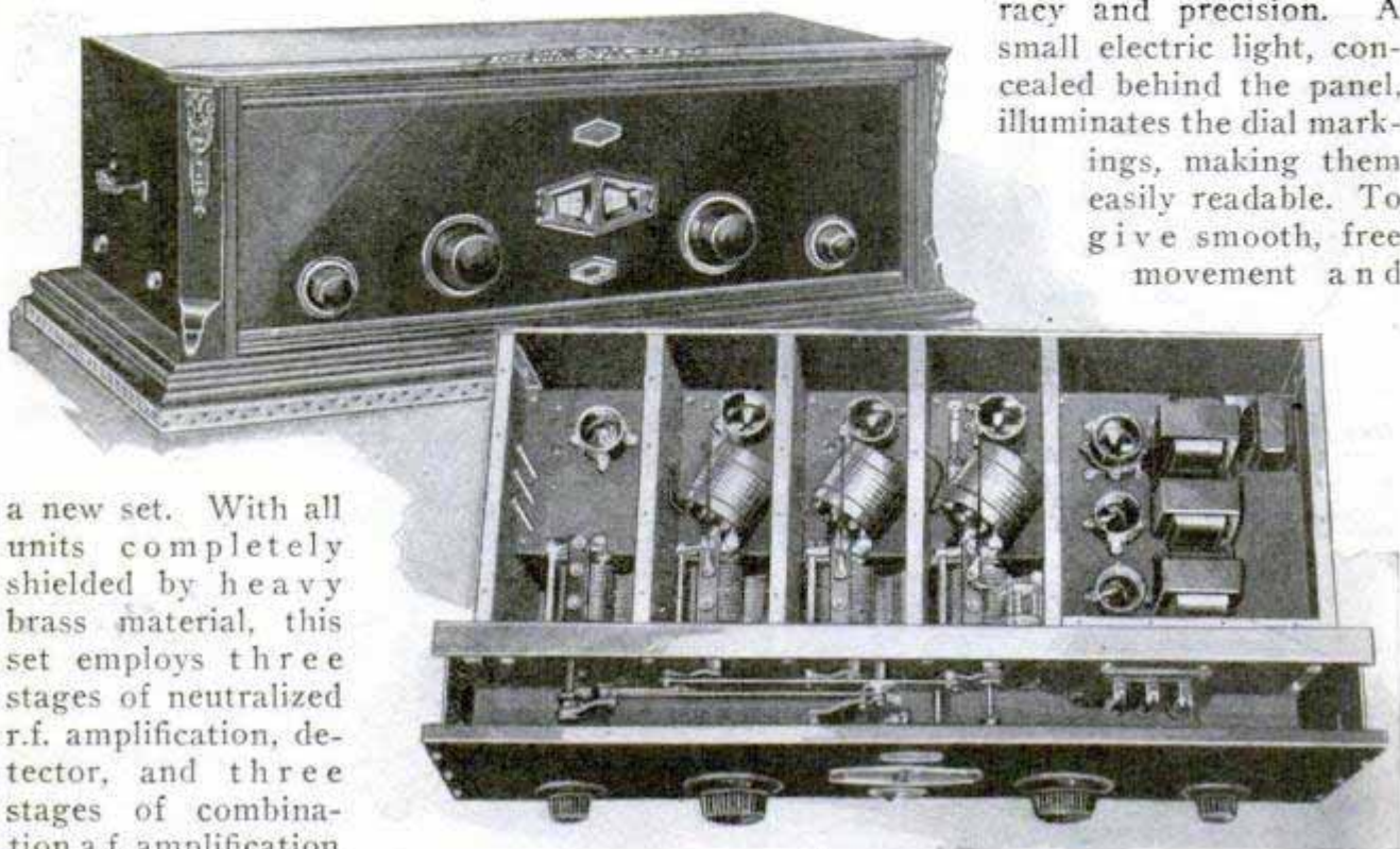
Above, Instrument in Cabinet Showing Tuning Controls and Windows for Dial Markings; Below, Interior View with Top Shield Removed
