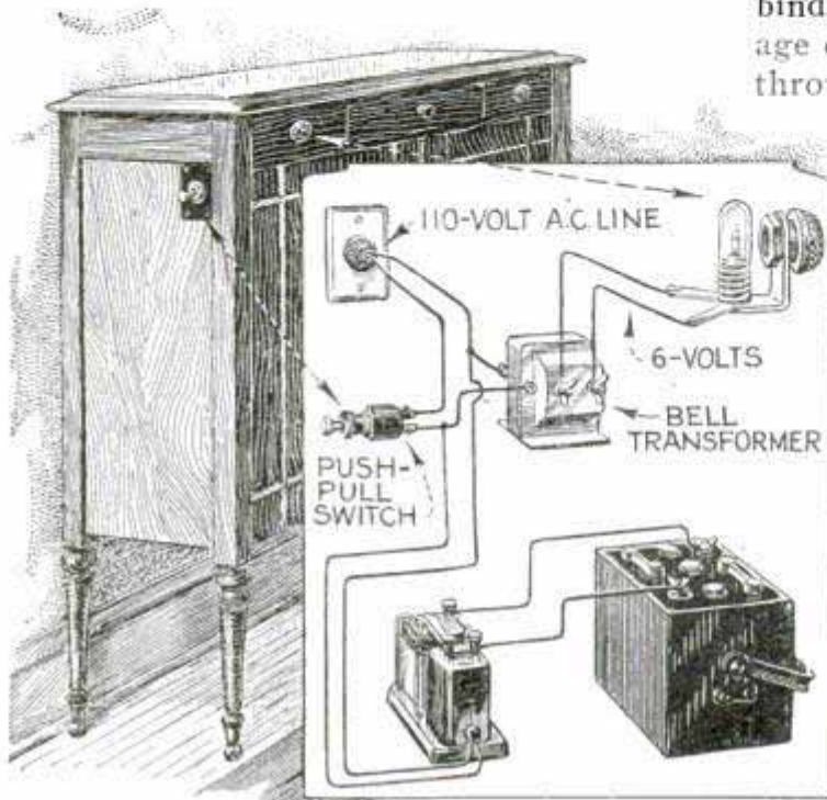
Radio Console, Showing Suggested Positions for Pilot Lamp and Switch; Insert, Detailed Wiring Diagram
