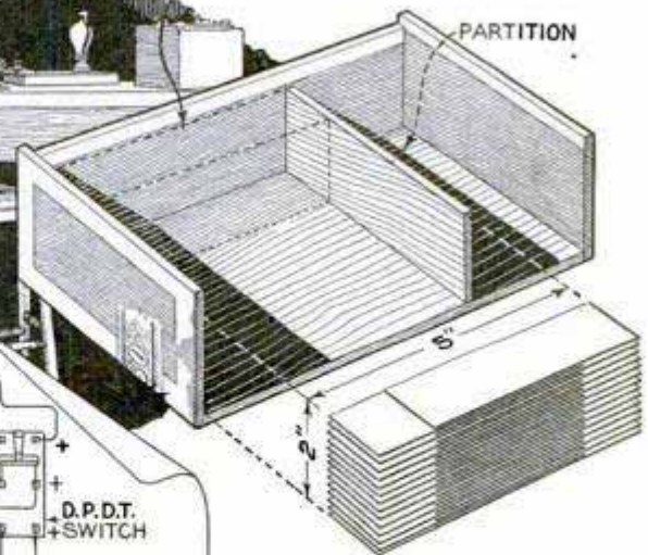
METHOD OF ASSEMBLING CORE
