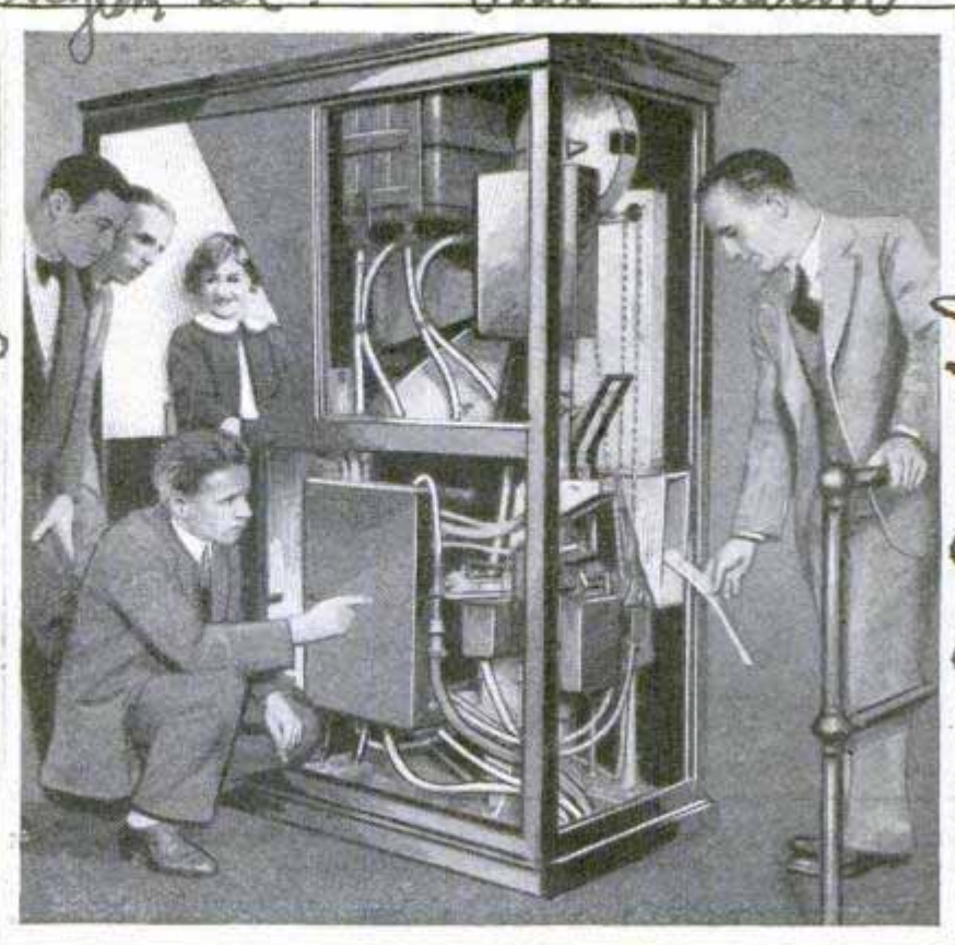
© Herbert Photos Panels Removed from Slot-Machine Camera to Expose Interior; Coin Aperture at Side and Film Delivery at Right
