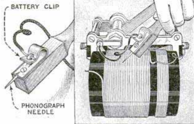
Details Showing Needle Mounted under Clip, and Right, Testing Coil to Determine Number of Turns
