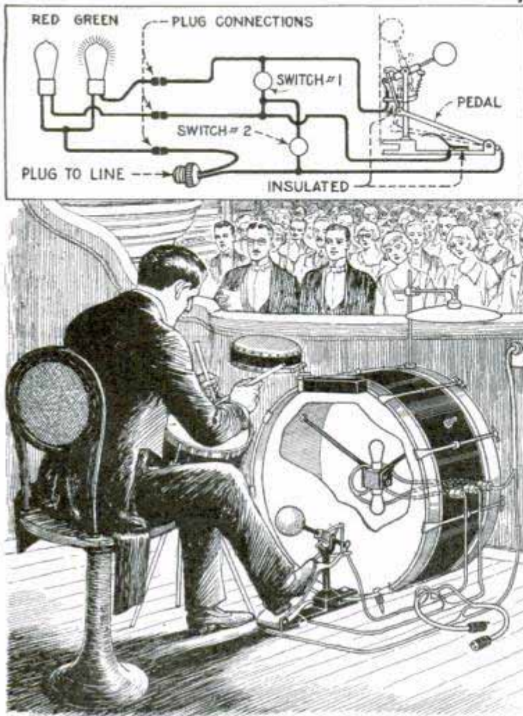
Colored Electric Lights Operated by the Pedal of an Orchestra Bassdrum Increase the Jazzy Effect of the Music
