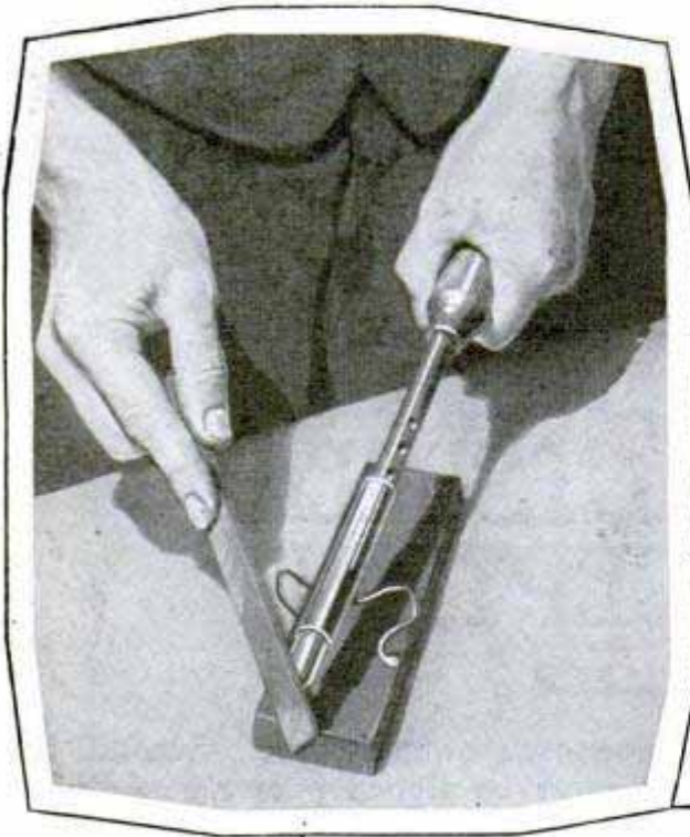
Top, Filing Tip of Soldering Iron; Center, Arrows Point to Contacts That Cannot Be Soldered; Bottom, Tinning Iron
