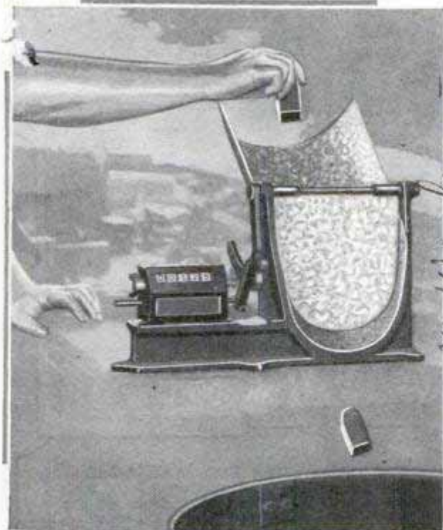
As Pieces Fall through Hopper, the Chute Tips, Registering the Count on Indicator at Left
