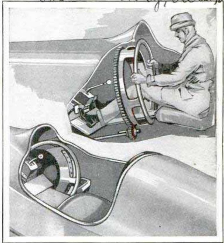
Steering Wheel and Part of Gear on Racing Car of Exceptionally Narrow Design to Decrease Wind Resistance
