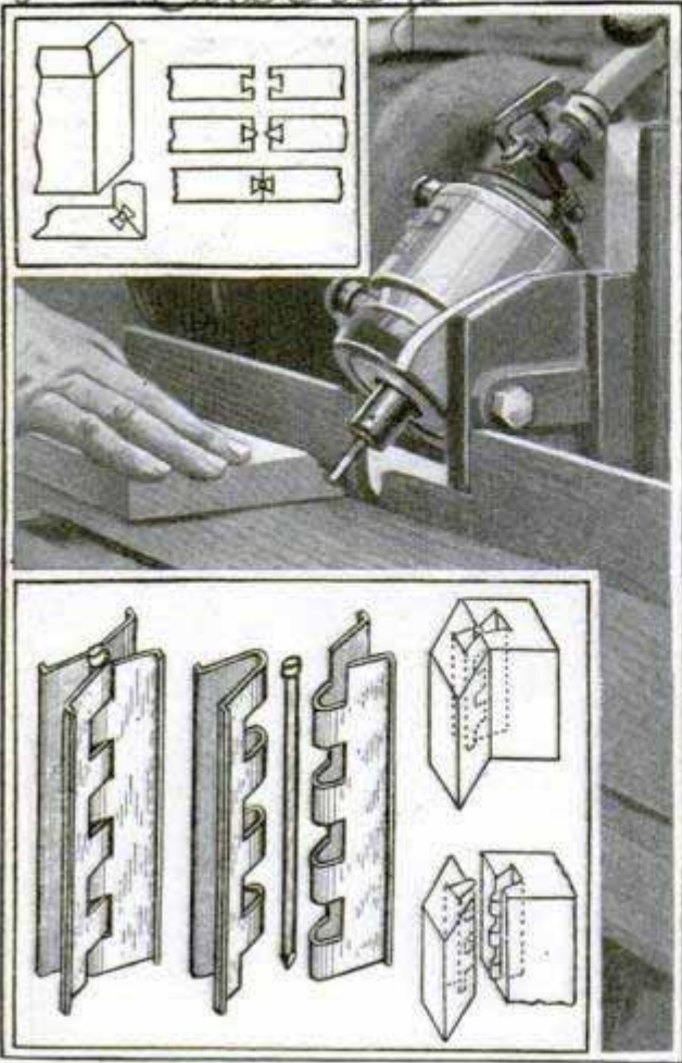
Diagrams Showing How Lock Joints Are Held Together with Nail, and Photograph of Slot Cutting
