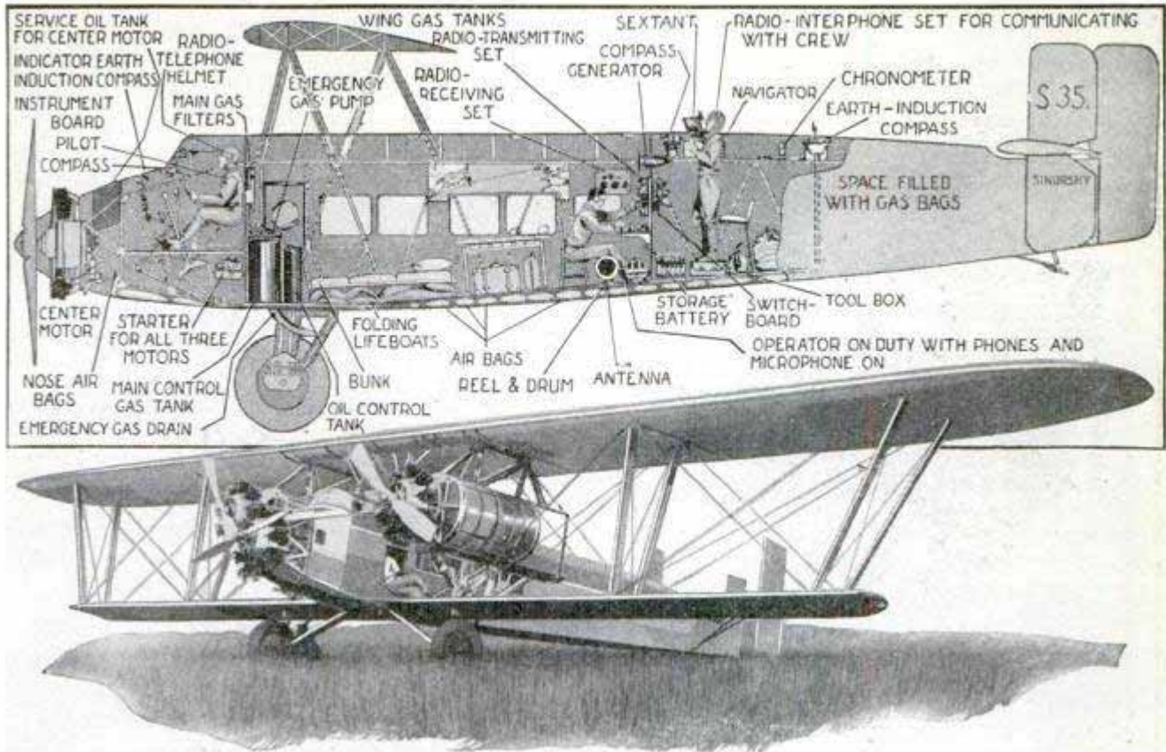
Photo and Diagram, Showing the Interior Arrangements of a Typical Big Plane; This Is Rene Fonck's Ill-Fated Three-Motored Sikorsky, Which He Hoped to Fly from New York to Paris
