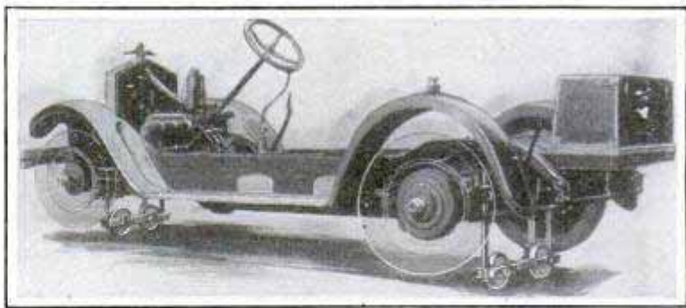
How the Auxiliary Wheels Are Lowered to Run the Car Side-ways for Parking
