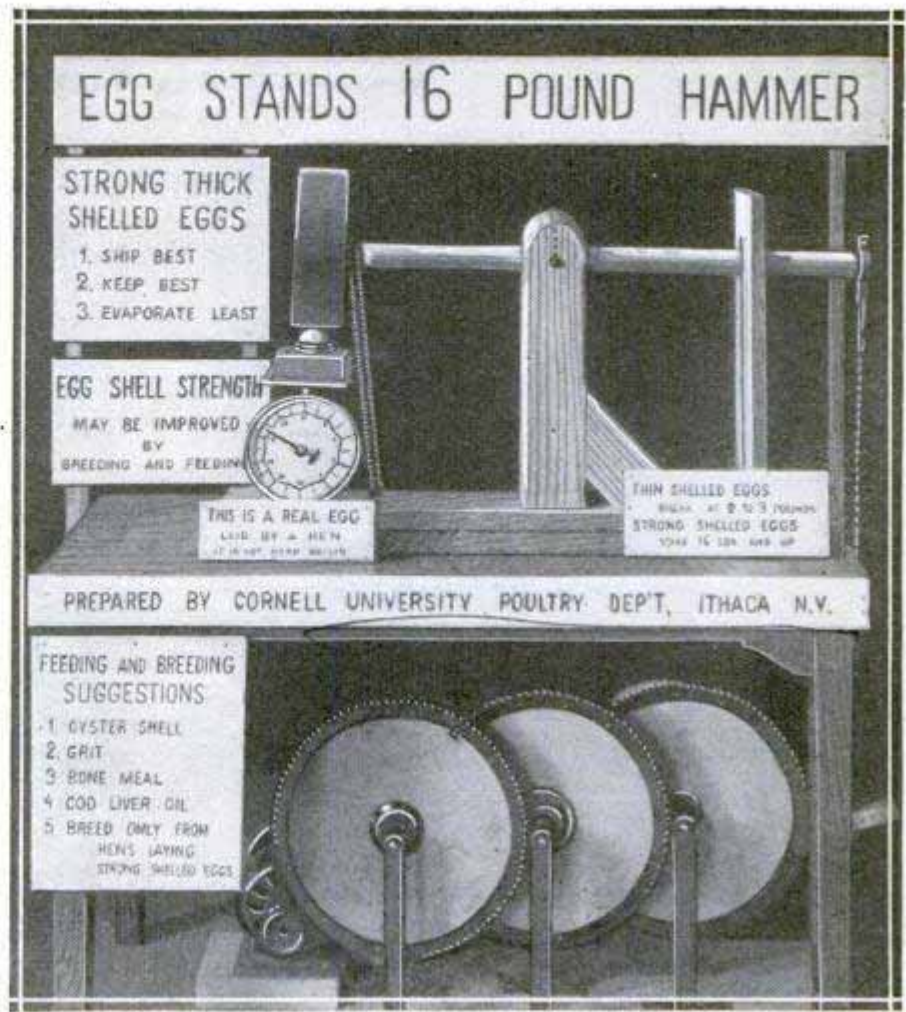
Geared Trip-Hammer Apparatus for Testing the Strength of Eggshells; Force of Blows Was Accurately Measured
