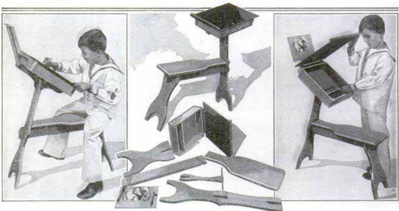
Junior Artist's Studio in One Unit; the Combination Drawing Board, Locker and Seat, and How Pieces Can Be Taken Apart and Reassembled; Holder for Copy at Top of Board
