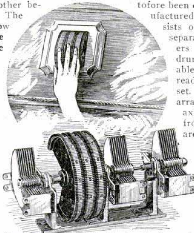
Drum-Type Control Unit, Showing Condensers in Parallel, Which Can Be Controlled with One Hand
