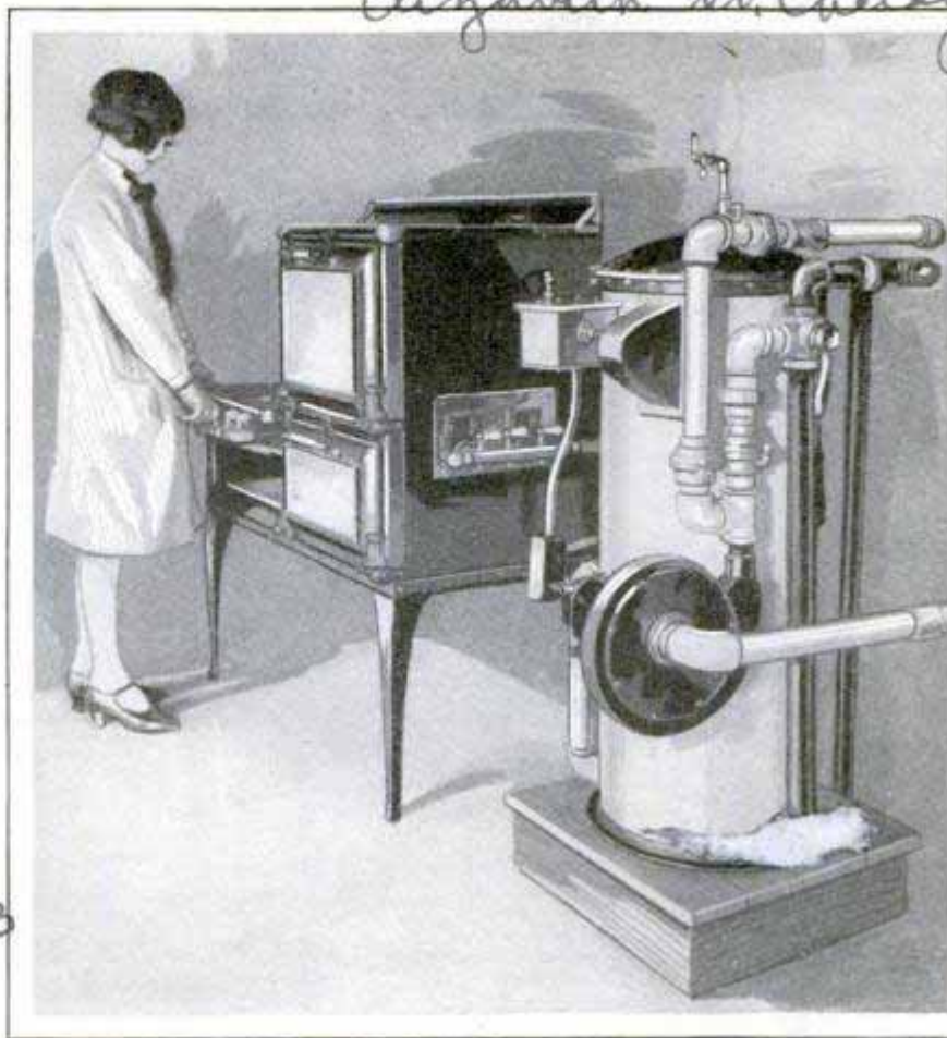
Gas-Generating Plant for Homes Not Served by City Supply; Outfit May Be Set Up Far from the Range
