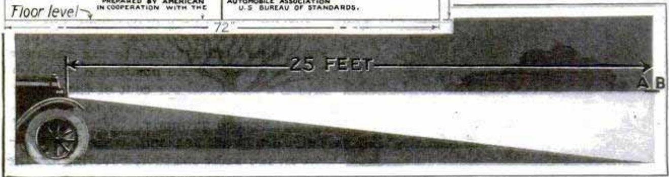
Above, Cleaning Reflector; Center, Official Focusing Chart; Below, Properly Aimed Beam Does Not Rise above Horizontal
