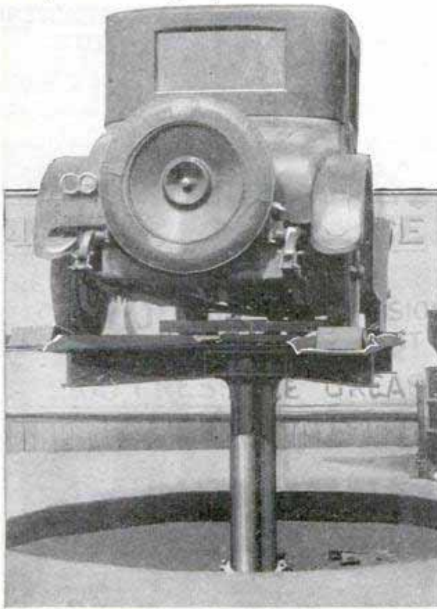
Car Raised on Lift for Inspection or Repair; It Rests on a Strong Platform of Channel Iron
