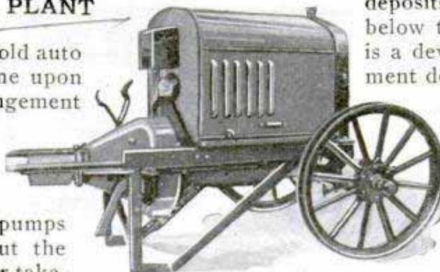
Old Auto Sawed in Two and Prepared for Service as a Power Plant
