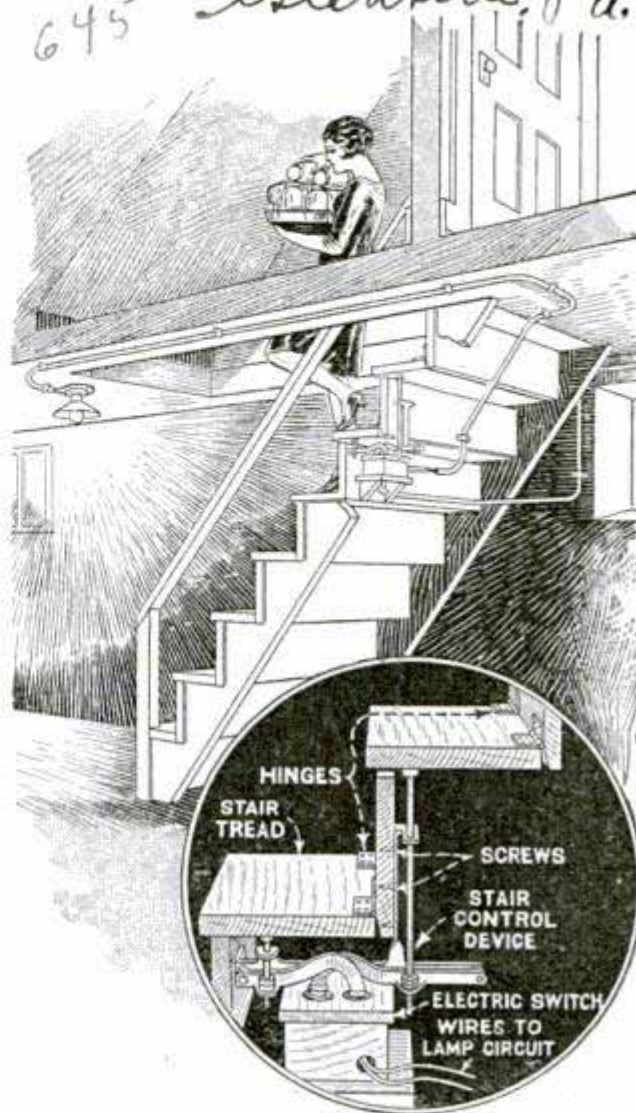
Drawing of Light Switch, Installed under Stairs, and Inset Explaining Details
