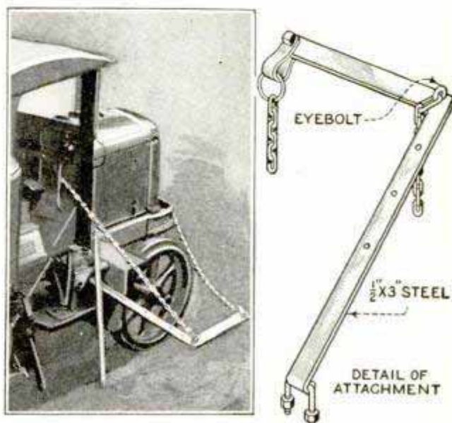
Handy Hook Attached to Side of Farm Tractor Pulls Light Implements
