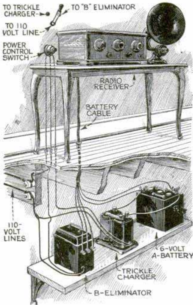
Simple Power-Control Switch for Trickle Charger and B-Eliminator with Connections
