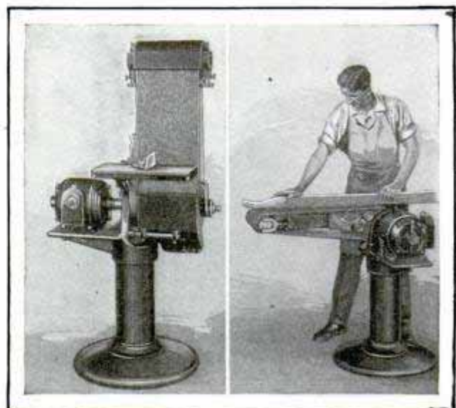
Sanding Machine Which May Be Operated Either as a Vertical or Horizontal Belt
