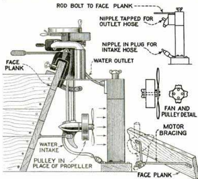
Side Elevation, Showing the Various Construction Details; There Is Very Little Work Necessary
