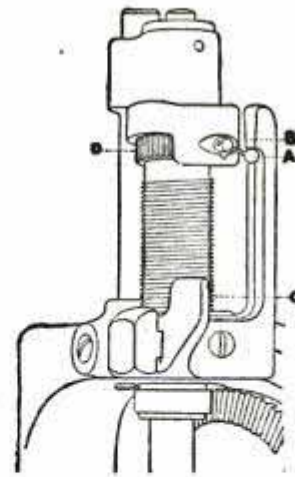
Enlargement of head of "Yankee" Automatic Bench Drill
