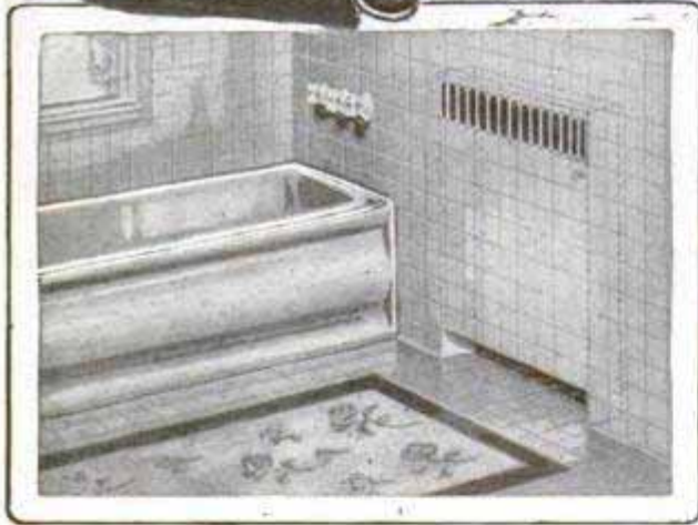
Introducing a Variation of the Usual Type of Radiator; Heating Pipes Pass through Series of Copper Fins Which Give Off Warmth; Cut-Out View of Cabinet and Typical Installations
