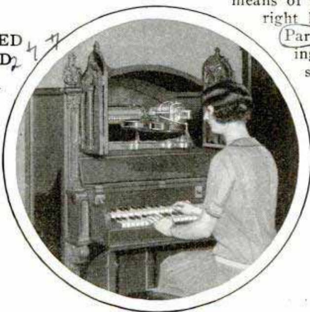
With a Piano Keyboard, This Violin Can Be Played without Learning to Use a Bow
