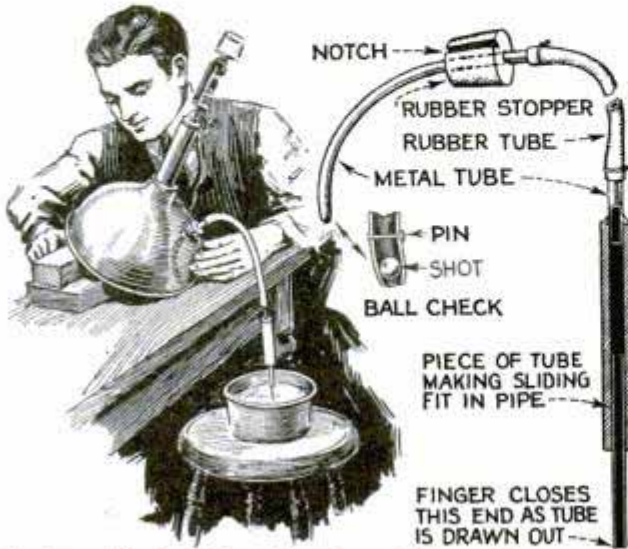
Getting All the Dirty Gas Out of Vapor Lamps with a Siphon
