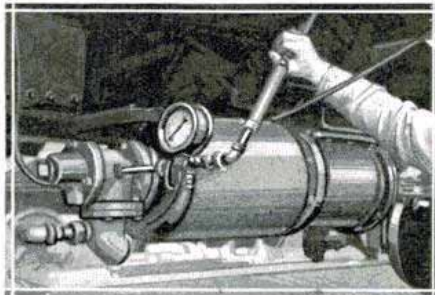
Method of Testing Air Cylinder and Retainer on Railway Car
