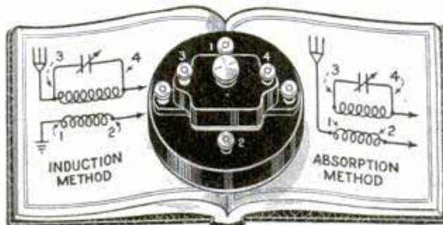
Interference-Eliminating Device, Showing Two Ways in Which It May Be Used
