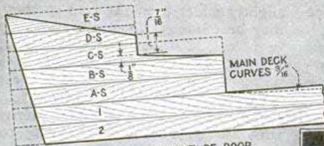
LAYOUT OF POOP
