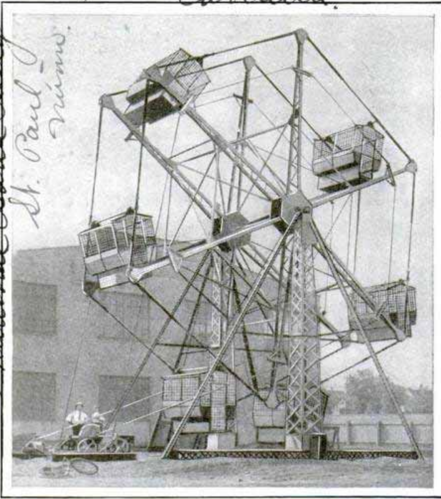
Putting a New Twist to the Staid Old Ferris Wheel; the Cars Slide Twelve Feet at Two Points in Each Revolution
