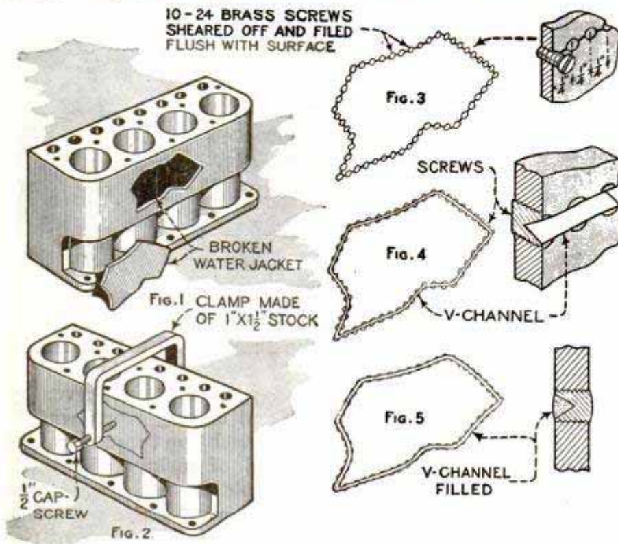
Cracked Water Jacket on Automobile Repaired by Simple Method Using Screws and Solder
