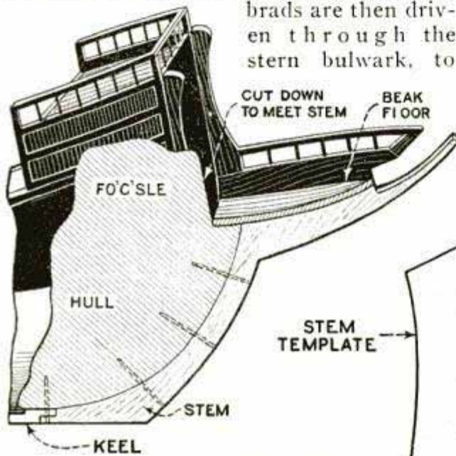
Full-Size Template of the Stem and Detail of How It Is Fitted
