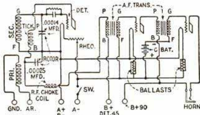
Schematic Circuit Diagram
