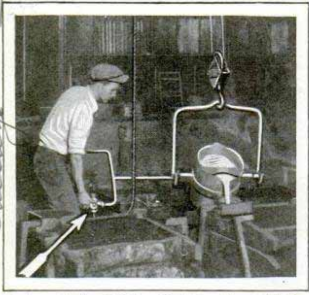
Pouring a Ladle of Molten Metal from Suspended Carrier Equipped with Handlebars to Simplify Operation
