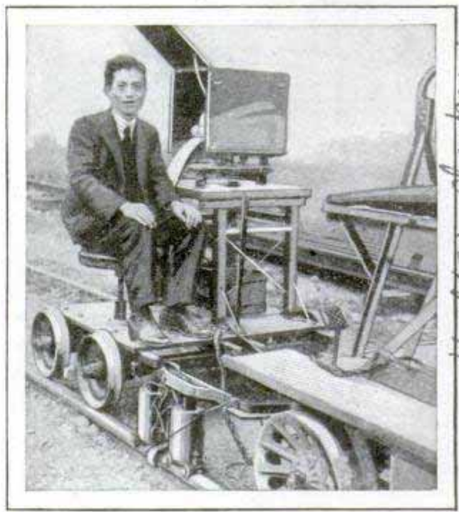
Rail Tester in Operation behind an Inspection Car on Japanese Line; Note Attachment to Rails
