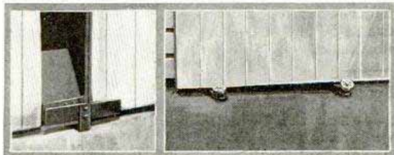
Fasteners on Sliding Garage Door Prevent It from Swinging in the Wind
