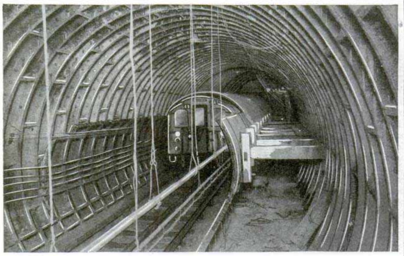
Difficult Engineering Feat in London Nearing the Close; after Building a Large Subway Tunnel around a Smaller One, the Workmen Begin Dismantling the Latter While It Is in Use
