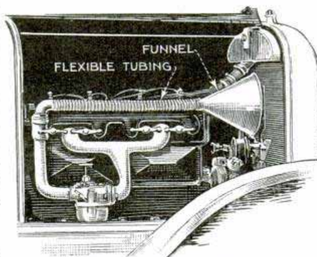
Increased Speed and Power, and More Mileage per Gallon Are the Results of This Installation
