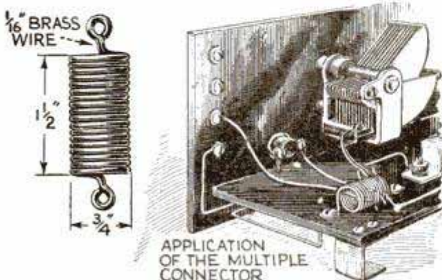
Detail of Coil-Spring Connector, and Mounted on Set with Leads in Position
