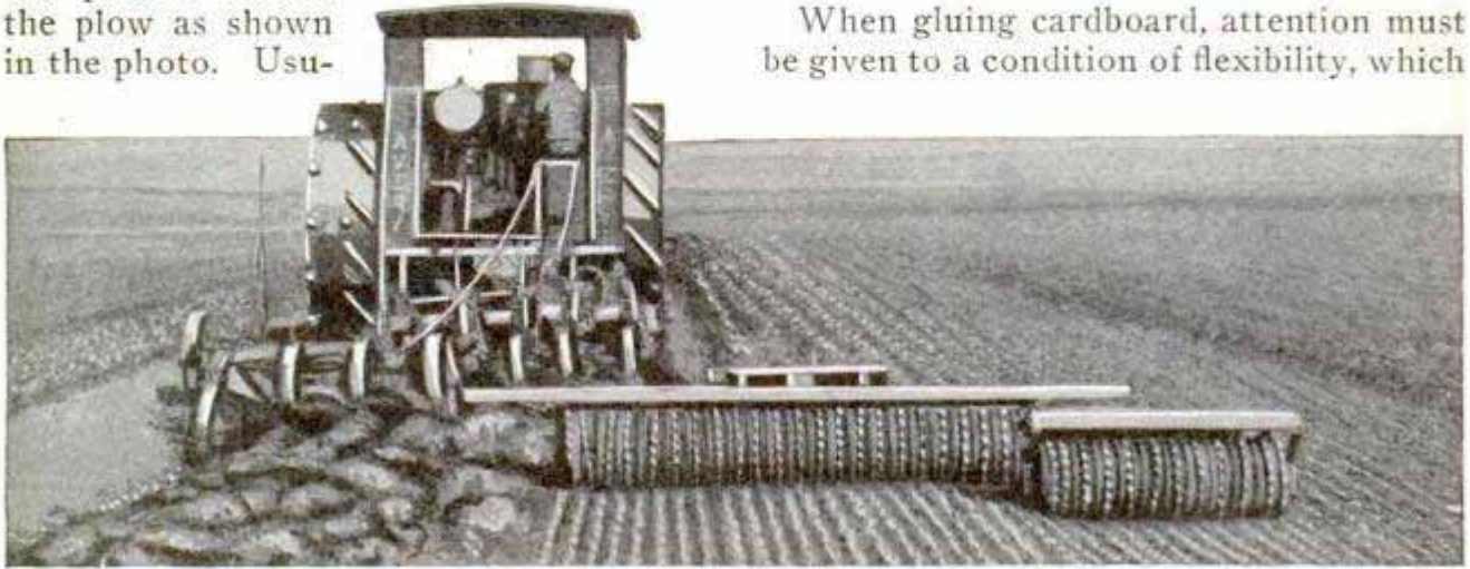
Saving Time When Plowing Stubble Ground for Fall Wheat by Attaching the Packer behind the Plow, Both Being Drawn by a Tractor
