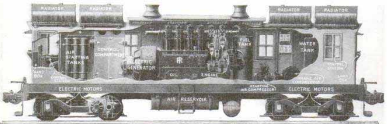
Oil-Electric Locomotive in Cross Section; There Is a Control Station at Either End; Less Noise, Absence of Smoke and Cinders and Economy Are Features Credited to These Engines
