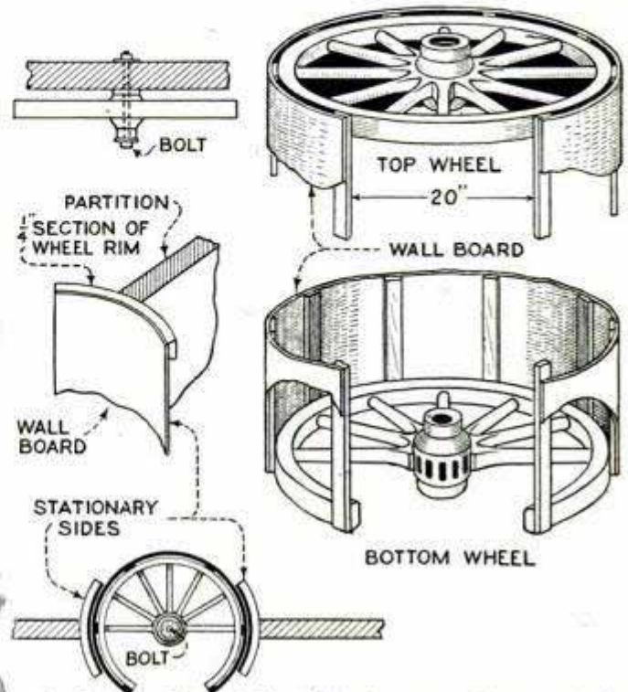
Excluding Light Effectively from a Photographer's Dark Room by Using a Revolving Door, Which Is Pivoted on Wagon Wheels
