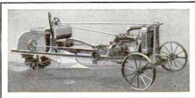
The Single Rear Wheel Enables This Motor Plow to Work within Six Inches of Trees
