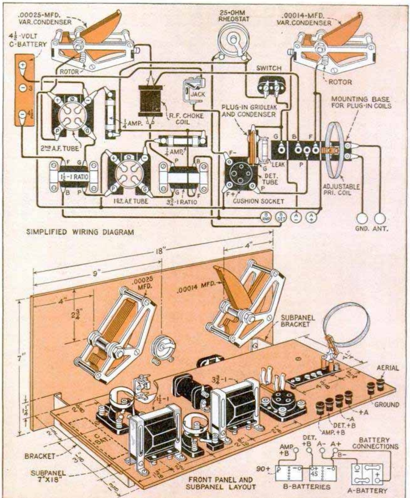
Above, Simplified Wiring Diagram, with All Instruments in Their Relative Positions; Below, Front-Panel and Subpanel Layouts with Battery Connections Shown at Lower Right
