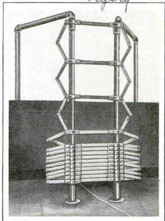
Folding Ladder, Sliding on Rods, Gives Access to Floating Deck of Fireproof Oil Tank
