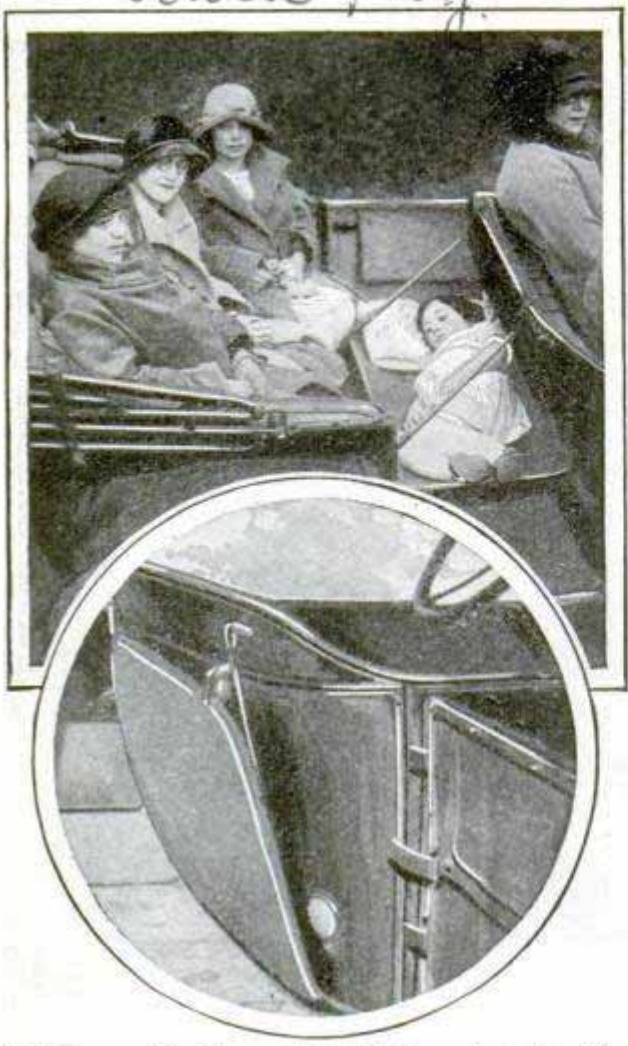
Crib Lowered for Use and Folded Up against Auto-Seat Back Where It Is Out of the Way
