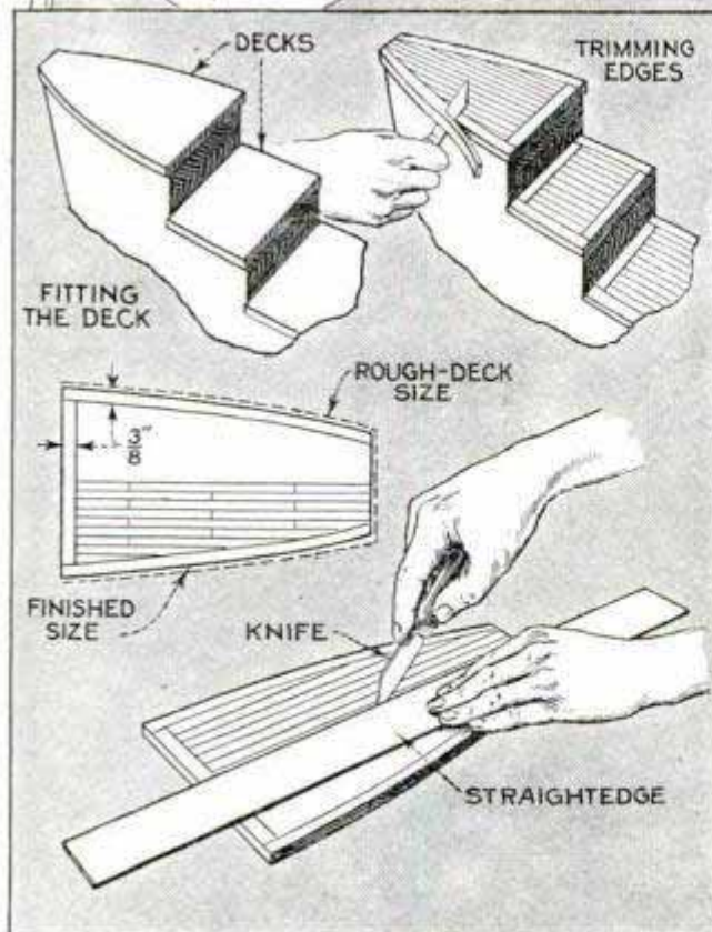
Above, Photo Showing Half-Finished Hull; the Drawings Illustrate Details of Hull Construction
