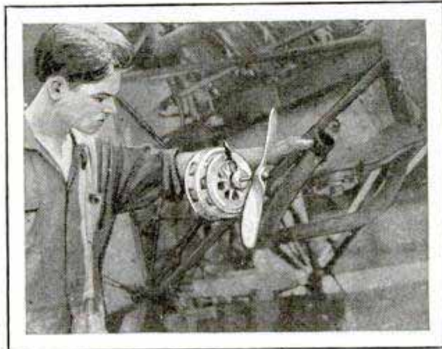
Siren and How It Is Attached to the Plane; It Shrieks a Two-Toned Warning as Craft Descends
