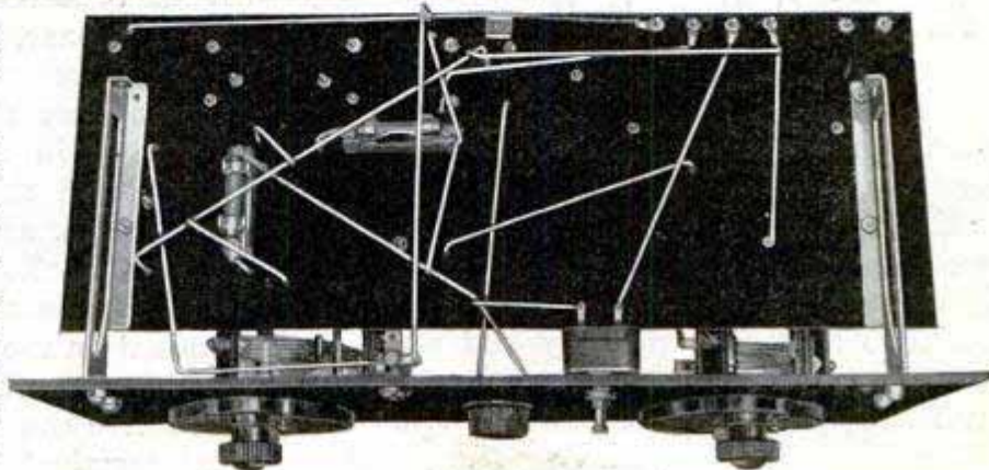
Looking Down on Subpanel: Right, Under-Subpanel View, Showing Ballasts and Method of Wiring
