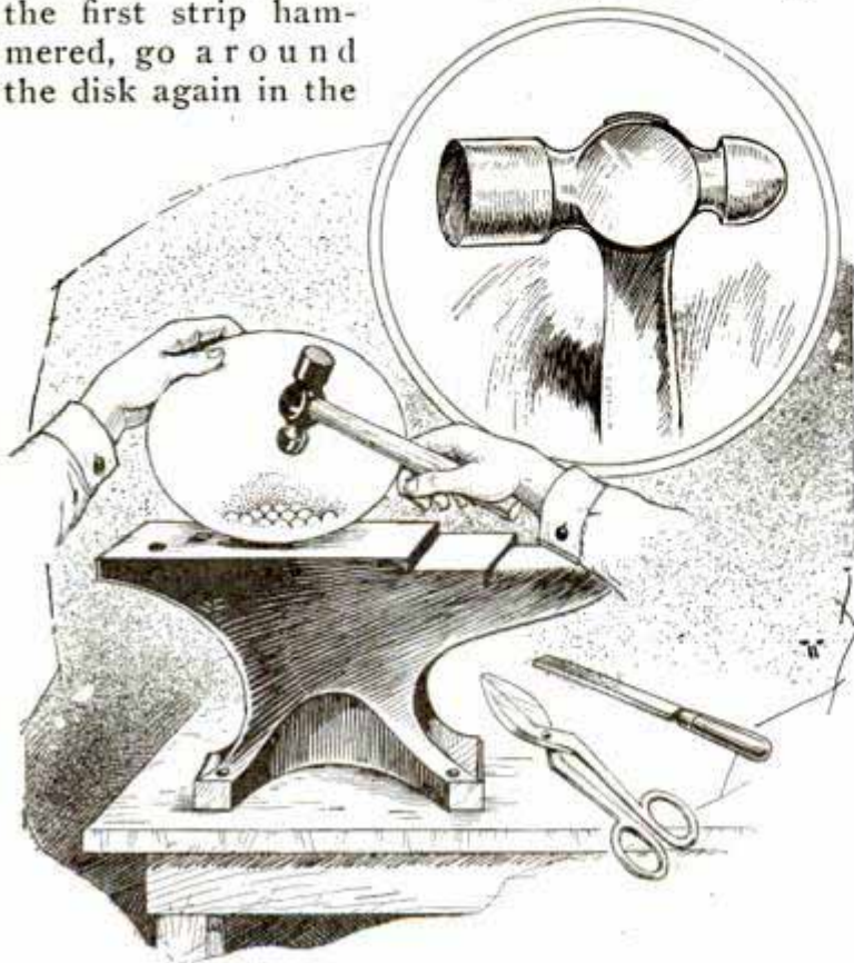
The Type of Hammer Used, and the Method of Starting the Cupping of the Copper Disk
