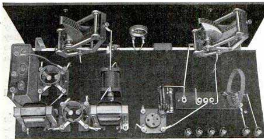
Looking Down on Subpanel: Right, Under-Subpanel View, Showing Ballasts and Method of Wiring
