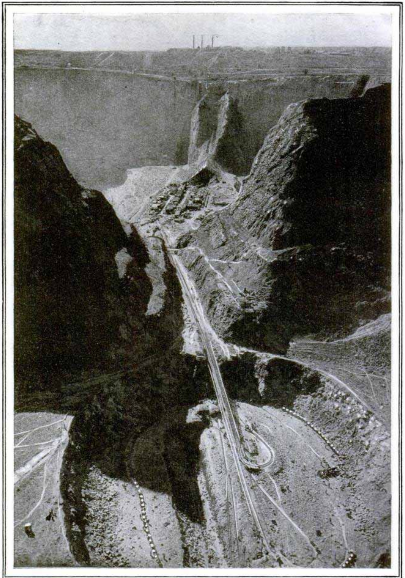
An Endless Trackway Conveys Trains of Little Electric Cars from the Depths of the Diamond Pipe at Premier Mine to the Washing Plant in the Distance—See Page 818
