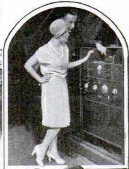
Apparatus Installed in Orchestra Pit, as for Reproducing Voices of a Musical Chorus Number, and Examining Details of the Recorder
