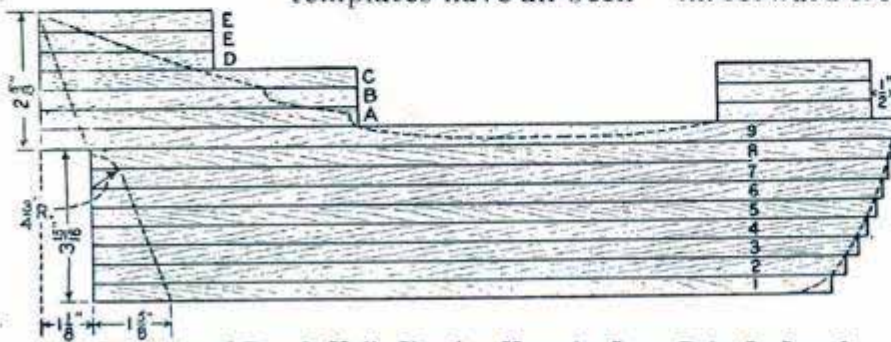
Side Elevation of Rough Hull, Showing How the Stern Rake Is Sawed
