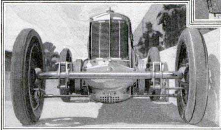
One of the Pigmy Front-Wheel-Drive Racers, Capable of Speeds of More Than One Hundred Miles an Hour; the "Blower" or Supercharger Is Shown at the Lower Right and the Motor Block Above
