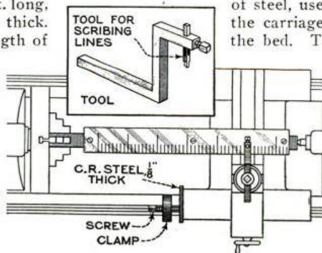
Graduating a 6-ft. Metal Scale in the Lathe for Use as Tailor's Measure
