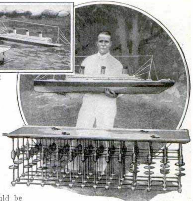
Model Landing Platform, Ship in Pool and View of Anchors on Float
