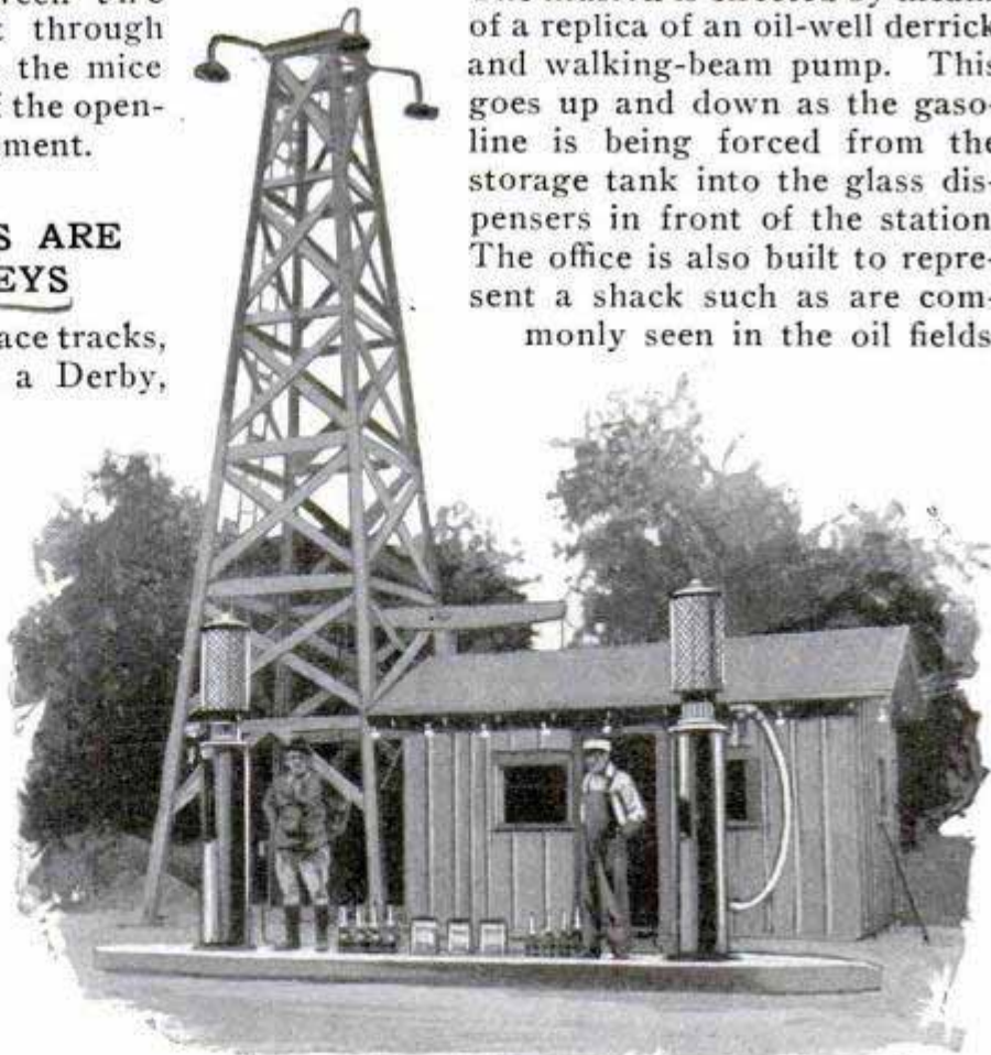
An Innovation in Filling-Station Architecture; the Derrick's Beam Pump Actually Runs When Cars Are Filled
