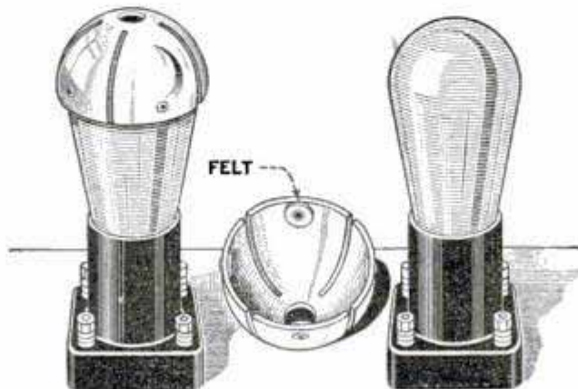
Left, Tube with Cap in Position; Right, Cap Removed, Showing Felt Pads That Separate Metal and Tube
