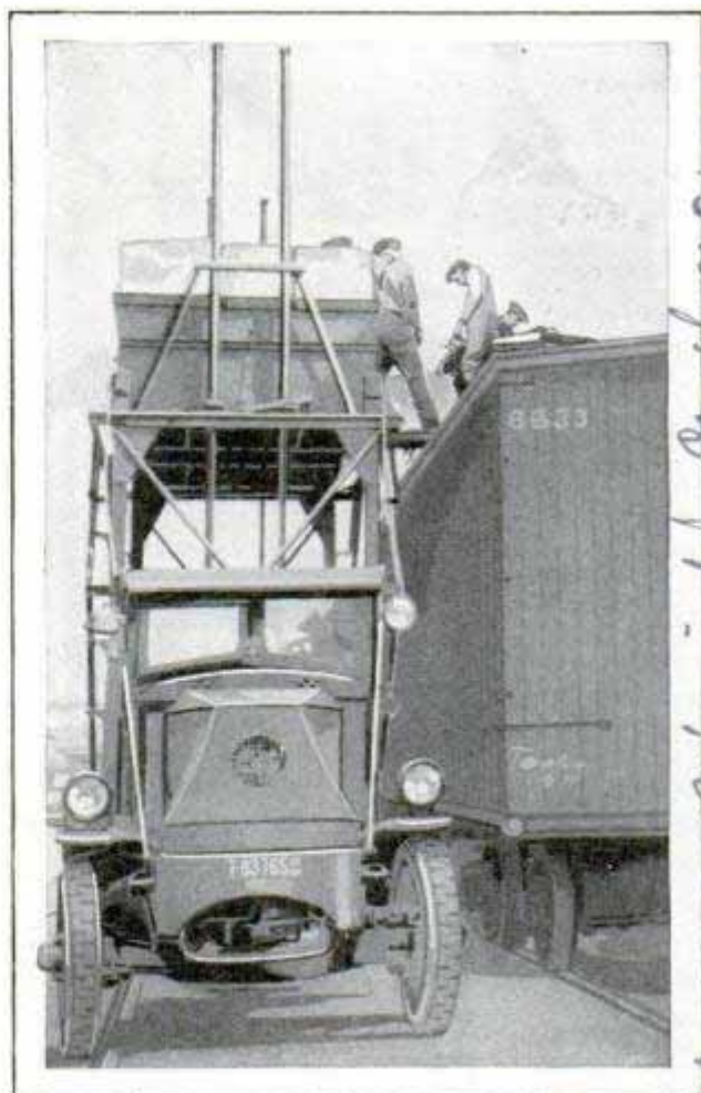
Icing Freight Car from Truck; Cakes Are Hoisted on Elevator Run by the Motor
