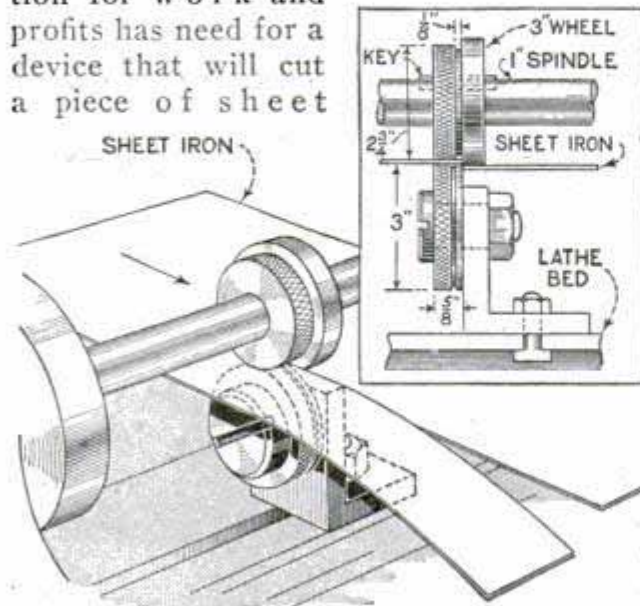
Rotary Shears Run by Lathe or Milling Machine Are Useful for Small Shops
