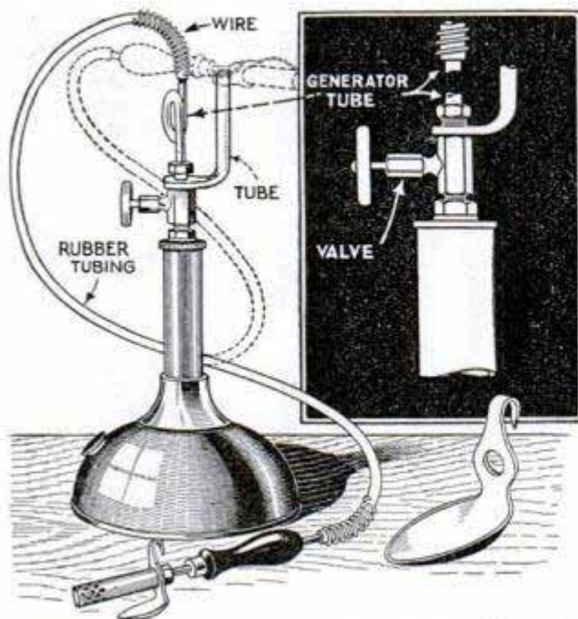
Construction Details and Assembly of the Blowtorch
