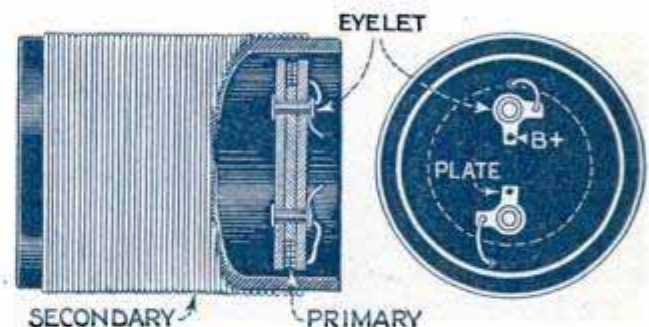
Cut-Away Section Shows Primary Coil in Position; Right, End View with Primary Terminals
