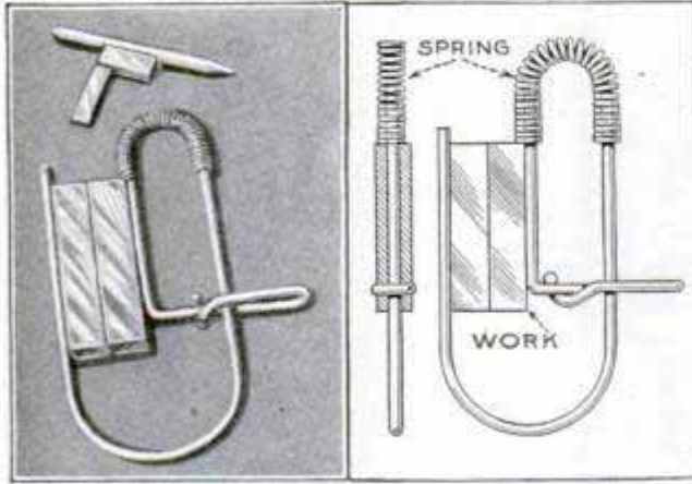
Spring Clamp Facilitates Marking Off Blocks by Handling Two at a Time
