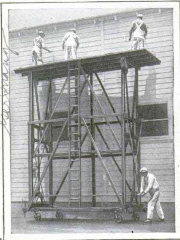
Portable Staging on Painting Job; Workman at Right Is Elevating the Platform with Crank
