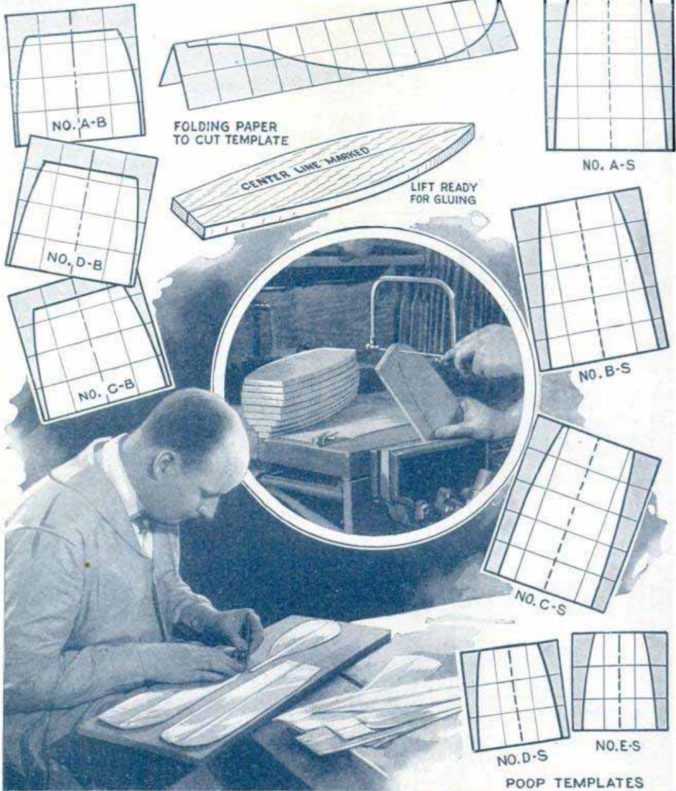
Details of Making and Using Templates, Marking Out Lifts from Templates, and Sawing Them Out
