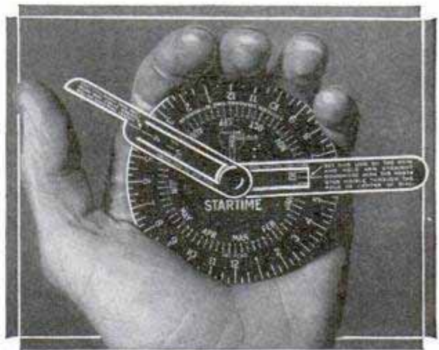
Dial for Telling Time by Stars, Showing Date and Time Arm and the Graduated Center
