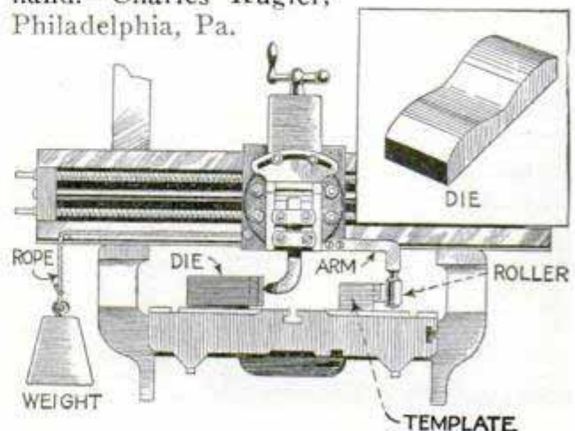
Profile Planing on Large Dies Was Done in Record Time by Using Template
