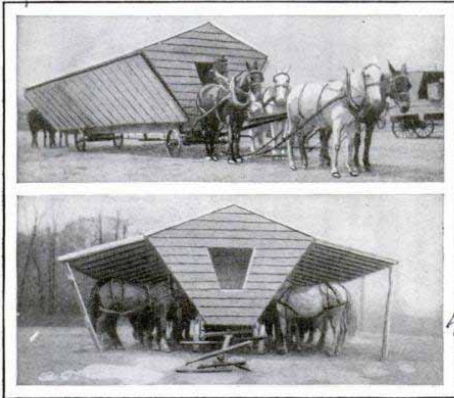
Barn Closed for Travel and Open; Sides Form Protecting Roofs for the Horses, Which Are Fed from Central Mangers
