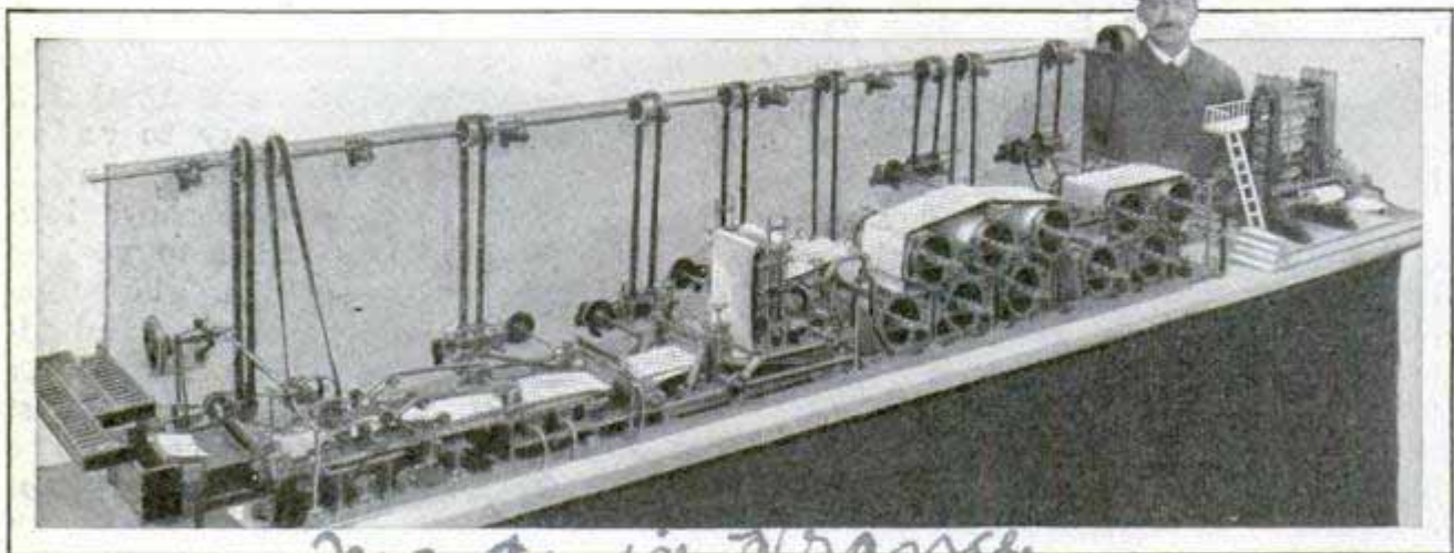
Model Paper Mill in Action; It Duplicates the Larger Units in Practically Every Detail, Making a Strip of Real Paper Four Inches Wide; the Machine Is Less Than Ten Feet Long
