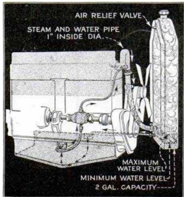
Steam-Cooling System That Gives Greater Efficiency and Reduces Size of Radiators
