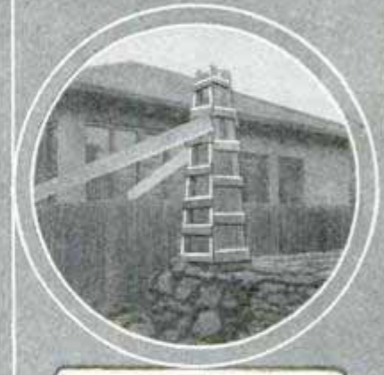
Framework and Bracing for a Rubble Pier
