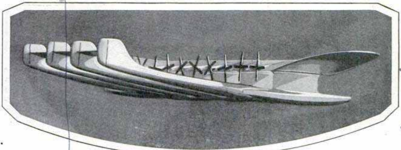
Side View of Model; the Craft Is to Be Constructed along Lines That Will Reduce Wind Resistance to a Minimum and Support Heavy Loads without Bending in Center
